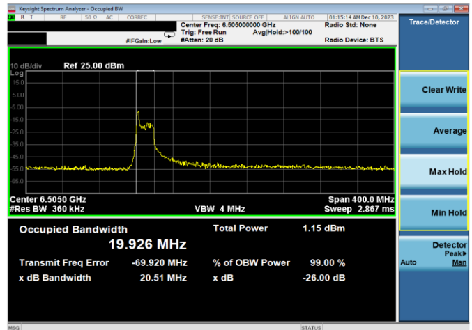
Plot 7-29. 26dB & 99% Bandwidth Plot Antenna WF8 (160MHz 802.11ax RU26 (UNII Band 6) – Ch. 111)
