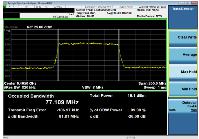
Plot 7-28. 26dB & 99% Bandwidth Plot Antenna WF8 (80MHz 802.11ax RU996 (UNII Band 6) – Ch. 103)
