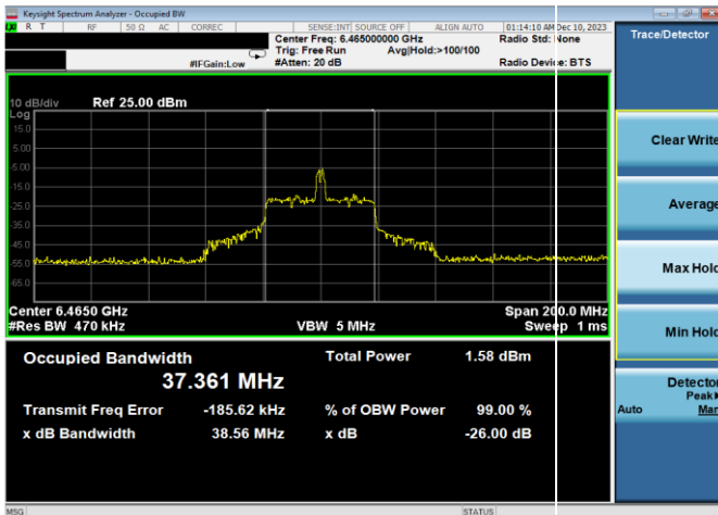
Plot 7-26. 26dB & 99% Bandwidth Plot Antenna WF8 (80MHz 802.11ax RU26 (UNII Band 6) – Ch. 103)
