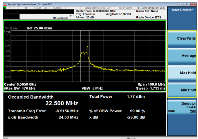
Plot 7-30. 26dB & 99% Bandwidth Plot Antenna WF8 (160MHz 802.11ax RU26 (UNII Band 6) – Ch. 111)
