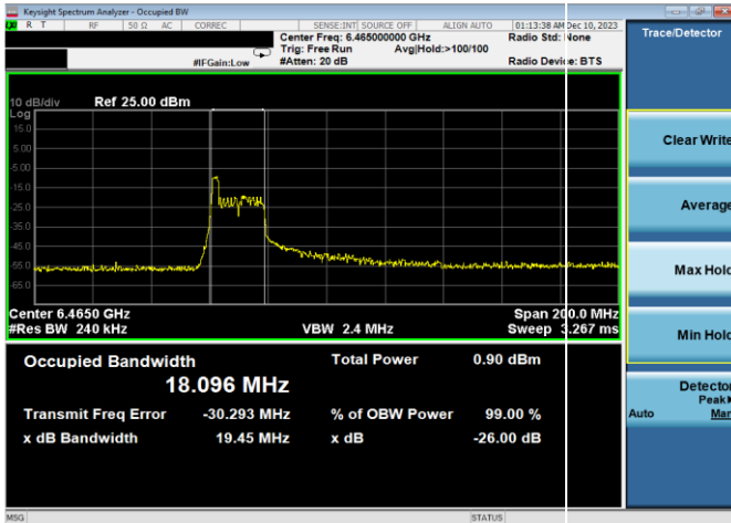
Plot 7-25. 26dB & 99% Bandwidth Plot Antenna WF8 (80MHz 802.11ax RU26 (UNII Band 6) – Ch. 103)
