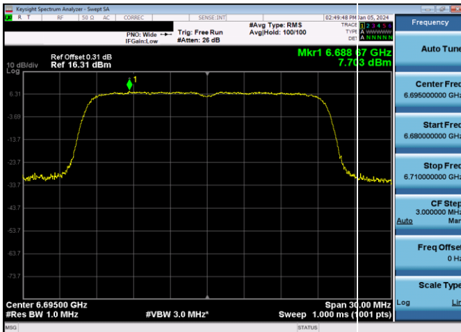
Plot 7-437. Power Spectral Density Plot SDM Antenna WF8 Standard Power (20MHz 802.11ax (UNII Band 7) – Ch. 149, MCS11)
