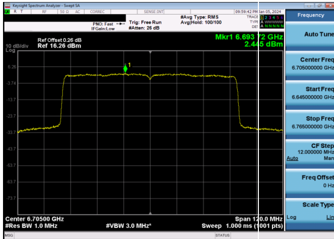
Plot 7-426. Power Spectral Density Plot SDM Antenna WF7a Standard Power (80MHz 802.11ax (UNII Band 7) – Ch. 151, MCS4)
