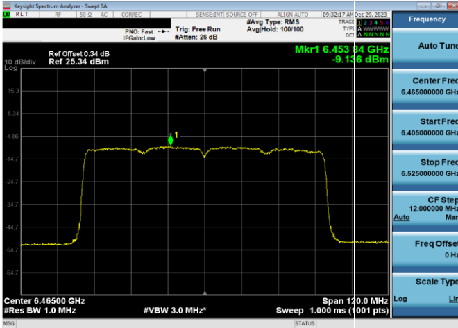
Plot 7-377. Power Spectral Density Plot SDM Antenna WF8 Low Power Indoor (80MHz 802.11ax (UNII Band 6) – Ch. 103, MCS11)
