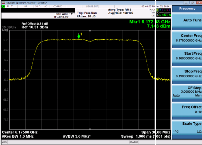
Plot 7-429. Power Spectral Density Plot SDM Antenna WF8 Standard Power (20MHz 802.11ax (UNII Band 5) – Ch. 45, MCS11)
