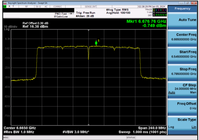
Plot 7-427. Power Spectral Density Plot SDM Antenna WF8 Standard Power (160MHz 802.11ax (UNII Band 7) – Ch. 143, MCS4)
