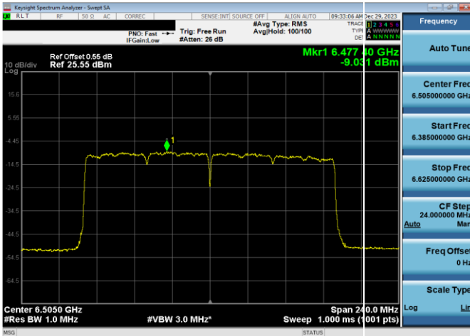
Plot 7-379. Power Spectral Density Plot SDM Antenna WF8 Low Power Indoor (160MHz 802.11ax (UNII Band 6) – Ch. 111, MCS11)
