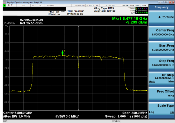
Plot 7-380. Power Spectral Density Plot SDM Antenna WF7a Low Power Indoor (160MHz 802.11ax (UNII Band 6) – Ch. 111, MCS11)
