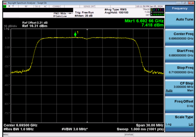
Plot 7-438. Power Spectral Density Plot SDM Antenna WF7a Standard Power (20MHz 802.11ax (UNII Band 7) – Ch. 149, MCS11)
