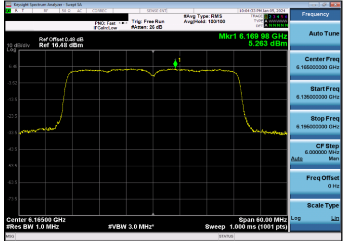
Plot 7-432. Power Spectral Density Plot SDM Antenna WF7a Standard Power (40MHz 802.11ax (UNII Band 5) – Ch. 43, MCS11)
