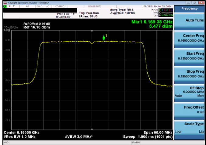
Plot 7-400. Power Spectral Density Plot SDM Antenna WF7a Standard Power (40MHz 802.11ax (UNII Band 5) – Ch. 43, MCS2)
