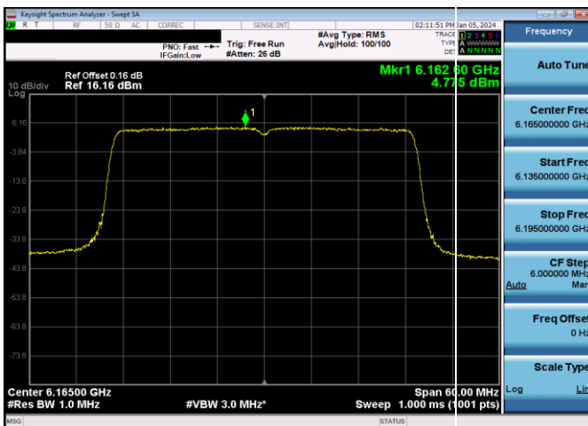
Plot 7-399. Power Spectral Density Plot SDM Antenna WF8 Standard Power (40MHz 802.11ax (UNII Band 5) – Ch. 43, MCS2)
