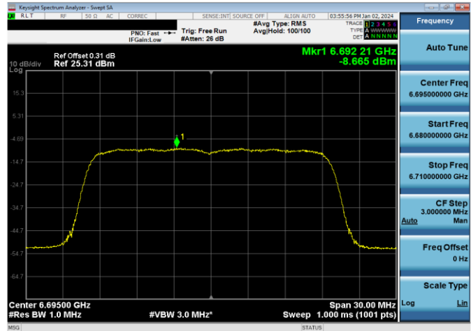
Plot 7-382. Power Spectral Density Plot SDM Antenna WF7a Low Power Indoor (20MHz 802.11ax (UNII Band 7) – Ch. 149, MCS11)
