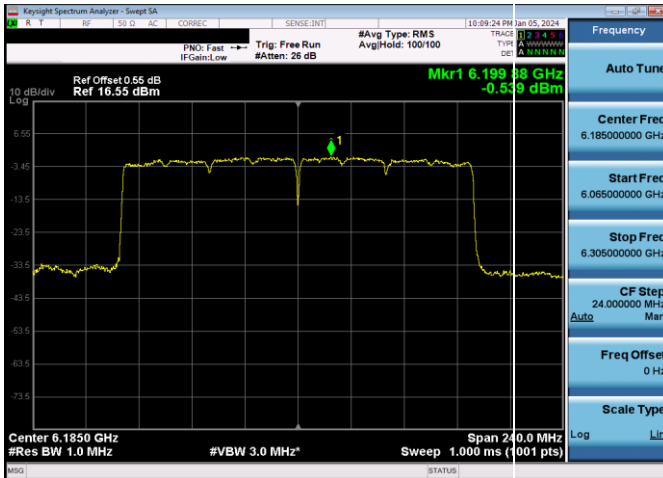
Plot 7-436. Power Spectral Density Plot SDM Antenna WF7a Standard Power (160MHz 802.11ax (UNII Band 5) – Ch. 47, MCS11)
