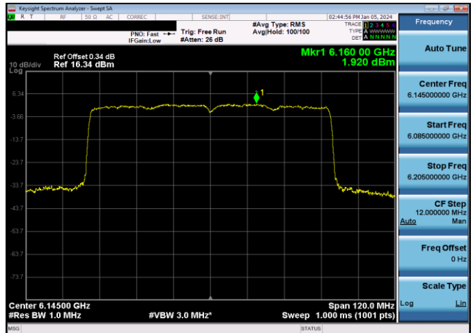
Plot 7-433. Power Spectral Density Plot SDM Antenna WF8 Standard Power (80MHz 802.11ax (UNII Band 5) – Ch. 39, MCS11)
