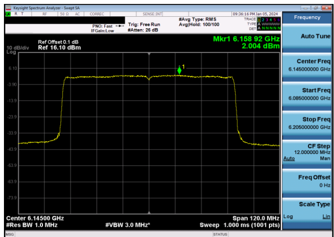
Plot 7-402. Power Spectral Density Plot SDM Antenna WF7a Standard Power (80MHz 802.11ax (UNII Band 5) – Ch. 39, MCS2)
