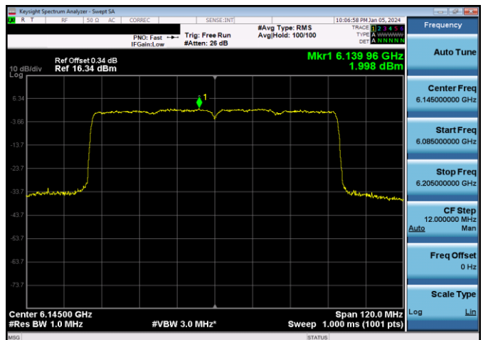
Plot 7-434. Power Spectral Density Plot SDM Antenna WF7a Standard Power (80MHz 802.11ax (UNII Band 5) – Ch. 39, MCS11)
