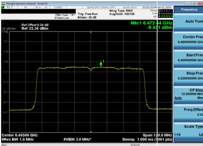
Plot 7-378. Power Spectral Density Plot SDM Antenna WF7a Low Power Indoor (80MHz 802.11ax (UNII Band 6) – Ch. 103, MCS11)
