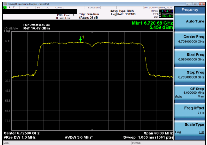
Plot 7-440. Power Spectral Density Plot SDM Antenna WF7a Standard Power (40MHz 802.11ax (UNII Band 7) – Ch. 155, MCS11)
