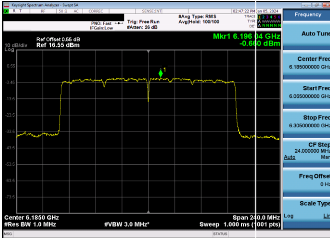
Plot 7-435. Power Spectral Density Plot SDM Antenna WF8 Standard Power (160MHz 802.11ax (UNII Band 5) – Ch. 47, MCS11)
