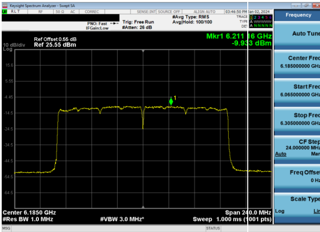
Plot 7-372. Power Spectral Density Plot SDM Antenna WF7a Low Power Indoor (160MHz 802.11ax (UNII Band 5) – Ch. 47, MCS11)
