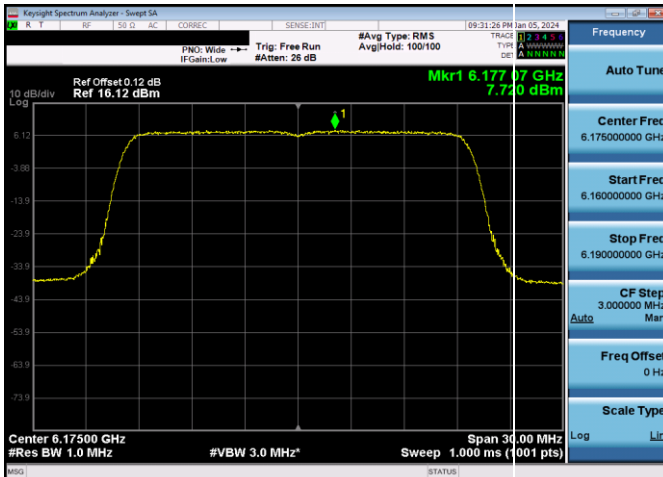
Plot 7-398. Power Spectral Density Plot SDM Antenna WF7a Standard Power (20MHz 802.11ax (UNII Band 5) – Ch. 45, MCS2)
