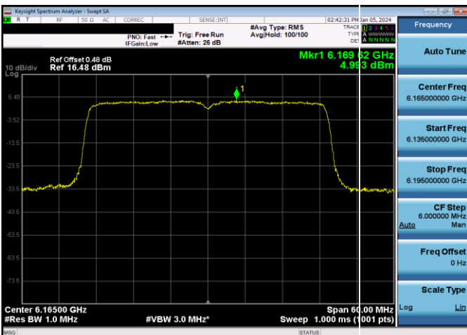
Plot 7-431. Power Spectral Density Plot SDM Antenna WF8 Standard Power (40MHz 802.11ax (UNII Band 5) – Ch. 43, MCS11)
