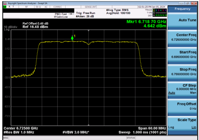
Plot 7-439. Power Spectral Density Plot SDM Antenna WF8 Standard Power (40MHz 802.11ax (UNII Band 7) – Ch. 155, MCS11)
