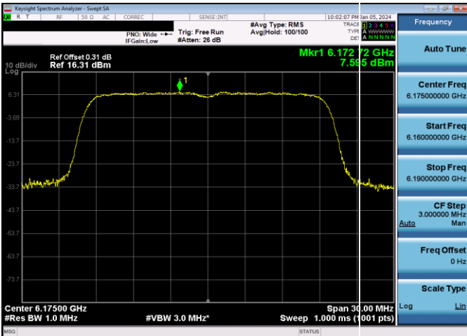
Plot 7-430. Power Spectral Density Plot SDM Antenna WF7a Standard Power (20MHz 802.11ax (UNII Band 5) – Ch. 45, MCS11)
