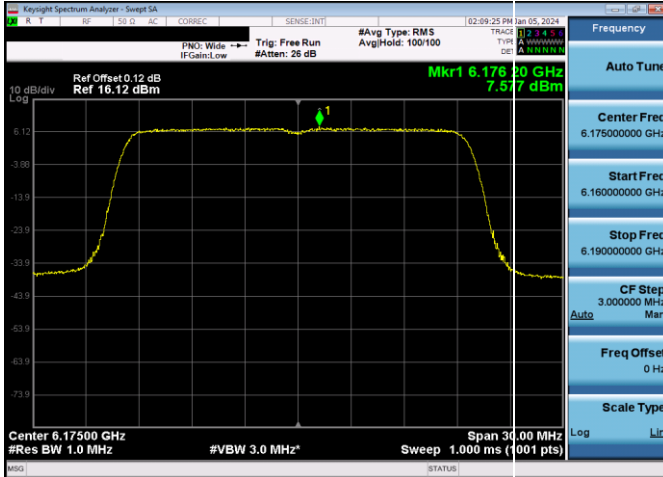
Plot 7-397. Power Spectral Density Plot SDM Antenna WF8 Standard Power (20MHz 802.11ax (UNII Band 5) – Ch. 45, MCS2)
