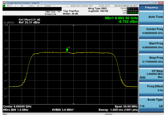
Plot 7-381. Power Spectral Density Plot SDM Antenna WF8 Low Power Indoor (20MHz 802.11ax (UNII Band 7) – Ch. 149, MCS11)
