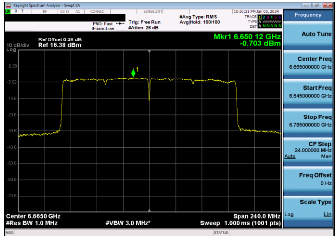
Plot 7-428. Power Spectral Density Plot SDM Antenna WF7a Standard Power (160MHz 802.11ax (UNII Band 7) – Ch. 143, MCS4)
