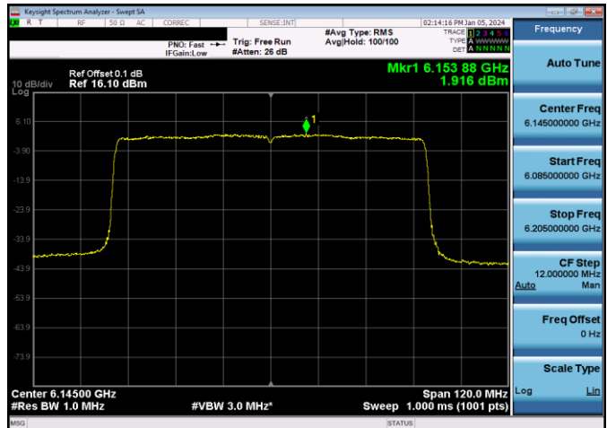
Plot 7-401. Power Spectral Density Plot SDM Antenna WF8 Standard Power (80MHz 802.11ax (UNII Band 5) – Ch. 39, MCS2)
