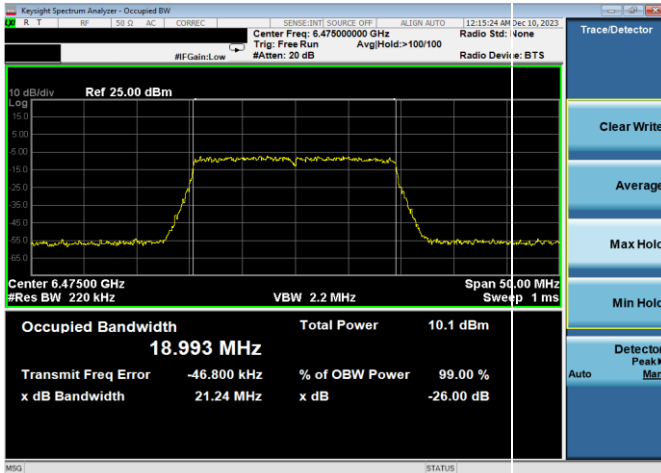
Plot 7-47. 26dB & 99% Bandwidth Plot Antenna WF8 (20MHz 802.11ax (UNII Band 6) – Ch. 105, MCS11)
