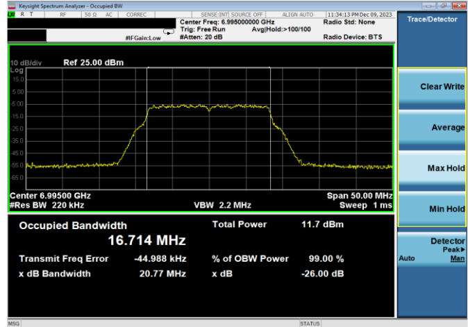
Plot 7-16. 26dB & 99% Bandwidth Plot Antenna WF8 (20MHz 802.11a (UNII Band 8) – Ch. 209, 12Mbps)
