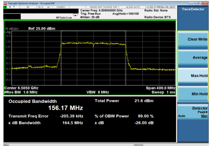
Plot 7-30. 26dB & 99% Bandwidth Plot Antenna WF8 (160MHz 802.11ax (UNII Band 6) – Ch. 111, MCS4)
