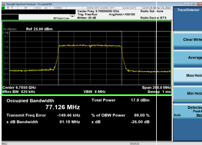
Plot 7-54. 26dB & 99% Bandwidth Plot Antenna WF8 (80MHz 802.11ax (UNII Band 7) – Ch. 151, MCS11)
