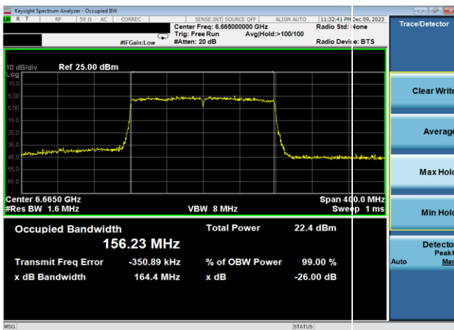
Plot 7-15. 26dB & 99% Bandwidth Plot Antenna WF8 (160MHz 802.11ax (UNII Band 7) – Ch. 143, MCS2)
