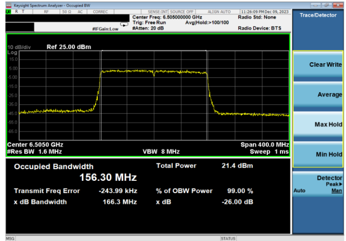
Plot 7-10. 26dB & 99% Bandwidth Plot Antenna WF8 (160MHz 802.11ax (UNII Band 6) – Ch. 111, MCS2)
