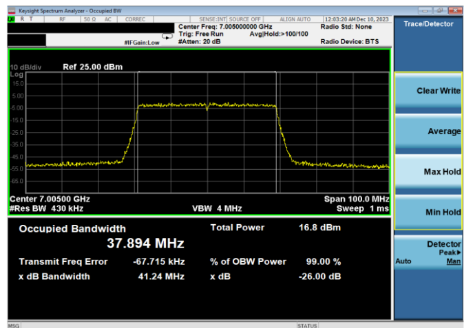
Plot 7-38. 26dB & 99% Bandwidth Plot Antenna WF8 (40MHz 802.11ax (UNII Band 8) – Ch. 211, MCS4)
