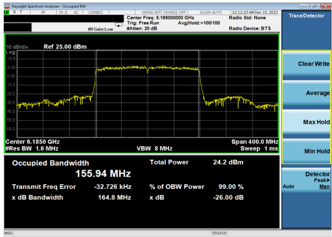
Plot 7-45. 26dB & 99% Bandwidth Plot Antenna WF8 (160MHz 802.11ax (UNII Band 5) – Ch. 47, MCS11)
