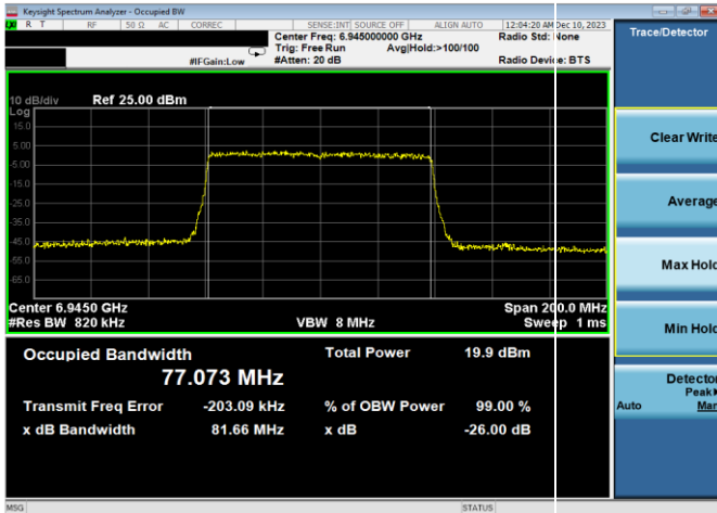
Plot 7-39. 26dB & 99% Bandwidth Plot Antenna WF8 (80MHz) 802.11ax (UNII Band 8) – Ch. 199, MCS4)
