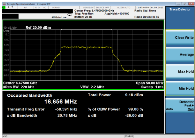
Plot 7-26. 26dB & 99% Bandwidth Plot Antenna WF8 (20MHz 802.11a (UNII Band 6) – Ch. 105, 24Mbps)
