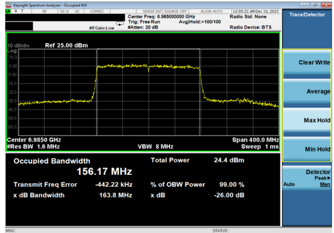
Plot 7-40. 26dB & 99% Bandwidth Plot Antenna WF8 (160MHz) 802.11ax (UNII Band 8) – Ch. 207, MCS4)
