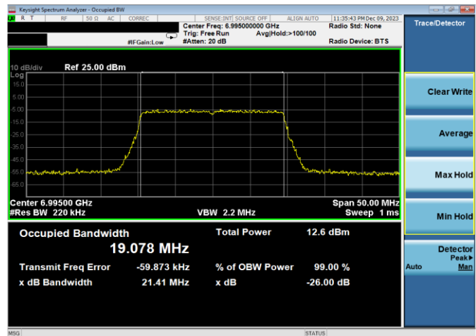
Plot 7-17. 26dB & 99% Bandwidth Plot Antenna WF8 (20MHz 802.11ax (UNII Band 8) – Ch. 209, MCS2)
