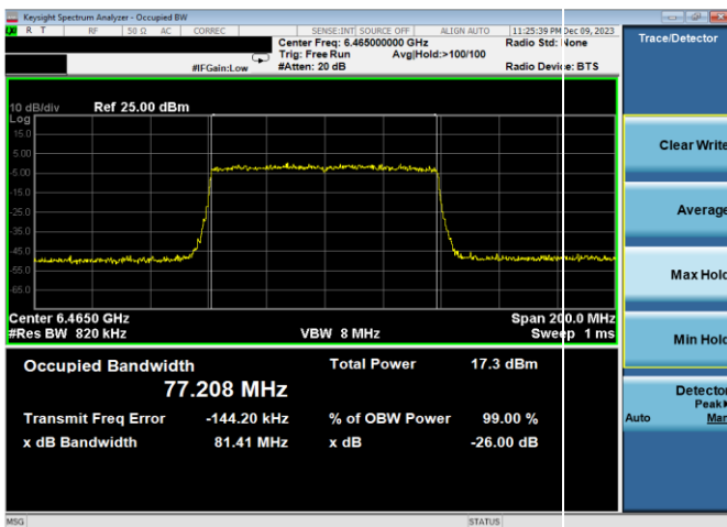
Plot 7-9. 26dB & 99% Bandwidth Plot Antenna WF8 (80MHz 802.11ax (UNII Band 6) – Ch. 103, MCS2)
