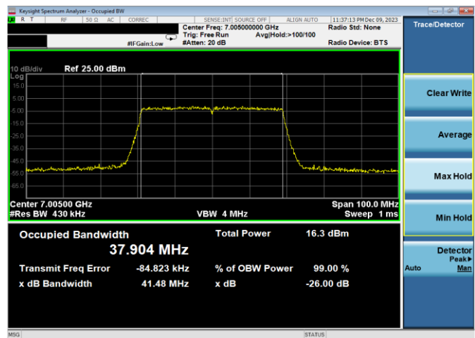
Plot 7-18. 26dB & 99% Bandwidth Plot Antenna WF8 (40MHz 802.11ax (UNII Band 8) – Ch. 211, MCS2)
