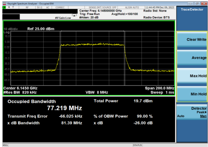
Plot 7-24. 26dB & 99% Bandwidth Plot Antenna WF8 (80MHz 802.11ax (UNII Band 5) – Ch. 39, MCS4)
