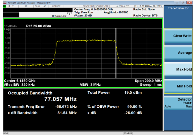
Plot 7-4. 26dB & 99% Bandwidth Plot Antenna WF8 (80MHz 802.11ax (UNII Band 5) – Ch. 39, MCS2)
