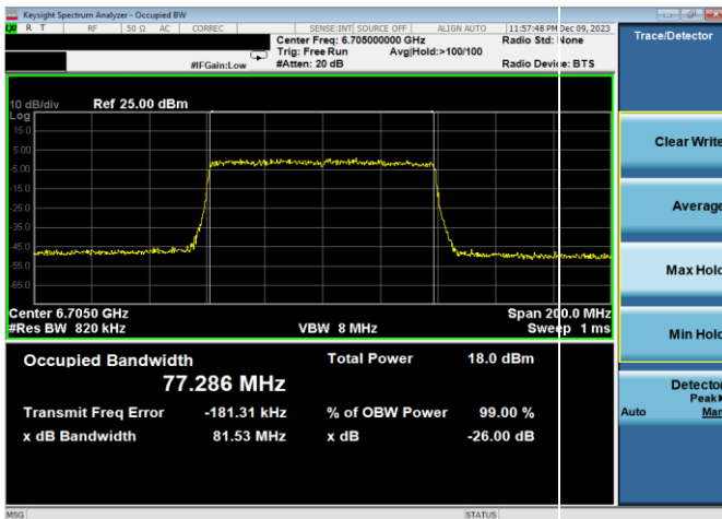
Plot 7-34. 26dB & 99% Bandwidth Plot Antenna WF8 (80MHz 802.11ax (UNII Band 7) – Ch. 151, MCS4)
