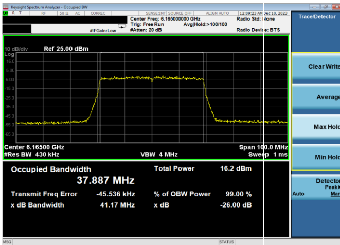
Plot 7-43. 26dB & 99% Bandwidth Plot Antenna WF8 (40MHz 802.11ax (UNII Band 5) – Ch. 43, MCS11)
