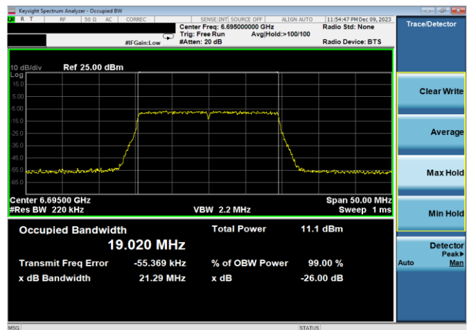
Plot 7-32. 26dB & 99% Bandwidth Plot Antenna WF8 (20MHz 802.11ax (UNII Band 7) – Ch. 149, MCS4)
