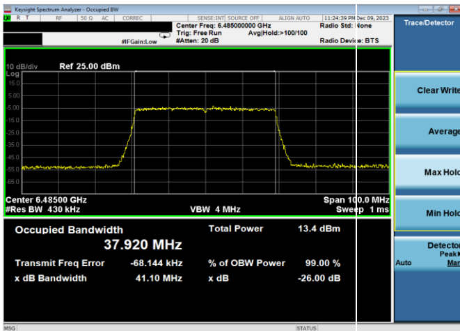
Plot 7-8. 26dB & 99% Bandwidth Plot Antenna WF8 (40MHz 802.11ax (UNII Band 6) – Ch. 107, MCS2)
