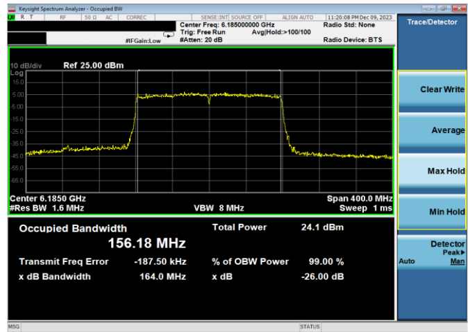
Plot 7-5. 26dB & 99% Bandwidth Plot Antenna WF8 (160MHz 802.11ax (UNII Band 5) – Ch. 47, MCS2)
