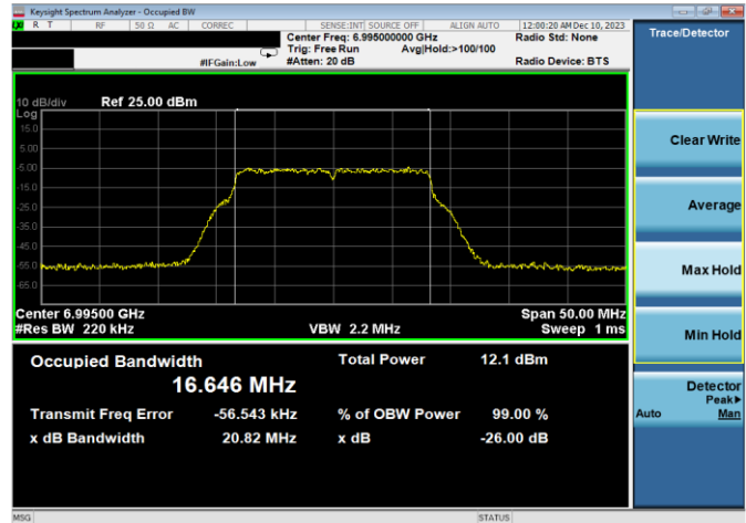
Plot 7-36. 26dB & 99% Bandwidth Plot Antenna WF8 (20MHz 802.11a (UNII Band 8) – Ch. 209, 24Mbps)
