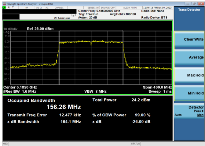
Plot 7-25. 26dB & 99% Bandwidth Plot Antenna WF8 (160MHz 802.11ax (UNII Band 5) – Ch. 47, MCS4)
