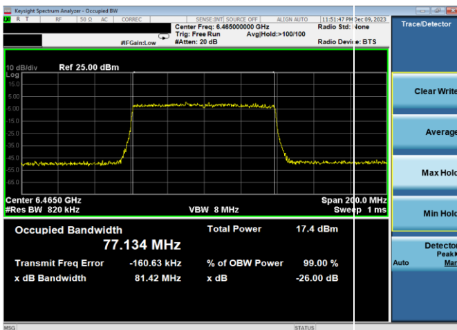
Plot 7-29. 26dB & 99% Bandwidth Plot Antenna WF8 (80MHz 802.11ax (UNII Band 6) – Ch. 103, MCS4)
