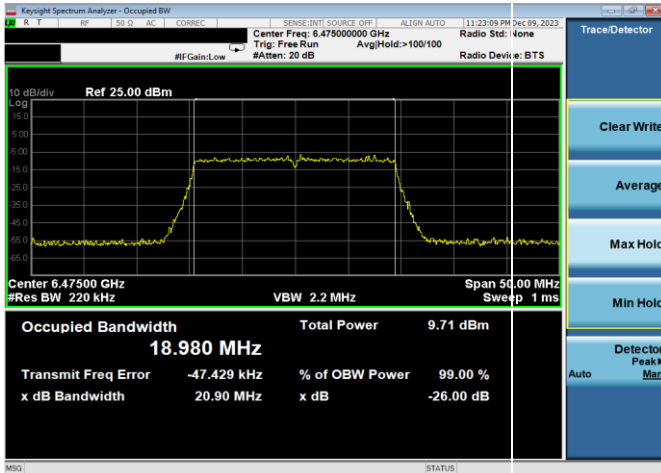
Plot 7-7. 26dB & 99% Bandwidth Plot Antenna WF8 (20MHz 802.11ax (UNII Band 6) – Ch. 105, MCS2)
