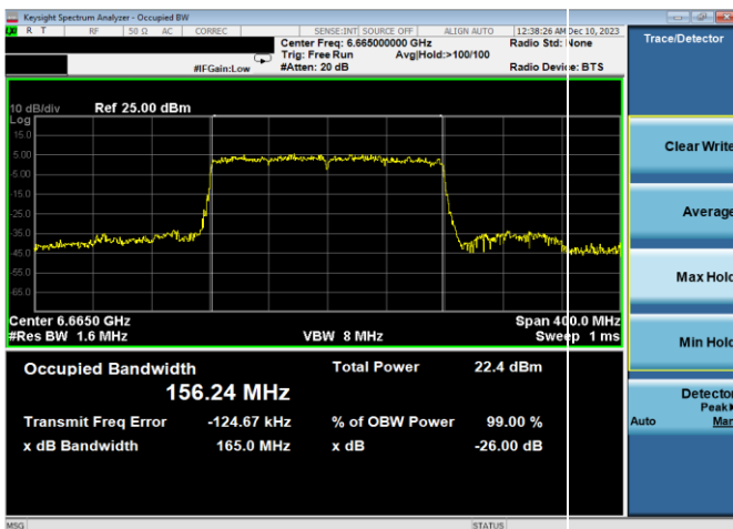
Plot 7-55. 26dB & 99% Bandwidth Plot Antenna WF8 (160MHz 802.11ax (UNII Band 7) – Ch. 143, MCS11)
