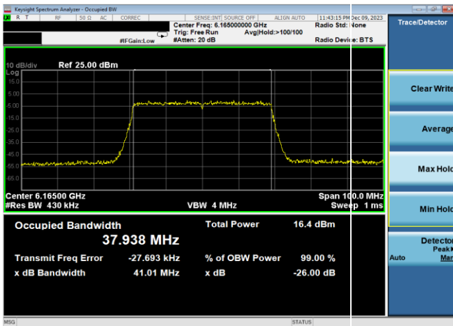
Plot 7-23. 26dB & 99% Bandwidth Plot Antenna WF8 (40MHz 802.11ax (UNII Band 5) – Ch. 43, MCS4)
