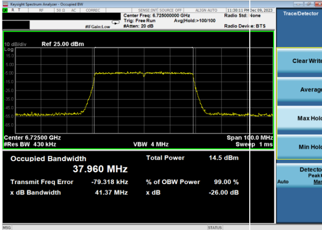
Plot 7-13. 26dB & 99% Bandwidth Plot Antenna WF8 (40MHz 802.11ax (UNII Band 7) – Ch. 155, MCS2)
