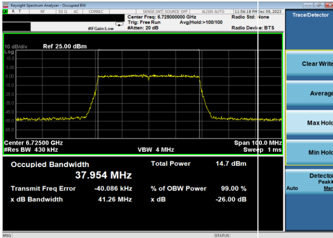
Plot 7-33. 26dB & 99% Bandwidth Plot Antenna WF8 (40MHz 802.11ax (UNII Band 7) – Ch. 155, MCS4)
