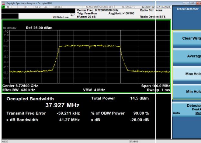
Plot 7-53. 26dB & 99% Bandwidth Plot Antenna WF8 (40MHz 802.11ax (UNII Band 7) – Ch. 155, MCS11)
