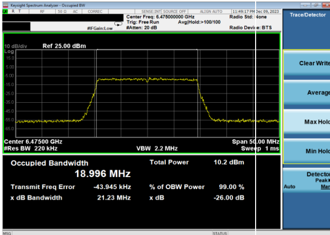
Plot 7-27. 26dB & 99% Bandwidth Plot Antenna WF8 (20MHz 802.11ax (UNII Band 6) – Ch. 105, MCS4)
