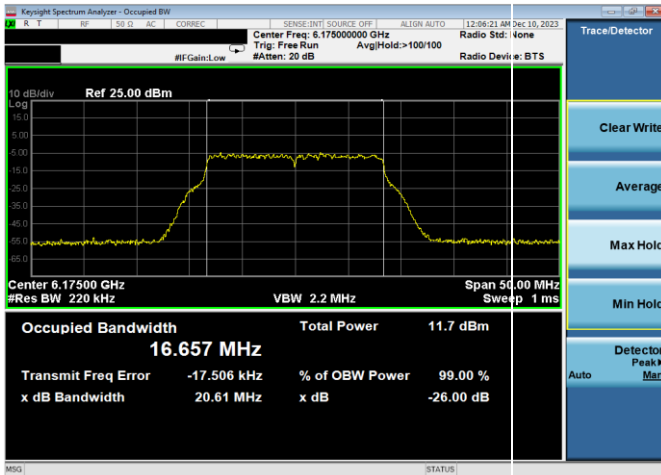
Plot 7-41. 26dB & 99% Bandwidth Plot Antenna WF8 (20MHz 802.11a (UNII Band 5) – Ch. 45, 54Mbps)
