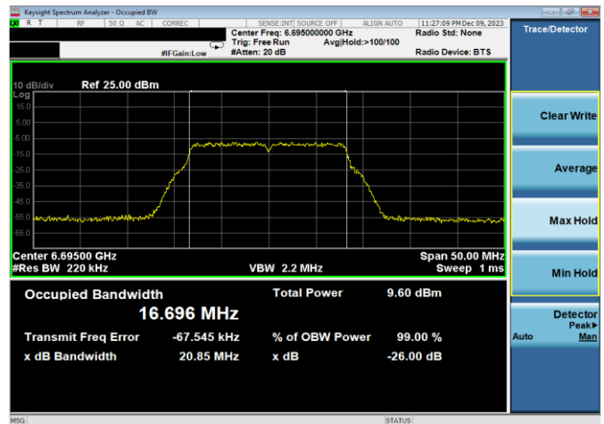
Plot 7-11. 26dB & 99% Bandwidth Plot Antenna WF8 (20MHz 802.11a (UNII Band 7) – Ch. 149, 12Mbps)
