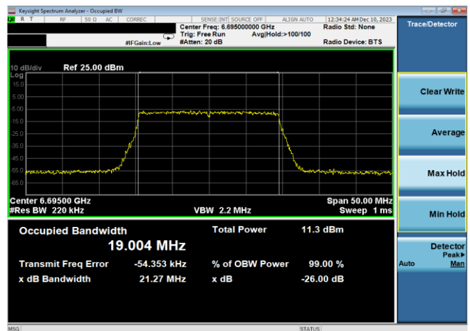
Plot 7-52. 26dB & 99% Bandwidth Plot Antenna WF8 (20MHz 802.11ax (UNII Band 7) – Ch. 149, MCS11)
