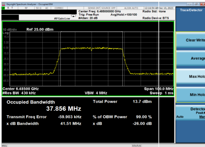
Plot 7-48. 26dB & 99% Bandwidth Plot Antenna WF8 (40MHz 802.11ax (UNII Band 6) – Ch. 107, MCS11)
