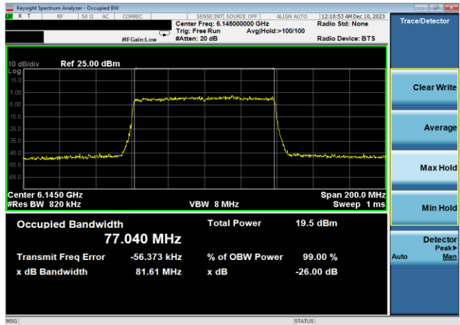
Plot 7-44. 26dB & 99% Bandwidth Plot Antenna WF8 (80MHz 802.11ax (UNII Band 5) – Ch. 39, MCS11)
