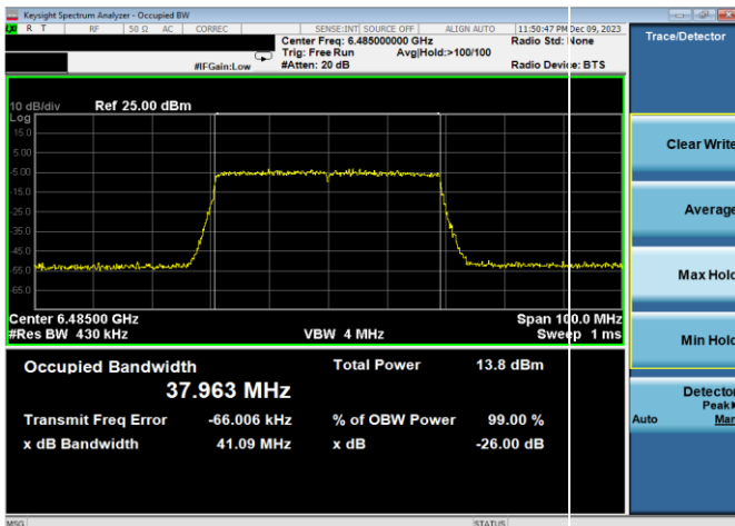
Plot 7-28. 26dB & 99% Bandwidth Plot Antenna WF8 (40MHz 802.11ax (UNII Band 6) – Ch. 107, MCS4)
