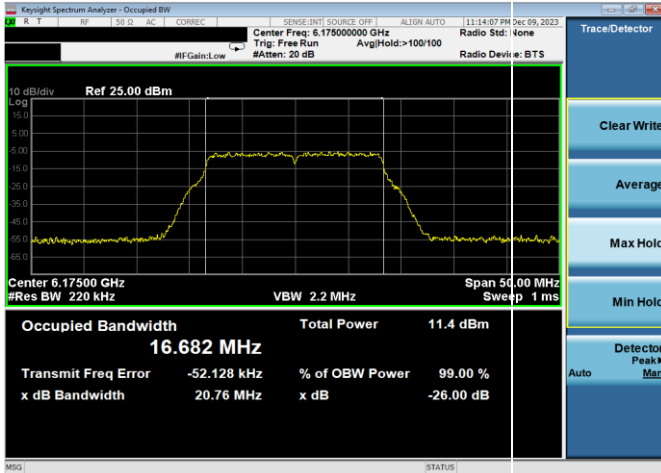
Plot 7-1. 26dB & 99% Bandwidth Plot Antenna WF8 (20MHz 802.11a (UNII Band 5) – Ch. 45, 12Mbps)
