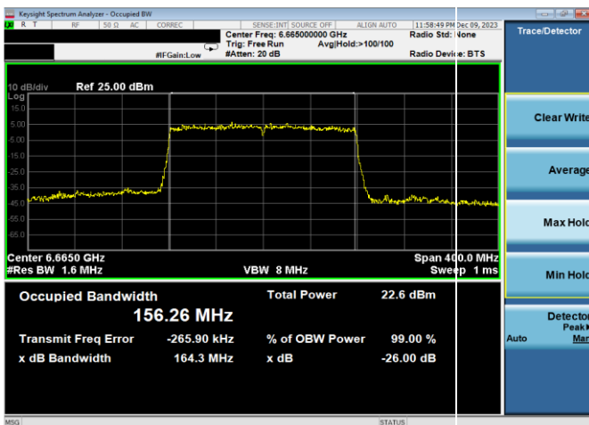
Plot 7-35. 26dB & 99% Bandwidth Plot Antenna WF8 (160MHz 802.11ax (UNII Band 7) – Ch. 143, MCS4)
