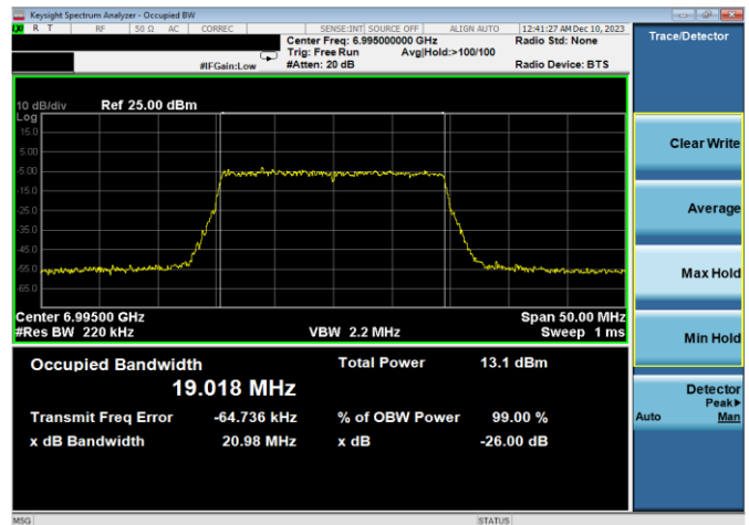
Plot 7-57. 26dB & 99% Bandwidth Plot Antenna WF8 (20MHz 802.11ax (UNII Band 8) – Ch. 209, MCS11)
