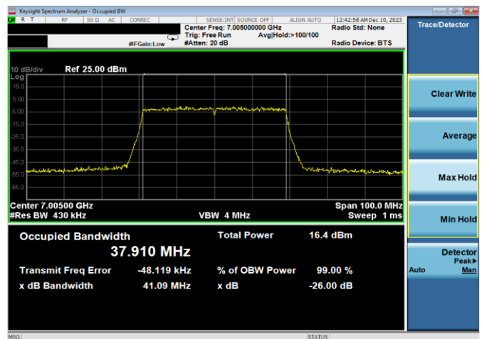
Plot 7-58. 26dB & 99% Bandwidth Plot Antenna WF8 (40MHz 802.11ax (UNII Band 8) – Ch. 211, MCS11)
