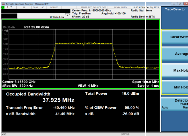
Plot 7-3. 26dB & 99% Bandwidth Plot Antenna WF8 (40MHz 802.11ax (UNII Band 5) – Ch. 43, MCS2)
