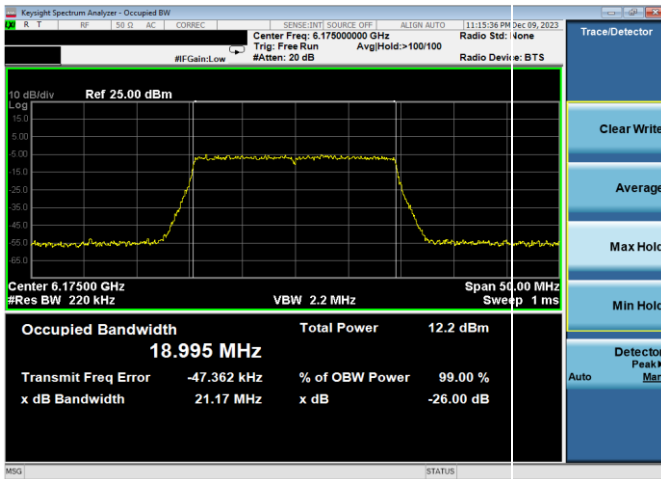
Plot 7-2. 26dB & 99% Bandwidth Plot Antenna WF8 (20MHz 802.11ax (UNII Band 5) – Ch. 45, MCS2)
