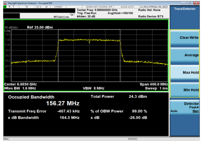
Plot 7-20. 26dB & 99% Bandwidth Plot Antenna WF8 (160MHz 802.11ax (UNII Band 8) – Ch. 207, MCS2)
