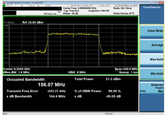
Plot 7-50. 26dB & 99% Bandwidth Plot Antenna WF8 (160MHz 802.11ax (UNII Band 6) – Ch. 111, MCS11)
