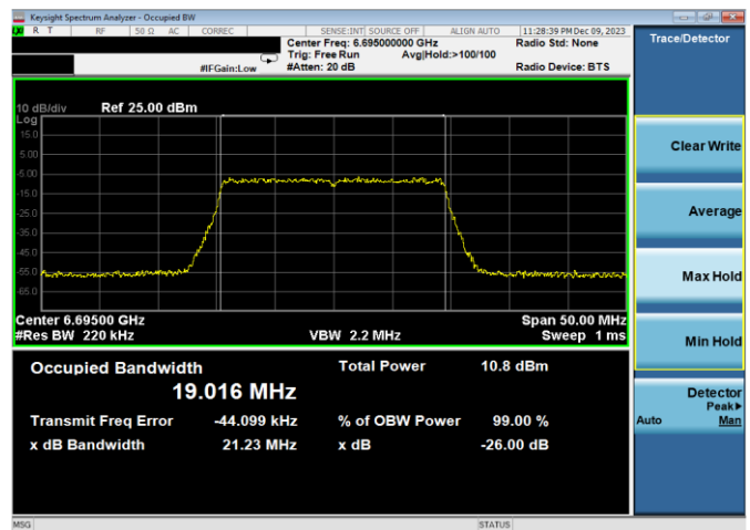
Plot 7-12. 26dB & 99% Bandwidth Plot Antenna WF8 (20MHz 802.11ax (UNII Band 7) – Ch. 149, MCS2)
