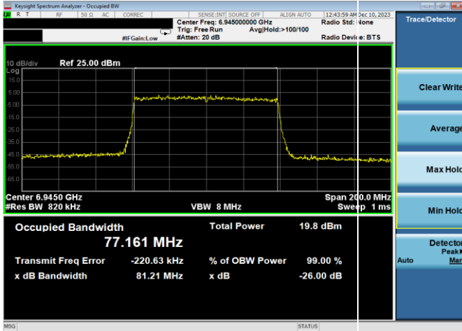
Plot 7-59. 26dB & 99% Bandwidth Plot Antenna WF8 (80MHz 802.11ax (UNII Band 8) – Ch. 199, MCS11)
