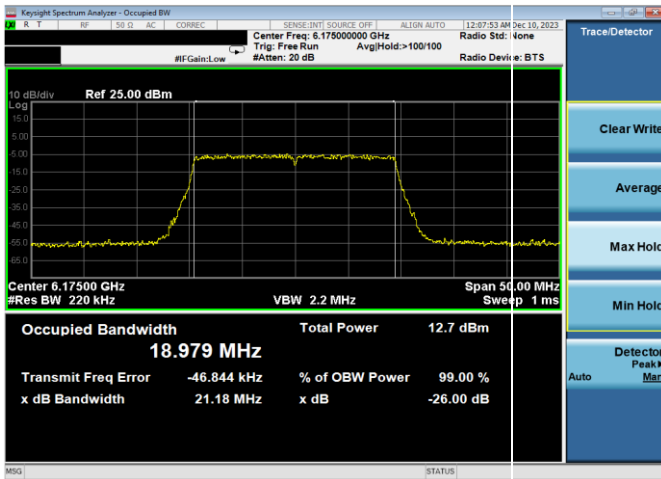
Plot 7-42. 26dB & 99% Bandwidth Plot Antenna WF8 (20MHz 802.11ax (UNII Band 5) – Ch. 45, MCS11)
