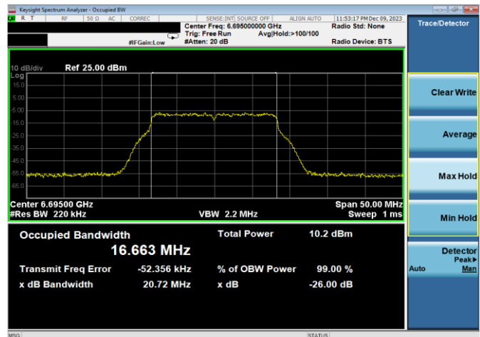
Plot 7-31. 26dB & 99% Bandwidth Plot Antenna WF8 (20MHz 802.11a (UNII Band 7) – Ch. 149, 24Mbps)
