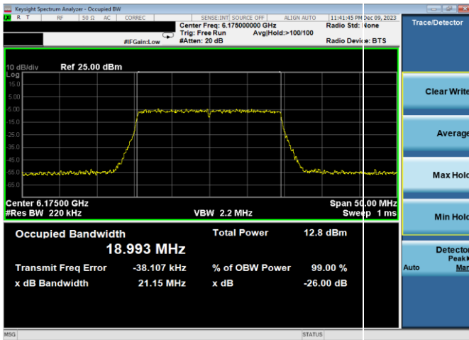
Plot 7-22. 26dB & 99% Bandwidth Plot Antenna WF8 (20MHz 802.11ax (UNII Band 5) – Ch. 45, MCS4)
