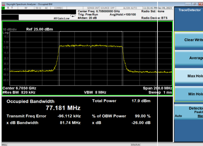
Plot 7-14. 26dB & 99% Bandwidth Plot Antenna WF8 (80MHz 802.11ax (UNII Band 7) – Ch. 151, MCS2)
