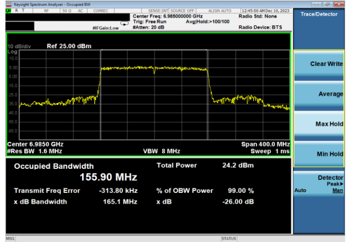
Plot 7-60. 26dB & 99% Bandwidth Plot Antenna WF8 (160MHz 802.11ax (UNII Band 8) – Ch. 207, MCS11)
