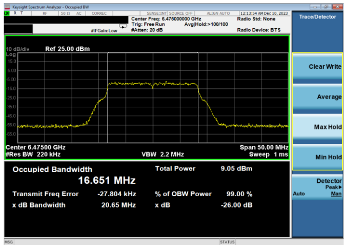
Plot 7-46. 26dB & 99% Bandwidth Plot Antenna WF8 (20MHz 802.11a (UNII Band 6) – Ch. 105, 54Mbps)
