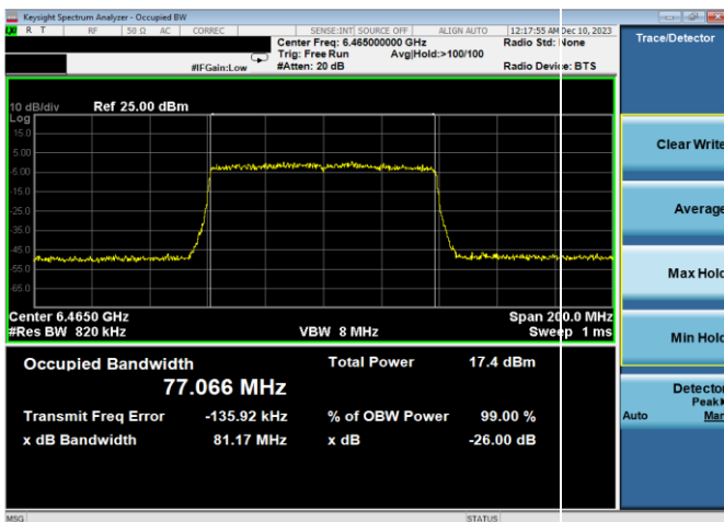
Plot 7-49. 26dB & 99% Bandwidth Plot Antenna WF8 (80MHz 802.11ax (UNII Band 6) – Ch. 103, MCS11)
