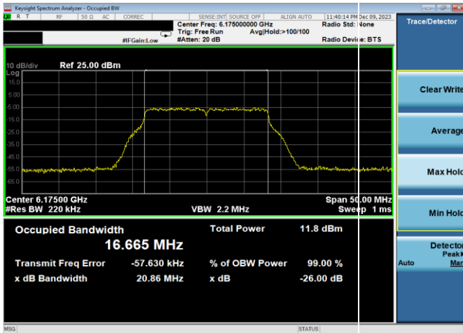
Plot 7-21. 26dB & 99% Bandwidth Plot Antenna WF8 (20MHz 802.11a (UNII Band 5) – Ch. 45, 24Mbps)
