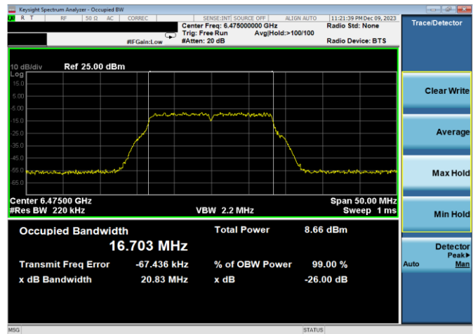
Plot 7-6. 26dB & 99% Bandwidth Plot Antenna WF8 (20MHz 802.11a (UNII Band 6) – Ch. 105, 12Mbps)
