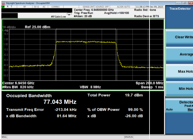
Plot 7-19. 26dB & 99% Bandwidth Plot Antenna WF8 (80MHz 802.11ax (UNII Band 8) – Ch. 199, MCS2)
