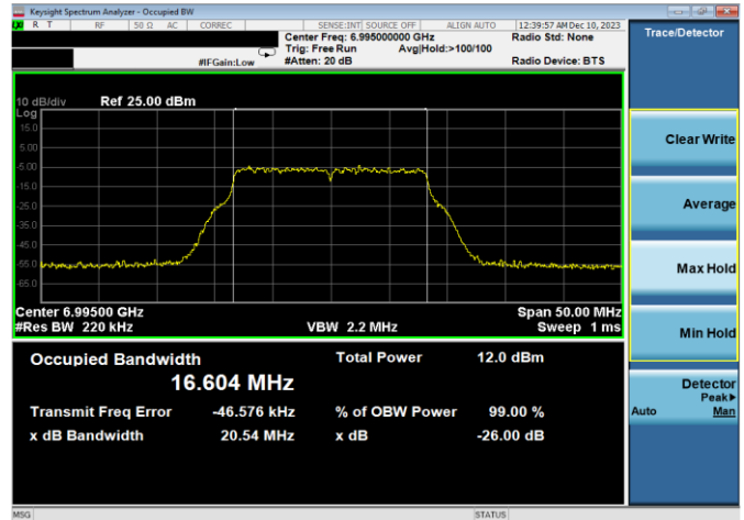
Plot 7-56. 26dB & 99% Bandwidth Plot Antenna WF8 (20MHz 802.11a (UNII Band 8) – Ch. 209, 54Mbps)
