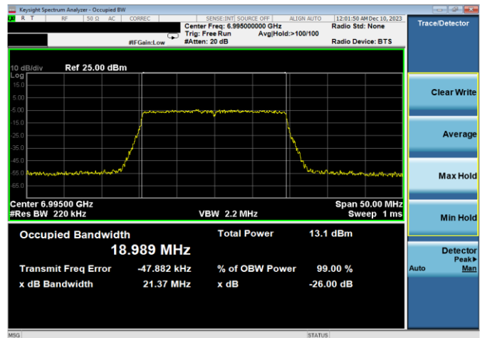
Plot 7-37. 26dB & 99% Bandwidth Plot Antenna WF8 (20MHz 802.11ax (UNII Band 8) – Ch. 209, MCS4)
