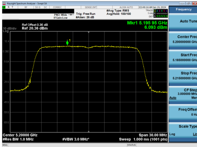
Plot 7-262. PSD CDD Antenna WF7a (20MHz BW 11ax - RU242 - Ch.40)
