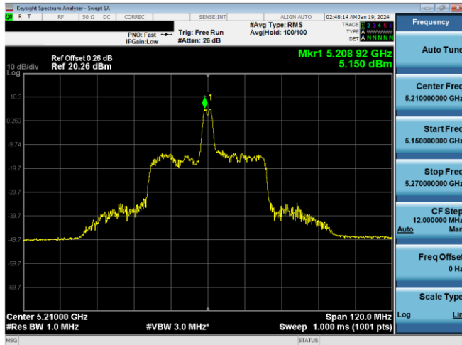
Plot 7-274. PSD CDD Antenna WF7a (80MHz BW 11ax Index 18 – RU26 – Ch.42)
