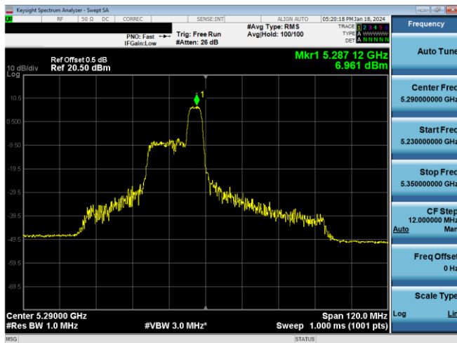
Plot 7-305. PSD CDD Antenna WF8 (80MHz BW 11ax Index 44 – RU52 – Ch.58)
