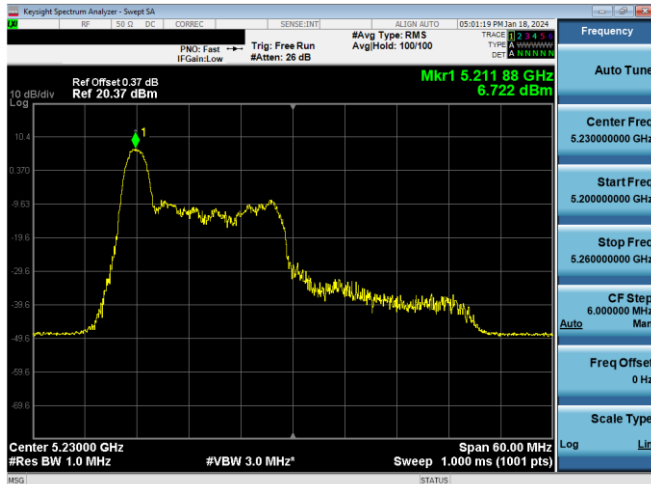
Plot 7-263. PSD CDD Antenna WF8 (40MHz BW 11ax Index 0 - RU26 - Ch.46)
