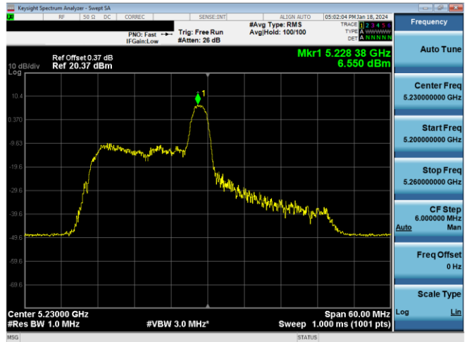
Plot 7-265. PSD CDD Antenna WF8 (40MHz BW 11ax Index 8 - RU26 - Ch.46)
