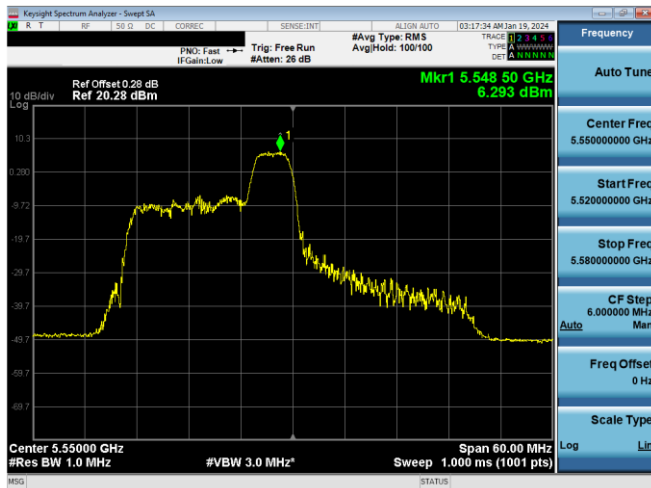
Plot 7-322. PSD SDM Antenna WF7a (40MHz BW 11ax Index 40 - RU52 - Ch.110)
