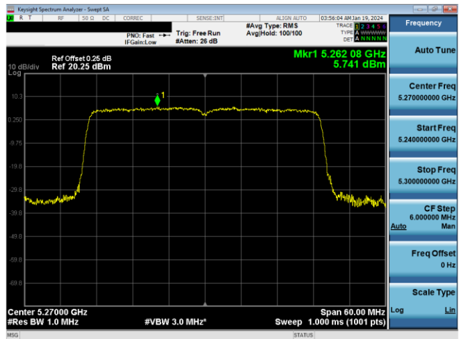
Plot 7-302. PSD CDD Antenna WF7a (40MHz BW 11ax - RU484 - Ch.54)
