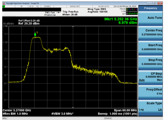
Plot 7-295. PSD CDD Antenna WF8 (40MHz BW 11ax Index 37 – RU52 – Ch.54)
