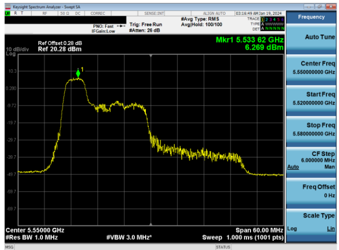
Plot 7-320. PSD SDM Antenna WF7a (40MHz BW 11ax Index 37 - RU52 - Ch.110)
