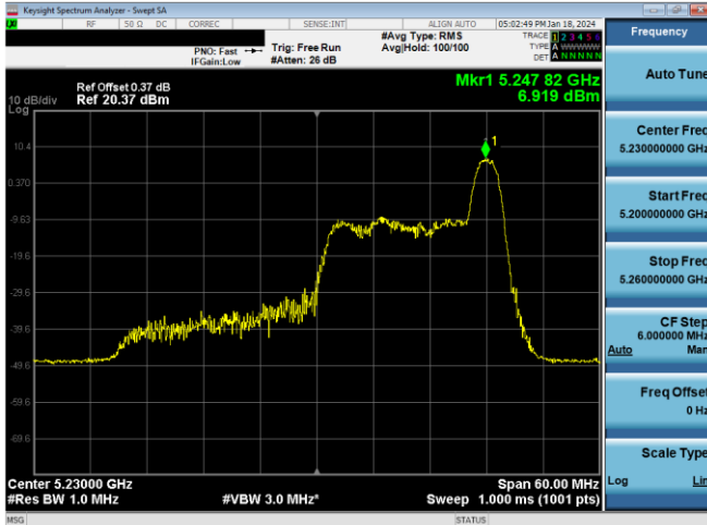
Plot 7-267. PSD CDD Antenna WF8 (40MHz BW 11ax Index 17 - RU26 - Ch.46)
