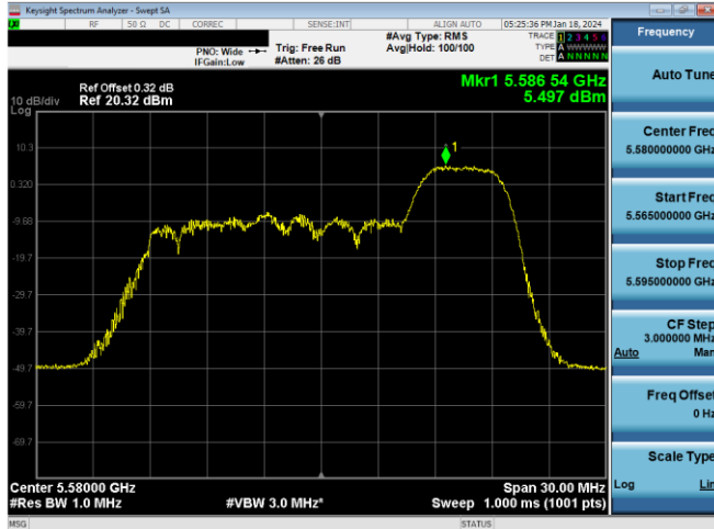
Plot 7-315. PSD SDM Antenna WF8 (20MHz BW 11ax Index 40 - RU52 - Ch.116)
