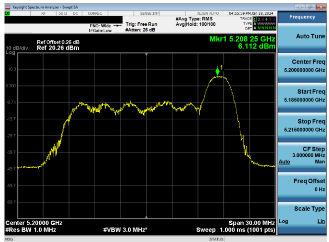
Plot 7-259. PSD CDD Antenna WF8 (20MHz BW 11ax Index 8 – RU26 – Ch.40)
