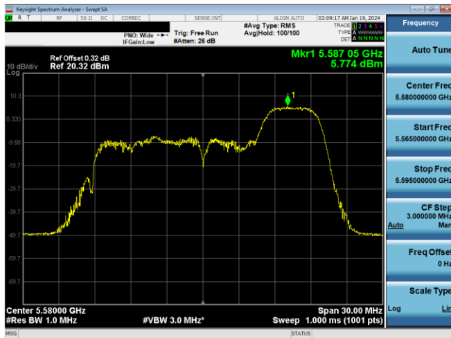
Plot 7-316. PSD SDM Antenna WF7a (20MHz BW 11ax Index 40 - RU52 - Ch.116)
