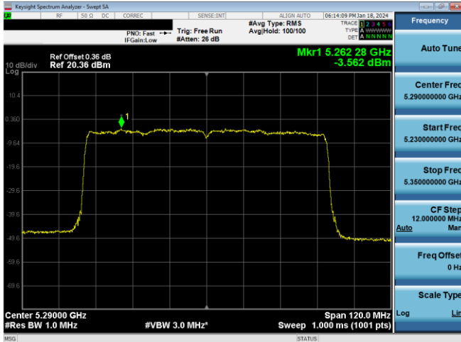
Plot 7-309. PSD CDD Antenna WF8 (80MHz BW 11ax - RU996 - Ch.58)
