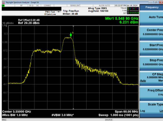
Plot 7-321. PSD SDM Antenna WF8 (40MHz BW 11ax Index 40 - RU52 - Ch.110)
