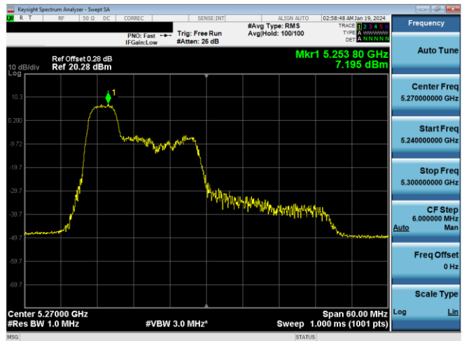
Plot 7-296. PSD CDD Antenna WF7a (40MHz BW 11ax Index 37 – RU52 – Ch.54)
