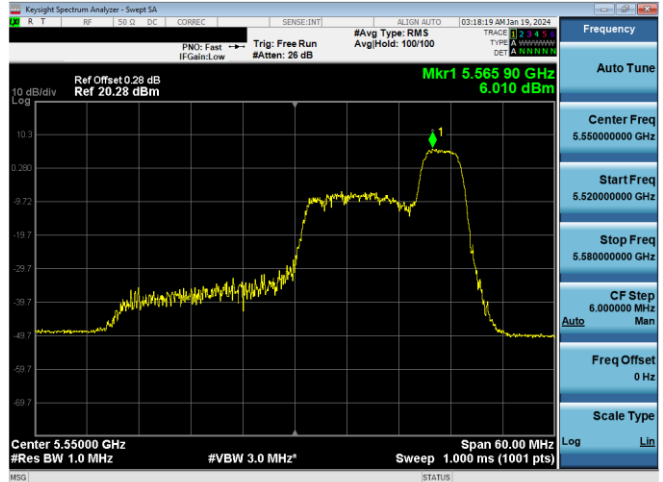
Plot 7-324. PSD SDM Antenna WF7a (40MHz BW 11ax Index 44 - RU52 - Ch.110)
