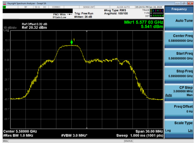
Plot 7-313. PSD SDM Antenna WF8 (20MHz BW 11ax Index 38 - RU52 - Ch.116)
