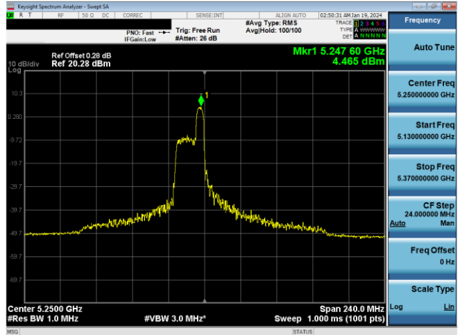
Plot 7-282. PSD CDD Antenna WF7a (160MHz BW 11ax Index 52 - RU52 - Ch.50 (L))
