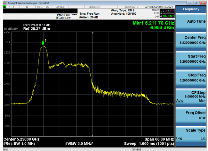
Plot 7-264. PSD CDD Antenna WF7a (40MHz BW 11ax Index 0 - RU26 - Ch.46)
