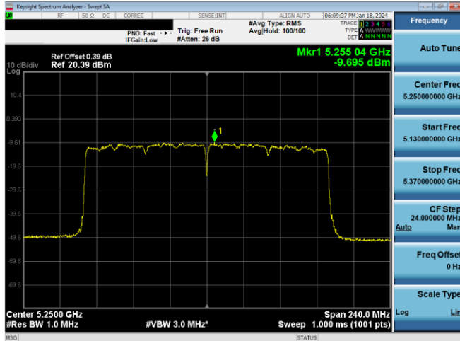
Plot 7-285. PSD CDD Antenna WF8 (160MHz BW 11ax - RU996x2 - Ch.50)
