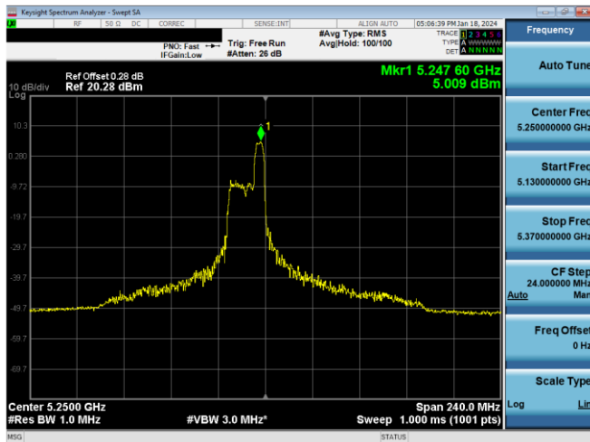
Plot 7-281. PSD CDD Antenna WF8 (160MHz BW 11ax Index 52 - RU52 - Ch.50 (L))
