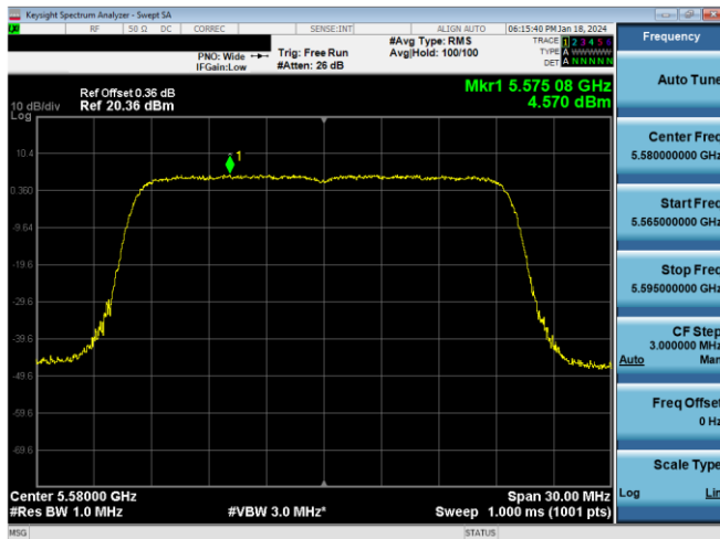
Plot 7-317. PSD SDM Antenna WF8 (20MHz BW 11ax- RU242 - Ch.116)
