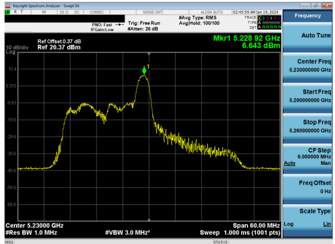
Plot 7-266. PSD CDD Antenna WF7a (40MHz BW 11ax Index 8 - RU26 - Ch.46)
