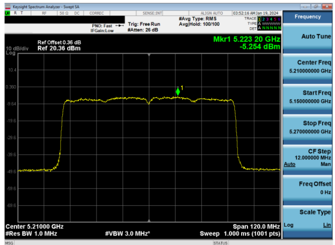
Plot 7-278. PSD CDD Antenna WF7a (80MHz BW 11ax – RU996 – Ch.42)
