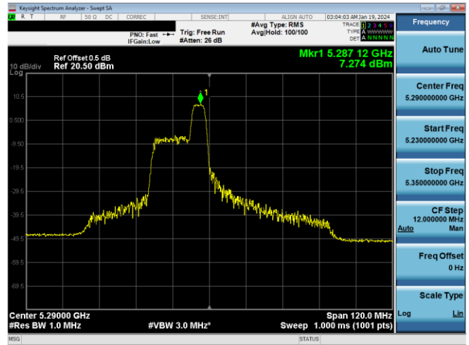
Plot 7-306. PSD CDD Antenna WF7a (80MHz BW 11ax Index 44 – RU52 – Ch.58)
