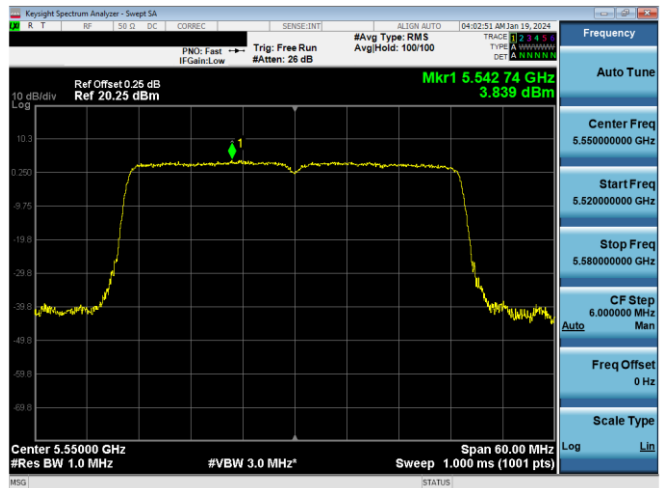
Plot 7-326. PSD CDD Antenna WF7a (40MHz BW 11ax - RU484 - Ch.110)
