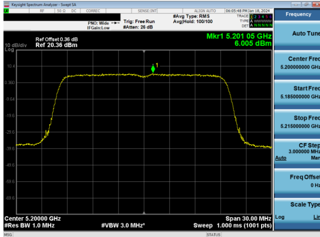
Plot 7-261. PSD CDD Antenna WF8 (20MHz BW 11ax - RU242 - Ch.40)
