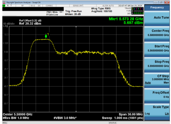
Plot 7-312. PSD SDM Antenna WF7a (20MHz BW 11ax Index 37 - RU52 - Ch.116)
