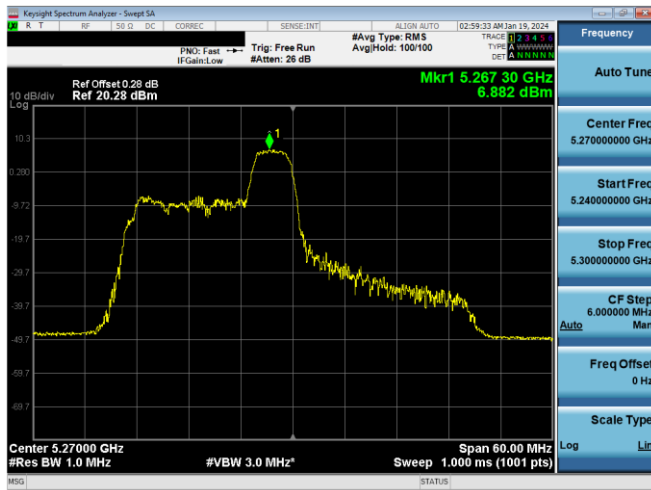
Plot 7-298. PSD CDD Antenna WF7a (40MHz BW 11ax Index 40 - RU52 - Ch.54)
