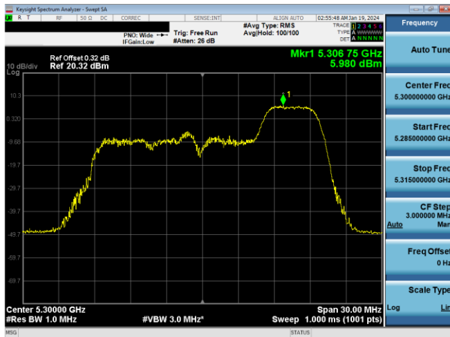
Plot 7-292. PSD CDD Antenna WF7a (20MHz BW 11ax Index 40 – RU52 – Ch.60)
