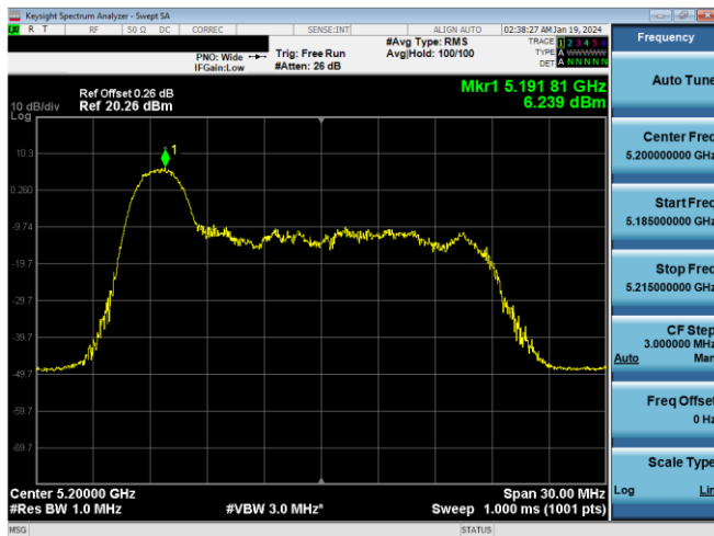
Plot 7-256. PSD CDD Antenna WF7a (20MHz BW 11ax Index 0 – RU26 – Ch.40)
