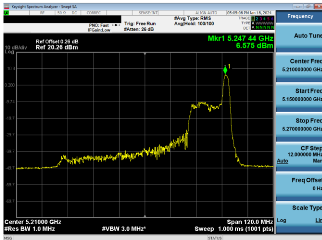
Plot 7-275. PSD CDD Antenna WF8 (80MHz BW 11ax Index 36 – RU26 – Ch.42)
