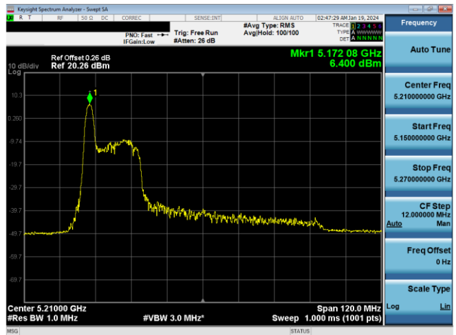
Plot 7-272. PSD CDD Antenna WF7a (80MHz BW 11ax Index 0 - RU26 - Ch.42)
