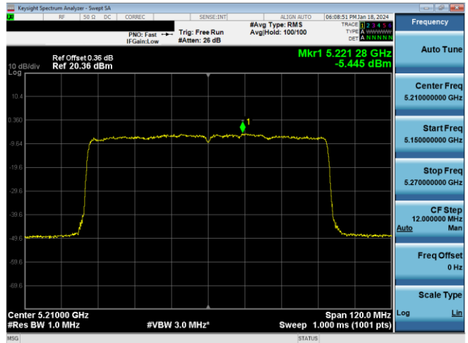
Plot 7-277. PSD CDD Antenna WF8 (80MHz BW 11ax – RU996 – Ch.42)
