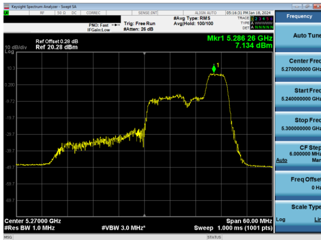
Plot 7-299. PSD CDD Antenna WF8 (40MHz BW 11ax Index 44 - RU52 - Ch.54)
