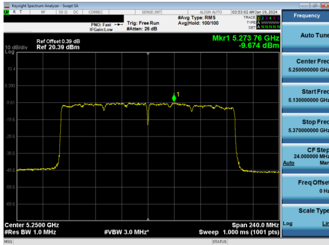
Plot 7-286. PSD CDD Antenna WF7a (160MHz BW 11ax - RU996x2 - Ch.50)
