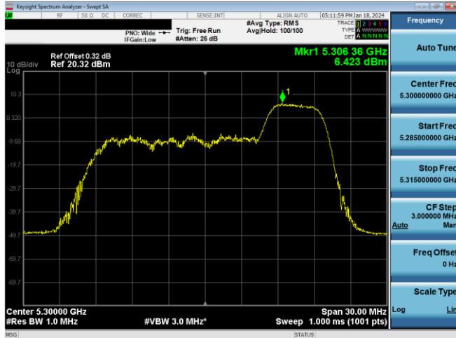
Plot 7-291. PSD CDD Antenna WF8 (20MHz BW 11ax Index 40 – RU52 – Ch.60)
