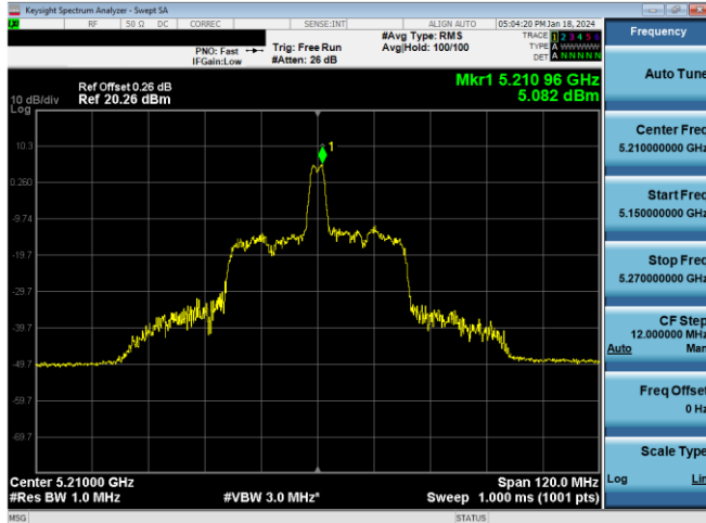
Plot 7-273. PSD CDD Antenna WF8 (80MHz BW 11ax Index 18 – RU26 – Ch.42)
