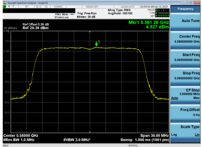
Plot 7-318. PSD SDM Antenna WF7a (20MHz BW 11ax- RU242 - Ch.116)
