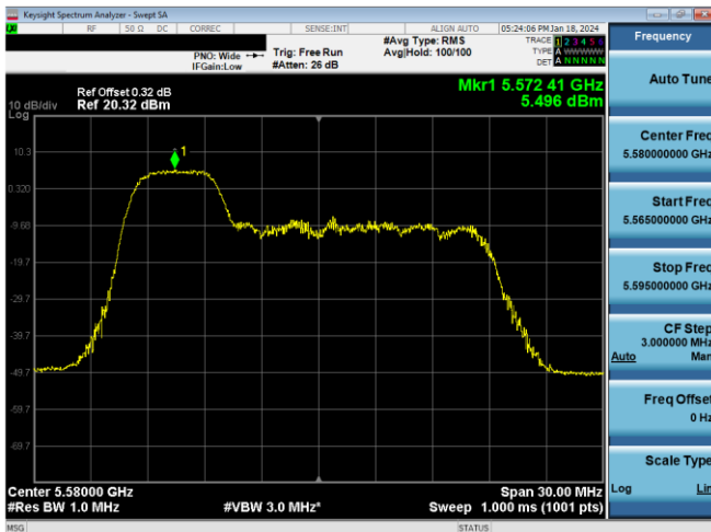
Plot 7-311. PSD SDM Antenna WF8 (20MHz BW 11ax Index 37 - RU52 - Ch.116)
