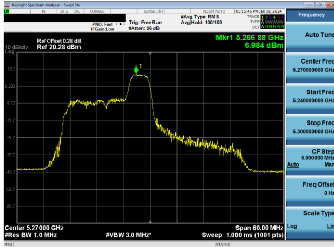
Plot 7-297. PSD CDD Antenna WF8 (40MHz BW 11ax Index 40 - RU52 - Ch.54)
