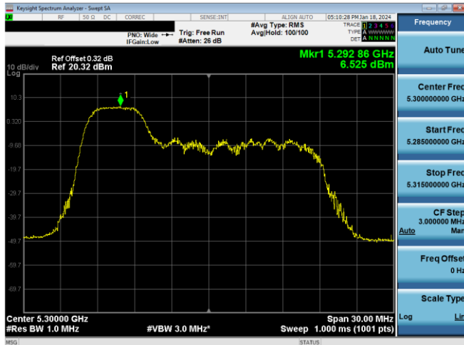
Plot 7-287. PSD CDD Antenna WF8 (20MHz BW 11ax Index 37 - RU52 - Ch.60)
