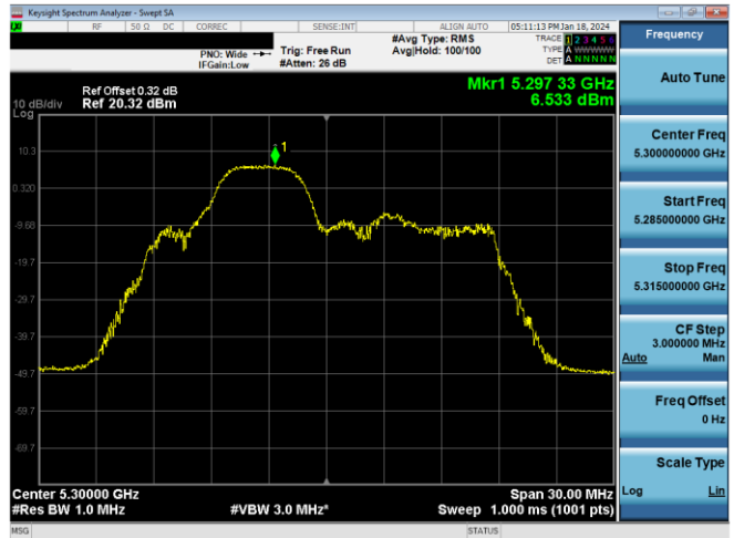
Plot 7-289. PSD CDD Antenna WF8 (20MHz BW 11ax Index 38 - RU52 - Ch.60)
