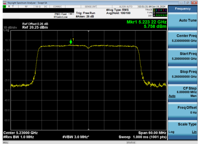
Plot 7-270. PSD CDD Antenna WF7a (40MHz BW 11ax - RU484 - Ch.46)
