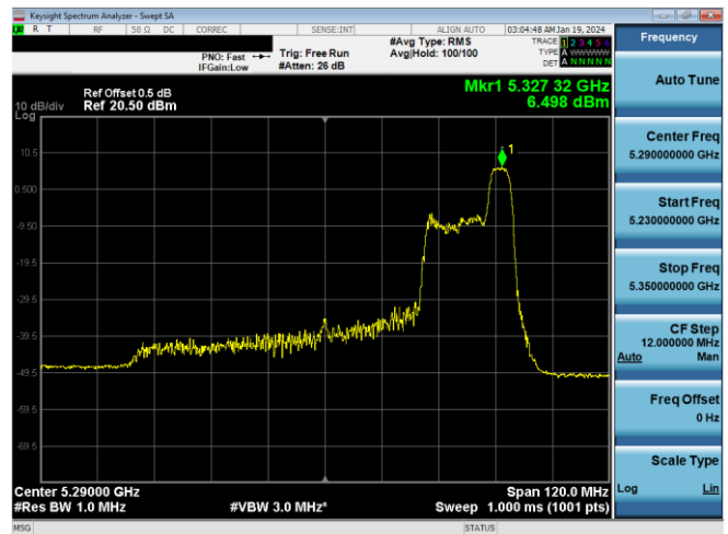
Plot 7-308. PSD CDD Antenna WF7a (80MHz BW 11ax Index 52 – RU52 – Ch.58)
