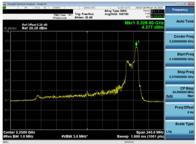
Plot 7-283. PSD CDD Antenna WF8 (160MHz BW 11ax Index 52 - RU52 - Ch.50 (U))
