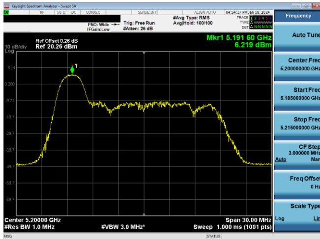
Plot 7-255. PSD CDD Antenna WF8 (20MHz BW 11ax Index 0 – RU26 – Ch.40)
