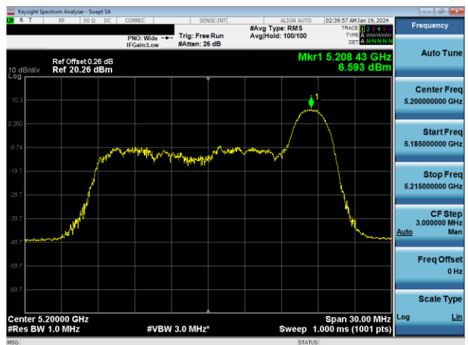
Plot 7-260. PSD CDD Antenna WF7a (20MHz BW 11ax Index 8 – RU26 – Ch.40)
