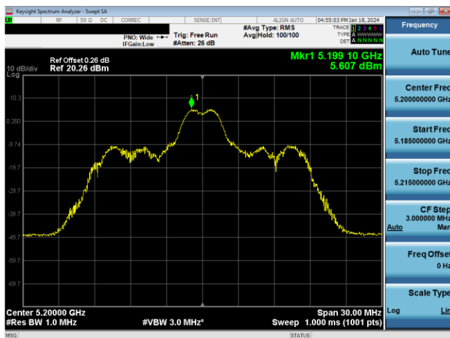
Plot 7-257. PSD CDD Antenna WF8 (20MHz BW 11ax Index 4 – RU26 – Ch.40)
