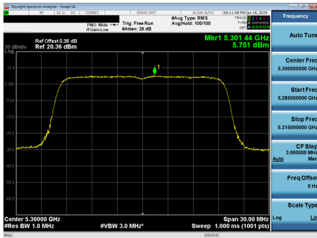
Plot 7-293. PSD CDD Antenna WF8 (20MHz BW 11ax – RU242 – Ch.60)
