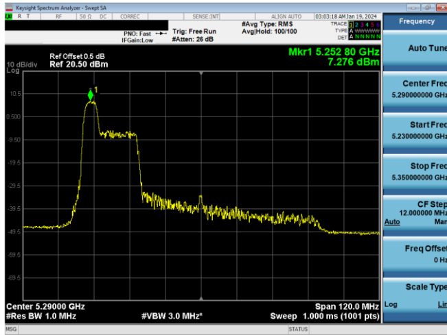
Plot 7-304. PSD CDD Antenna WF7a (80MHz BW 11ax Index 37 – RU52 – Ch.58)
