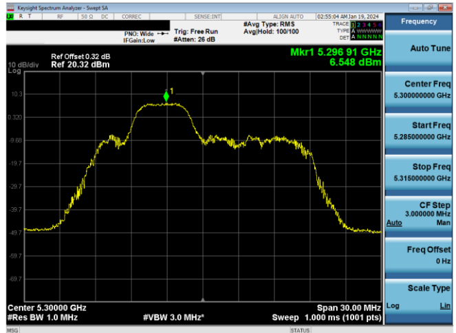
Plot 7-290. PSD CDD Antenna WF7a (20MHz BW 11ax Index 38 - RU52 - Ch.60)
