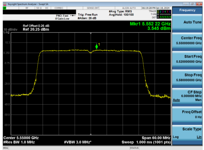
Plot 7-325. PSD CDD Antenna WF8 (40MHz BW 11ax - RU484 - Ch.110)
