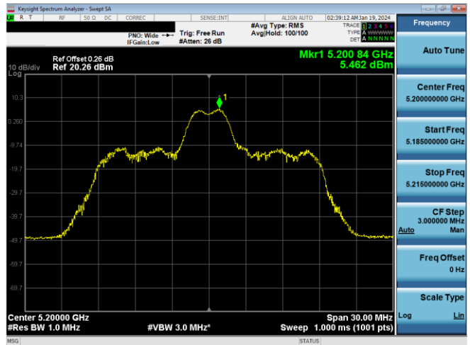
Plot 7-258. PSD CDD Antenna WF7a (20MHz BW 11ax Index 4 – RU26 – Ch.40)
