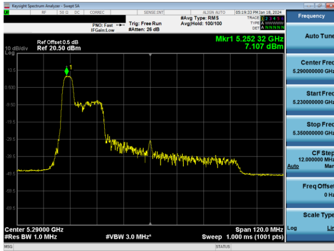
Plot 7-303. PSD CDD Antenna WF8 (80MHz BW 11ax Index 37 – RU52 – Ch.58)
