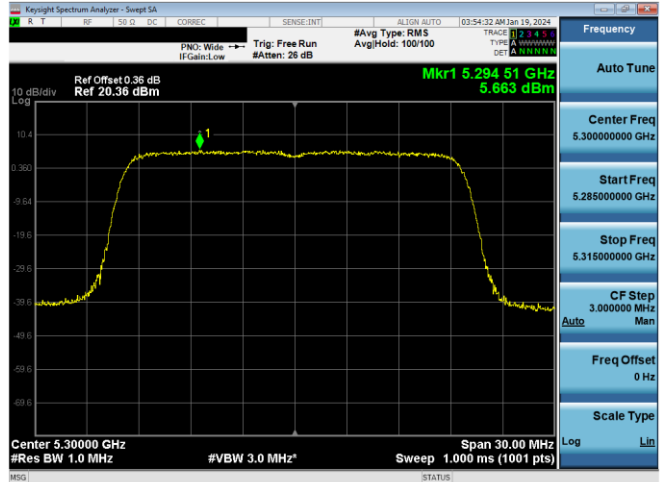
Plot 7-294. PSD CDD Antenna WF7a (20MHz BW 11ax – RU242 – Ch.60)
