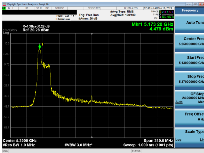
Plot 7-280. PSD CDD Antenna WF7a (160MHz BW 11ax Index 37 - RU52 - Ch.50 (L))
