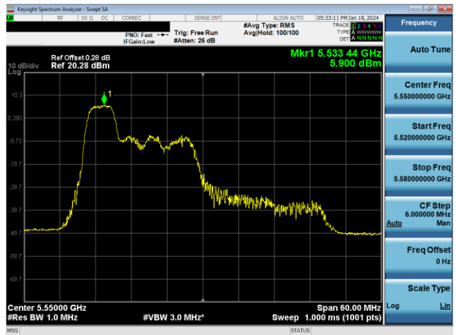
Plot 7-319. PSD SDM Antenna WF8 (40MHz BW 11ax Index 37 - RU52 - Ch.110)
