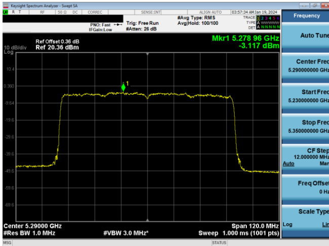
Plot 7-310. PSD CDD Antenna WF7a (80MHz BW 11ax - RU996 - Ch.58)
