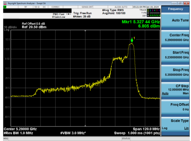
Plot 7-307. PSD CDD Antenna WF8 (80MHz BW 11ax Index 52 – RU52 – Ch.58)
