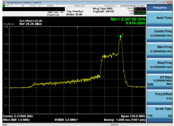
Plot 7-276. PSD CDD Antenna WF7a (80MHz BW 11ax Index 36 – RU26 – Ch.42)
