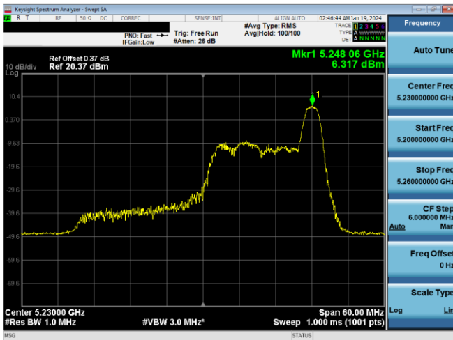
Plot 7-268. PSD CDD Antenna WF7a (40MHz BW 11ax Index 17 - RU26 - Ch.46)
