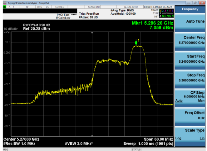
Plot 7-300. PSD CDD Antenna WF7a (40MHz BW 11ax Index 44 - RU52 - Ch.54)
