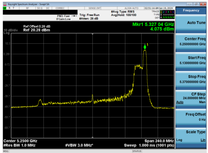
Plot 7-284. PSD CDD Antenna WF7a (160MHz BW 11ax Index 52 - RU52 - Ch.50 (U))
