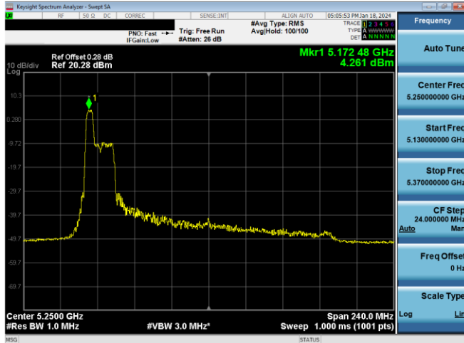
Plot 7-279. PSD CDD Antenna WF8 (160MHz BW 11ax Index 37 - RU52 - Ch.50 (L))
