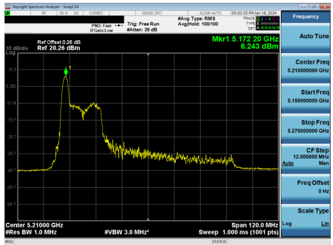
Plot 7-271. PSD CDD Antenna WF8 (80MHz BW 11ax Index 0 - RU26 - Ch.42)
