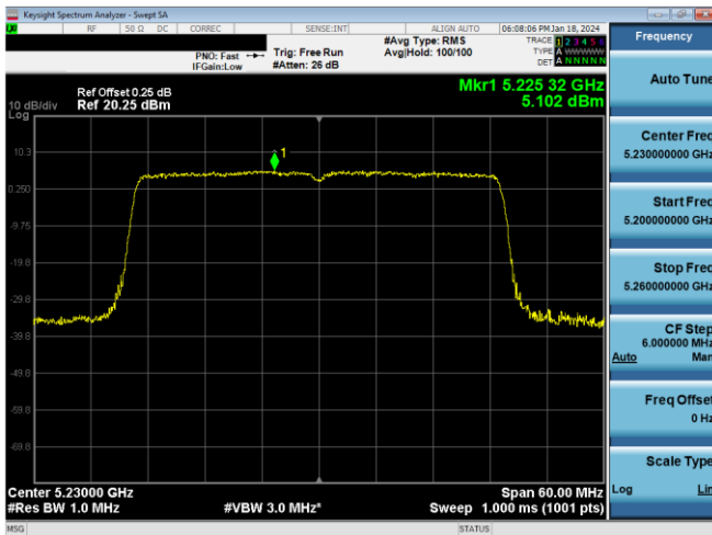
Plot 7-269. PSD CDD Antenna WF8 (40MHz BW 11ax - RU484 - Ch.46)
