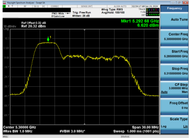
Plot 7-288. PSD CDD Antenna WF7a (20MHz BW 11ax Index 37 - RU52 - Ch.60)
