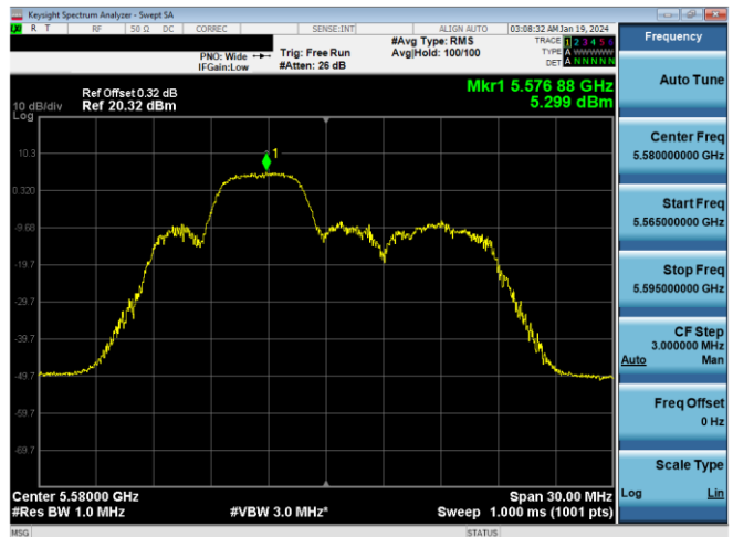
Plot 7-314. PSD SDM Antenna WF7a (20MHz BW 11ax Index 38 - RU52 - Ch.116)
