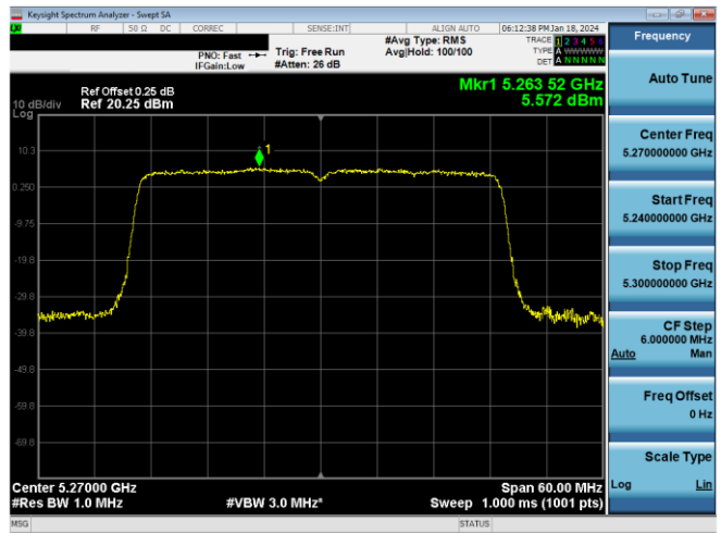
Plot 7-301. PSD CDD Antenna WF8 (40MHz BW 11ax - RU484 - Ch.54)
