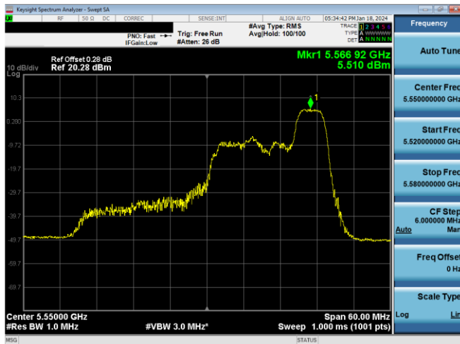
Plot 7-323. PSD SDM Antenna WF8 (40MHz BW 11ax Index 44 - RU52 - Ch.110)
