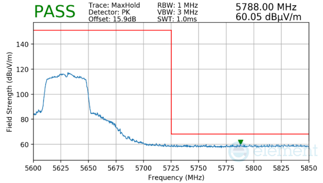
Plot 7-927. (FCC Only) Antenna WF7a (Pk, Ch.126, 802.11n, MCS4)
