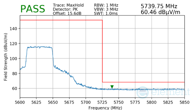
Plot 7-961. (FCC Only) Antenna WF7a (Pk, Ch.126, 80.11ax(SU), MCS11)
