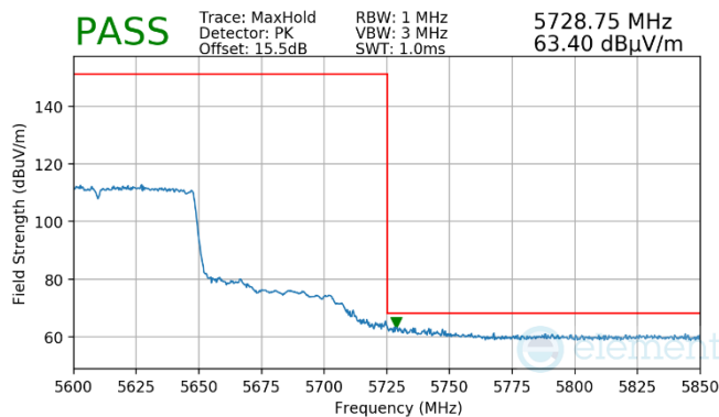
Plot 7-985. (FCC Only) Antenna WF7a (Pk, Ch.122, 802.11ac, MCS9)
