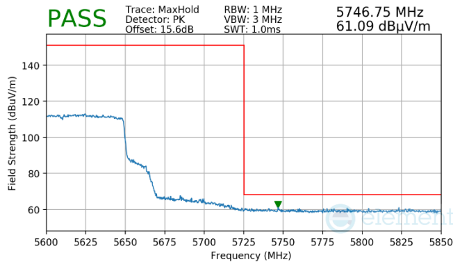
Plot 7-1004. (FCC Only) Antenna WF7a (Pk, Ch.122, 802.11ax(SU), MCS2)
