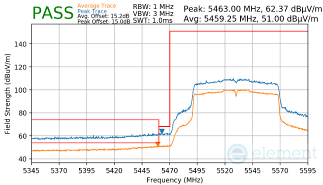
Plot 7-977. Antenna WF7a (Pk & Avg, Ch.106, 802.11ac, MCS2)
