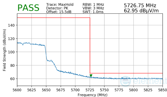
Plot 7-984. (FCC Only) Antenna WF7a (Pk, Ch.122, 802.11ac, MCS4)
