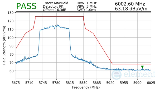
Plot 7-989. Antenna WF7a (Pk, Ch.155, 802.11ac, MCS2)
