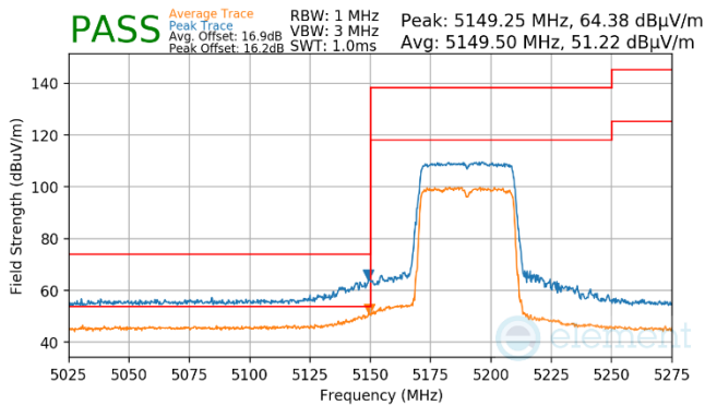
Plot 7-940. Antenna WF7a (Pk & Avg, Ch.38, 80.11ax(SU), MCS11)
