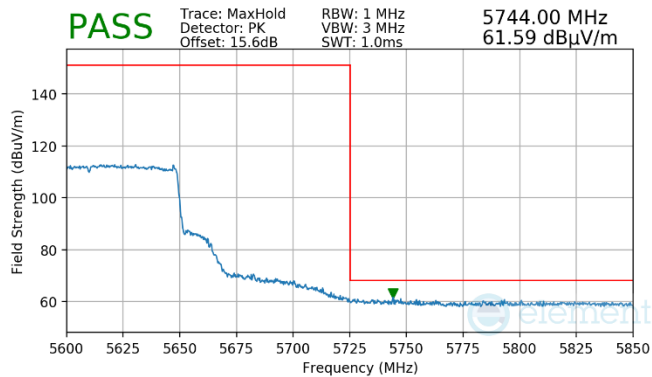
Plot 7-1005. (FCC Only) Antenna WF7a (Pk, Ch.122, 802.11ax(SU), MCS4)
