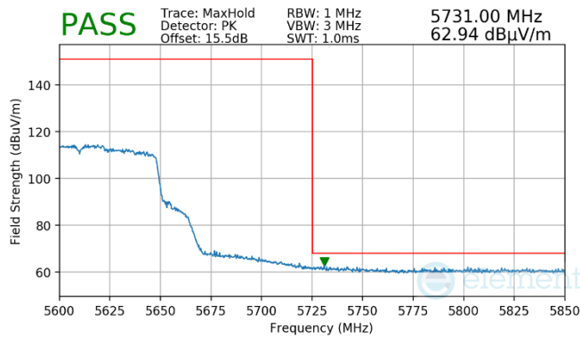
Plot 7-983. (FCC Only) Antenna WF7a (Pk, Ch.122, 802.11ac, MCS2)
