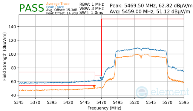
Plot 7-978. Antenna WF7a (Pk & Avg, Ch.106, 802.11ac, MCS4)
