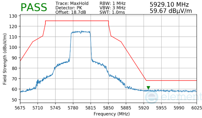
Plot 7-968. Antenna WF7a (Pk, Ch.159, 80.11ax(SU), MCS2)
