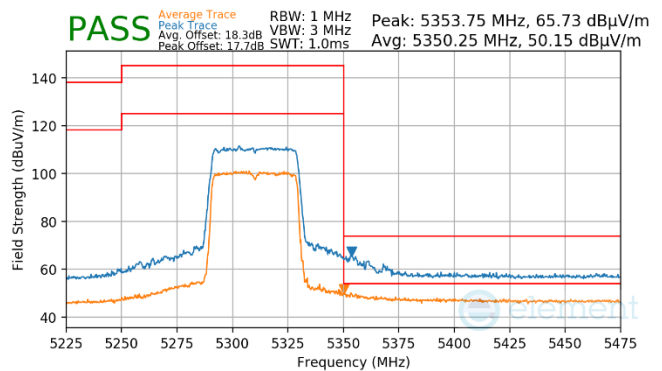
Plot 7-949. Antenna WF7a (Pk & Avg, Ch.62, 80.11ax(SU), MCS11)
