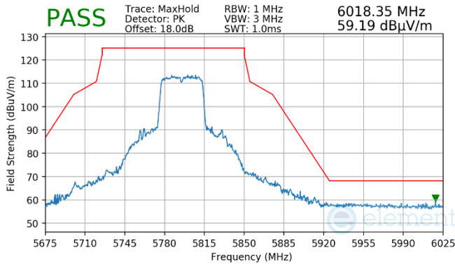
Plot 7-937. Antenna WF7a (Pk, Ch.159, 802.11n, MCS7)
