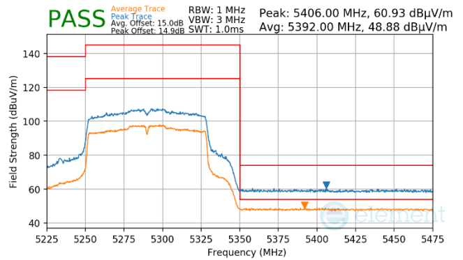
Plot 7-974. Antenna WF7a (Pk & Avg, Ch.58, 802.11ac, MCS2)
