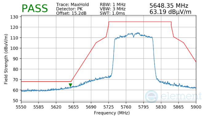
Plot 7-986. Antenna WF7a (Pk, Ch.155, 802.11ac, MCS2)
