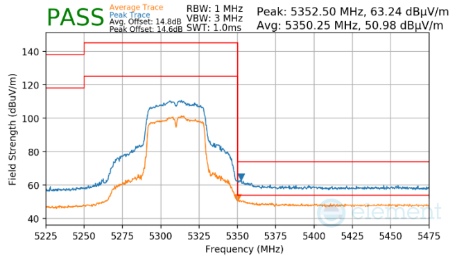
Plot 7-916. Antenna WF7a (Pk & Avg, Ch.62, 802.11n, MCS4)
