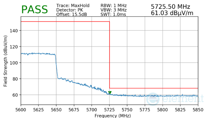
Plot 7-1006. (FCC Only) Antenna WF7a (Pk, Ch.122, 802.11ax(SU), MCS11)
