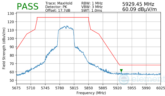
Plot 7-936. Antenna WF7a (Pk, Ch.159, 802.11n, MCS4)
