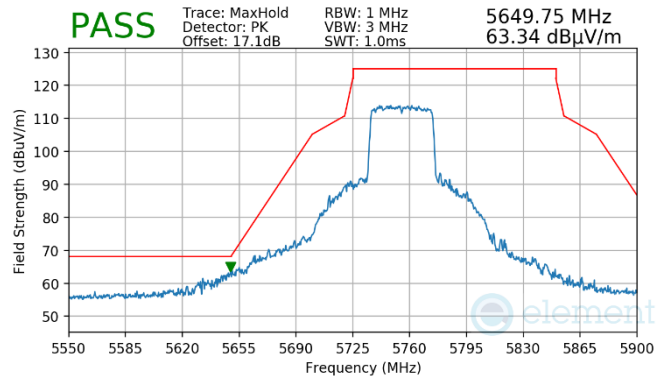
Plot 7-967. Antenna WF7a (Pk, Ch.151, 80.11ax(SU), MCS11)
