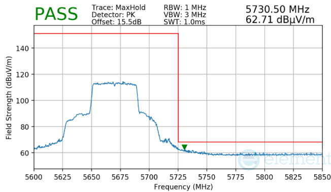
Plot 7-963. Antenna WF7a (Pk, Ch.134, 80.11ax(SU), MC4)
