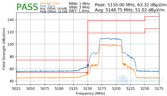
Plot 7-939. Antenna WF7a (Pk & Avg, Ch.38, 80.11ax(SU), MCS4)
