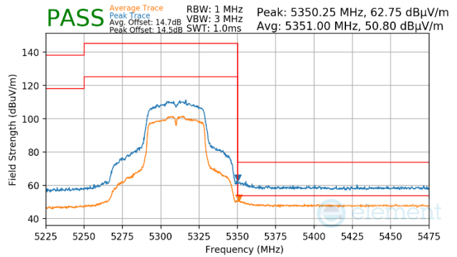
Plot 7-915. Antenna WF7a (Pk & Avg, Ch.62, 802.11n, MCS2)
