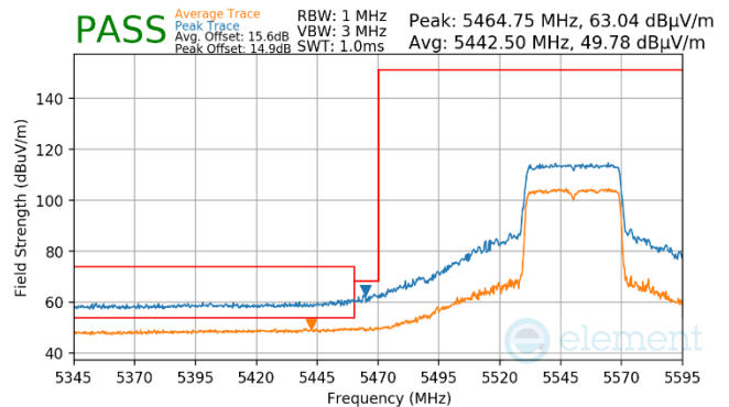
Plot 7-955. Antenna WF7a (Pk & Avg, Ch.110, 80.11ax(SU), MCS11)
