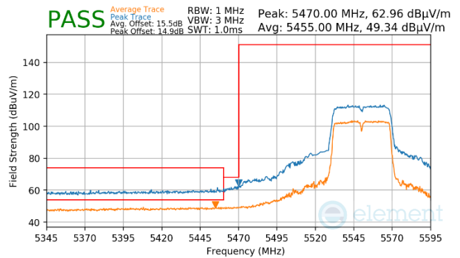
Plot 7-923. Antenna WF7a (Pk & Avg, Ch.110, 802.11n, MCS7)
