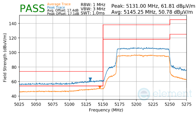
Plot 7-992. Antenna WF7a (Pk & Avg, Ch.42, 802.11ax(SU), MCS2)
