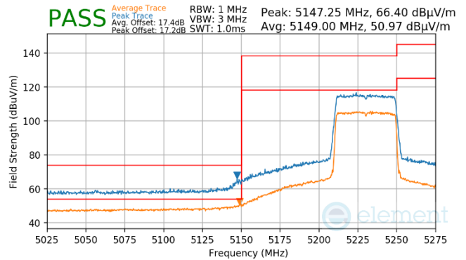
Plot 7-941. Antenna WF7a (Pk & Avg, Ch.46, 80.11ax(SU), MCS2)
