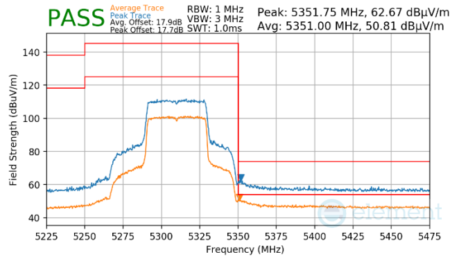
Plot 7-947. Antenna WF7a (Pk & Avg, Ch.62, 80.11ax(SU), MCS2)
