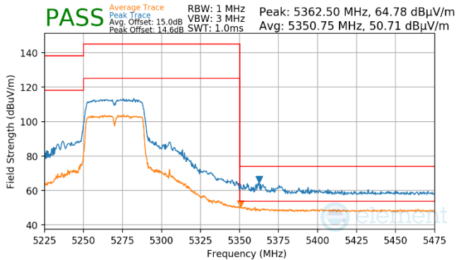
Plot 7-914. Antenna WF7a (Pk & Avg, Ch.54, 802.11n, MCS7)
