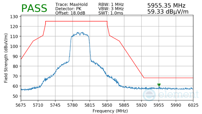
Plot 7-935. Antenna WF7a (Pk, Ch.159, 802.11n, MCS2)
