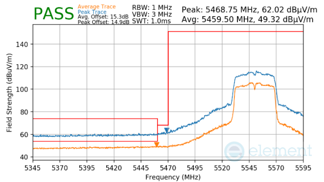
Plot 7-922. Antenna WF7a (Pk & Avg, Ch.110, 802.11n, MCS4)
