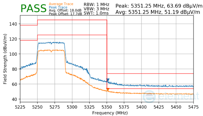
Plot 7-945. Antenna WF7a (Pk & Avg, Ch.54, 80.11ax(SU), MCS4)
