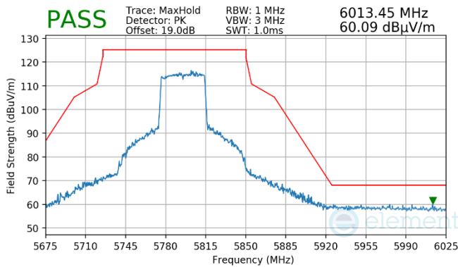
Plot 7-969. Antenna WF7a (Pk, Ch.159, 80.11ax(SU), MCS4)
