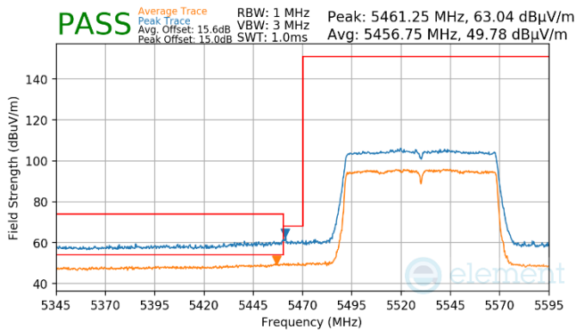
Plot 7-979. Antenna WF7a (Pk & Avg, Ch.106, 802.11ac, MCS9)
