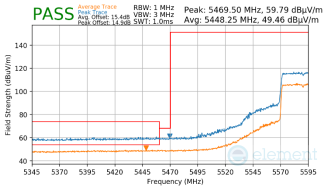
Plot 7-957. (FCC Only) Antenna WF7a (Pk & Avg, Ch.118, 80.11ax(SU), MCS4)
