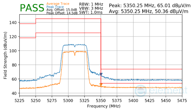
Plot 7-917. Antenna WF7a (Pk & Avg, Ch.62, 802.11n, MCS7)
