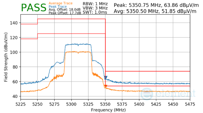
Plot 7-948. Antenna WF7a (Pk & Avg, Ch.62, 80.11ax(SU), MCS4)
