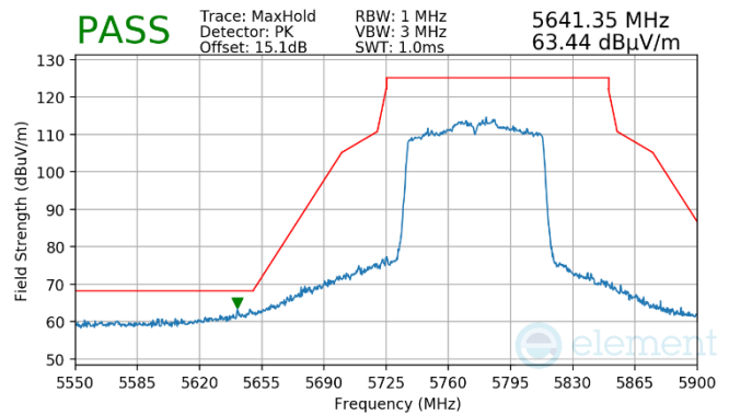
Plot 7-987. Antenna WF7a (Pk, Ch.155, 802.11ac, MCS4)
