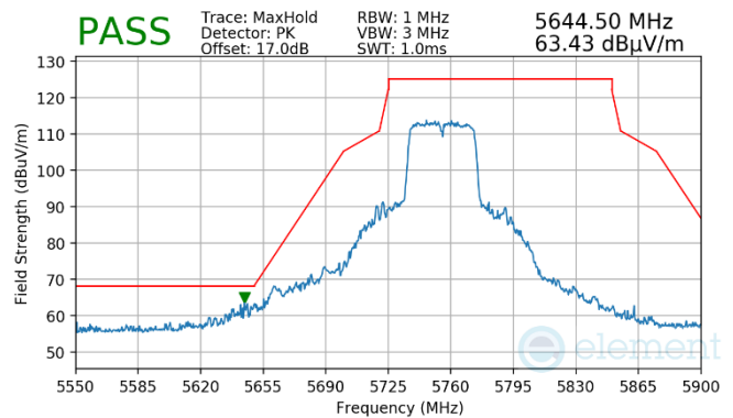
Plot 7-934. Antenna WF7a (Pk, Ch.151, 802.11n, MCS7)
