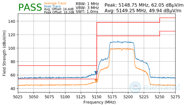
Plot 7-938. Antenna WF7a (Pk & Avg, Ch.38, 80.11ax(SU), MCS2)
