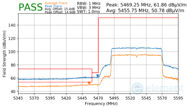
Plot 7-999. Antenna WF7a (Pk & Avg, Ch.106, 802.11ax(SU), MCS4)
