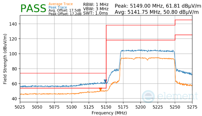
Plot 7-993. Antenna WF7a (Pk & Avg, Ch.42, 802.11ax(SU), MCS4)
