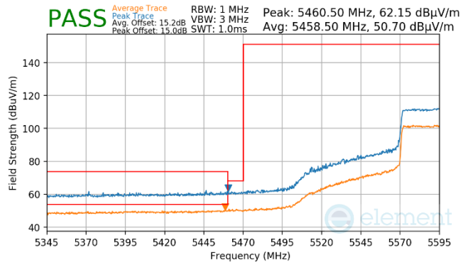
Plot 7-1001. (FCC Only) Antenna WF7a (Pk & Avg, Ch.122, 802.11ax(SU), MCS2)
