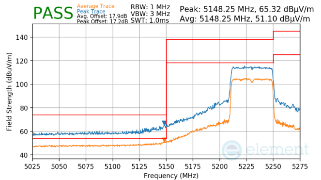
Plot 7-943. Antenna WF7a (Pk & Avg, Ch.46, 80.11ax(SU), MCS11)
