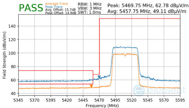
Plot 7-952. Antenna WF7a (Pk & Avg, Ch.102, 80.11ax(SU), MCS11)
