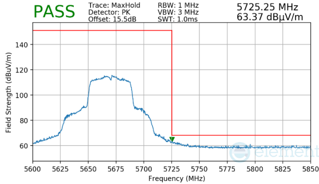
Plot 7-930. Antenna WF7a (Pk, Ch.134, 802.11n, MCS4)
