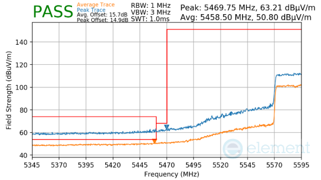
Plot 7-1003. (FCC Only) Antenna WF7a (Pk & Avg, Ch.122, 802.11ax(SU), MCS11)
