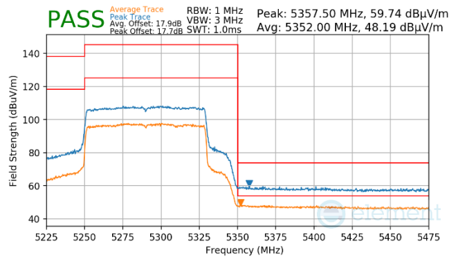
Plot 7-995. Antenna WF7a (Pk & Avg, Ch.58, 802.11ax(SU), MCS2)
