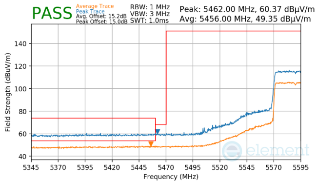
Plot 7-956. (FCC Only) Antenna WF7a (Pk & Avg, Ch.118, 80.11ax(SU), MCS2)
