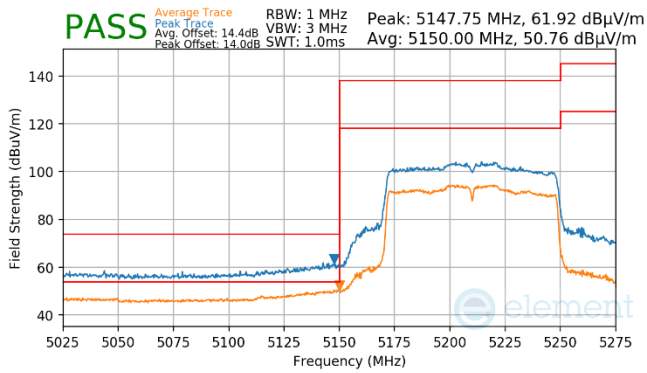
Plot 7-972. Antenna WF7a (Pk & Avg, Ch.42, 802.11ac, MCS4)
