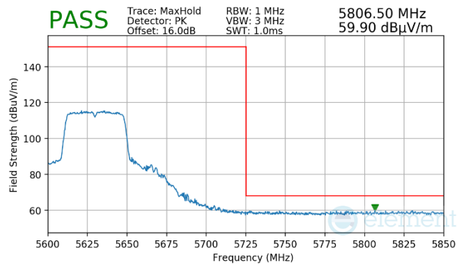
Plot 7-928. (FCC Only) Antenna WF7a (Pk, Ch.126, 802.11n, MCS7)
