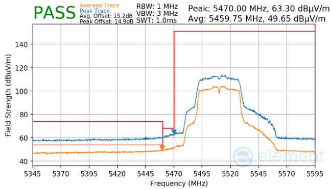
Plot 7-918. Antenna WF7a (Pk & Avg, Ch.102, 802.11n, MCS2)
