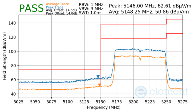
Plot 7-973. Antenna WF7a (Pk & Avg, Ch.42, 802.11ac, MCS9)
