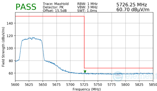
Plot 7-926. (FCC Only) Antenna WF7a (Pk, Ch.126, 802.11n, MCS2)
