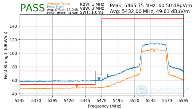
Plot 7-921. Antenna WF7a (Pk & Avg, Ch.110, 802.11n, MCS2)
