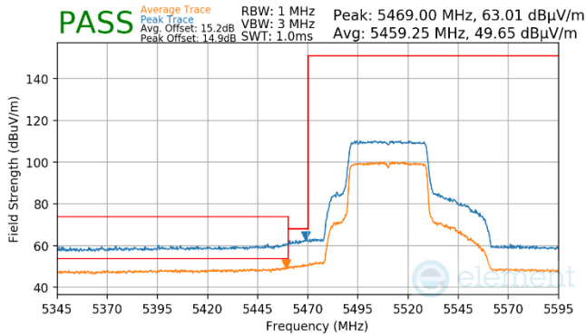
Plot 7-950. Antenna WF7a (Pk & Avg, Ch.102, 80.11ax(SU), MCS2)
