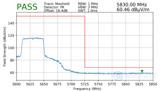
Plot 7-960. (FCC Only) Antenna WF7a (Pk, Ch.126, 80.11ax(SU), MCS4)
