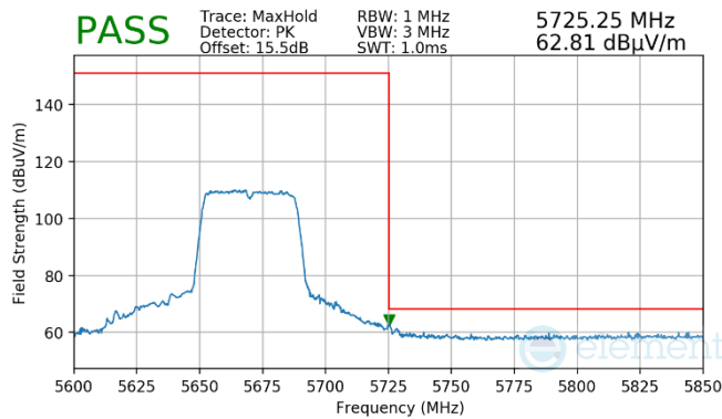
Plot 7-931. Antenna WF7a (Pk, Ch.134, 802.11n, MCS7)
