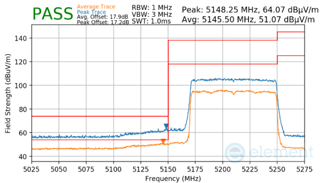
Plot 7-994. Antenna WF7a (Pk & Avg, Ch.42, 802.11ax(SU), MCS11)
