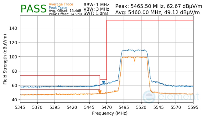
Plot 7-920. Antenna WF7a (Pk & Avg, Ch.102, 802.11n, MCS7)
