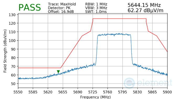
Plot 7-1008. Antenna WF7a (Pk, Ch.155, 802.11ax(SU), MCS2)
