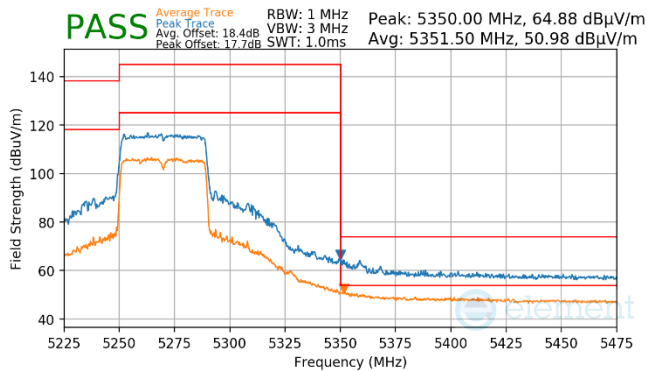
Plot 7-946. Antenna WF7a (Pk & Avg, Ch.54, 80.11ax(SU), MCS11)
