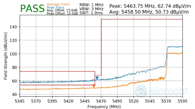
Plot 7-982. (FCC Only) Antenna WF7a (Pk & Avg, Ch.122, 802.11ac, MCS9)
