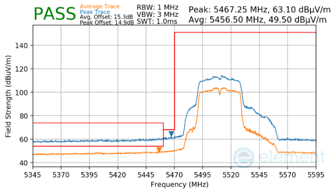
Plot 7-919. Antenna WF7a (Pk & Avg, Ch.102, 802.11n, MCS4)
