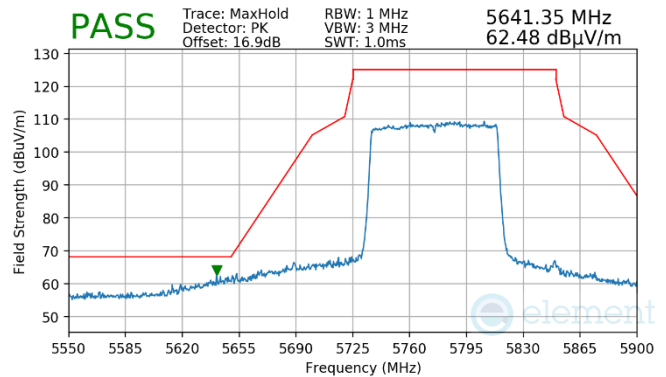
Plot 7-1007. Antenna WF7a (Pk, Ch.155, 802.11ax(SU), MCS2)
