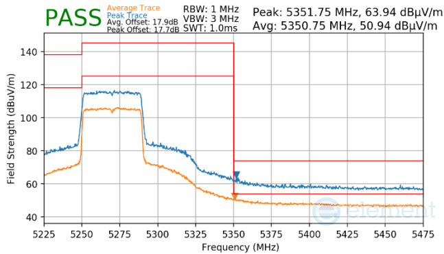
Plot 7-944. Antenna WF7a (Pk & Avg, Ch.54, 80.11ax(SU), MCS2)
