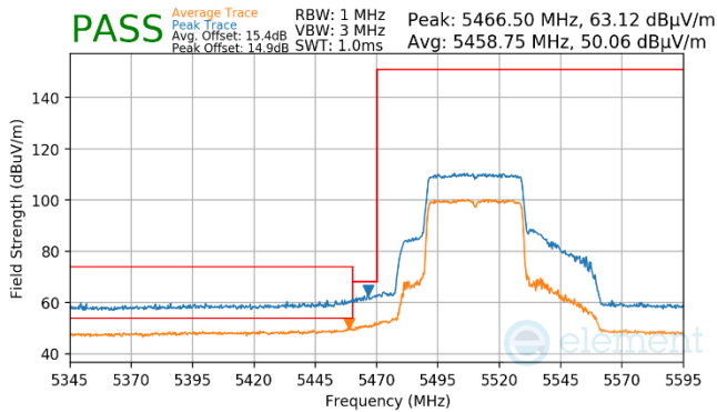
Plot 7-951. Antenna WF7a (Pk & Avg, Ch.102, 80.11ax(SU), MCS4)
