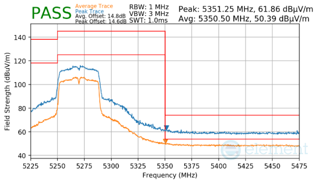
Plot 7-913. Antenna WF7a (Pk & Avg, Ch.54, 802.11n, MCS4)
