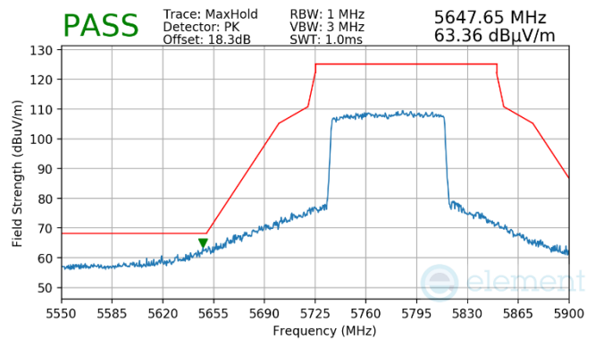
Plot 7-1009. Antenna WF7a (Pk, Ch.155, 802.11ax(SU), MCS11)
