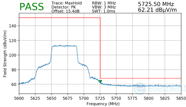
Plot 7-962. Antenna WF7a (Pk, Ch.134, 80.11ax(SU), MCS2)
