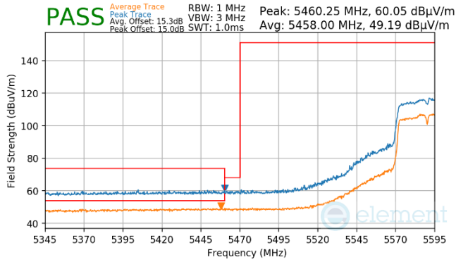
Plot 7-924. (FCC Only) Antenna WF7a (Pk, Ch.118, 802.11n, MCS4)
