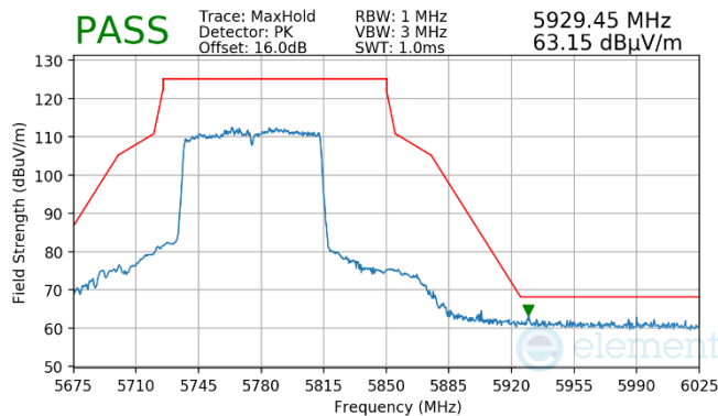
Plot 7-991. Antenna WF7a (Pk, Ch.155, 802.11ac, MC9)
