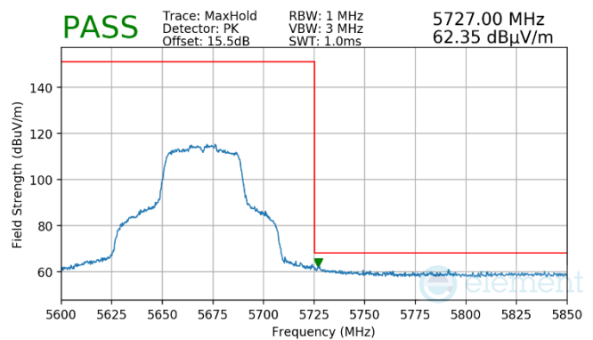
Plot 7-929. Antenna WF7a (Pk, Ch.134, 802.11n, MCS2)
