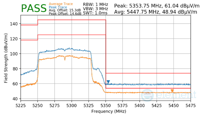
Plot 7-975. Antenna WF7a (Pk & Avg, Ch.58, 802.11ac, MCS4)
