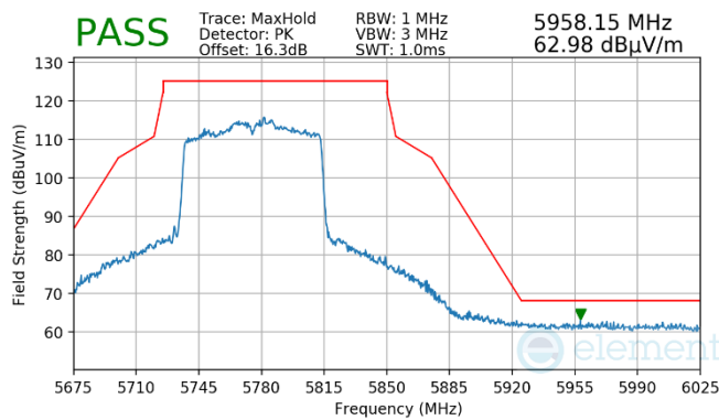
Plot 7-990. Antenna WF7a (Pk, Ch.155, 802.11ac, MCS4)
