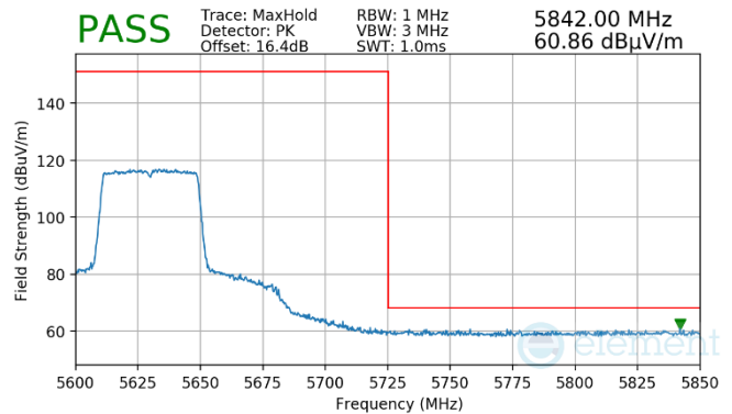
Plot 7-959. (FCC Only) Antenna WF7a (Pk, Ch.126, 80.11ax(SU), MCS2)
