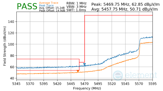
Plot 7-980. (FCC Only) Antenna WF7a (Pk & Avg, Ch.122, 802.11ac, MCS2)
