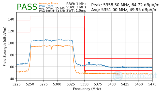
Plot 7-976. Antenna WF7a (Pk & Avg, Ch.58, 802.11ac, MC9)
