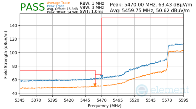
Plot 7-981. (FCC Only) Antenna WF7a (Pk & Avg, Ch.122, 802.11ac, MCS4)
