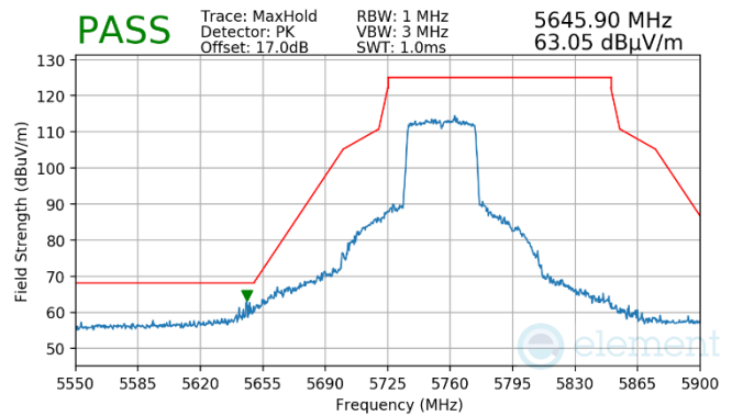
Plot 7-966. Antenna WF7a (Pk, Ch.151, 80.11ax(SU), MCS4)
