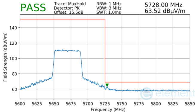
Plot 7-964. Antenna WF7a (Pk, Ch.134, 80.11ax(SU), MCS11)
