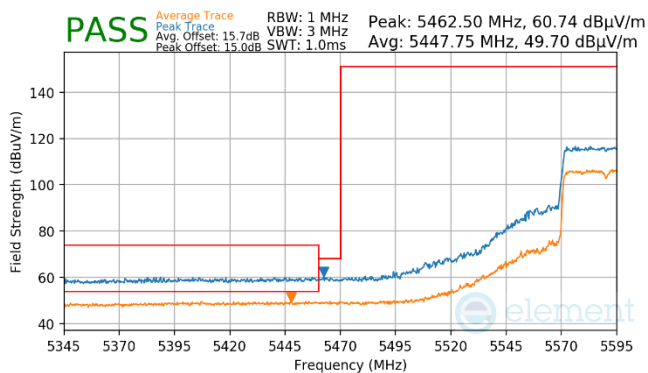
Plot 7-958. (FCC Only) Antenna WF7a (Pk & Avg, Ch.118, 80.11ax(SU), MCS11)
