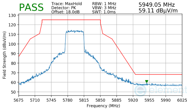
Plot 7-970. Antenna WF7a (Pk, Ch.159, 80.11ax(SU), MCS11)
