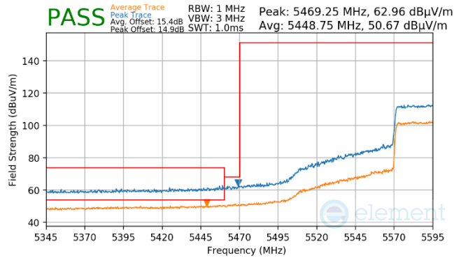
Plot 7-1002. (FCC Only) Antenna WF7a (Pk & Avg, Ch.122, 802.11ax(SU), MC4)
