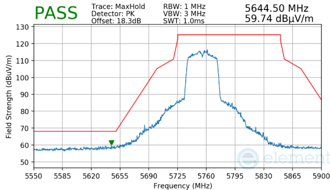
Plot 7-932. Antenna WF7a (Pk, Ch.151, 802.11n, MCS2)
