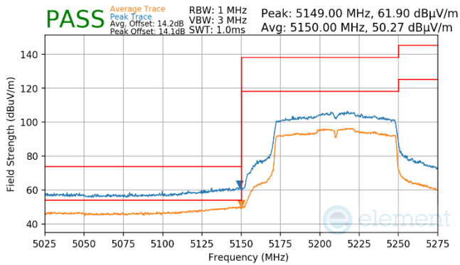
Plot 7-971. Antenna WF7a (Pk & Avg, Ch.42, 802.11ac, MCS2)
