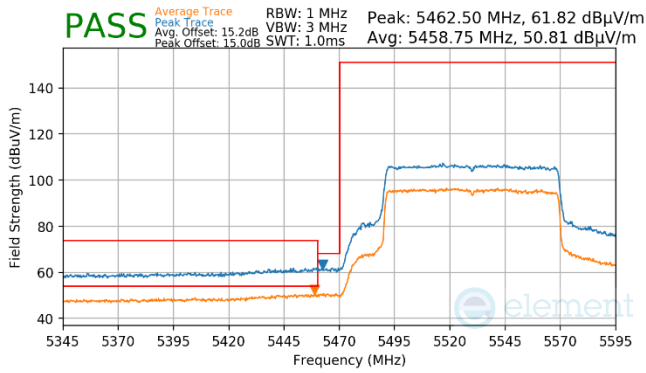
Plot 7-998. Antenna WF7a (Pk & Avg, Ch.106, 802.11ax(SU), MCS2)
