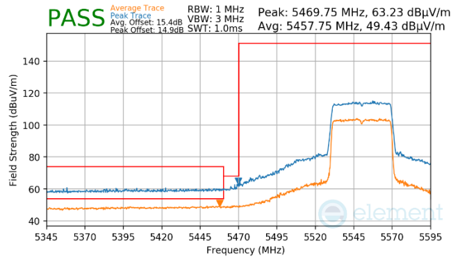
Plot 7-954. Antenna WF7a (Pk & Avg, Ch.110, 80.11ax(SU), MCS4)
