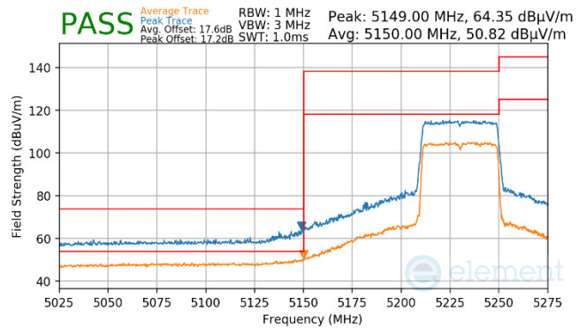
Plot 7-942. Antenna WF7a (Pk & Avg, Ch.46, 80.11ax(SU), MCS4)
