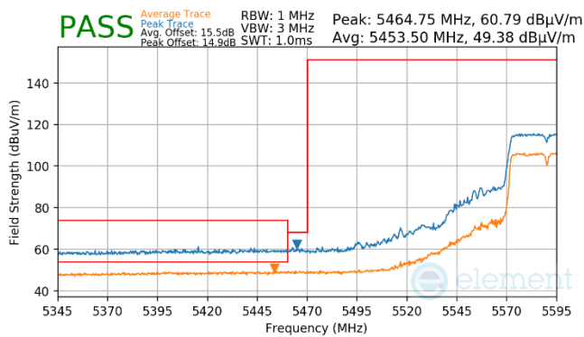
Plot 7-925. (FCC Only) Antenna WF7a (Pk, Ch.118, 802.11n, MCS7)
