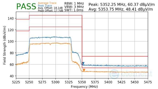
Plot 7-996. Antenna WF7a (Pk & Avg, Ch.58, 802.11ax(SU), MCS4)
