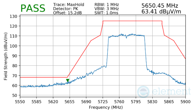
Plot 7-988. Antenna WF7a (Pk, Ch.155, 802.11ac, MCS9)
