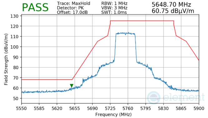
Plot 7-965. Antenna WF7a (Pk, Ch.151, 80.11ax(SU), MCS2)
