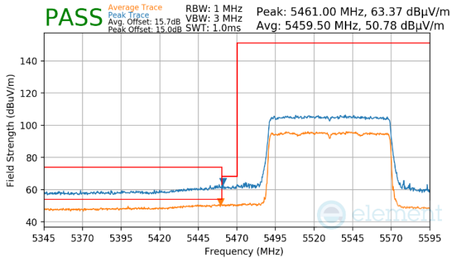
Plot 7-1000. Antenna WF7a (Pk & Avg, Ch.106, 802.11ax(SU), MCS11)
