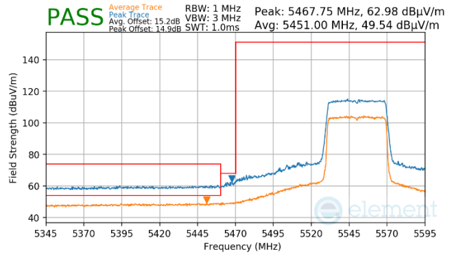
Plot 7-953. Antenna WF7a (Pk & Avg, Ch.110, 80.11ax(SU), MCS2)
