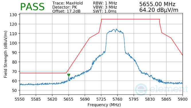
Plot 7-933. Antenna WF7a (Pk, Ch.151, 802.11n, MCS4)
