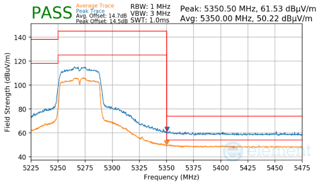
Plot 7-912. Antenna WF7a (Pk & Avg, Ch.54, 802.11n, MCS2)
