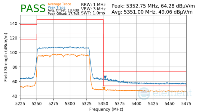
Plot 7-997. Antenna WF7a (Pk & Avg, Ch.58, 802.11ax(SU), MCS11)
