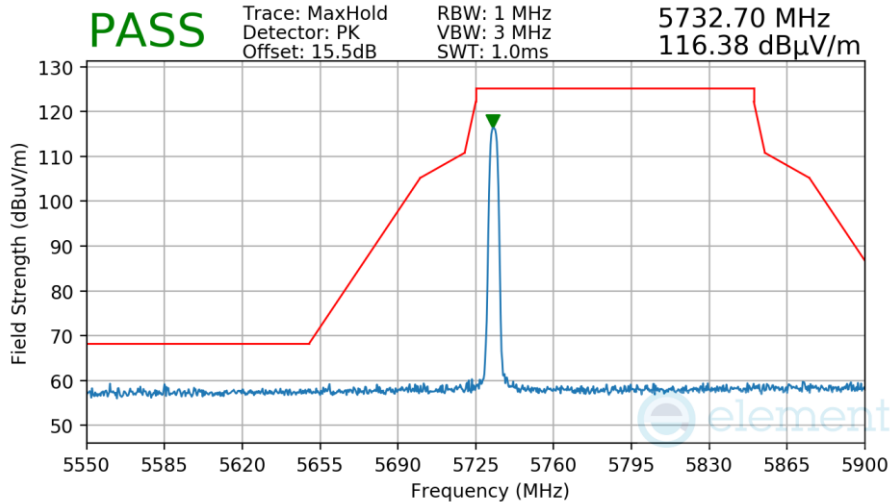
Plot 7-176. Radiated Lower Band Edge Measurement TxBF
