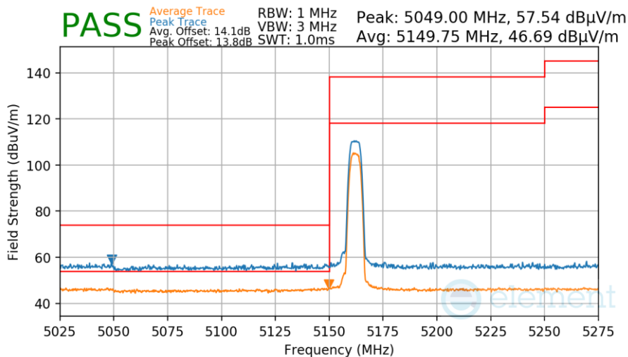
Plot 7-169. Radiated Lower Band Edge Measurement Antenna WF7a
