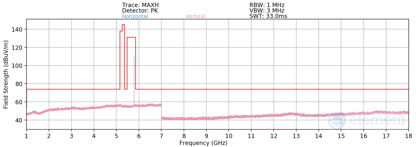
Plot 7-152. Radiated Spurious Emissions 1-18GHz Antenna WF7a (HDR4, ePA – 5789MHz)
