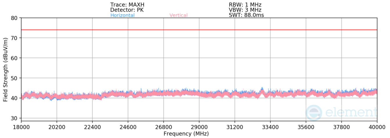
Plot 7-160. Radiated Spurious Emissions Above 18GHz TxBF (HDR4, ePA - 5789MHz)
