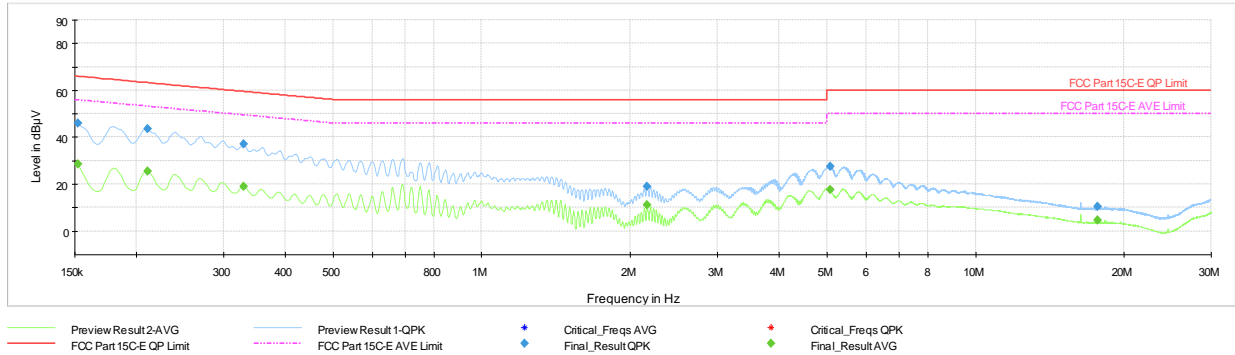
Plot 7-185. AC Line Conducted Plot TxBF (HDR4, ePA – 5789MHz) (N) with AC/DC Adapter
