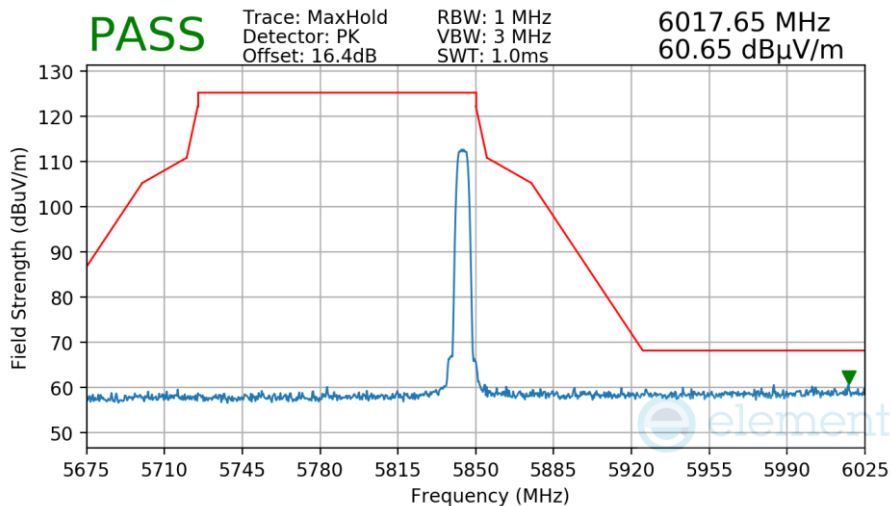
Plot 7-167. Radiated Upper Band Edge Measurement Antenna WF8
