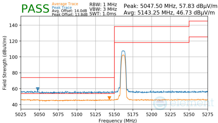
Plot 7-163. Radiated Lower Band Edge Measurement Antenna WF8
