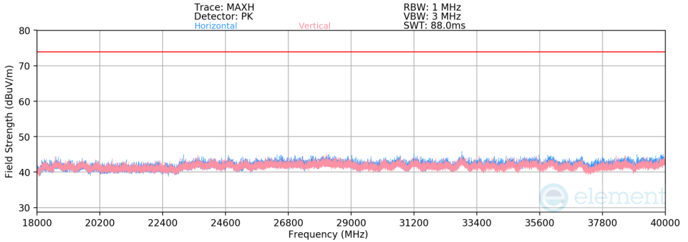
Plot 7-156. Radiated Spurious Emissions Above 18GHz TxBF (HDR4, ePA – 5204MHz)
