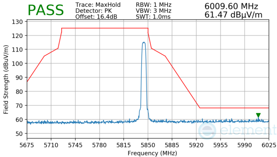
Plot 7-179. Radiated Upper Band Edge Measurement TxBF
