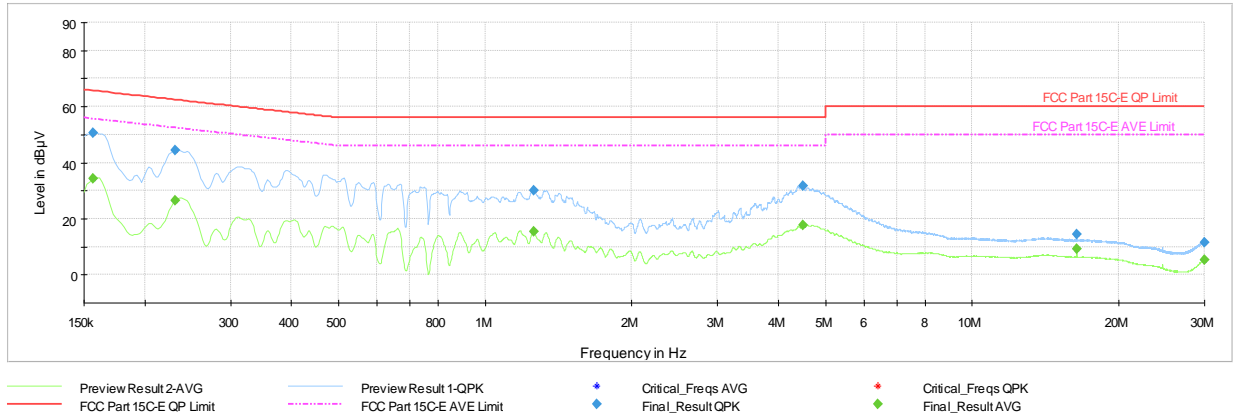
Plot 7-183. AC Line Conducted Plot TxBF (HDR4, ePA – 5204MHz) (N) with AC/DC Adapter
