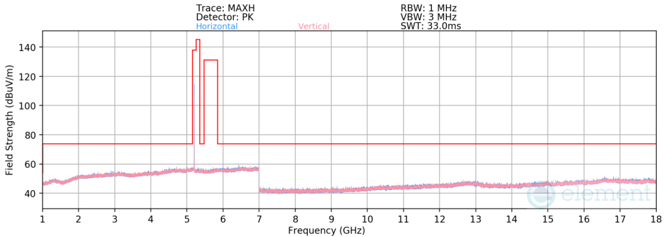
Plot 7-155. Radiated Spurious Emissions 1-18GHz TxBF (HDR4, ePA – 5204MHz)
