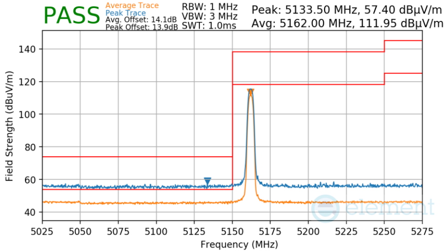
Plot 7-174. Radiated Lower Band Edge Measurement TxBF
