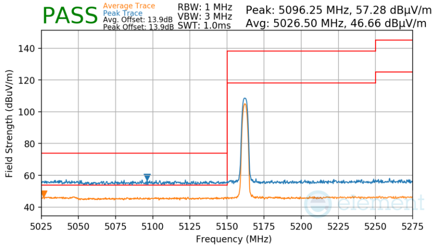
Plot 7-162. Radiated Lower Band Edge Measurement Antenna WF8
