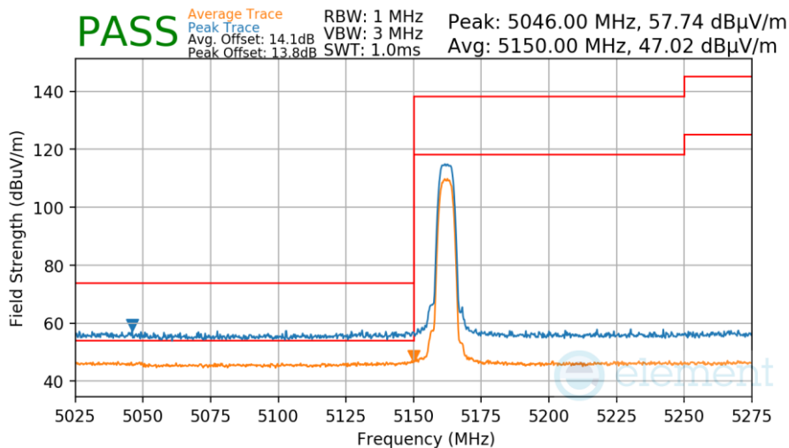
Plot 7-175. Radiated Lower Band Edge Measurement TxBF
