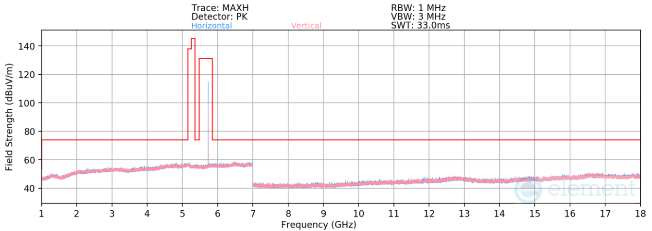
Plot 7-158. Radiated Spurious Emissions 1-18GHz TxBF (HDR4, ePA – 5733MHz)
