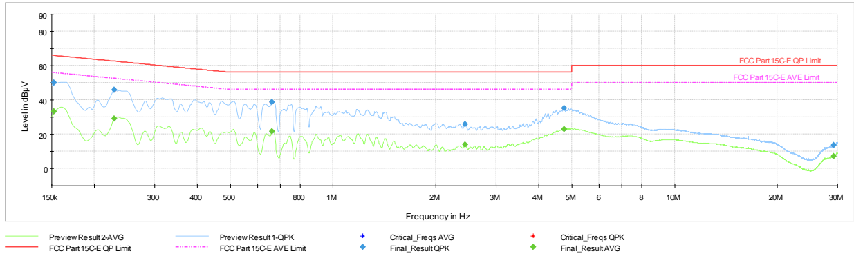
Plot 7-184. AC Line Conducted Plot TxBF (HDR4, ePA – 5789MHz) (L1) with AC/DC Adapter
