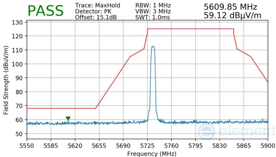
Plot 7-165. Radiated Lower Band Edge Measurement Antenna WF8
