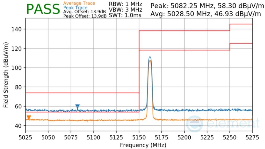
Plot 7-168. Radiated Lower Band Edge Measurement Antenna WF7a
