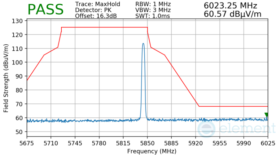
Plot 7-166. Radiated Upper Band Edge Measurement Antenna WF8
