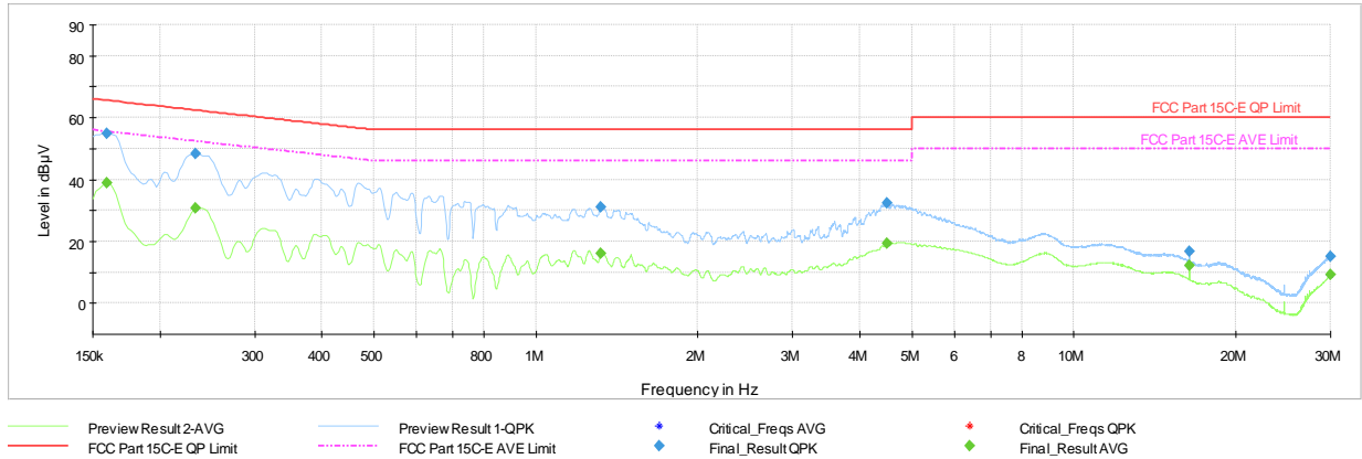
Plot 7-182. AC Line Conducted Plot TxBF (HDR4, ePA – 5204MHz) (L1) with AC/DC Adapter
