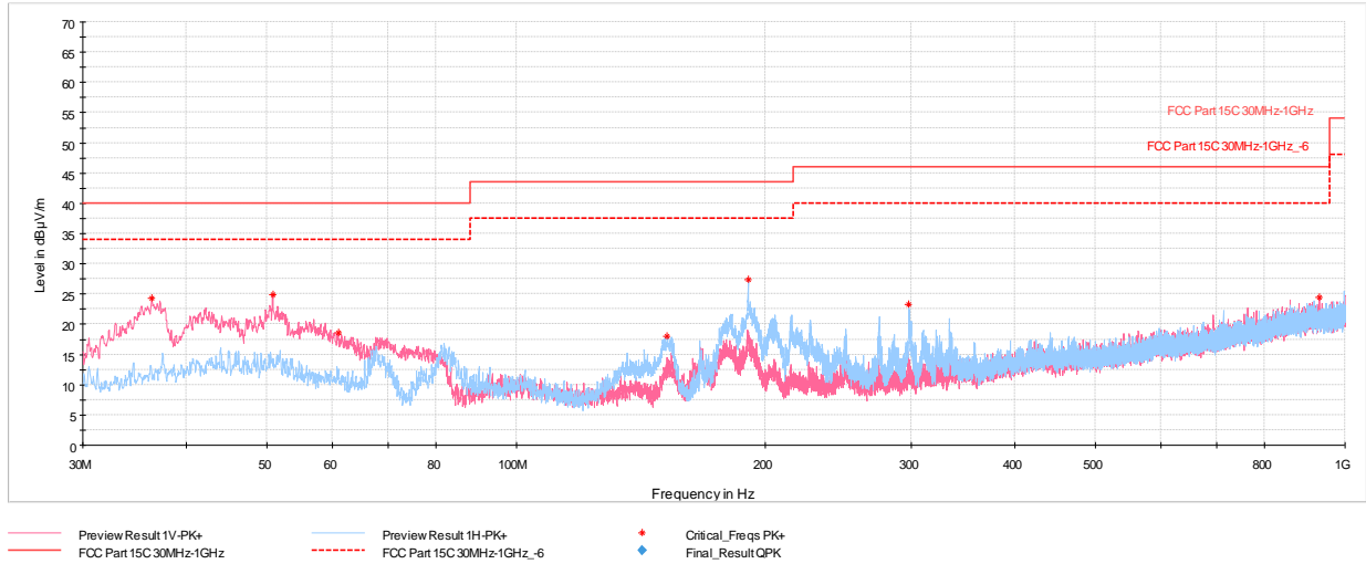
Plot 7-180. Radiated Spurious Emissions Below 1GHz TxBF (HDR4, ePA – 5204MHz), with AC/DC Adapter
