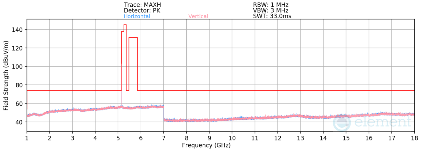
Plot 7-154. Radiated Spurious Emissions 1-18GHz TxBF (HDR4, ePA – 5162MHz)
