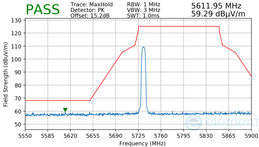
Plot 7-171. Radiated Lower Band Edge Measurement Antenna WF7a
