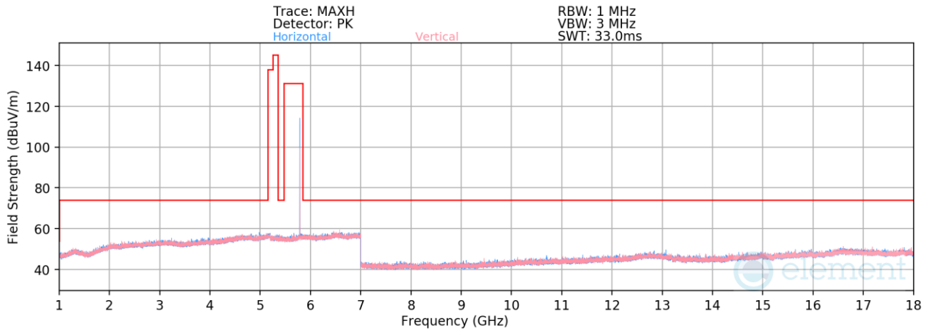
Plot 7-159. Radiated Spurious Emissions 1-18GHz TxBF (HDR4 – 5789MHz)
