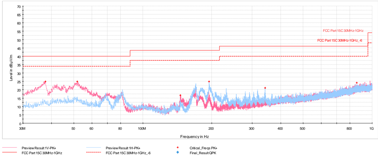
Plot 7-181 Radiated Spurious Emissions Below 1GHz TxBF (HDR4, ePA – 5789MHz), with AC/DC Adapter
