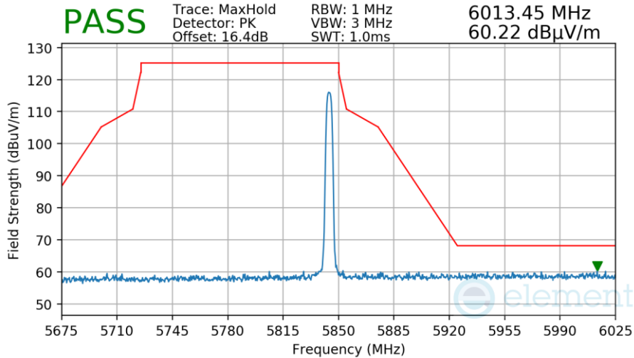
Plot 7-178. Radiated Upper Band Edge Measurement TxBF
