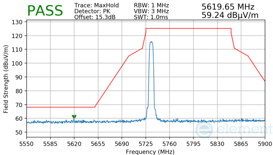
Plot 7-177. Radiated Lower Band Edge Measurement TxBF
