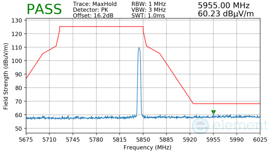
Plot 7-172. Radiated Upper Band Edge Measurement Antenna WF7a
