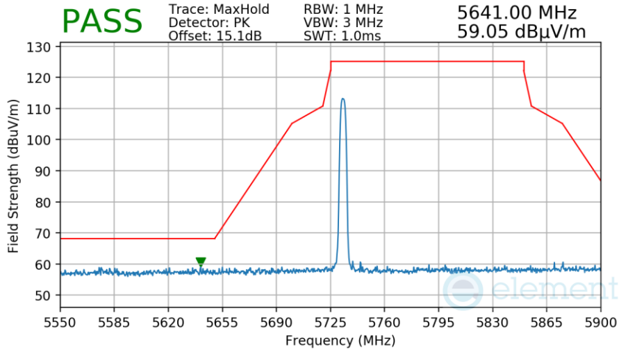
Plot 7-164. Radiated Lower Band Edge Measurement Antenna WF8
