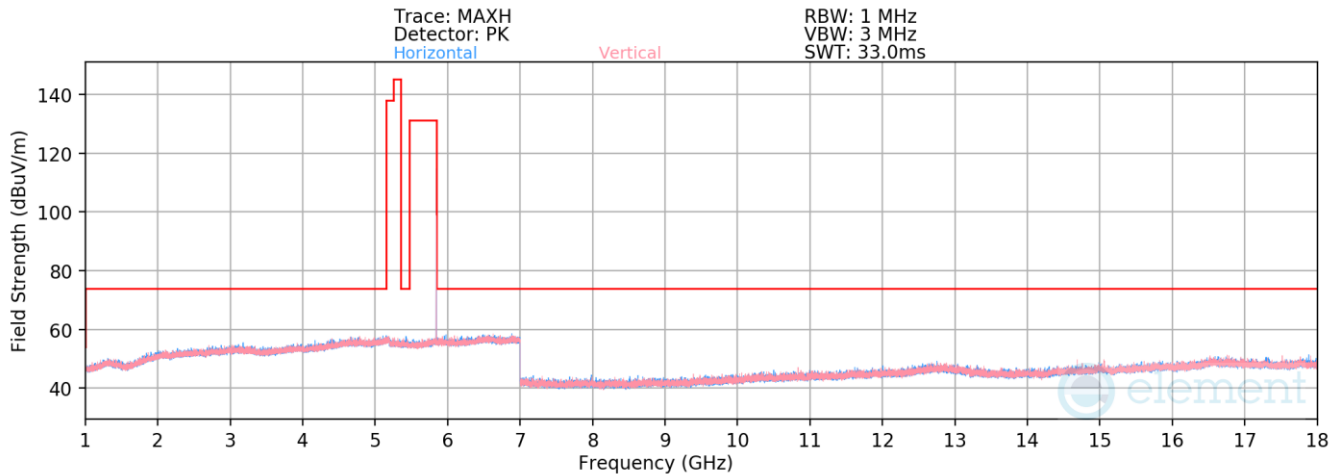
Plot 7-161. Radiated Spurious Emissions 1-18GHz TxBF (HDR4, ePA – 5844MHz)
