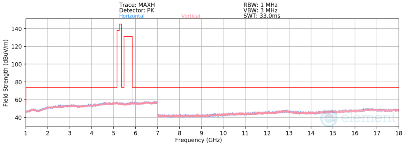
Plot 7-153. Radiated Spurious Emissions 1-18GHz Antenna WF7a (HDR4, ePA – 5844MHz)
