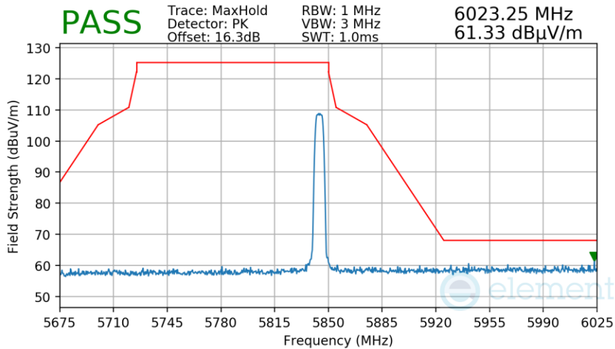
Plot 7-173. Radiated Upper Band Edge Measurement Antenna WF7a
