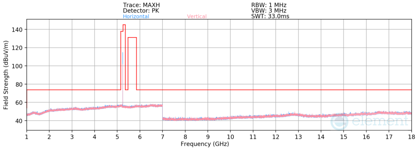
Plot 7-157. Radiated Spurious Emissions 1-18GHz TxBF (HDR4, ePA – 5245MHz)
