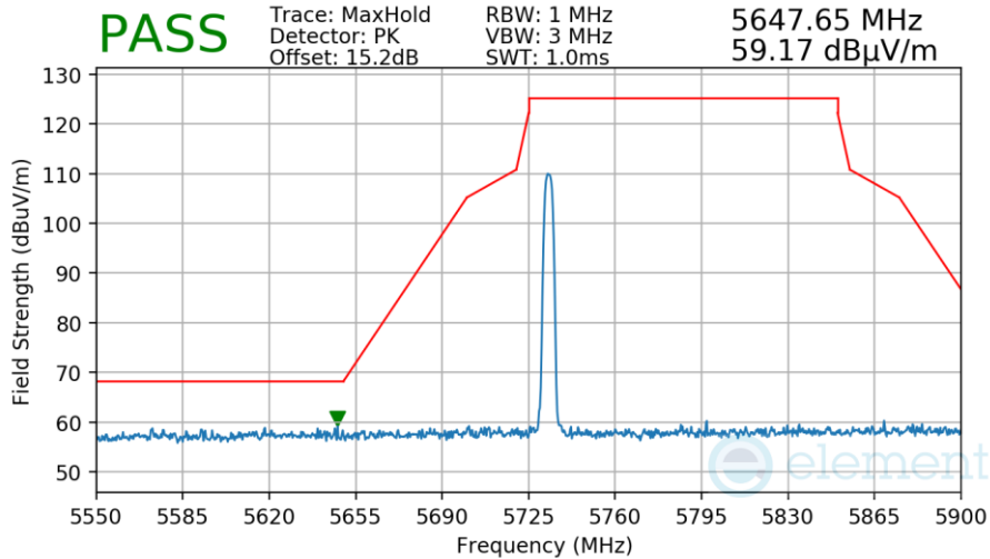
Plot 7-170. Radiated Lower Band Edge Measurement Antenna WF7a
