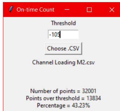
Figure 9-6. 5530MHz - Channel Loading Calculation - Mode 2 (80MHz)
