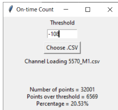
Figure 9-4. 5570MHz - Channel Loading Calculation - Mode 1 (160MHz)
