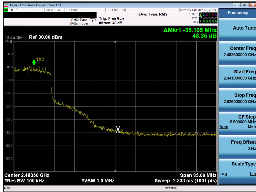
Plot 7-252. Band Edge Plot Antenna WF8 (802.11ax (SU - 2.4GHz) – Ch. 8) – MCS4
