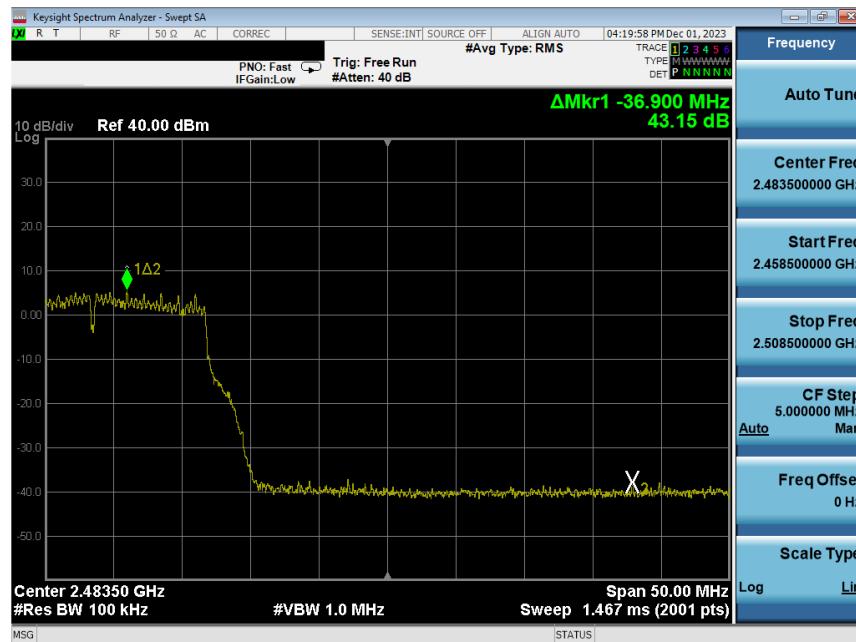
Plot 7-227. Band Edge Plot Antenna WF8 (802.11g – Ch. 11) – 24Mbps
