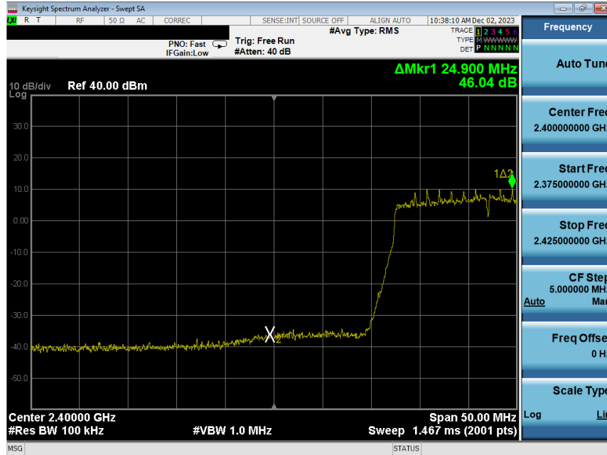
Plot 7-205. Band Edge Plot Antenna WF8 (802.11ax (SU - 2.4GHz) – Ch. 3) – MCS2
