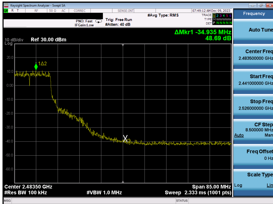
Plot 7-270. Band Edge Plot Antenna WF8 (802.11g – Ch. 8) – 54Mbps
