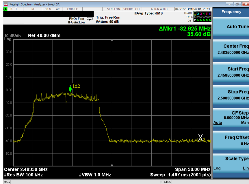
Plot 7-229. Band Edge Plot Antenna WF8 (802.11g – Ch. 13) – 24Mbps
