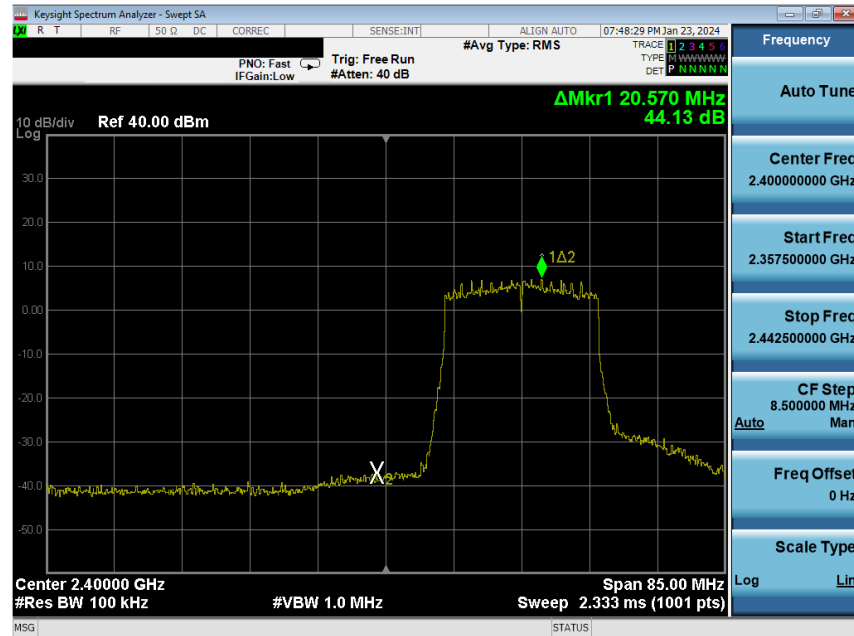
Plot 7-245. Band Edge Plot Antenna WF8 (802.11ax (SU - 2.4GHz) – Ch. 2) – MCS4
