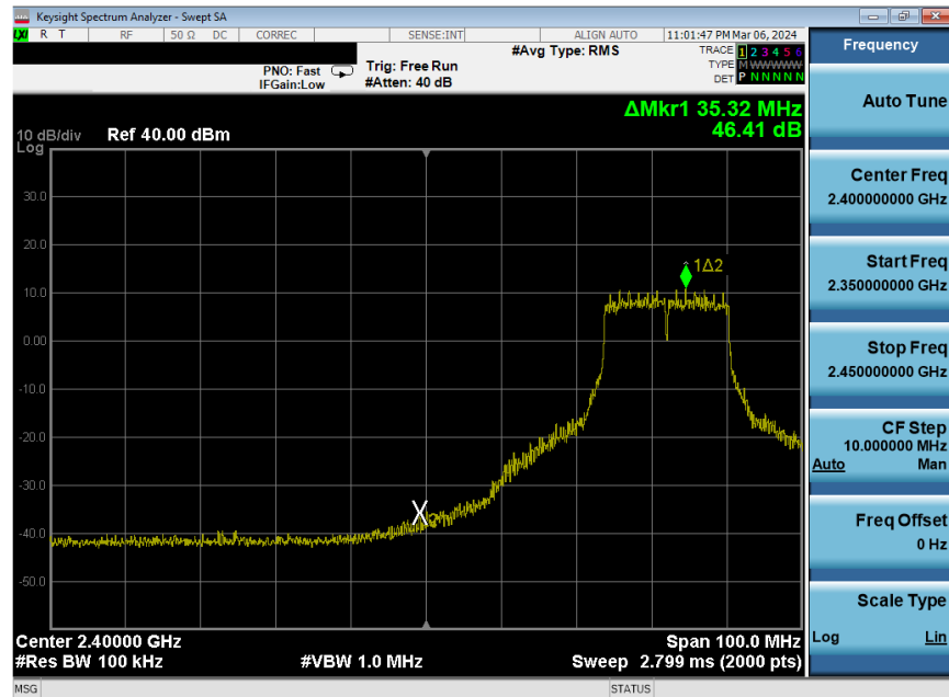
Plot 7-266. Band Edge Plot Antenna WF8 (802.11g – Ch. 5) – 54Mbps
