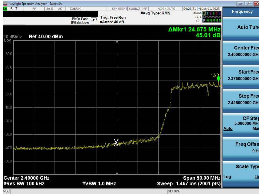
Plot 7-232. Band Edge Plot Antenna WF8 (802.11n (2.4GHz) – Ch. 3) – MCS4
