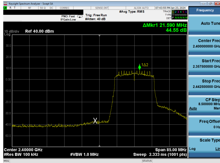
Plot 7-204. Band Edge Plot Antenna WF8 (802.11ax (SU - 2.4GHz) – Ch. 2) – MCS2
