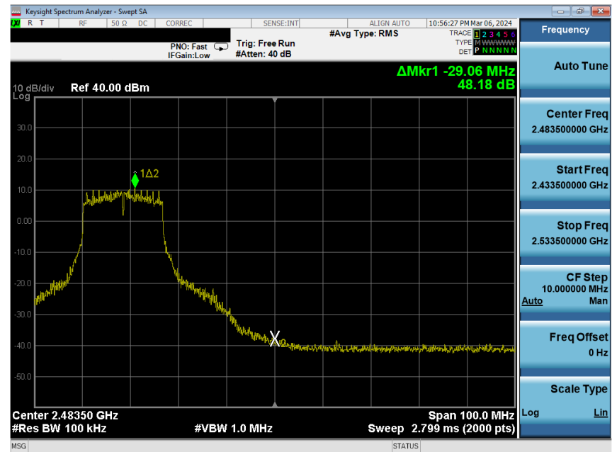
Plot 7-225. Band Edge Plot Antenna WF8 (802.11g – Ch. 9) – 24Mbps
