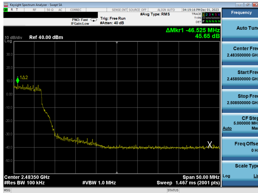
Plot 7-226. Band Edge Plot Antenna WF8 (802.11g – Ch. 10) – 24Mbps
