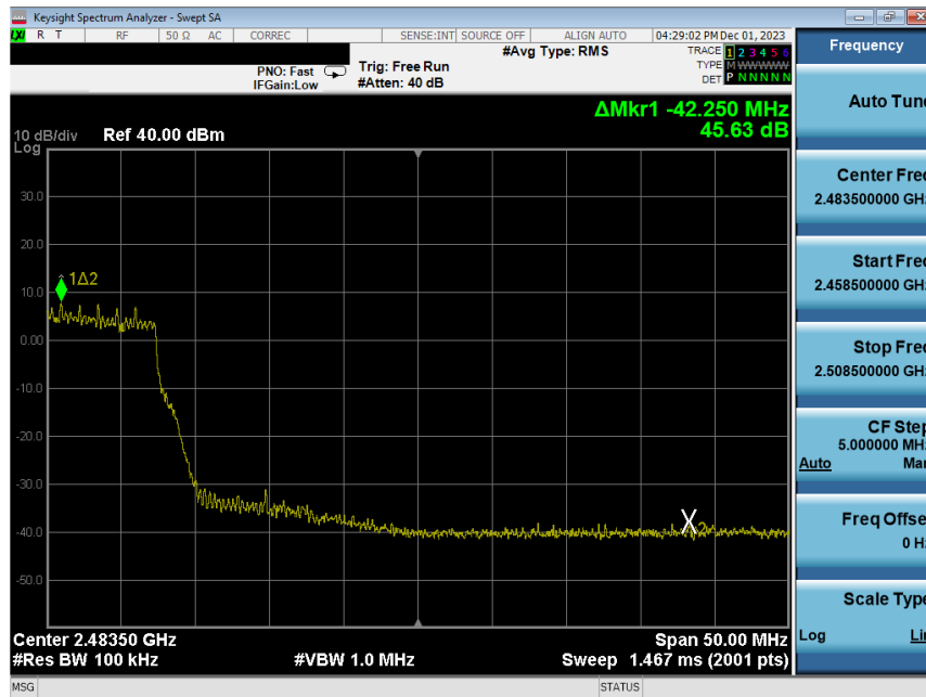
Plot 7-240. Band Edge Plot Antenna WF8 (802.11n (2.4GHz) – Ch. 10) – MCS4
