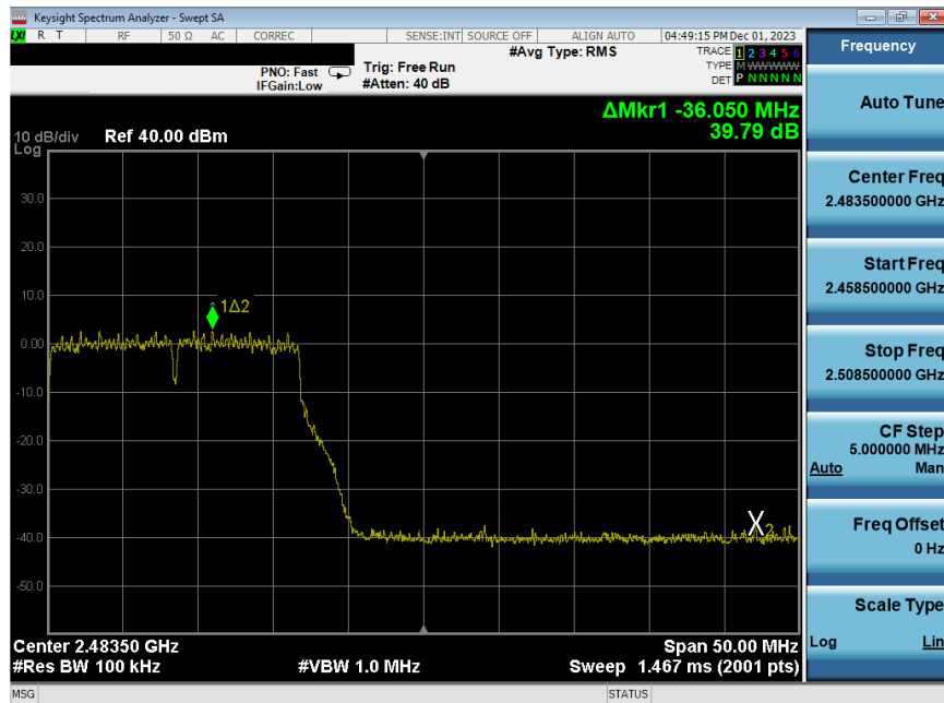
Plot 7-274. Band Edge Plot Antenna WF8 (802.11g – Ch. 12) – 54Mbps
