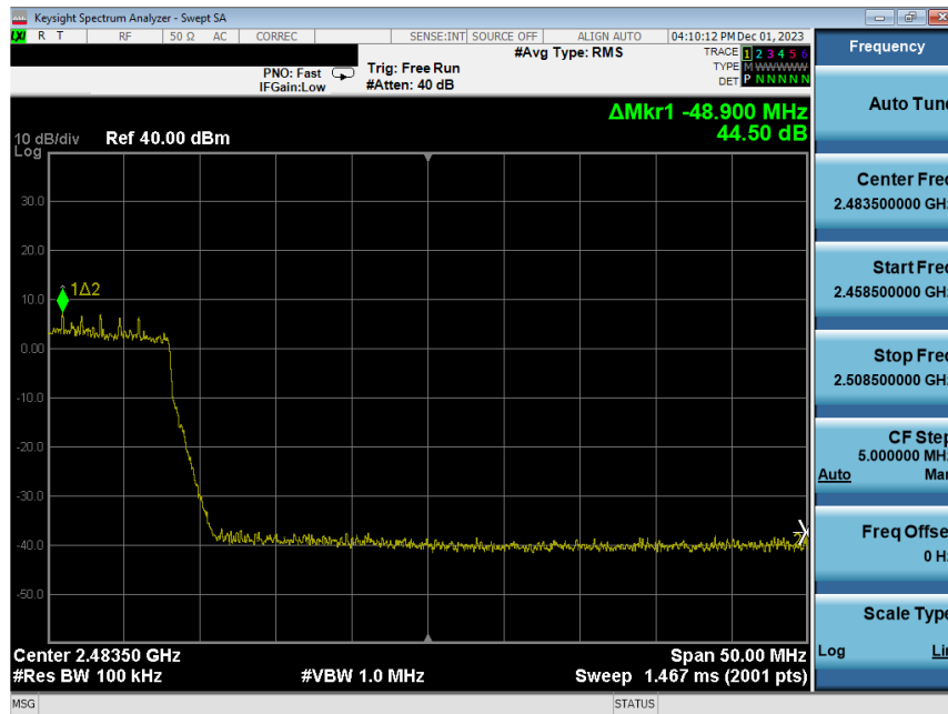
Plot 7-213. Band Edge Plot Antenna WF8 (802.11ax (SU - 2.4GHz) – Ch. 10) – MCS2
