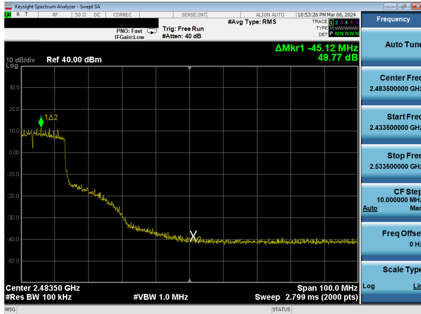
Plot 7-209. Band Edge Plot Antenna WF8 (802.11ax (SU - 2.4GHz) – Ch. 6 (high)) – MCS2
