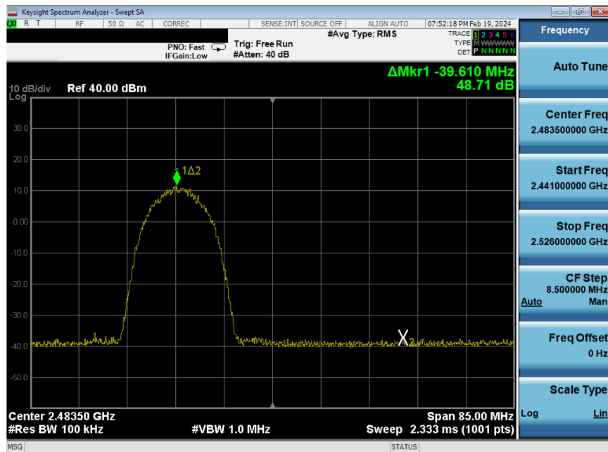
Plot 7-260. Band Edge Plot Antenna WF8 (802.11b - Ch. 12) - 11Mbps
