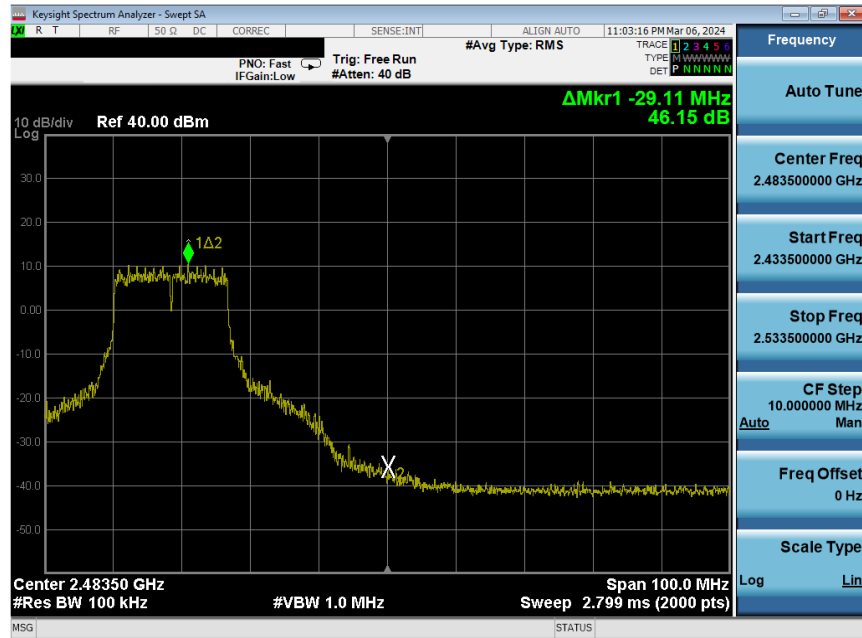
Plot 7-271. Band Edge Plot Antenna WF8 (802.11g – Ch. 9) – 54Mbps
