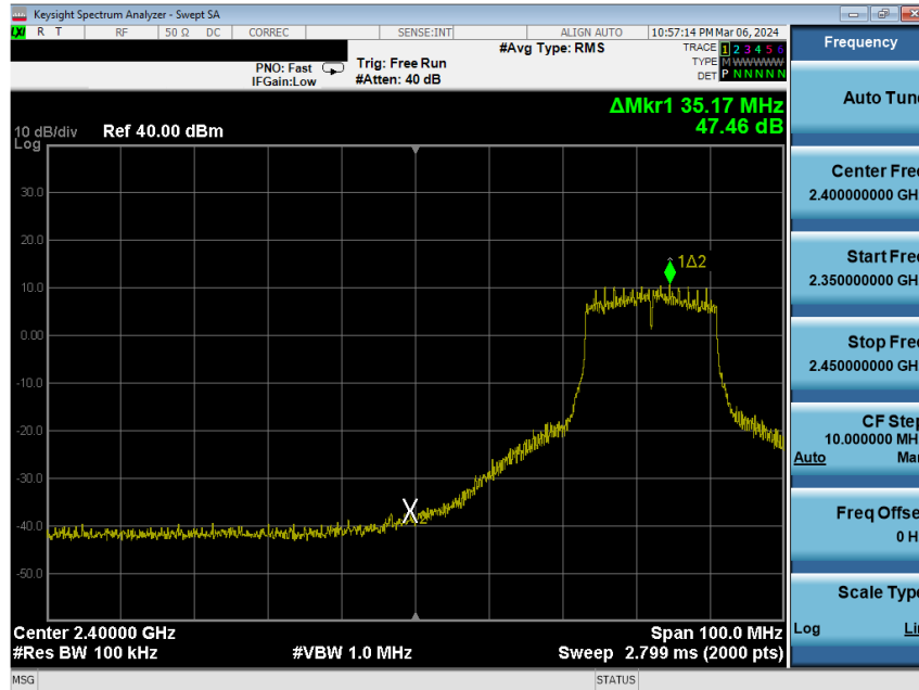
Plot 7-234. Band Edge Plot Antenna WF8 (802.11n (2.4GHz) – Ch. 5) – MCS4
