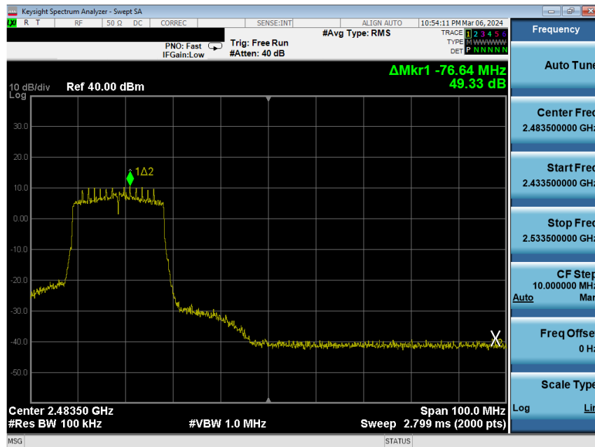
Plot 7-212. Band Edge Plot Antenna WF8 (802.11ax (SU - 2.4GHz) – Ch. 9) – MCS2
