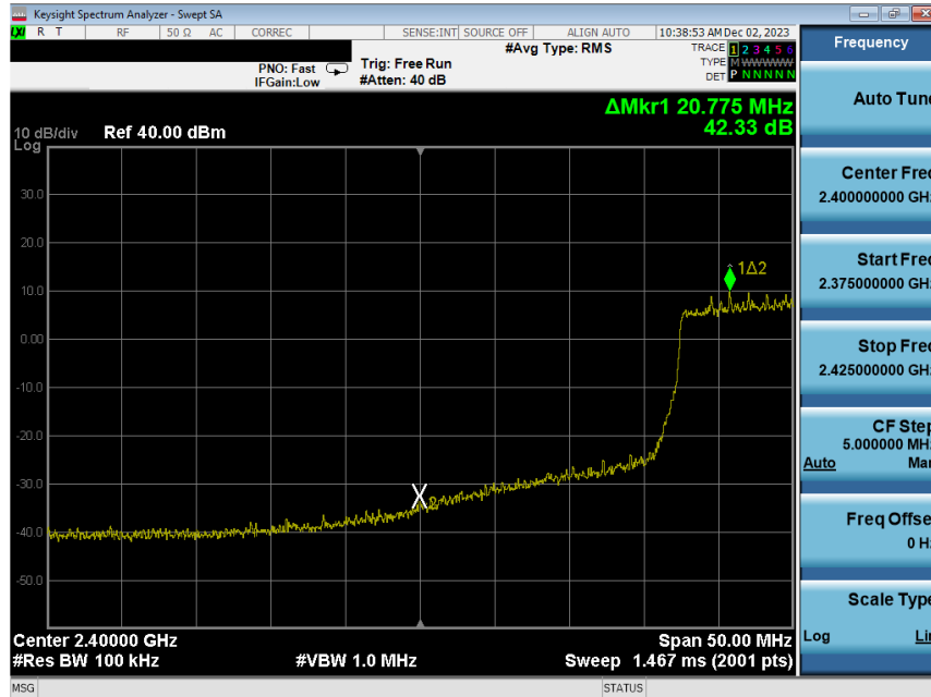
Plot 7-206. Band Edge Plot Antenna WF8 (802.11ax (SU - 2.4GHz) – Ch. 4) – MCS2
