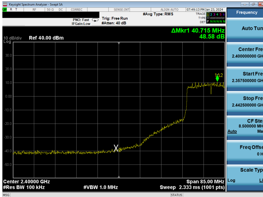
Plot 7-249. Band Edge Plot Antenna WF8 (802.11ax (SU - 2.4GHz) – Ch. 6 (low)) – MCS4
