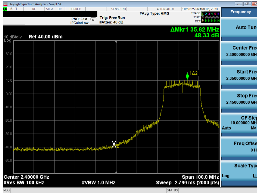
Plot 7-193. Band Edge Plot Antenna WF8 (802.11n (2.4GHz) – Ch. 5) – MCS2
