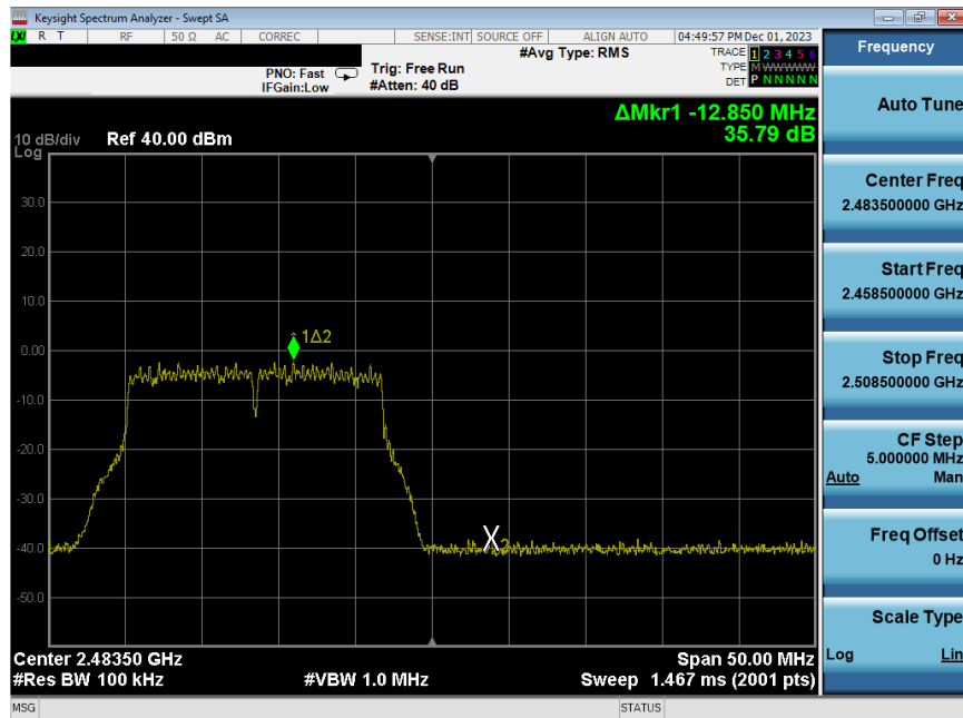
Plot 7-275. Band Edge Plot Antenna WF8 (802.11g – Ch. 13) – 54Mbps
