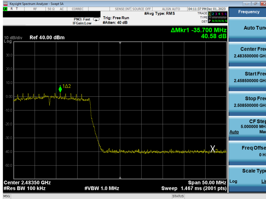
Plot 7-215. Band Edge Plot Antenna WF8 (802.11ax (SU - 2.4GHz) – Ch. 12) – MCS2
