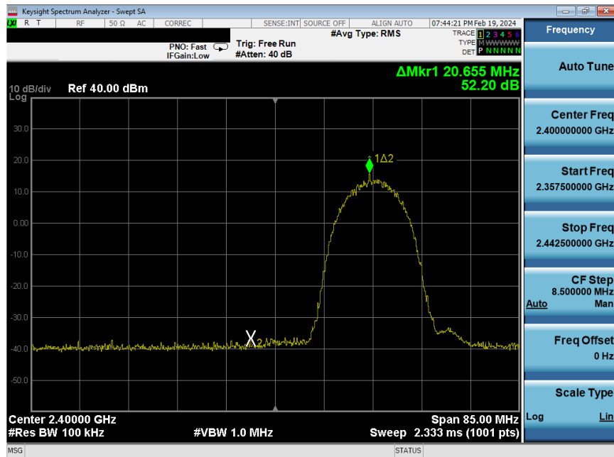
Plot 7-258. Band Edge Plot Antenna WF8 (802.11b – Ch. 2) – 11Mbps
