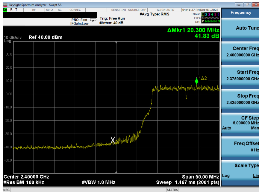
Plot 7-263. Band Edge Plot Antenna WF8 (802.11g – Ch. 2) – 54Mbps
