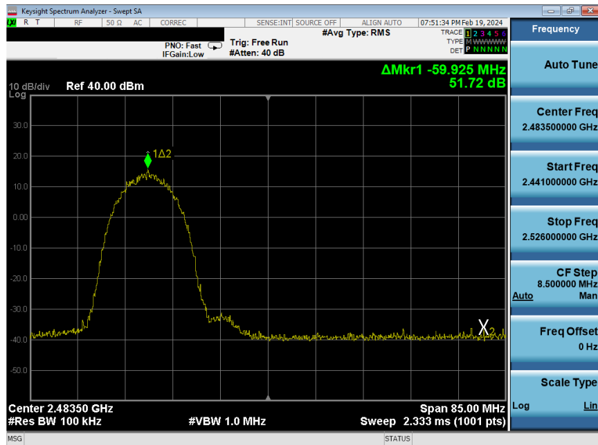
Plot 7-259. Band Edge Plot Antenna WF8 (802.11b - Ch. 11) - 11Mbps
