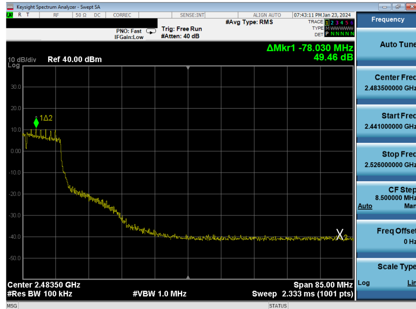
Plot 7-196. Band Edge Plot Antenna WF8 (802.11n (2.4GHz) – Ch. 7) – MCS2
