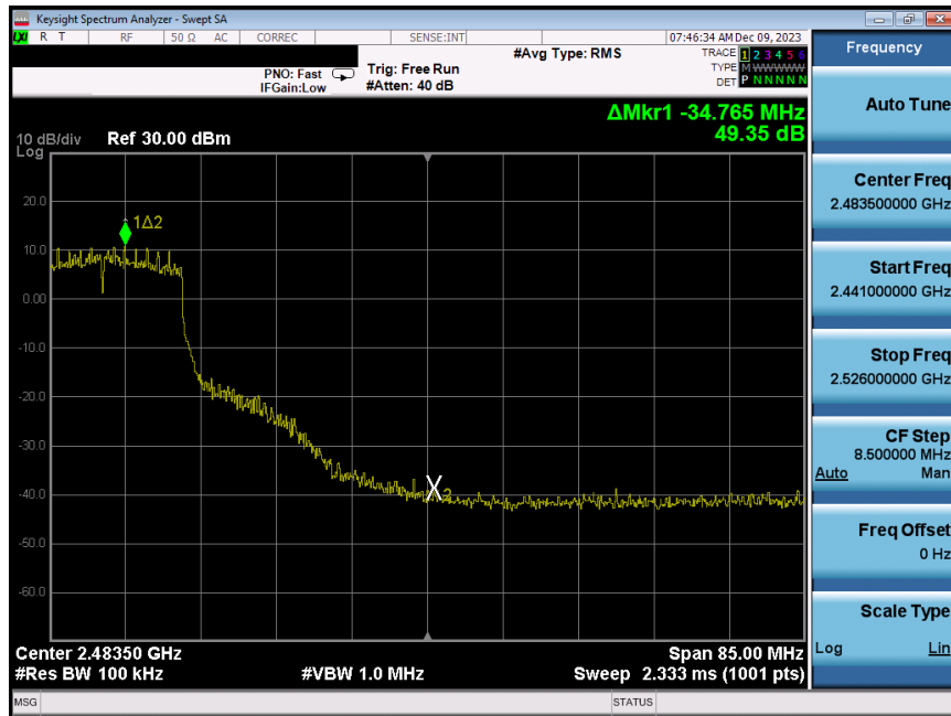
Plot 7-238. Band Edge Plot Antenna WF8 (802.11n (2.4GHz) – Ch. 8) – MCS4
