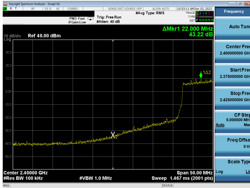
Plot 7-247. Band Edge Plot Antenna WF8 (802.11ax (SU - 2.4GHz) – Ch. 4) – MCS4
