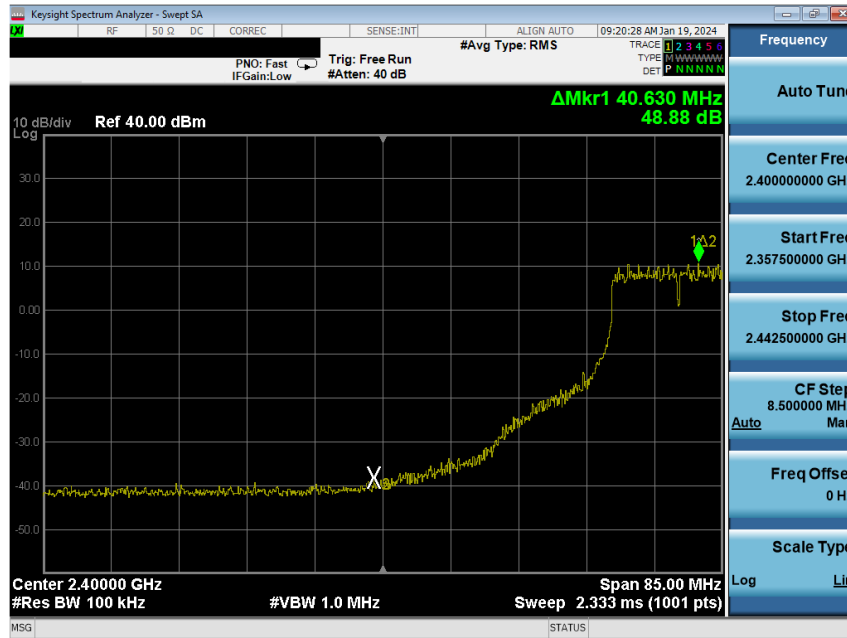
Plot 7-267. Band Edge Plot Antenna WF8 (802.11g – Ch. 6 (low)) – 54Mbps
