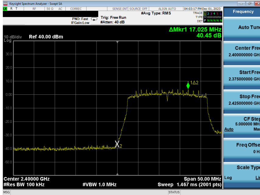
Plot 7-203. Band Edge Plot Antenna WF8 (802.11ax (SU - 2.4GHz) – Ch. 1) – MCS2
