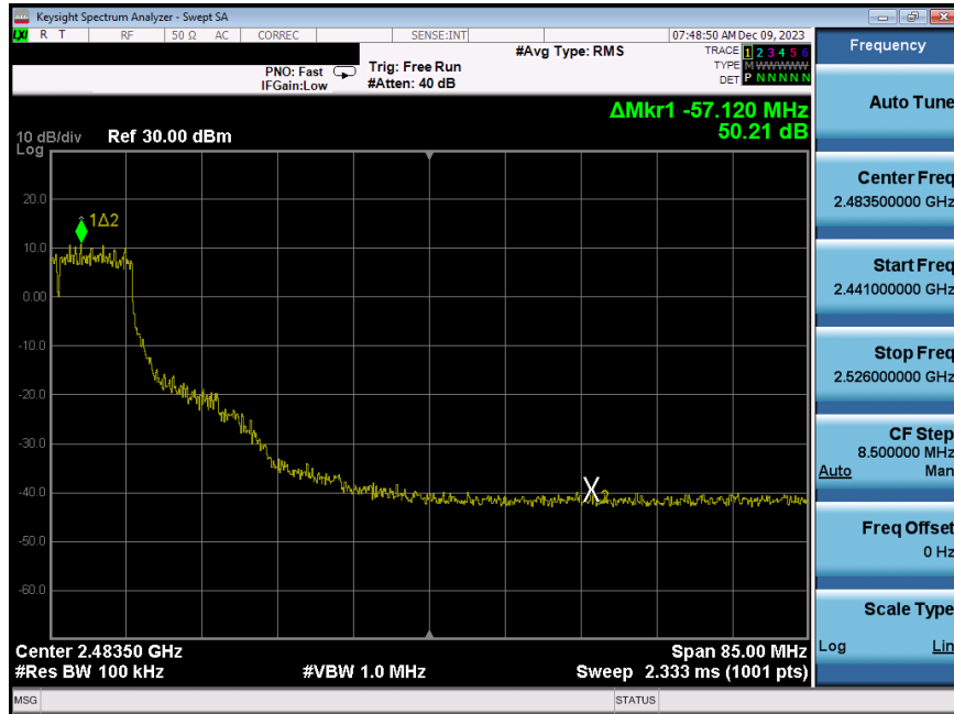
Plot 7-269. Band Edge Plot Antenna WF8 (802.11g – Ch. 7) – 54Mbps
