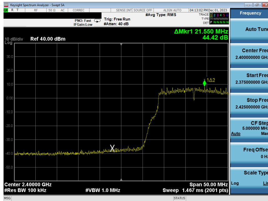
Plot 7-217. Band Edge Plot Antenna WF8 (802.11g – Ch. 2) – 24Mbps
