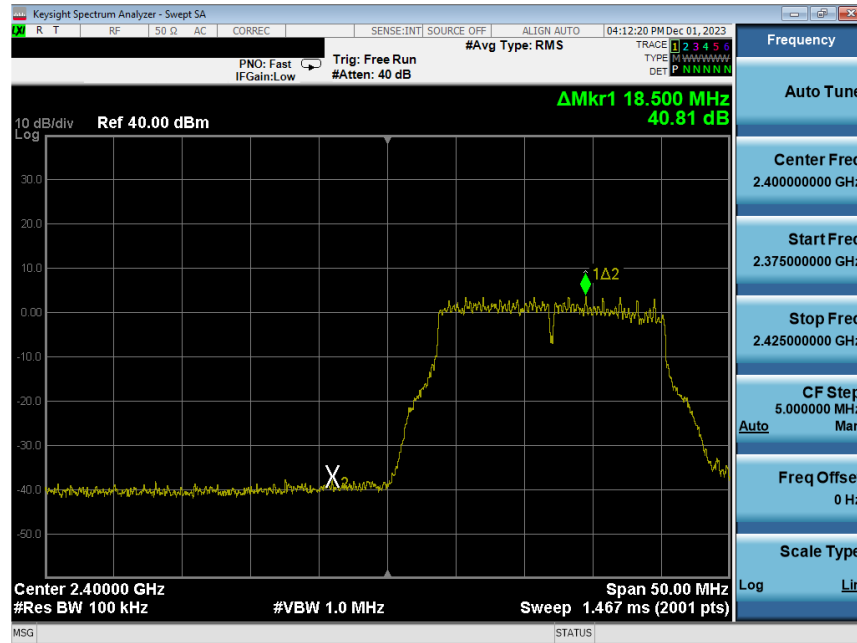
Plot 7-216. Band Edge Plot Antenna WF8 (802.11g – Ch. 1) – 24Mbps
