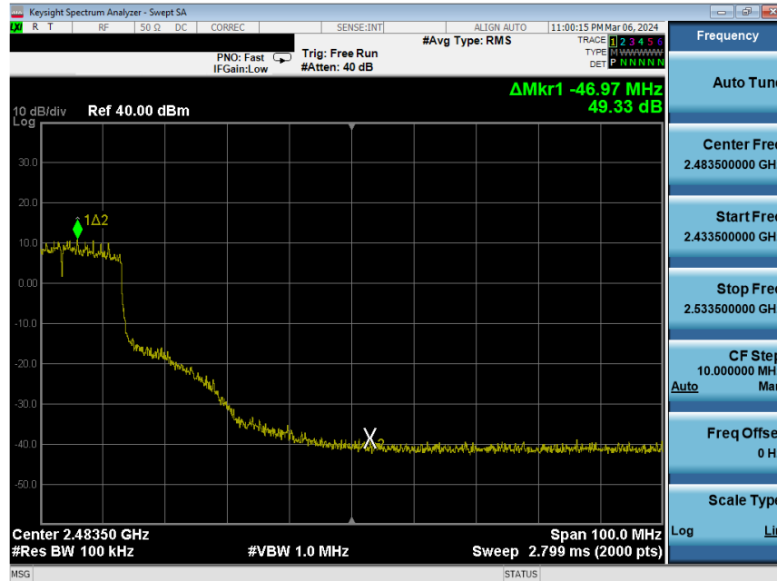
Plot 7-250. Band Edge Plot Antenna WF8 (802.11ax (SU - 2.4GHz) – Ch. 6 (high)) – MCS4
