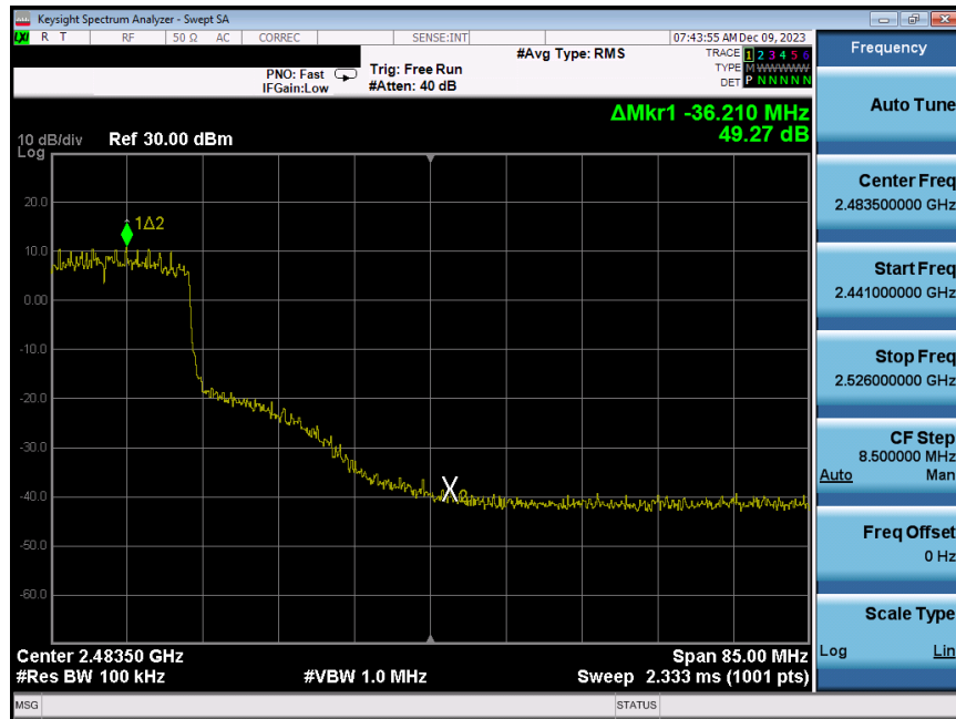
Plot 7-211. Band Edge Plot Antenna WF8 (802.11ax (SU - 2.4GHz) – Ch. 8) – MCS2
