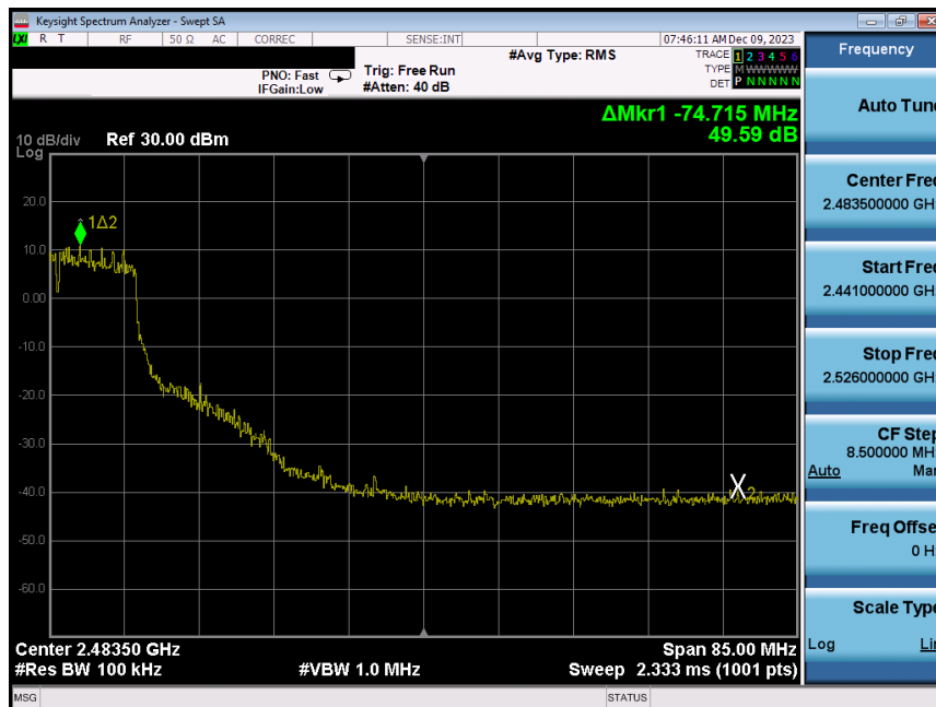
Plot 7-237. Band Edge Plot Antenna WF8 (802.11n (2.4GHz) – Ch. 7) – MCS4
