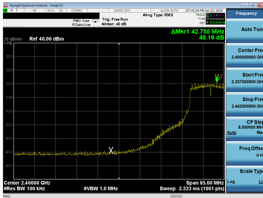
Plot 7-221. Band Edge Plot Antenna WF8 (802.11g – Ch. 6 (low)) – 24Mbps
