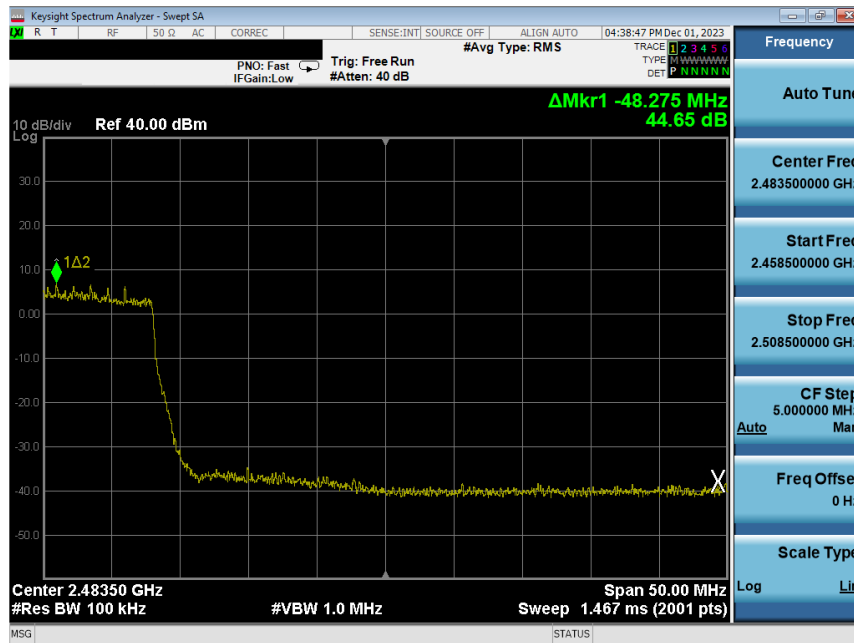
Plot 7-254. Band Edge Plot Antenna WF8 (802.11ax (SU - 2.4GHz) – Ch. 10) – MCS4
