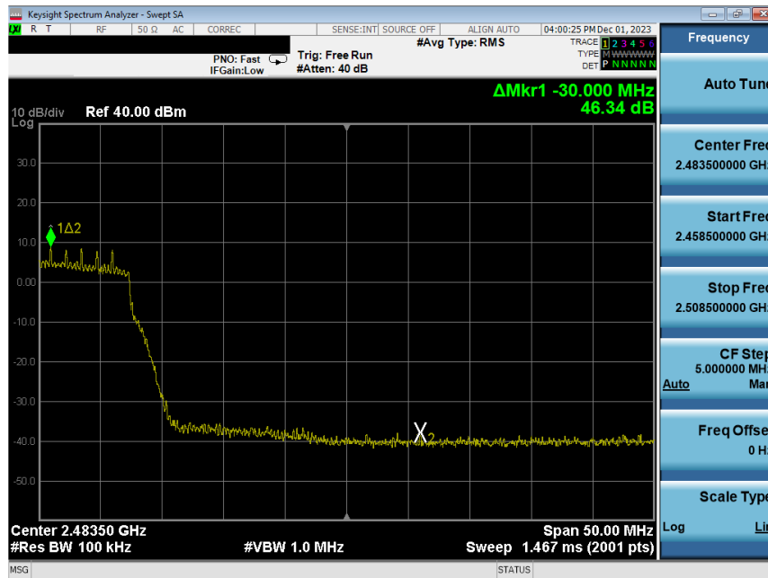
Plot 7-199. Band Edge Plot Antenna WF8 (802.11n (2.4GHz) – Ch. 10) – MCS2
