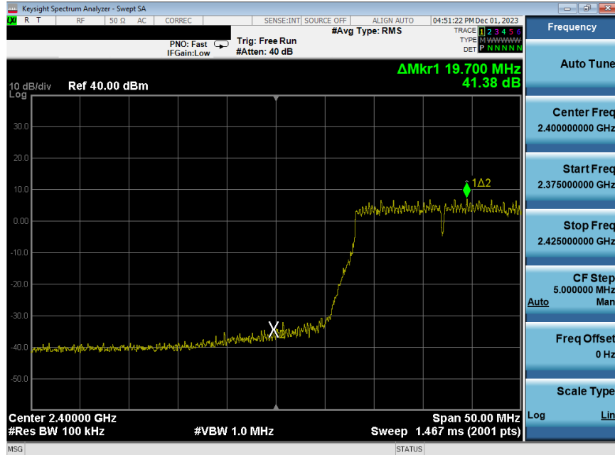
Plot 7-277. Band Edge Plot Antenna WF8 (802.11n (2.4GHz) – Ch. 2) – MCS7
