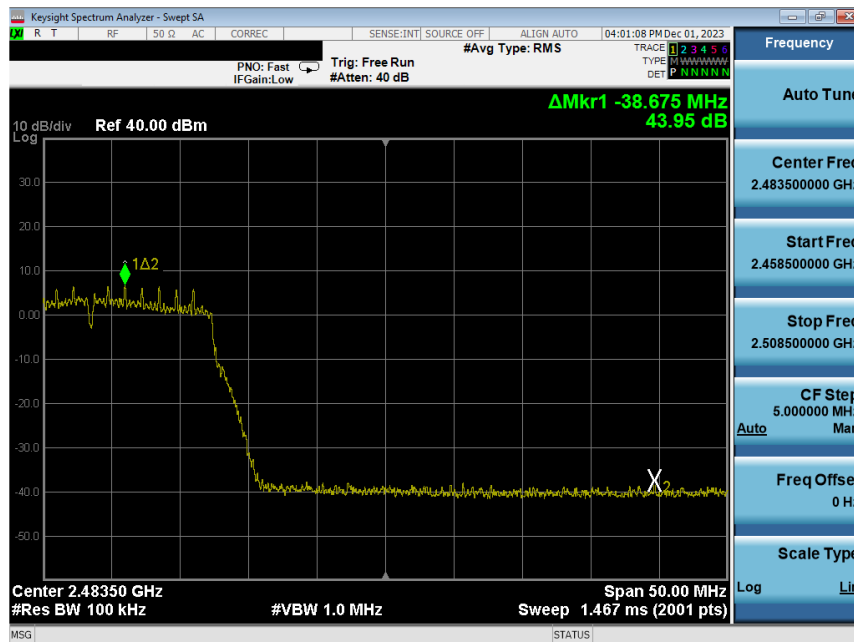
Plot 7-200. Band Edge Plot Antenna WF8 (802.11n (2.4GHz) – Ch. 11) – MCS2
