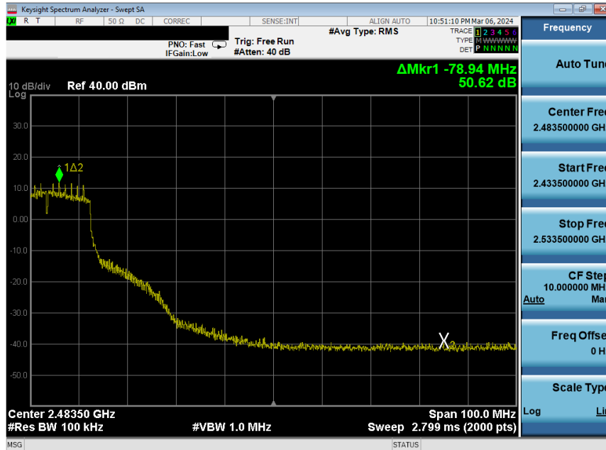
Plot 7-195. Band Edge Plot Antenna WF8 (802.11n (2.4GHz) – Ch. 6 (high)) – MCS2
