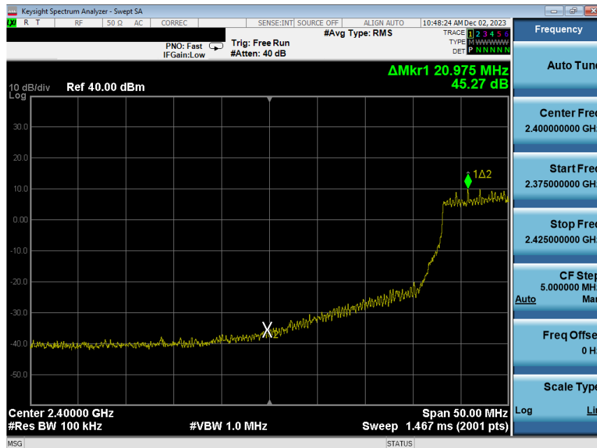
Plot 7-233. Band Edge Plot Antenna WF8 (802.11n (2.4GHz) – Ch. 4) – MCS4
