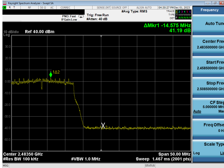
Plot 7-242. Band Edge Plot Antenna WF8 (802.11n (2.4GHz) – Ch. 12) – MCS4
