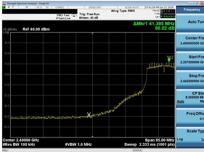
Plot 7-194. Band Edge Plot Antenna WF8 (802.11n (2.4GHz) – Ch. 6(low)) – MCS2
