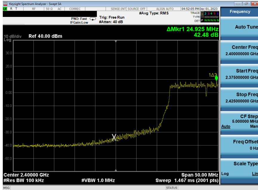
Plot 7-278. Band Edge Plot Antenna WF8 (802.11n (2.4GHz) – Ch. 3) – MCS7
