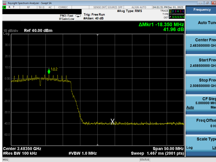
Plot 7-201. Band Edge Plot Antenna WF8 (802.11n (2.4GHz) – Ch. 12) – MCS2
