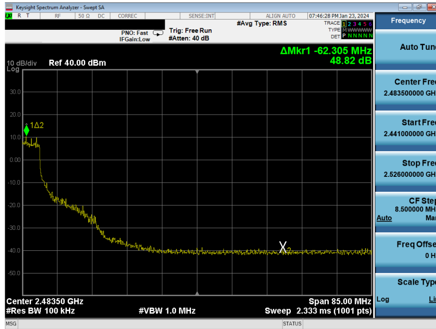
Plot 7-222. Band Edge Plot Antenna WF8 (802.11g – Ch. 6 (high)) – 24Mbps
