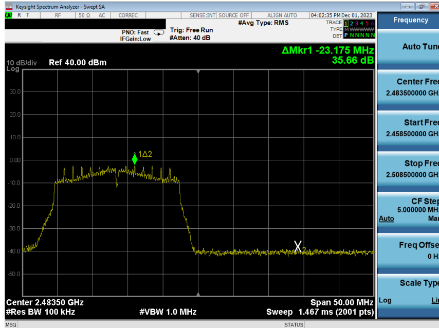
Plot 7-202. Band Edge Plot Antenna WF8 (802.11n (2.4GHz) – Ch. 13) – MCS2
