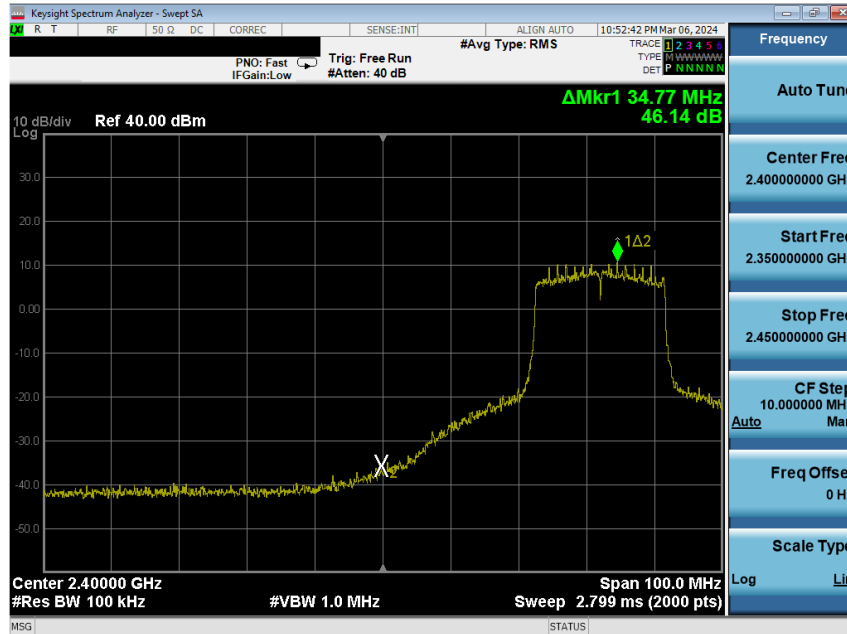
Plot 7-207. Band Edge Plot Antenna WF8 (802.11ax (SU - 2.4GHz) – Ch. 5) – MCS2
