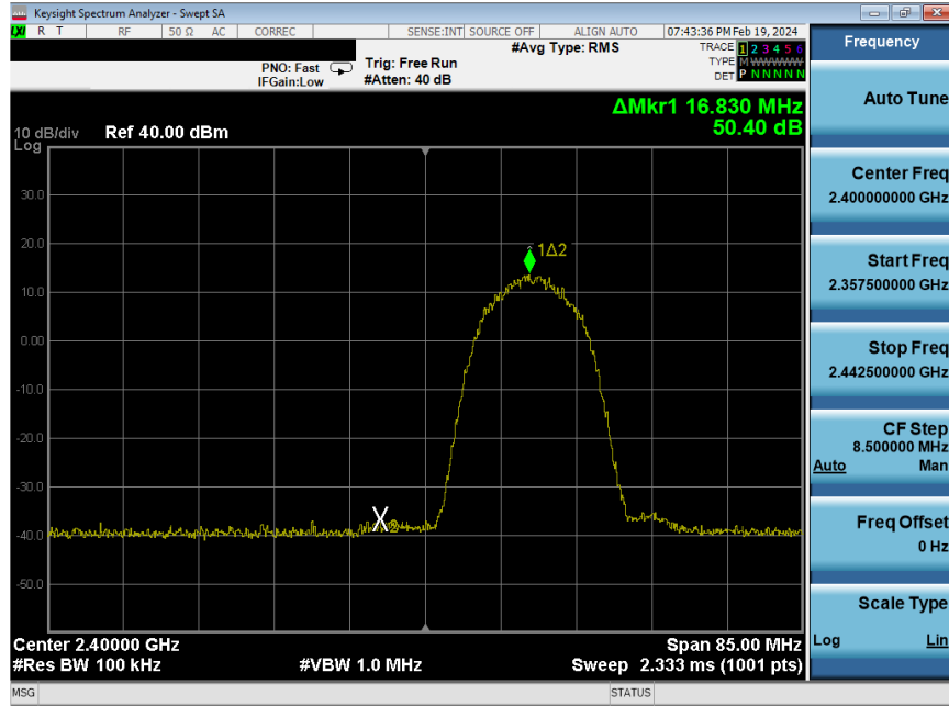
Plot 7-257. Band Edge Plot Antenna WF8 (802.11b – Ch. 1) – 11Mbps
