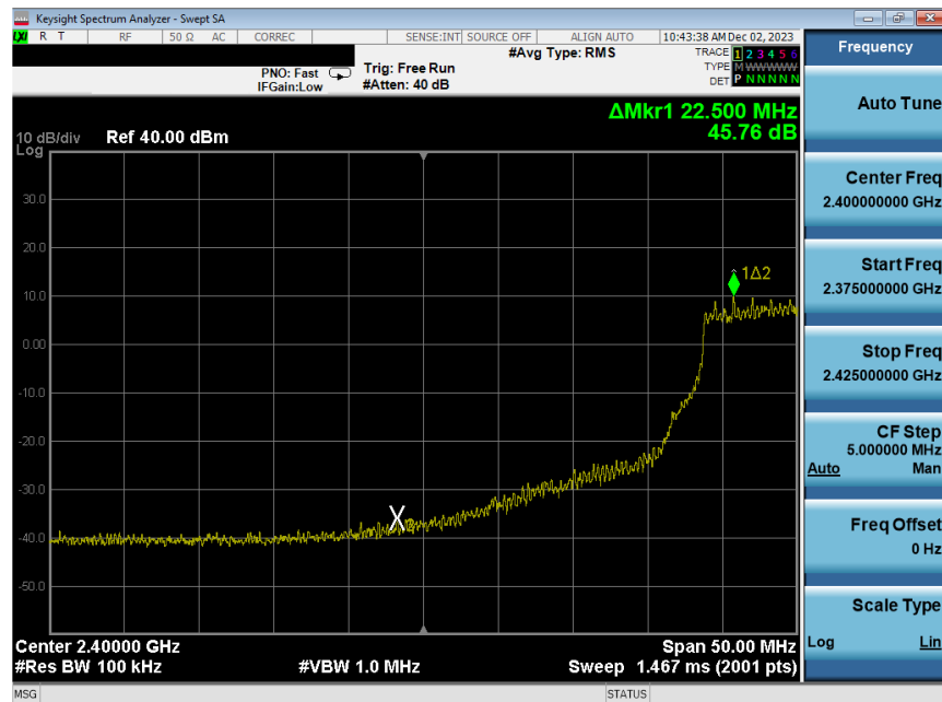
Plot 7-219. Band Edge Plot Antenna WF8 (802.11g – Ch. 4) – 24Mbps
