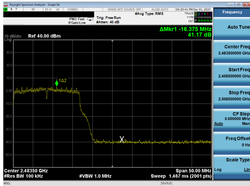
Plot 7-228. Band Edge Plot Antenna WF8 (802.11g – Ch. 12) – 24Mbps
