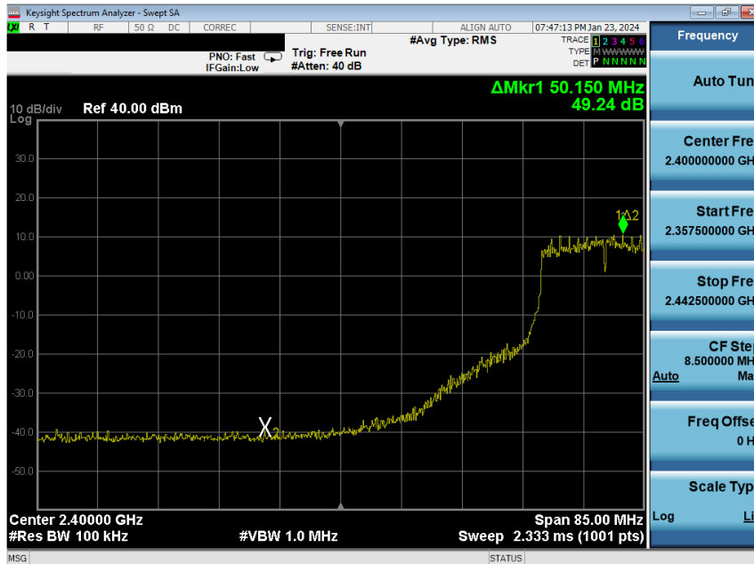
Plot 7-235. Band Edge Plot Antenna WF8 (802.11n (2.4GHz) – Ch. 6(low)) – MCS4
