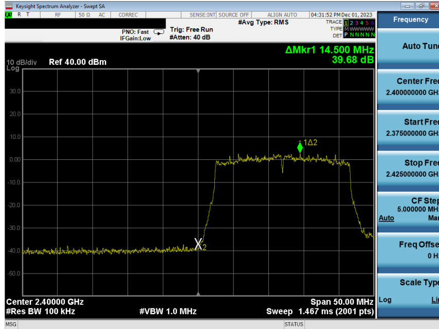
Plot 7-244. Band Edge Plot Antenna WF8 (802.11ax (SU - 2.4GHz) – Ch. 1) – MCS4
