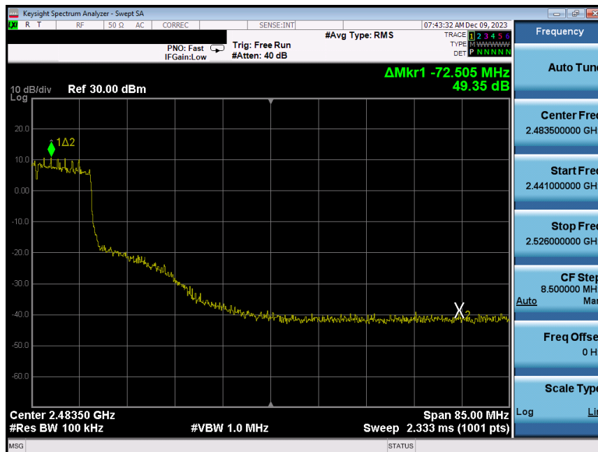
Plot 7-210. Band Edge Plot Antenna WF8 (802.11ax (SU - 2.4GHz) – Ch. 7) – MCS2
