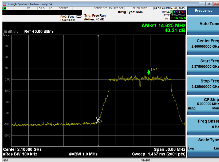
Plot 7-276. Band Edge Plot Antenna WF8 (802.11n (2.4GHz) – Ch. 1) – MCS7
