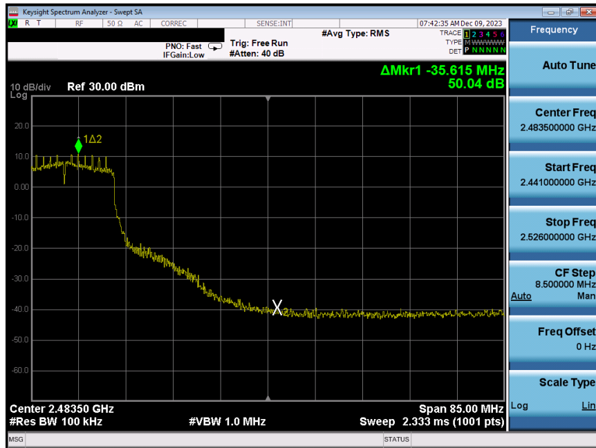
Plot 7-197. Band Edge Plot Antenna WF8 (802.11n (2.4GHz) – Ch. 8) – MCS2
