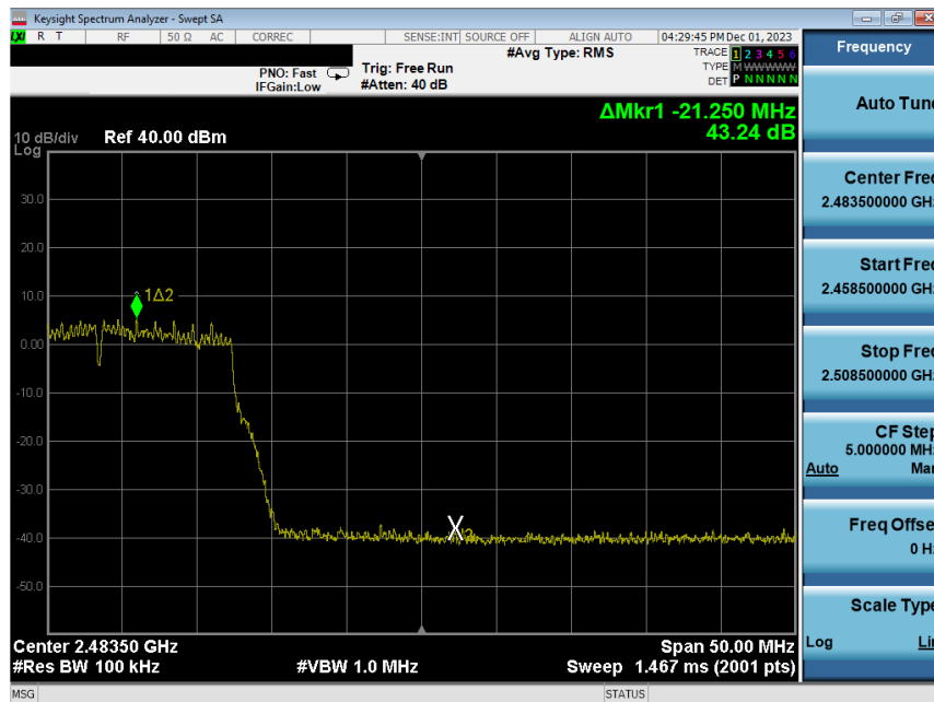
Plot 7-241. Band Edge Plot Antenna WF8 (802.11n (2.4GHz) – Ch. 11) – MCS4
