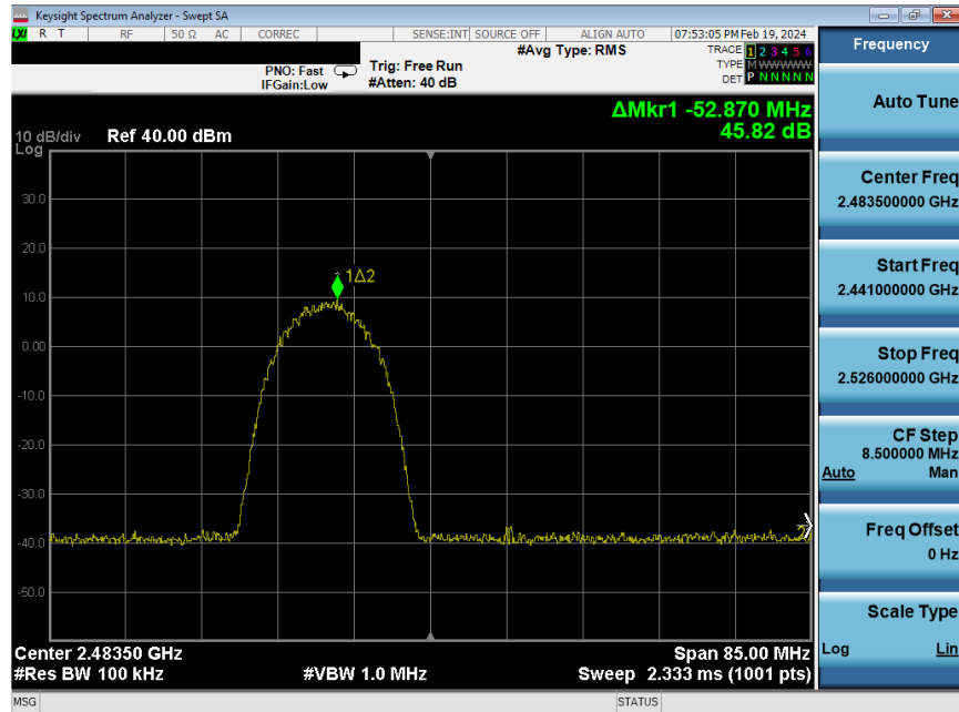
Plot 7-261. Band Edge Plot Antenna WF8 (802.11b – Ch. 13) – 11Mbps
