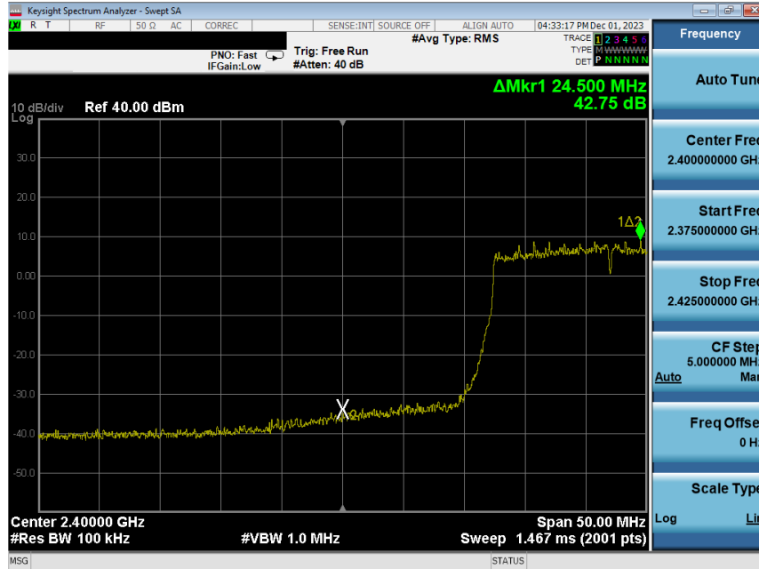
Plot 7-246. Band Edge Plot Antenna WF8 (802.11ax (SU - 2.4GHz) – Ch. 3) – MCS4
