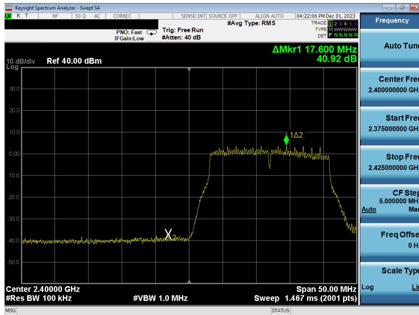
Plot 7-230. Band Edge Plot Antenna WF8 (802.11n (2.4GHz) – Ch. 1) – MCS4
