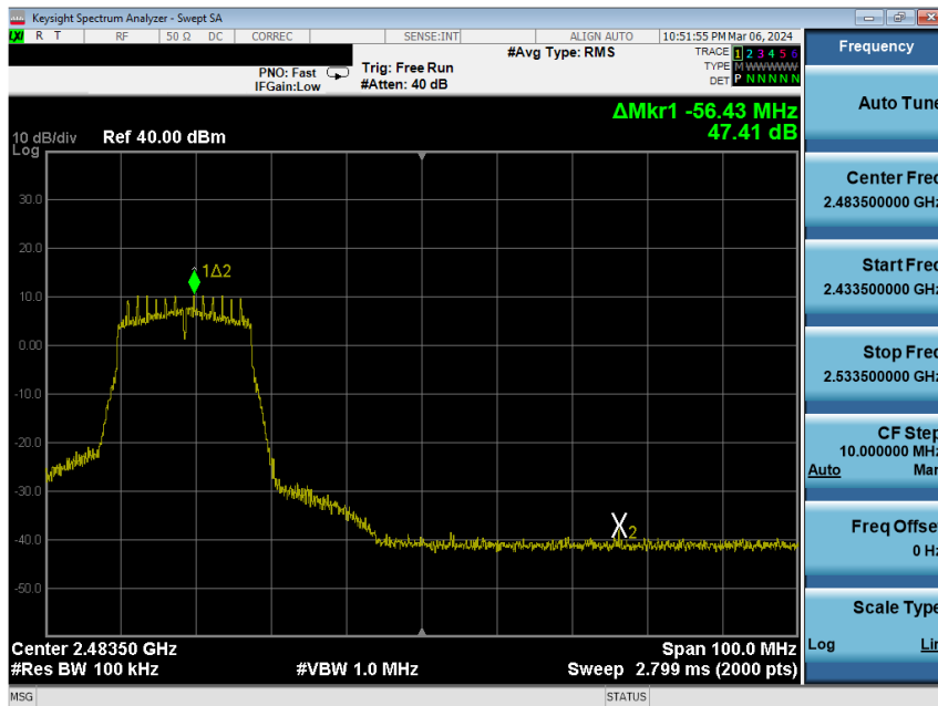
Plot 7-198. Band Edge Plot Antenna WF8 (802.11n (2.4GHz) – Ch. 9) – MCS2
