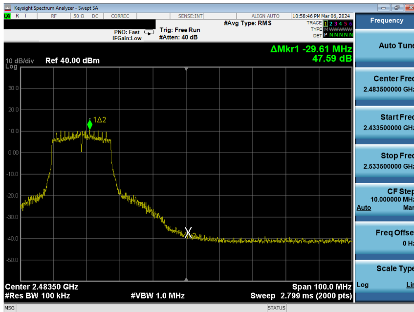
Plot 7-239. Band Edge Plot Antenna WF8 (802.11n (2.4GHz) – Ch. 9) – MCS4
