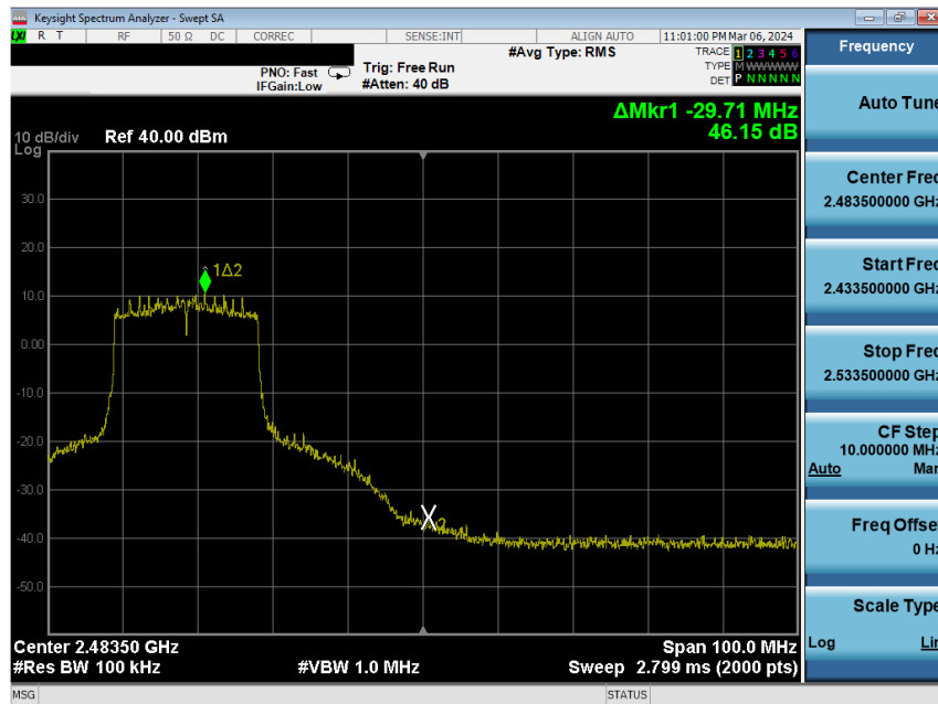
Plot 7-253. Band Edge Plot Antenna WF8 (802.11ax (SU - 2.4GHz) – Ch. 9) – MCS4
