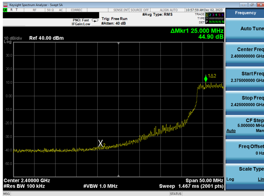
Plot 7-265. Band Edge Plot Antenna WF8 (802.11g – Ch. 4) – 54Mbps
