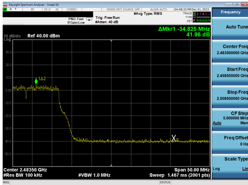
Plot 7-273. Band Edge Plot Antenna WF8 (802.11g – Ch. 11) – 54Mbps
