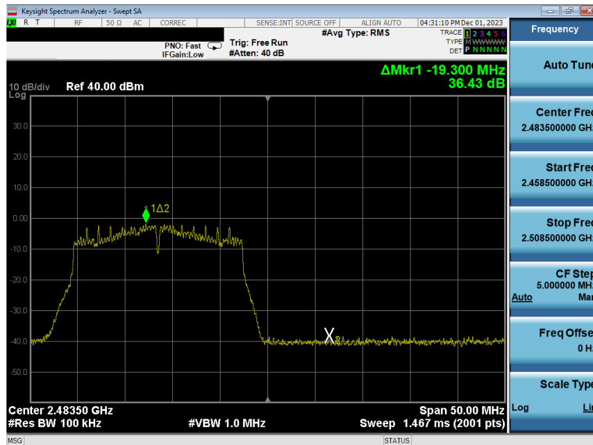
Plot 7-243. Band Edge Plot Antenna WF8 (802.11n (2.4GHz) – Ch. 13) – MCS4
