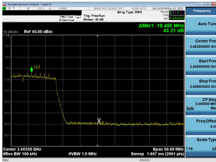
Plot 7-214. Band Edge Plot Antenna WF8 (802.11ax (SU - 2.4GHz) – Ch. 11) – MCS2
