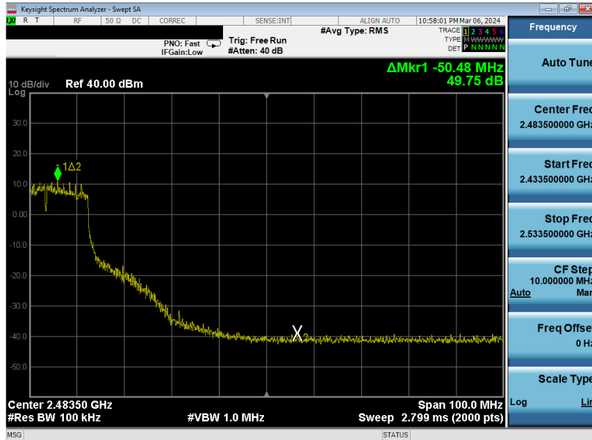
Plot 7-236. Band Edge Plot Antenna WF8 (802.11n (2.4GHz) – Ch. 6 (high)) – MCS4
