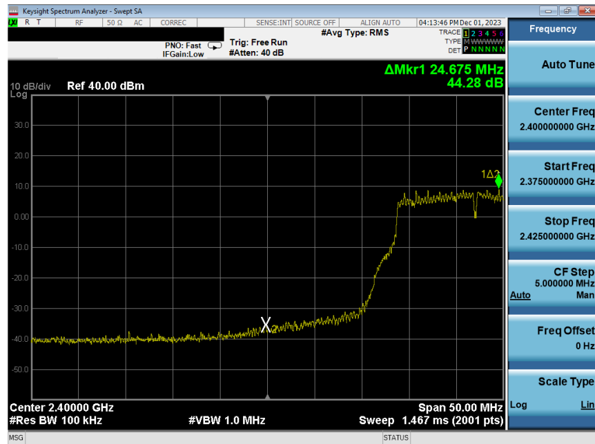
Plot 7-218. Band Edge Plot Antenna WF8 (802.11g – Ch. 3) – 24Mbps
