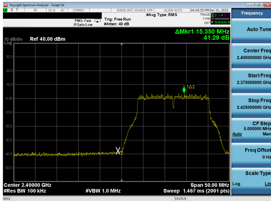
Plot 7-262. Band Edge Plot Antenna WF8 (802.11g – Ch. 1) – 54Mbps
