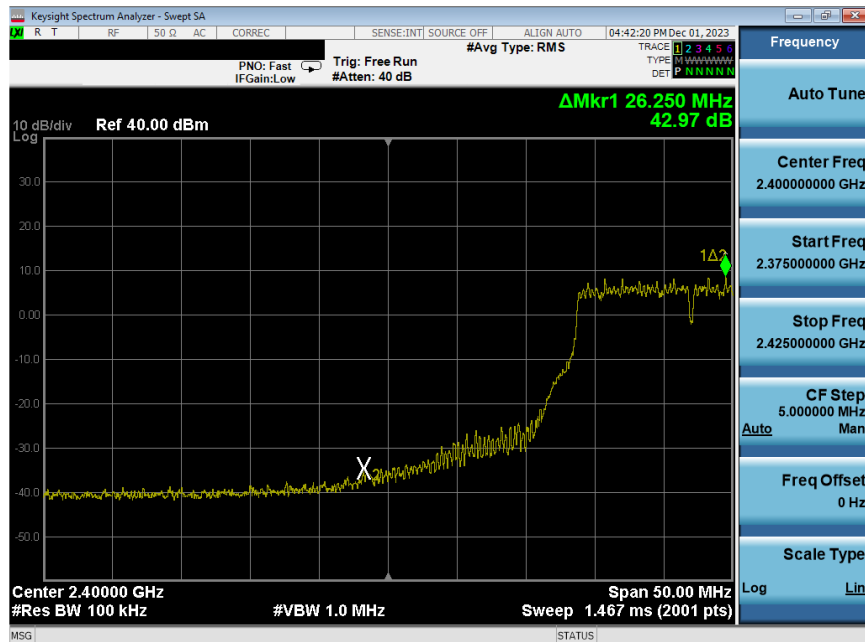
Plot 7-264. Band Edge Plot Antenna WF8 (802.11g – Ch. 3) – 54Mbps
