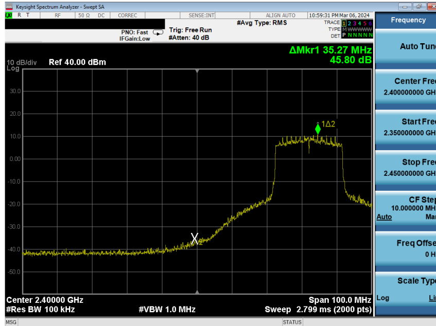
Plot 7-248. Band Edge Plot Antenna WF8 (802.11ax (SU - 2.4GHz) – Ch. 5) – MCS4
