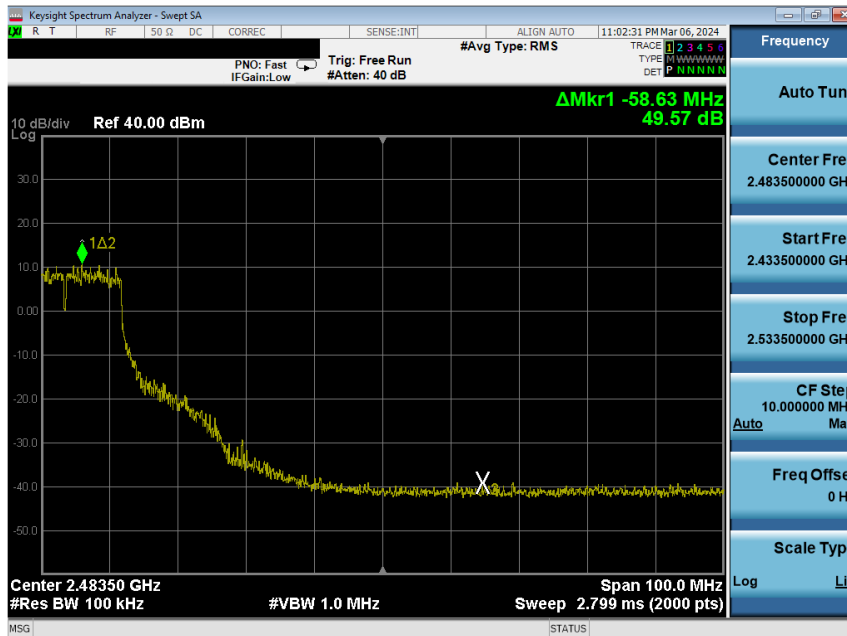
Plot 7-268. Band Edge Plot Antenna WF8 (802.11g – Ch. 6 (high)) – 54Mbps
