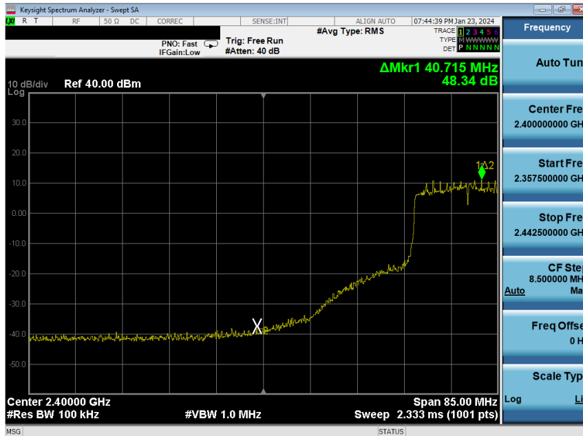
Plot 7-208. Band Edge Plot Antenna WF8 (802.11ax (SU - 2.4GHz) – Ch. 6 (low)) – MCS2
