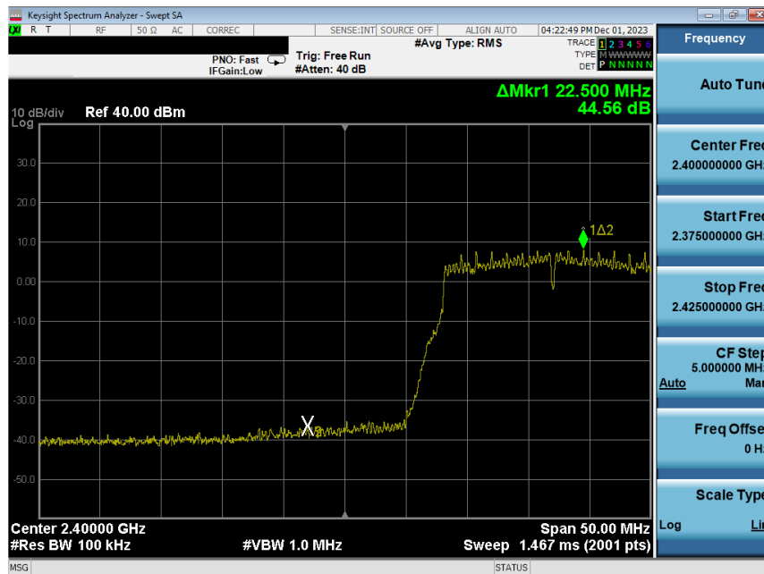
Plot 7-231. Band Edge Plot Antenna WF8 (802.11n (2.4GHz) – Ch. 2) – MCS4
