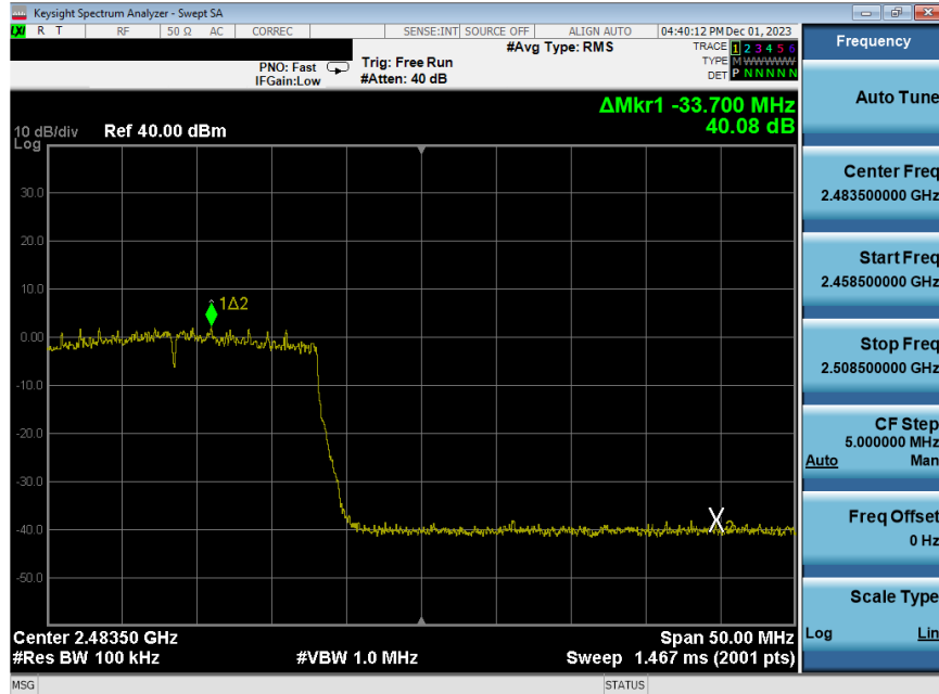
Plot 7-256. Band Edge Plot Antenna WF8 (802.11ax (SU - 2.4GHz) – Ch. 12) – MCS4
