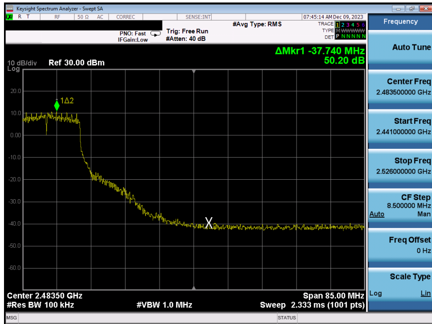
Plot 7-224. Band Edge Plot Antenna WF8 (802.11g – Ch. 8) – 24Mbps
