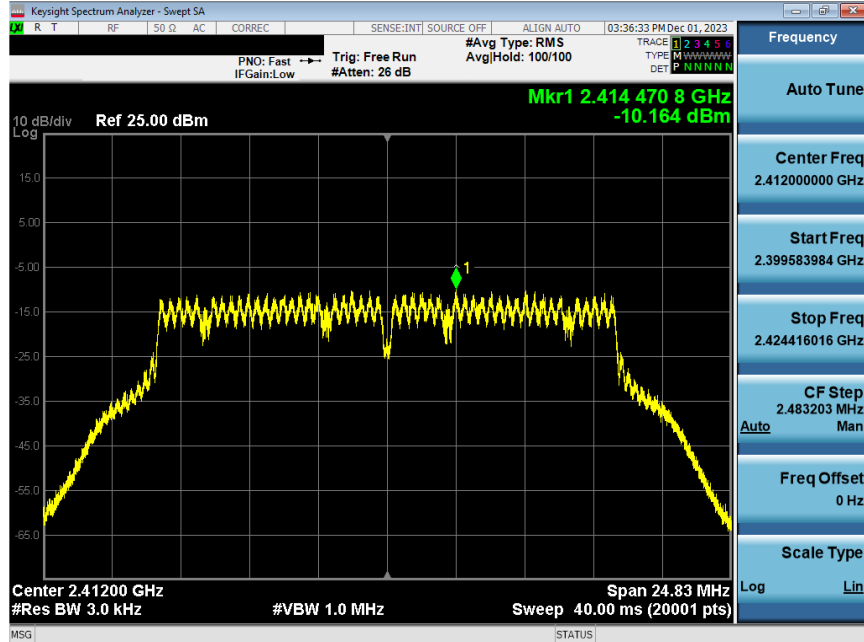
Plot 7-82. Power Spectral Density Plot Antenna WF8 (802.11g – Ch. 1) – 54Mbps
