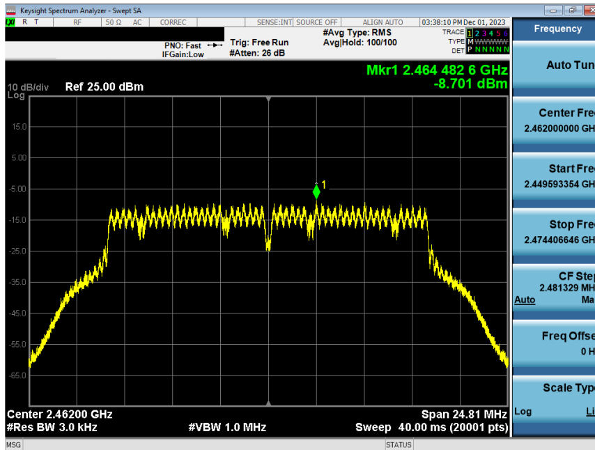
Plot 7-84. Power Spectral Density Plot Antenna WF8 (802.11g – Ch. 11) – 54Mbps
