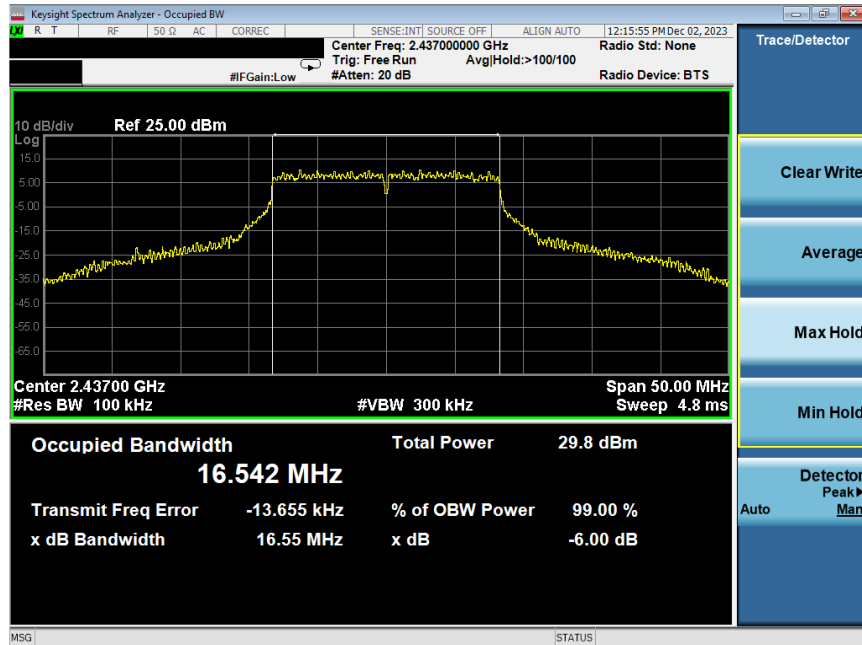
Plot 7-53. 6 dB BW and 99% OBW Plot Antenna WF7b (802.11g – Ch. 6) – 54Mbps
