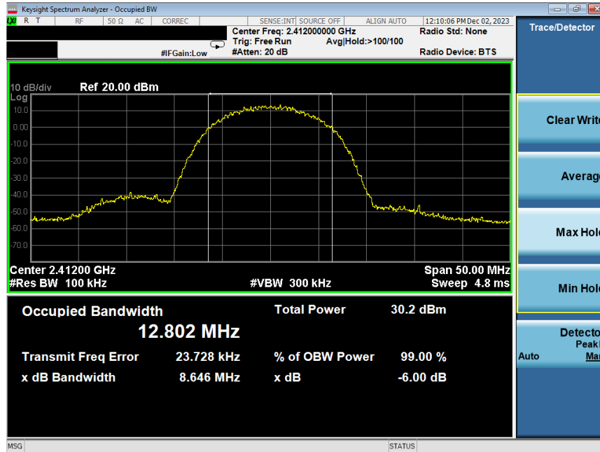
Plot 7-49. 6 dB BW and 99% OBW Plot Antenna WF7b (802.11b – Ch. 1) – 11Mbps
