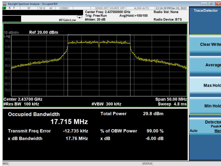
Plot 7-56. 6 dB BW and 99% OBW Plot Antenna WF7b (802.11n (2.4GHz) – Ch. 6) – MCS7
