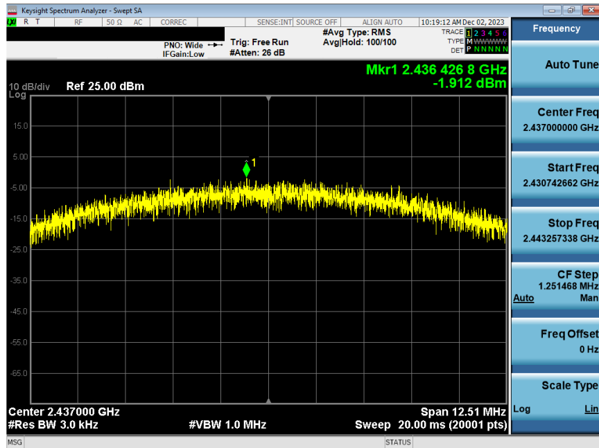
Plot 7-80. Power Spectral Density Plot Antenna WF8 (802.11b – Ch. 6) – 11Mbps
