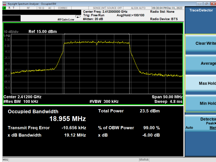
Plot 7-58. 6 dB BW and 99% OBW Plot Antenna WF7b (802.11ax (SU - 2.4GHz) – Ch. 1) – MCS9
