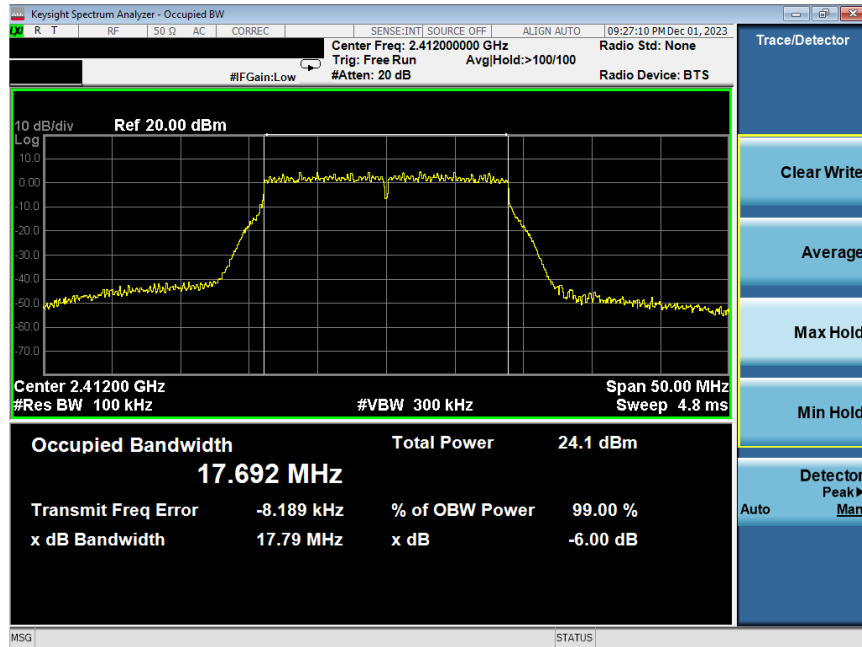
Plot 7-55. 6 dB BW and 99% OBW Plot Antenna WF7b (802.11n (2.4GHz) – Ch. 1) – MCS7
