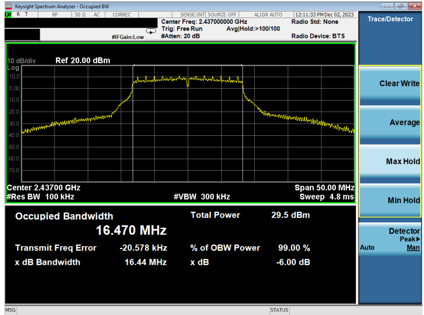
Plot 7-32. 6 dB BW and 99% OBW Plot Antenna WF7b (802.11g – Ch. 6) – 6Mbps
