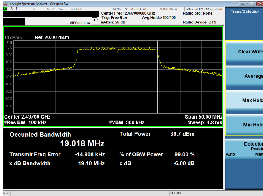
Plot 7-59. 6 dB BW and 99% OBW Plot Antenna WF7b (802.11ax (SU - 2.4GHz) – Ch. 6) – MCS9
