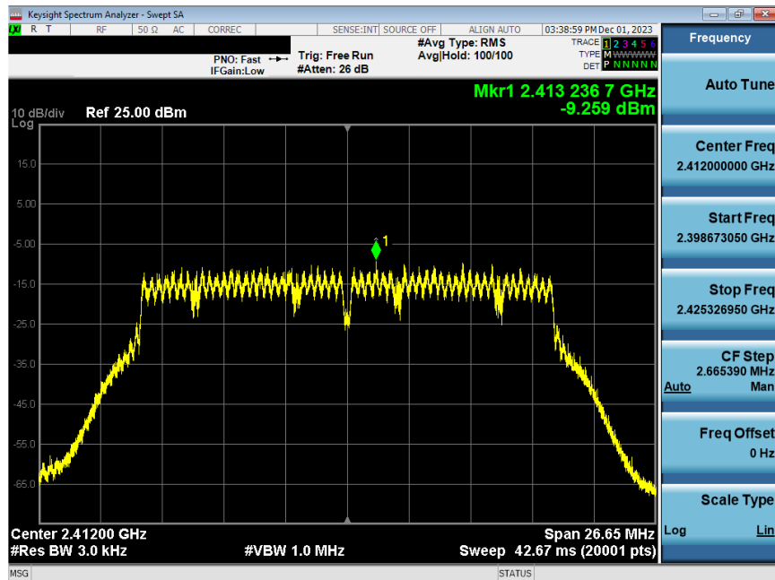
Plot 7-85. Power Spectral Density Plot Antenna WF8 (802.11n (2.4GHz) – Ch. 1) – MCS7
