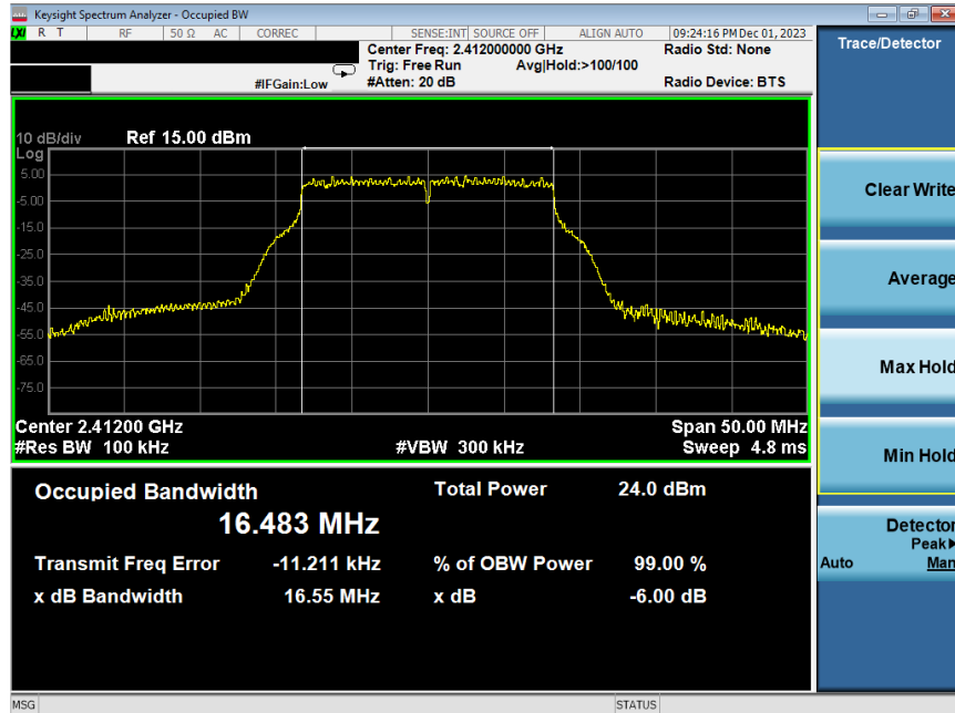
Plot 7-52. 6 dB BW and 99% OBW Plot Antenna WF7b (802.11g – Ch. 1) – 54Mbps
