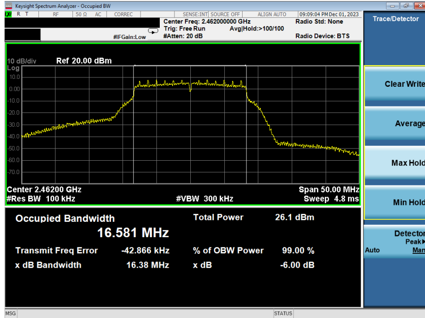
Plot 7-33. 6 dB BW and 99% OBW Plot Antenna WF7b (802.11g – Ch. 11) – 6Mbps
