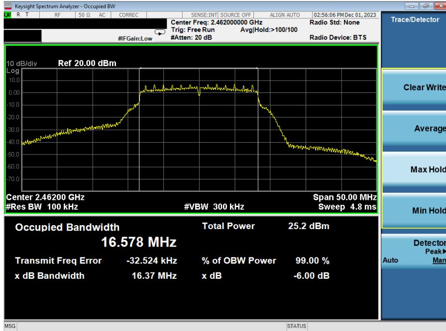
Plot 7-3. 6 dB BW and 99% OBW Plot Antenna WF8 (802.11g – Ch. 11) – 12Mbps
