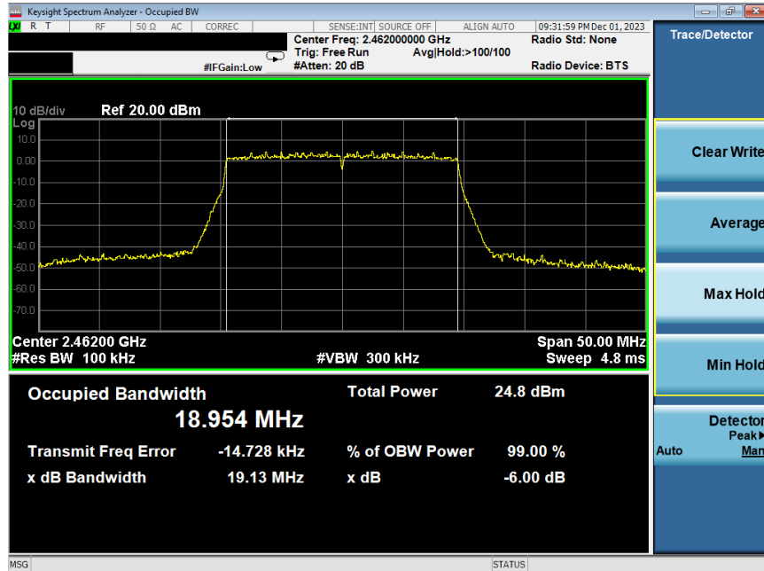
Plot 7-60. 6 dB BW and 99% OBW Plot Antenna WF7b (802.11ax (SU - 2.4GHz) – Ch. 11) – MCS9
