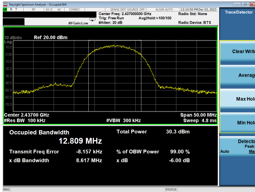
Plot 7-50. 6 dB BW and 99% OBW Plot Antenna WF7b (802.11b – Ch. 6) – 11Mbps
