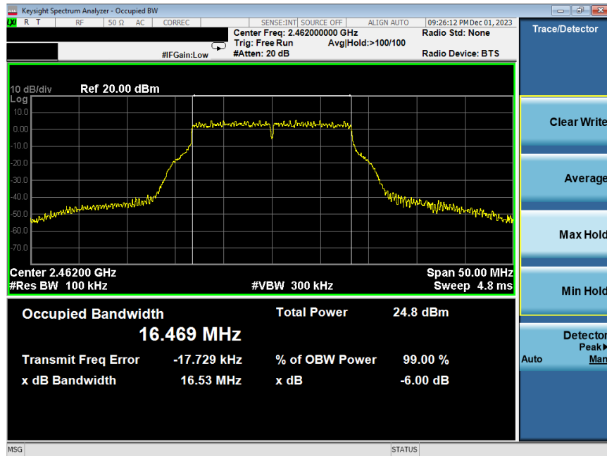
Plot 7-54. 6 dB BW and 99% OBW Plot Antenna WF7b (802.11g – Ch. 11) – 54Mbps
