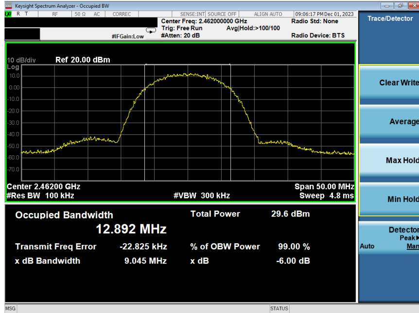
Plot 7-51. 6 dB BW and 99% OBW Plot Antenna WF7b (802.11b – Ch. 11) – 11Mbps
