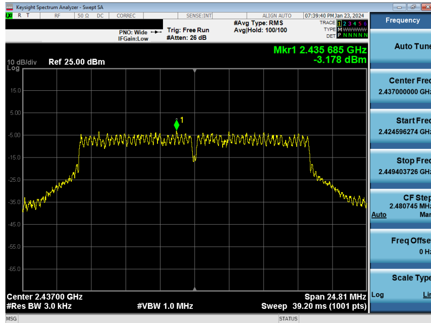
Plot 7-83. Power Spectral Density Plot Antenna WF8 (802.11g – Ch. 6) – 54Mbps
