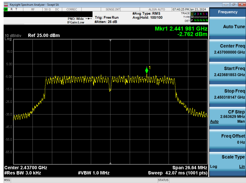
Plot 7-86. Power Spectral Density Plot Antenna WF8 (802.11n (2.4GHz) – Ch. 6) – MCS7
