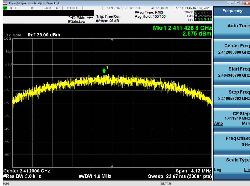
Plot 7-79. Power Spectral Density Plot Antenna WF8 (802.11b – Ch. 1) – 11Mbps
