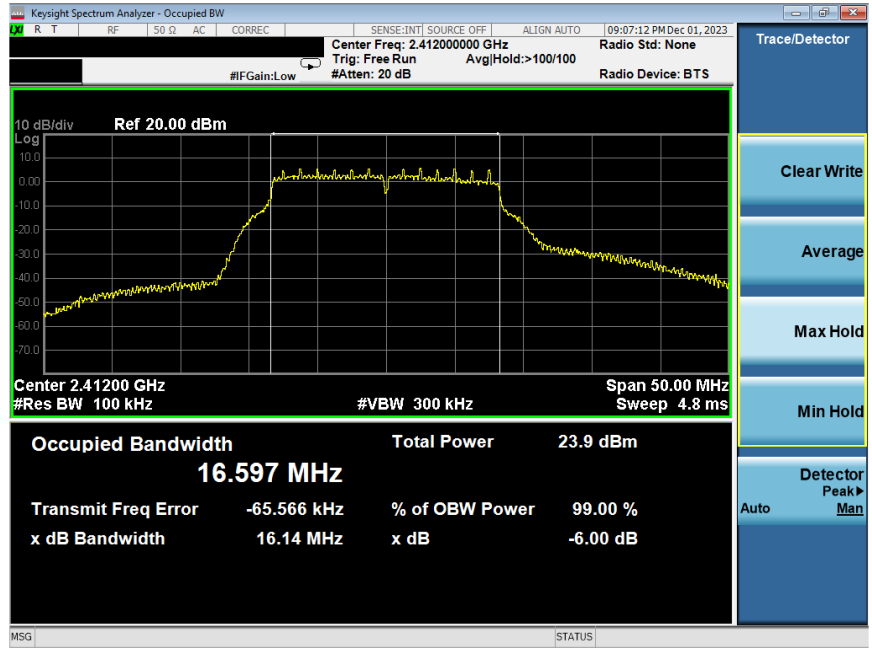
Plot 7-31. 6 dB BW and 99% OBW Plot Antenna WF7b (802.11g – Ch. 1) – 6Mbps
