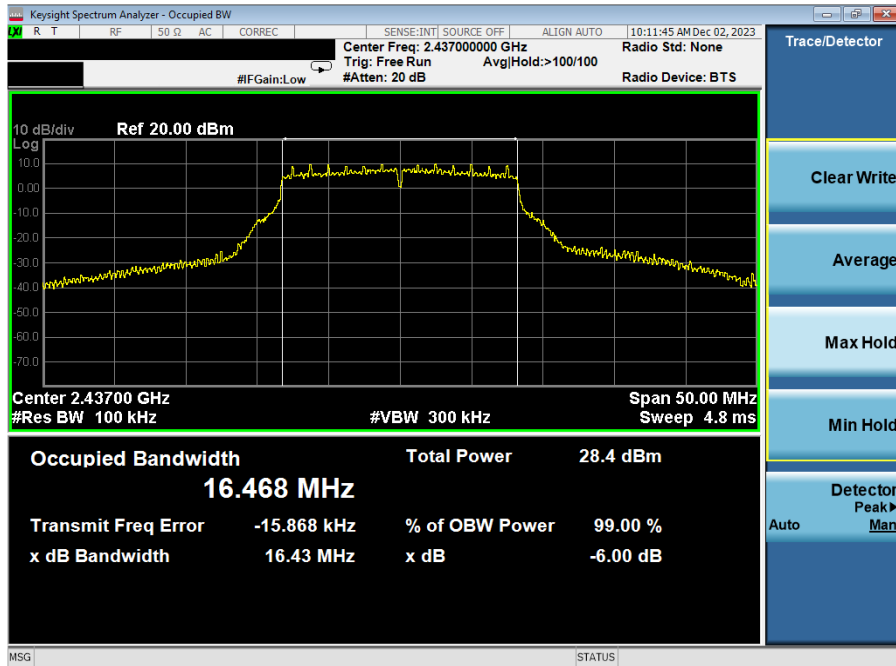
Plot 7-2. 6 dB BW and 99% OBW Plot Antenna WF8 (802.11g – Ch. 6) – 12Mbps
