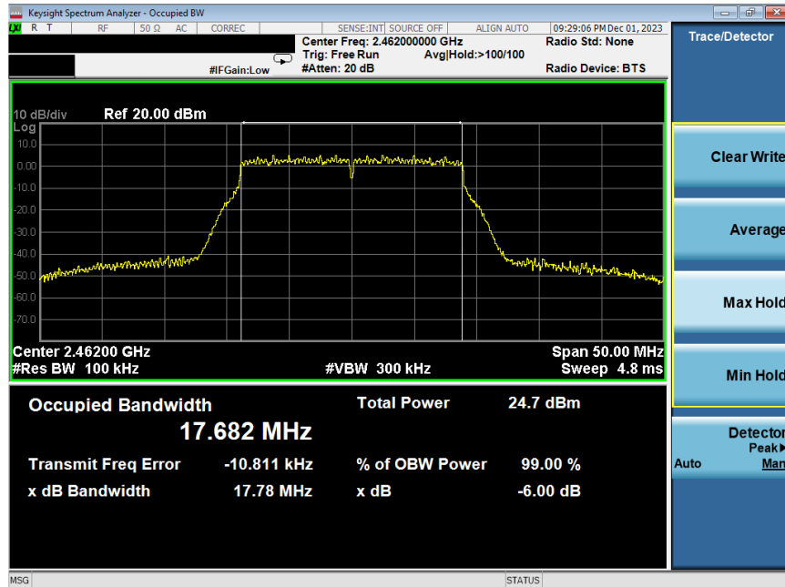
Plot 7-57. 6 dB BW and 99% OBW Plot Antenna WF7b (802.11n (2.4GHz) – Ch. 11) – MCS7
