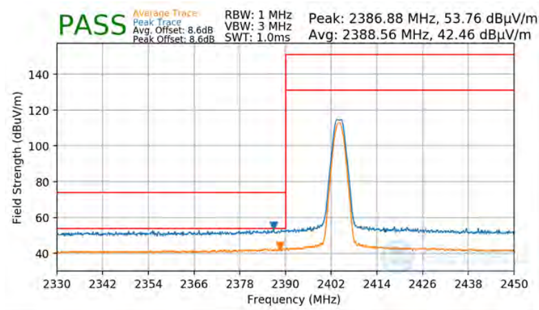
Plot 7-97. Radiated Restricted Lower Band Edge Measurement Antenna WF7b (Average & Peak)
