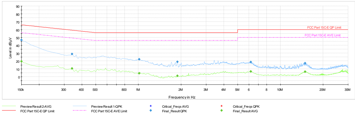
Plot 7-104. AC Line Conducted Plot with Bluetooth LE Tx BF (L1, 1Mbps ePA – Ch.19 with AC/DC Adapter)
