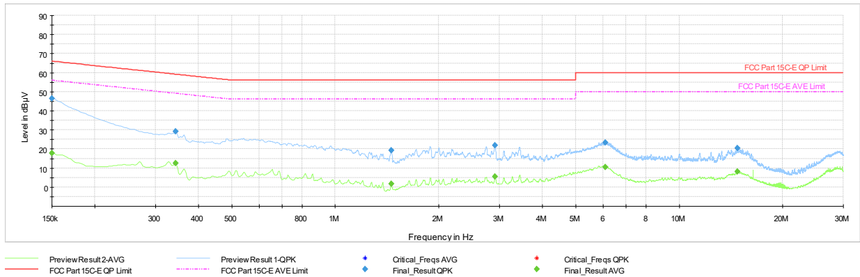
Plot 7-105. AC Line Conducted Plot with Bluetooth LE TxBF (N, 1Mbps ePA – Ch.19, with AC/DC Adapter)
