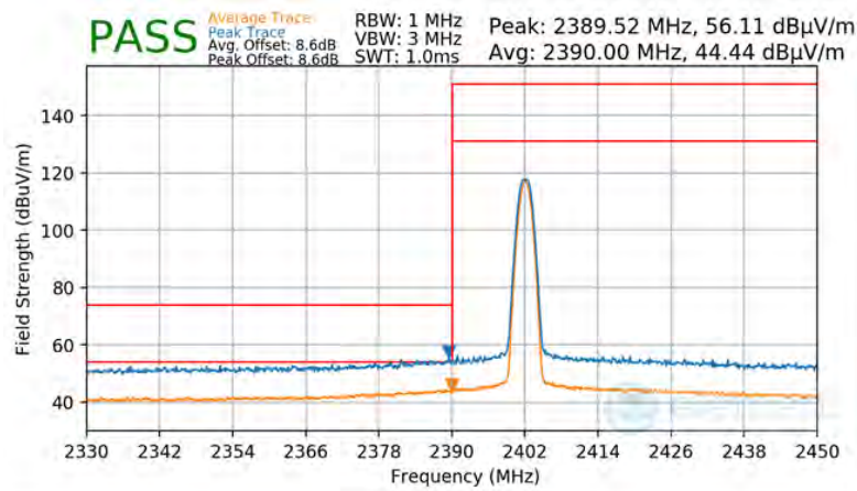
Plot 7-91. Radiated Restricted Lower Band Edge Measurement Antenna WF8 (Average & Peak)
