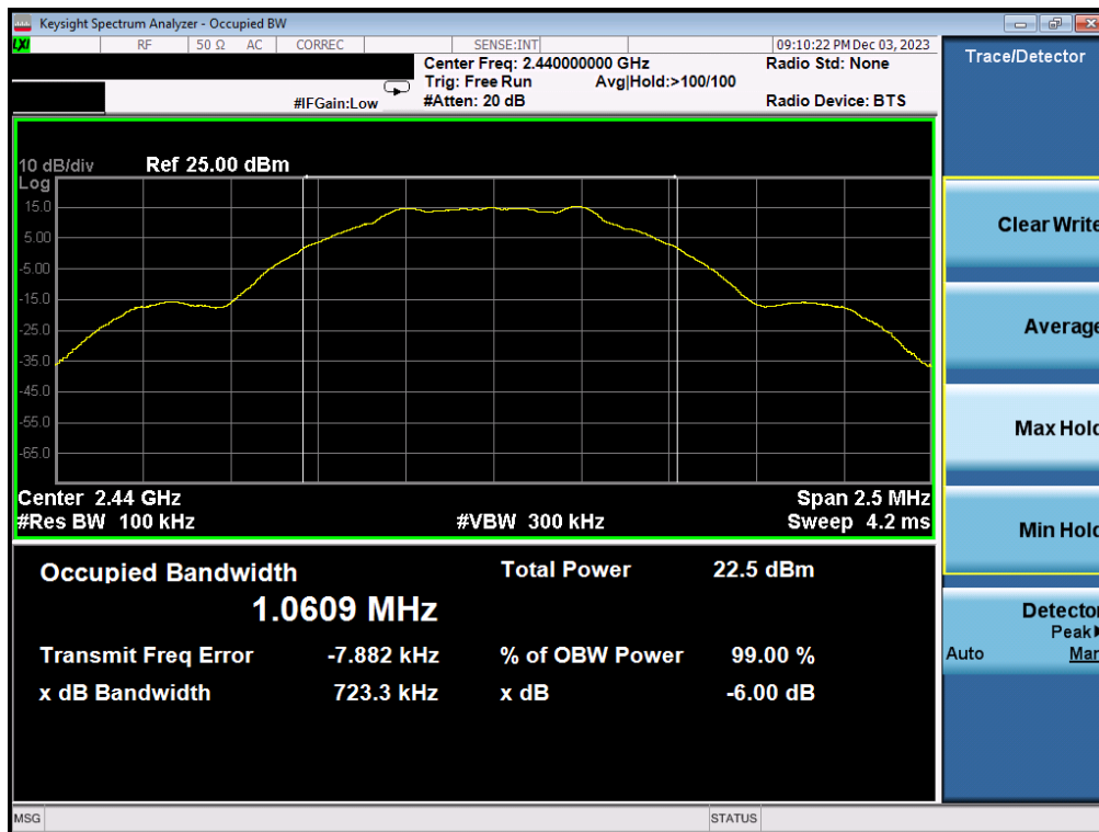
Plot 7-8. 6dB BW & 99% OBW Plot Antenna WF7b (Bluetooth (LE), 1Mbps, ePA – Ch. 19)
