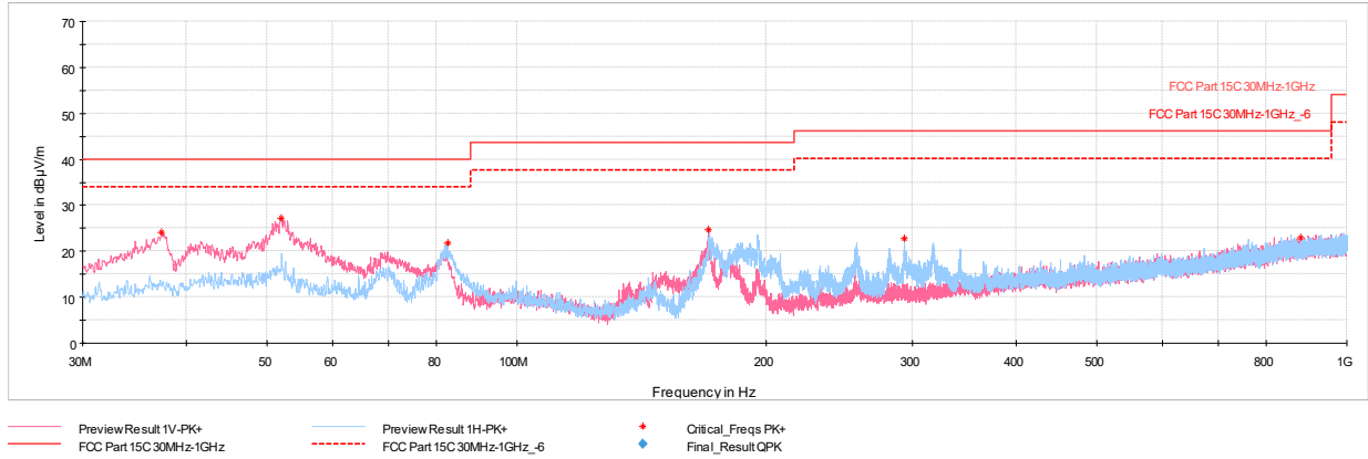
Plot 7-103. Radiated Spurious Emissions Below 1GHz TxBF (1Mbps, ePA – Ch.19, Pol. H & V, with AC/DC Adapter)
