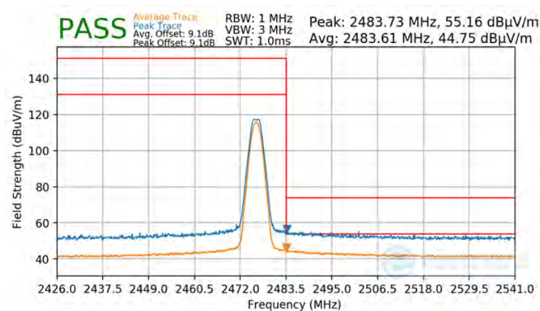
Plot 7-98. Radiated Restricted Upper Band Edge Measurement Antenna WF7b (Average & Peak)
