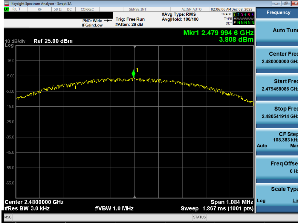
Plot 7-42. Power Spectral Density Plot Antenna WF7b (Bluetooth (LE), 1Mbps, ePA – Ch. 39)
