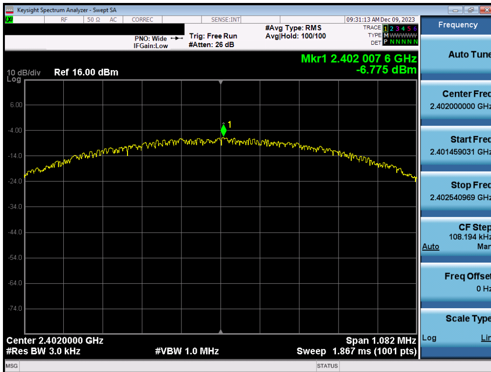
Plot 7-28. Power Spectral Density Plot Antenna WF7b (Bluetooth (LE), 1Mbps, iPA – Ch. 0)
