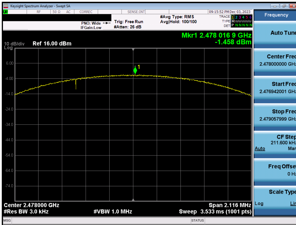
Plot 7-33. Power Spectral Density Plot Antenna WF7b (Bluetooth (LE), 2Mbps, ePA – Ch. 38)
