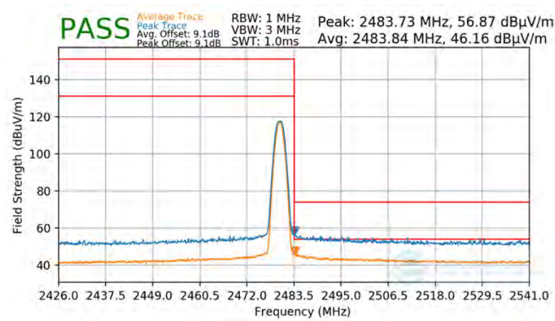
Plot 7-96. Radiated Restricted Upper Band Edge Measurement Antenna WF7b (Average & Peak)
