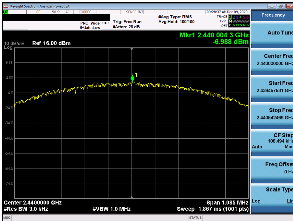
Plot 7-46. Power Spectral Density Plot Antenna WF7b (Bluetooth (LE), 1Mbps, iPA – Ch. 19)
