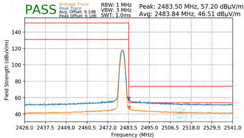
Plot 7-92. Radiated Restricted Upper Band Edge Measurement Antenna WF8 (Average & Peak)
