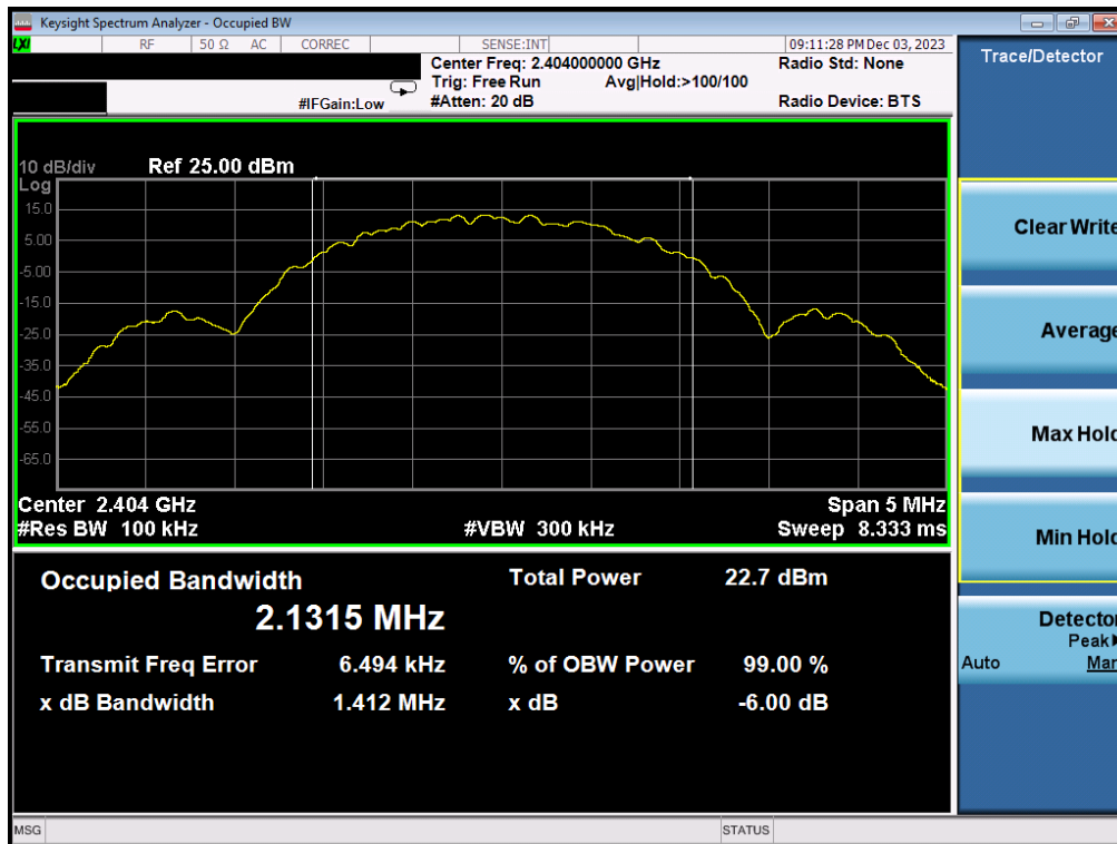
Plot 7-10. 6dB BW & 99% OBW Plot Antenna WF7b (Bluetooth (LE), 2Mbps, ePA – Ch. 1)
