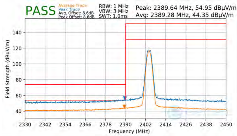
Plot 7-93. Radiated Restricted Lower Band Edge Measurement Antenna WF8 (Average & Peak)
