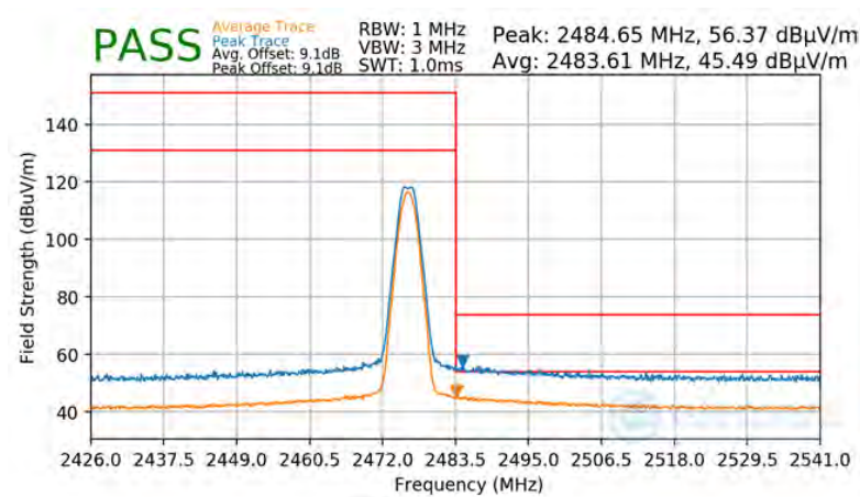
Plot 7-94. Radiated Restricted Upper Band Edge Measurement Antenna WF8 (Average & Peak)
