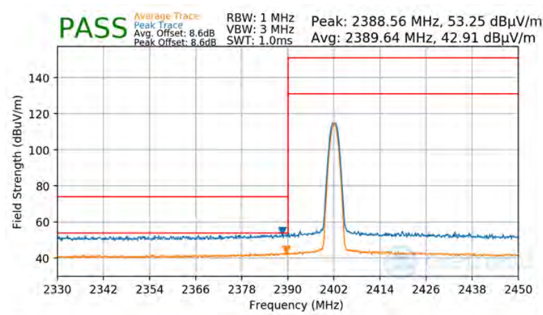
Plot 7-95. Radiated Restricted Lower Band Edge Measurement Antenna WF7b (Average & Peak)
