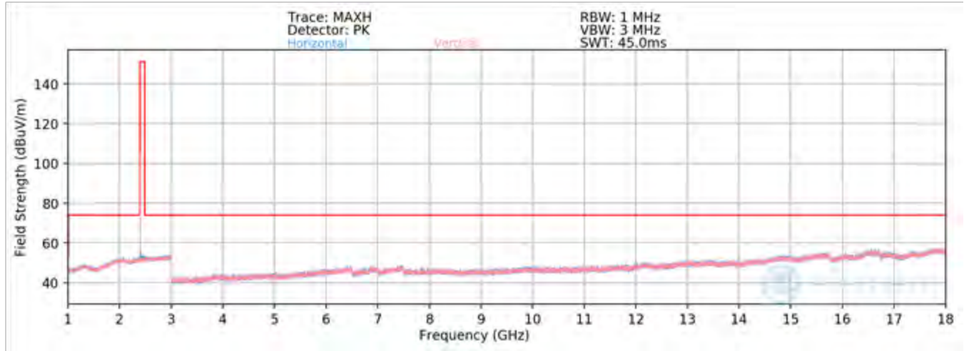
Plot 7-81. Radiated Spurious Emissions 1-18GHz Antenna WF8 (1Mbps, ePA – Ch. 0)
