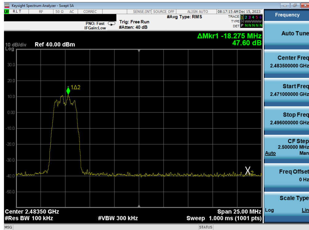
Plot 7-62. Band Edge Plot Antenna WF8 (Bluetooth (HDR4), ePA – Ch. 73)
