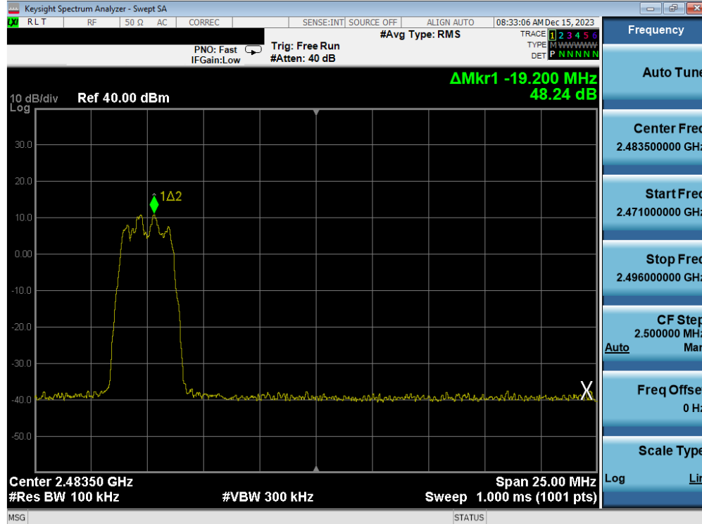
Plot 7-66. Band Edge Plot Antenna WF7b (Bluetooth (HDR4), ePA – Ch. 73)
