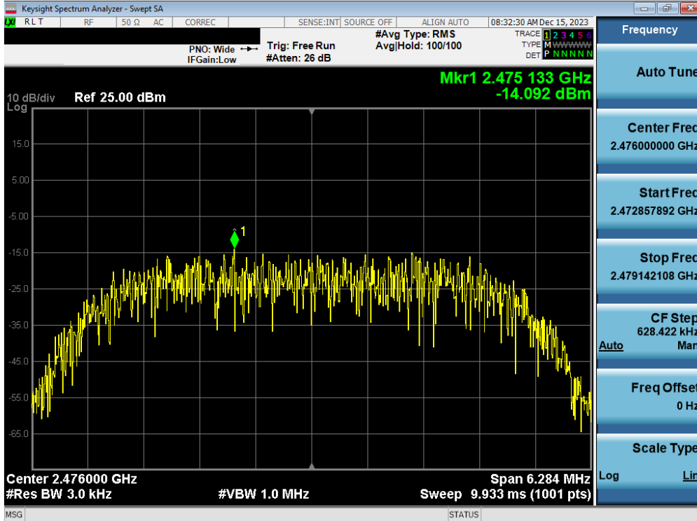
Plot 7-60. Power Spectral Density Plot TxBF Antenna WF7b (Bluetooth (HDR8), 8Mbps, iPA – Ch. 73)
