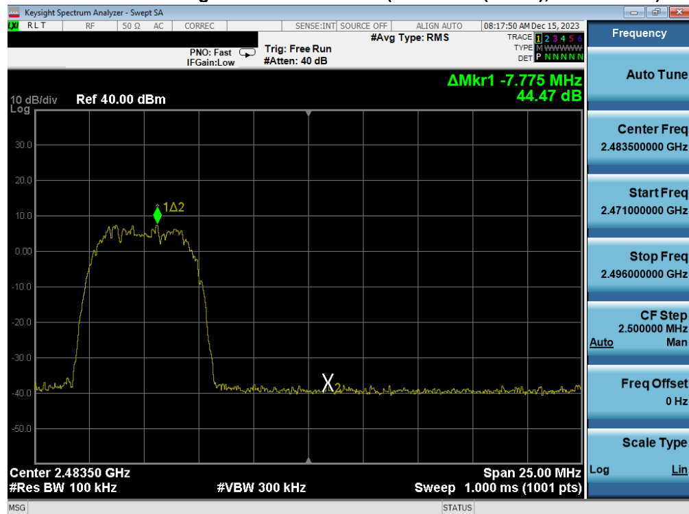
Plot 7-64. Band Edge Plot Antenna WF8 (Bluetooth (HDR8), ePA – Ch. 73)
