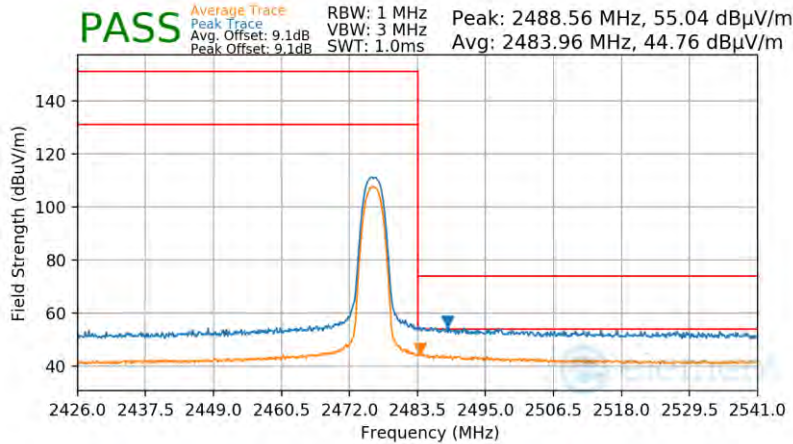
Plot 7-93. Radiated Restricted Upper Band Edge Measurement Antenna WF8
