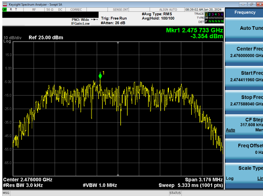
Plot 7-27. Power Spectral Density Plot Antenna WF7b (Bluetooth (HDR4), 4Mbps, ePA – Ch. 73)
