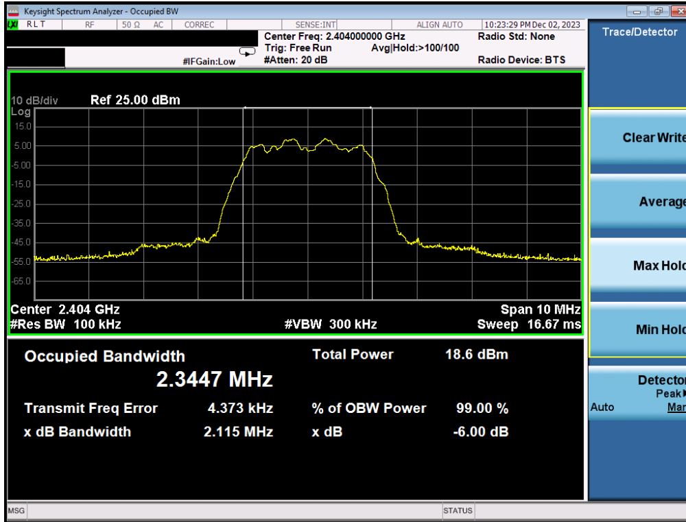
Plot 7-1. 6dB BW & 99% OBW Plot Antenna WF8 (Bluetooth (HDR4), 4Mbps, ePA – Ch. 1)
