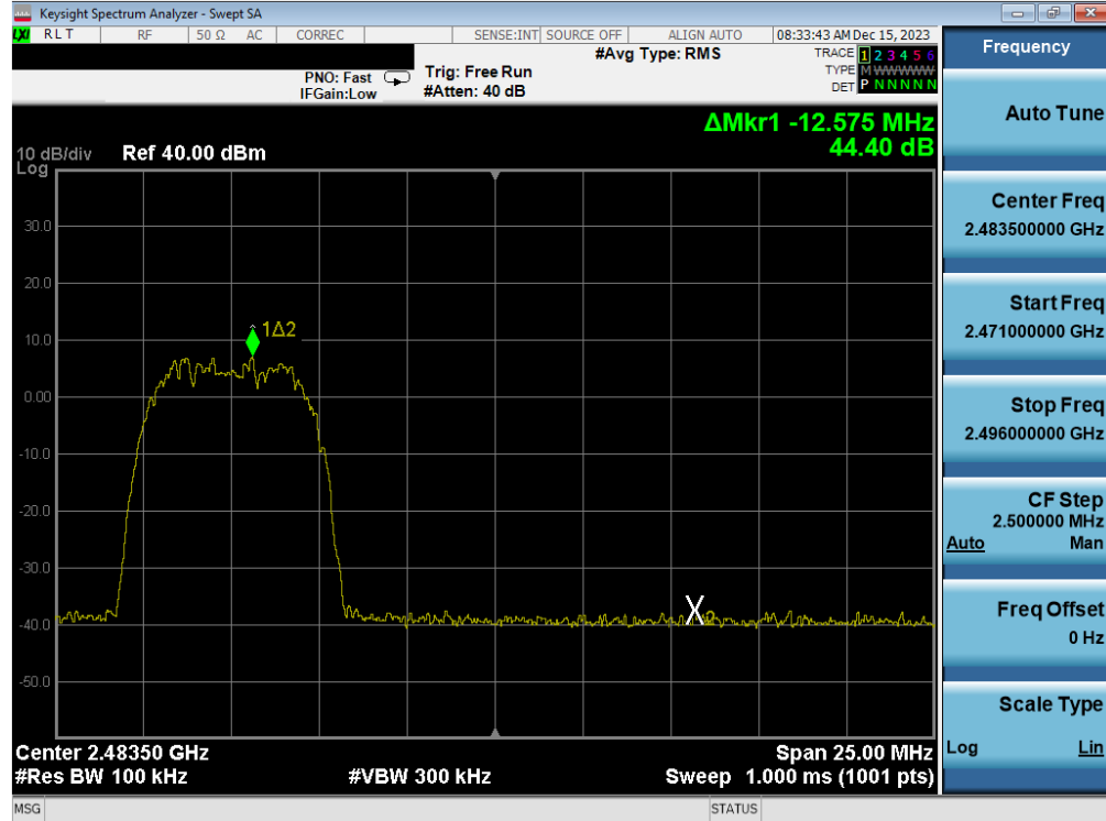
Plot 7-68. Band Edge Plot Antenna WF7b (Bluetooth (HDR8), ePA – Ch. 73)
