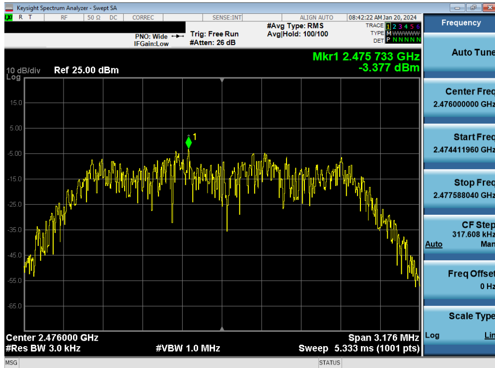
Plot 7-42. Power Spectral Density Plot TxBF Antenna WF7b (Bluetooth (HDR4), 4Mbps, ePA – Ch. 73)
