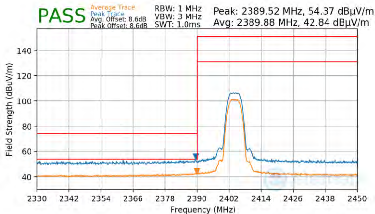
Plot 7-96. Radiated Restricted Lower Band Edge Measurement Antenna WF7b
