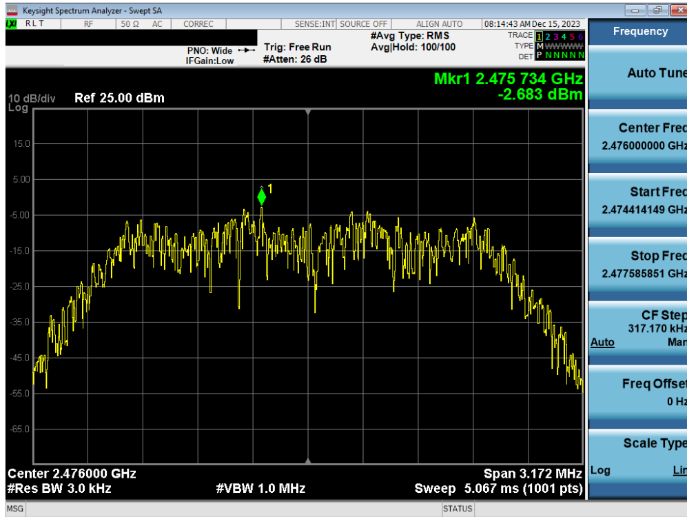
Plot 7-41. Power Spectral Density Plot TxBF Antenna WF8 (Bluetooth (HDR4), 4Mbps, ePA – Ch. 73)
