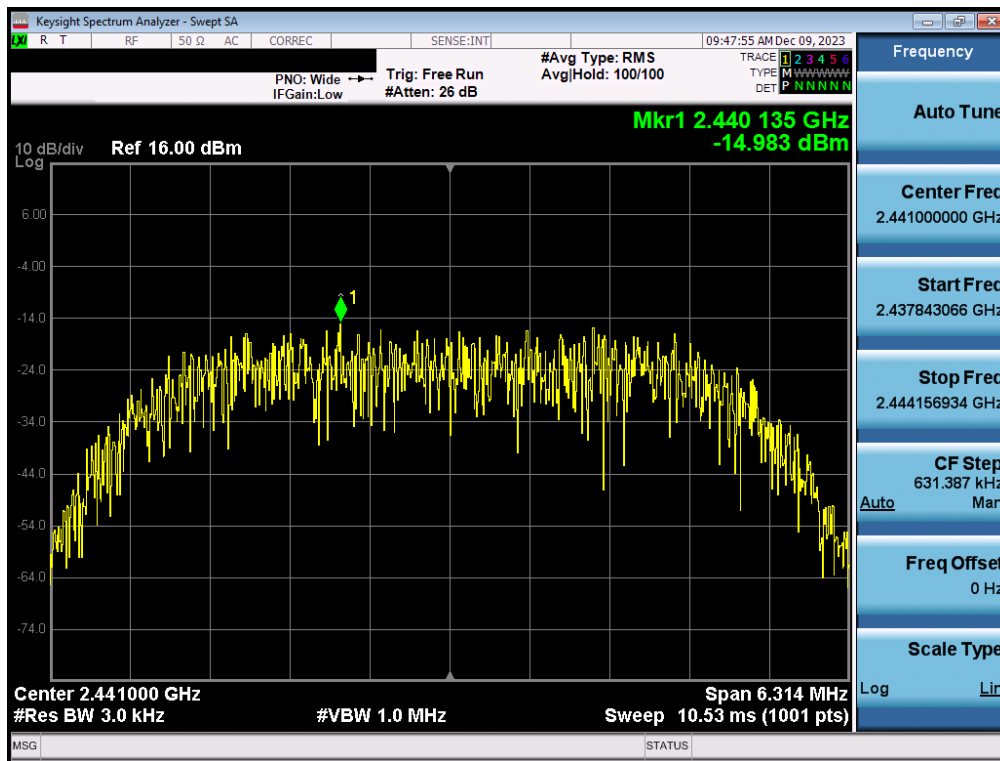
Plot 7-57. Power Spectral Density Plot TxBF Antenna WF8 (Bluetooth (HDR8), 8Mbps, iPA – Ch. 38)
