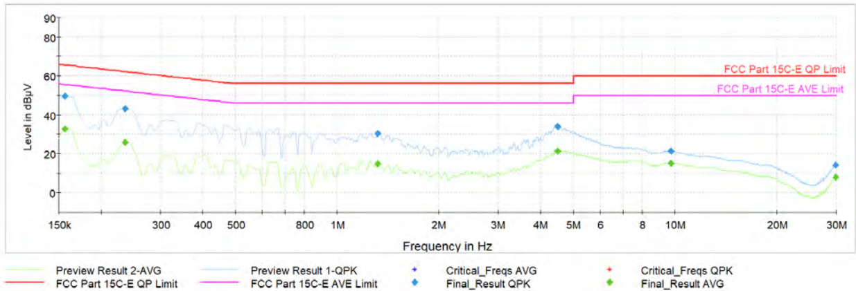
Plot 7-105. AC Line Conducted Plot with Bluetooth HDR (N, 4Mbps ePA - Ch.38 with AC/DC Adapter)
