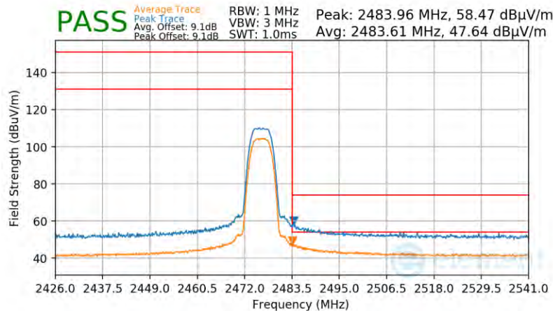
Plot 7-94. Radiated Restricted Upper Band Edge Measurement Antenna WF8
