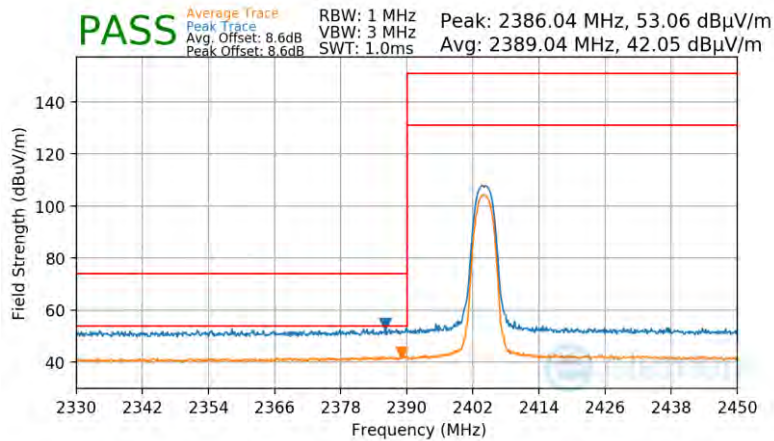
Plot 7-95. Radiated Restricted Lower Band Edge Measurement Antenna WF7b
