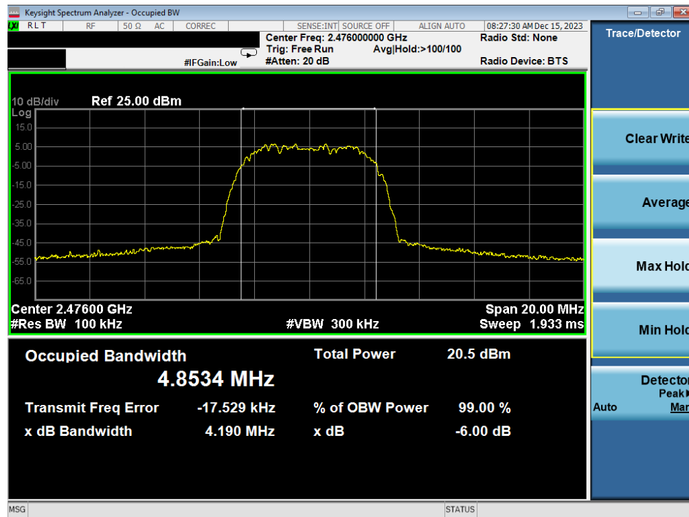
Plot 7-12. 6dB BW & 99% OBW Plot Antenna WF7b (Bluetooth (HDR8), 8Mbps, ePA – Ch. 73)
