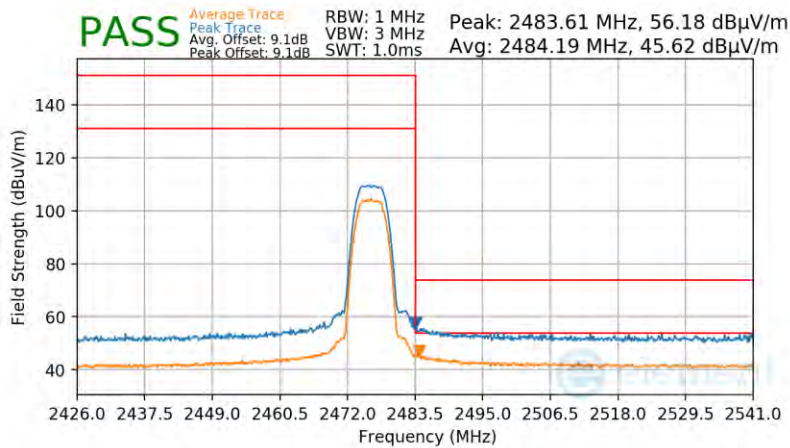
Plot 7-98. Radiated Restricted Upper Band Edge Measurement Antenna WF7b
