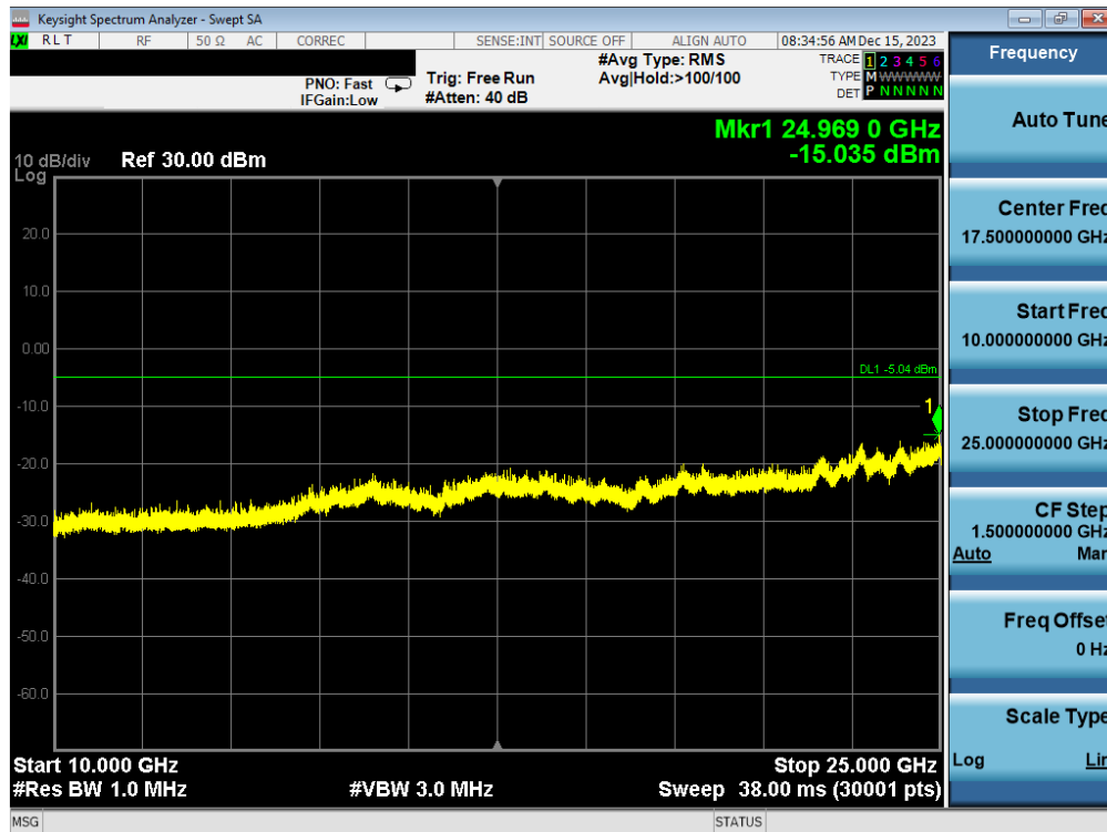
Plot 7-80. Conducted Spurious Plot Antenna WF7b (Bluetooth (HDR4), 4 Mbps, ePA – Ch. 73)
