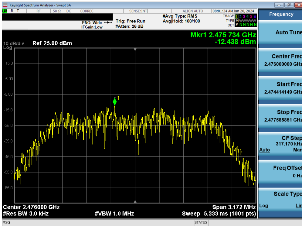
Plot 7-47. Power Spectral Density Plot Tx BF Antenna WF8 (Bluetooth (HDR4), 4Mbps, iPA – Ch. 73)
