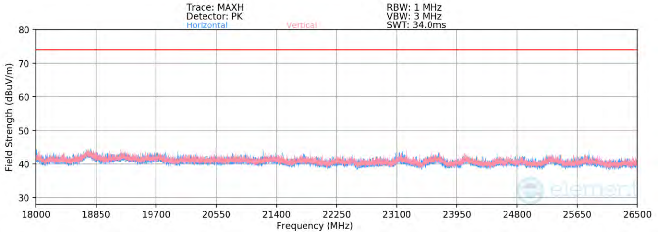
Plot 7-90. Radiated Spurious Emissions Above 18GHz TxBF (4Mbps, HDR4, ePA – Ch. 38)
