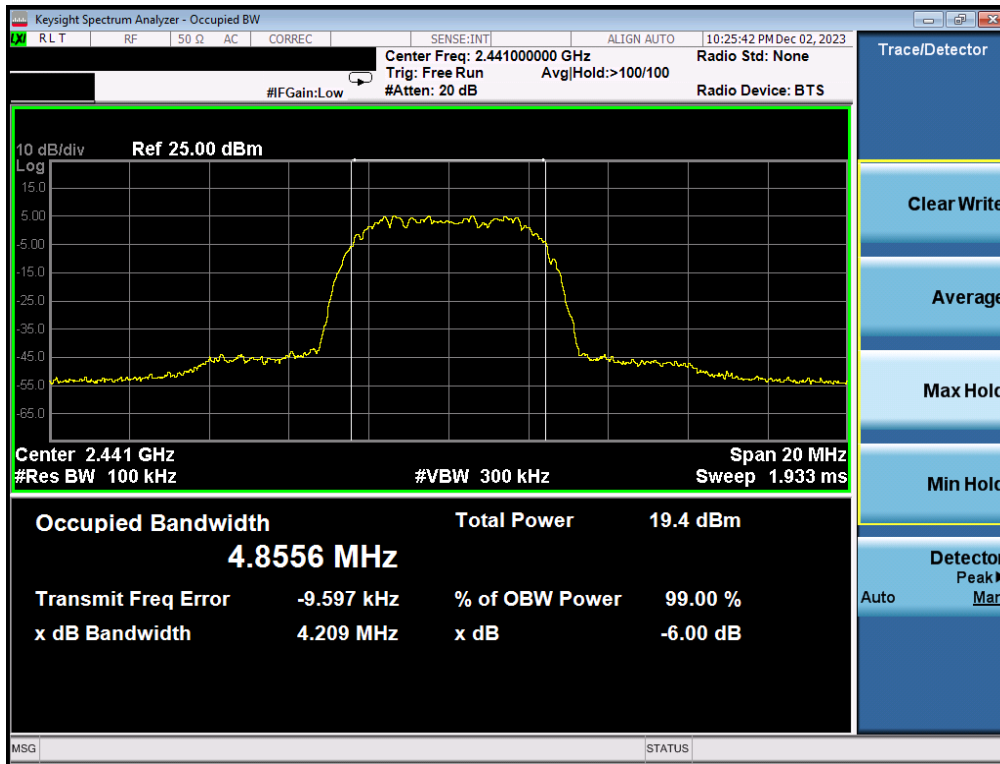
Plot 7-5. 6dB BW & 99% OBW Plot Antenna WF8 (Bluetooth (HDR8), 8Mbps, ePA – Ch. 38)
