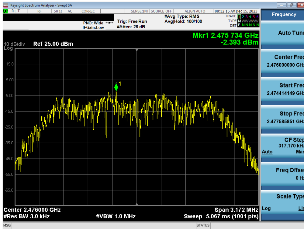
Plot 7-15. Power Spectral Density Plot Antenna WF8 (Bluetooth (HDR4), 4Mbps, ePA – Ch. 73)
