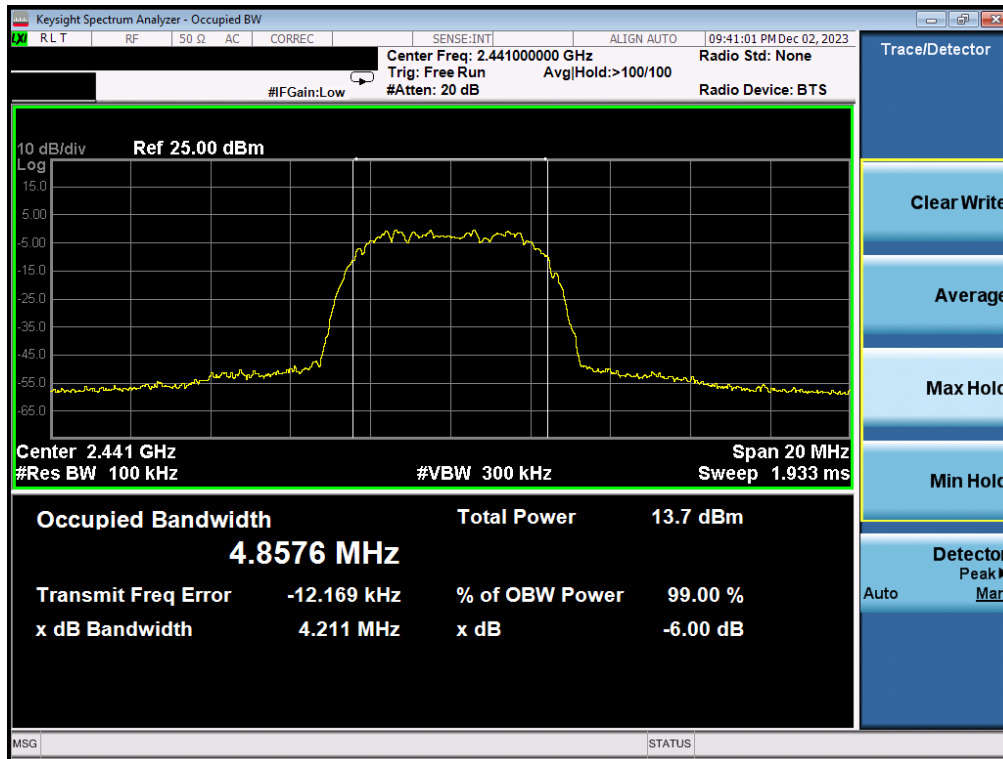
Plot 7-11. 6dB BW & 99% OBW Plot Antenna WF7b (Bluetooth (HDR8), 8Mbps, ePA – Ch. 38)
