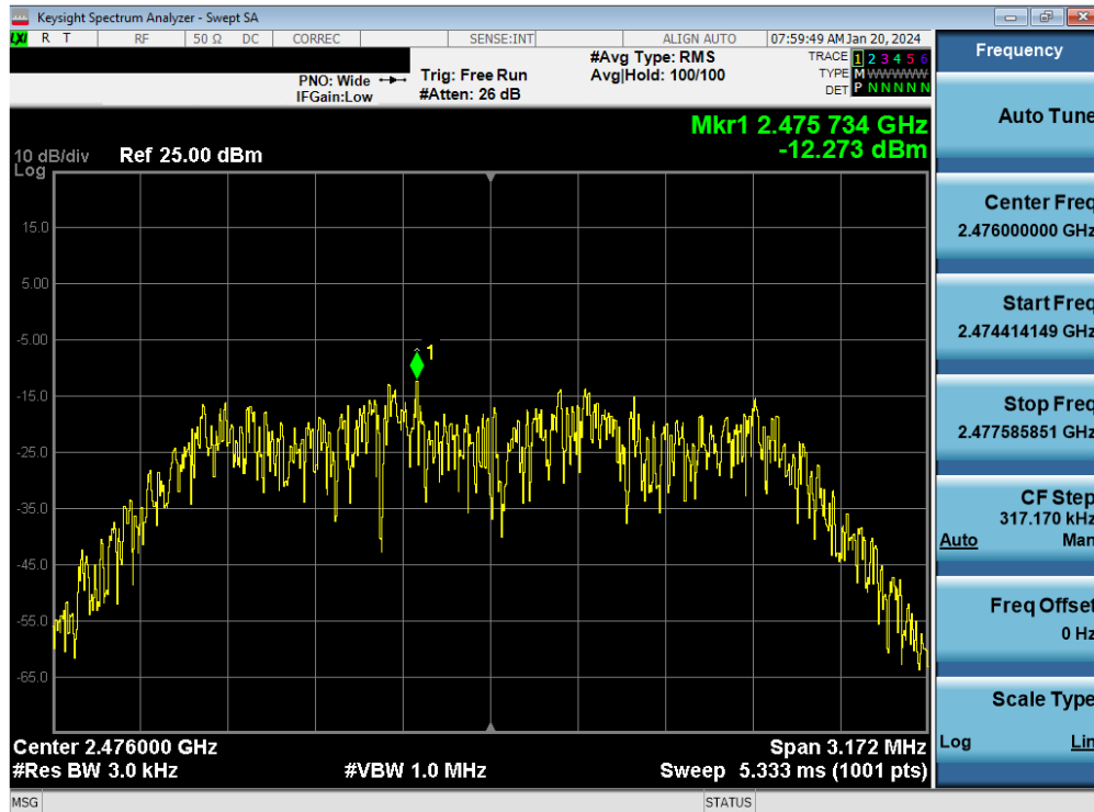
Plot 7-18. Power Spectral Density Plot Antenna WF8 (Bluetooth (HDR4), 4Mbps, iPA – Ch. 73)
