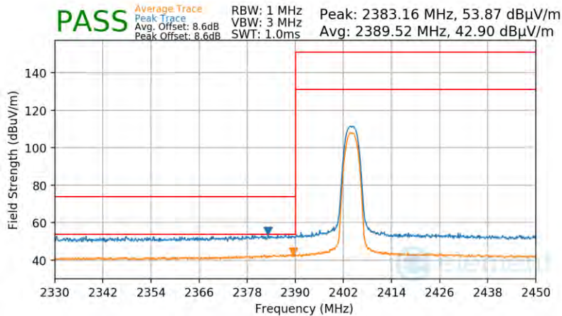
Plot 7-91. Radiated Restricted Lower Band Edge Measurement Antenna WF8
