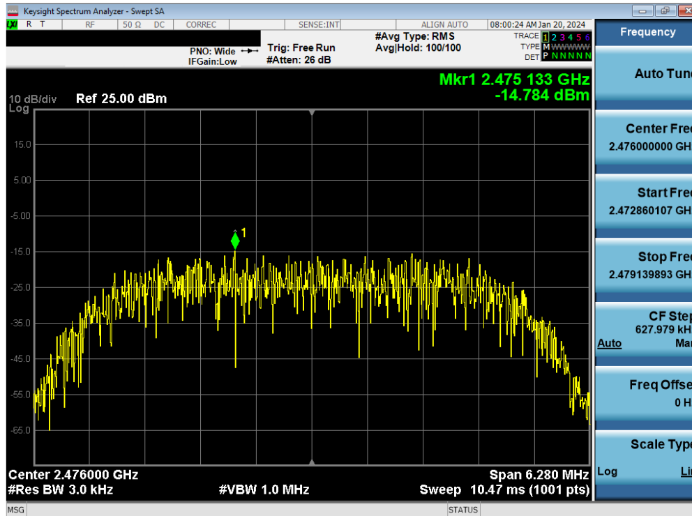
Plot 7-24. Power Spectral Density Plot Antenna WF8 (Bluetooth (HDR8), 8Mbps, iPA – Ch. 73)
