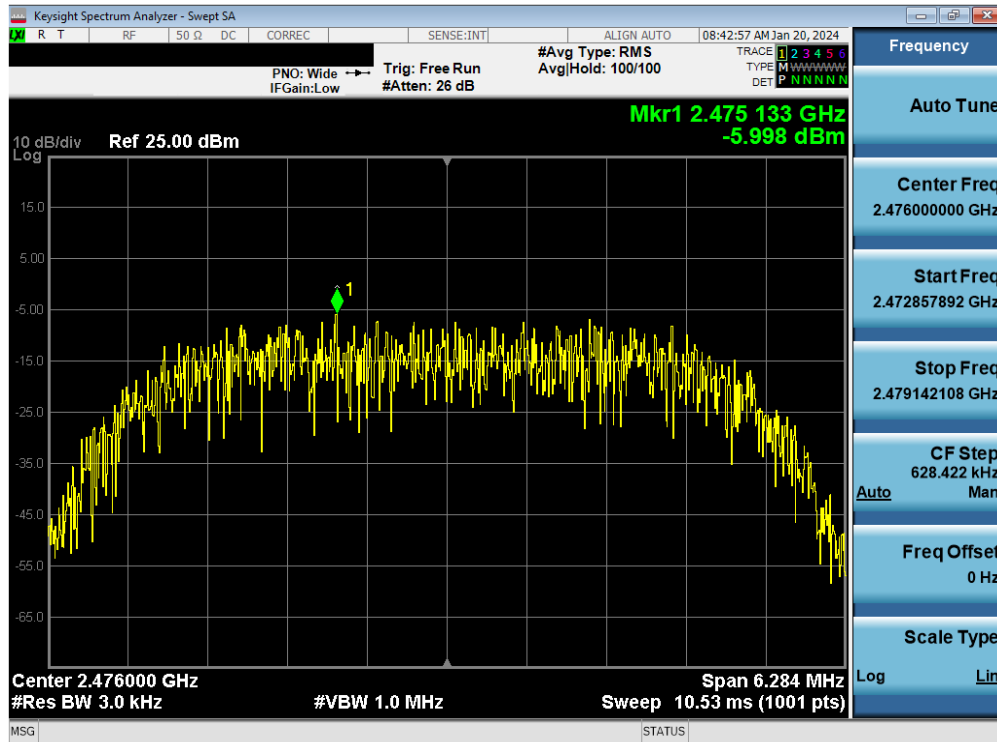
Plot 7-54. Power Spectral Density Plot TxBF Antenna WF7b (Bluetooth (HDR8), 8Mbps, ePA – Ch. 73)
