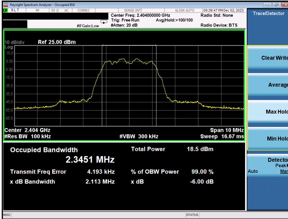
Plot 7-7. 6dB BW & 99% OBW Plot Antenna WF7b (Bluetooth (HDR4), 4Mbps, ePA – Ch. 1)
