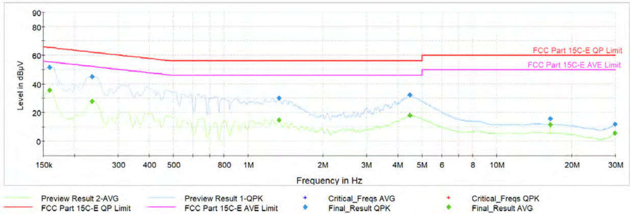
Plot 7-104. AC Line Conducted Plot with Bluetooth HDR TxBF (L1, 4Mbps ePA - Ch.38 with AC/DC Adapter)
