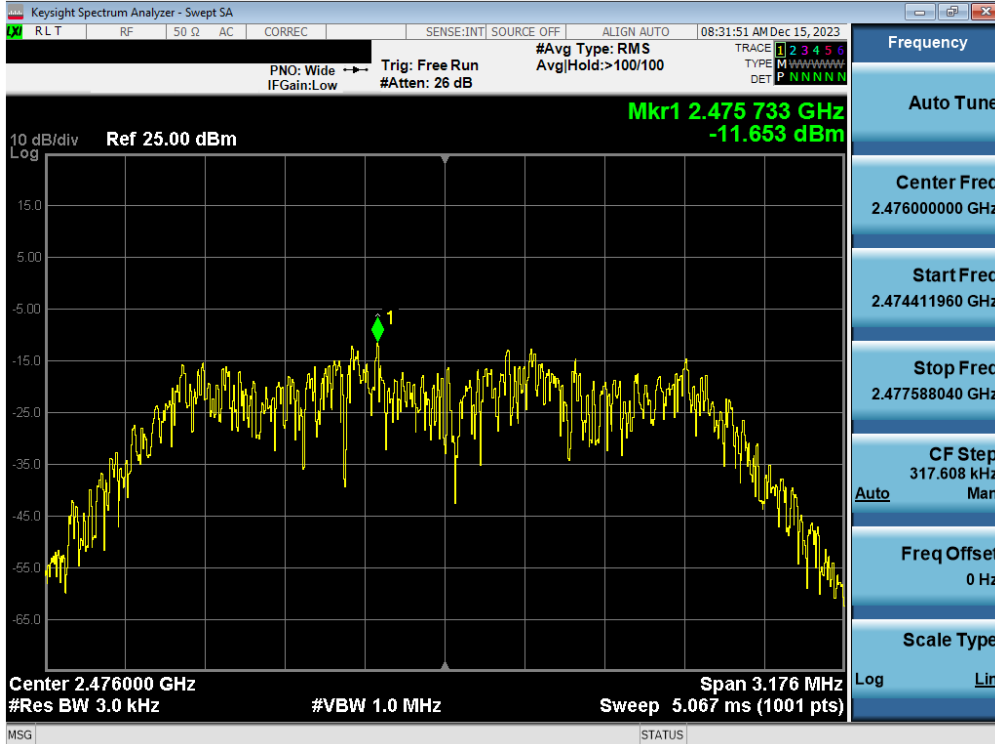
Plot 7-48. Power Spectral Density Plot Tx BF Antenna WF7b (Bluetooth (HDR4), 4Mbps, iPA – Ch. 73)
