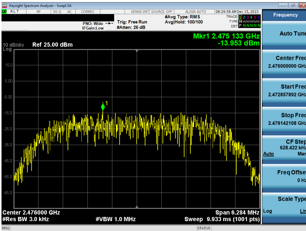
Plot 7-36. Power Spectral Density Plot Antenna WF7b (Bluetooth (HDR8), 8Mbps, iPA – Ch. 73)
