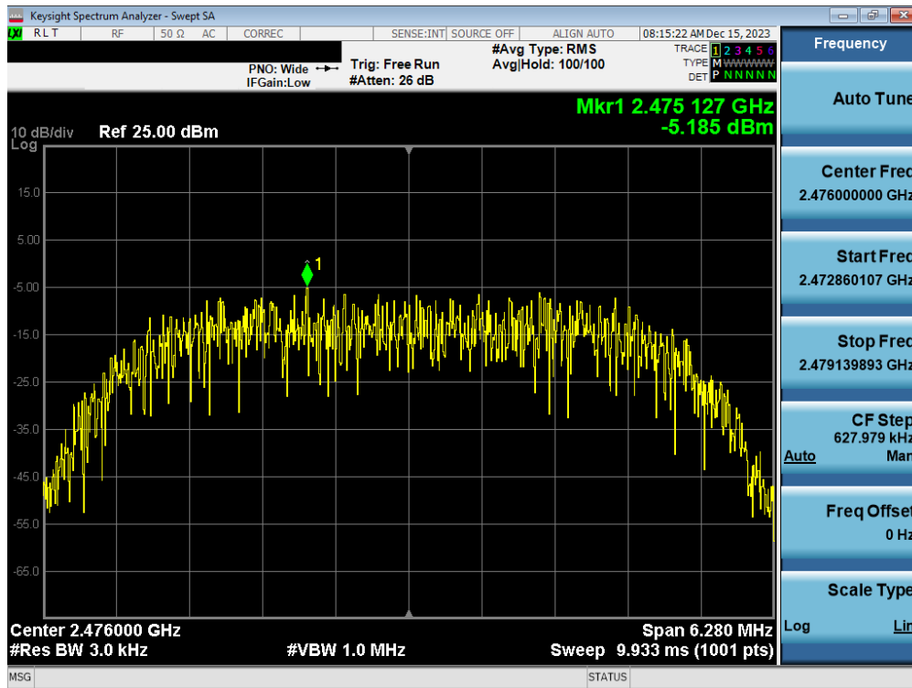
Plot 7-53. Power Spectral Density Plot TxBF Antenna WF8 (Bluetooth (HDR8), 8Mbps, ePA – Ch. 73)
