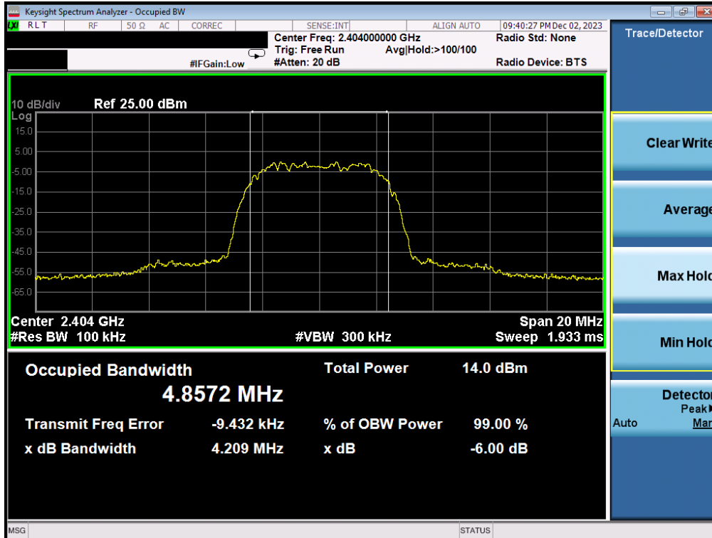
Plot 7-10. 6dB BW & 99% OBW Plot Antenna WF7b (Bluetooth (HDR8), 8Mbps, ePA – Ch. 1)
