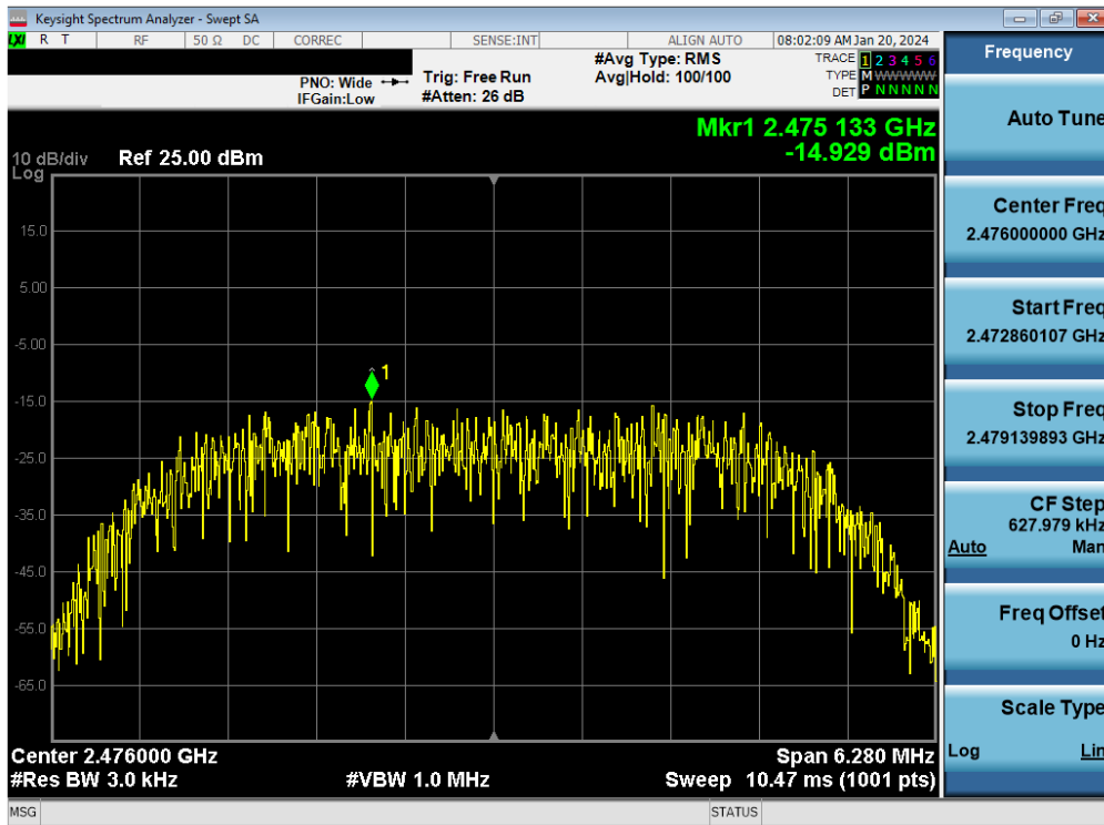
Plot 7-59. Power Spectral Density Plot TxBF Antenna WF8 (Bluetooth (HDR8), 8Mbps, iPA – Ch. 73)
