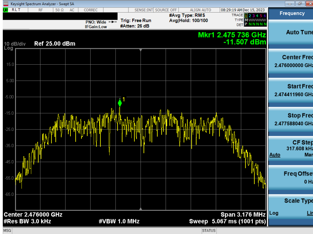
Plot 7-30. Power Spectral Density Plot Antenna WF7b (Bluetooth (HDR4), 4Mbps, iPA – Ch. 73)
