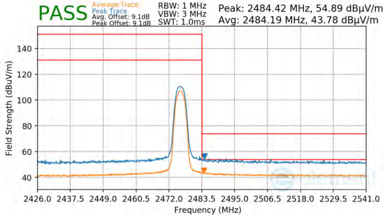
Plot 7-97. Radiated Restricted Upper Band Edge Measurement Antenna WF7b
