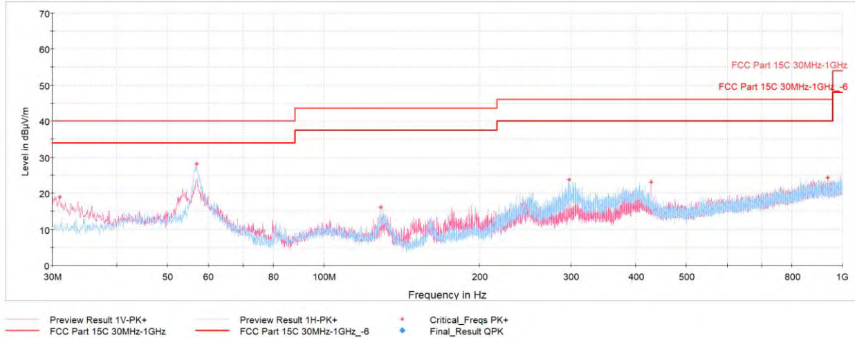
Plot 7-103. Radiated Spurious Emissions Below 1GHz TxBF (4Mbps, ePA – Ch.38 with Laptop)
