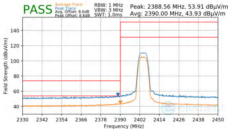
Plot 7-92. Radiated Restricted Lower Band Edge Measurement Antenna WF8
