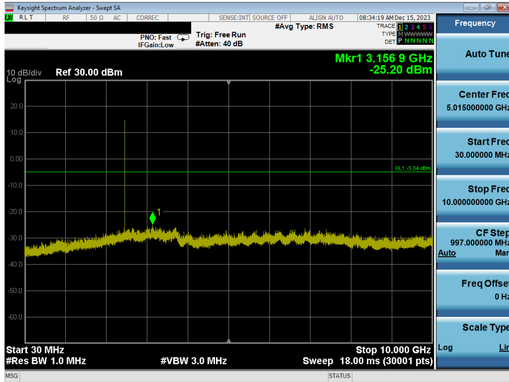
Plot 7-79. Conducted Spurious Plot Antenna WF7b (Bluetooth (HDR4), 4 Mbps, ePA – Ch. 73)
