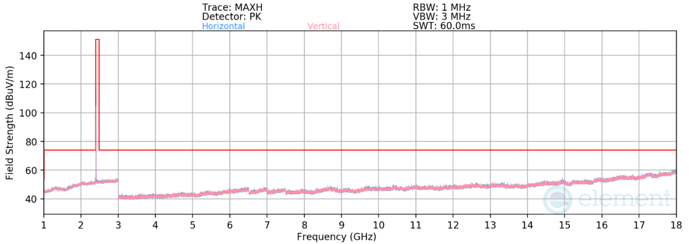
Plot 7-35. Radiated Spurious Emissions 1-18GHz Antenna WF8 (802.15.4 ePA – Ch. 11)
