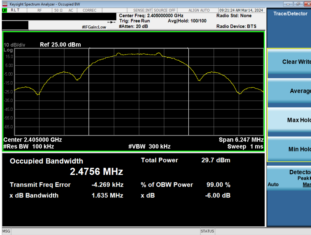
Plot 7-4. 6dB BW & 99% OBW Antenna WF7b (802.15.4, Ch. 11)
