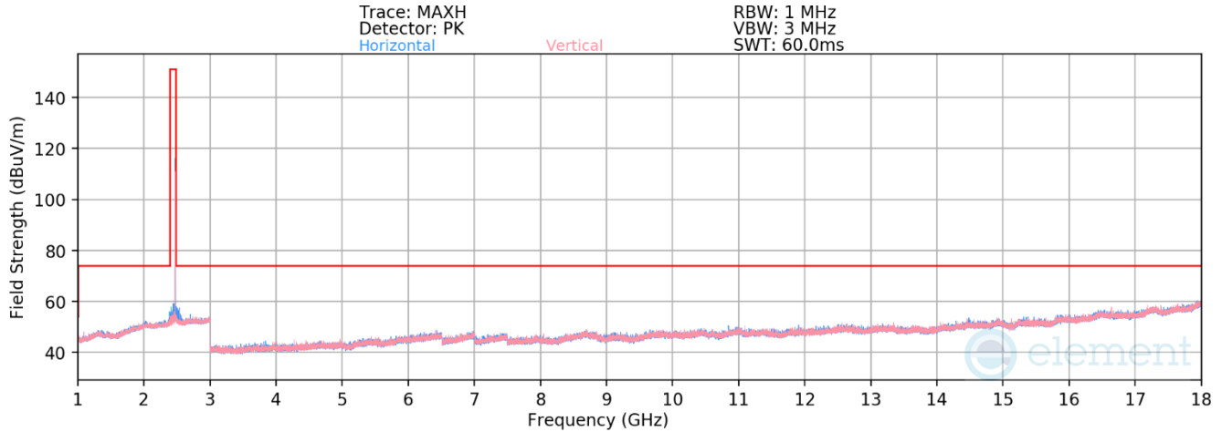
Plot 7-40. Radiated Spurious Emissions 1-18GHz Antenna WF7b (802.15.4 ePA – Ch. 25)
