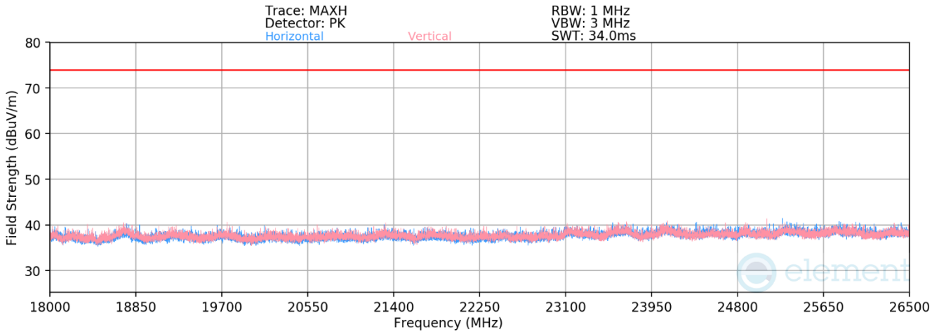
Plot 7-41. Radiated Spurious Emissions Antenna WF7b (802.15.4 ePA – Ch.11)
