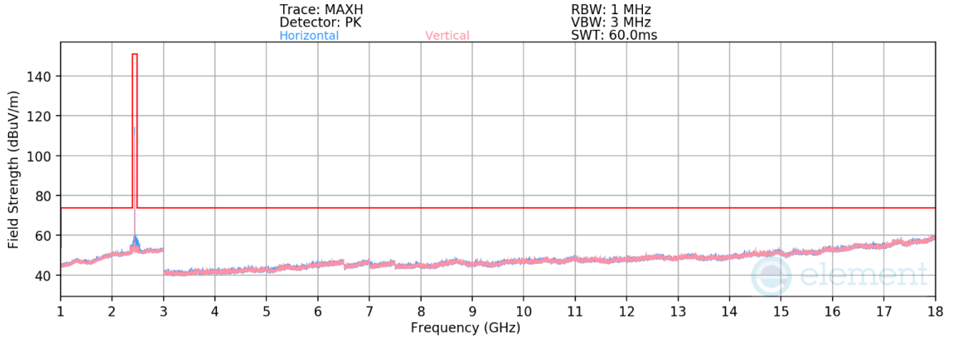
Plot 7-39. Radiated Spurious Emissions 1-18GHz Antenna WF7b (802.15.4 ePA – Ch. 18)
