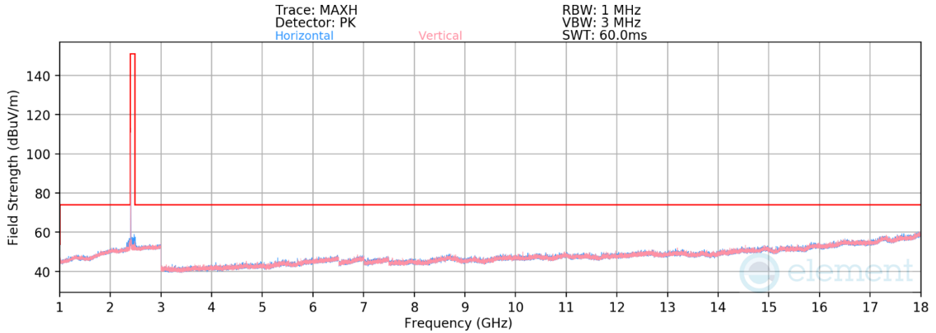
Plot 7-38. Radiated Spurious Emissions 1-18GHz Antenna WF7b (802.15.4 ePA – Ch. 11)
