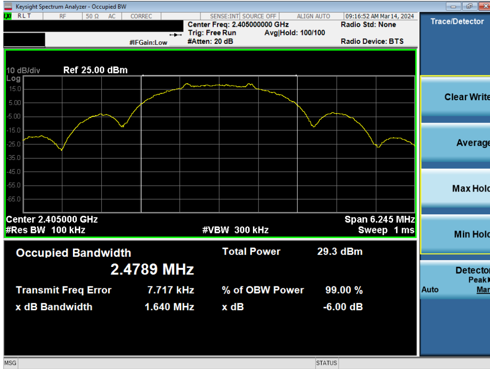
Plot 7-1. 6dB BW & 99% OBW Antenna WF8 (802.15.4, Ch. 11)
