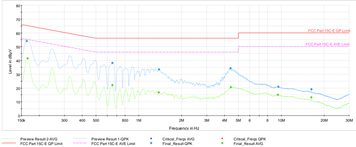
Plot 7-47. AC Line Conducted Emission with 802.15.4 Antenna WF7b (L1, 250 kbps, ePA - Ch.11, with AC/DC Adapter)
