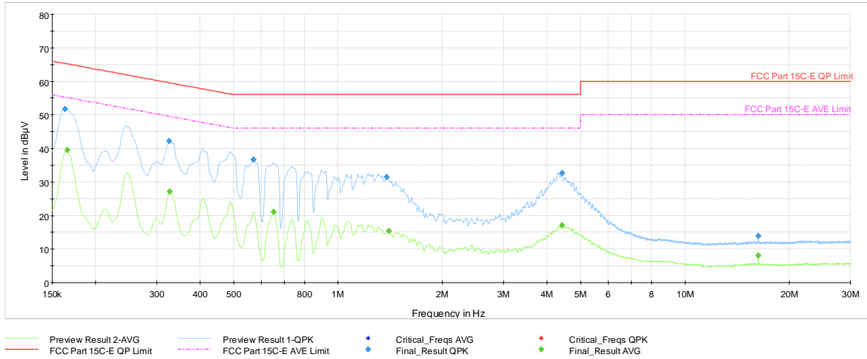
Plot 7-48. AC Line Conducted Emission with 802.15.4 Antenna WF7b (N, 250 kbps, ePA - Ch.11, with AC/DC Adapter)
