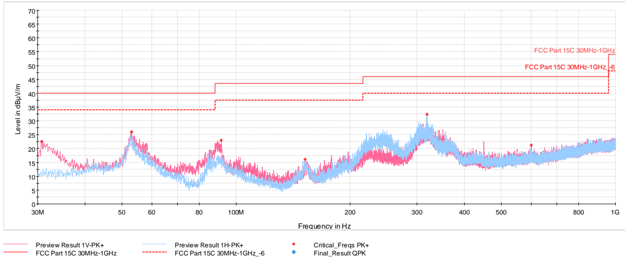
Plot 7-46. Radiated Spurious Emissions 30MHz-1GHz Antenna WF7b (250kbps, ePA - Ch.11, with Laptop)
