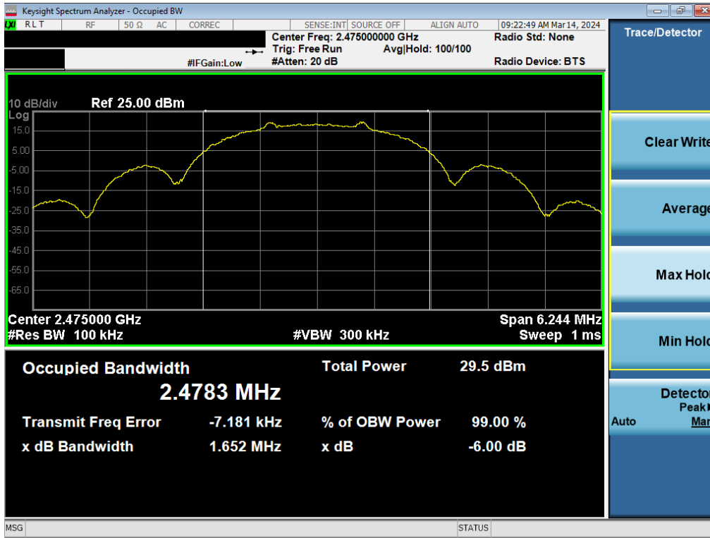
Plot 7-6. 6dB BW & 99% OBW Antenna WF7b (802.15.4, Ch. 25)
