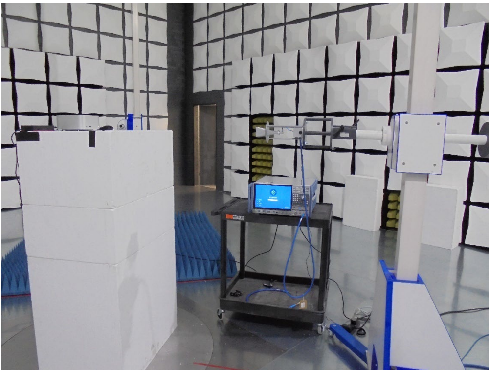
Figure 3 Radiated Disturbance - Above 1 GHz
