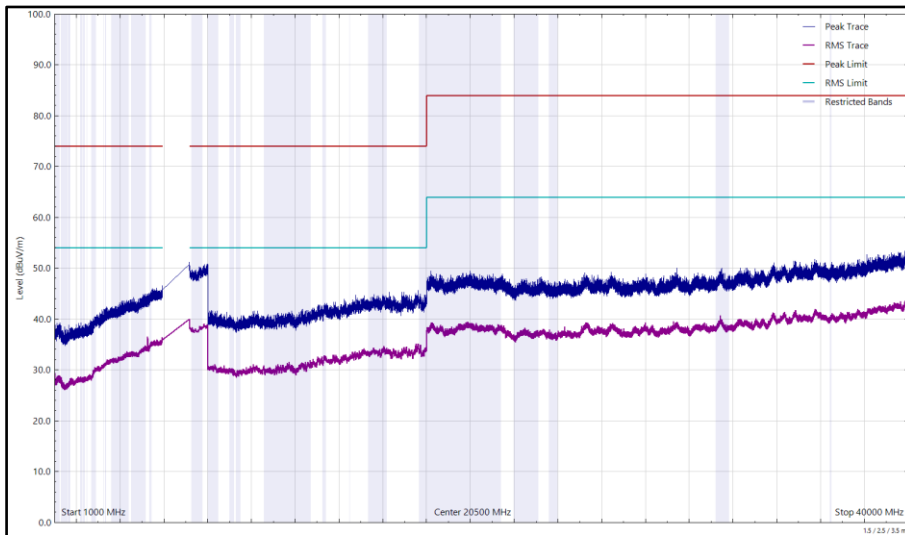
Figure 140 - U-NII-8 - 6995 MHz (CH209), HE20, SU, CDD, Core 0 + Core 1, 1 GHz to 40 GHz, Horizontal
