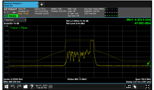
Figure 158 - A (Core 0) 802.11ax HE20 RU26 6255 MHz (CH61)
