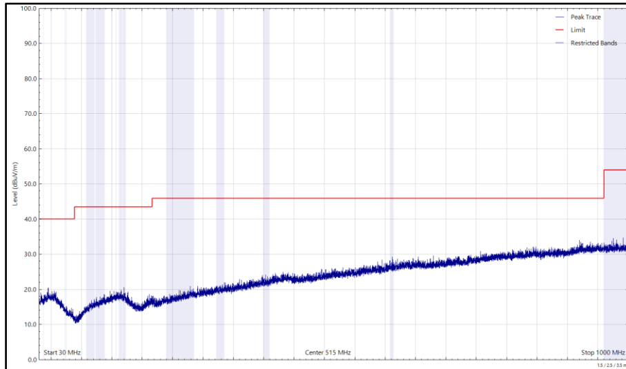
Figure 131 - U-NII-7 - 6695 MHz (CH149), HE20, SU, CDD, Core 0 + Core 1, 30 MHz to 1 GHz, Horizontal (Peak)
