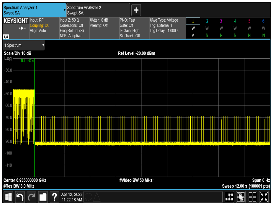
Figure 187 - U-NII-8, Minimum Bandwidth (AWGN High)
