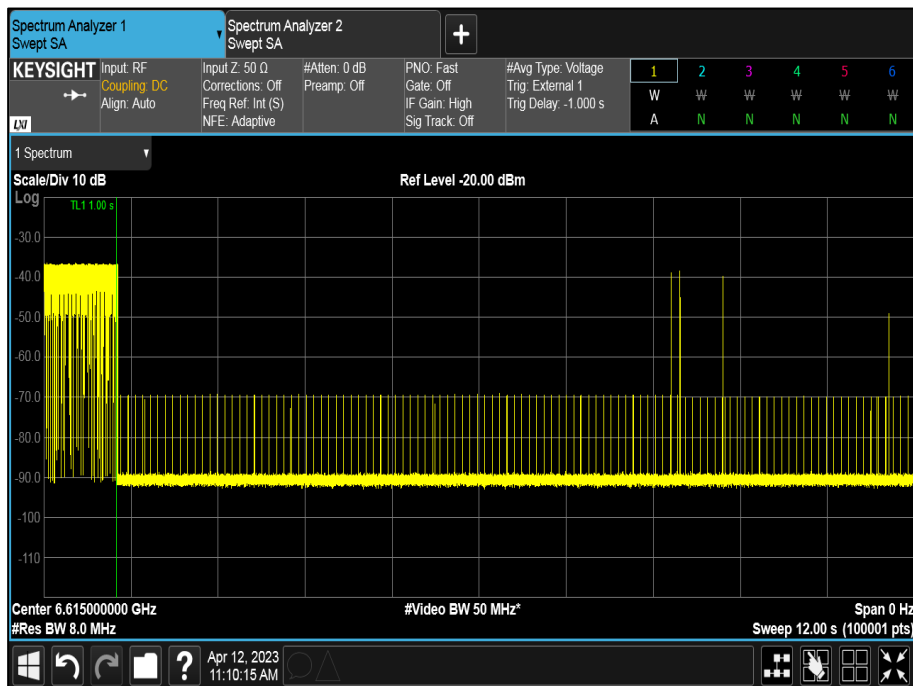
Figure 182 - U-NII-7, Minimum Bandwidth (AWGN Mid)
