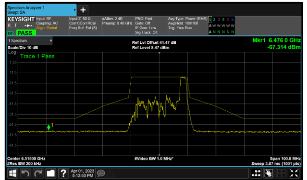
Figure 151 - A (Core 0) 802.11ax HE20 RU26 6515 MHz (CH113)
