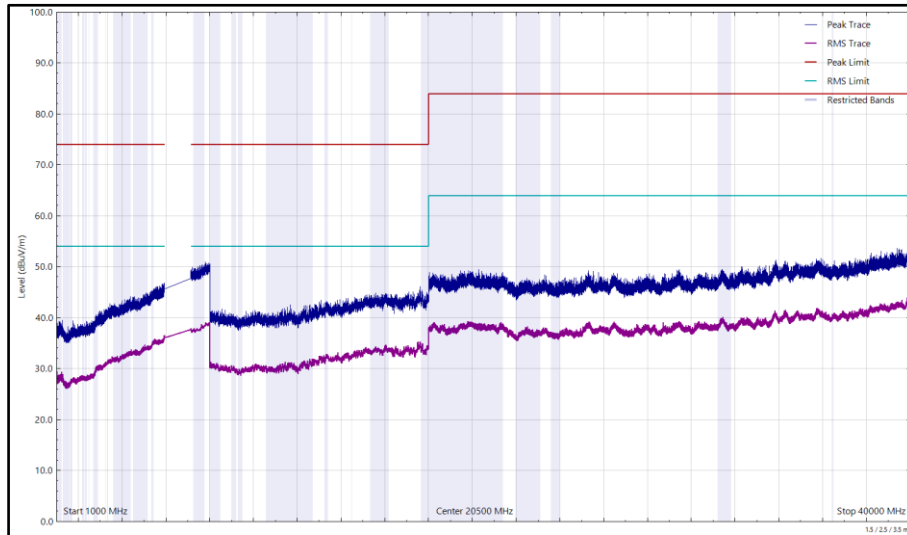
Figure 121 - U-NII-6 - 6435 MHz (CH97), HE20, SU, CDD, Core 0 + Core 1, 1 GHz to 40 GHz, Horizontal
