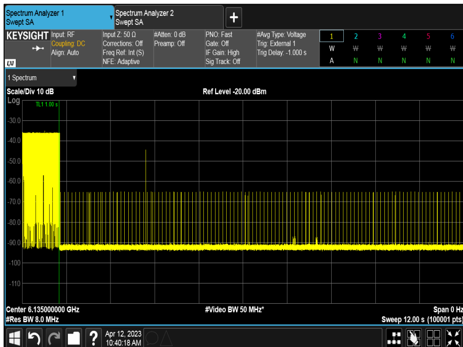
Figure 173 - U-NII-5, Minimum Bandwidth (AWGN Low)
