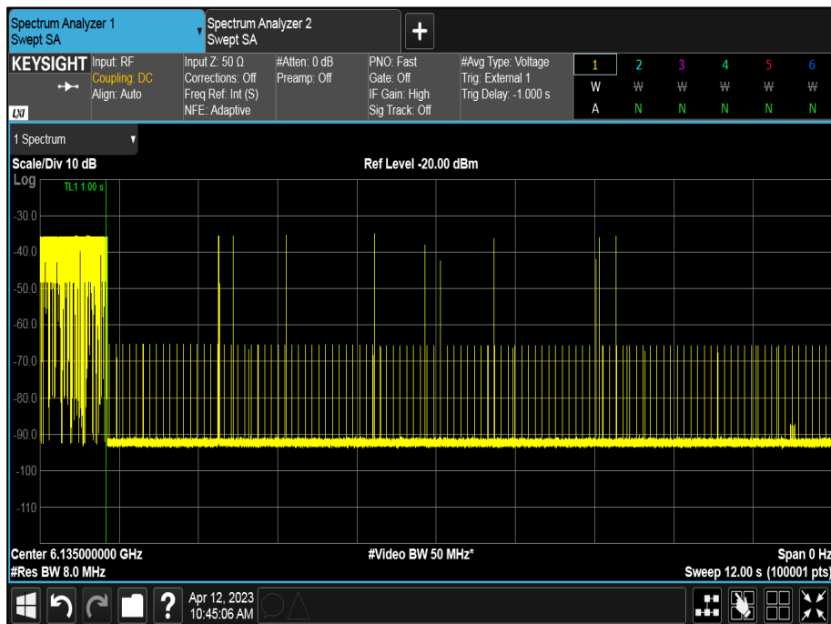
Figure 174 - U-NII-5, Minimum Bandwidth (AWGN Mid)
