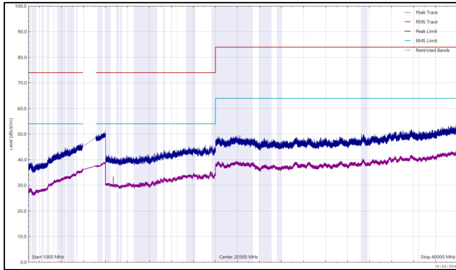
Figure 129 - U-NII-7 - 6535 MHz (CH117), HE20, SU, CDD, Core 0 + Core 1, 1 GHz to 40 GHz, Horizontal
