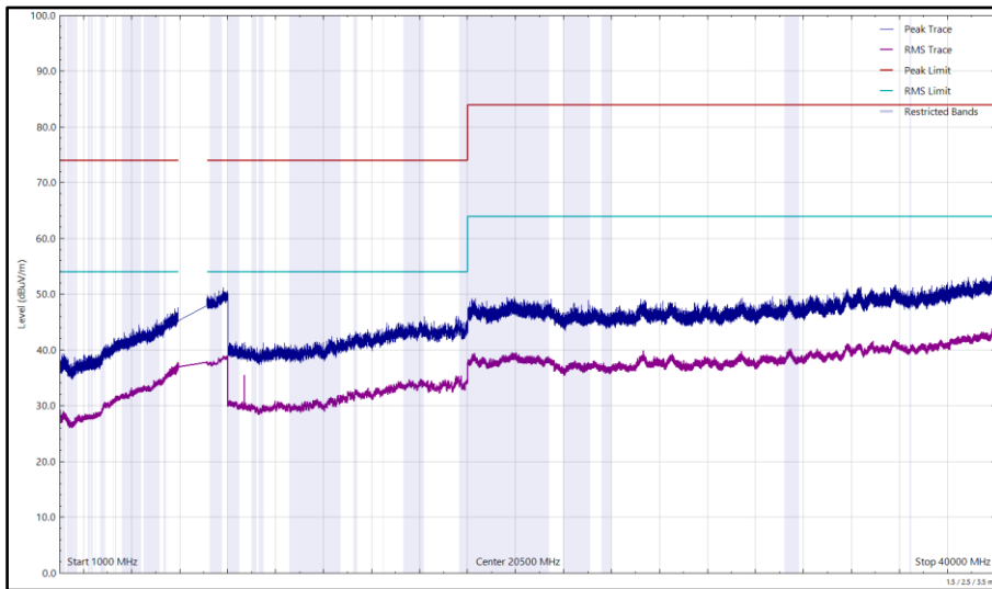
Figure 128 - U-NII-6 - 6515 MHz (CH113), HE20, SU, CDD, Core 0 + Core 1, 1 GHz to 40 GHz, Vertical
