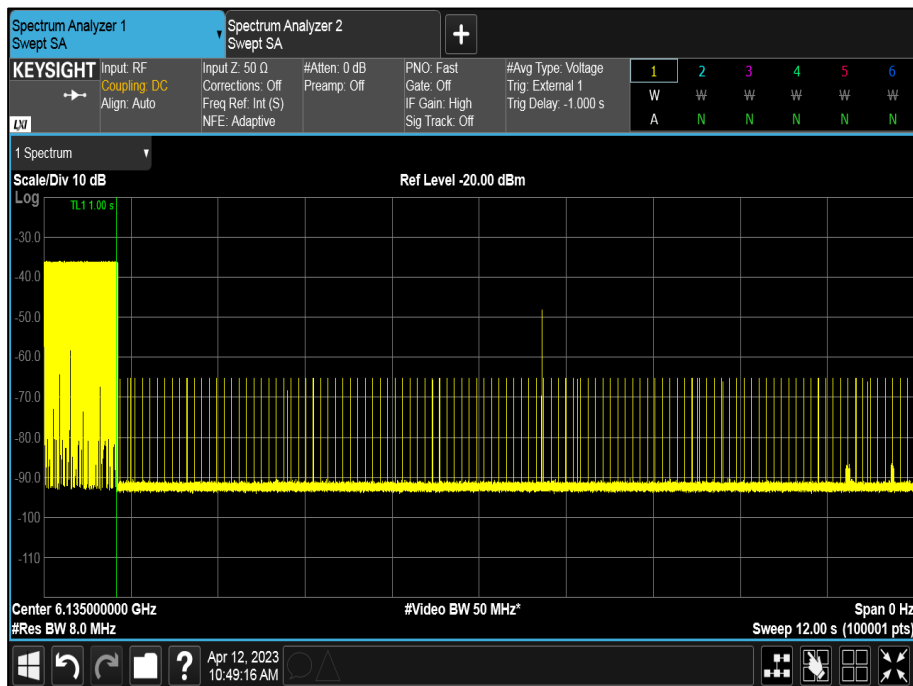
Figure 175 - U-NII-5, Minimum Bandwidth (AWGN High)
