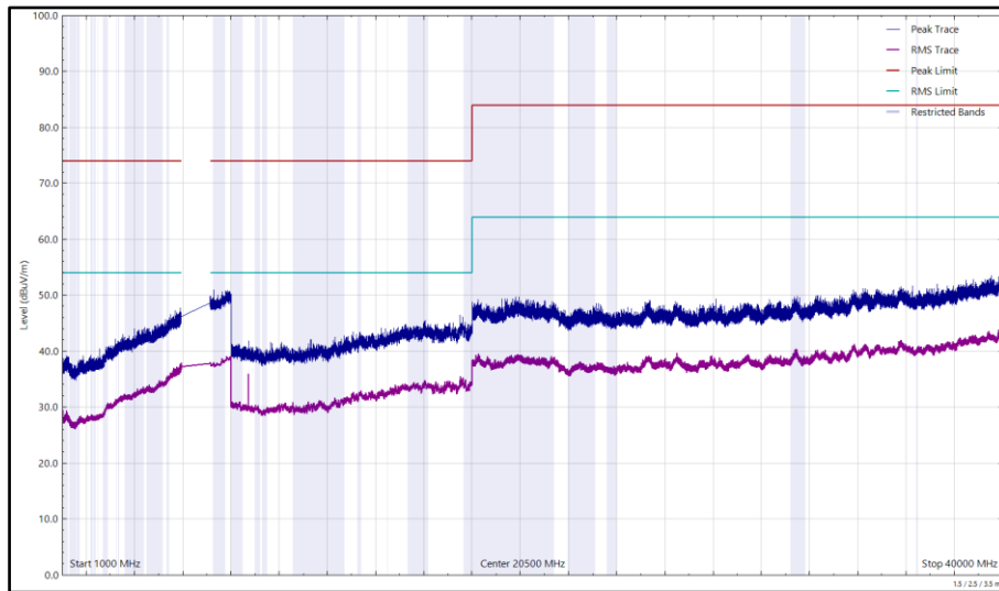
Figure 130 - U-NII-7 - 6535 MHz (CH117), HE20, SU, CDD, Core 0 + Core 1, 1 GHz to 40 GHz, Vertical
