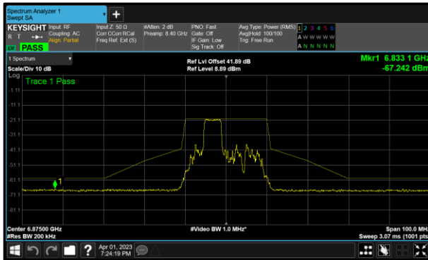
Figure 159 - A (Core 0) 802.11ax HE20 RU52 6875 MHz (CH185)
