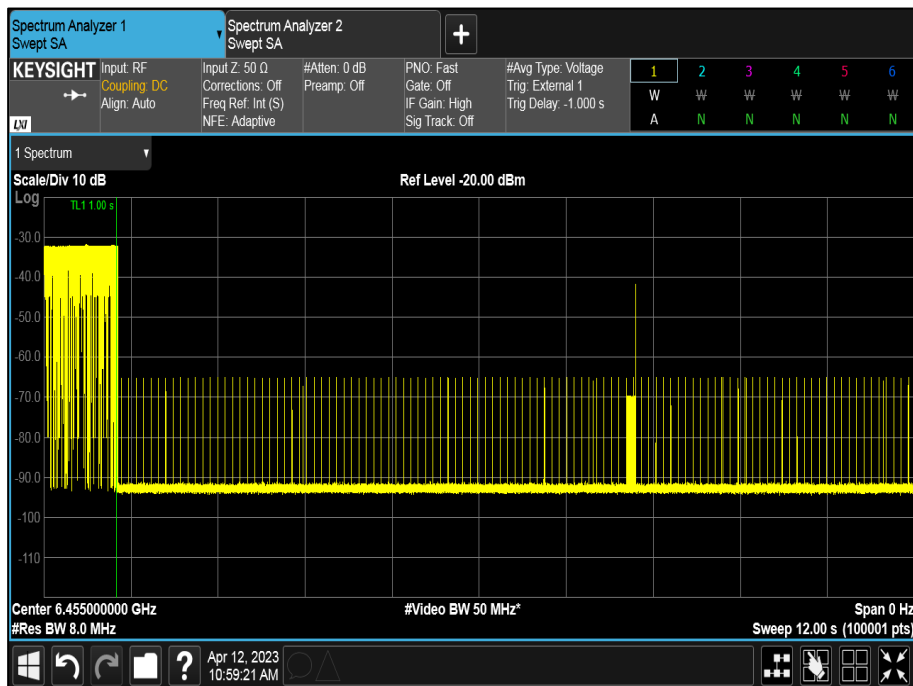
Figure 179 - U-NII-6, Minimum Bandwidth (AWGN High)
