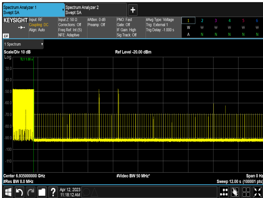
Figure 185 - U-NII-8, Minimum Bandwidth (AWGN Low)
