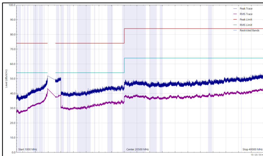
Figure 118 - U-NII-5 - 6175 MHz (CH45), HE20, SU, CDD, Core 0 + Core 1, 1 GHz to 40 GHz, Vertical
