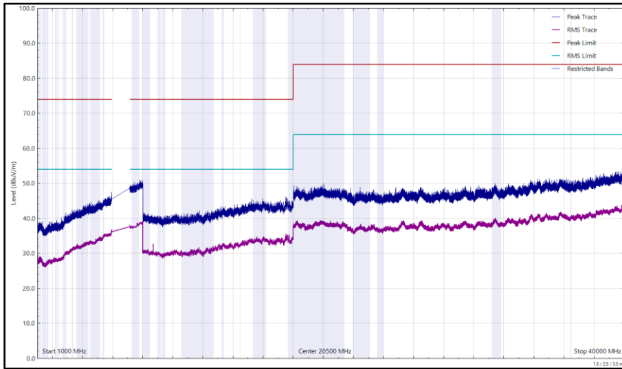
Figure 127 - U-NII-6 - 6515 MHz (CH113), HE20, SU, CDD, Core 0 + Core 1, 1 GHz to 40 GHz, Horizontal
