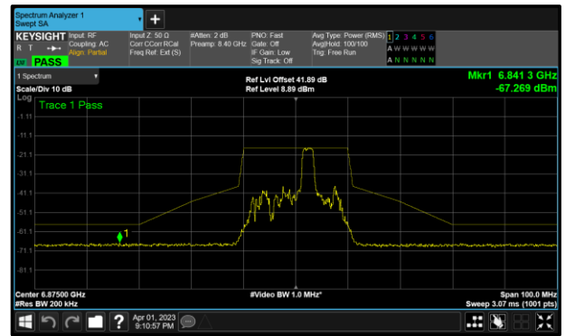
Figure 165 - A (Core 0) 802.11ax HE20 RU26 6875 MHz (CH185)
