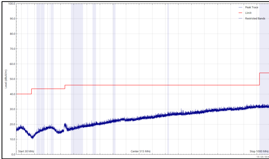
Figure 123 - U-NII-6 - 6475 MHz (CH105), HE20, SU, CDD, Core 0 + Core 1, 30 MHz to 1 GHz, Horizontal (Peak)
