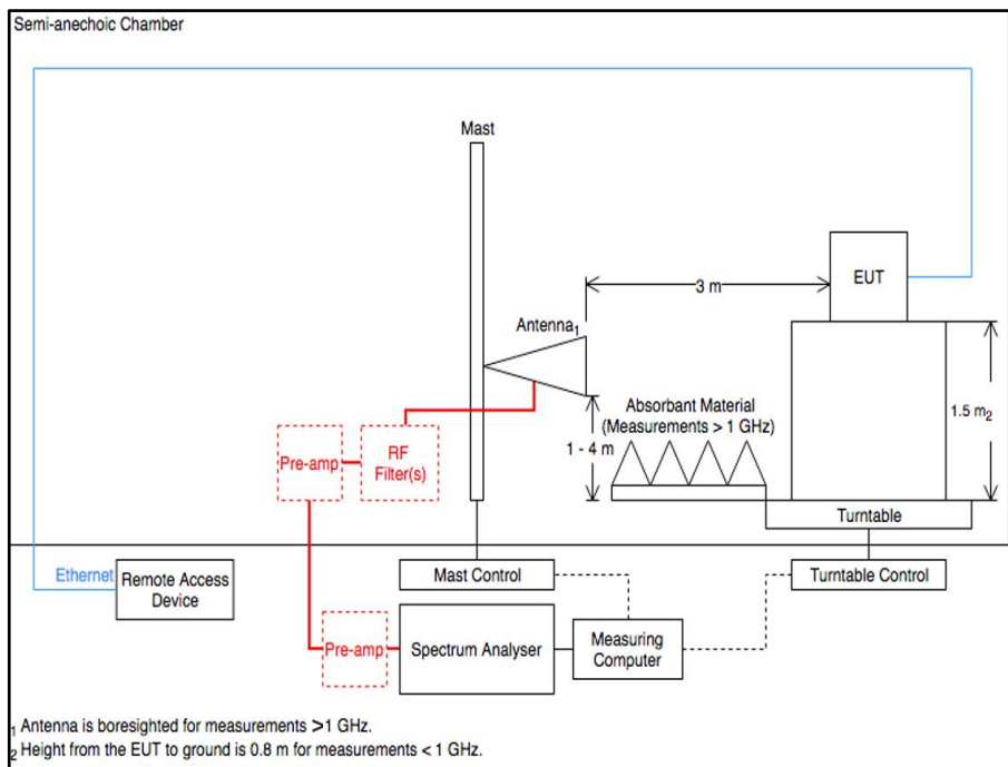
Figure 112 - Radiated Emissions Test Setup Diagram
