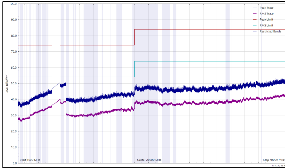
Figure 135 - U-NII-7 - 6855 MHz (CH181), HE20, SU, CDD, Core 0 + Core 1, 1 GHz to 40 GHz, Horizontal
