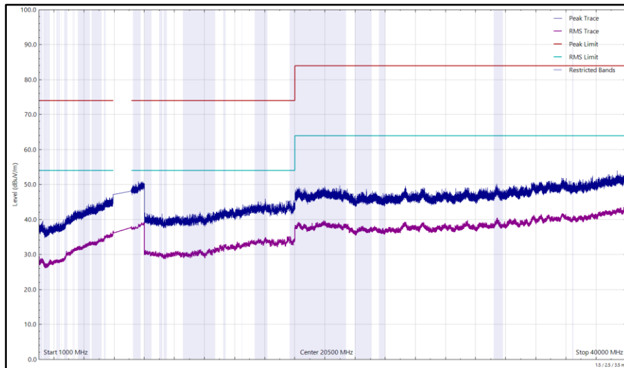
Figure 132 - U-NII-7 - 6695 MHz (CH149), HE20, SU, CDD, Core 0 + Core 1, 1 GHz to 40 GHz, Horizontal
