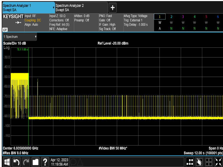
Figure 186 - U-NII-8, Minimum Bandwidth (AWGN Mid)
