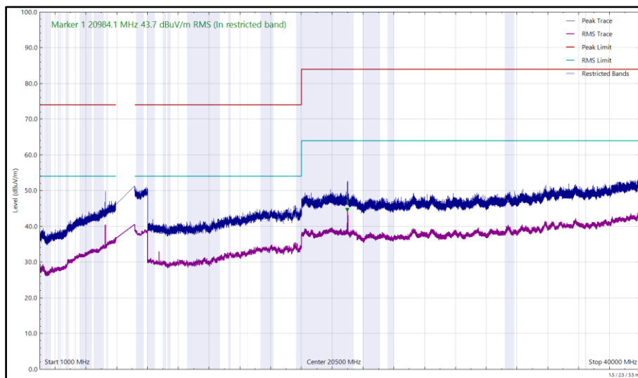
Figure 142 - U-NII-8 - 6995 MHz (CH209), HE20, SU, CDD, Core 0 + Core 1, 1 GHz to 40 GHz, Vertical
