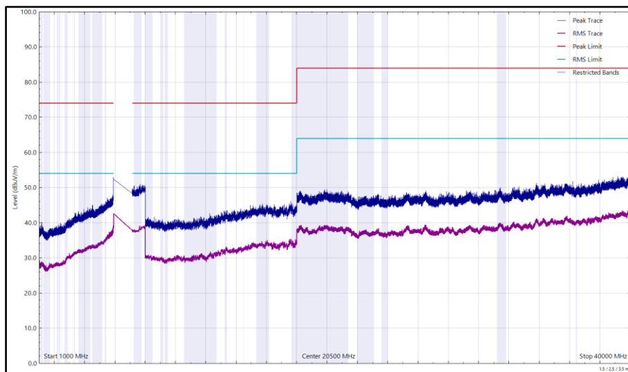
Figure 120 - U-NII-5 - 6415 MHz (CH93), HE20, SU, CDD, Core 0 + Core 1, 1 GHz to 40 GHz, Vertical
