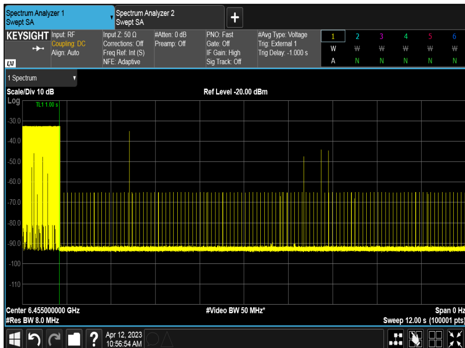
Figure 178 - U-NII-6, Minimum Bandwidth (AWGN Mid)
