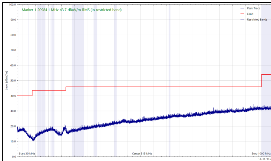
Figure 141 - U-NII-8 - 6995 MHz (CH209), HE20, SU, CDD, Core 0 + Core 1, 30 MHz to 1 GHz, Vertical (Peak)
