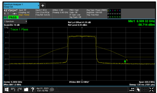
Figure 148 - A (Core 0) 802.11ax HE80 SU 6385 MHz (CH87)
