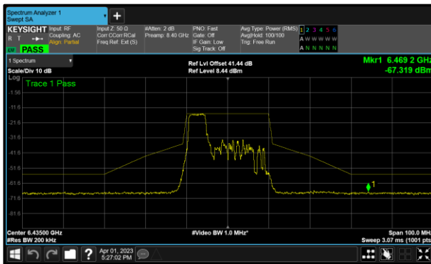
Figure 152 - A (Core 0) 802.11ax HE20 RU52 6435 MHz (CH97)
