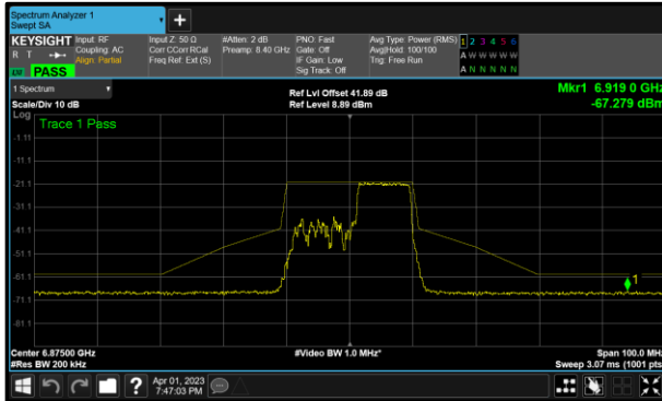
Figure 157 - A (Core 0) 802.11ax HE20 RU106 6875 MHz (CH185)
