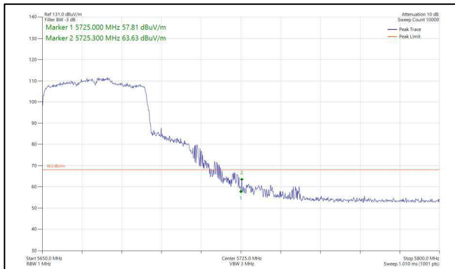
Figure 426 - 802.11ax, HE40, SU, TxBF, Core 0-1 - 5670 MHz, Band Edge Frequency 5725 MHz
