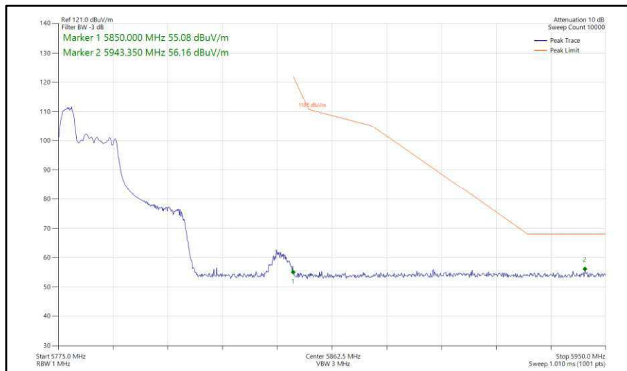
Figure 366 - 802.11ax, HE40, RU 52-37, SISO, Core 0 - 5795 MHz, Band Edge Frequency 5850 MHz
