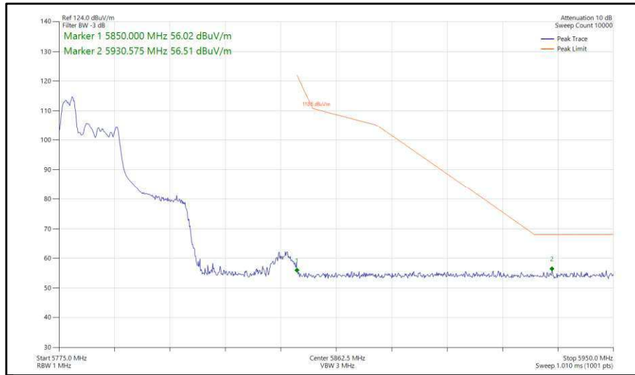
Figure 420 - 802.11ax, HE40, RU 52-37, SDM, Core 0-1 - 5795 MHz, Band Edge Frequency 5850 MHz
