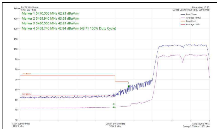
Figure 403 - 802.11n, HT40, SDM, Core 0-1 - 5510 MHz, Band Edge Frequency 5470 MHz
