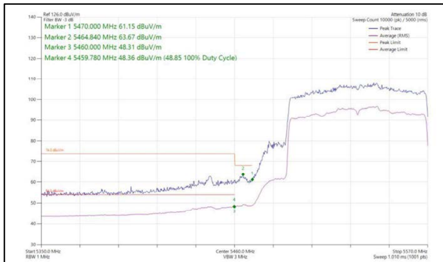
Figure 478 - 802.11ax, HE80, SU, SDM, Core 0-1 - 5530 MHz, Band Edge Frequency 5470 MHz
