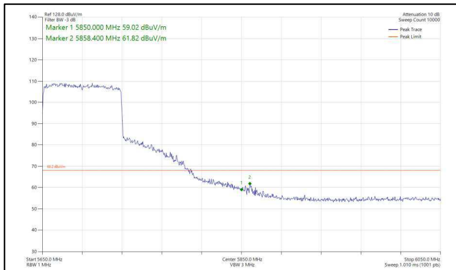
Figure 458 - 802.11ax, HE80, SU, SISO, Core 1 - 5690 MHz, Band Edge Frequency 5850 MHz
