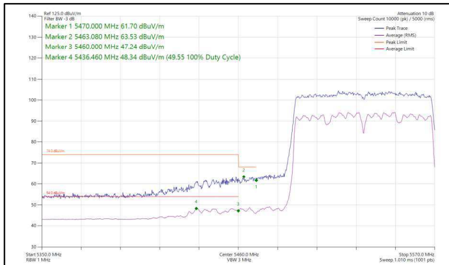
Figure 477 - 802.11ac, VHT80, SDM, Core 0-1 - 5530 MHz, Band Edge Frequency 5470 MHz
