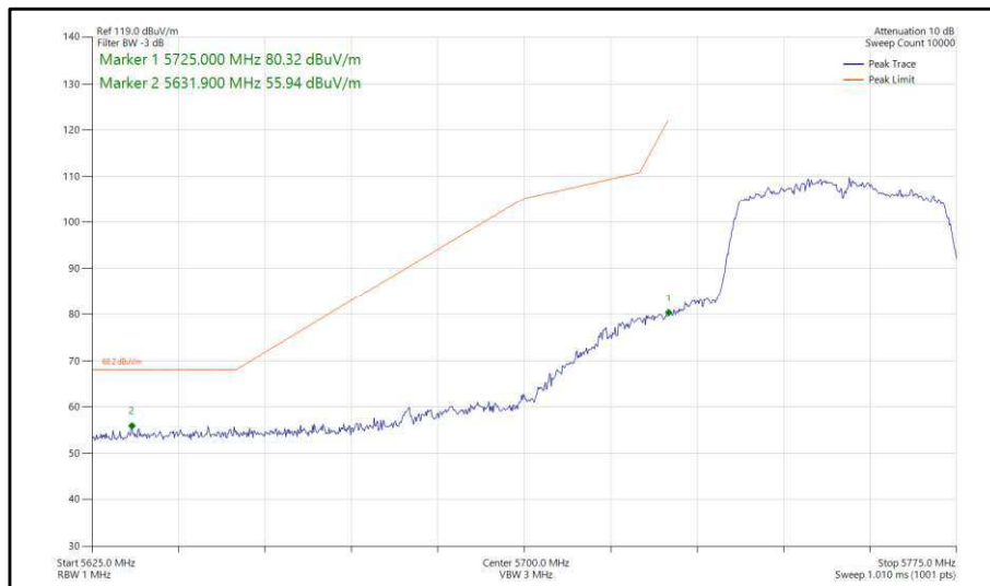
Figure 370 - 802.11n, HT40, SISO, Core 1 - 5755 MHz, Band Edge Frequency 5725 MHz
