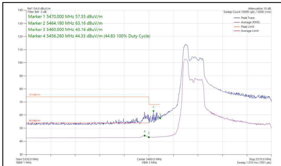
Figure 434 - 802.11ax, HE80, RU 52-37, SISO, Core 0 - 5530 MHz, Band Edge Frequency 5470 MHz
