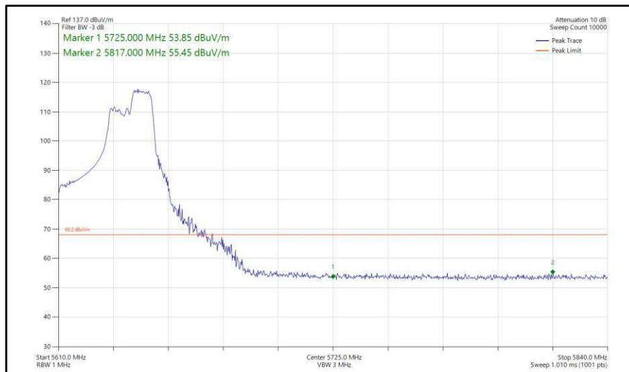
Figure 376 - 802.11ax, HE40, RU 106-56, SISO, Core 1 - 5630 MHz, Band Edge Frequency 5725 MHz
