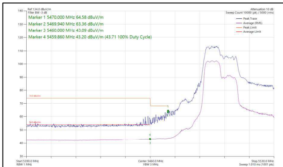
Figure 387 - 802.11ax, HE40, RU 106-53, CDD, Core 0-1 - 5510 MHz, Band Edge Frequency 5470 MHz
