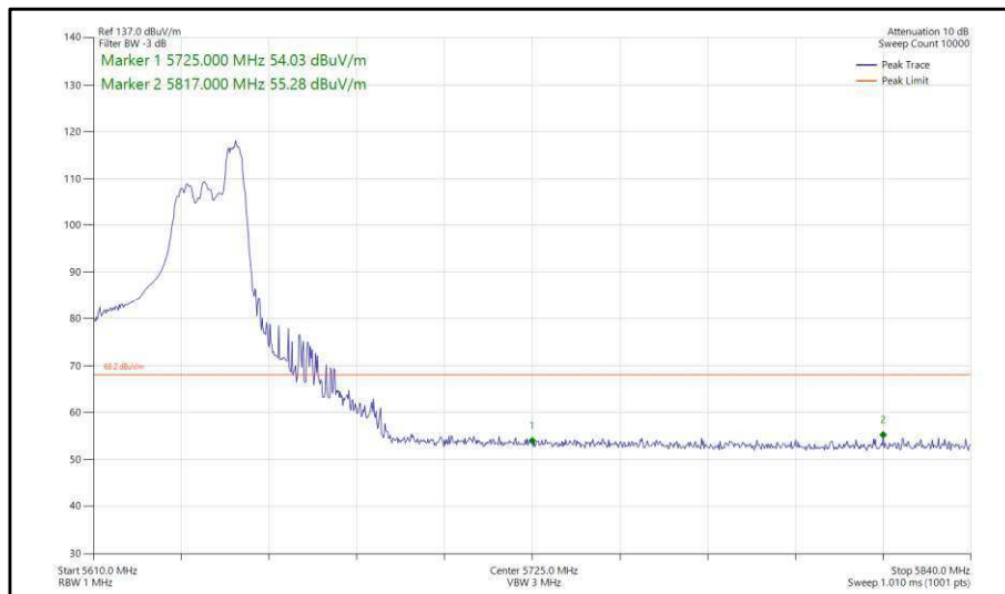
Figure 412 - 802.11ax, HE40, RU 52-44, SDM, Core 0-1 - 5630 MHz, Band Edge Frequency 5725 MHz
