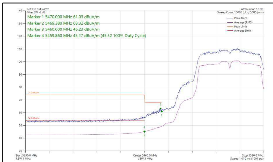
Figure 367 - 802.11n, HT40, SISO, Core 1 - 5510 MHz, Band Edge Frequency 5470 MHz
