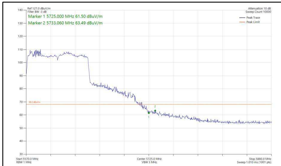
Figure 494 - 802.11ac, VHT80, TxBF, Core 0-1 - 5610 MHz, Band Edge Frequency 5725 MHz
