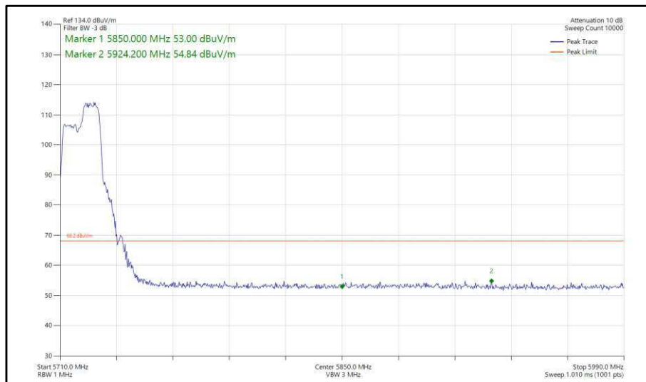
Figure 341 - 802.11ax, HE20, RU 106-54, SDM, Core 0-1 - 5720 MHz, Band Edge Frequency 5850 MHz
