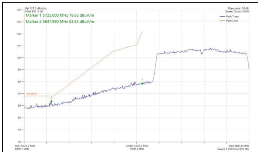
Figure 450 - 802.11ac, VHT80, SISO, Core 1 - 5775 MHz, Band Edge Frequency 5725 MHz
