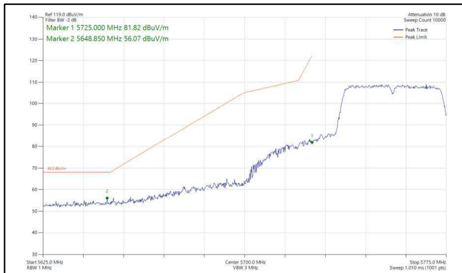
Figure 352 - 802.11n, HT40, SISO, Core 0 - 5755 MHz, Band Edge Frequency 5725 MHz
