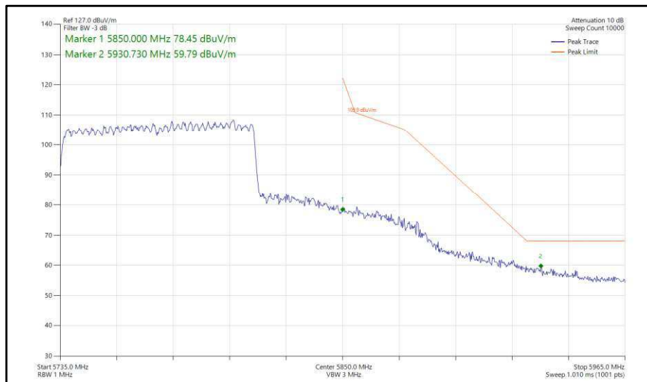
Figure 475 - 802.11ax, HE80, SU, CDD, Core 0-1 - 5775 MHz, Band Edge Frequency 5850 MHz
