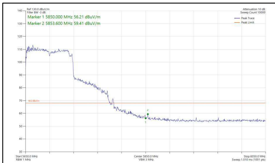
Figure 495 - 802.11ac, VHT80, TxBF, Core 0-1 - 5690 MHz, Band Edge Frequency 5850 MHz
