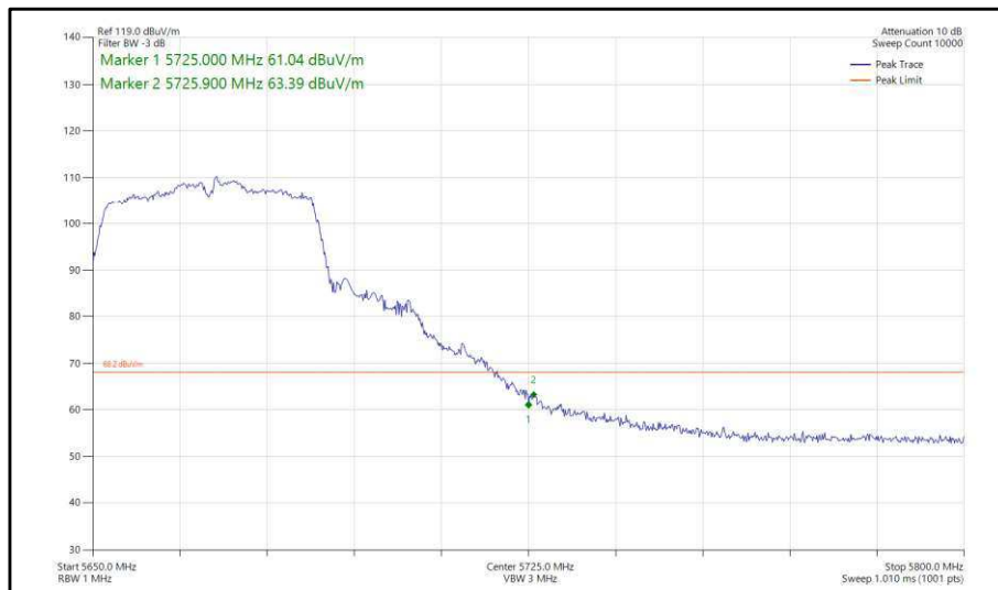
Figure 410 - 802.11n, HT40, SDM, Core 0-1 - 5670 MHz, Band Edge Frequency 5725 MHz
