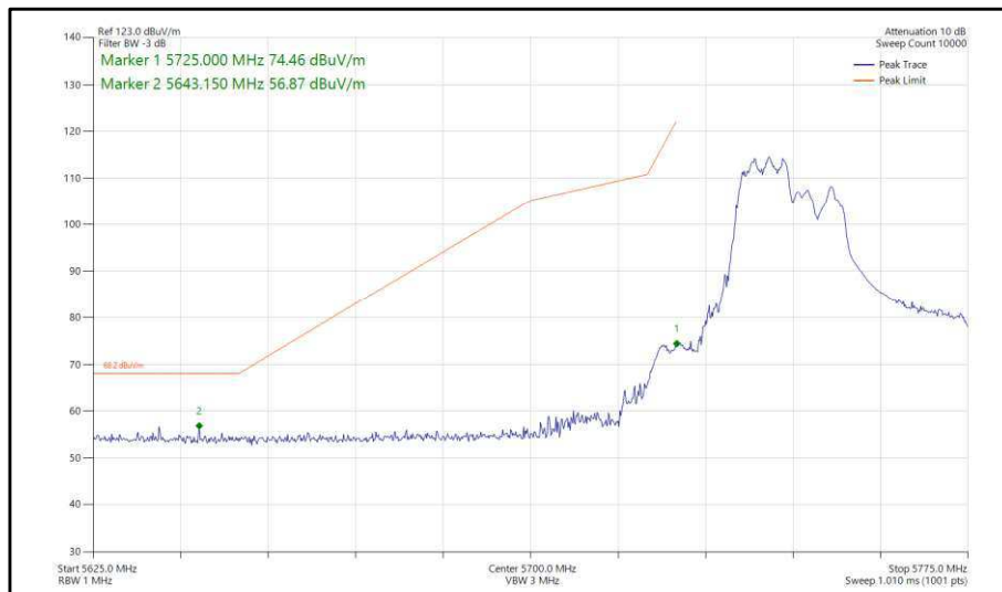
Figure 390 - 802.11ax, HE40, RU 106-53, CDD, Core 0-1 - 5755 MHz, Band Edge Frequency 5725 MHz
