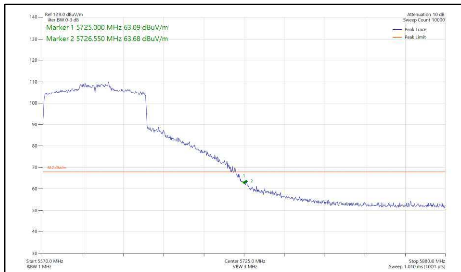
Figure 484 - 802.11ax, HE80, SU, SDM, Core 0-1 - 5610 MHz, Band Edge Frequency 5725 MHz
