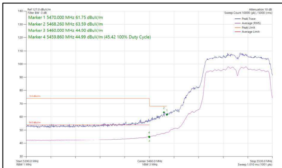
Figure 385 - 802.11n, HT40, CDD, Core 0-1 - 5510 MHz, Band Edge Frequency 5470 MHz
