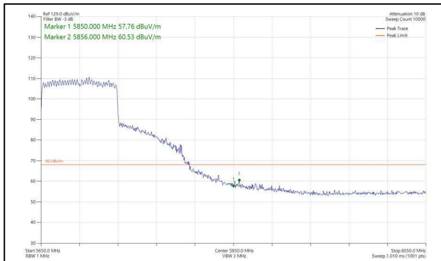
Figure 473 - 802.11ax, HE80, SU, CDD, Core 0-1 - 5690 MHz, Band Edge Frequency 5850 MHz
