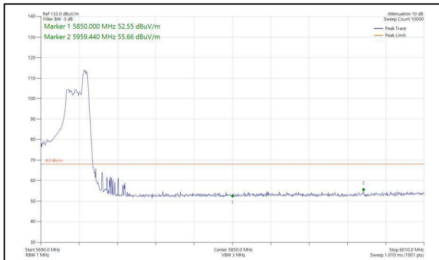
Figure 382 - 802.11ax, HE40, RU 52-44, SISO, Core 1 - 5710 MHz, Band Edge Frequency 5850 MHz
