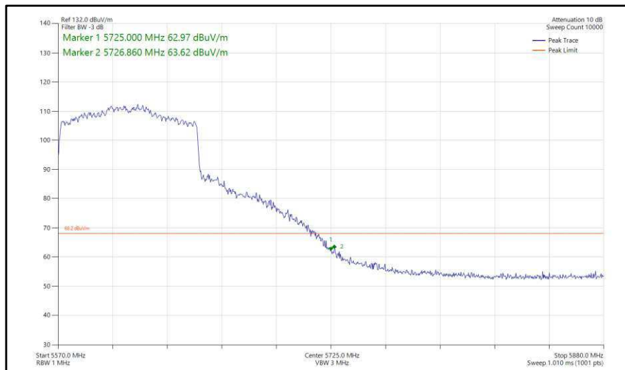
Figure 469 - 802.11ax, HE80, SU, CDD, Core 0-1 - 5610 MHz, Band Edge Frequency 5725 MHz
