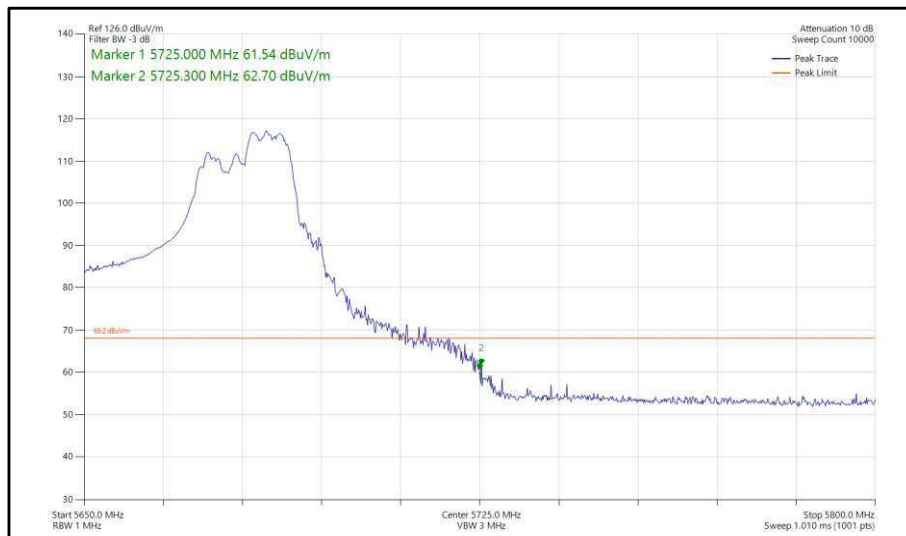
Figure 396 - 802.11ax, HE40, RU 106-56, CDD, Core 0-1 - 5670 MHz, Band Edge Frequency 5725 MHz
