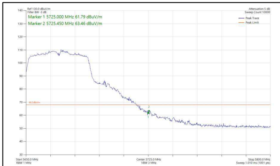
Figure 356 - 802.11n, HT40, SISO, Core 0 - 5670 MHz, Band Edge Frequency 5725 MHz
