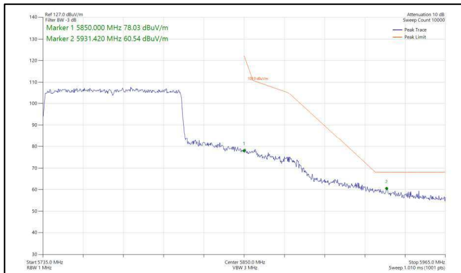
Figure 460 - 802.11ax, HE80, SU, SISO, Core 1 - 5775 MHz, Band Edge Frequency 5850 MHz
