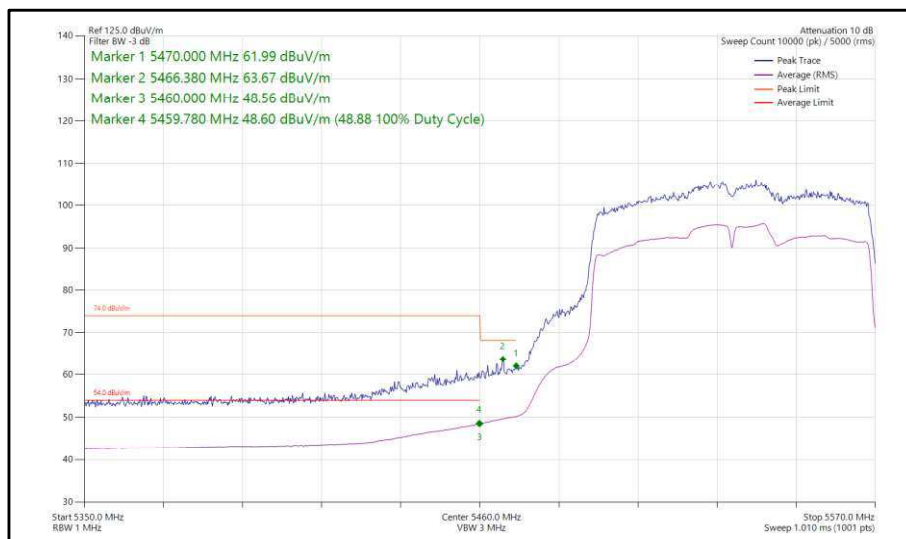
Figure 492 - 802.11ac, VHT80, TxBF, Core 0-1 - 5530 MHz, Band Edge Frequency 5470 MHz
