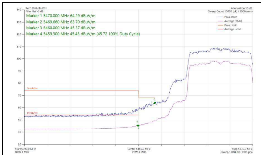
Figure 386 - 802.11ax, HE40, SU, CDD, Core 0-1 - 5510 MHz, Band Edge Frequency 5470 MHz
