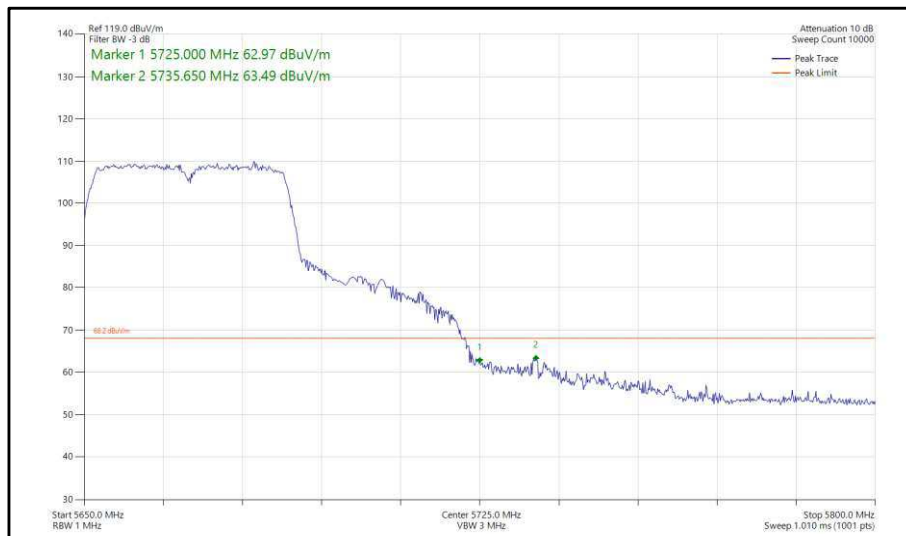
Figure 374 - 802.11n, HT40, SISO, Core 1 - 5670 MHz, Band Edge Frequency 5725 MHz
