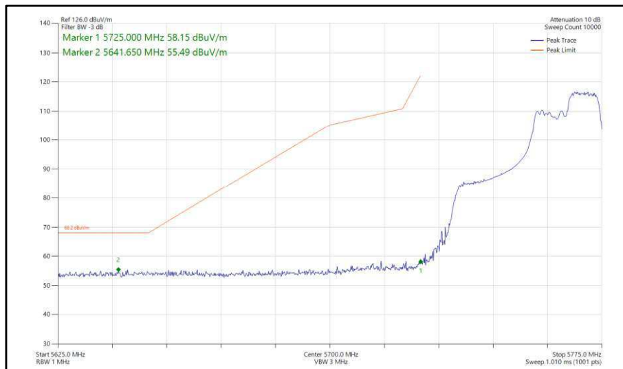
Figure 372 - 802.11ax, HE40, RU 106-56, SISO, Core 1 - 5755 MHz, Band Edge Frequency 5725 MHz
