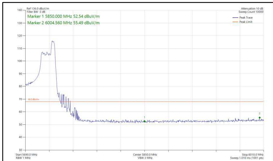
Figure 364 - 802.11ax, HE40, RU 52-44, SISO, Core 0 - 5710 MHz, Band Edge Frequency 5850 MHz
