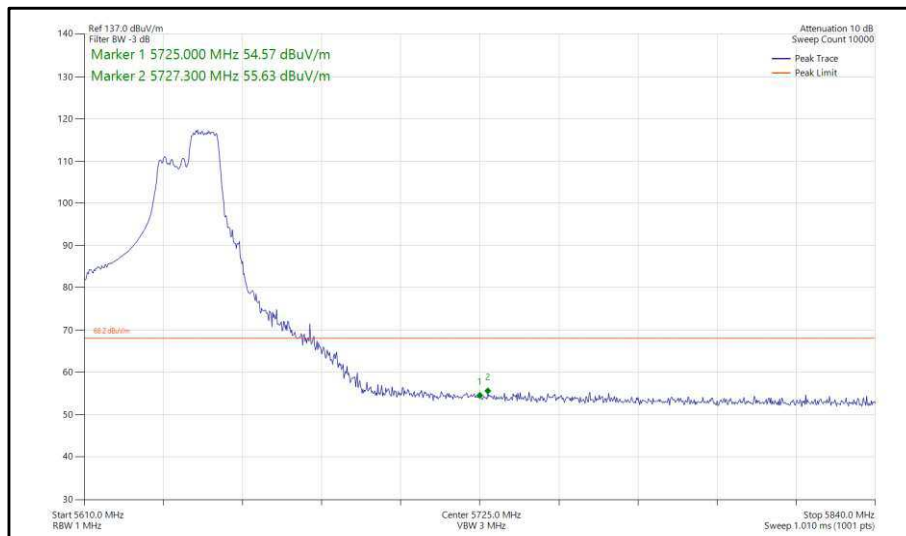
Figure 358 - 802.11ax, HE40, RU 106-56, SISO, Core 0 - 5630 MHz, Band Edge Frequency 5725 MHz
