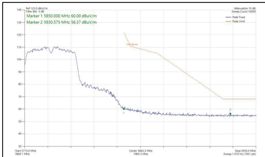
Figure 398 - 802.11n, HT40, CDD, Core 0-1 - 5795 MHz, Band Edge Frequency 5850 MHz
