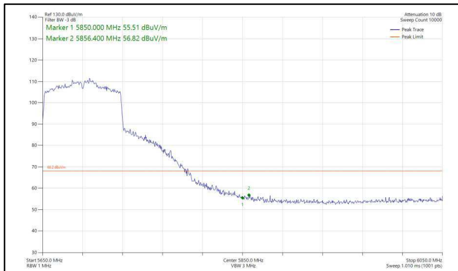
Figure 471 - 802.11ac, VHT80, CDD, Core 0-1 - 5690 MHz, Band Edge Frequency 5850 MHz
