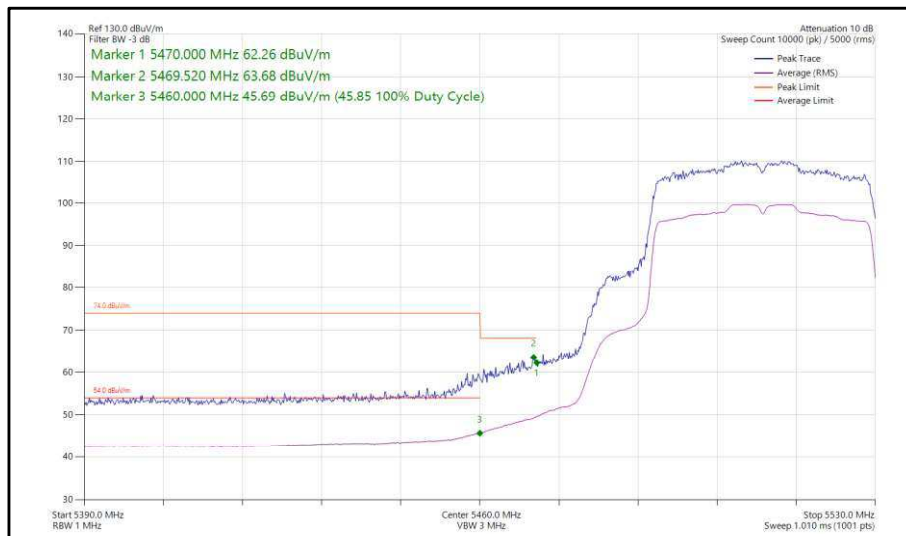
Figure 350 - 802.11ax, HE40, SU, SISO, Core 0 - 5510 MHz, Band Edge Frequency 5470 MHz
