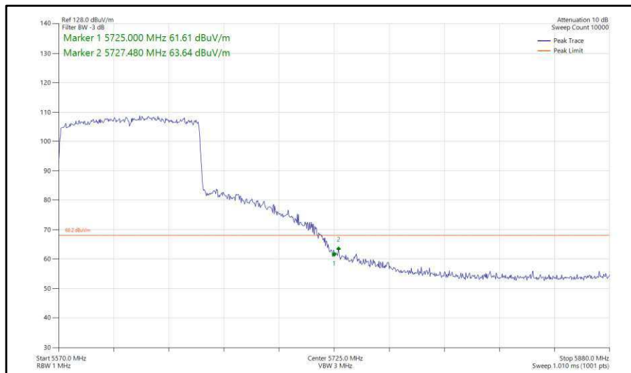
Figure 454 - 802.11ax, HE80, SU, SISO, Core 1 - 5610 MHz, Band Edge Frequency 5725 MHz
