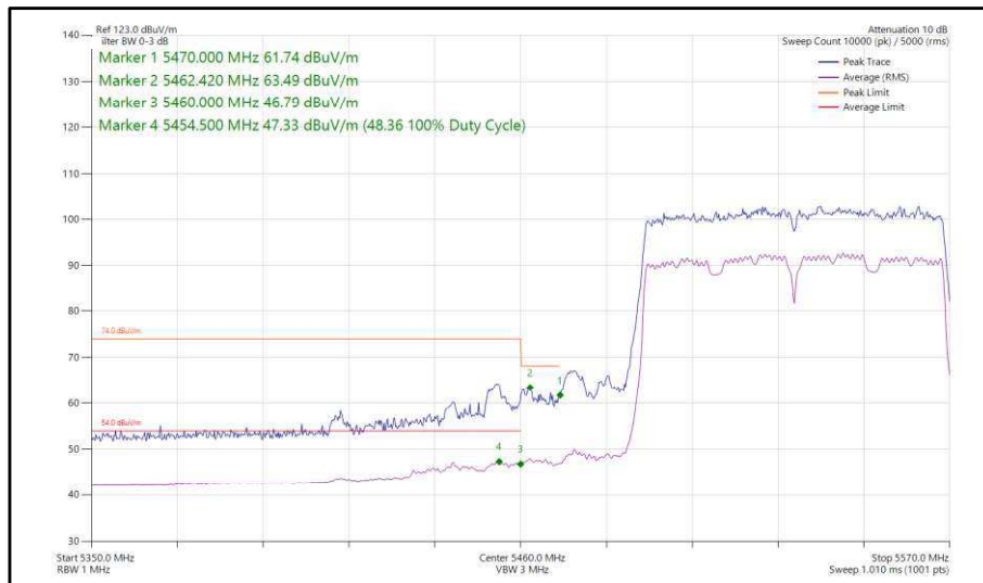
Figure 432 - 802.11ac, VHT80, SISO, Core 0 - 5530 MHz, Band Edge Frequency 5470 MHz
