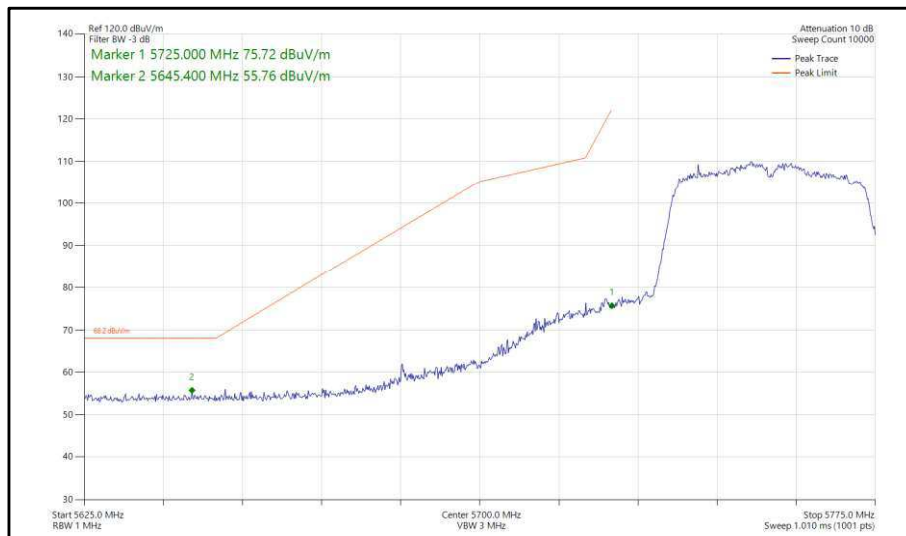
Figure 388 - 802.11n, HT40, CDD, Core 0-1 - 5755 MHz, Band Edge Frequency 5725 MHz
