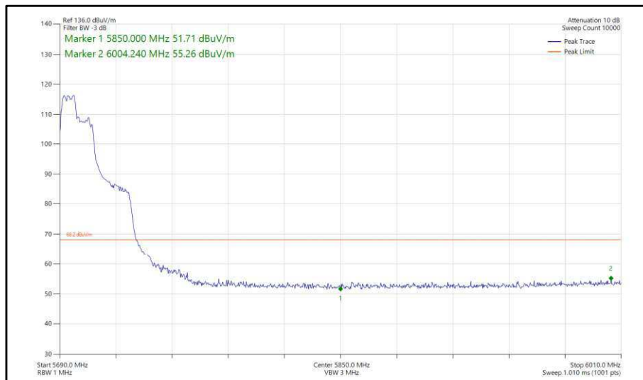
Figure 418 - 802.11ax, HE40, RU 106-53, SDM, Core 0-1 - 5710 MHz, Band Edge Frequency 5850 MHz
