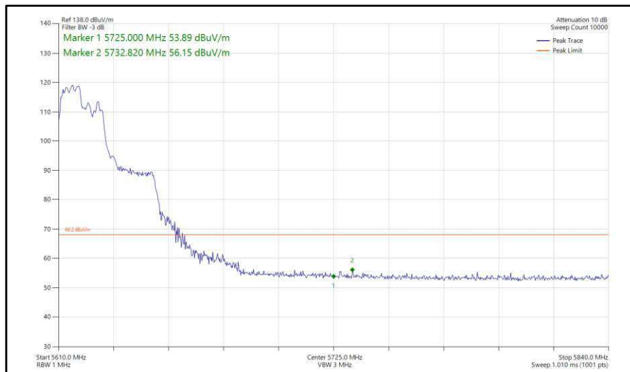
Figure 394 - 802.11ax, HE40, RU 106-53, CDD, Core 0-1 - 5630 MHz, Band Edge Frequency 5725 MHz
