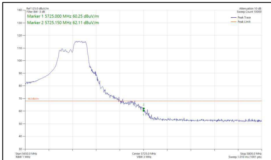
Figure 360 - 802.11ax, HE40, RU 106-56, SISO, Core 0 - 5670 MHz, Band Edge Frequency 5725 MHz
