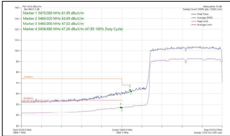
Figure 433 - 802.11ax, HE80, SU, SISO, Core 0 - 5530 MHz, Band Edge Frequency 5470 MHz
