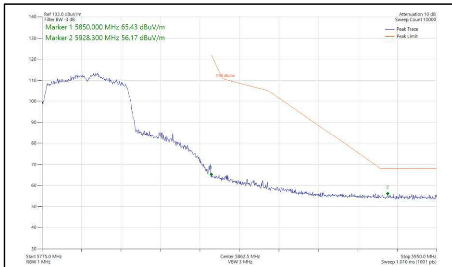
Figure 428 - 802.11n, HT40, TxBF, Core 0-1 - 5795 MHz, Band Edge Frequency 5850 MHz
