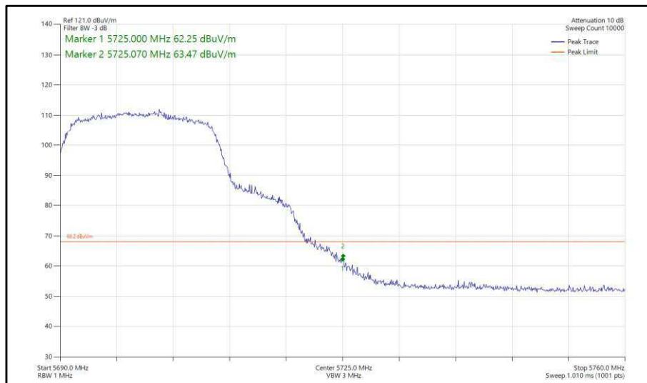
Figure 346 - 802.11n, HT20, TxBF, Core 0-1 - 5700 MHz, Band Edge Frequency 5725 MHz
