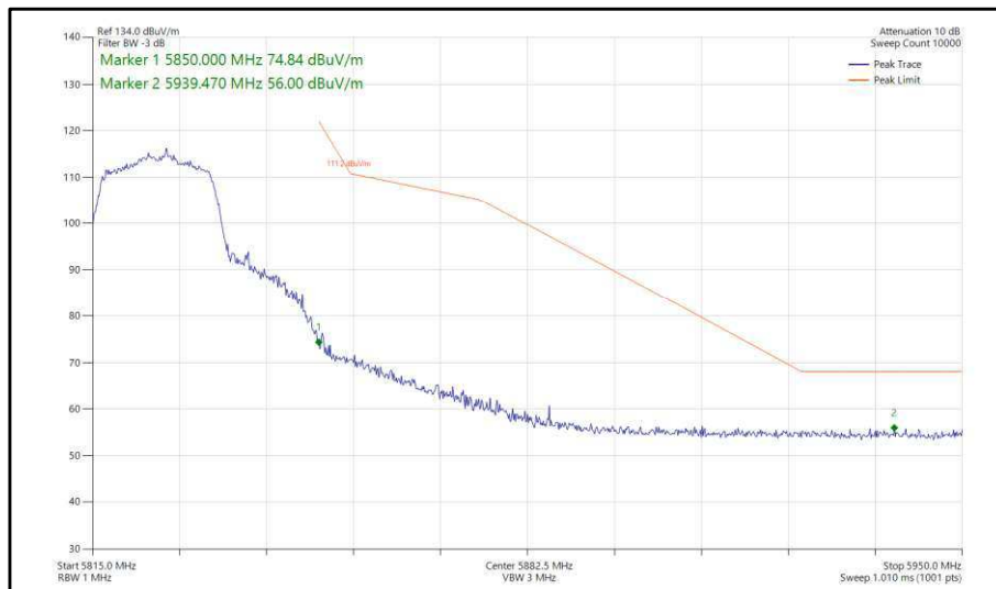
Figure 348 - 802.11n, HT20, TxBF, Core 0-1 - 5825 MHz, Band Edge Frequency 5850 MHz
