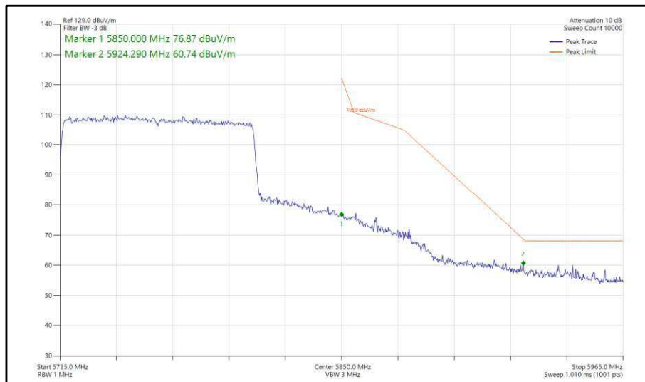
Figure 445 - 802.11ax, HE80, SU, SISO, Core 0 - 5775 MHz, Band Edge Frequency 5850 MHz
