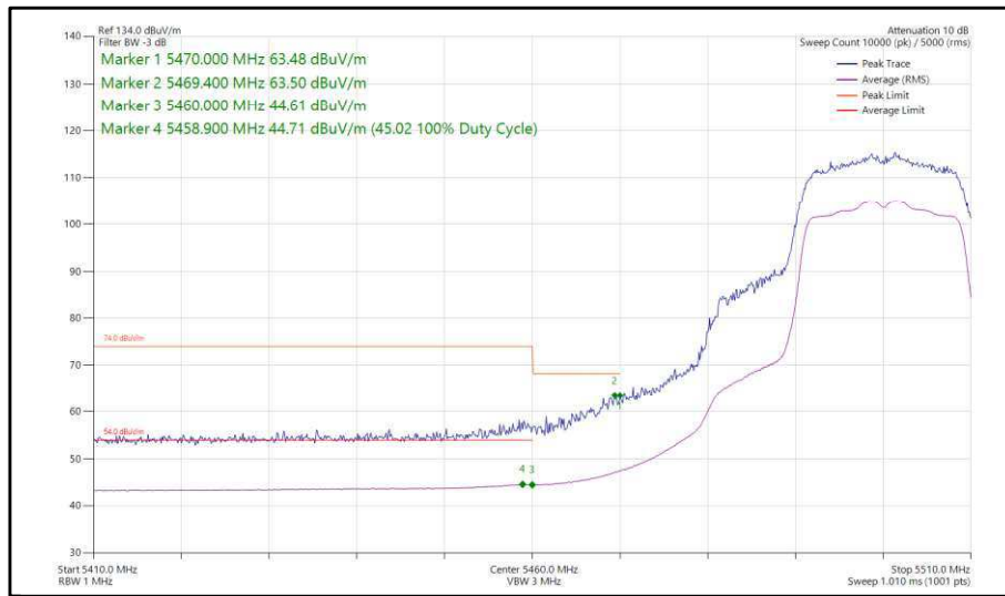
Figure 344 - 802.11n, HT20, TxBF, Core 0-1 - 5500 MHz, Band Edge Frequency 5470 MHz
