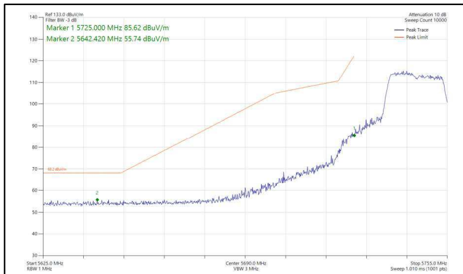
Figure 345 - 802.11n, HT20, TxBF, Core 0-1 - 5745 MHz, Band Edge Frequency 5725 MHz
