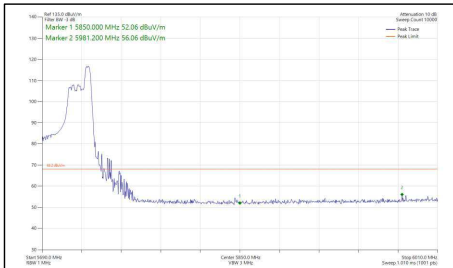
Figure 400 - 802.11ax, HE40, RU 52-44, CDD, Core 0-1 - 5710 MHz, Band Edge Frequency 5850 MHz
