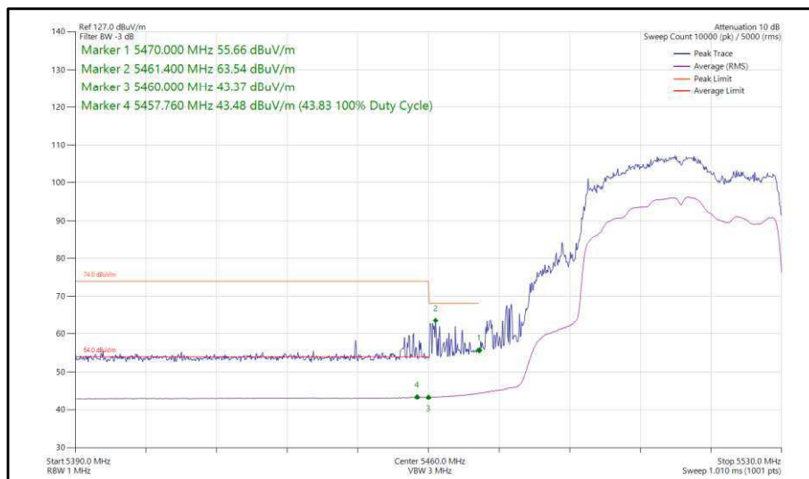
Figure 422 - 802.11ax, HE40, SU, TxBF, Core 0-1 - 5510 MHz, Band Edge Frequency 5470 MHz
