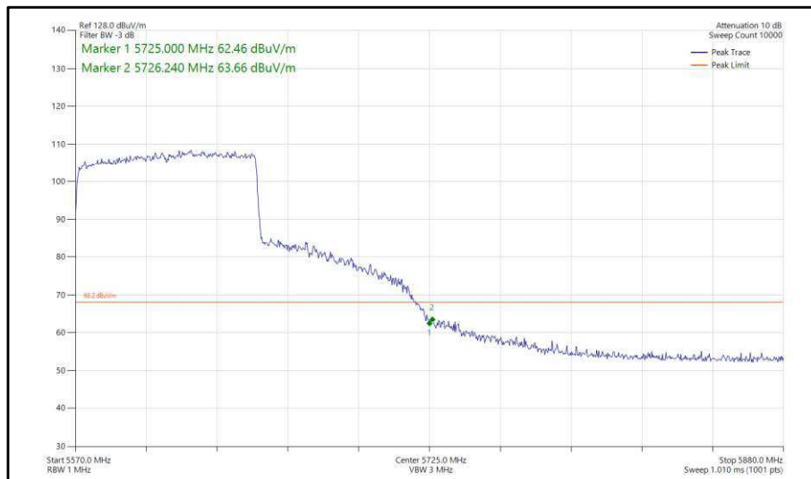
Figure 439 - 802.11ax, HE80, SU, SISO, Core 0 - 5610 MHz, Band Edge Frequency 5725 MHz
