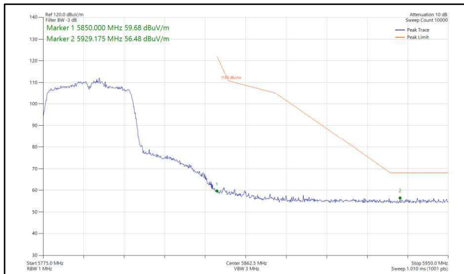
Figure 416 - 802.11n, HT40, SDM, Core 0-1 - 5795 MHz, Band Edge Frequency 5850 MHz
