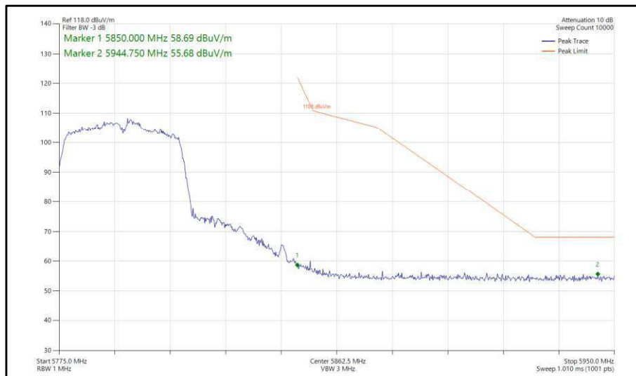
Figure 362 - 802.11n, HT40, SISO, Core 0 - 5795 MHz, Band Edge Frequency 5850 MHz
