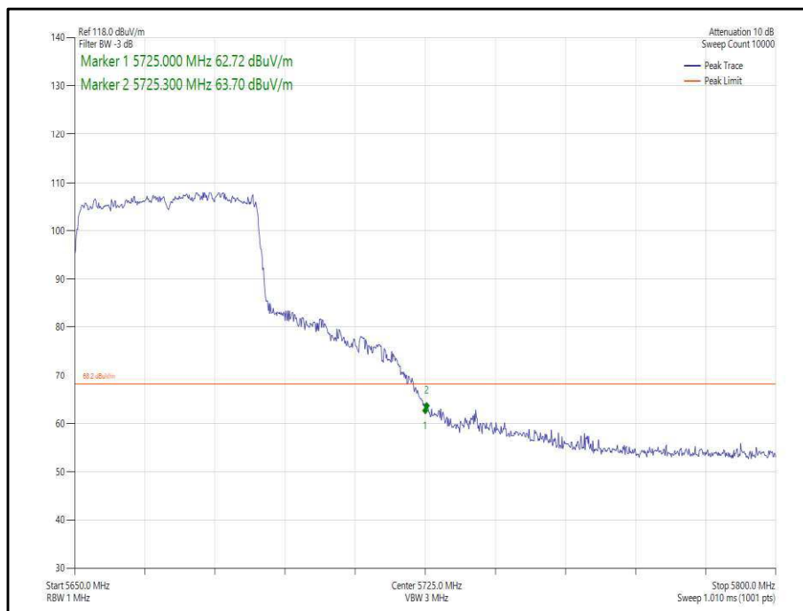
Figure 413 - 802.11ax, HE40, SU, SDM, Core 0-1 - 5670 MHz, Band Edge Frequency 5725 MHz
