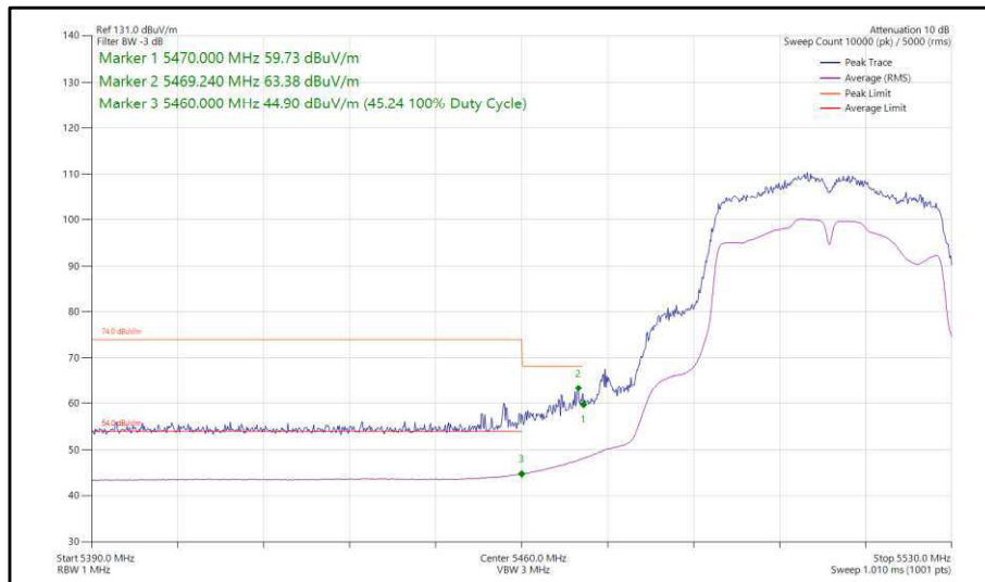
Figure 421 - 802.11n, HT40, TxBF, Core 0-1 - 5510 MHz, Band Edge Frequency 5470 MHz
