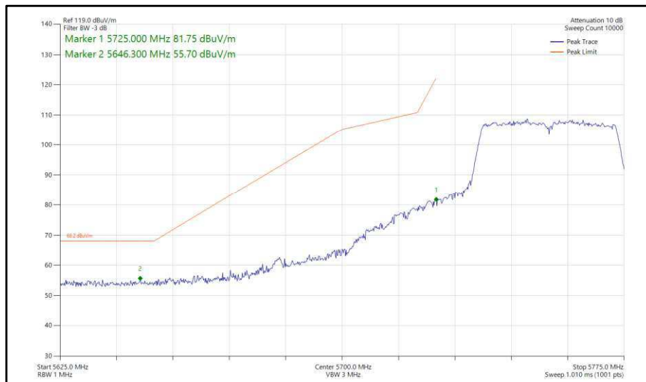
Figure 406 - 802.11n, HT40, SDM, Core 0-1 - 5755 MHz, Band Edge Frequency 5725 MHz
