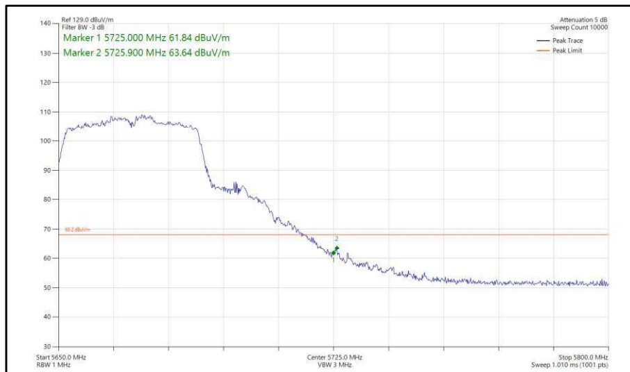
Figure 392 - 802.11n, HT40, CDD, Core 0-1 - 5670 MHz, Band Edge Frequency 5725 MHz
