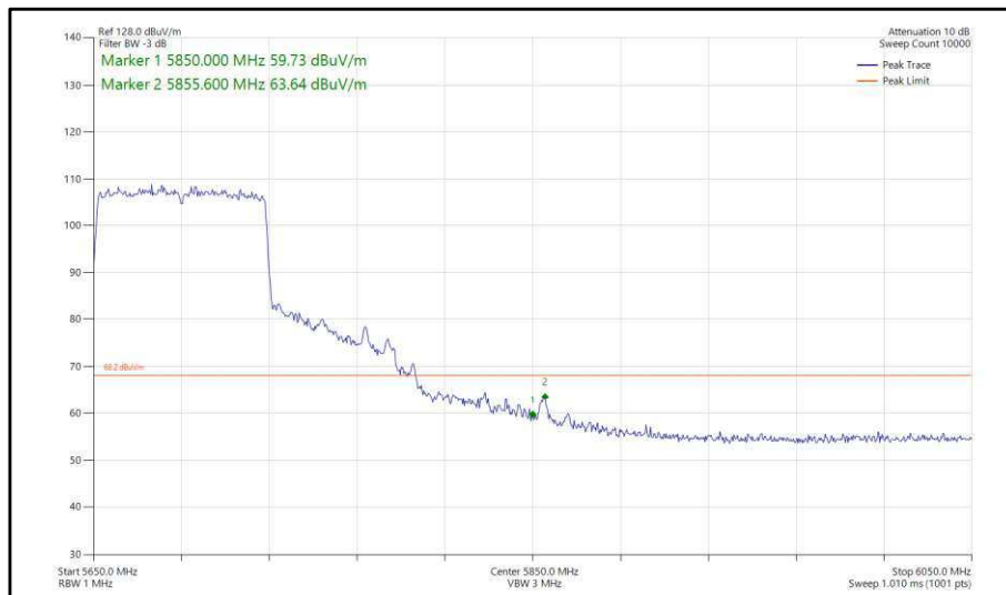
Figure 456 - 802.11ac, VHT80, SISO, Core 1 - 5690 MHz, Band Edge Frequency 5850 MHz
