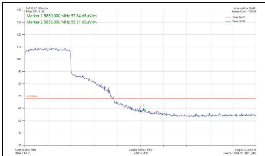
Figure 443 - 802.11ax, HE80, SU, SISO, Core 0 - 5690 MHz, Band Edge Frequency 5850 MHz
