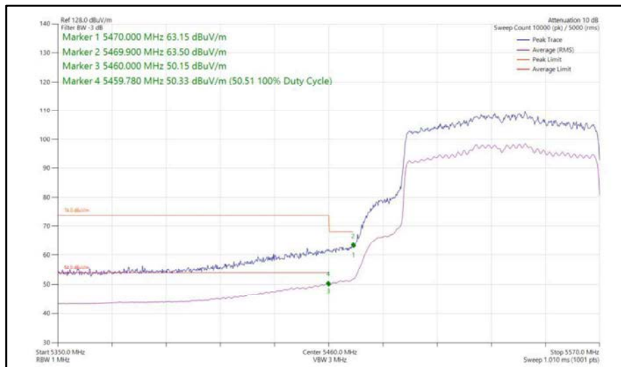
Figure 463 - 802.11ax, HE80, SU, CDD, Core 0-1 - 5530 MHz, Band Edge Frequency 5470 MHz
