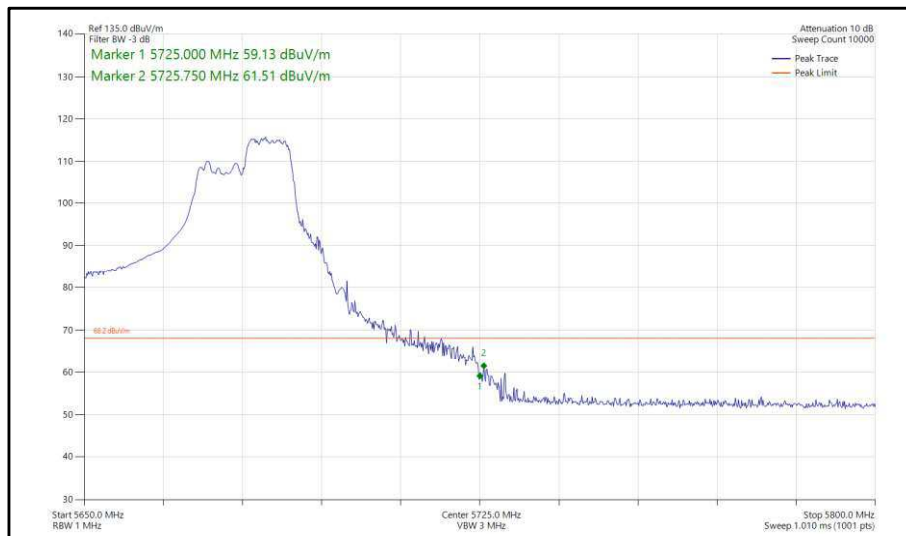
Figure 414 - 802.11ax, HE40, RU 106-56, SDM, Core 0-1 - 5670 MHz, Band Edge Frequency 5725 MHz
