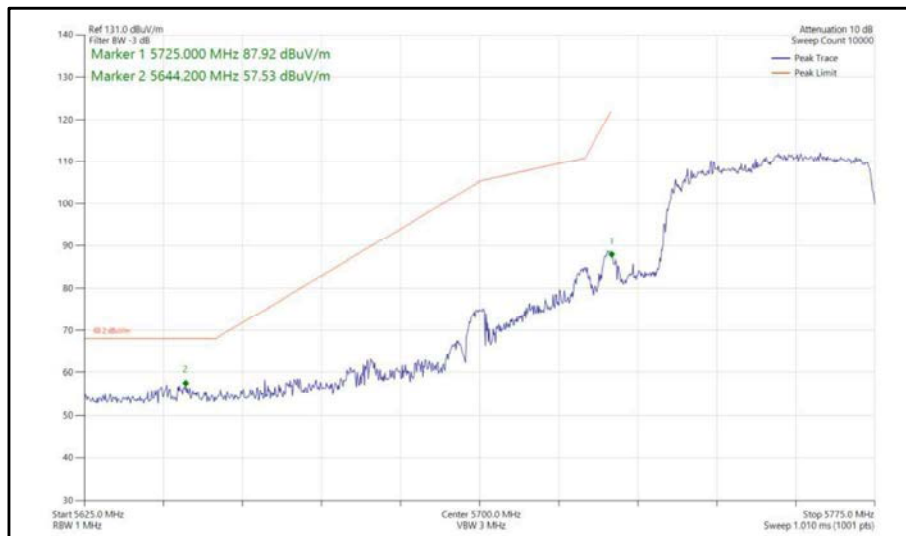
Figure 424 - 802.11ax, HE40, SU, TxBF, Core 0-1 - 5755 MHz, Band Edge Frequency 5725 MHz
