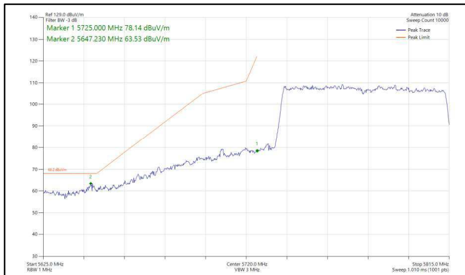
Figure 480 - 802.11ac, VHT80, SDM, Core 0-1 - 5775 MHz, Band Edge Frequency 5725 MHz
