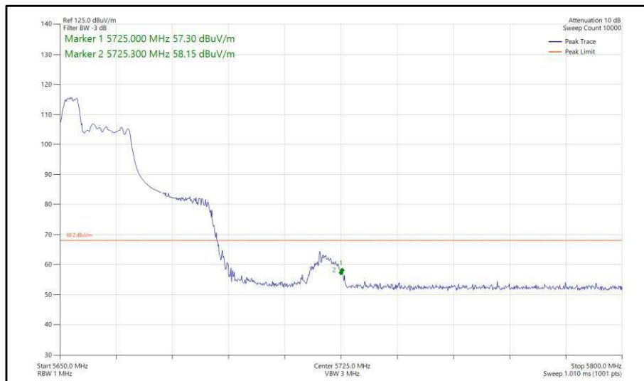
Figure 378 - 802.11ax, HE40, RU 52-37, SISO, Core 1 - 5670 MHz, Band Edge Frequency 5725 MHz
