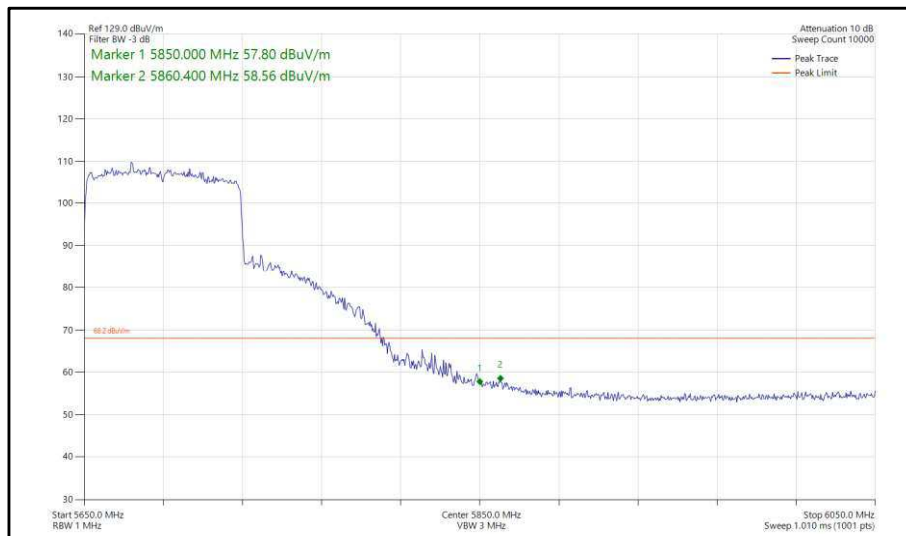
Figure 488 - 802.11ax, HE80, SU, SDM, Core 0-1 - 5690 MHz, Band Edge Frequency 5850 MHz
