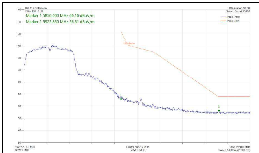
Figure 380 - 802.11n, HT40, SISO, Core 1 - 5795 MHz, Band Edge Frequency 5850 MHz
