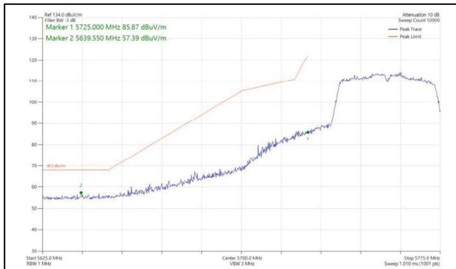
Figure 423 - 802.11n, HT40, TxBF, Core 0-1 - 5755 MHz, Band Edge Frequency 5725 MHz
