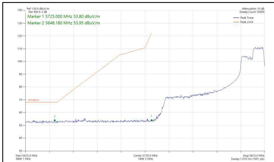
Figure 437 - 802.11ax, HE80, RU 106-60, SISO, Core 0 - 5775 MHz, Band Edge Frequency 5725 MHz
