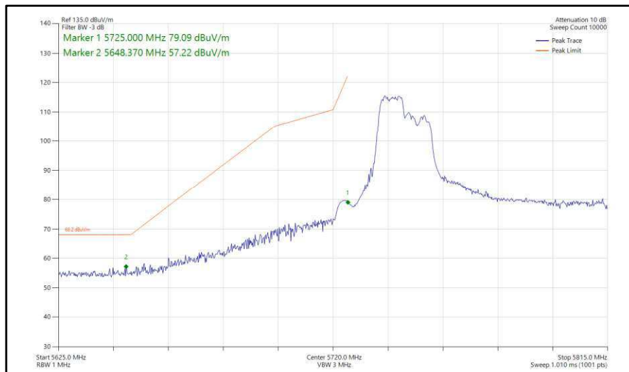
Figure 482 - 802.11ax, HE80, RU 106-53, SDM, Core 0-1 - 5775 MHz, Band Edge Frequency 5725 MHz
