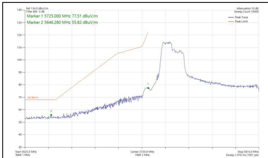
Figure 467 - 802.11ax, HE80, RU 106-53, CDD, Core 0-1 - 5775 MHz, Band Edge Frequency 5725 MHz
