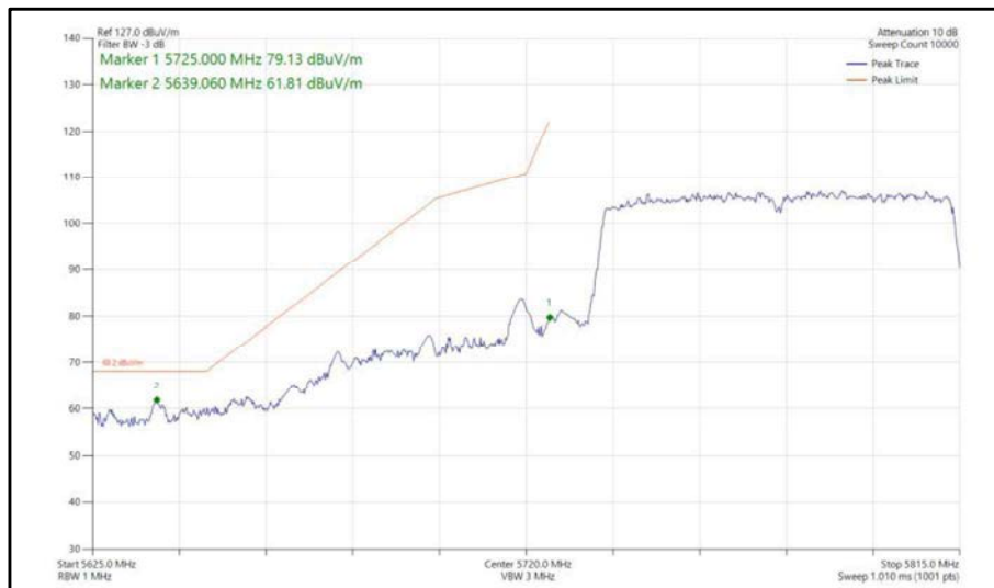
Figure 465 - 802.11ac, VHT80, CDD, Core 0-1 - 5775 MHz, Band Edge Frequency 5725 MHz
