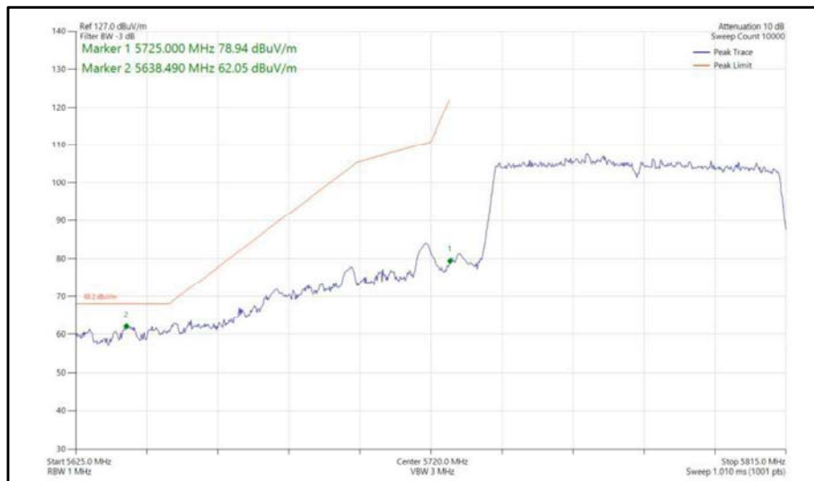
Figure 435 - 802.11ac, VHT80, SISO, Core 0 - 5775 MHz, Band Edge Frequency 5725 MHz
