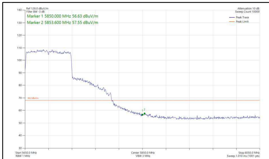
Figure 441 - 802.11ac, VHT80, SISO, Core 0 - 5690 MHz, Band Edge Frequency 5850 MHz
