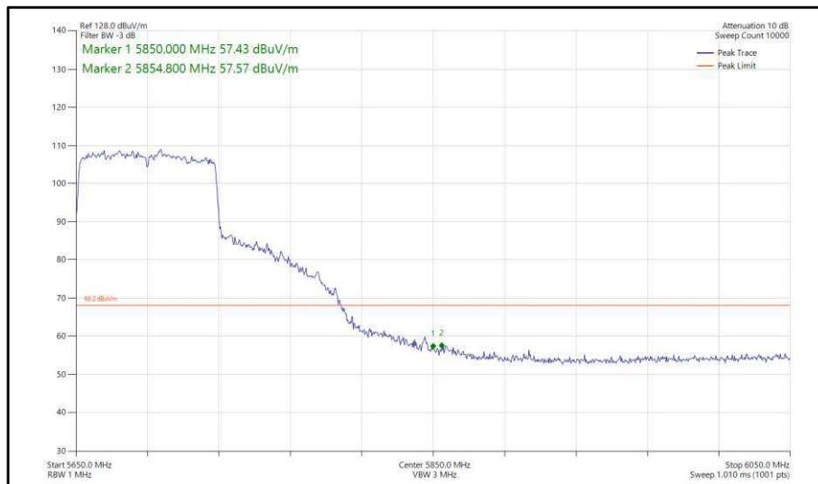
Figure 486 - 802.11ac, VHT80, SDM, Core 0-1 - 5690 MHz, Band Edge Frequency 5850 MHz
