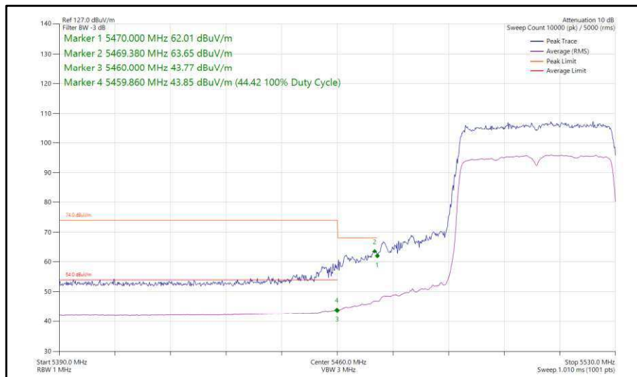
Figure 368 - 802.11ax, HE40, SU, SISO, Core 1 - 5510 MHz, Band Edge Frequency 5470 MHz
