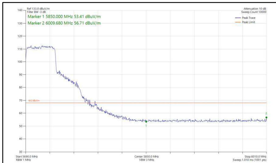
Figure 430 - 802.11ax, HE40, SU, TxBF, Core 0-1 - 5710 MHz, Band Edge Frequency 5850 MHz
