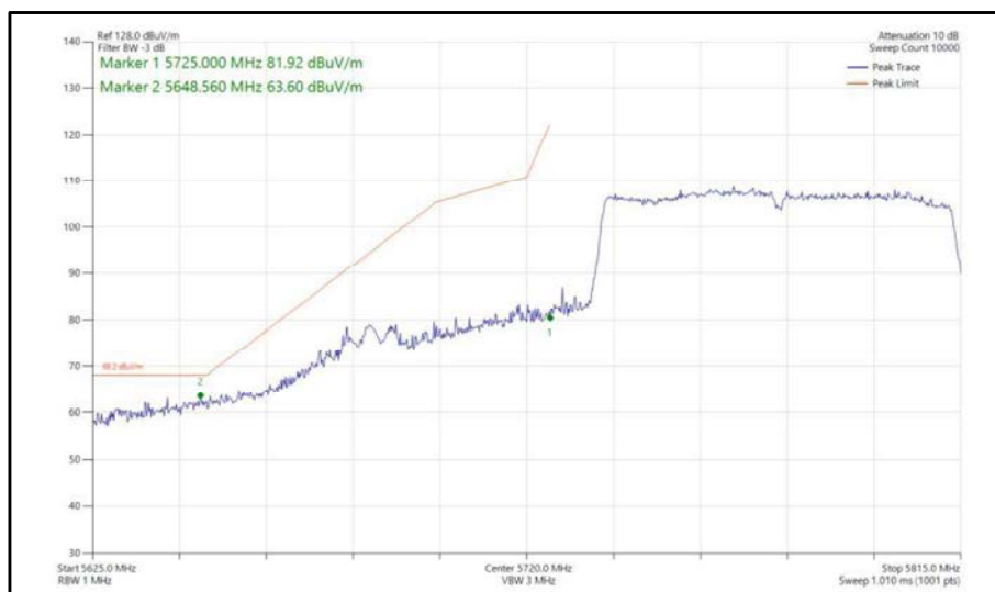
Figure 493 - 802.11ac, VHT80, TxBF, Core 0-1 - 5775 MHz, Band Edge Frequency 5725 MHz
