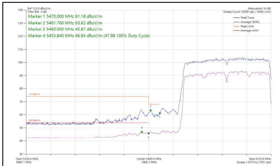
Figure 462 - 802.11ac, VHT80, CDD, Core 0-1 - 5530 MHz, Band Edge Frequency 5470 MHz
