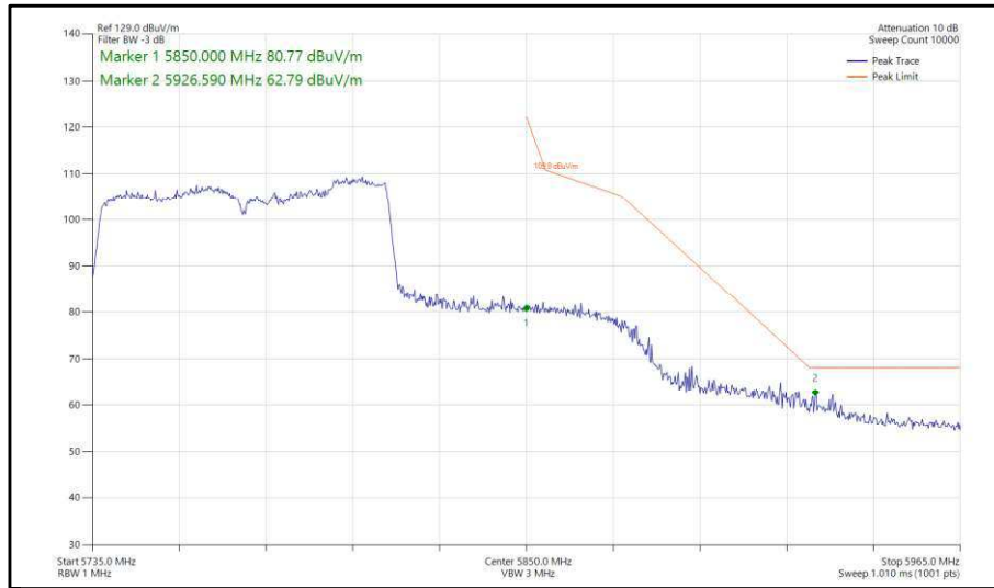
Figure 496 - 802.11ac, VHT80, TxBF, Core 0-1 - 5775 MHz, Band Edge Frequency 5850 MHz
