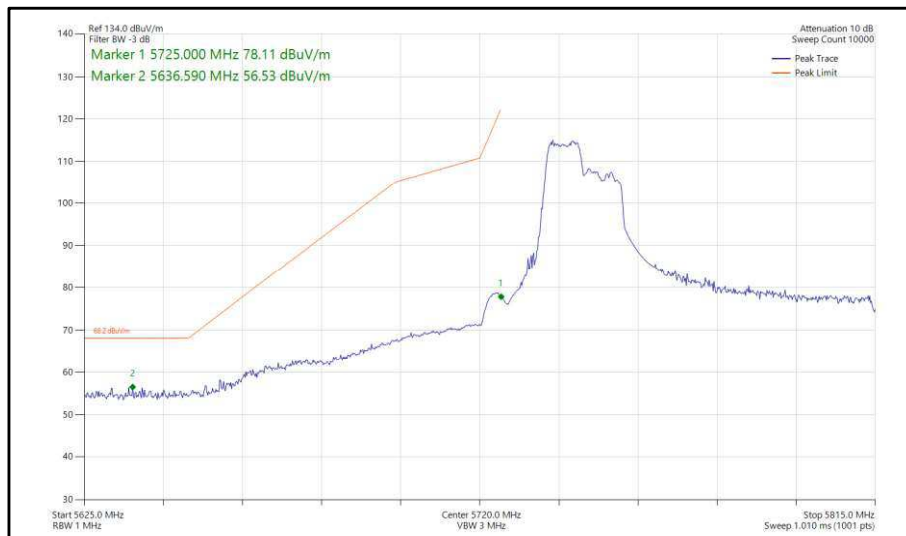
Figure 452 - 802.11ax, HE80, RU 106-53, SISO, Core 1 - 5775 MHz, Band Edge Frequency 5725 MHz
