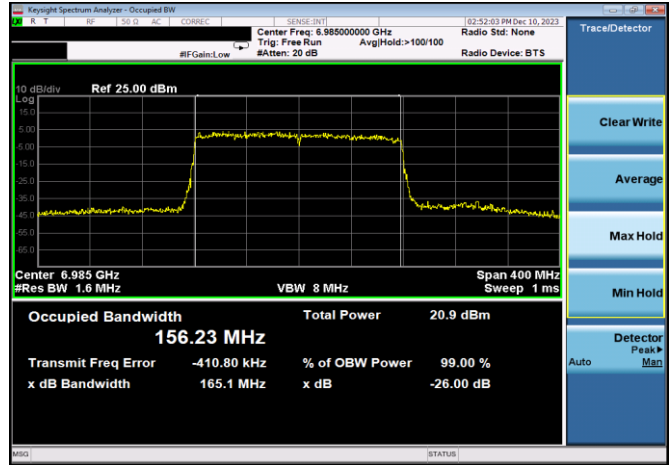
Plot 7-100. 26dB & 99% Bandwidth Plot Antenna 3b (160MHz) 802.11ax (UNII Band 8) – Ch. 207, MCS4)
