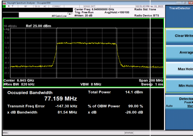
Plot 7-99. 26dB & 99% Bandwidth Plot Antenna 3b (80MHz) 802.11ax (UNII Band 8) – Ch. 199, MCS4)
