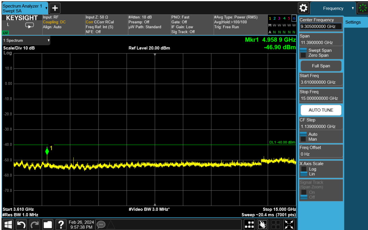
Plot 7-92. Simultaneous Tx Conducted Spurious Plot (FR1-n48 + BT)
