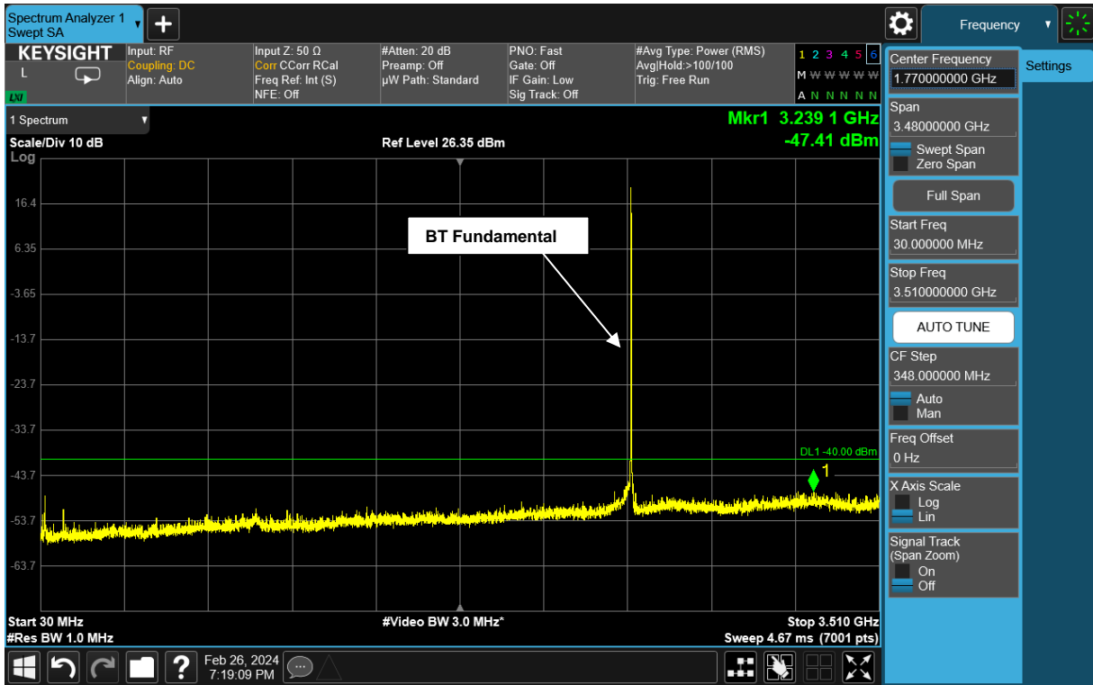
Plot 7-91. Simultaneous Tx Conducted Spurious Plot (FR1-n48 + BT)
