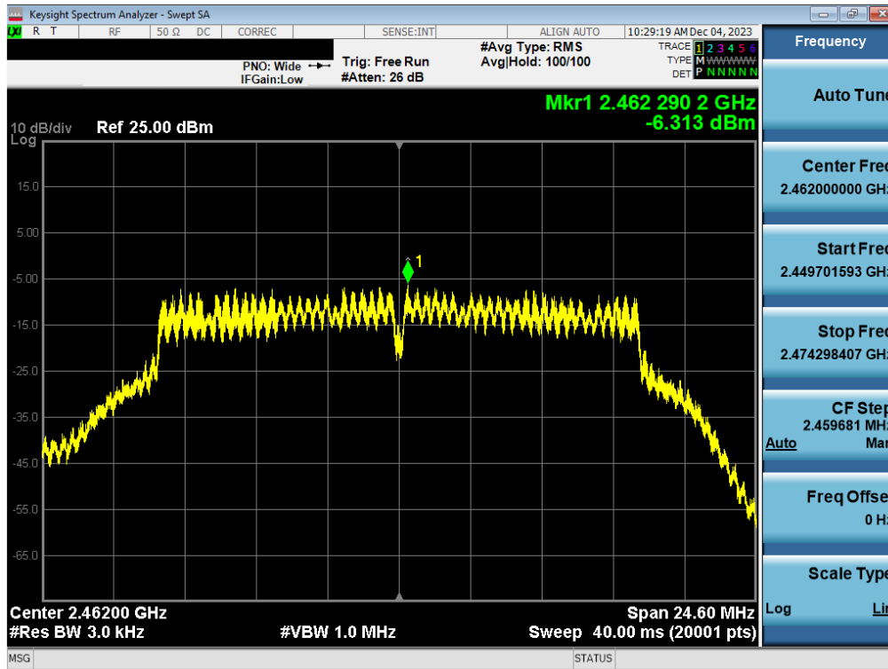
Plot 7-93. Power Spectral Density Plot Antenna 1a (802.11g – Ch. 11) – 6Mbps
