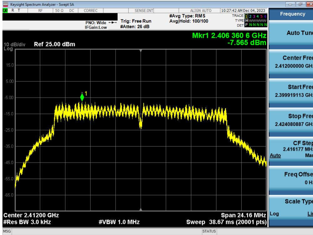
Plot 7-91. Power Spectral Density Plot Antenna 1a (802.11g – Ch. 1) – 6Mbps
