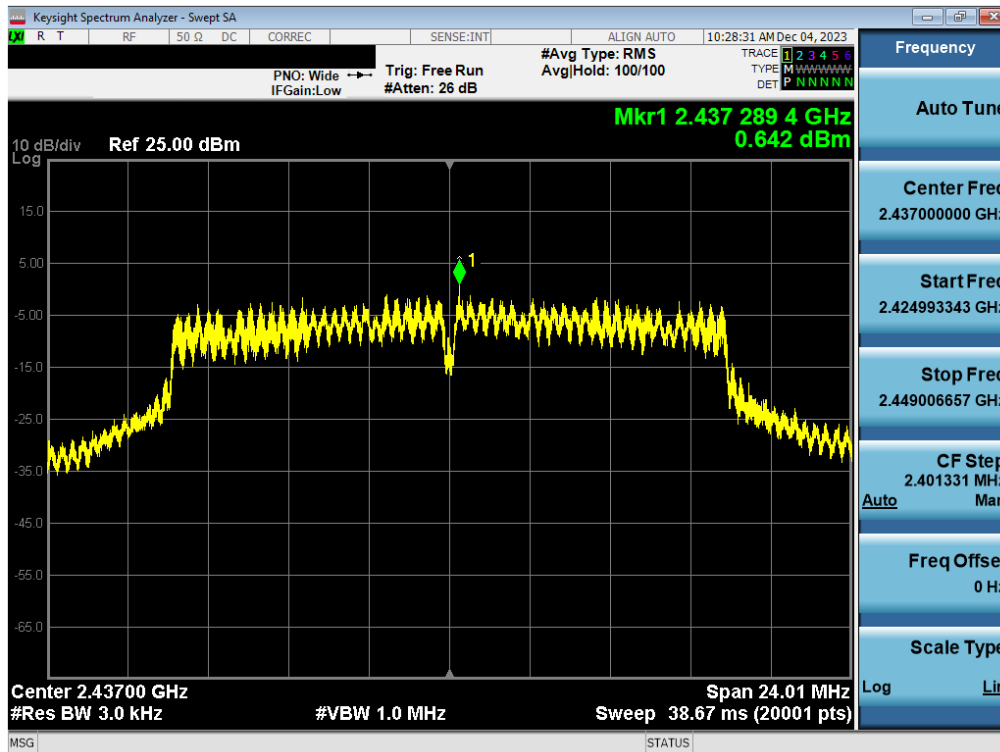
Plot 7-92. Power Spectral Density Plot Antenna 1a (802.11g – Ch. 6) – 6Mbps
