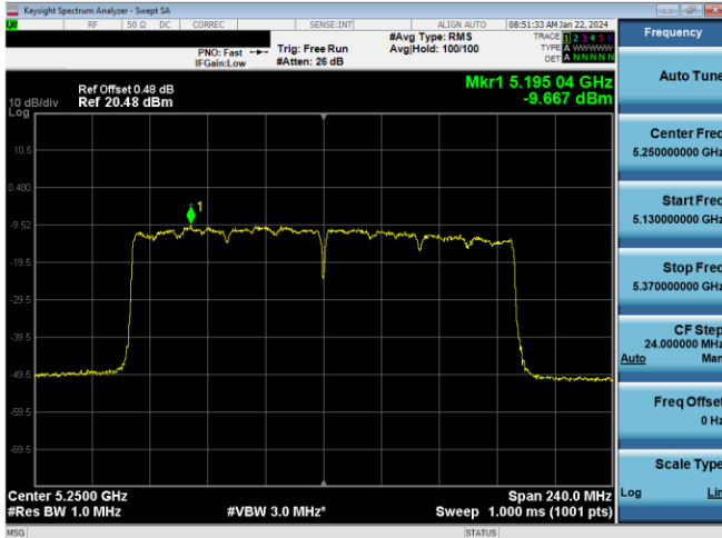
Plot 7-412. PSD CDD Primary Antenna 5T (160MHz BW 11ax - RU996x2 - Ch.50)
