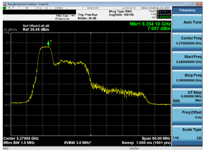
Plot 7-423. PSD CDD Primary Antenna 3b (40MHz BW 11ax Index 37 - RU52 - Ch.54)
