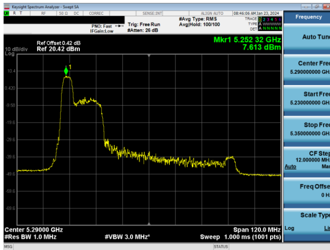
Plot 7-431. PSD CDD Primary Antenna 3b (80MHz BW 11ax Index 37 - RU52 - Ch.58)
