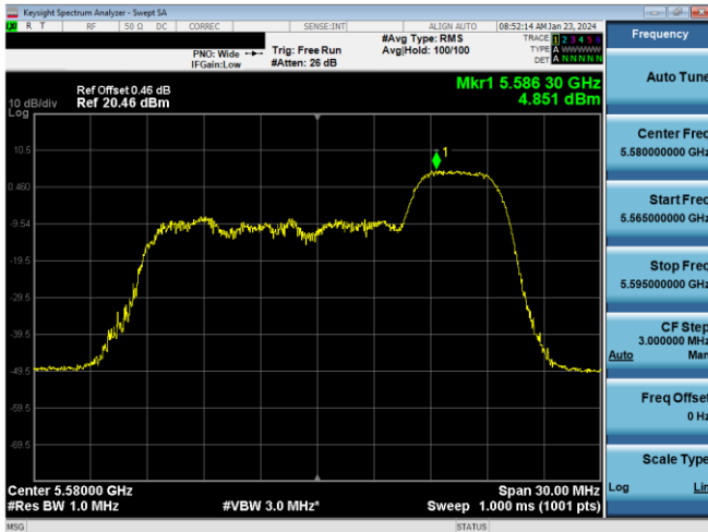
Plot 7-443. PSD CDD Primary Antenna 3b (20MHz BW 11ax Index 40 - RU52 - Ch.116)
