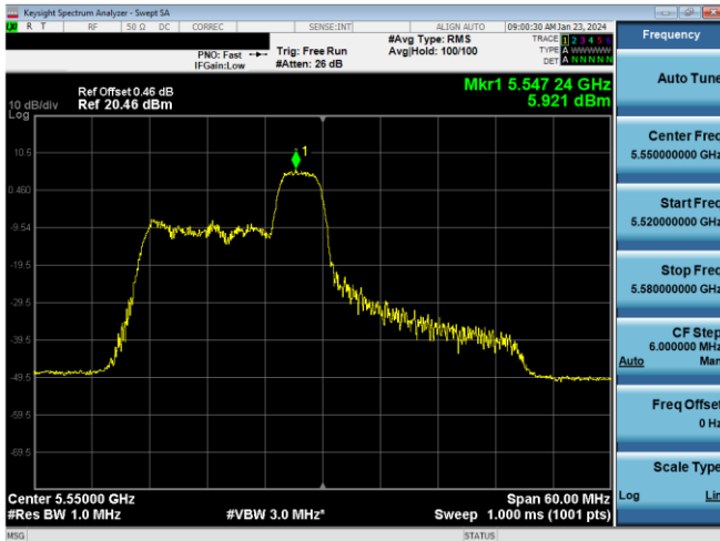
Plot 7-449. PSD CDD Primary Antenna 3b (40MHz BW 11ax Index 40 - RU52 - Ch.110)
