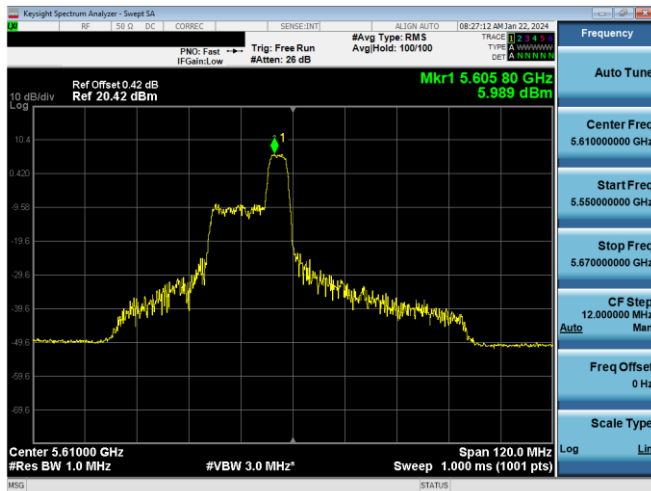
Plot 7-456. PSD CDD Primary Antenna 5T (80MHz BW 11ax Index 44 - RU52 - Ch.122)
