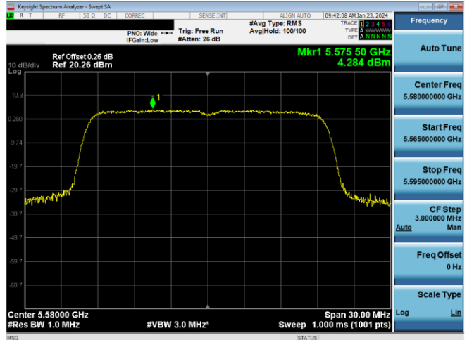
Plot 7-445. PSD CDD Primary Antenna 3b (20MHz BW 11ax- RU242 - Ch.116)
