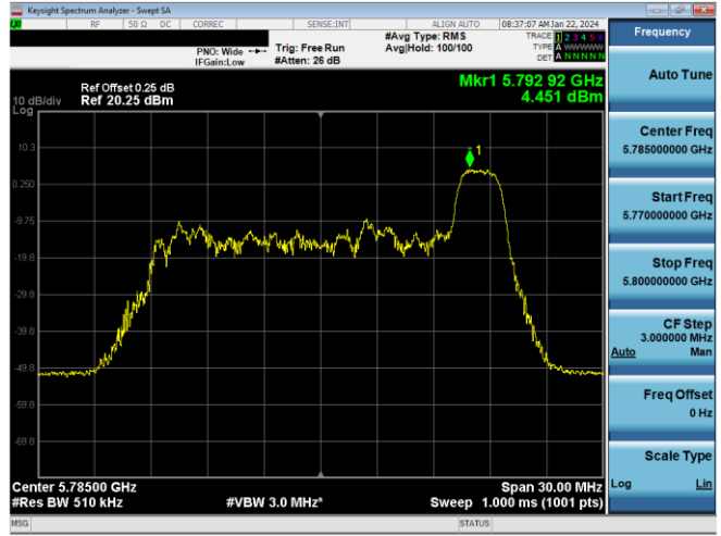
Plot 7-474. PSD CDD Primary Antenna 5T (20MHz BW 11ax Index 8 – RU26 – Ch.157)
