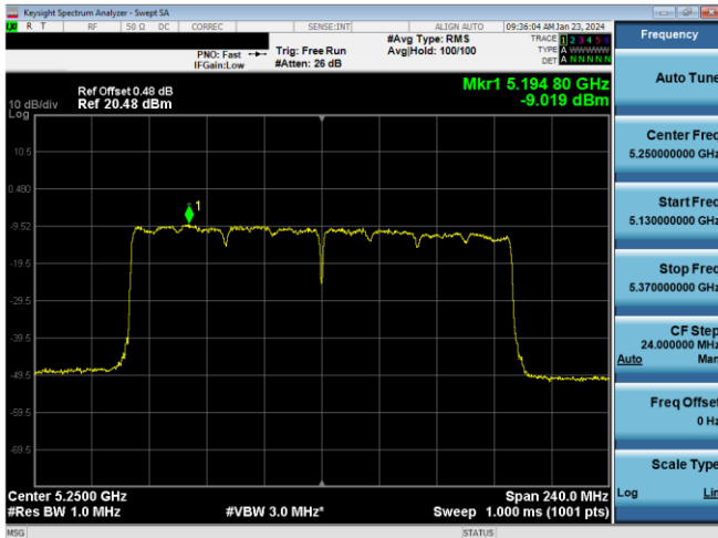
Plot 7-413. PSD CDD Primary Antenna 3b (160MHz BW 11ax - RU996x2 - Ch.50)
