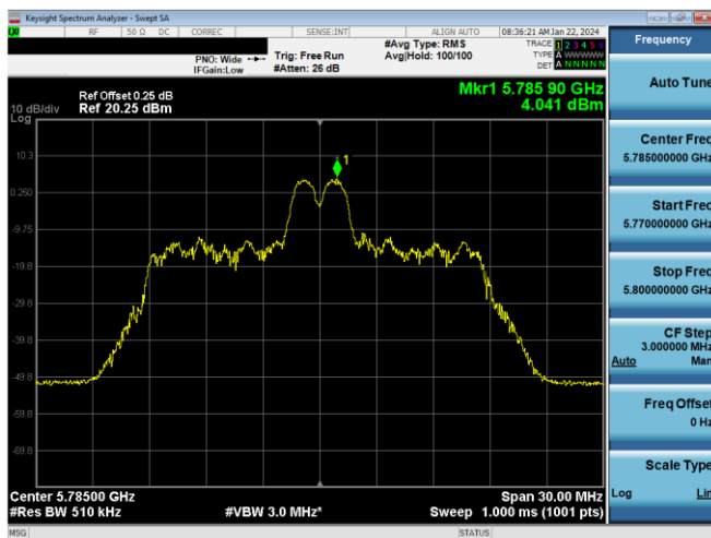
Plot 7-472. PSD CDD Primary Antenna 5T (20MHz BW 11ax Index 4 – RU26 – Ch.157)
