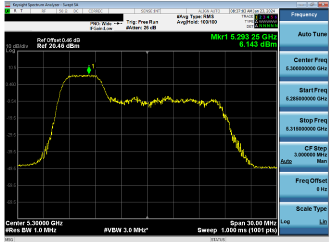
Plot 7-415. PSD CDD Primary Antenna 3b (20MHz BW 11ax Index 37 - RU52 - Ch.60)
