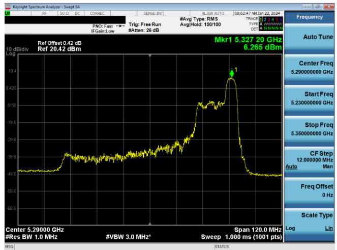
Plot 7-434. PSD CDD Primary Antenna 5T (80MHz BW 11ax Index 52 - RU52 - Ch.58)
