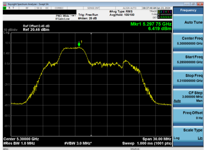
Plot 7-417. PSD CDD Primary Antenna 3b (20MHz BW 11ax Index 38 - RU52 - Ch.60)
