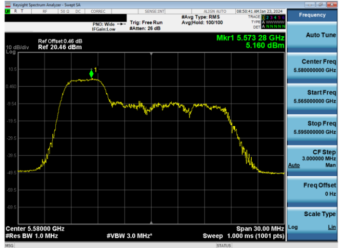
Plot 7-439. PSD CDD Primary Antenna 3b (20MHz BW 11ax Index 37 - RU52 - Ch.116)
