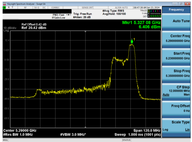
Plot 7-435. PSD CDD Primary Antenna 3b (80MHz BW 11ax Index 52 - RU52 - Ch.58)
