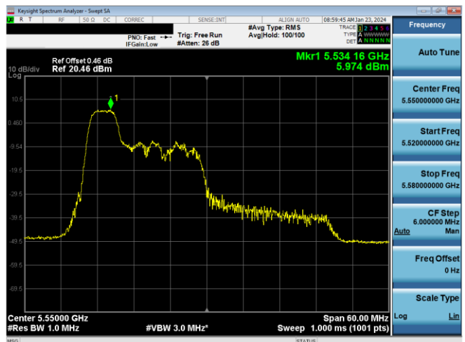
Plot 7-447. PSD CDD Primary Antenna 3b (40MHz BW 11ax Index 37 - RU52 - Ch.110)
