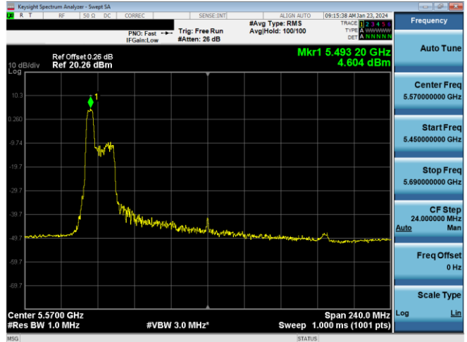
Plot 7-463. PSD CDD Primary Antenna 3b (160MHz BW 11ax Index 37 - RU52 - Ch.14 (L))
