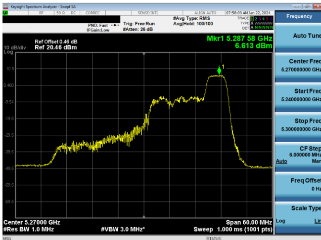
Plot 7-426. PSD CDD Primary Antenna 5T (40MHz BW 11ax Index 44 - RU52 - Ch.54)
