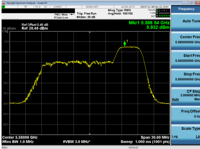
Plot 7-442. PSD CDD Primary Antenna 5T (20MHz BW 11ax Index 40 - RU52 - Ch.116)
