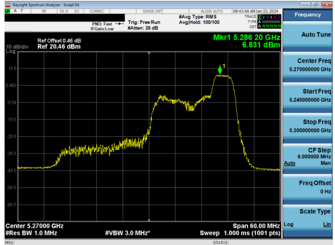
Plot 7-427. PSD CDD Primary Antenna 3b (40MHz BW 11ax Index 44 - RU52 - Ch.54)
