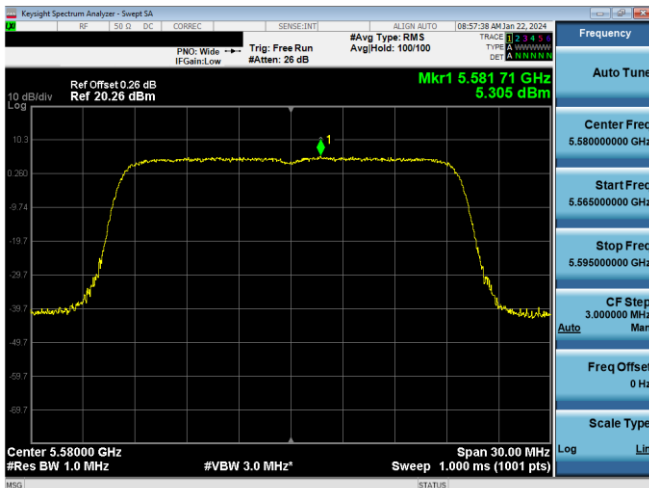
Plot 7-444. PSD CDD Primary Antenna 5T (20MHz BW 11ax- RU242 - Ch.116)
