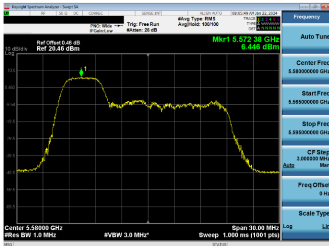
Plot 7-438. PSD CDD Primary Antenna 5T (20MHz BW 11ax Index 37 - RU52 - Ch.116)
