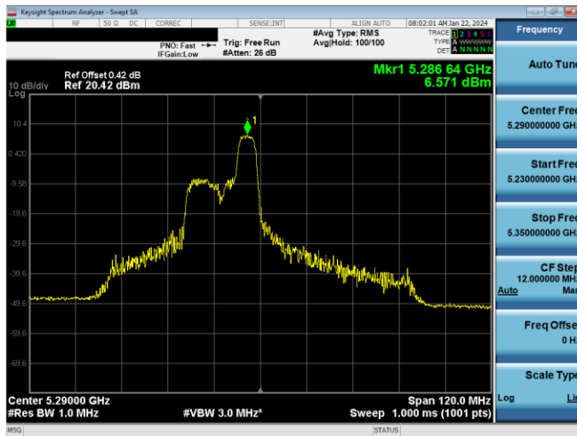
Plot 7-432. PSD CDD Primary Antenna 5T (80MHz BW 11ax Index 44 - RU52 - Ch.58)
