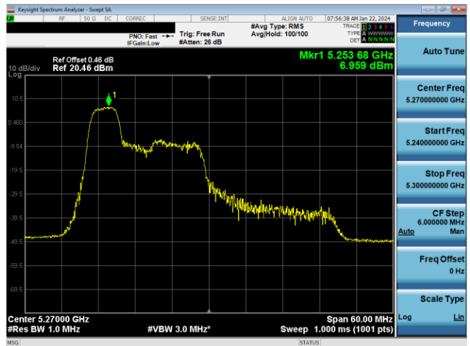
Plot 7-422. PSD CDD Primary Antenna 5T (40MHz BW 11ax Index 37 - RU52 - Ch.54)
