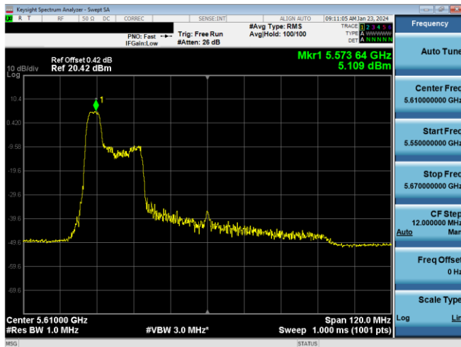
Plot 7-455. PSD CDD Primary Antenna 3b (80MHz BW 11ax Index 37 - RU52 - Ch.122)
