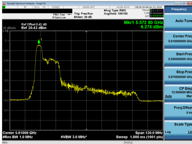
Plot 7-454. PSD CDD Primary Antenna 5T (80MHz BW 11ax Index 37 - RU52 - Ch.122)
