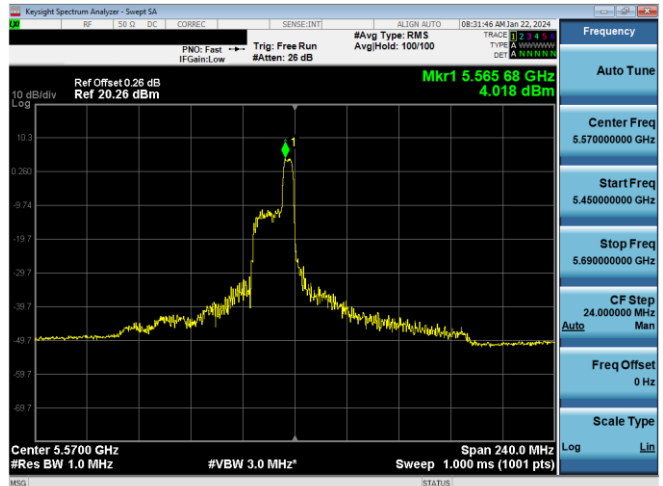
Plot 7-464. PSD CDD Primary Antenna 5T (160MHz BW 11ax Index 52 - RU52 - Ch.14 (L))
