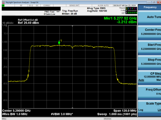
Plot 7-436. PSD CDD Primary Antenna 5T (80MHz BW 11ax - RU96 - Ch.58)
