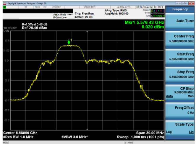
Plot 7-440. PSD CDD Primary Antenna 5T (20MHz BW 11ax Index 38 - RU52 - Ch.116)
