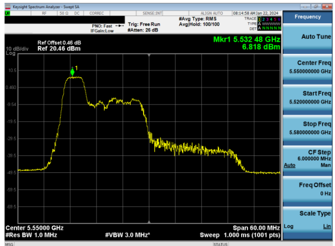
Plot 7-446. PSD CDD Primary Antenna 5T (40MHz BW 11ax Index 37 - RU52 - Ch.110)
