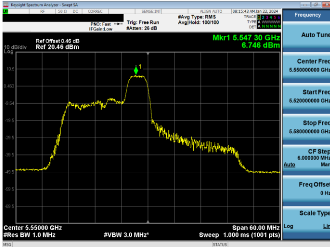
Plot 7-448. PSD CDD Primary Antenna 5T (40MHz BW 11ax Index 40 - RU52 - Ch.110)
