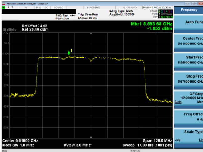
Plot 7-461. PSD CDD Primary Antenna 3b (80MHz BW 11ax - RU96 - Ch.122)
