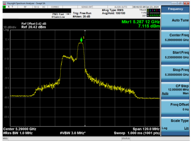
Plot 7-433. PSD CDD Primary Antenna 3b (80MHz BW 11ax Index 44 - RU52 - Ch.58)
