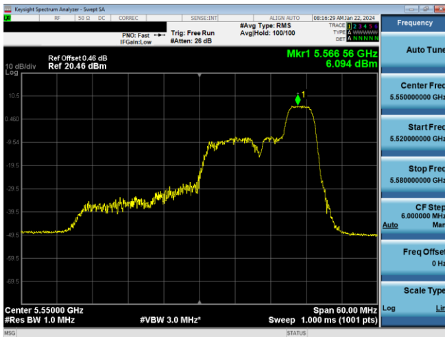
Plot 7-450. PSD CDD Primary Antenna 5T (40MHz BW 11ax Index 44 - RU52 - Ch.110)
