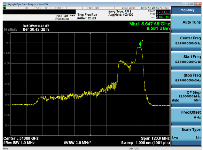
Plot 7-458. PSD CDD Primary Antenna 5T (80MHz BW 11ax Index 52 - RU52 - Ch.122)
