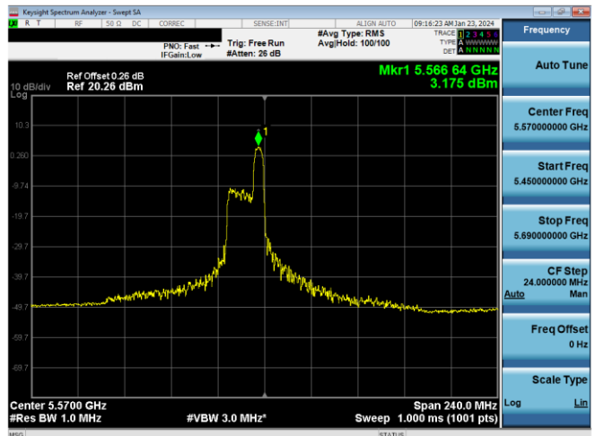
Plot 7-465. PSD CDD Primary Antenna 3b (160MHz BW 11ax Index 52 - RU52 - Ch.14 (L))
