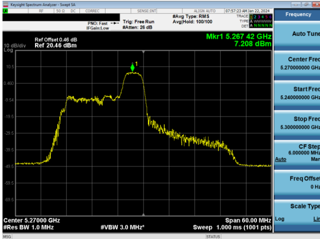
Plot 7-424. PSD CDD Primary Antenna 5T (40MHz BW 11ax Index 40 - RU52 - Ch.54)
