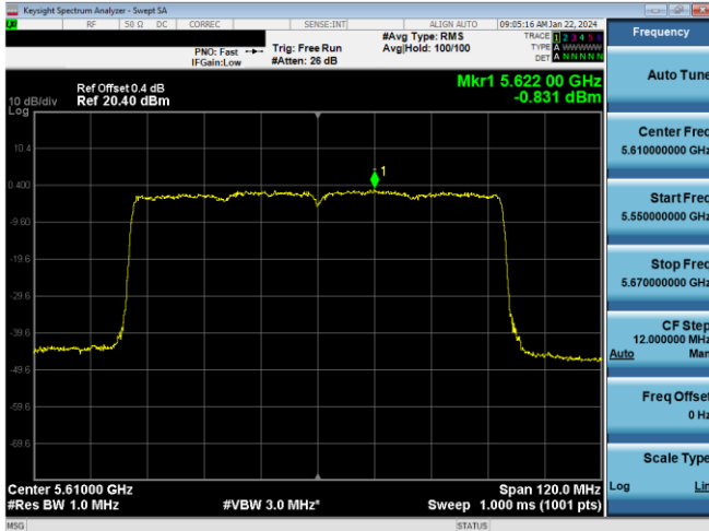
Plot 7-460. PSD CDD Primary Antenna 5T (80MHz BW 11ax - RU96 - Ch.122)
