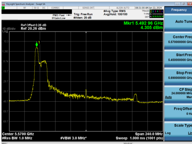
Plot 7-462. PSD CDD Primary Antenna 5T (160MHz BW 11ax Index 37 - RU52 - Ch.14 (L))
