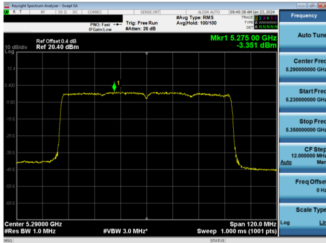
Plot 7-437. PSD CDD Primary Antenna 3b (80MHz BW 11ax - RU96 - Ch.58)
