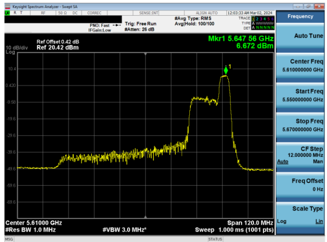
Plot 7-459. PSD CDD Primary Antenna 3b (80MHz BW 11ax Index 52 - RU52 - Ch.122)
