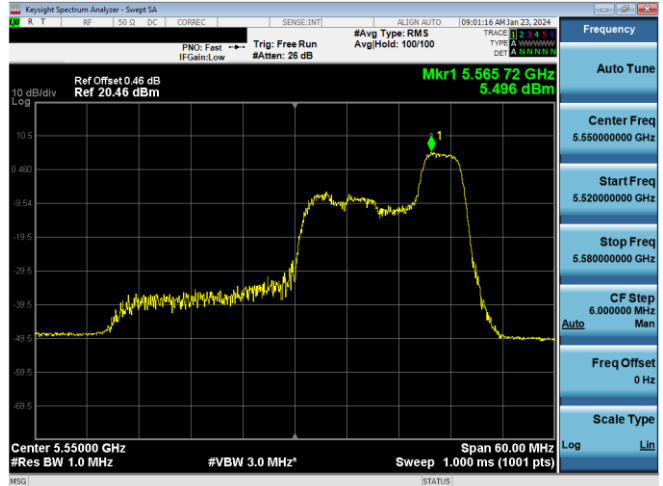
Plot 7-451. PSD CDD Primary Antenna 3b (40MHz BW 11ax Index 44 - RU52 - Ch.110)
