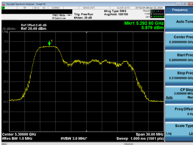
Plot 7-414. PSD CDD Primary Antenna 5T (20MHz BW 11ax Index 37 - RU52 - Ch.60)
