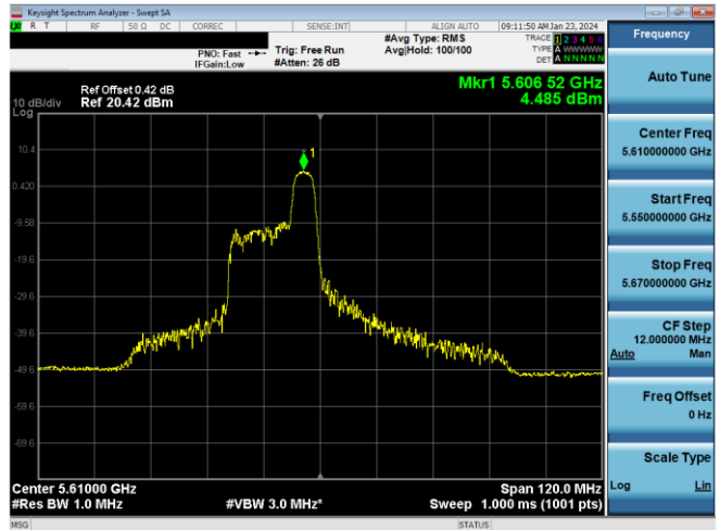
Plot 7-457. PSD CDD Primary Antenna 3b (80MHz BW 11ax Index 44 - RU52 - Ch.122)
