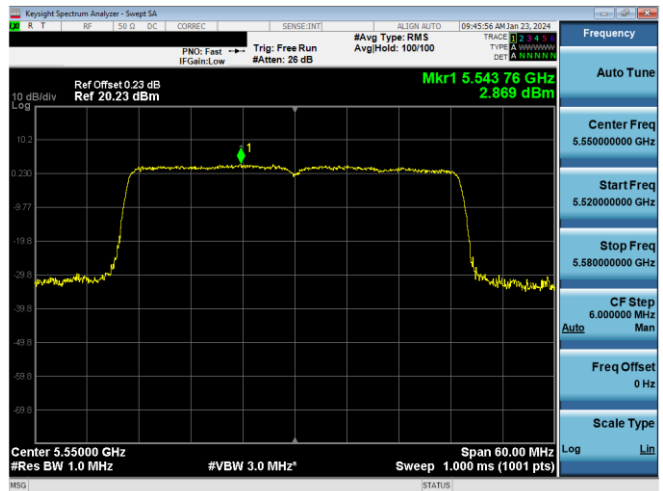
Plot 7-453. PSD CDD Primary Antenna 3b (40MHz BW 11ax - RU484 - Ch.110)
