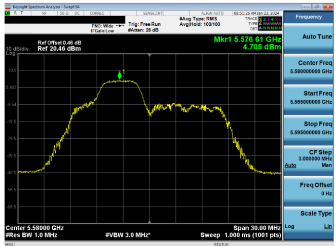
Plot 7-441. PSD CDD Primary Antenna 3b (20MHz BW 11ax Index 38 - RU52 - Ch.116)
