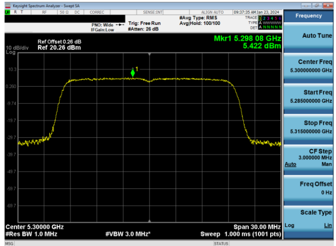
Plot 7-421. PSD CDD Primary Antenna 3b (20MHz BW 11ax- RU242 - Ch.60)
