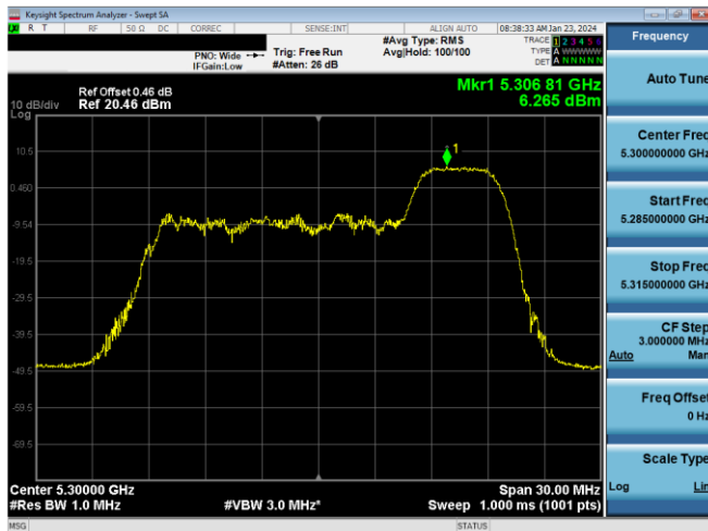
Plot 7-419. PSD CDD Primary Antenna 3b (20MHz BW 11ax Index 40 - RU52 - Ch.60)
