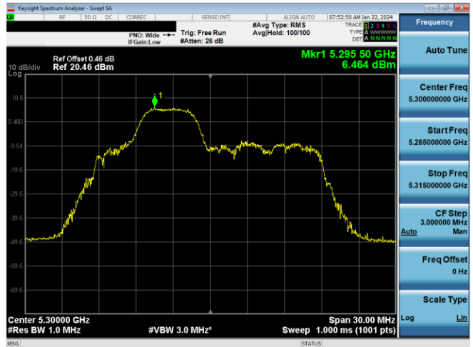
Plot 7-416. PSD CDD Primary Antenna 5T (20MHz BW 11ax Index 38 - RU52 - Ch.60)
