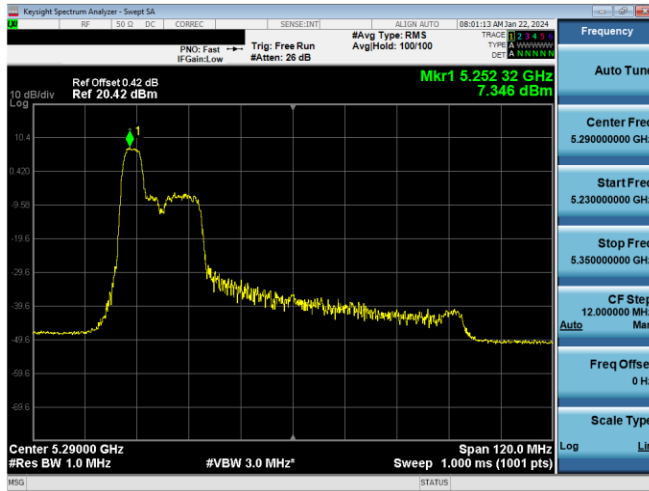
Plot 7-430. PSD CDD Primary Antenna 5T (80MHz BW 11ax Index 37 - RU52 - Ch.58)
