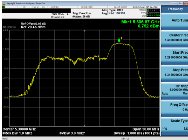
Plot 7-418. PSD CDD Primary Antenna 5T (20MHz BW 11ax Index 40 - RU52 - Ch.60)
