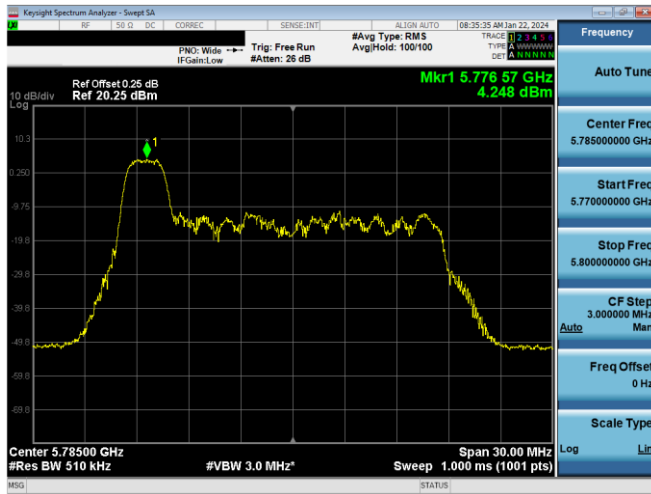
Plot 7-470. PSD CDD Primary Antenna 5T (20MHz BW 11ax Index 0 – RU26 – Ch.157)
