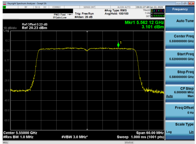
Plot 7-452. PSD CDD Primary Antenna 5T (40MHz BW 11ax - RU484 - Ch.110)
