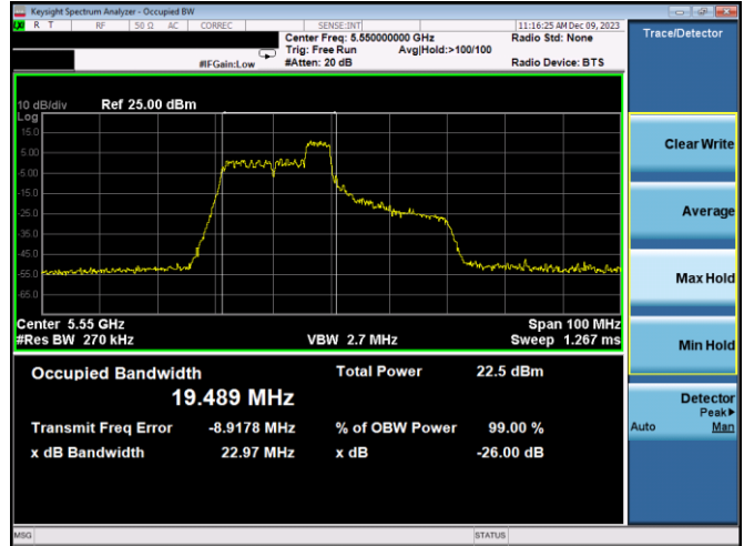
Plot 7-34. 26dB BW & 99% OBW Antenna 5T (40MHz BW 11ax Index 40 – RU52 – Ch.110)
