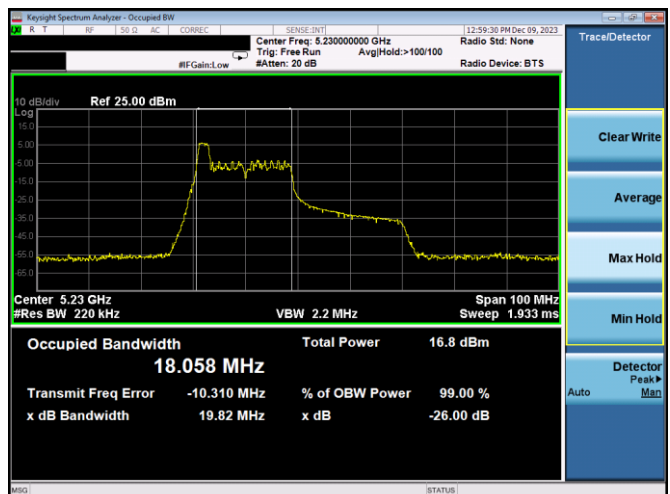
Plot 7-49. 26dB BW & 99% OBW Antenna 3b (40MHz BW 11ax Index 0 – RU26 – Ch.46)
