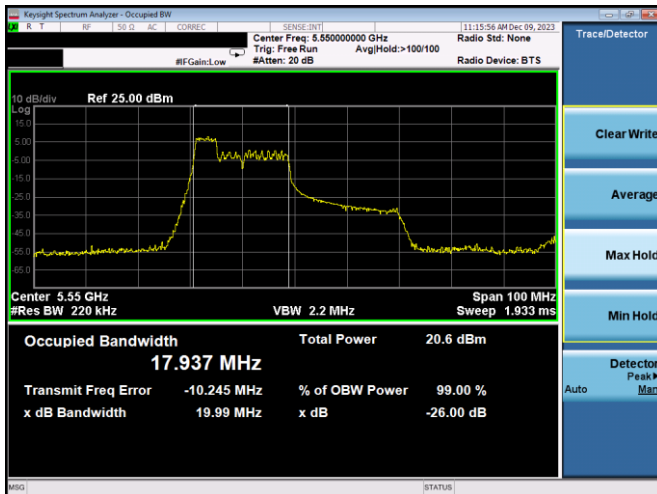
Plot 7-33. 26dB BW & 99% OBW Antenna 5T (40MHz BW 11ax Index 37 – RU52 – Ch.110)
