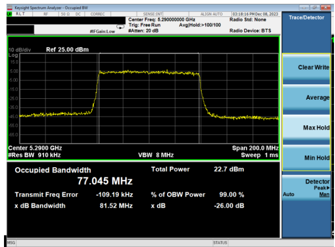
Plot 7-28. 26dB BW & 99% OBW Antenna 5T (80MHz BW 11ax – RU96 – Ch.58)
