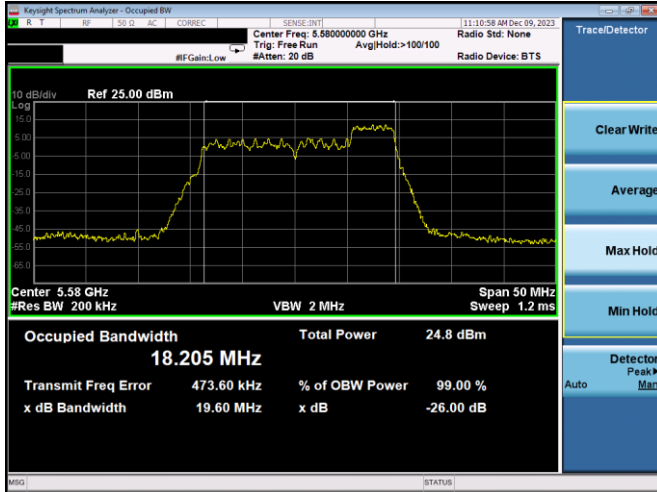
Plot 7-31. 26dB BW & 99% OBW Antenna 5T (20MHz BW 11ax Index 40 – RU52 – Ch.116)
