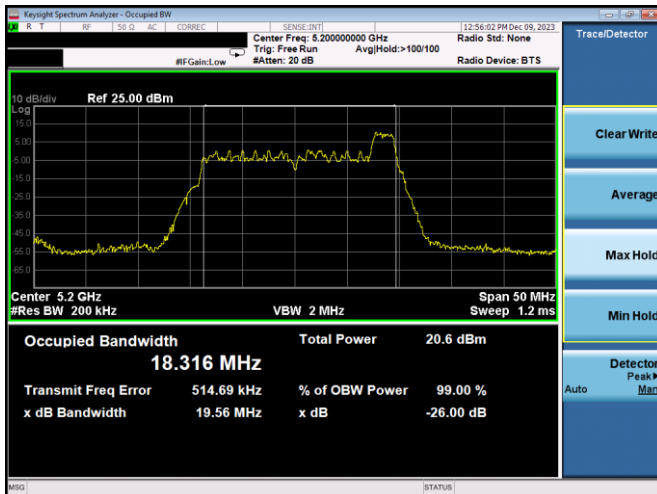
Plot 7-47. 26dB BW & 99% OBW Antenna 3b (20MHz BW 11ax Index 8 – RU26 – Ch.40)
