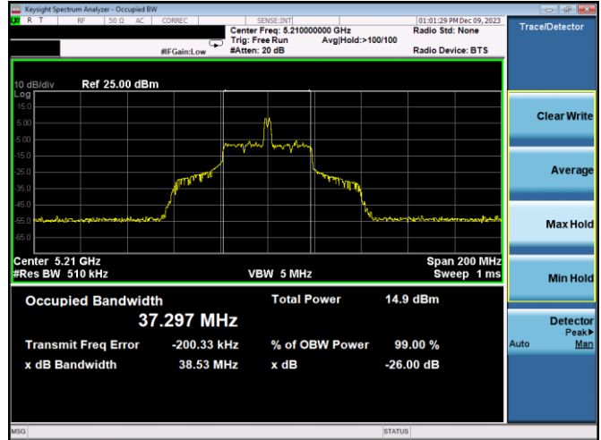
Plot 7-54. 26dB BW & 99% OBW Antenna 3b (80MHz BW 11ax Index 18 - RU26 - Ch.42)
