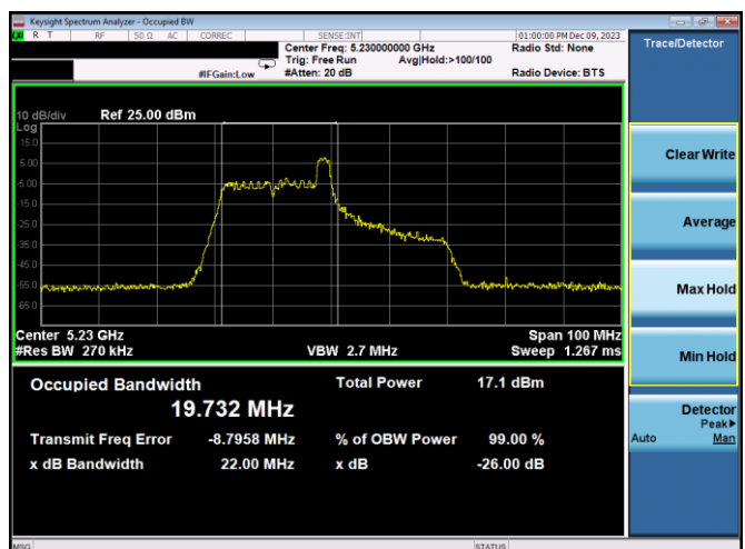
Plot 7-50. 26dB BW & 99% OBW Antenna 3b (40MHz BW 11ax Index 8 – RU26 – Ch.46)
