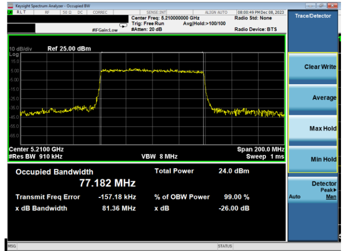
Plot 7-56. 26dB BW & 99% OBW Antenna 3b (80MHz BW 11ax - RU996 - Ch.42)
