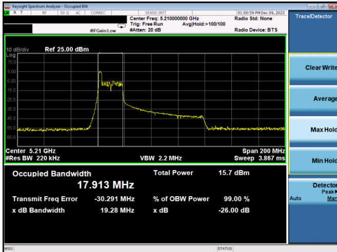
Plot 7-53. 26dB BW & 99% OBW Antenna 3b (80MHz BW 11ax Index 0 - RU26 - Ch.42)
