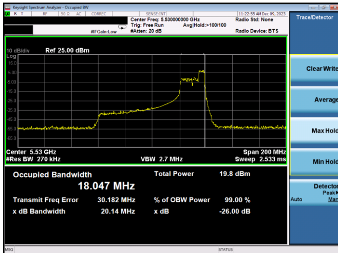
Plot 7-39. 26dB BW & 99% OBW Antenna 5T (80MHz BW 11ax Index 52 – RU52 – Ch.106)
