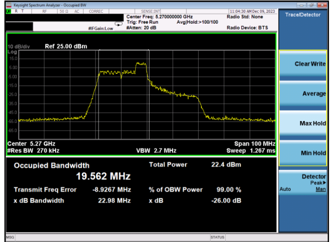
Plot 7-22. 26dB BW & 99% OBW Antenna 5T (40MHz BW 11ax Index 40 – RU52 – Ch.54)
