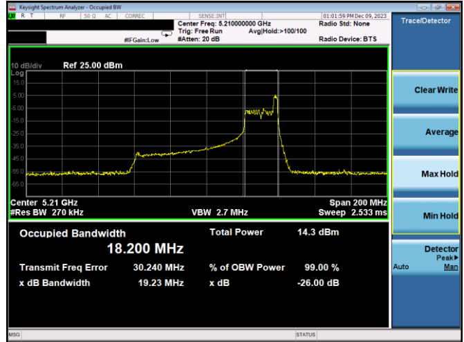
Plot 7-55. 26dB BW & 99% OBW Antenna 3b (80MHz BW 11ax Index 36 - RU26 - Ch.42)
