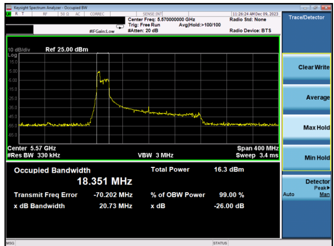
Plot 7-41. 26dB BW & 99% OBW Antenna 5T (160MHz BW 11ax Index 37 – RU52 – Ch.114 (L))
