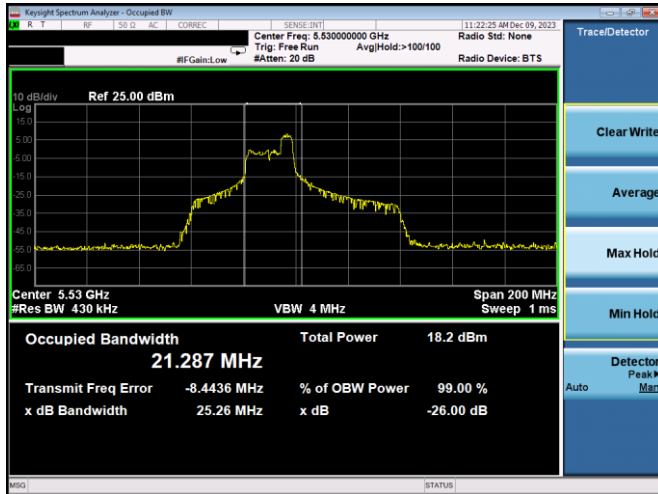
Plot 7-38. 26dB BW & 99% OBW Antenna 5T (80MHz BW 11ax Index 44 – RU52 – Ch.106)
