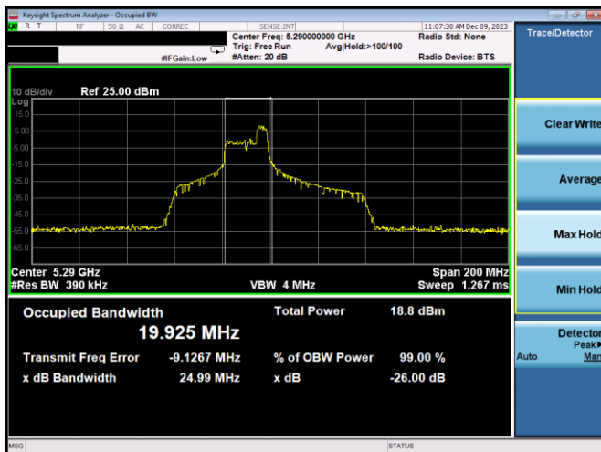
Plot 7-26. 26dB BW & 99% OBW Antenna 5T (80MHz BW 11ax Index 44 – RU52 – Ch.58)
