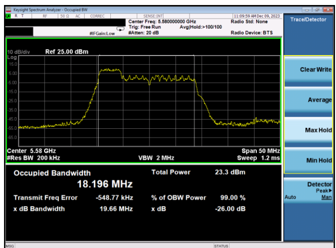
Plot 7-29. 26dB BW & 99% OBW Antenna 5T (20MHz BW 11ax Index 37 – RU52 – Ch.116)
