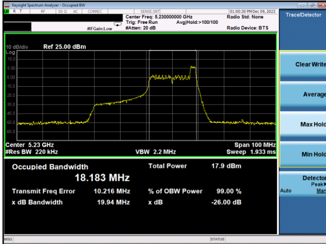
Plot 7-51. 26dB BW & 99% OBW Antenna 3b (40MHz BW 11ax Index 17 - RU26 - Ch.46)
