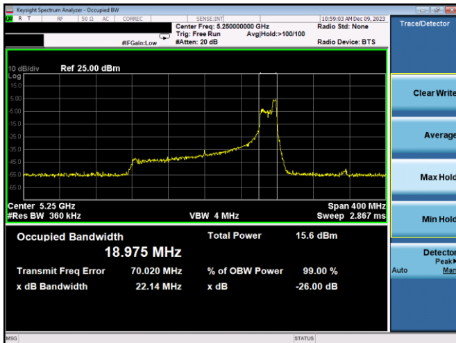
Plot 7-15. 26dB BW & 99% OBW Antenna 5T (160MHz BW 11ax Index 52 – RU52 – Ch.50 (U))
