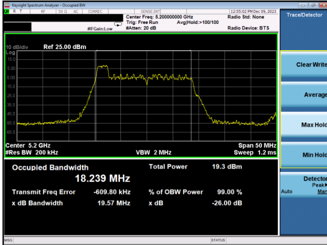
Plot 7-45. 26dB BW & 99% OBW Antenna 3b (20MHz BW 11ax Index 0 – RU26 – Ch.40)
