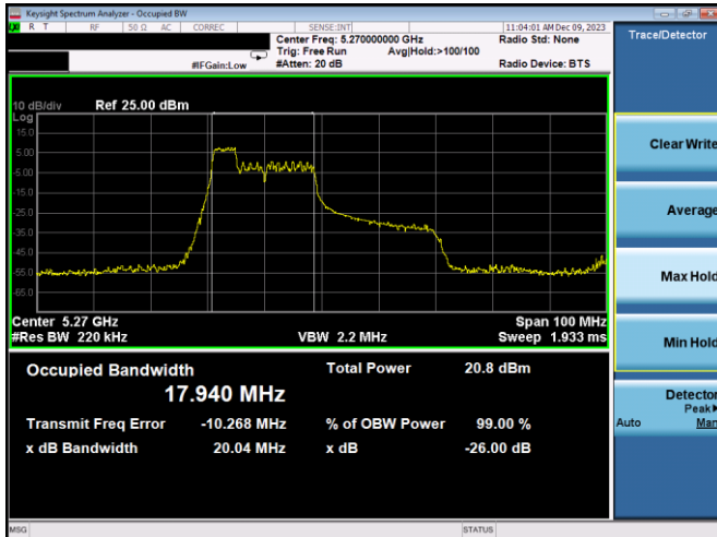
Plot 7-21. 26dB BW & 99% OBW Antenna 5T (40MHz BW 11ax Index 37 – RU52 – Ch.54)
