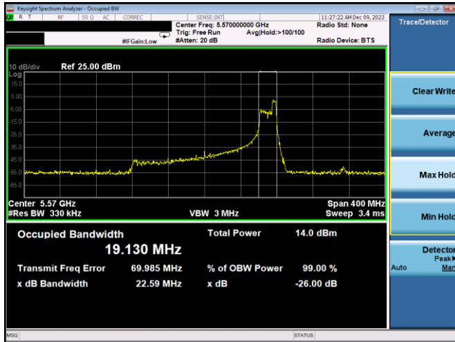
Plot 7-43. 26dB BW & 99% OBW Antenna 5T (160MHz BW 11ax Index 52 – RU52 – Ch.114 (U))
