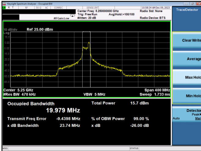
Plot 7-14. 26dB BW & 99% OBW Antenna 5T (160MHz BW 11ax Index 52 – RU52 – Ch.50 (L))
