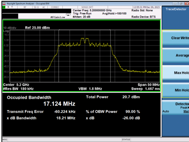
Plot 7-46. 26dB BW & 99% OBW Antenna 3b (20MHz BW 11ax Index 4 – RU26 – Ch.40)
