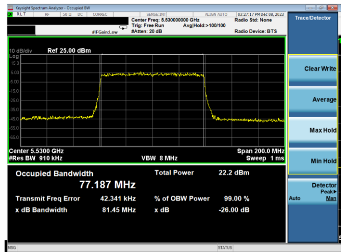
Plot 7-40. 26dB BW & 99% OBW Antenna 5T (80MHz BW 11ax – RU996 – Ch.106)
