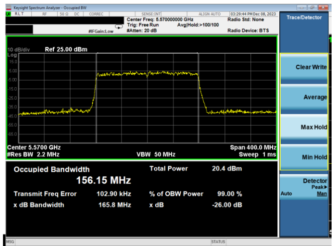
Plot 7-44. 26dB BW & 99% OBW Antenna 5T (160MHz BW 11ax – RU996x2 – Ch.114)
