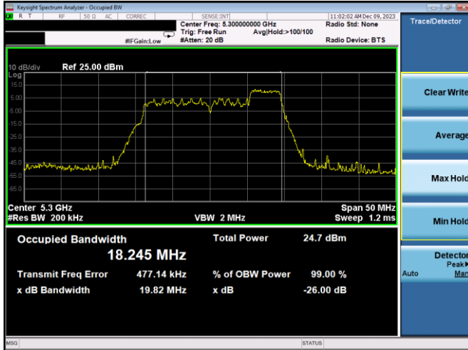
Plot 7-19. 26dB BW & 99% OBW Antenna 5T (20MHz BW 11ax Index 40 – RU52 – Ch.60)
