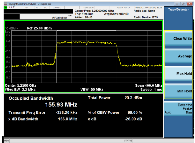
Plot 7-16. 26dB BW & 99% OBW Antenna 5T (160MHz BW 11ax – RU996x2 – Ch.50)
