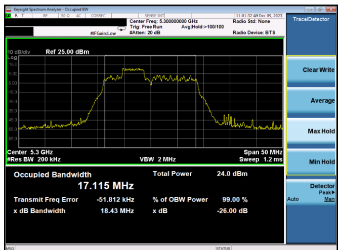
Plot 7-18. 26dB BW & 99% OBW Antenna 5T (20MHz BW 11ax Index 38 – RU52 – Ch.60)
