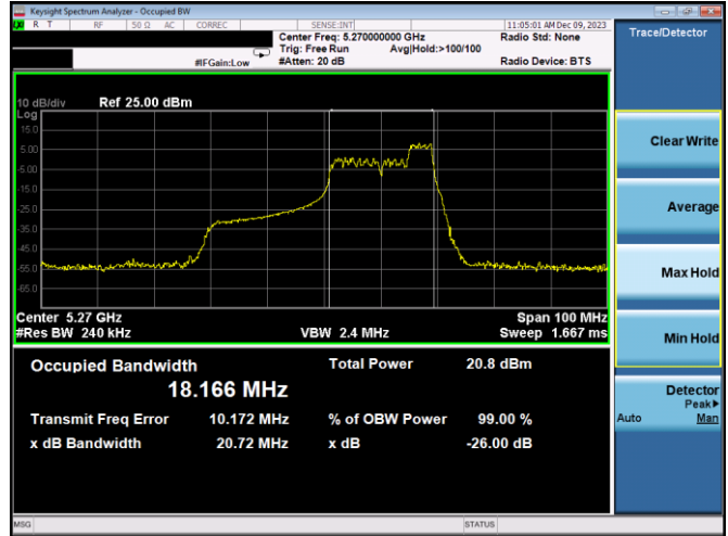
Plot 7-23. 26dB BW & 99% OBW Antenna 5T (40MHz BW 11ax Index 44 – RU52 – Ch.54)
