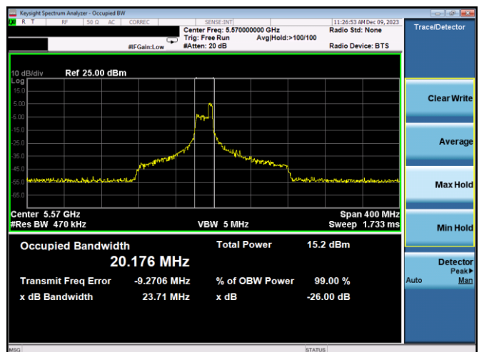
Plot 7-42. 26dB BW & 99% OBW Antenna 5T (160MHz BW 11ax Index 52 – RU52 – Ch.114 (L))
