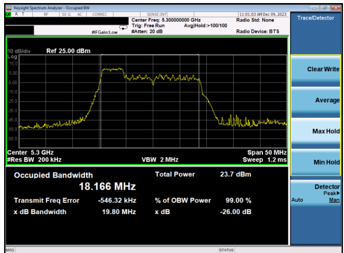
Plot 7-17. 26dB BW & 99% OBW Antenna 5T (20MHz BW 11ax Index 37 – RU52 – Ch.60)
