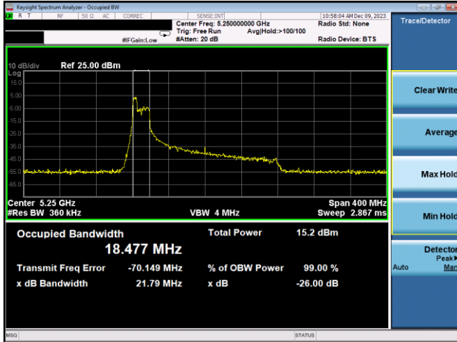
Plot 7-13. 26dB BW & 99% OBW Antenna 5T (160MHz BW 11ax Index 37 – RU52 – Ch.50 (L))
