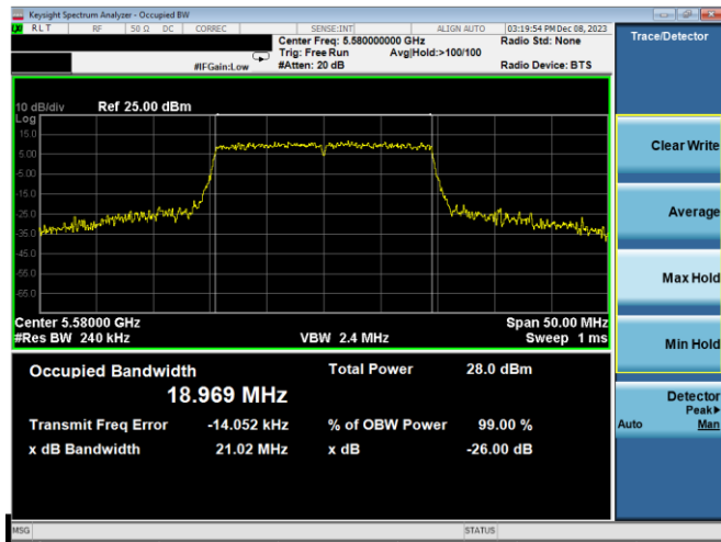
Plot 7-32. 26dB BW & 99% OBW Antenna 5T (20MHz BW 11ax- RU242 – Ch.116)
