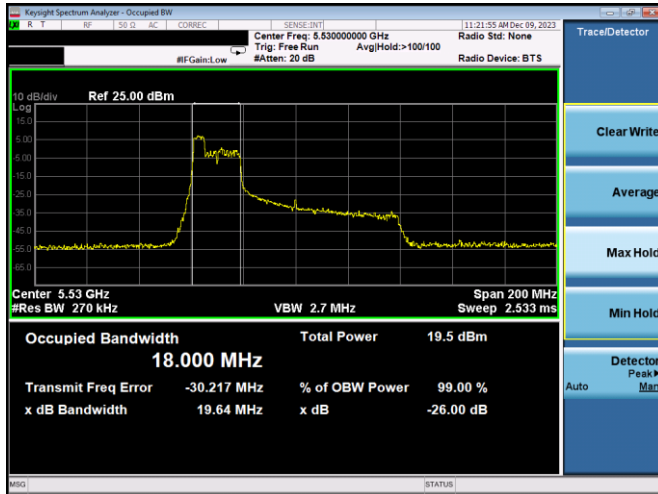
Plot 7-37. 26dB BW & 99% OBW Antenna 5T (80MHz BW 11ax Index 37 – RU52 – Ch.106)
