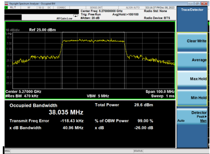
Plot 7-24. 26dB BW & 99% OBW Antenna 5T (40MHz BW 11ax – RU484 – Ch.54)
