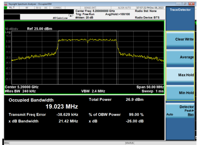
Plot 7-48. 26dB BW & 99% OBW Antenna 3b (20MHz BW 11ax – RU242 – Ch.40)
