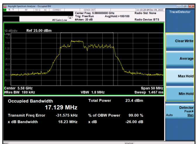
Plot 7-30. 26dB BW & 99% OBW Antenna 5T (20MHz BW 11ax Index 38 – RU52 – Ch.116)
