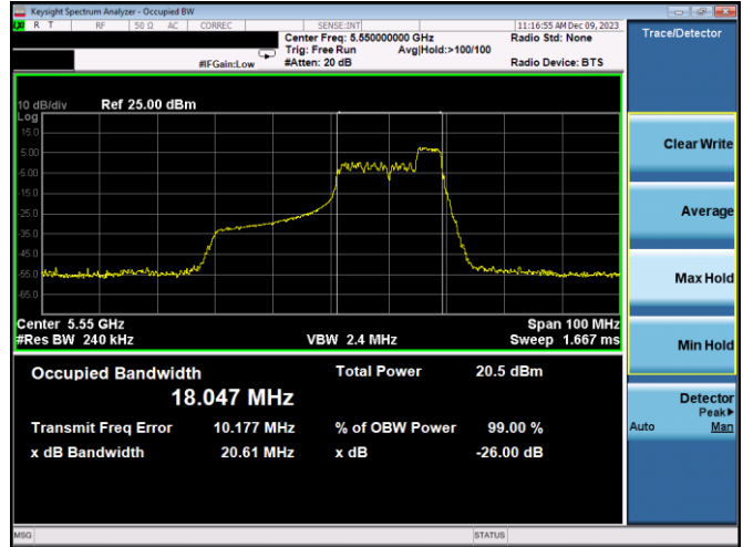
Plot 7-35. 26dB BW & 99% OBW Antenna 5T (40MHz BW 11ax Index 44 – RU52 – Ch.110)
