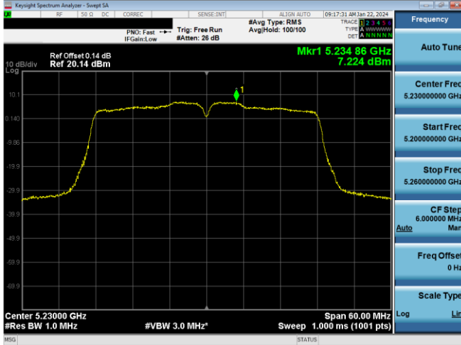
Plot 7-583. PSD CDD Primary Antenna 5T (40MHz BW 802.11n - Ch. 46, MCS10)
