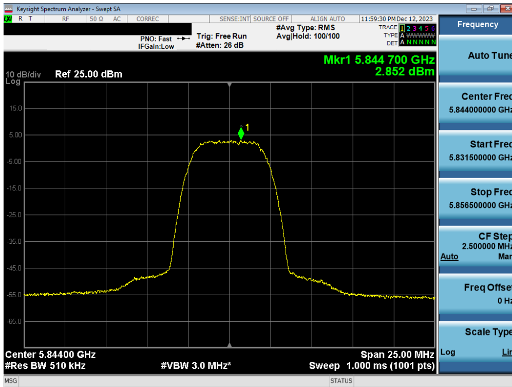
Plot 7-57. PSD Antenna 5T (HDR8, ePA 5844MHz)
