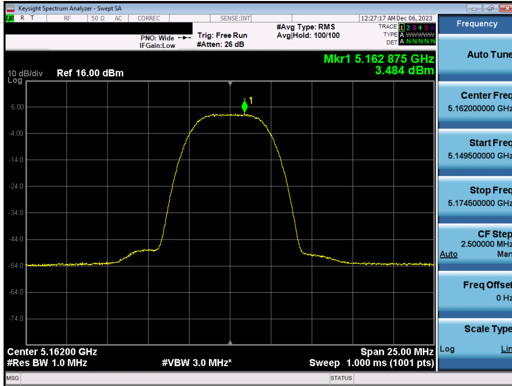
Plot 7-91. PSD Antenna 1b (HDR8, ePA – 5162MHz)
