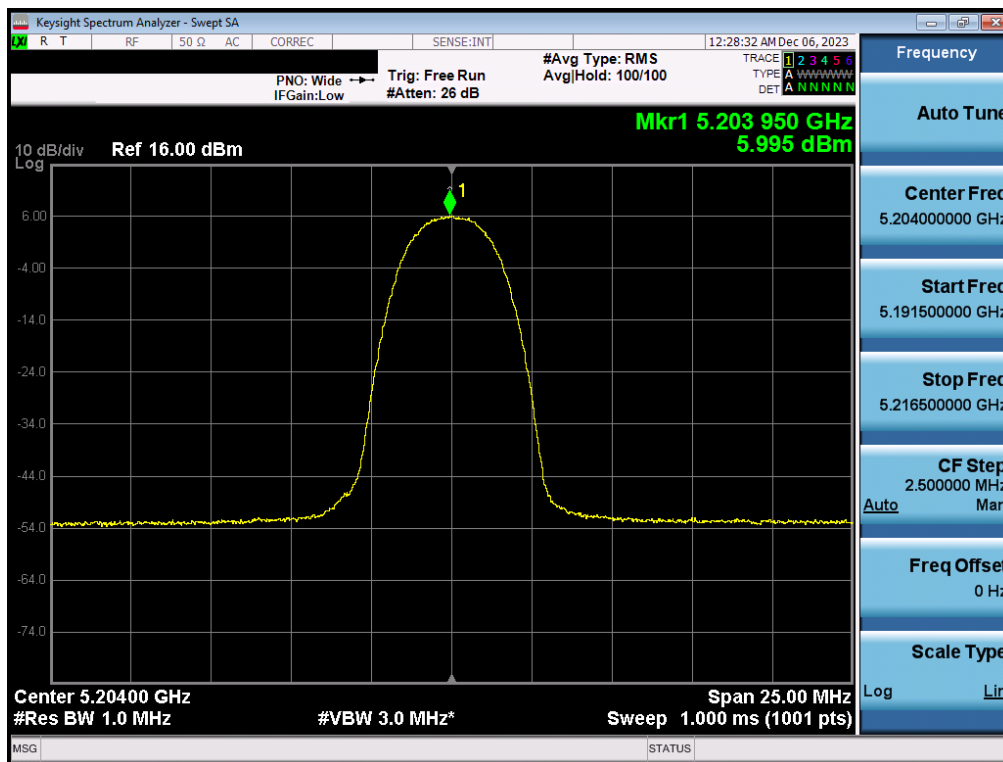
Plot 7-86. PSD Antenna 1b (HDR4, ePA – 5204MHz)
