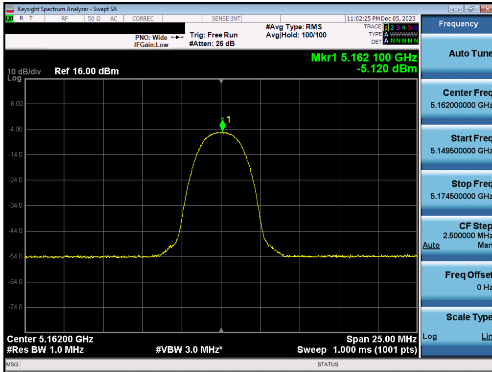
Plot 7-64. PSD Antenna 3b (HDR4, iPA – 5162MHz)
