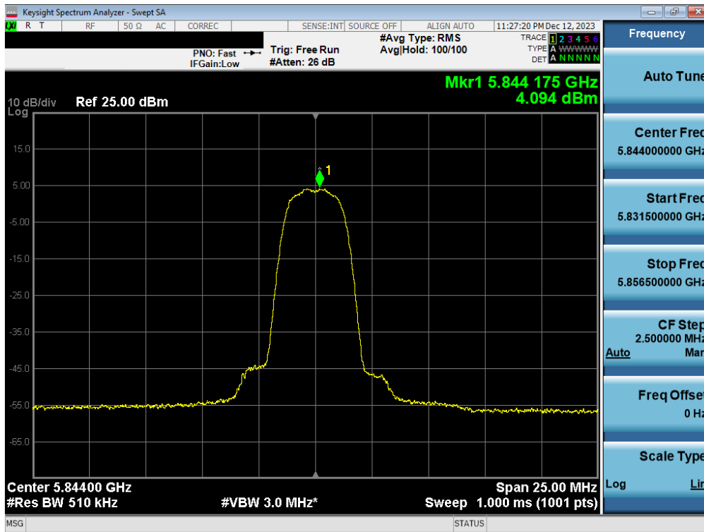
Plot 7-99. PSD Antenna 1b (HDR4, ePA 5844MHz)
