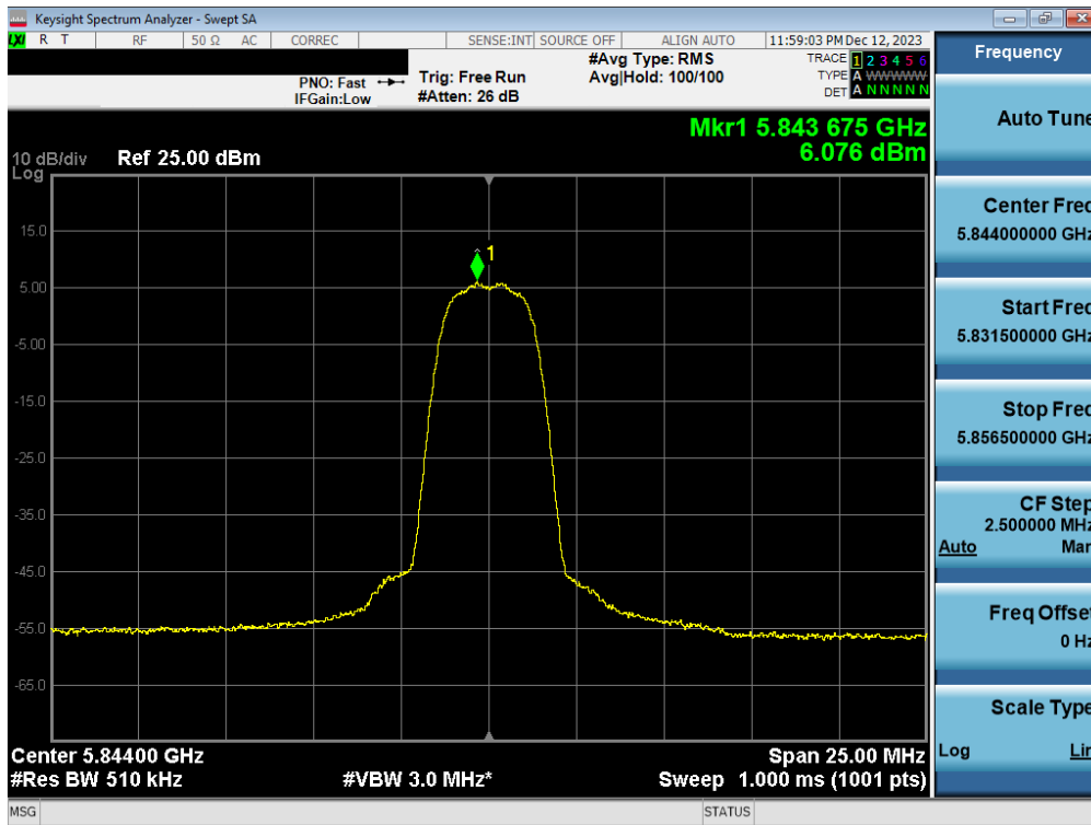
Plot 7-51. PSD Antenna 5T (HDR4, ePA 5844MHz)
