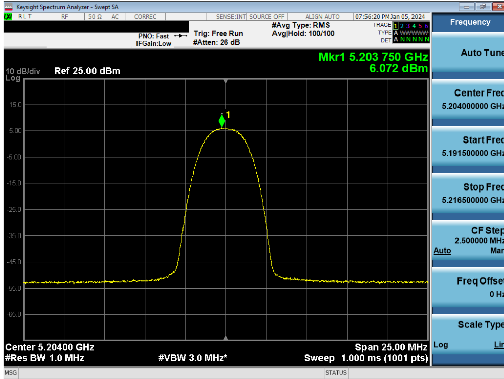
Plot 7-111. FCC PSD TxBF Antenna 5T (HDR4, ePA - 5204MHz)
