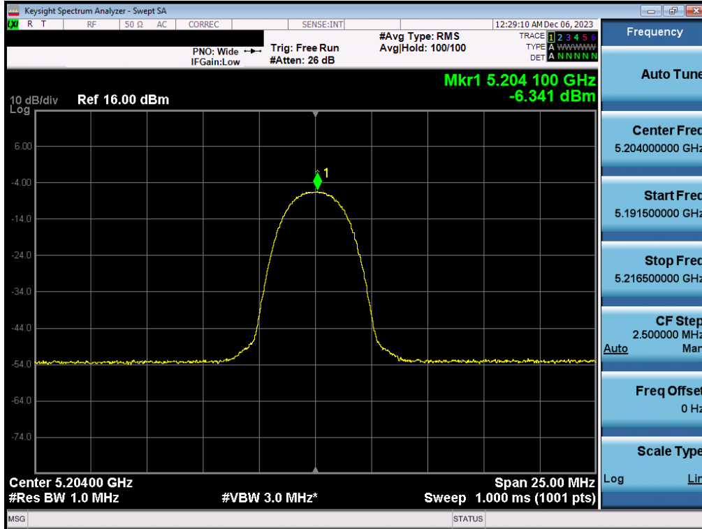
Plot 7-89. PSD Antenna 1b (HDR4, iPA – 5204MHz)
