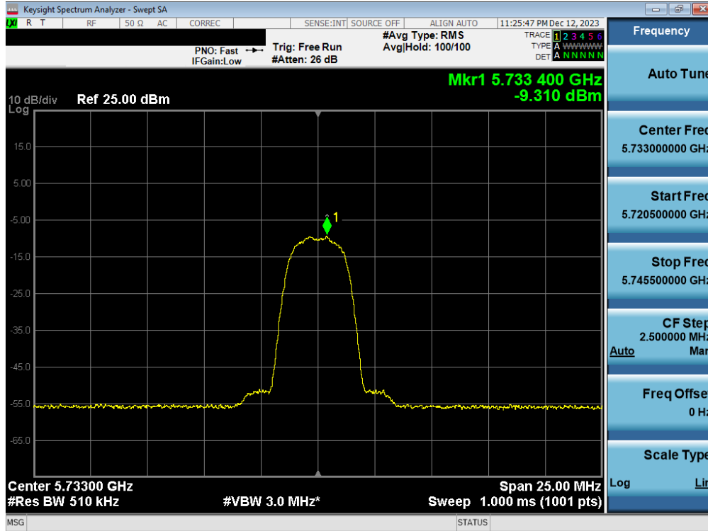
Plot 7-100. PSD Antenna 1b (HDR4, iPA 5733MHz)
