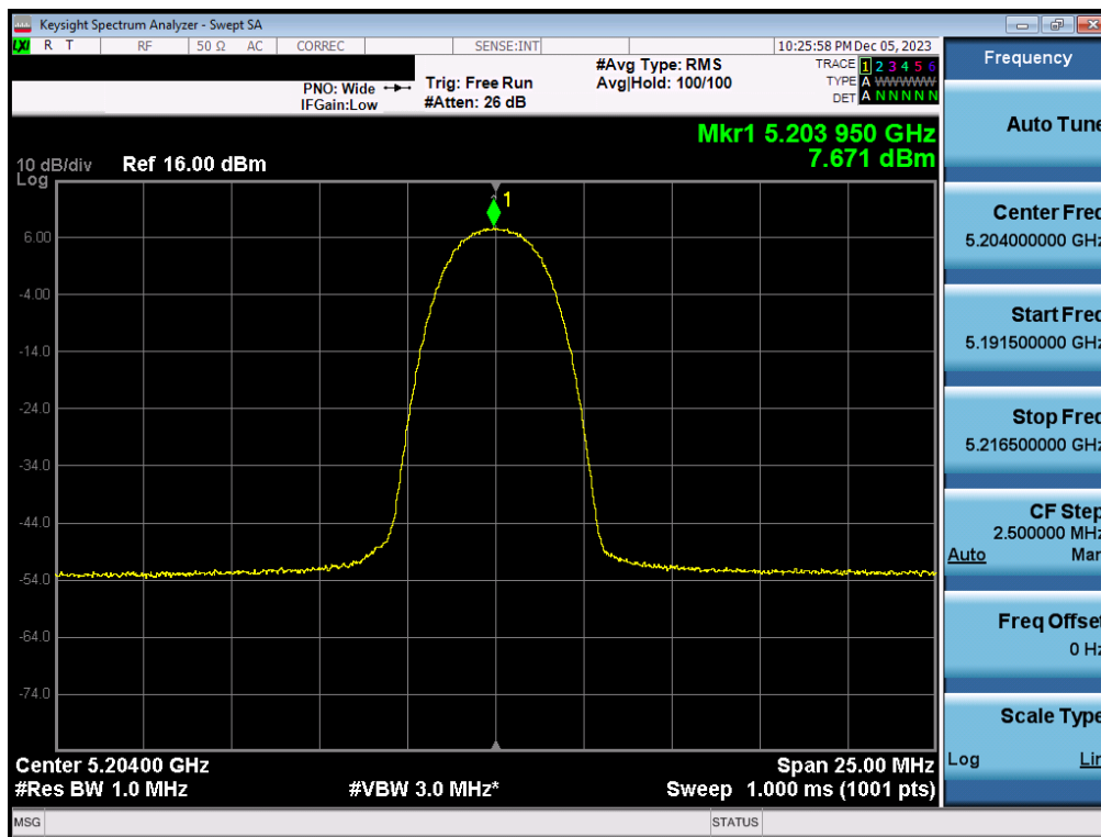
Plot 7-38. PSD Antenna 5T (HDR4, ePA – 5204MHz)
