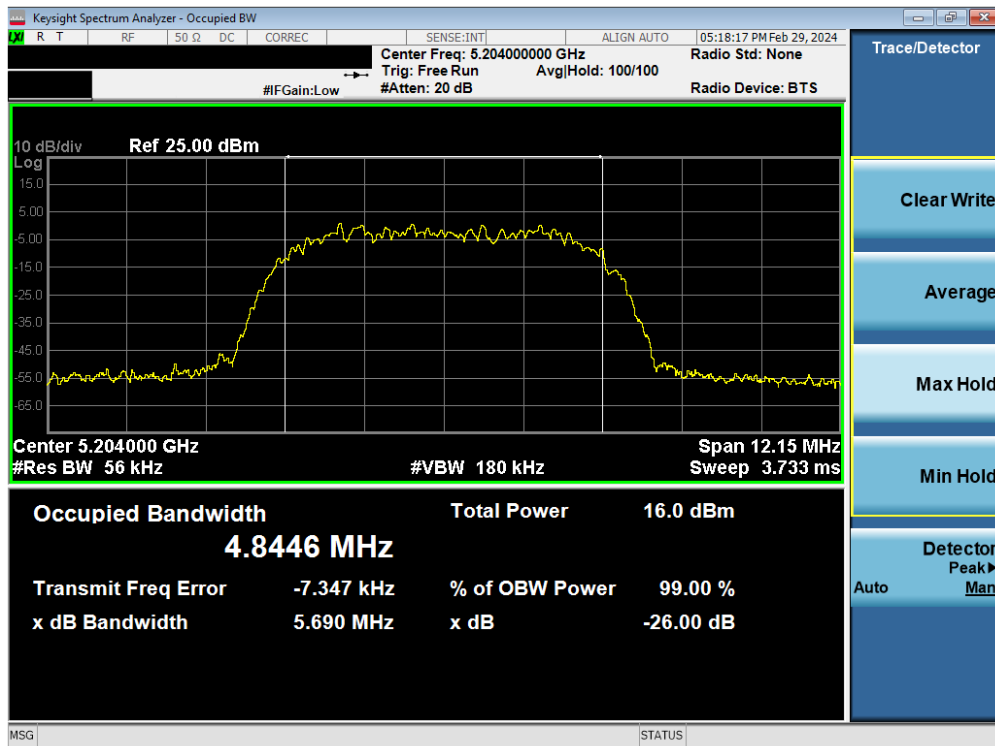
Plot 7-5. 26dB BW & 99% OBW Antenna 5T (HDR8, ePA– 5204MHz)
