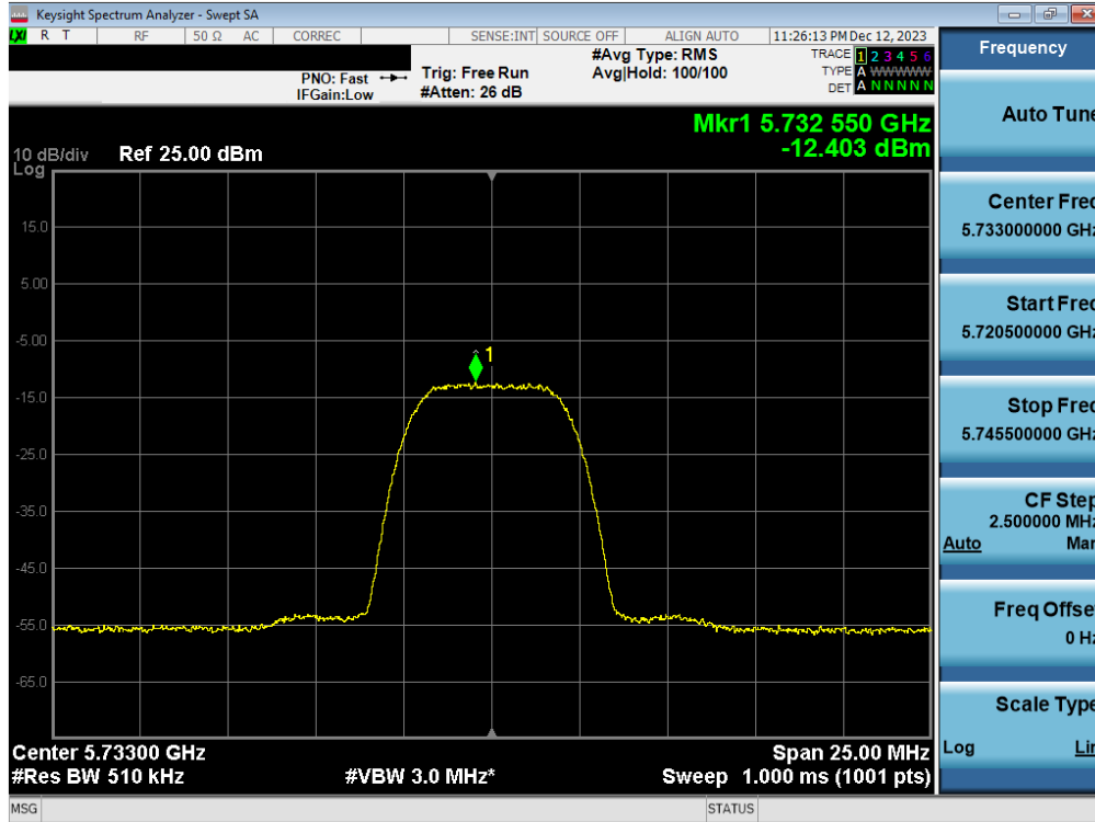
Plot 7-106. PSD Antenna 1b (HDR8, iPA 5733MHz)
