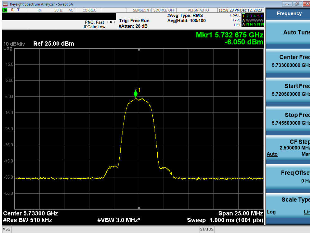
Plot 7-52. PSD Antenna 5T (HDR4, iPA 5733MHz)
