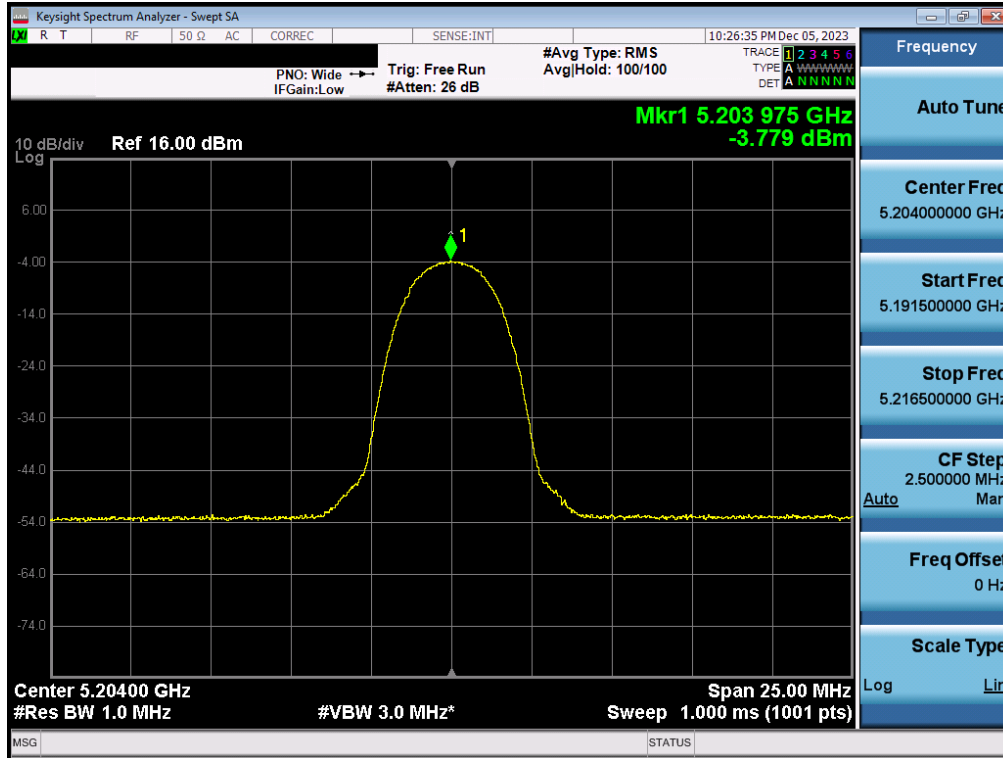
Plot 7-41. PSD Antenna 5T (HDR4, iPA – 5204MHz)
