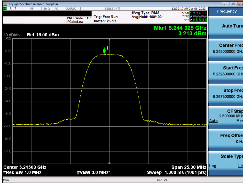
Plot 7-93. PSD Antenna 1b (HDR8, ePA – 5245MHz)
