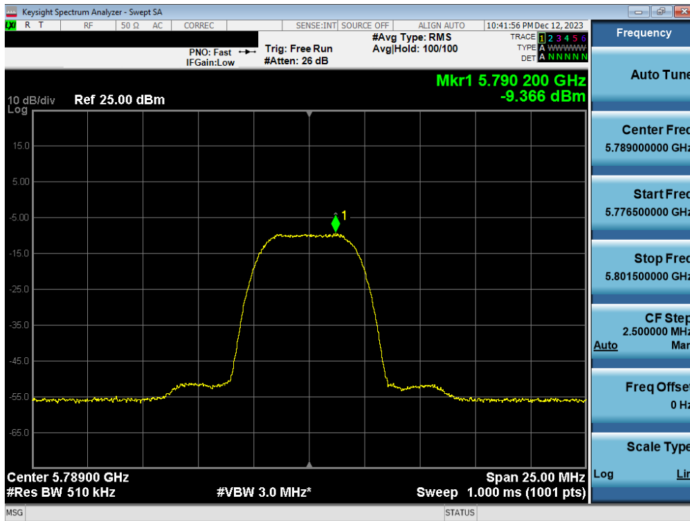
Plot 7-59. PSD Antenna 5T (HDR8, iPA 5789MHz)
