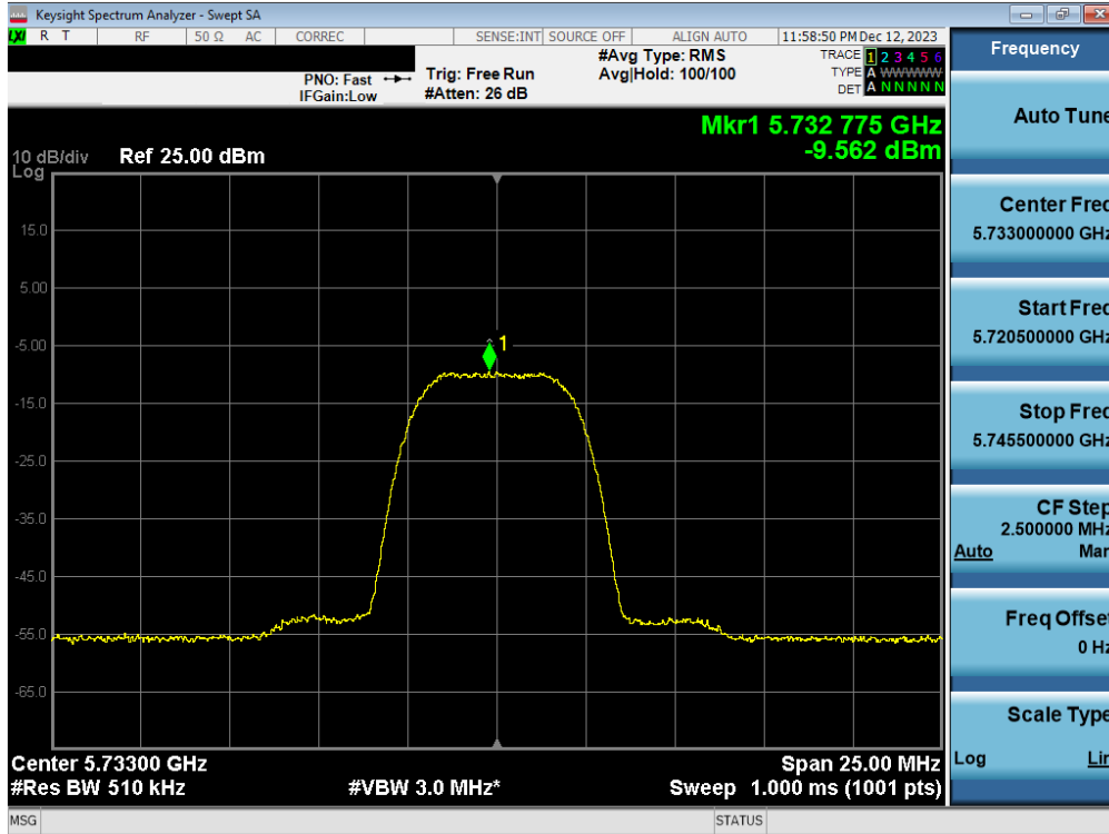
Plot 7-58. PSD Antenna 5T (HDR8, iPA 5733MHz)
