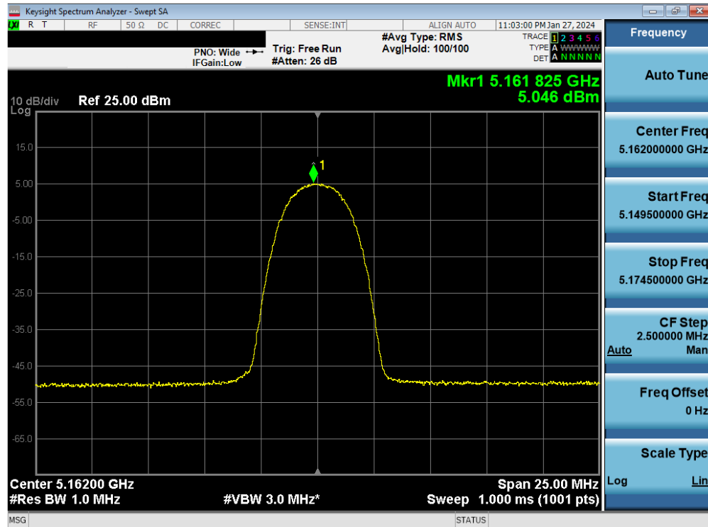
Plot 7-110. FCC PSD TxBF Antenna 3b (HDR4, ePA - 5162MHz)
