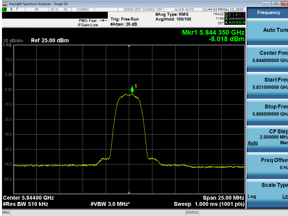
Plot 7-78. PSD Antenna 3b (HDR4, iPA 5844MHz)
