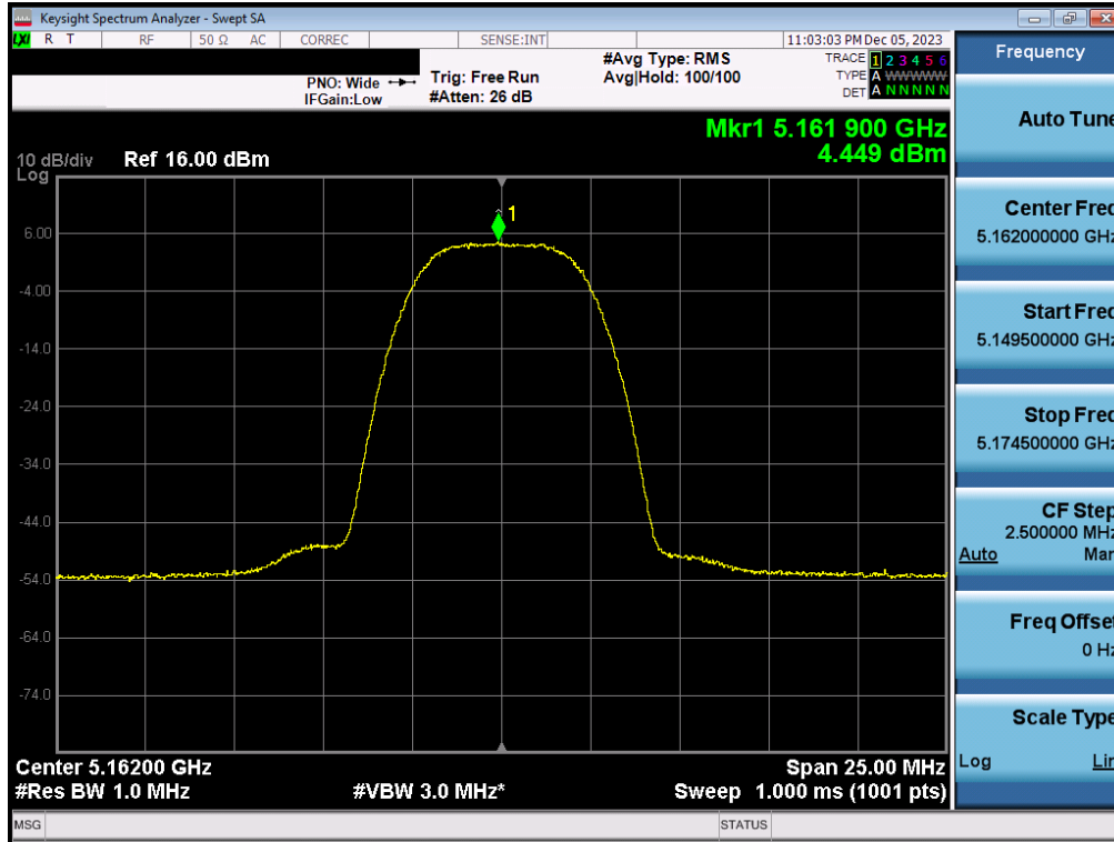
Plot 7-67. PSD Antenna 3b (HDR8, ePA – 5162MHz)
