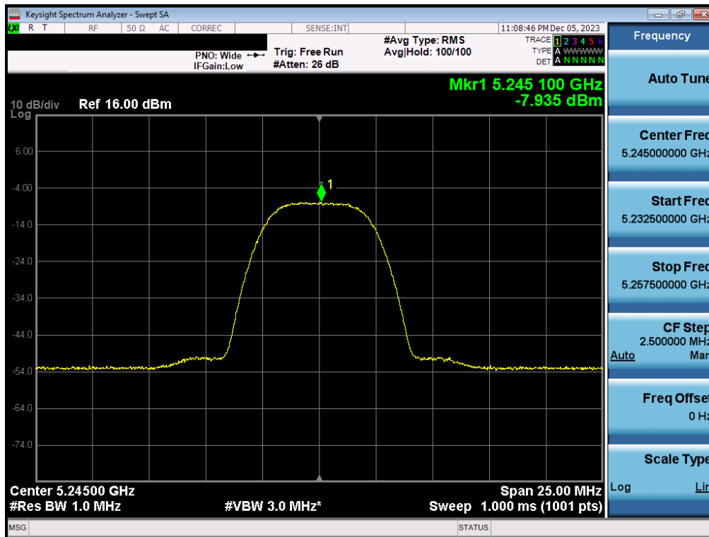
Plot 7-72. PSD Antenna 3b (HDR8, iPA– 5245MHz)
