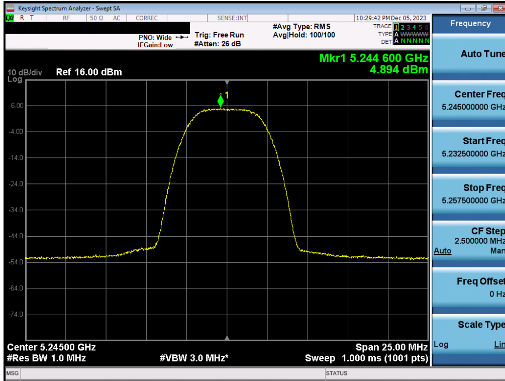
Plot 7-45. PSD Antenna 5T (HDR8, ePA – 5245MHz)
