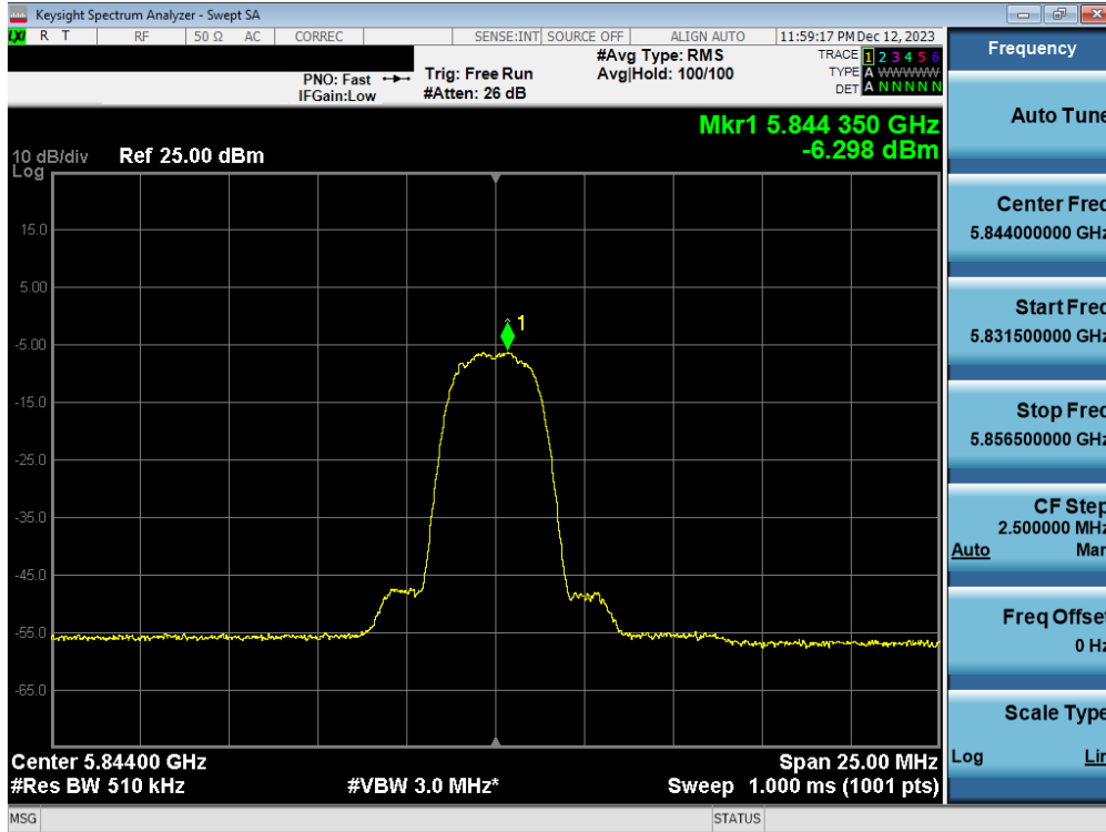
Plot 7-54. PSD Antenna 5T (HDR4, iPA 5844MHz)
