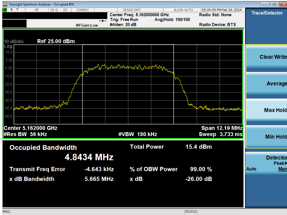
Plot 7-10. 26dB BW & 99% OBW Antenna 3b (HDR8, ePA- 5162MHz)
