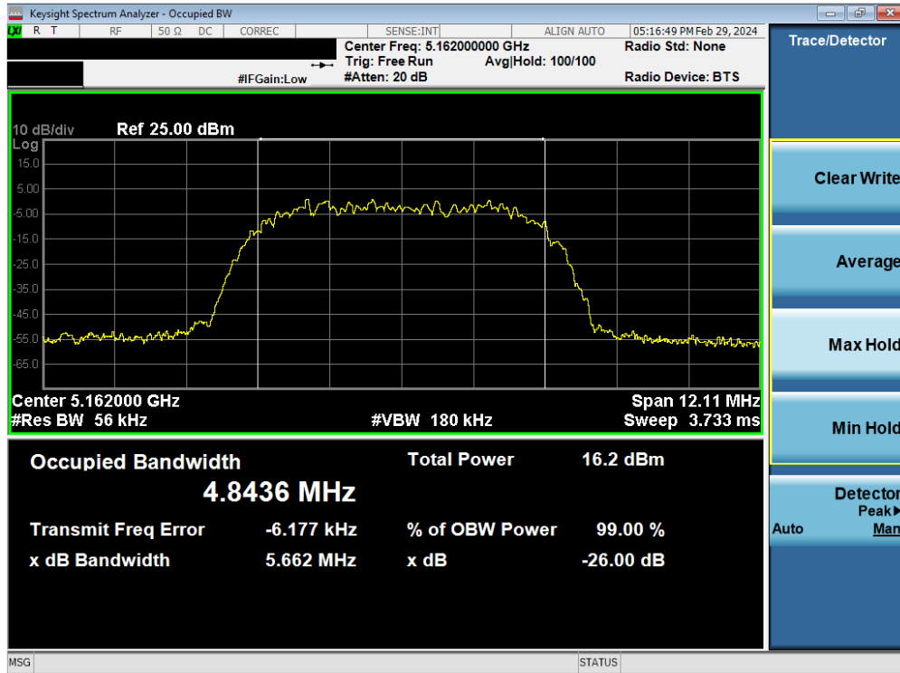
Plot 7-4. 26dB BW & 99% OBW Antenna 5T (HDR8, ePA– 5162MHz)
