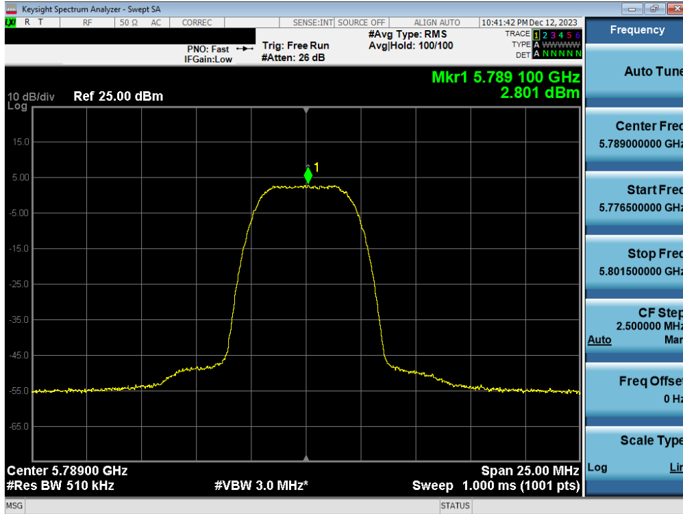
Plot 7-56. PSD Antenna 5T (HDR8, ePA 5789MHz)
