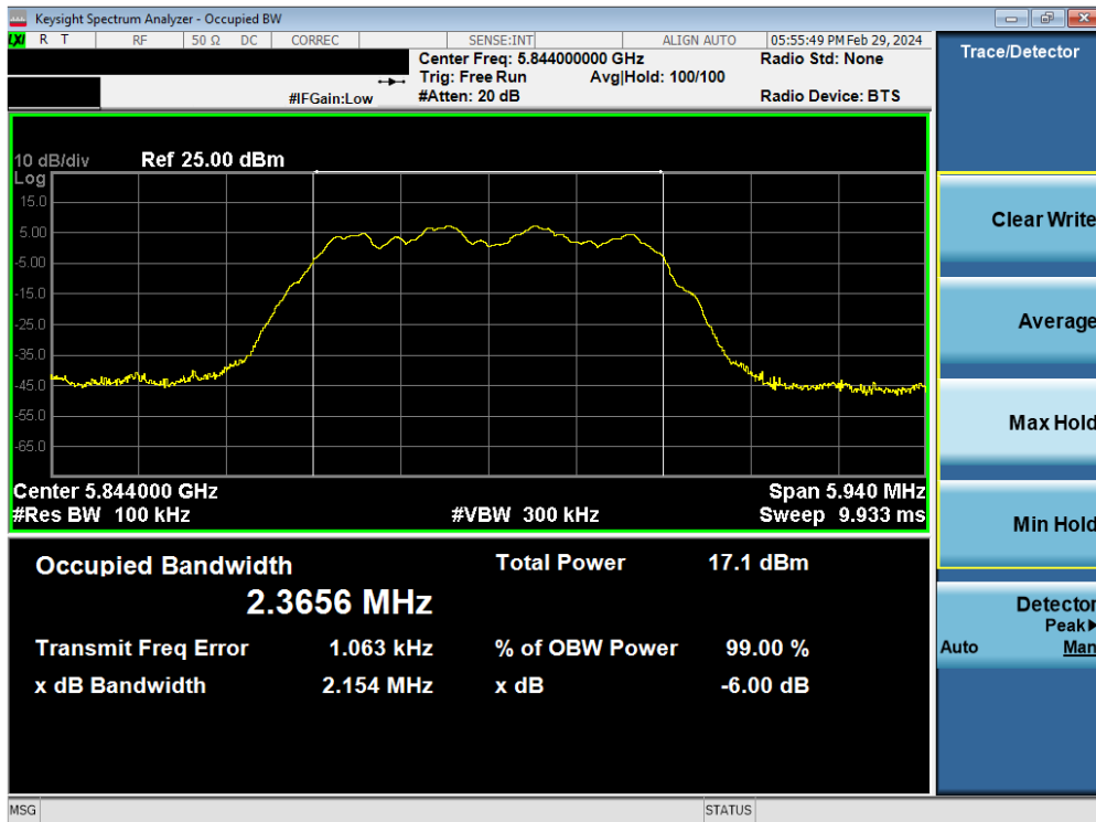
Plot 7-27. 6dB BW & 99% OBW Antenna 3b (HDR4, ePA, 5844MHz)
