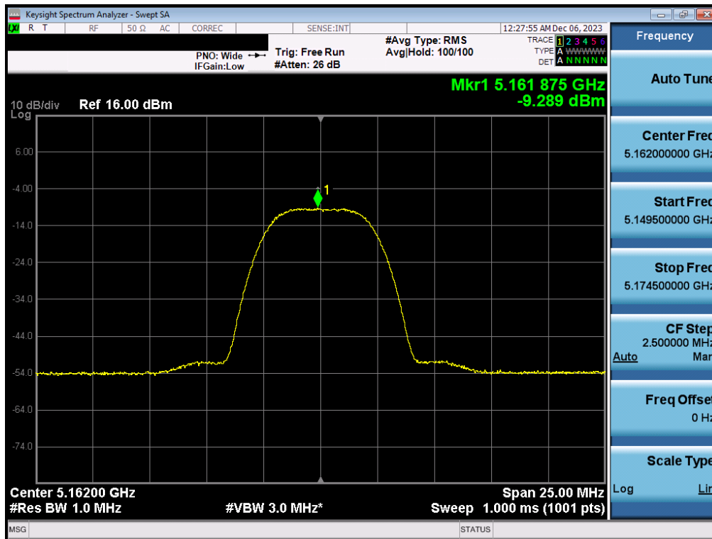
Plot 7-94. PSD Antenna 1b (HDR8, iPA – 5162MHz)
