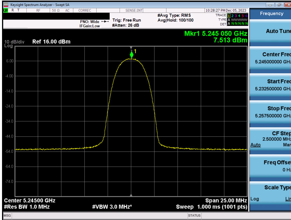
Plot 7-39. PSD Antenna 5T (HDR4, ePA – 5245MHz)
