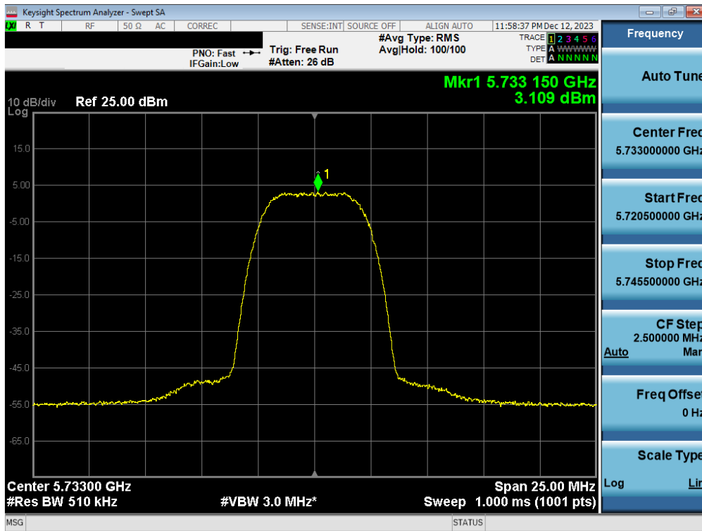
Plot 7-55. PSD Antenna 5T (HDR8, ePA 5733MHz)
