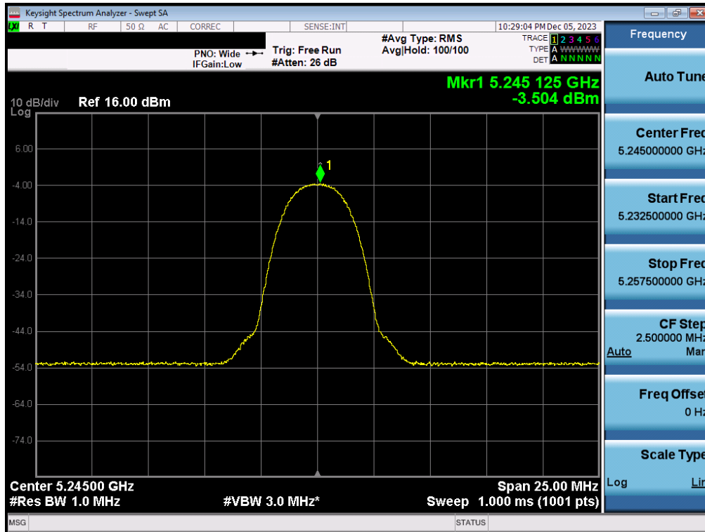
Plot 7-42. PSD Antenna 5T (HDR4, iPA– 5245MHz)
