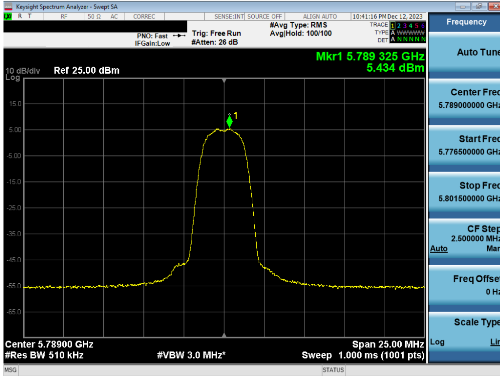
Plot 7-50. PSD Antenna 5T (HDR4, ePA 5789MHz)
