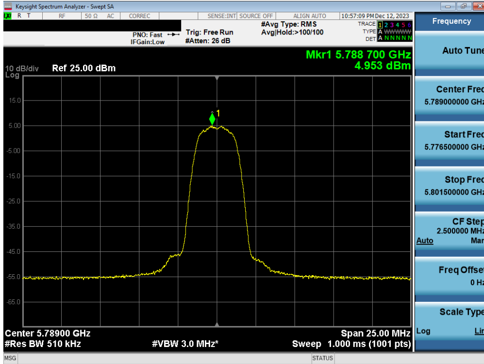
Plot 7-74. PSD Antenna 3b (HDR4, ePA 5789MHz)
