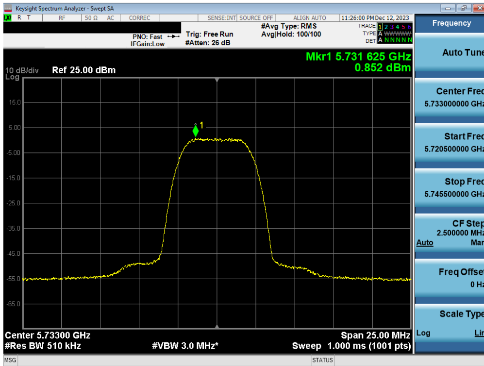
Plot 7-103. PSD Antenna 1b (HDR8, ePA 5733MHz)
