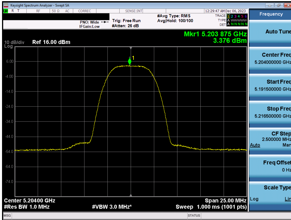
Plot 7-92. PSD Antenna 1b (HDR8, ePA – 5204MHz)
