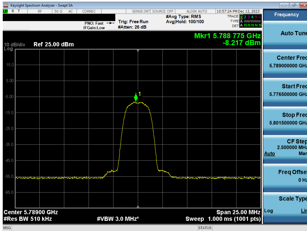
Plot 7-77. PSD Antenna 3b (HDR4, iPA 5789MHz)
