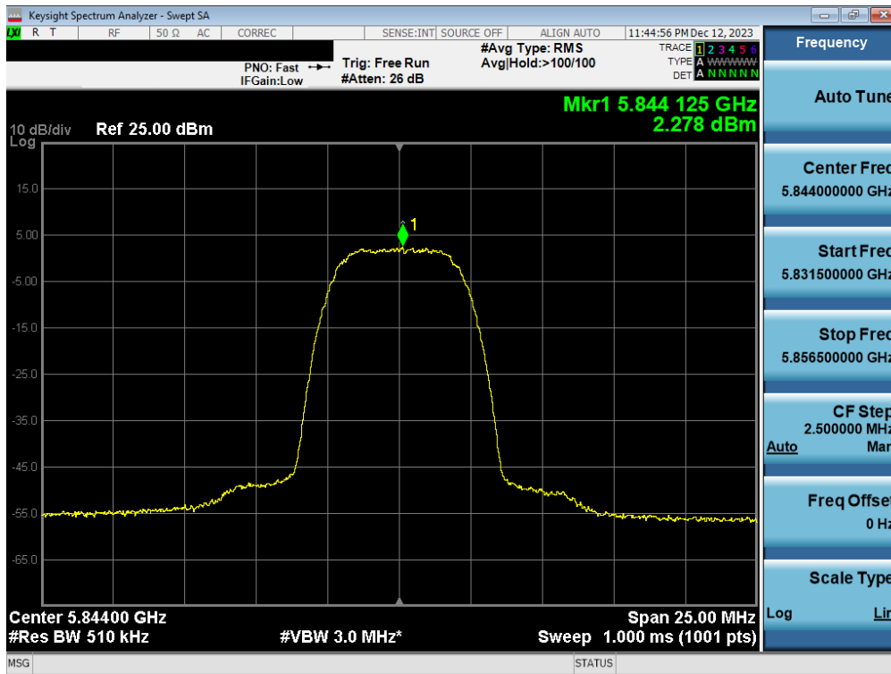
Plot 7-81. PSD Antenna 3b (HDR8, ePA 5844MHz)
