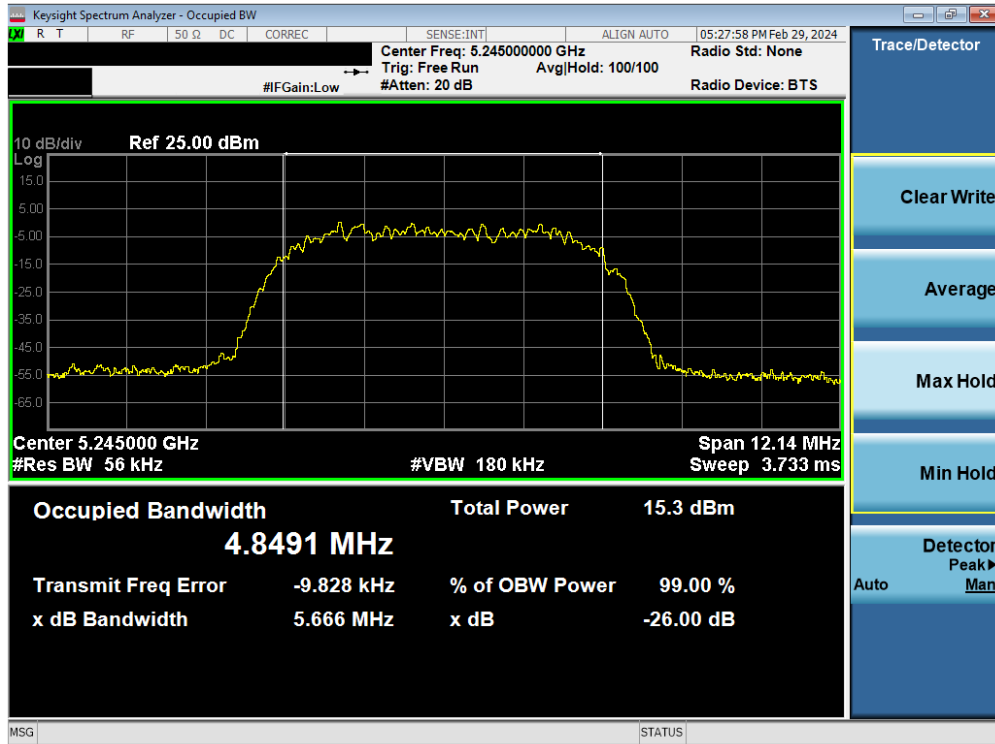
Plot 7-12. 26dB BW & 99% OBW Antenna 3b (HDR8, ePA- 5245MHz)
