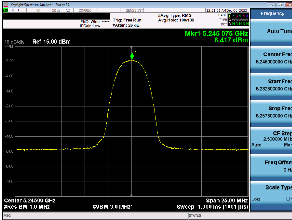
Plot 7-87. PSD Antenna 1b (HDR4, ePA– 5245MHz)
