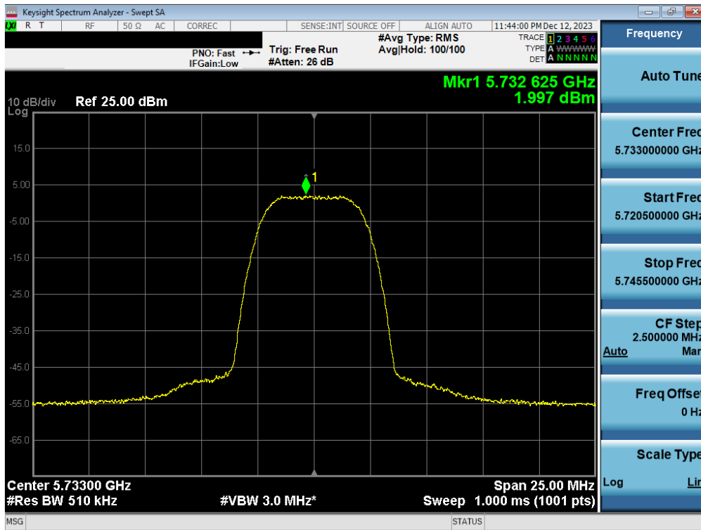
Plot 7-79. PSD Antenna 3b (HDR8, ePA 5733MHz)
