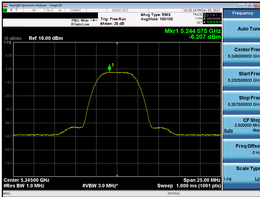
Plot 7-48. PSD Antenna 5T (HDR8, iPA– 5245MHz)
