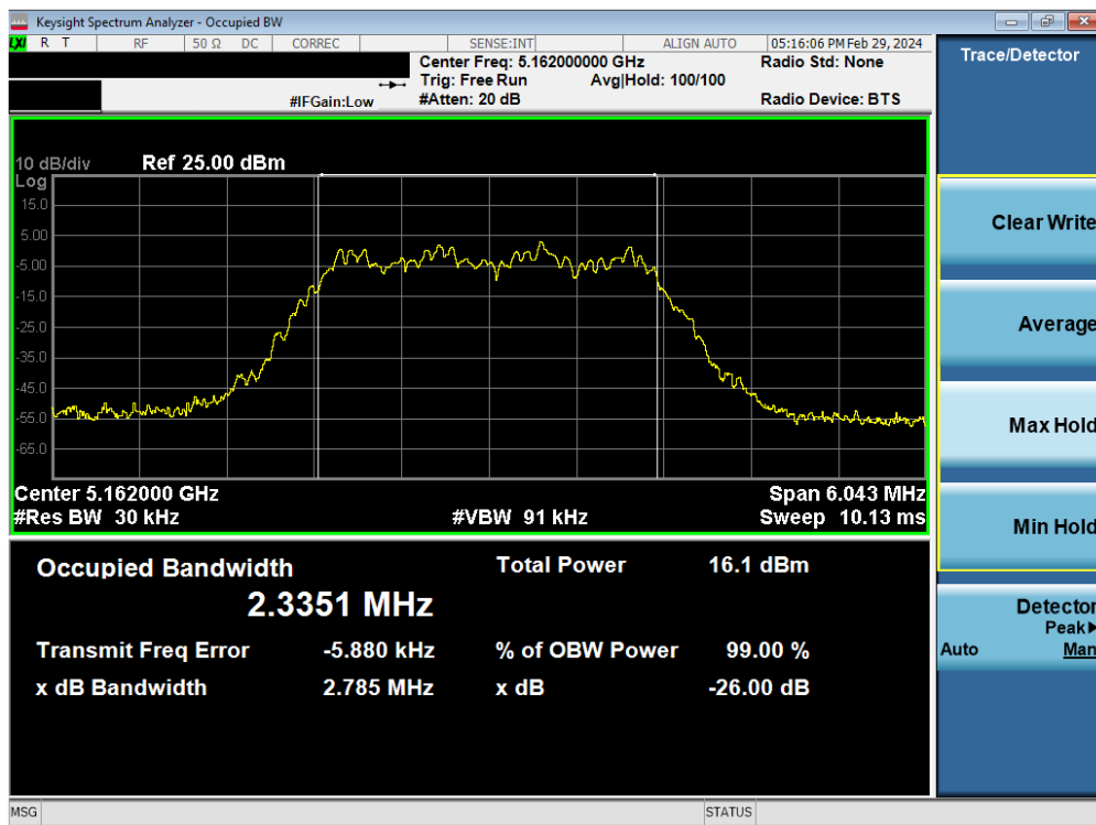
Plot 7-1. 26dB BW & 99% OBW Antenna 5T (HDR4, ePA– 5162MHz)
