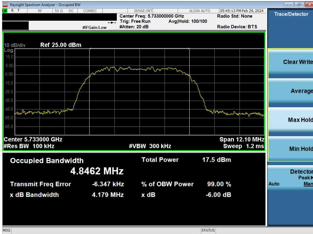
Plot 7-22. 6dB BW & 99% OBW Antenna 5T (HDR8, ePA, 5733MHz)
