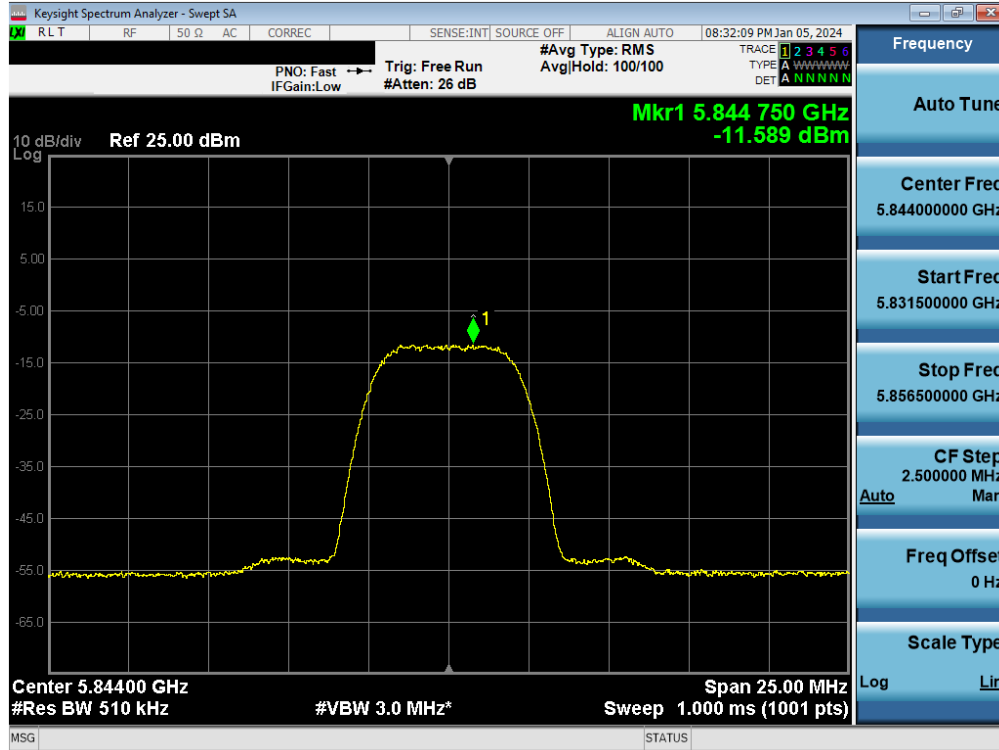
Plot 7-108. PSD Antenna 1b (HDR8, iPA 5844MHz)
