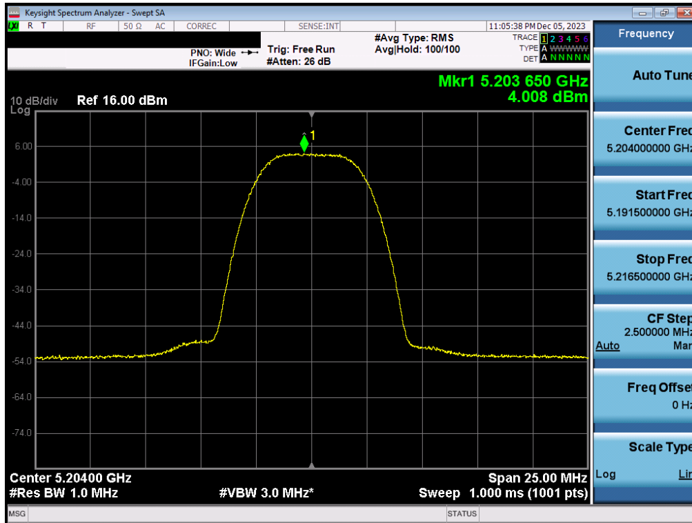
Plot 7-68. PSD Antenna 3b (HDR8, ePA – 5204MHz)
