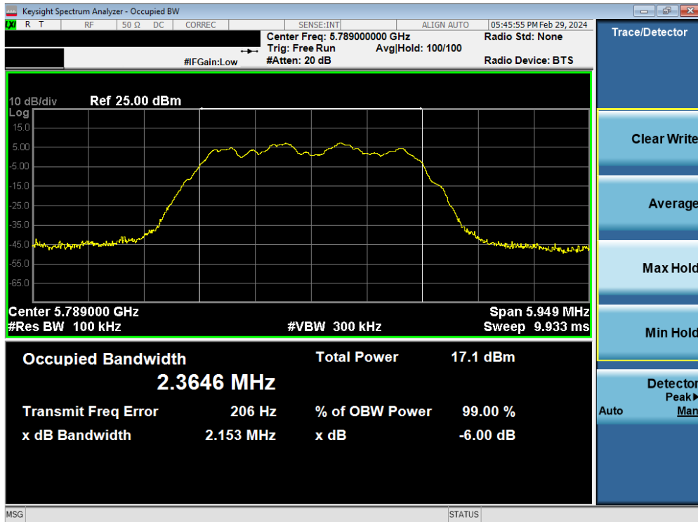
Plot 7-20. 6dB BW & 99% OBW Antenna 5T (HDR4, ePA, 5789MHz)
