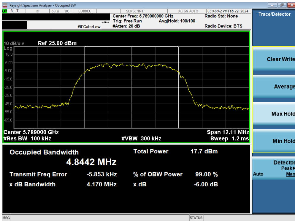
Plot 7-23. 6dB BW & 99% OBW Antenna 5T (HDR8, ePA, 5789MHz)
