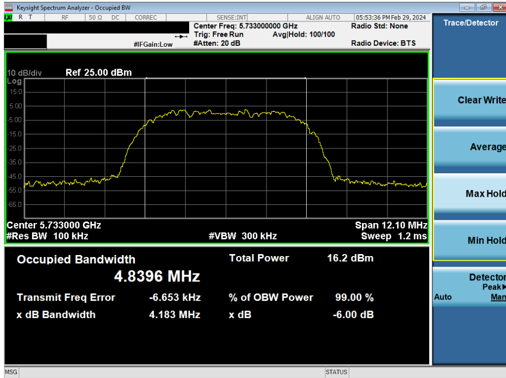
Plot 7-28. 6dB BW & 99% OBW Antenna 3b (HDR8, ePA, 5733MHz)
