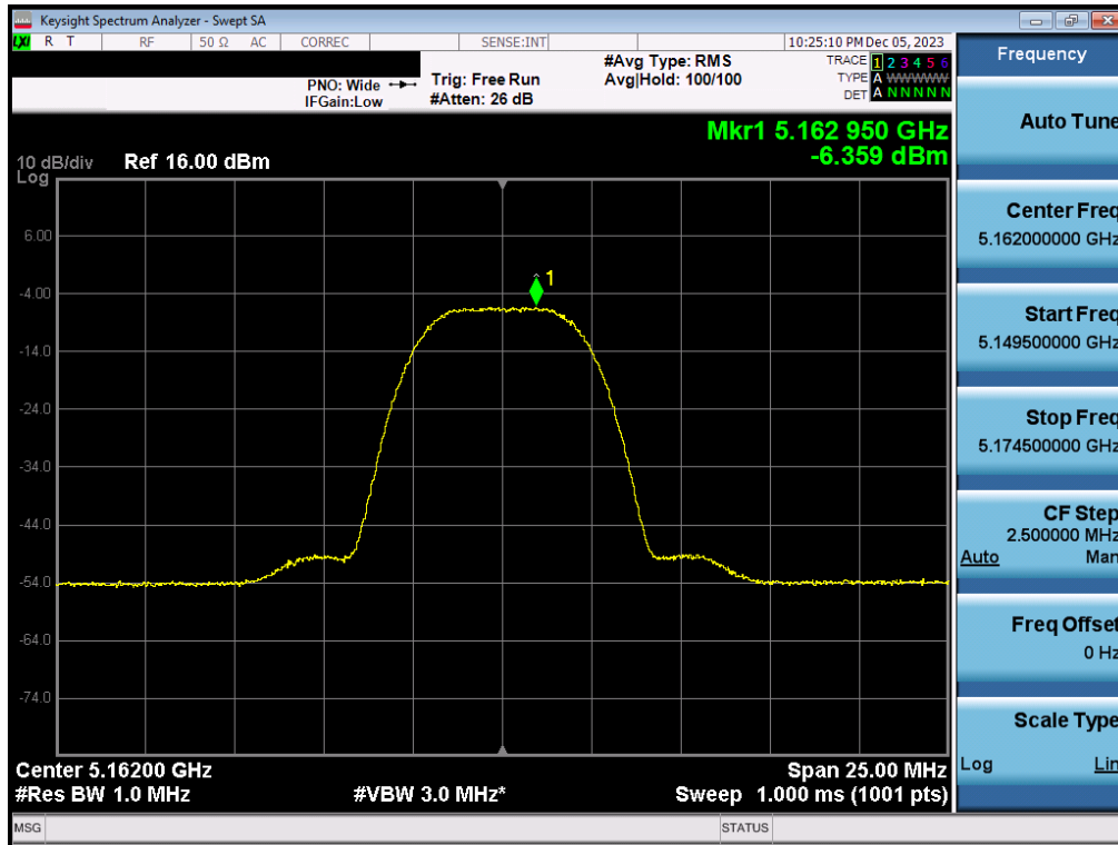
Plot 7-46. PSD Antenna 5T (HDR8, iPA – 5162MHz)
