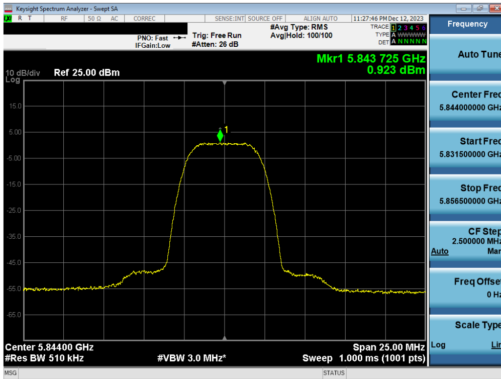
Plot 7-105. PSD Antenna 1b (HDR8, ePA 5844MHz)
