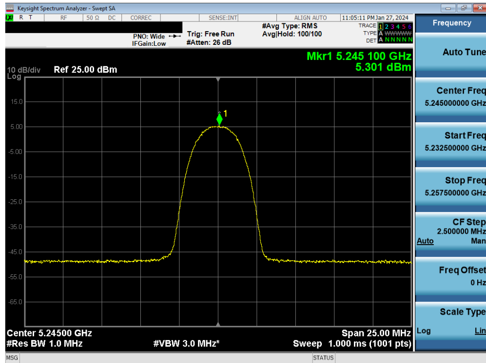
Plot 7-114. FCC PSD TxBF Antenna 3b (HDR4, ePA- 5245MHz)
