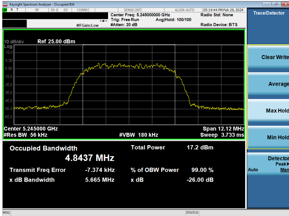
Plot 7-6. 26dB BW & 99% OBW Antenna 5T (HDR8, ePA – 5245MHz)
