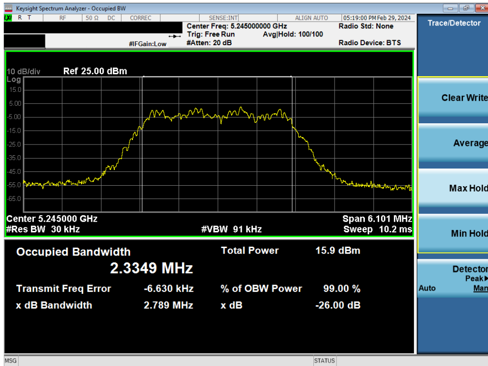
Plot 7-3. 26dB BW & 99% OBW Antenna 5T (HDR4, ePA – 5245MHz)
