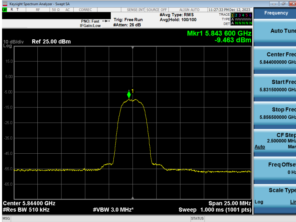
Plot 7-102. PSD Antenna 1b (HDR4, iPA 5844MHz)
