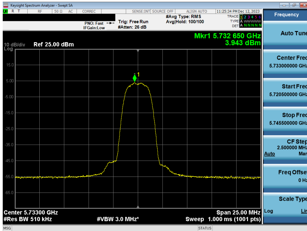
Plot 7-97. PSD Antenna 1b (HDR4, ePA 5733MHz)
