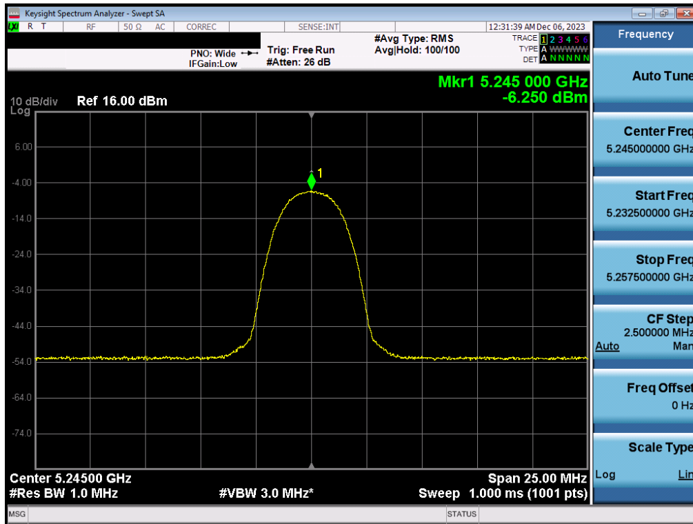
Plot 7-90. PSD Antenna 1b (HDR4, iPA– 5245MHz)
