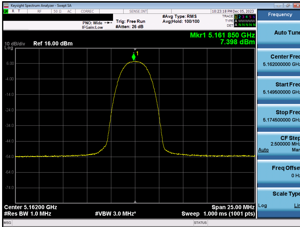
Plot 7-37. PSD Antenna 5T (HDR4, ePA – 5162MHz)
