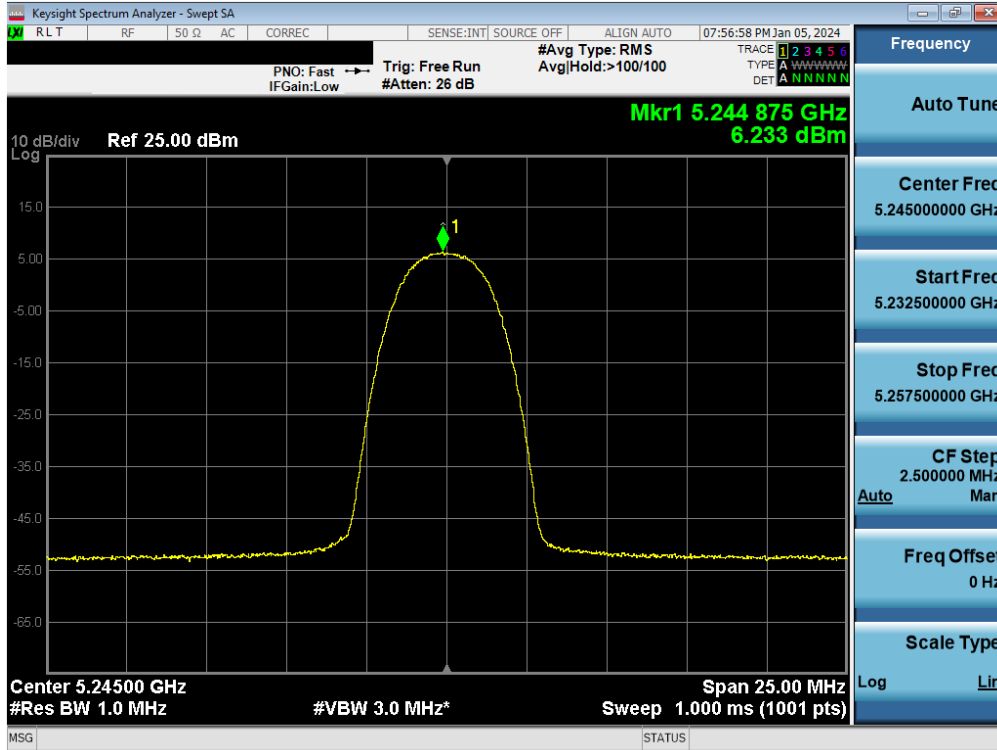
Plot 7-113. FCC PSD TxBF Antenna 5T (HDR4, ePA- 5245MHz)
