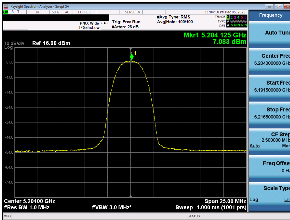
Plot 7-62. PSD Antenna 3b (HDR4, ePA – 5204MHz)
