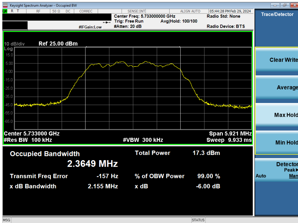
Plot 7-19. 6dB BW & 99% OBW Antenna 5T (HDR4, ePA, 5733MHz)
