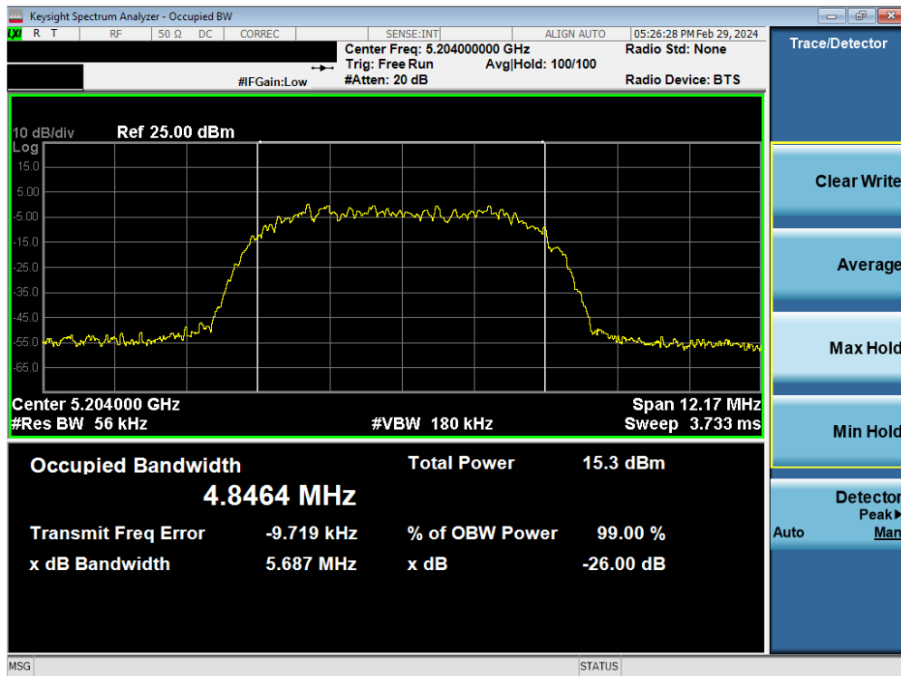
Plot 7-11. 26dB BW & 99% OBW Antenna 3b (HDR8, ePA- 5204MHz)
