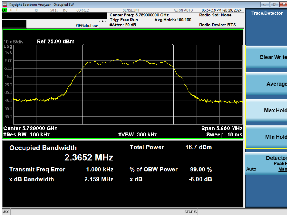
Plot 7-26. 6dB BW & 99% OBW Antenna 3b (HDR4, ePA, 5789MHz)
