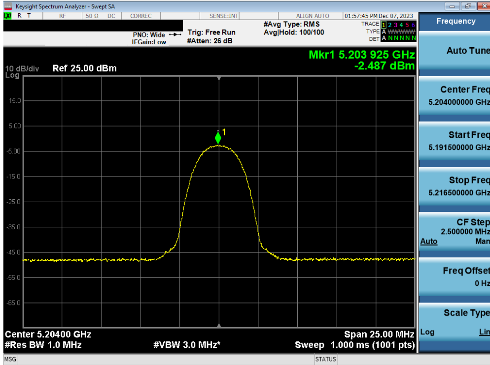
Plot 7-117. FCC/ISED PSD TxBF Antenna 5T (HDR4, iPA – 5204MHz)
