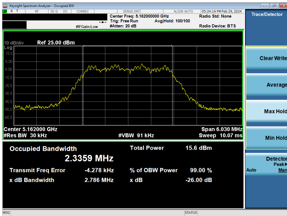
Plot 7-7. 26dB BW & 99% OBW Antenna 3b (HDR4, ePA– 5162MHz)
