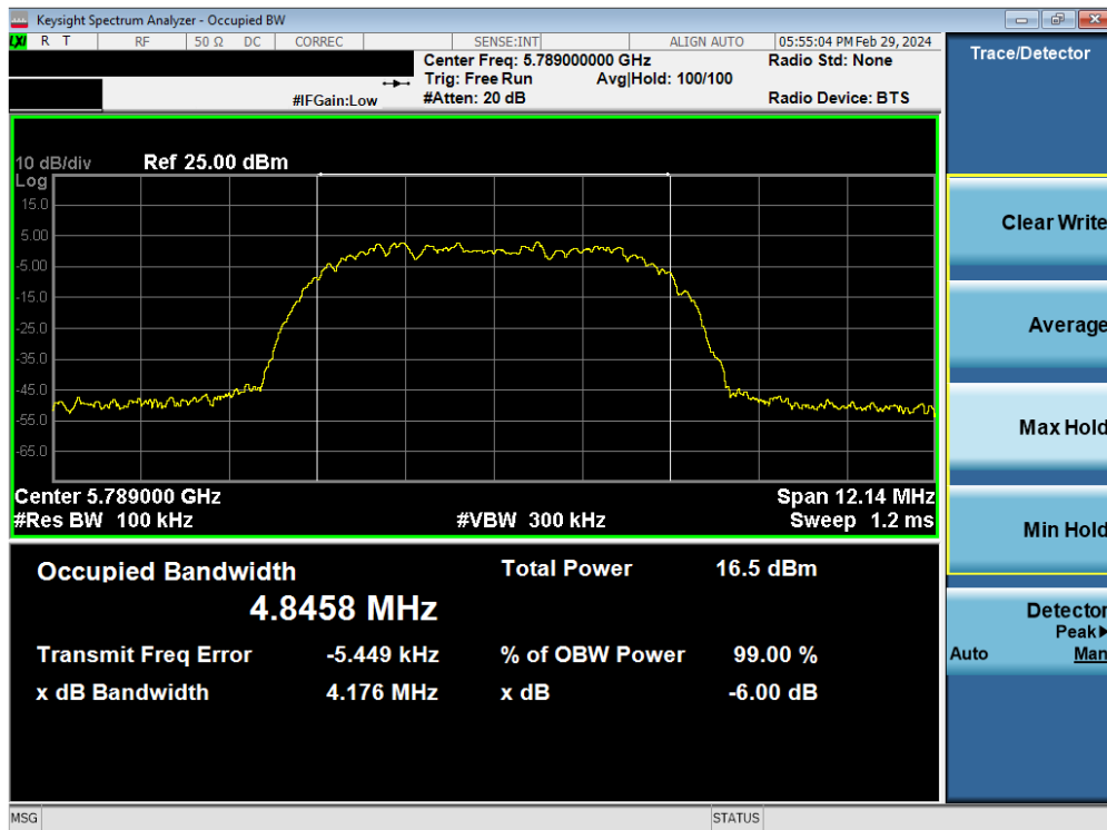
Plot 7-29. 6dB BW & 99% OBW Antenna 3b (HDR8, ePA, 5789MHz)
