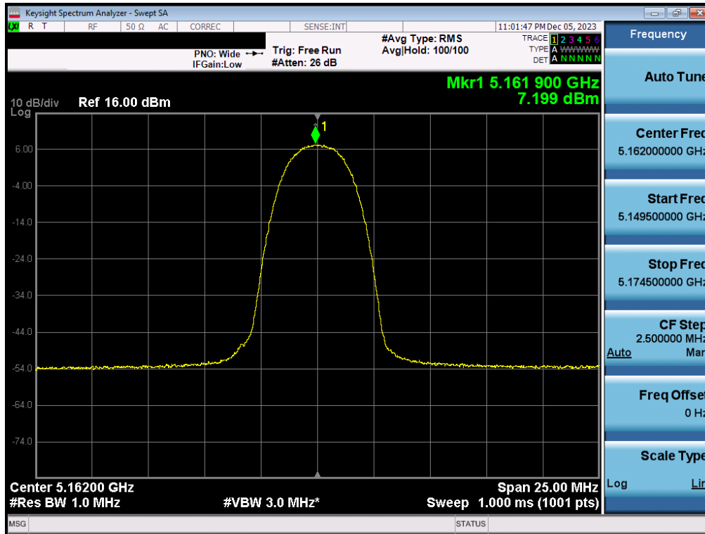
Plot 7-61. PSD Antenna 3b (HDR4, ePA – 5162MHz)
