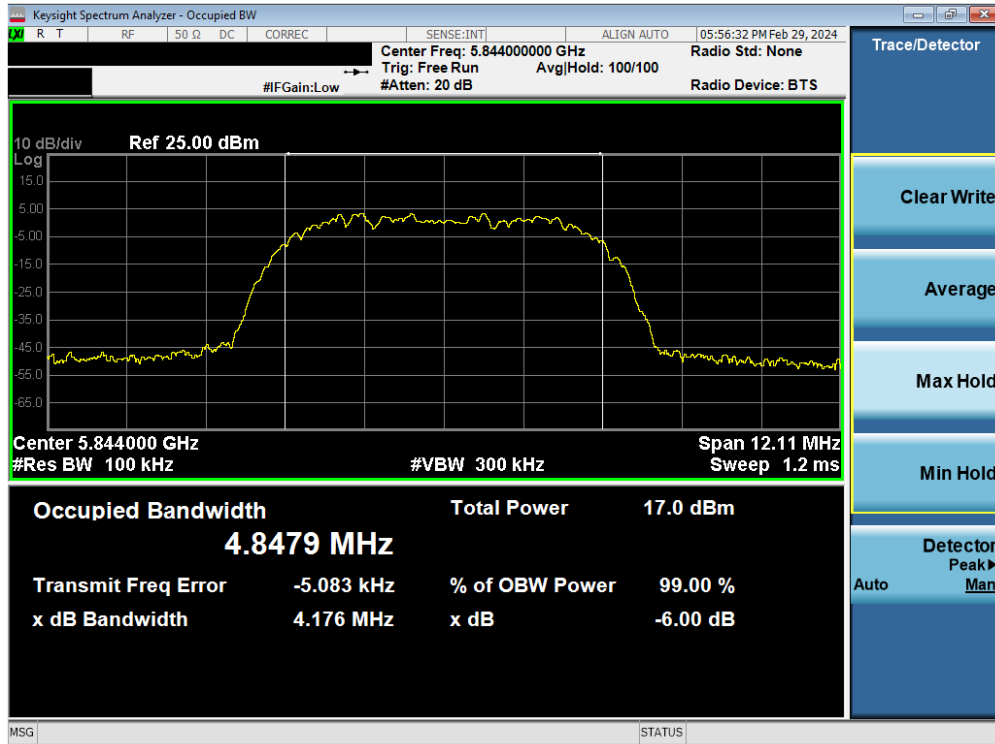
Plot 7-30. 6dB BW & 99% OBW Antenna 3b (HDR8, ePA, 5844MHz)
