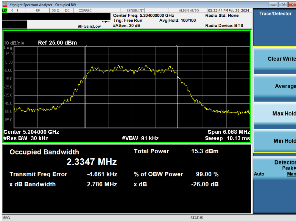
Plot 7-8. 26dB BW & 99% OBW Antenna 3b (HDR4, ePA– 5204MHz)
