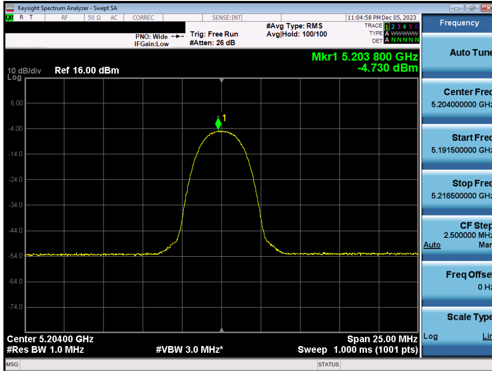
Plot 7-65. PSD Antenna 3b (HDR4, iPA – 5204MHz)
