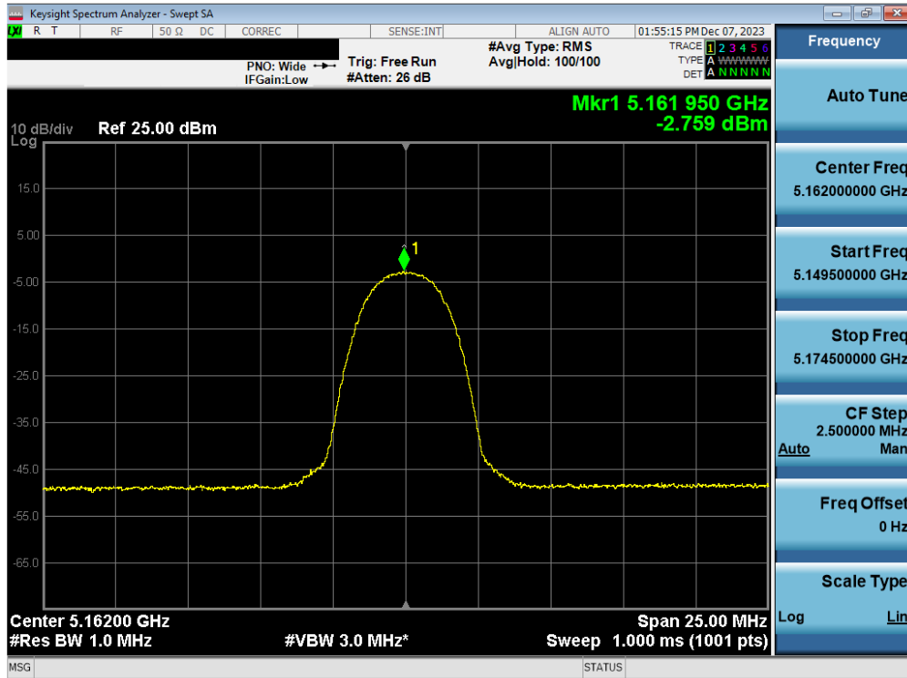
Plot 7-115. FCC/ISED PSD TxBF Antenna 5T (HDR4, iPA – 5162MHz)
