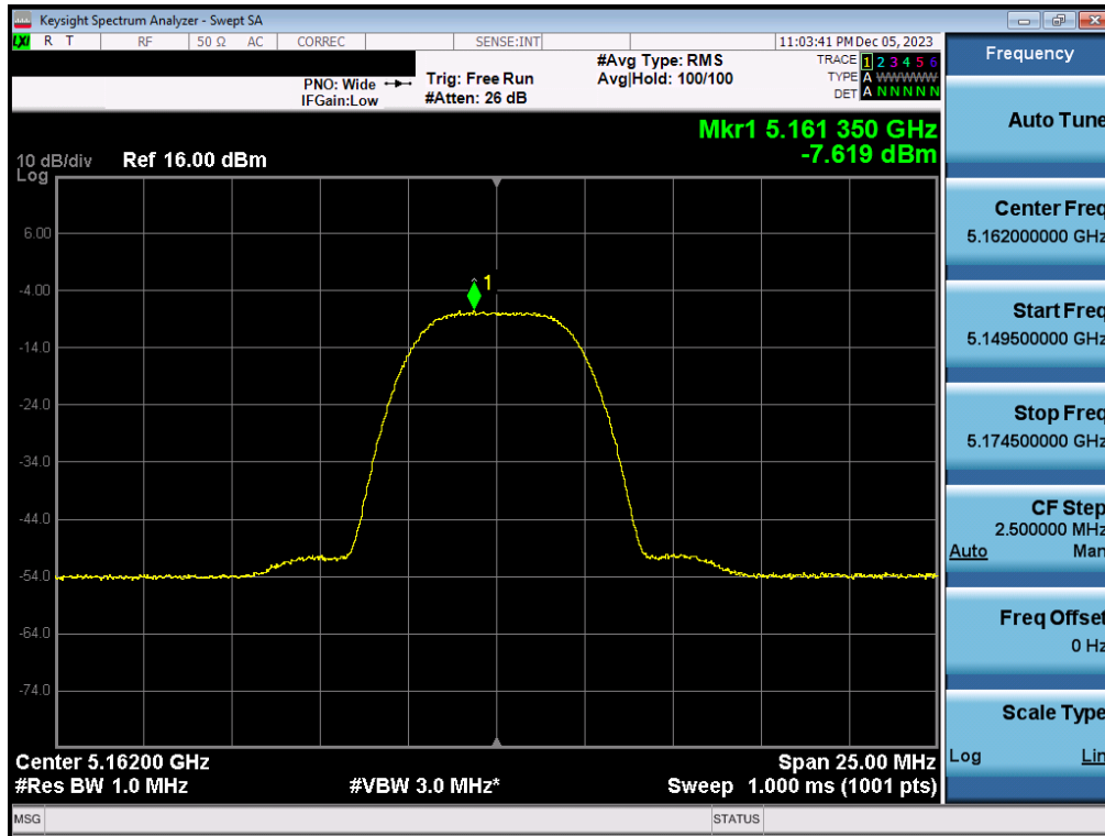
Plot 7-70. PSD Antenna 3b (HDR8, iPA – 5162MHz)
