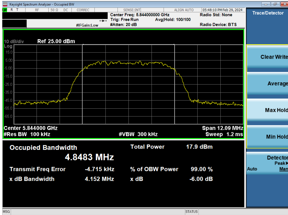
Plot 7-24. 6dB BW & 99% OBW Antenna 5T (HDR8, ePA, 5844MHz)
