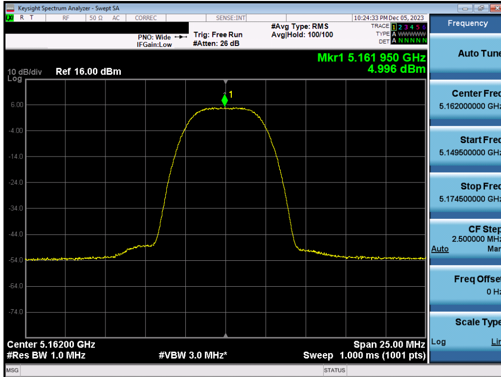
Plot 7-43. Antenna 5T (HDR8, ePA – 5162MHz)
