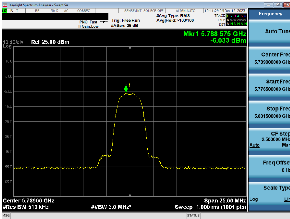
Plot 7-53. PSD Antenna 5T (HDR4, iPA 5789MHz)
