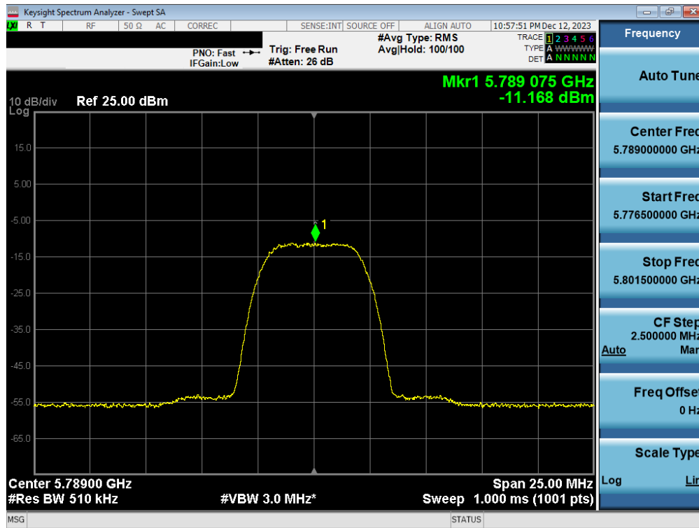
Plot 7-83. PSD Antenna 3b (HDR8, iPA 5789MHz)
