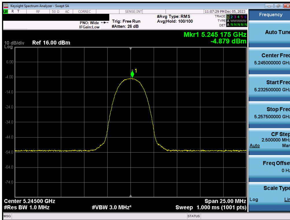
Plot 7-66. PSD Antenna 3b (HDR4, iPA– 5245MHz)
