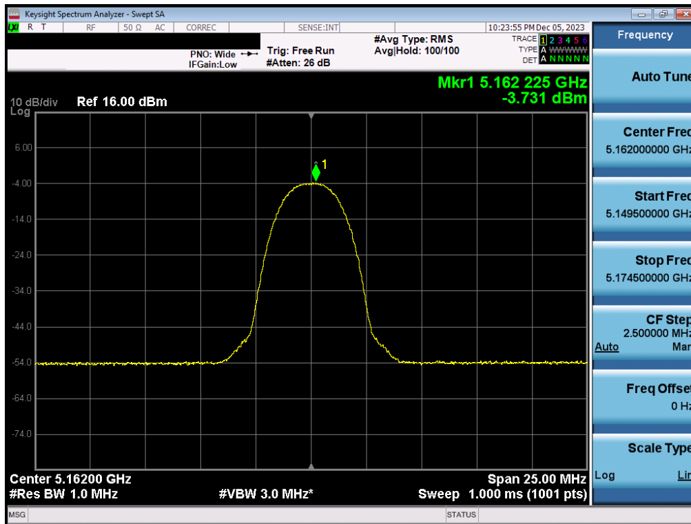
Plot 7-40. PSD Antenna 5T (HDR4, iPA – 5162MHz)
