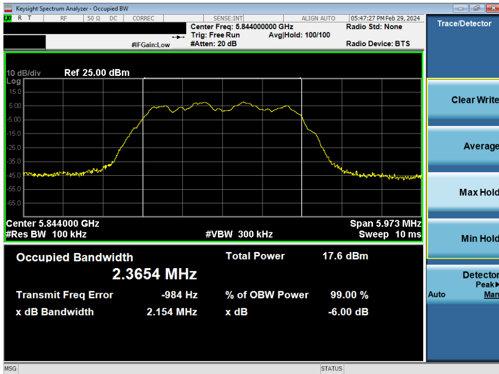
Plot 7-21. 6dB BW & 99% OBW Antenna 5T (HDR4, ePA, 5844MHz)
