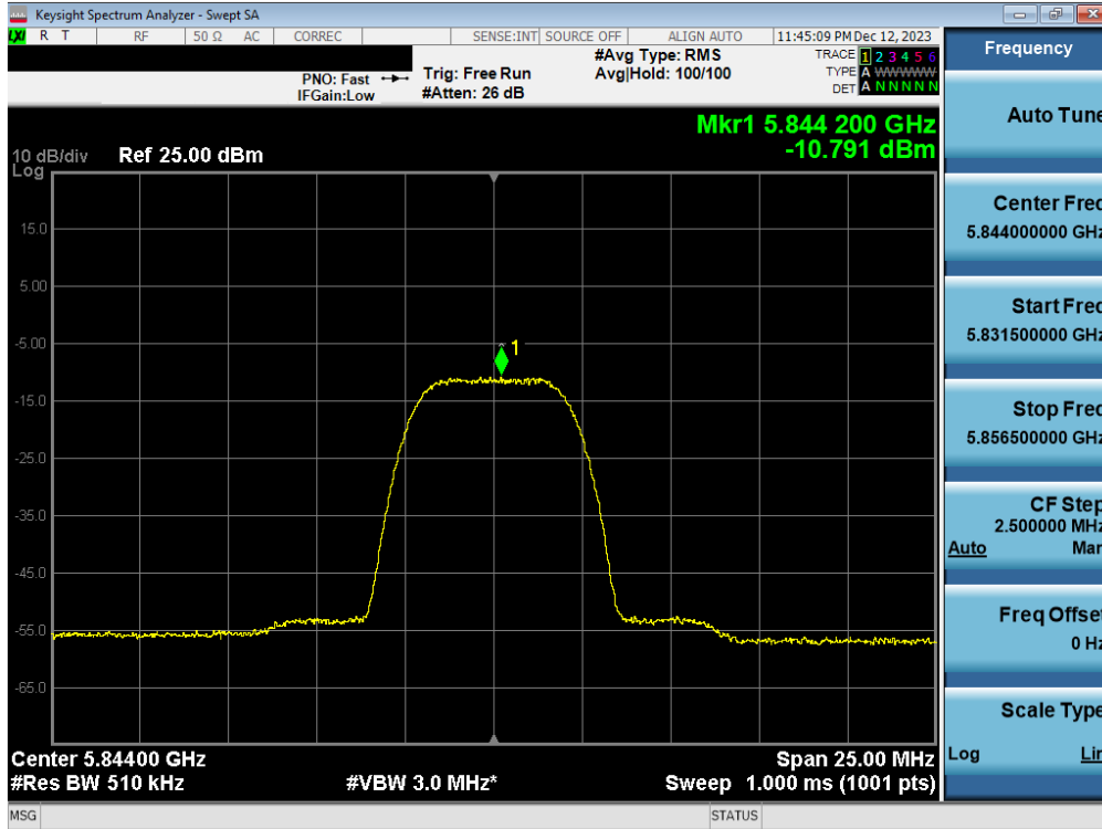
Plot 7-84. PSD Antenna 3b (HDR8, iPA 5844MHz)
