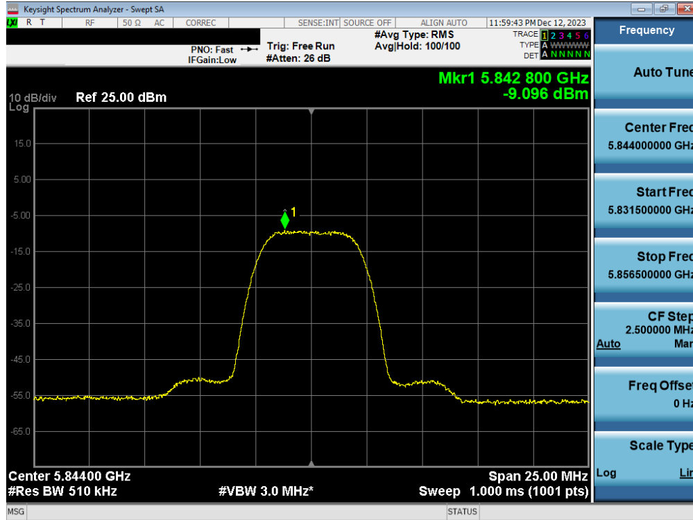
Plot 7-60. PSD Antenna 5T (HDR8, iPA 5844MHz)
