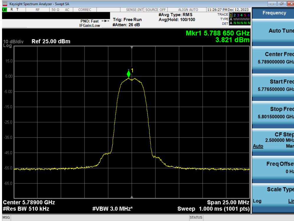
Plot 7-98. PSD Antenna 1b (HDR4, ePA 5789MHz)
