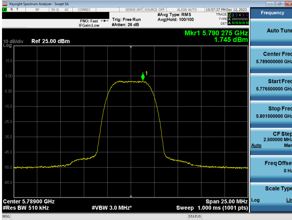
Plot 7-80. PSD Antenna 3b (HDR8, ePA 5789MHz)
