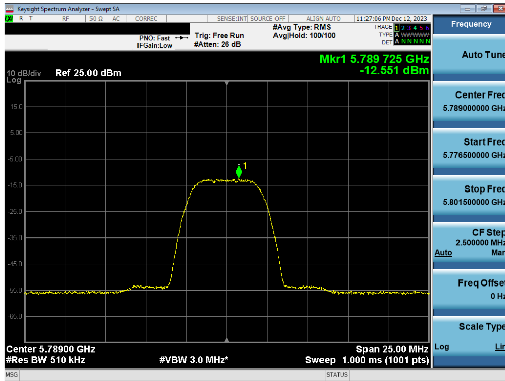
Plot 7-107. PSD Antenna 1b (HDR8, iPA 5789MHz)
