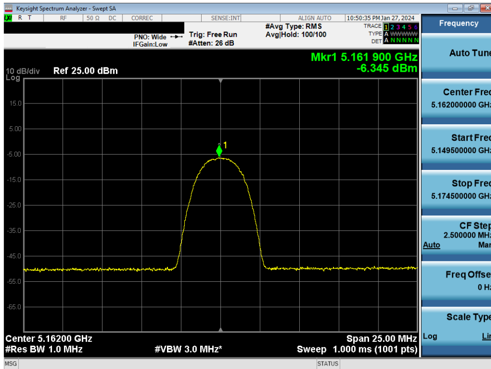
Plot 7-88. PSD Antenna 1b (HDR4, iPA – 5162MHz)
