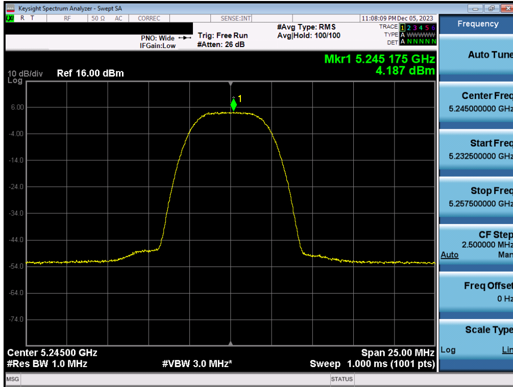
Plot 7-69. PSD Antenna 3b (HDR8, ePA– 5245MHz)
