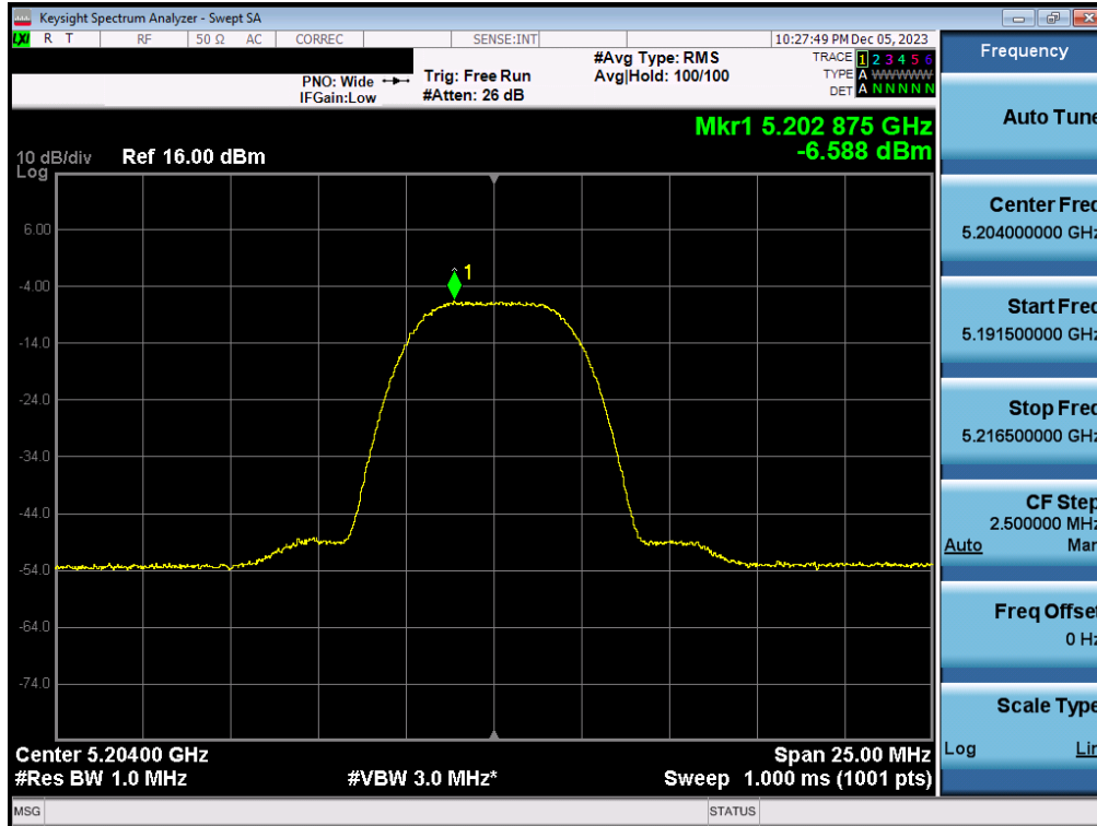
Plot 7-47. PSD Antenna 5T (HDR8, iPA – 5204MHz)
