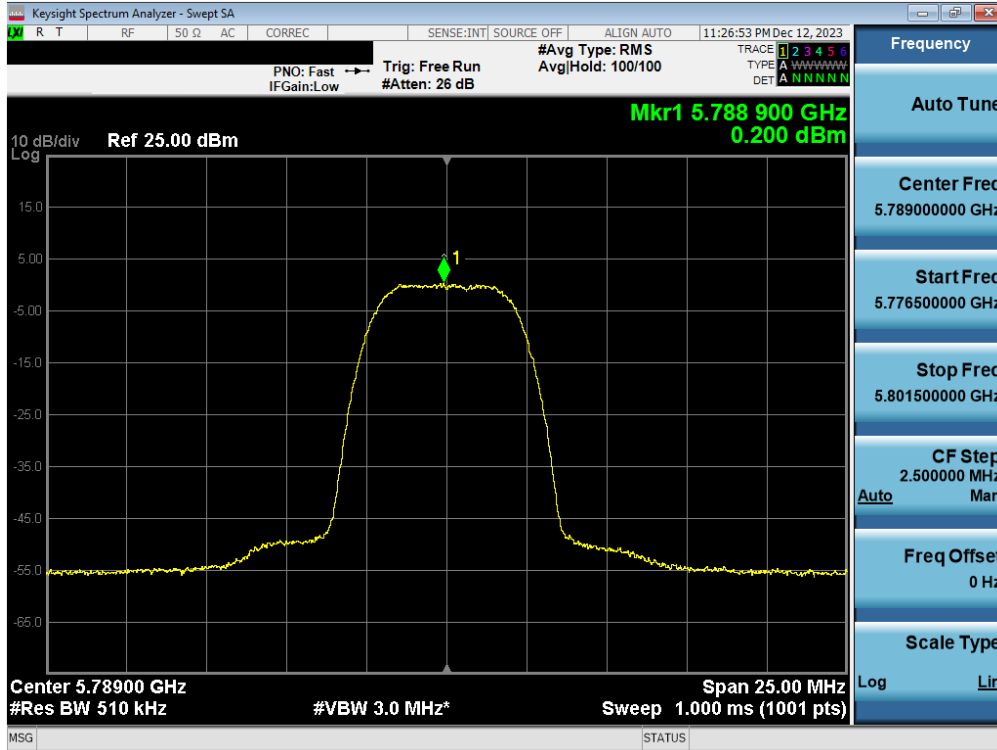
Plot 7-104. PSD Antenna 1b (HDR8, ePA 5789MHz)
