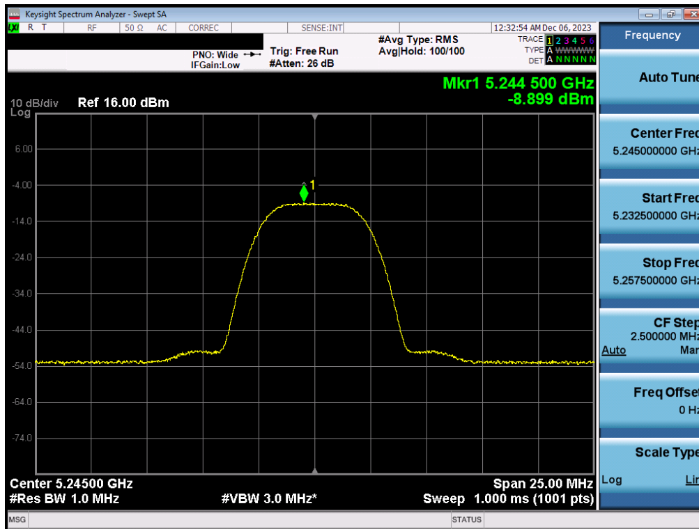
Plot 7-96. PSD Antenna 1b (HDR8, iPA– 5245MHz)
