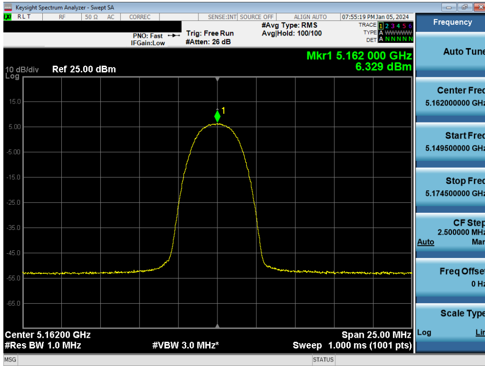
Plot 7-109. FCC PSD TxBF Antenna 5T (HDR4, ePA - 5162MHz)
