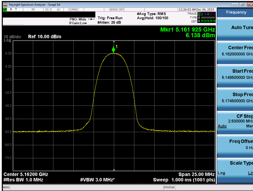
Plot 7-85. PSD Antenna 1b (HDR4, ePA – 5162MHz)
