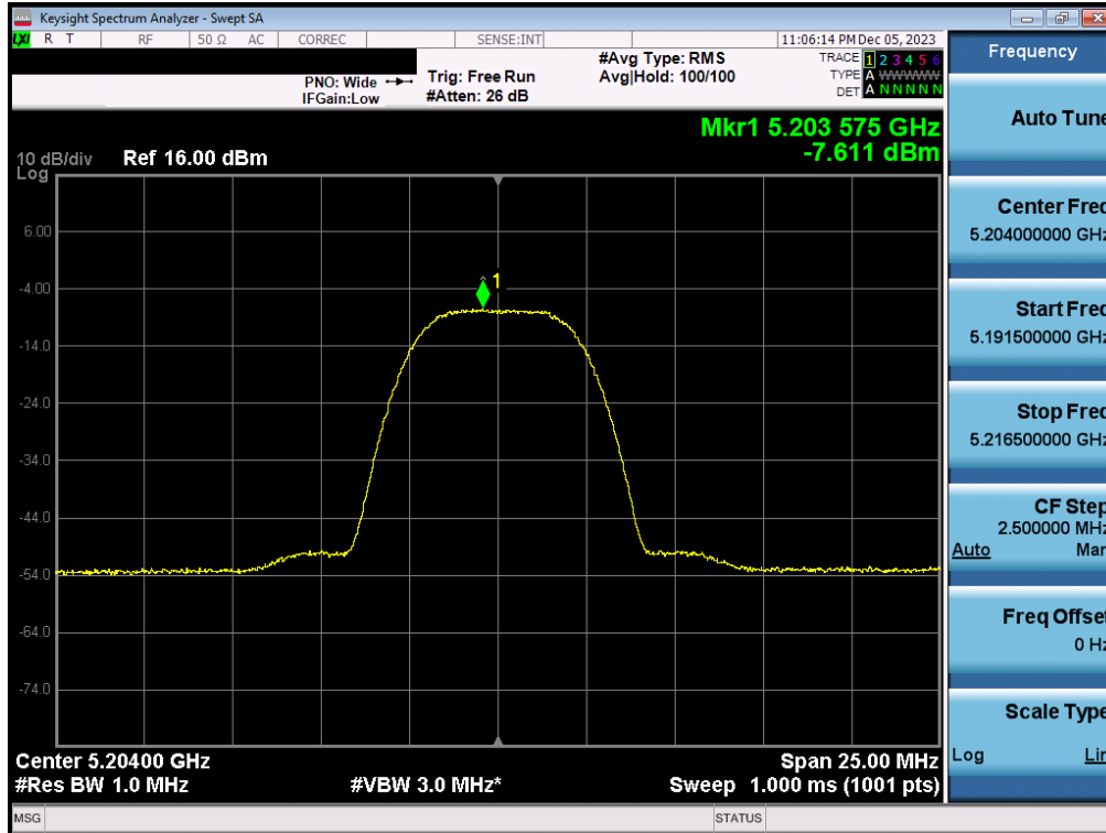
Plot 7-71. PSD Antenna 3b (HDR8, iPA – 5204MHz)
