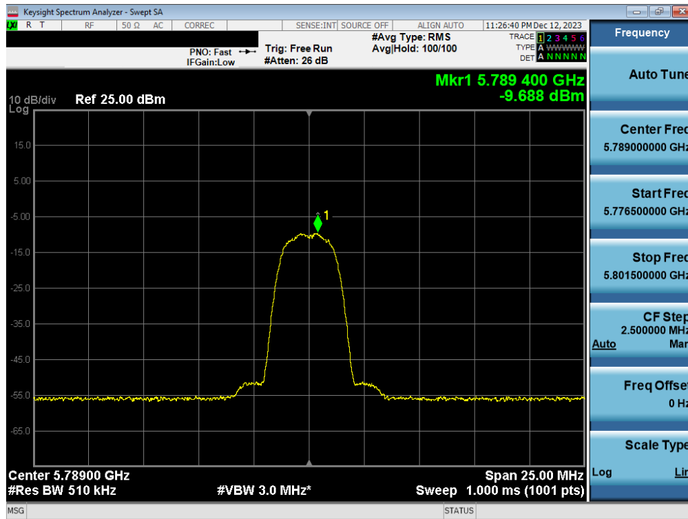
Plot 7-101. PSD Antenna 1b (HDR4, iPA 5789MHz)
