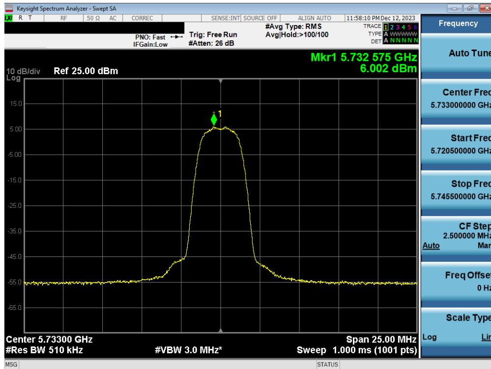
Plot 7-49. PSD Antenna 5T (HDR4, ePA 5733MHz)
