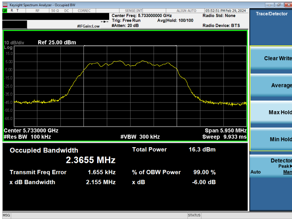
Plot 7-25. 6dB BW & 99% OBW Antenna 3b (HDR4, ePA, 5733MHz)
