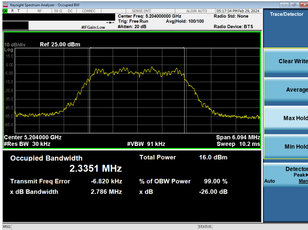
Plot 7-2. 26dB BW & 99% OBW Antenna 5T (HDR4, ePA– 5204MHz)
