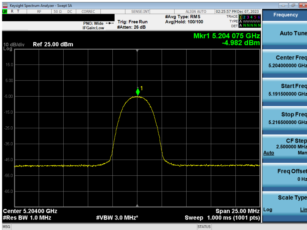
Plot 7-118. FCC/ISED PSD TxBF Antenna 3b (HDR4, iPA – 5204MHz)
