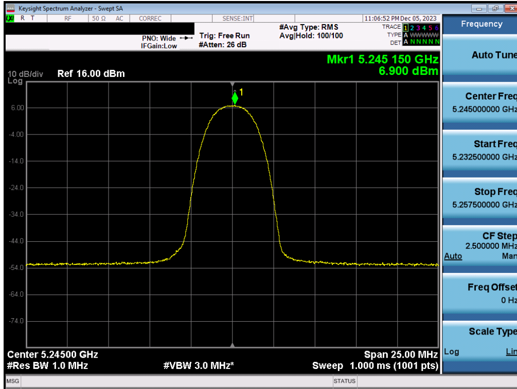
Plot 7-63. PSD Antenna 3b (HDR4, ePA – 5245MHz)
