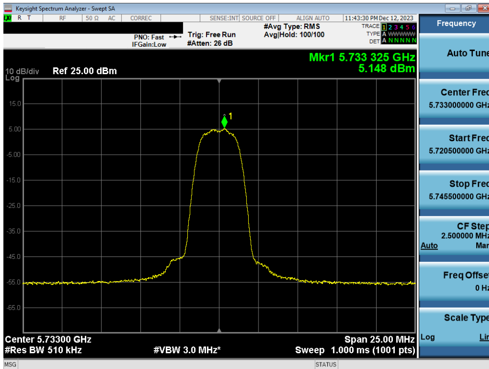
Plot 7-73. PSD Antenna 3b (HDR4, ePA 5733MHz)
