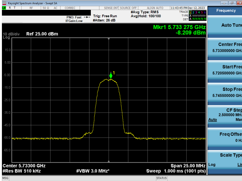
Plot 7-76. PSD Antenna 3b (HDR4, iPA 5733MHz)
