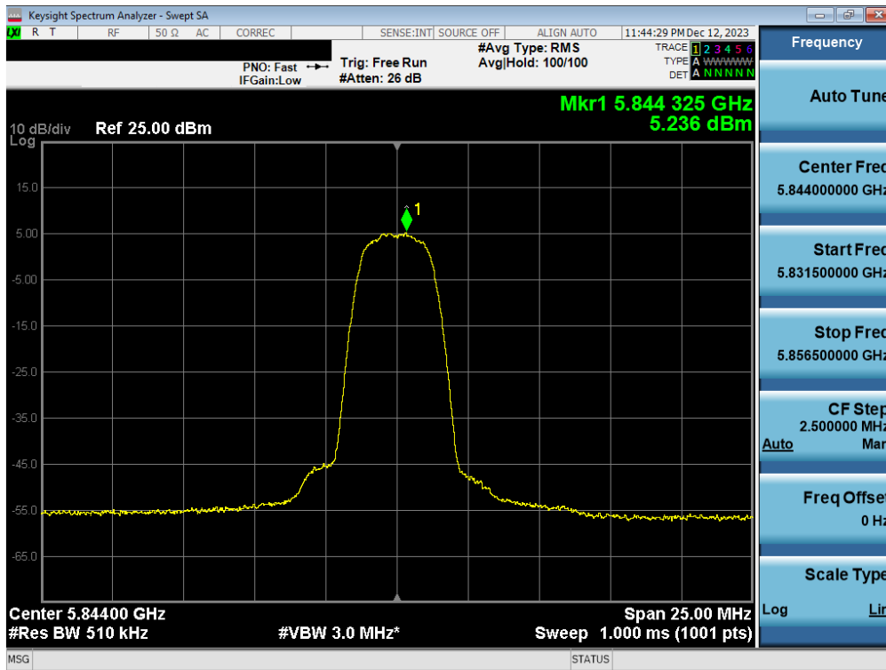
Plot 7-75. PSD Antenna 3b (HDR4, ePA 5844MHz)
