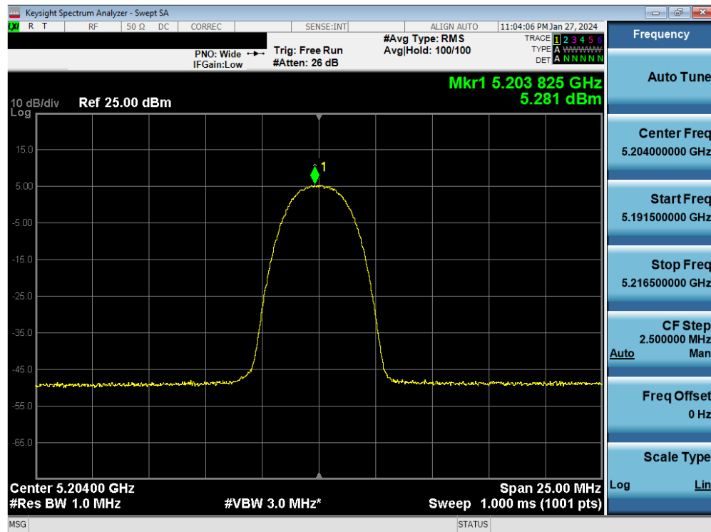
Plot 7-112. FCC PSD TxBF Antenna 3b (HDR4, ePA - 5204MHz)
