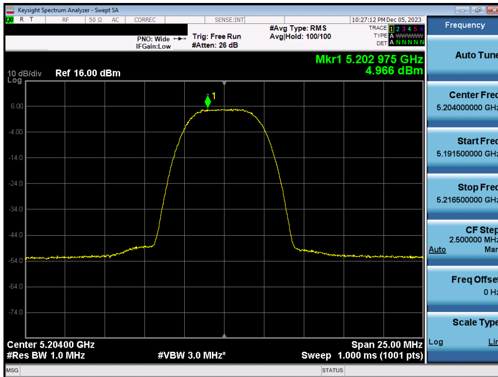
Plot 7-44. PSD Antenna 5T (HDR8, ePA – 5204MHz)
