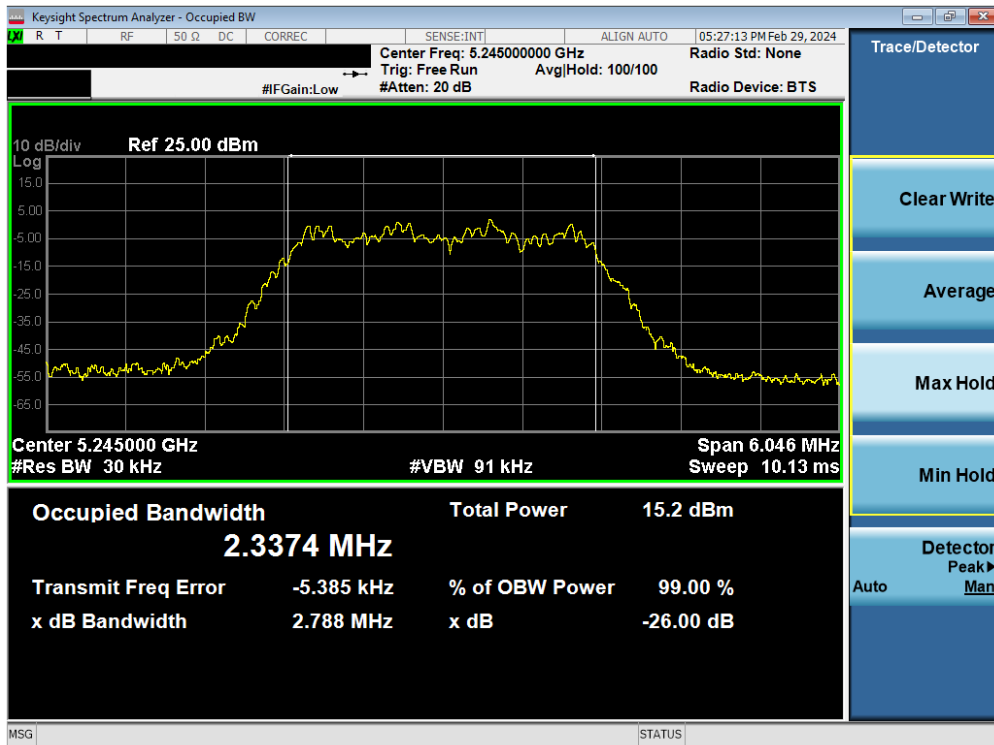
Plot 7-9. 26dB BW & 99% OBW Antenna 3b (HDR4, ePA– 5245MHz)
