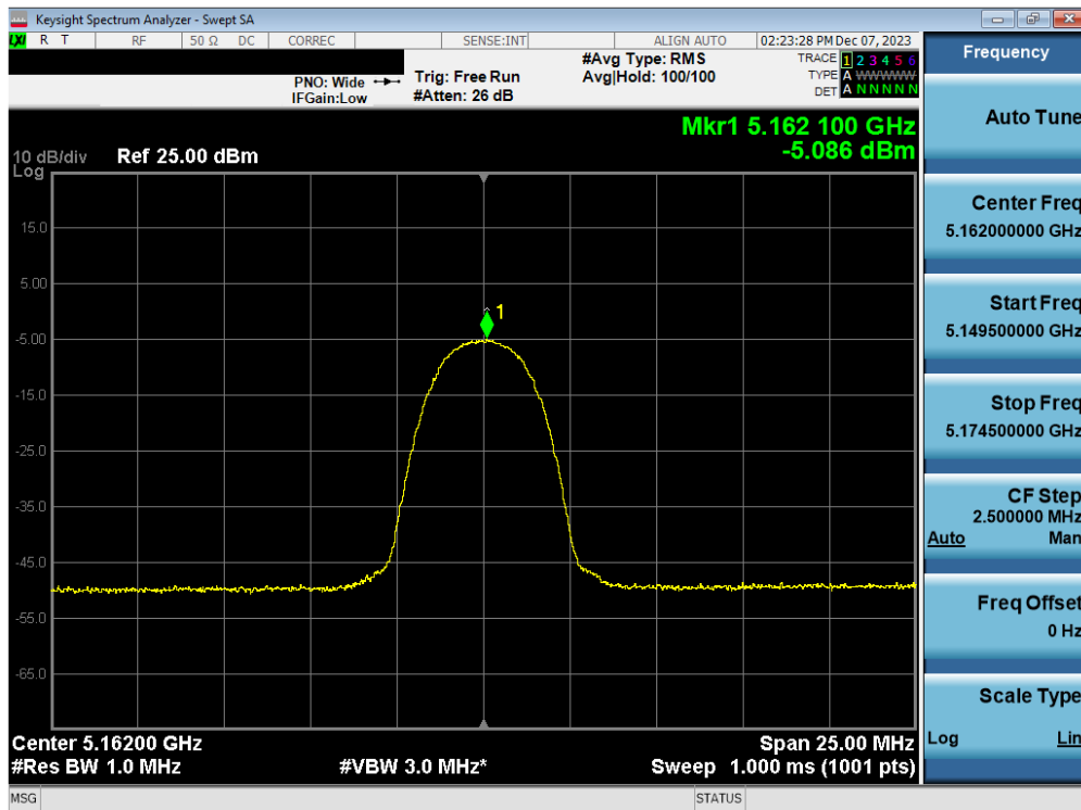
Plot 7-116. FCC/ISED PSD TxBF Antenna 3b (HDR4, iPA – 5162MHz)
