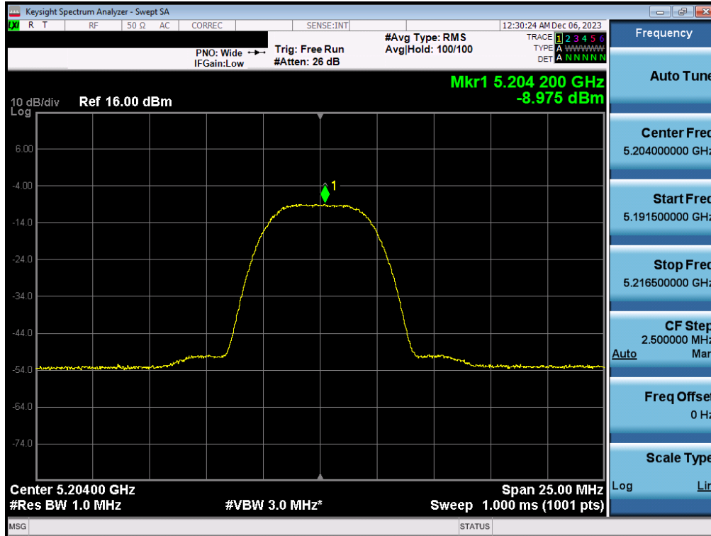
Plot 7-95. PSD Antenna 1b (HDR8, iPA – 5204MHz)
