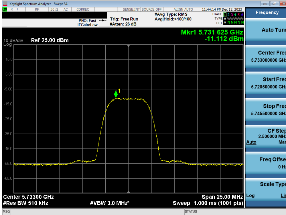
Plot 7-82. PSD Antenna 3b (HDR8, iPA 5733MHz)
