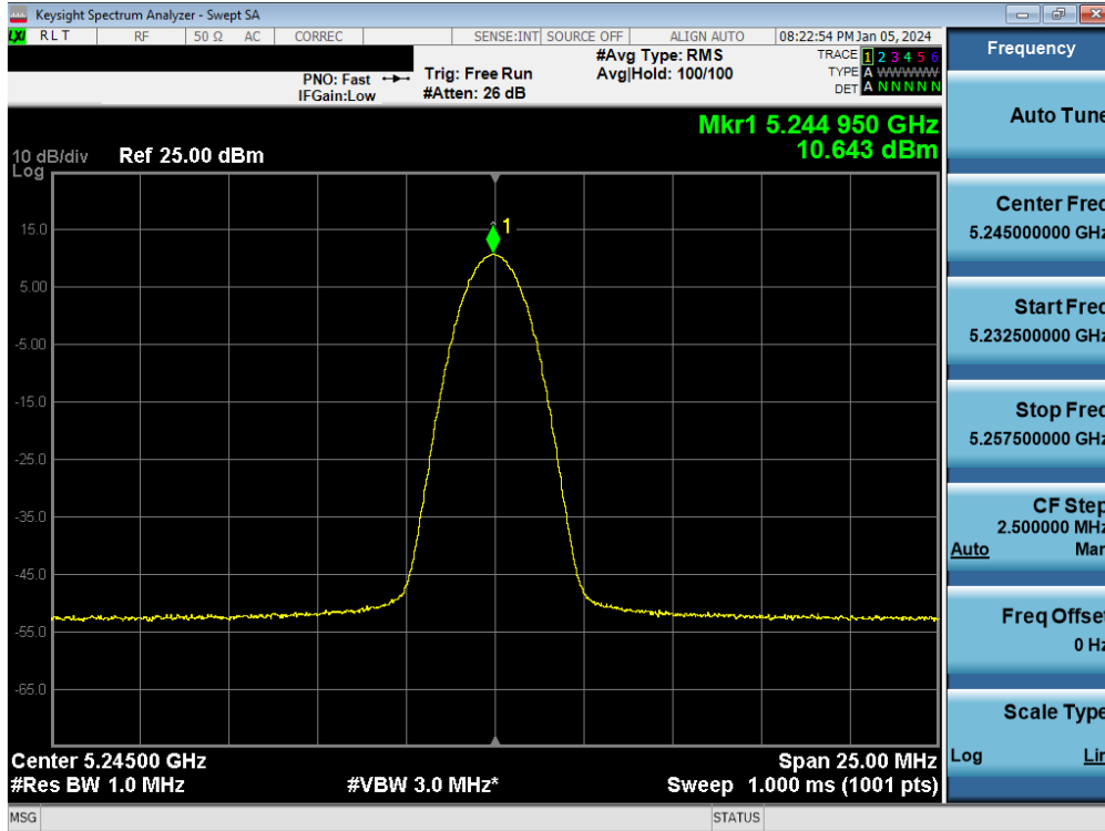
Plot 7-48. FCC/ISED PSD Antenna 1b (BDR, ePA- 5245MHz)
