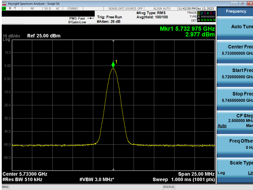
Plot 7-43. PSD Antenna 3b (BDR, iPA 5733MHz)
