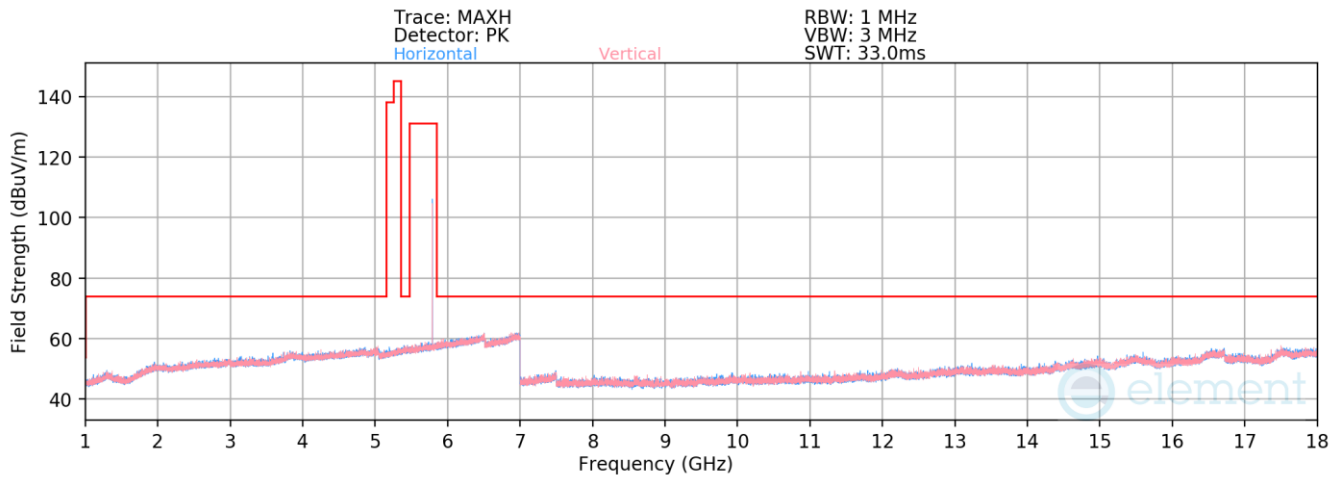
Plot 7-101. Radiated Spurious Emissions 1-18GHz Antenna 3b (BDR GFSK ePA – 5789MHz)
