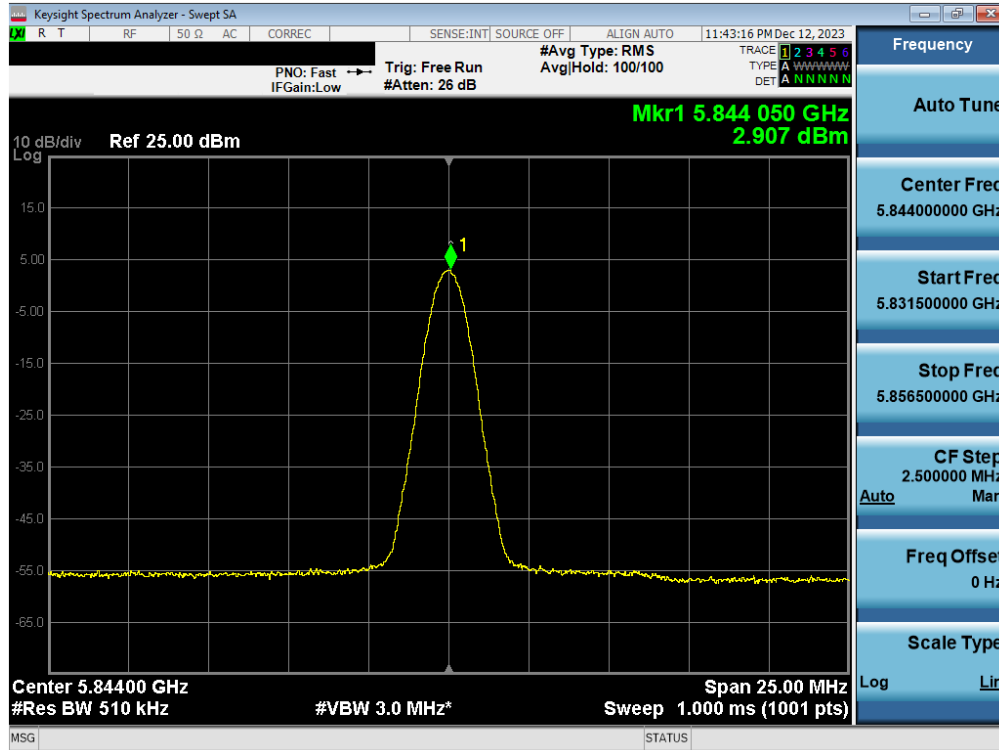
Plot 7-45. PSD Antenna 3b (BDR, iPA 5844MHz)
