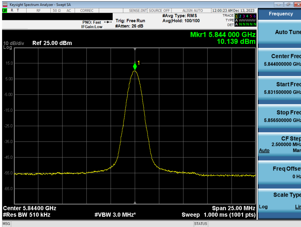
Plot 7-83. PSD TxBF Antenna 5T (BDR, ePA 5844MHz)
