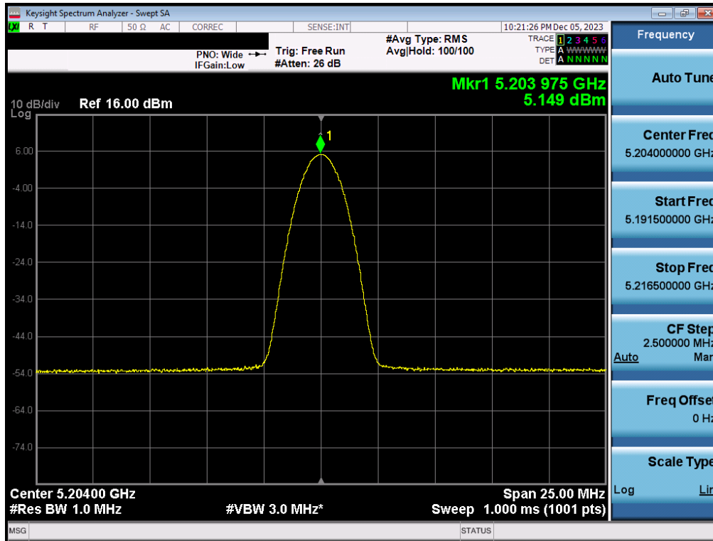
Plot 7-23. FCC/ISED PSD Antenna 5T (BDR, iPA – 5204MHz)
