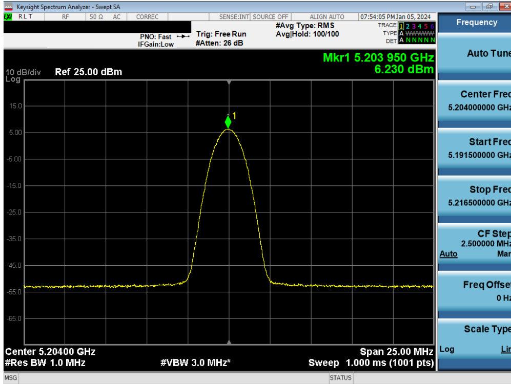
Plot 7-60. FCC PSD TxBF Antenna 5T (BDR, ePA – 5204MHz)
