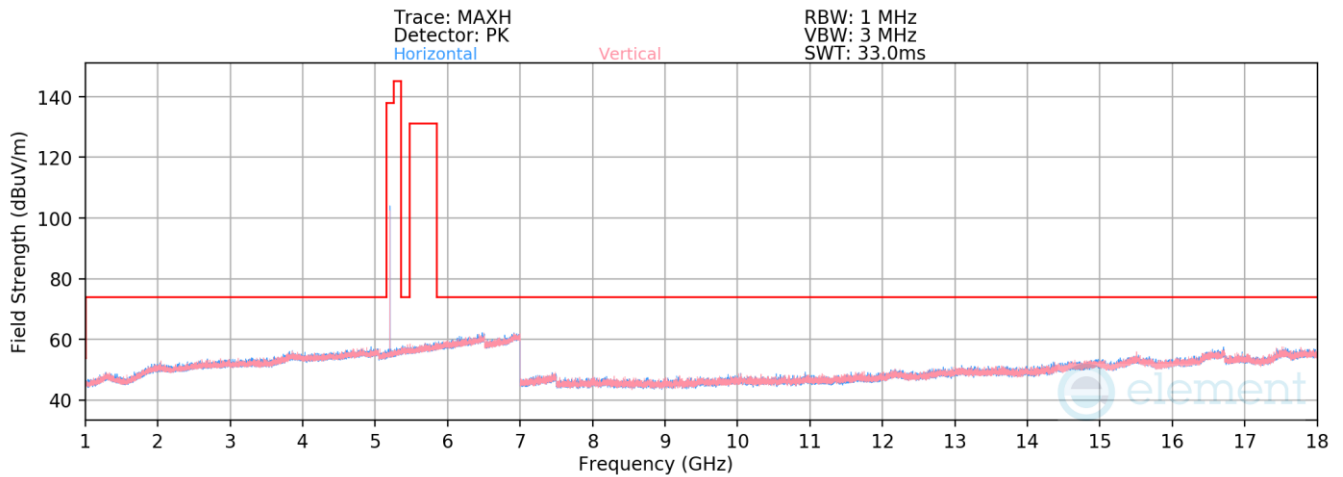
Plot 7-98. Radiated Spurious Emissions 1-18GHz Antenna 3b (BDR GFSK ePA – 5204MHz)
