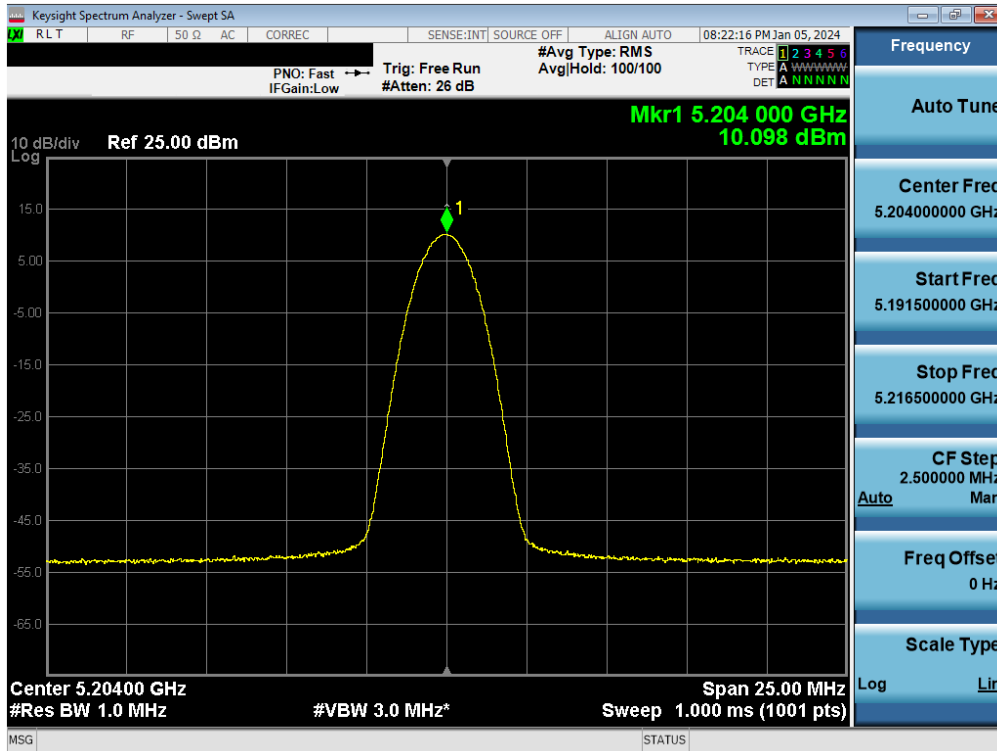
Plot 7-47. FCC/ISED PSD Antenna 1b (BDR, ePA – 5204MHz)
