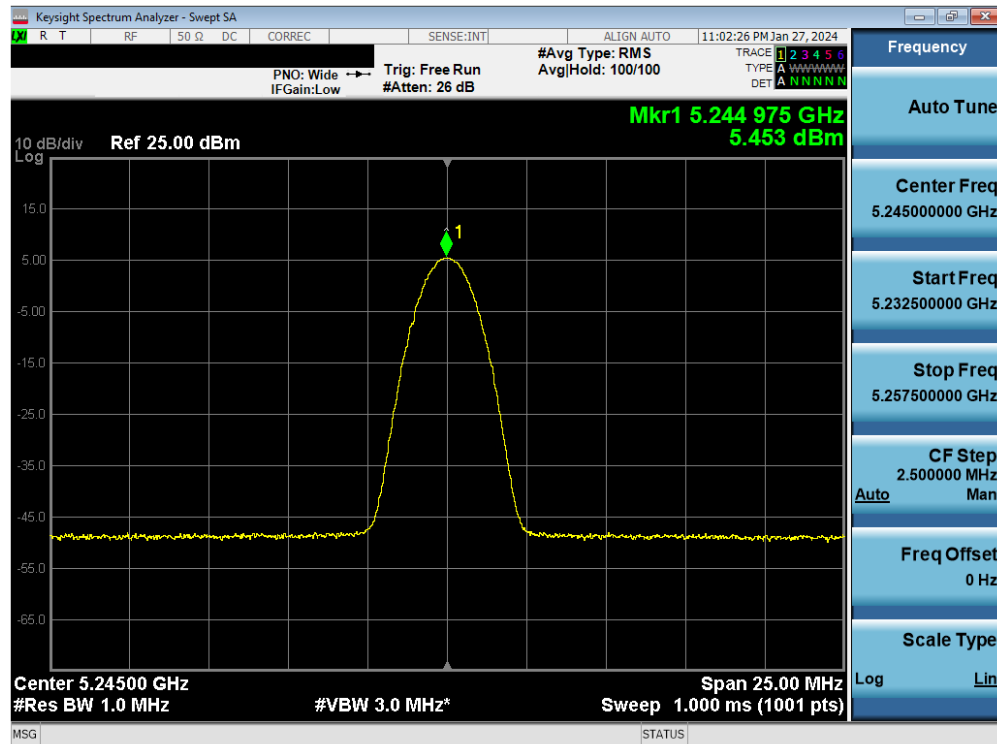
Plot 7-63. FCC PSD TxBF Antenna 3b (BDR, ePA- 5245MHz)
