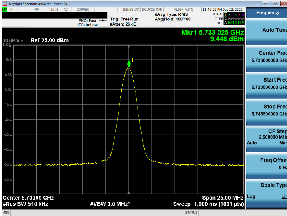
Plot 7-80. PSD TxBF Antenna 3b (BDR, ePA 5733MHz)
