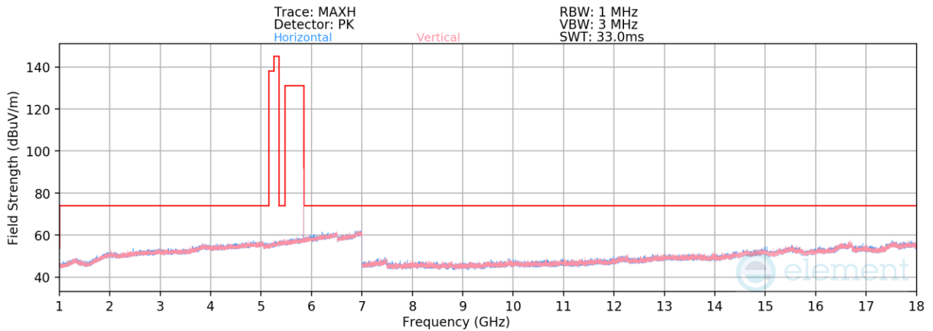
Plot 7-96. Radiated Spurious Emissions 1-18GHz Antenna 5T (BDR GFSK ePA– 5844MHz)
