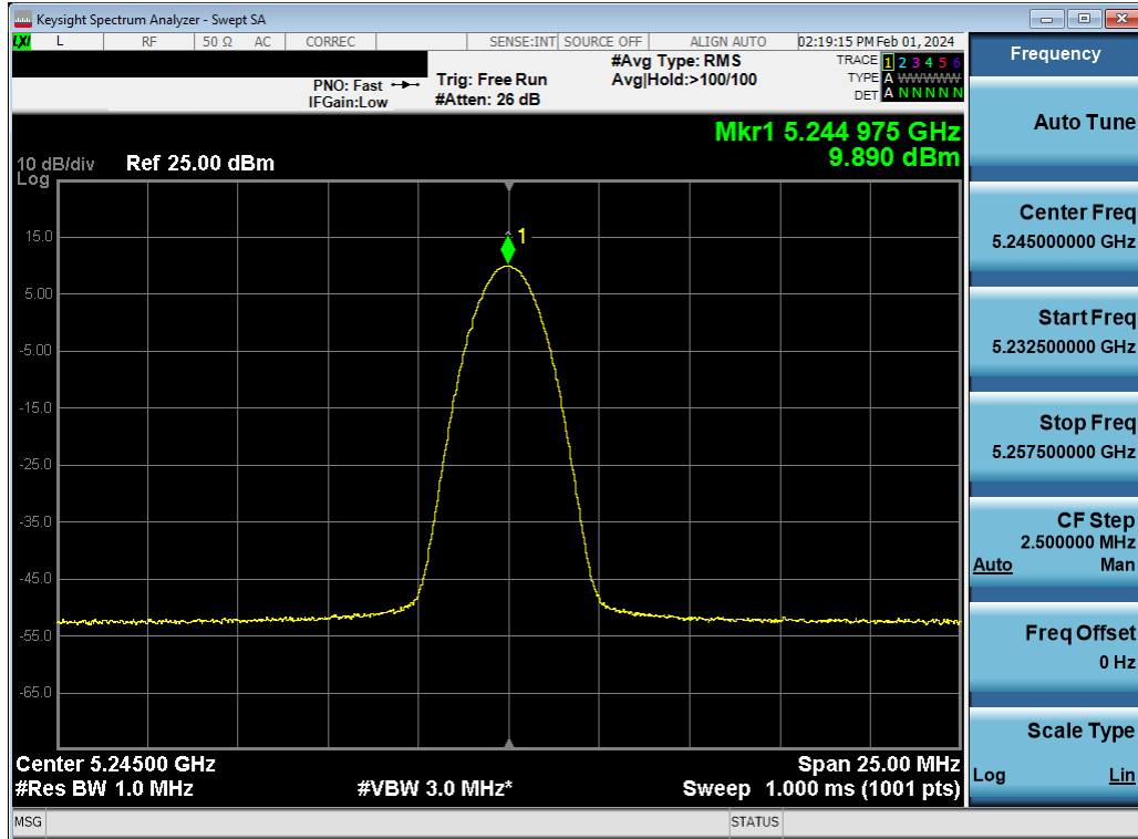
Plot 7-27. ISED PSD Antenna 5T (BDR, ePA- 5245MHz)
