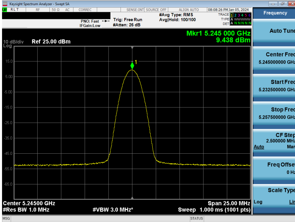
Plot 7-36. FCC/ISED PSD Antenna 3b (BDR, ePA– 5245MHz)
