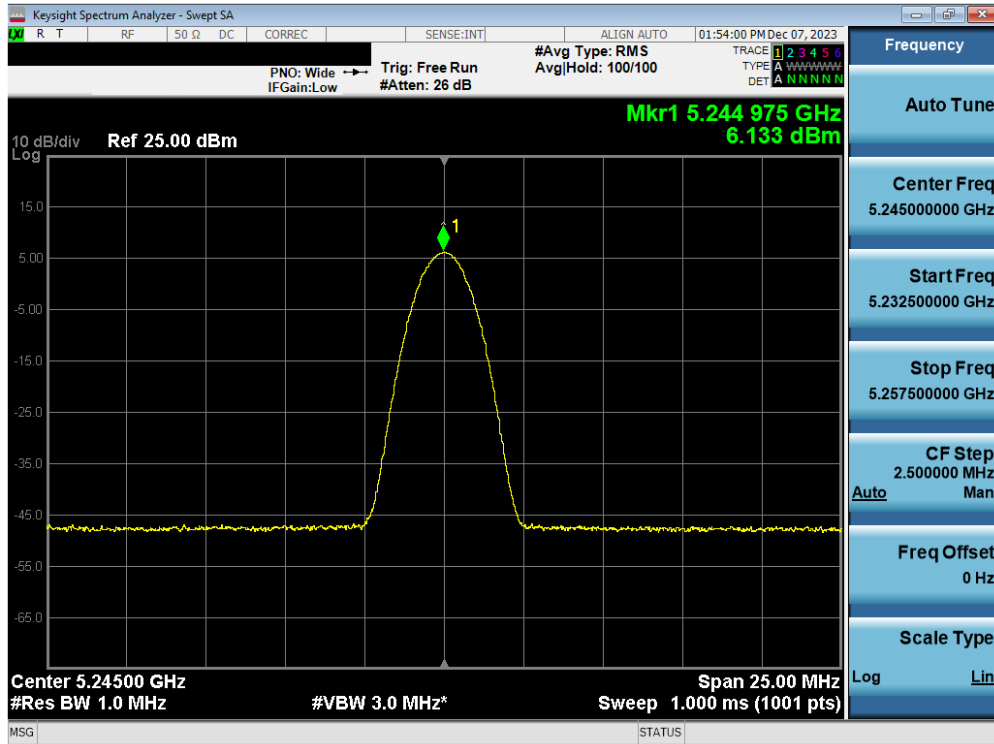
Plot 7-68. FCC PSD TxBF Antenna 5T (BDR, iPA- 5245MHz)
