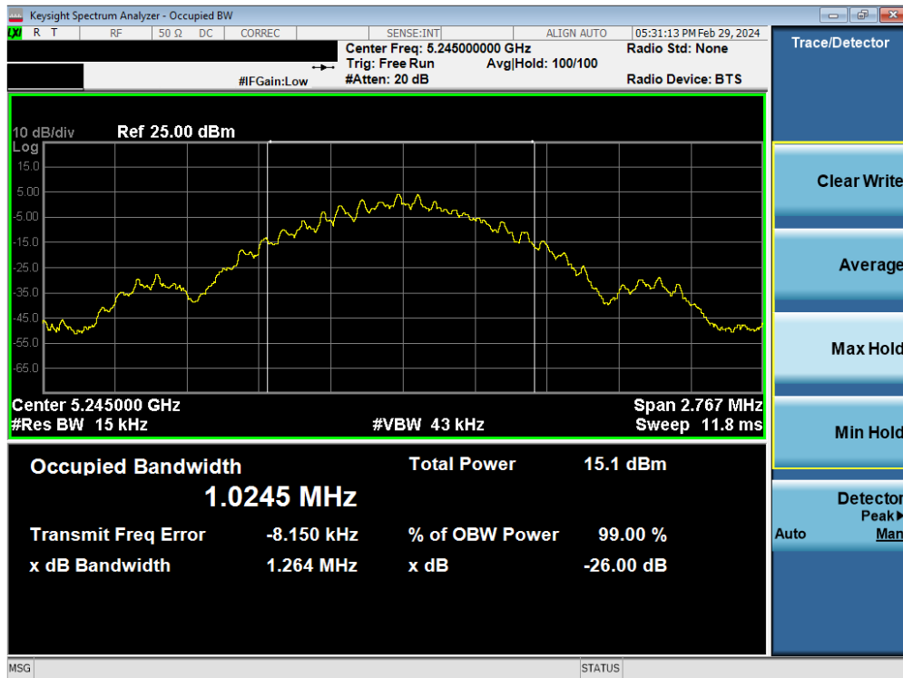
Plot 7-9. 26dB BW & 99% OBW Antenna 1b (BDR GFSK, ePA - 5245MHz)
