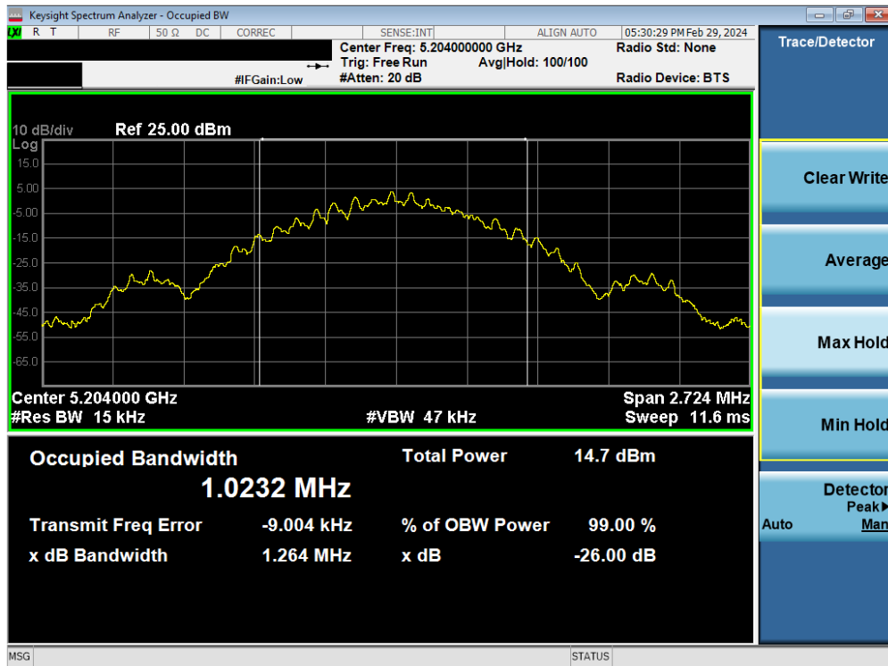
Plot 7-8. 26dB BW & 99% OBW Antenna 1b (BDR GFSK, ePA- 5204MHz)
