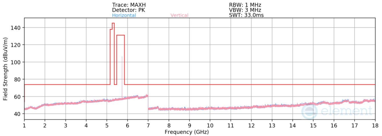
Plot 7-100. Radiated Spurious Emissions 1-18GHz Antenna 3b (BDR GFSK ePA – 5733MHz)
