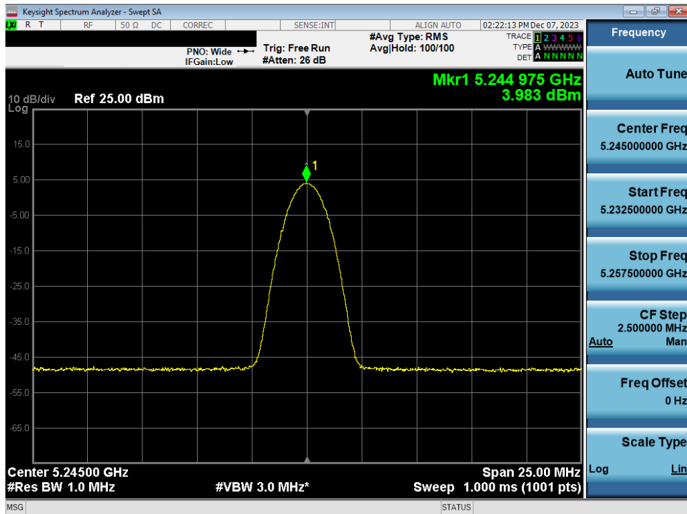
Plot 7-69. FCC/ISED PSD TxBF Antenna 3b (BDR, iPA- 5245MHz)
