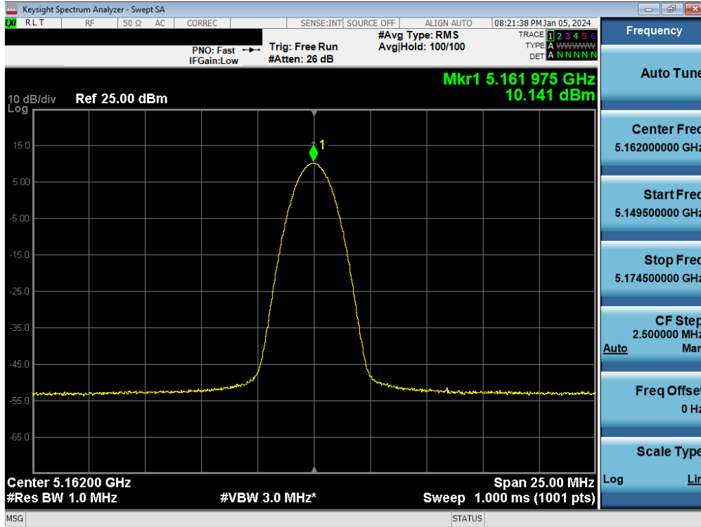
Plot 7-46. FCC/ISED PSD Antenna 1b (BDR, ePA – 5162MHz)
