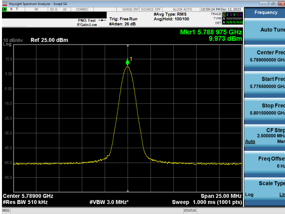
Plot 7-82. PSD TxBF Antenna 3b (BDR, ePA 5789MHz)
