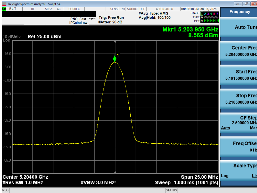
Plot 7-35. FCC/ISED PSD Antenna 3b (BDR, ePA – 5204MHz)
