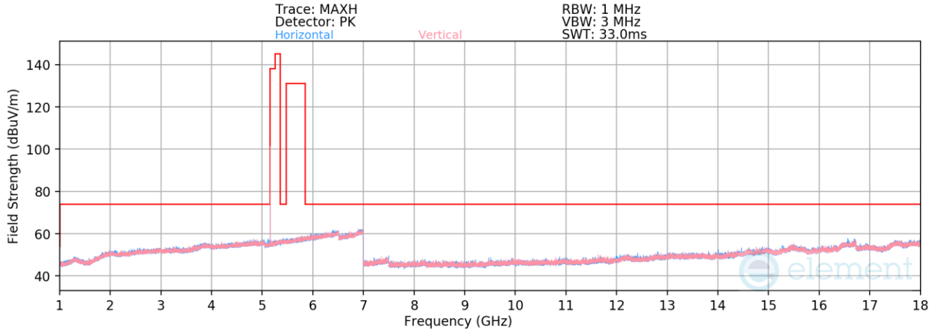
Plot 7-97. Radiated Spurious Emissions 1-18GHz Antenna 3b (BDR GFSK ePA – 5162MHz)
