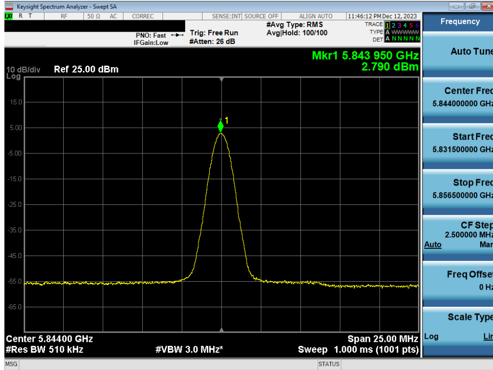
Plot 7-90. PSD TxBF Antenna 3b (BDR, iPA 5844MHz)
