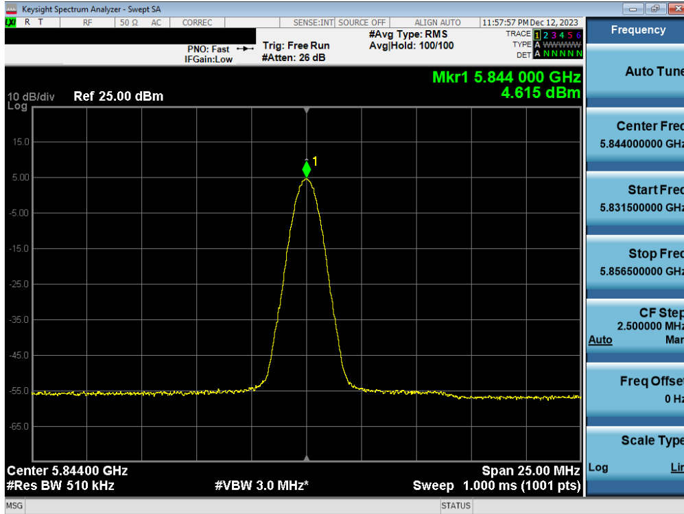
Plot 7-33. PSD Antenna 5T (BDR, iPA 5844MHz)
