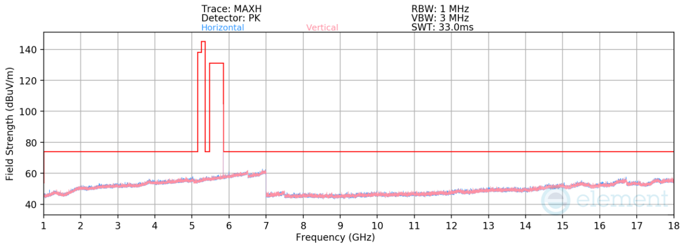
Plot 7-102. Radiated Spurious Emissions 1-18GHz Antenna 3b (BDR GFSK ePA – 5844MHz)
