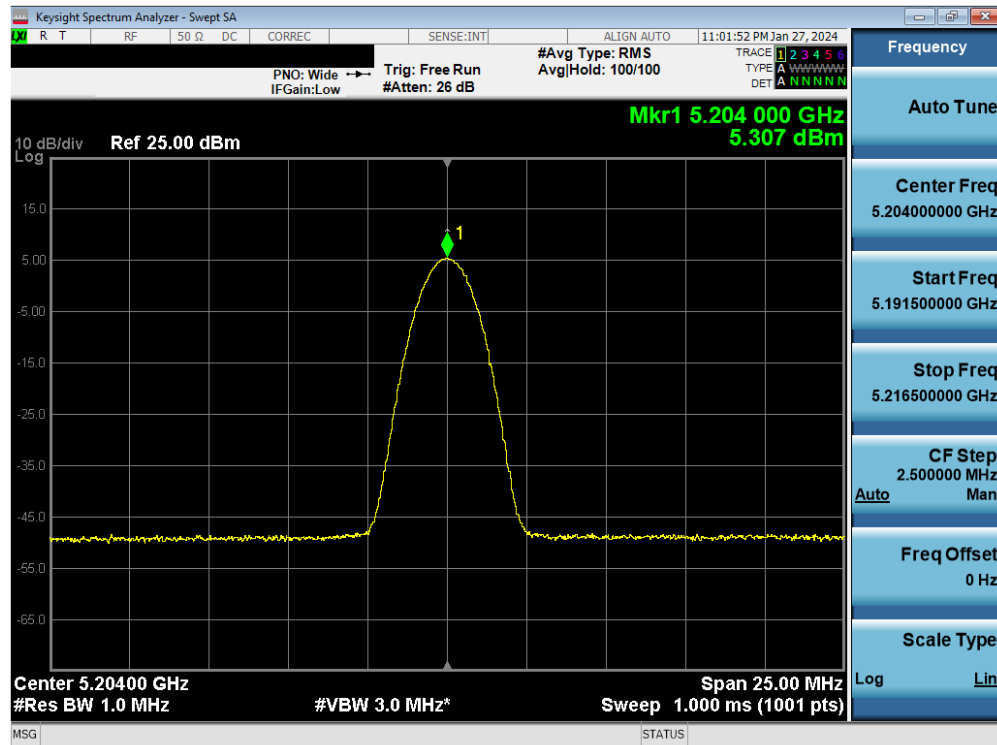
Plot 7-61. FCC PSD TxBF Antenna 3b (BDR, ePA – 5204MHz)
