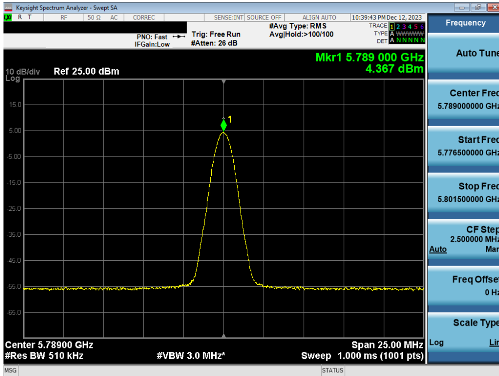
Plot 7-32. PSD Antenna 5T (BDR, iPA 5789MHz)
