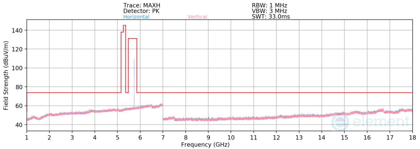
Plot 7-94. Radiated Spurious Emissions 1-18GHz Antenna 5T (BDR GFSK ePA – 5733MHz)
