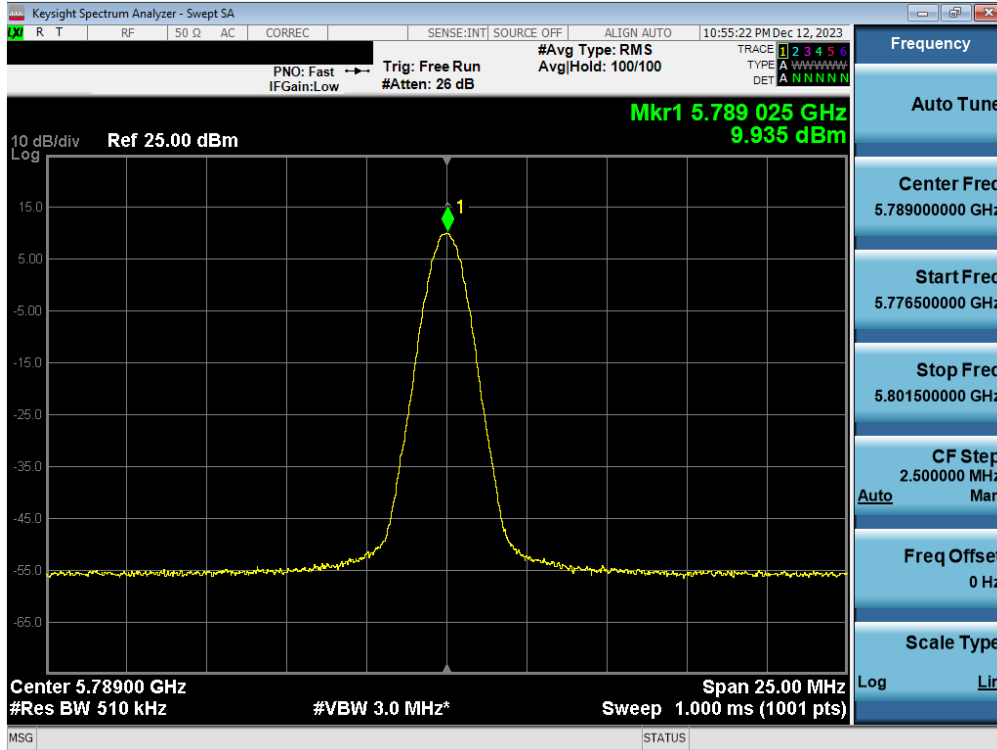
Plot 7-41. PSD Antenna 3b (BDR, ePA 5789MHz)
