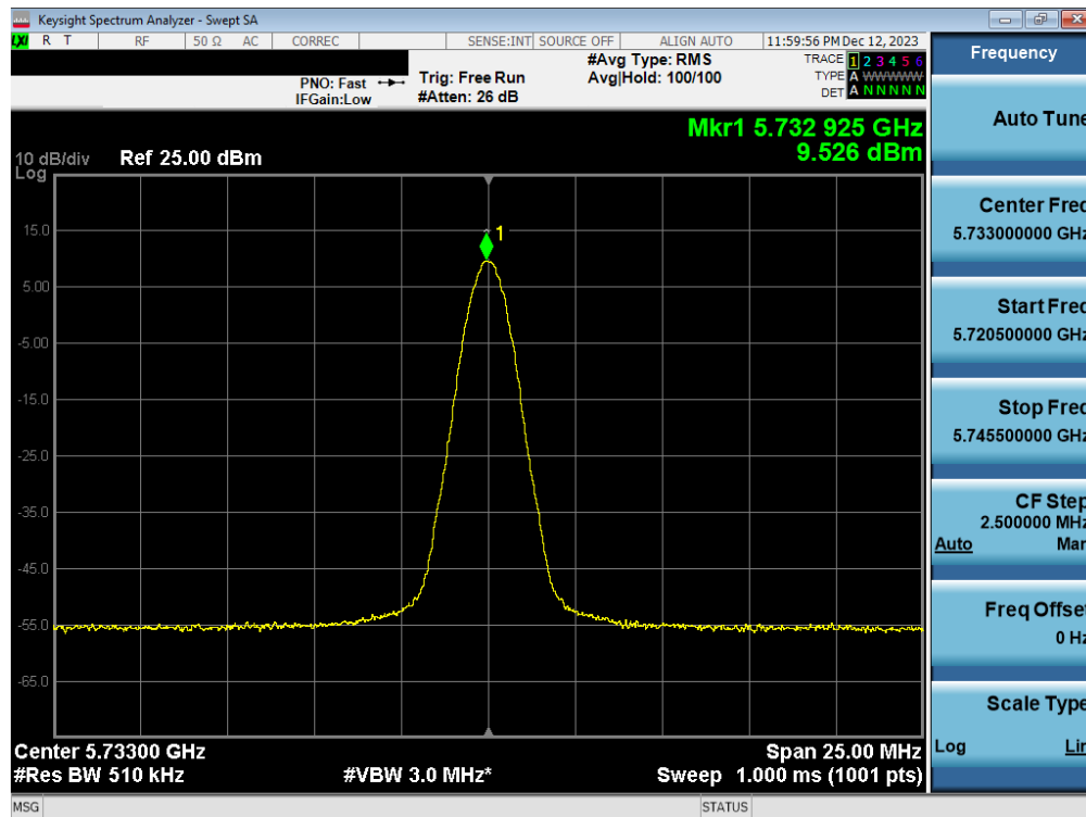
Plot 7-79. PSD TxBF Antenna 5T (BDR, ePA 5733MHz)
