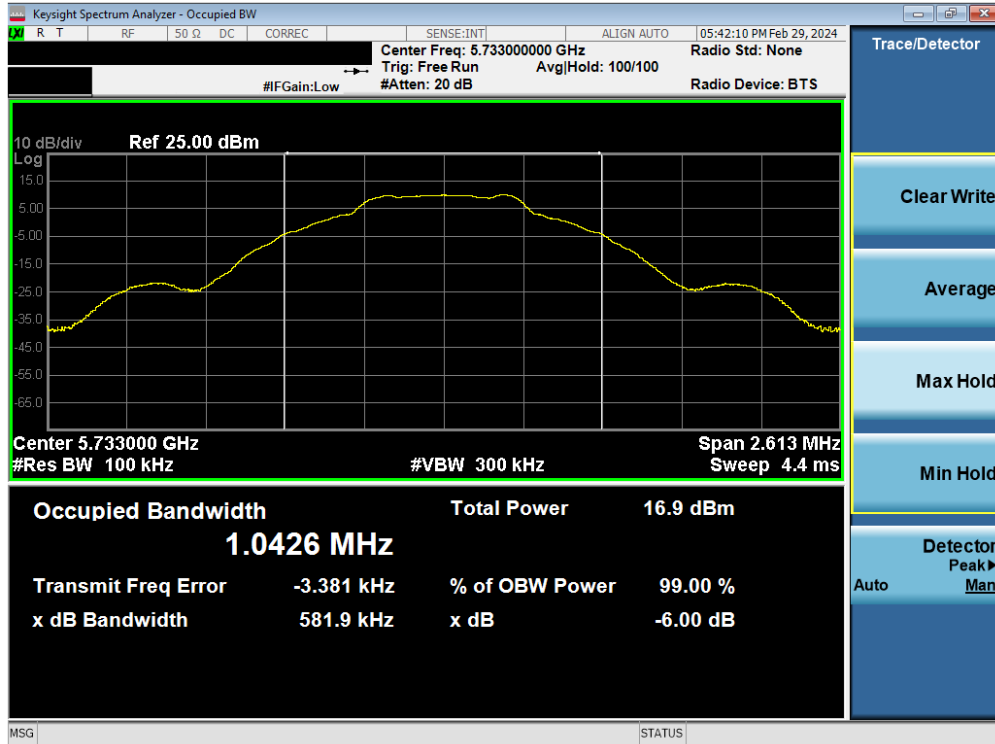
Plot 7-10. 6dB BW & 99% OBW Antenna 5T (BDR GFSK, 5733MHz)
