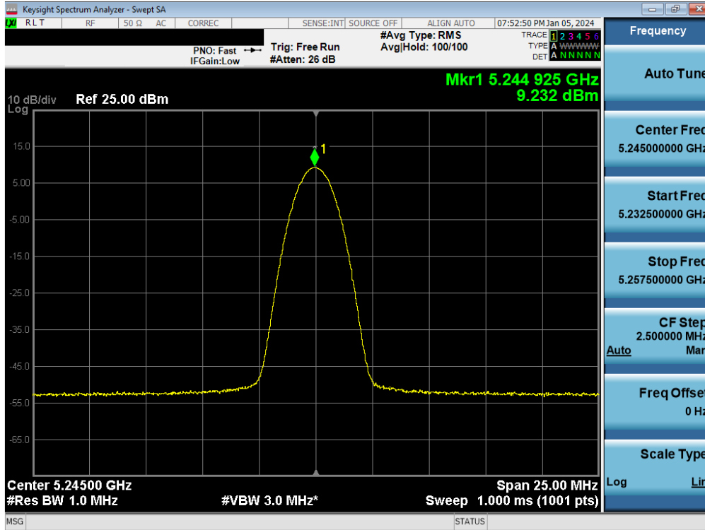
Plot 7-21. FCC PSD Antenna 5T (BDR, ePA- 5245MHz)
