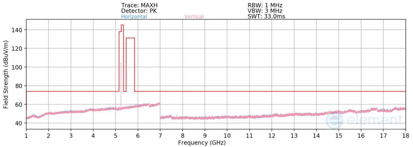
Plot 7-99. Radiated Spurious Emissions 1-18GHz Antenna 3b (BDR GFSK ePA – 5245MHz)
