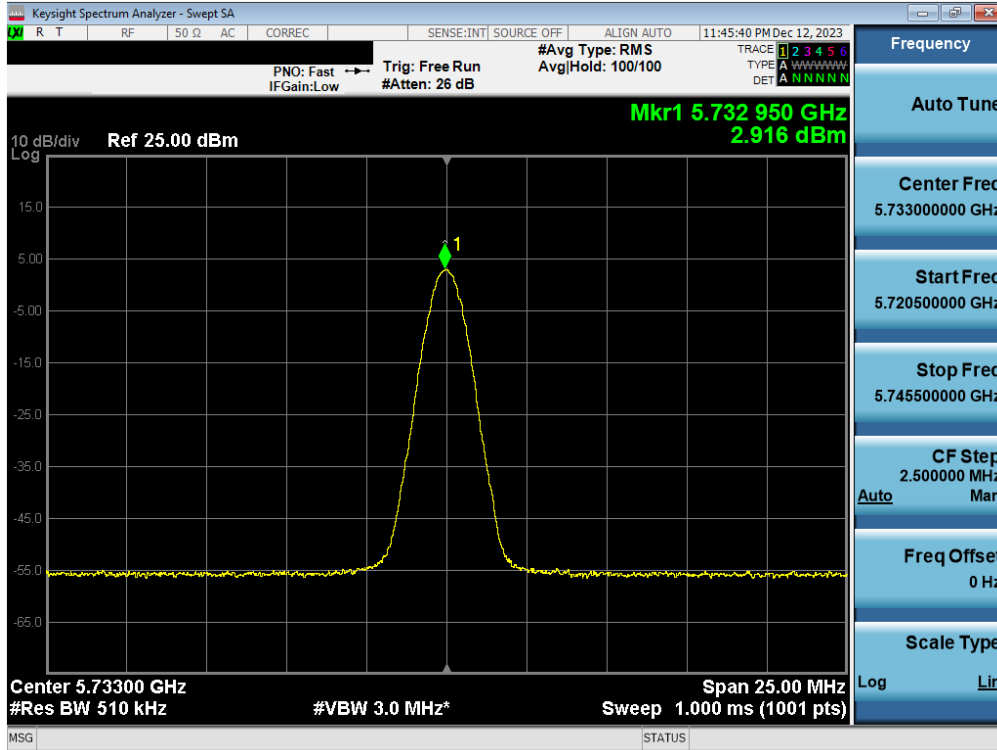
Plot 7-86. PSD TxBF Antenna 3b (BDR, iPA 5733MHz)
