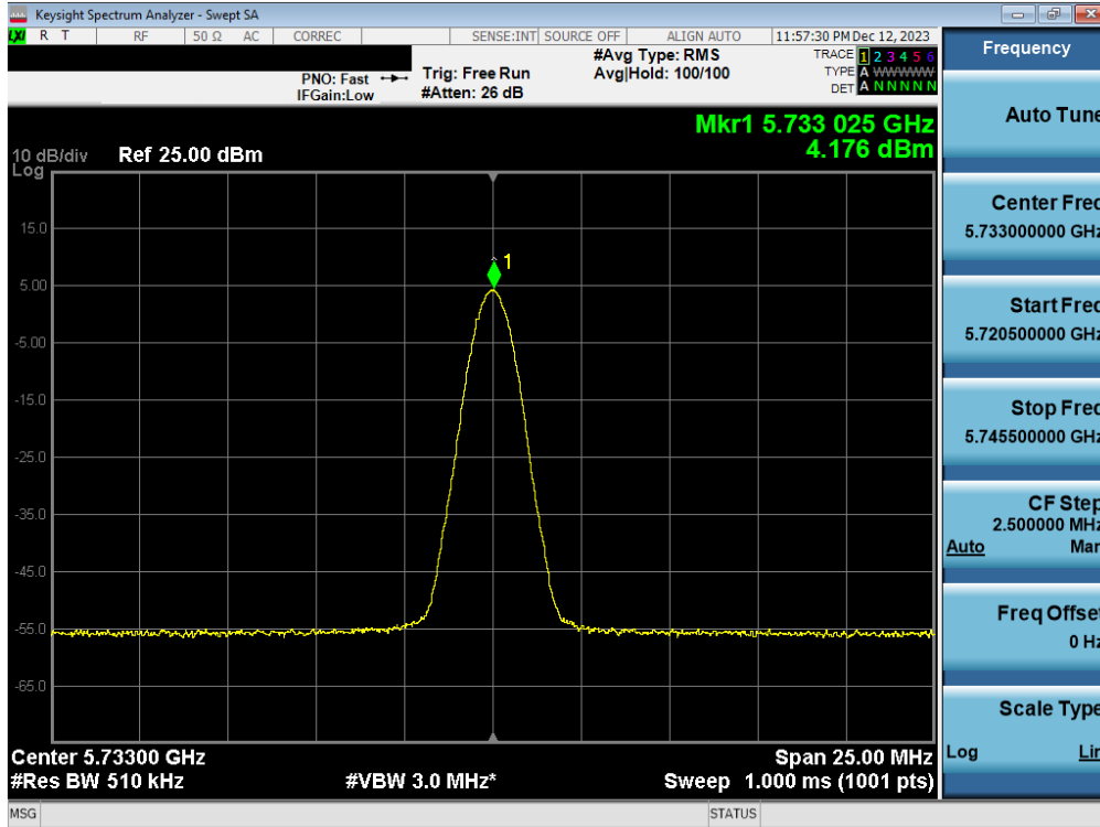
Plot 7-31. PSD Antenna 5T (BDR, iPA 5733MHz)
