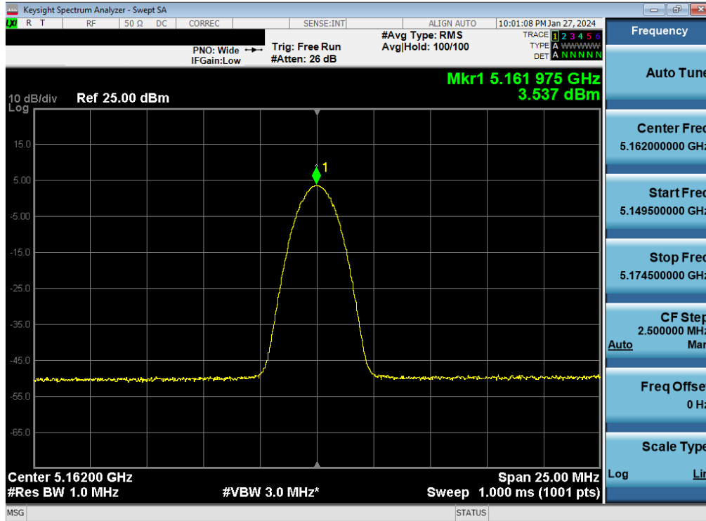
Plot 7-70. ISED PSD TxBF Antenna 5T (BDR, ePA – 5162MHz)
