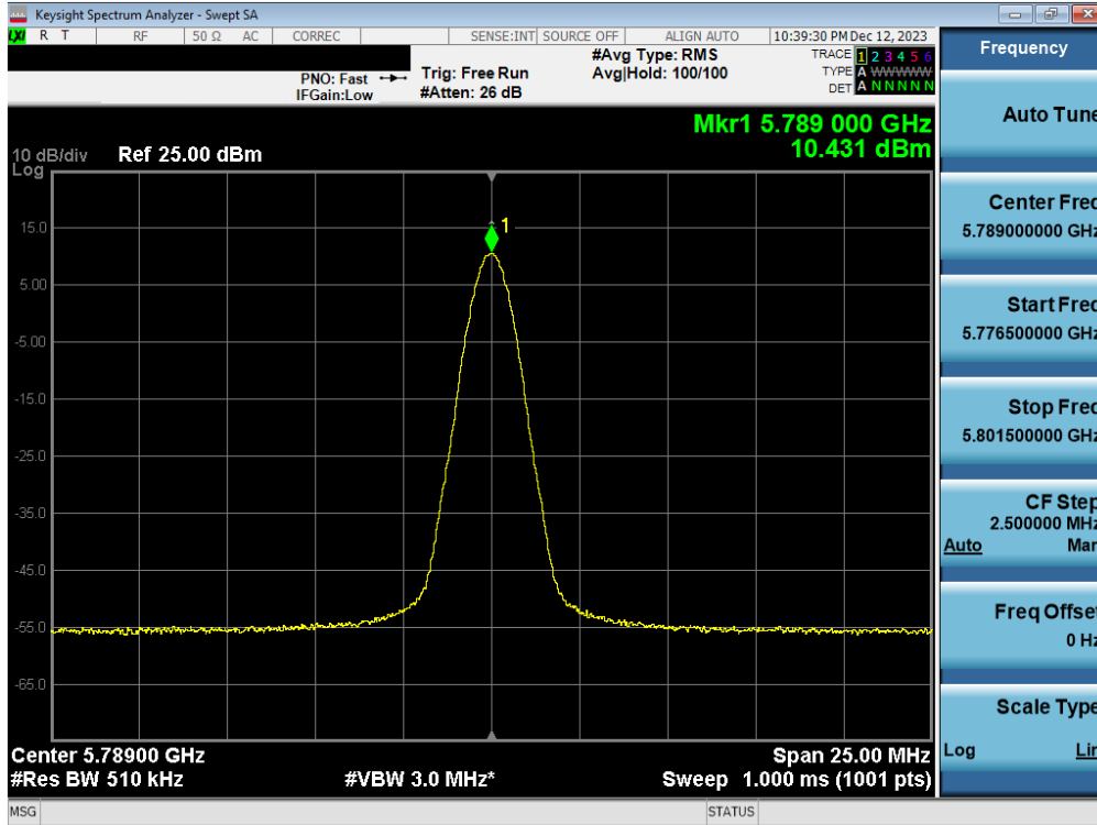
Plot 7-29. PSD Antenna 5T (BDR, ePA 5789MHz)
