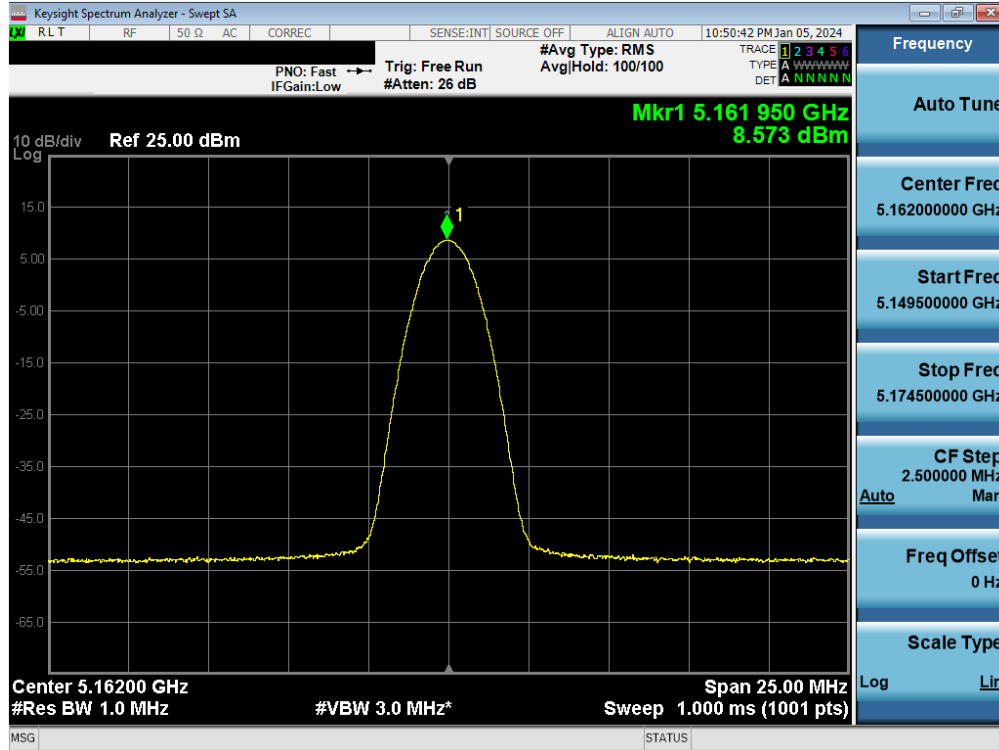
Plot 7-19. FCC PSD Antenna 5T (BDR, ePA – 5162MHz)
