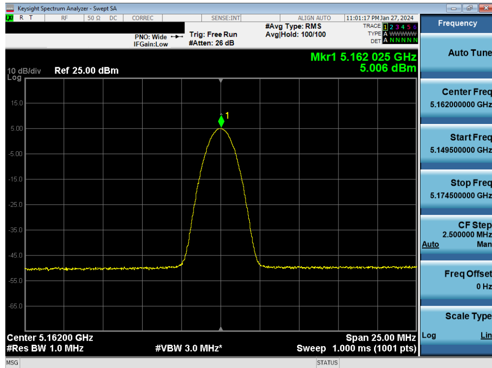
Plot 7-59. FCC PSD TxBF Antenna 3b (BDR, ePA – 5162MHz)
