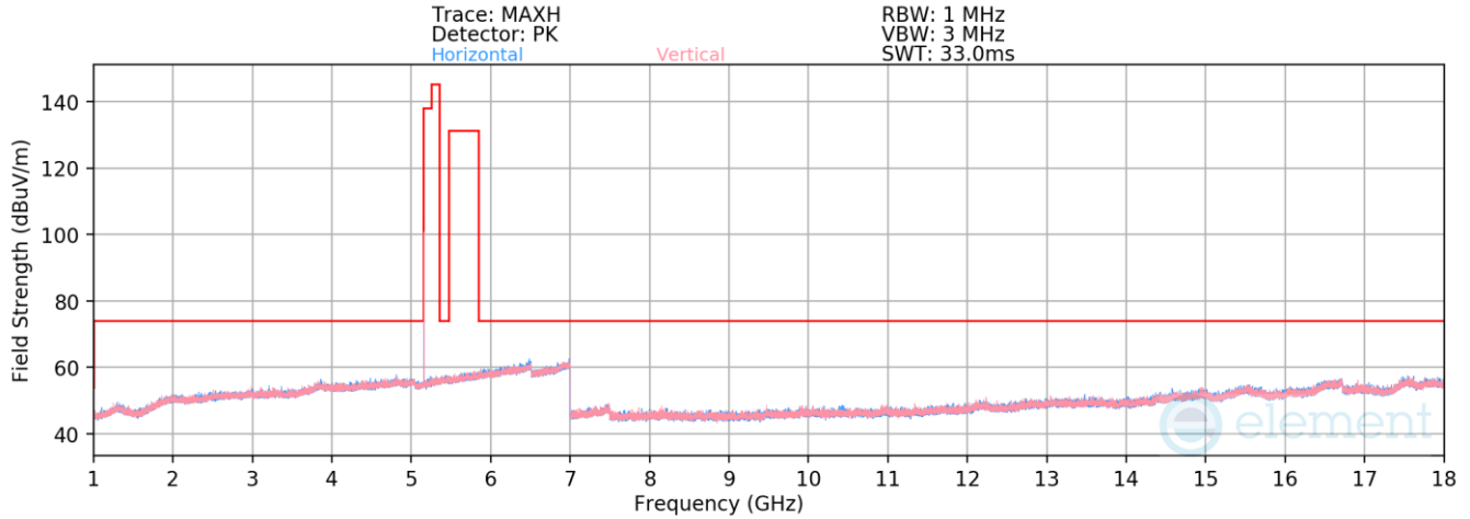
Plot 7-103. Radiated Spurious Emissions 1-18GHz Antenna 1b (BDR GFSK ePA – 5162MHz)
