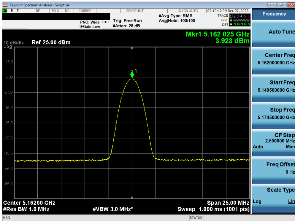
Plot 7-65. FCC/ISED PSD TxBF Antenna 3b (BDR, iPA – 5162MHz)
