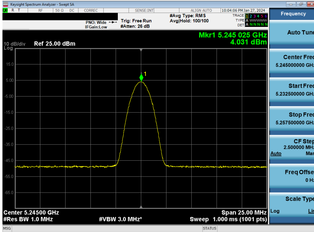
Plot 7-78. ISED PSD TxBF Antenna 5T (BDR, iPA- 5245MHz)
