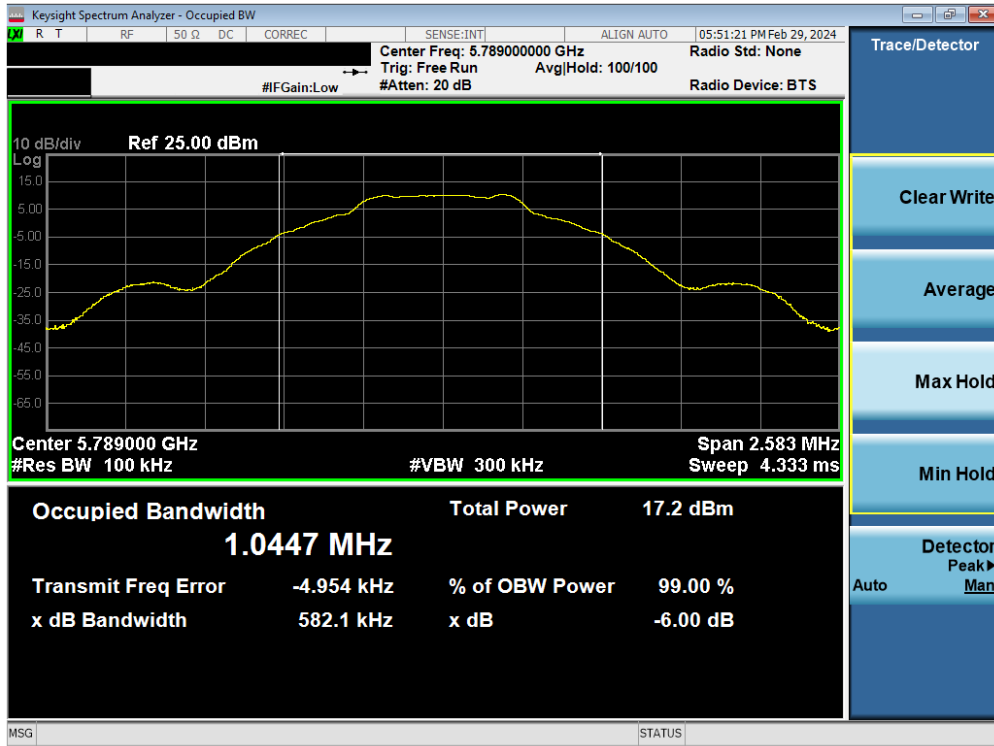
Plot 7-14. 6dB BW & 99% OBW Antenna 3b (BDR GFSK, 5789MHz)
