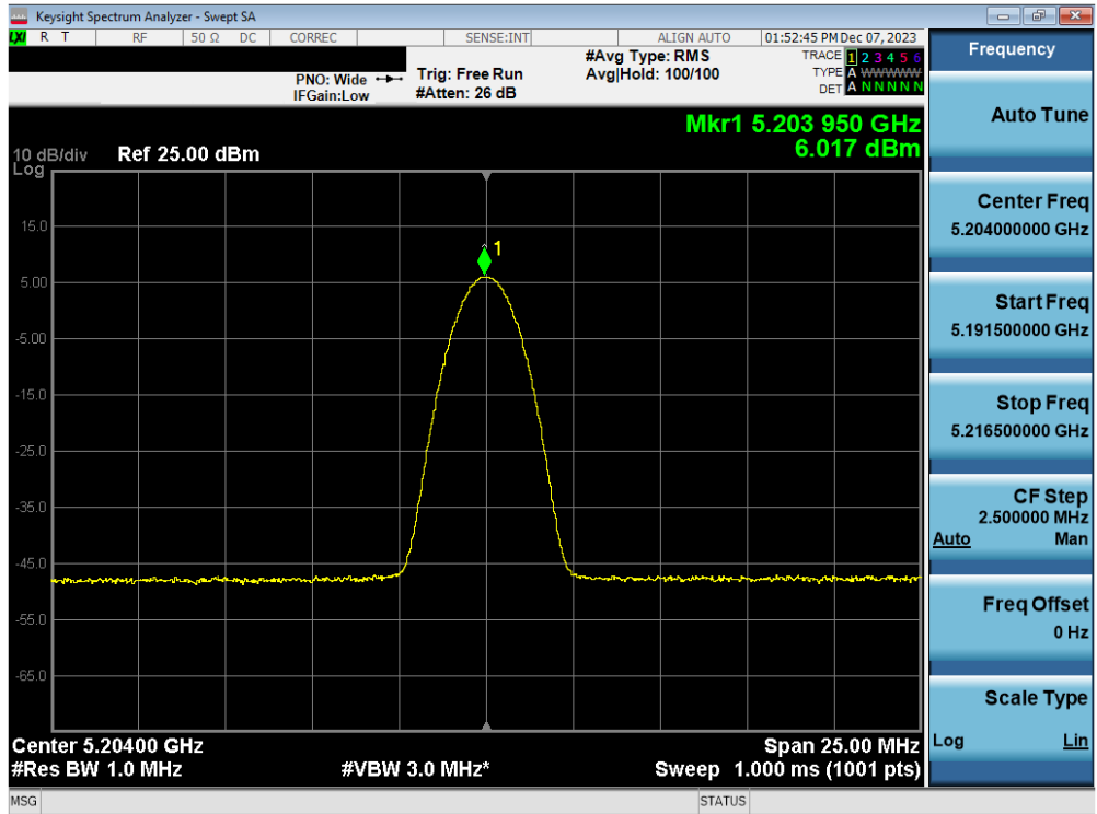
Plot 7-66. FCC PSD TxBF Antenna 5T (BDR, iPA – 5204MHz)
