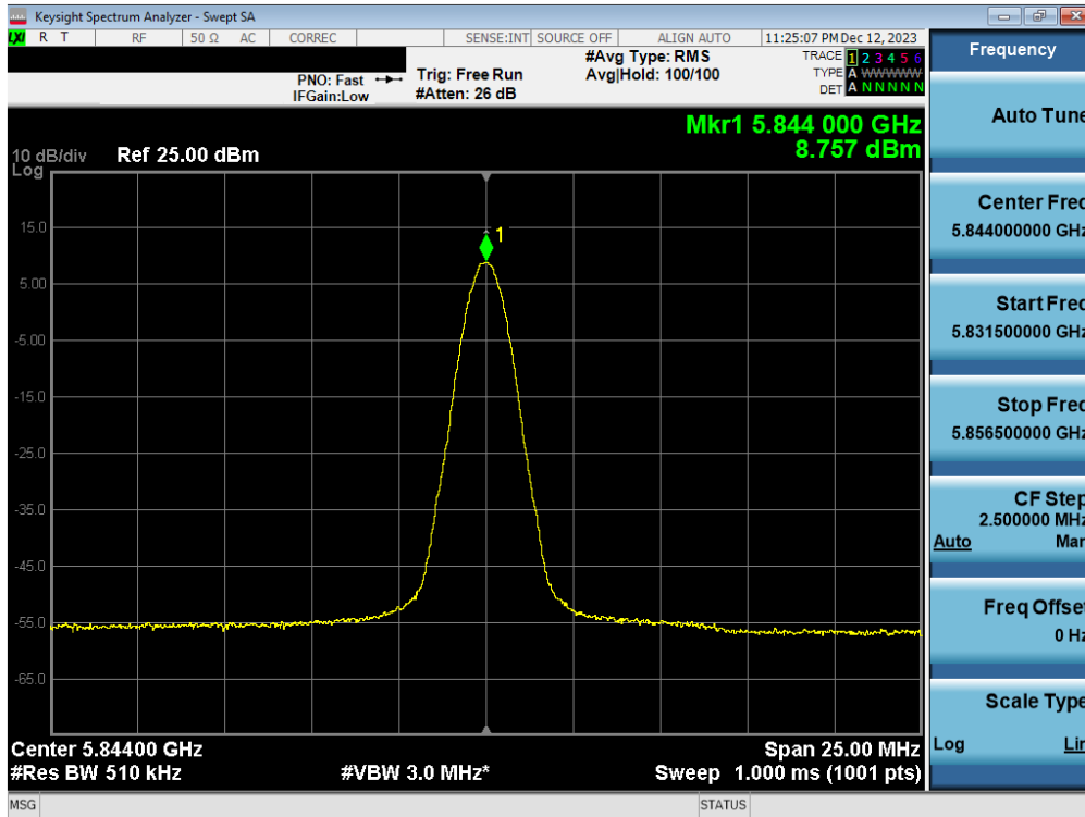
Plot 7-54. PSD Antenna 1b (BDR, ePA 5844MHz)
