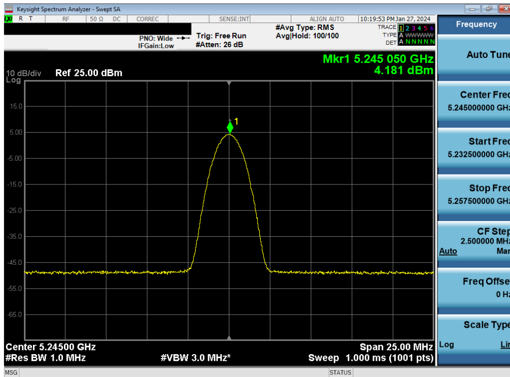
Plot 7-75. ISED PSD TxBF Antenna 3b (BDR, ePA- 5245MHz)
