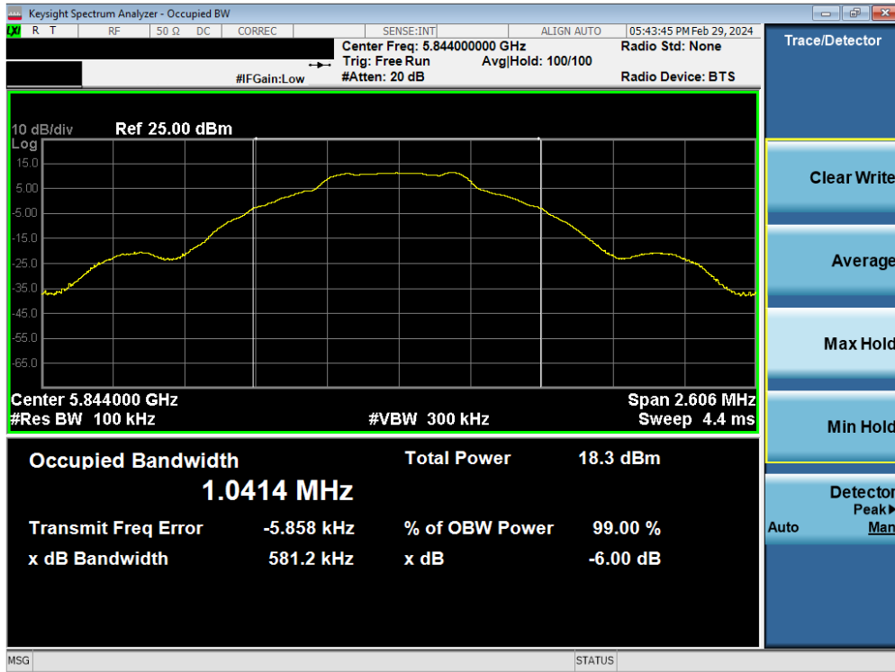
Plot 7-12. 6dB BW & 99% OBW Antenna 5T (BDR GFSK, 5844MHz)
