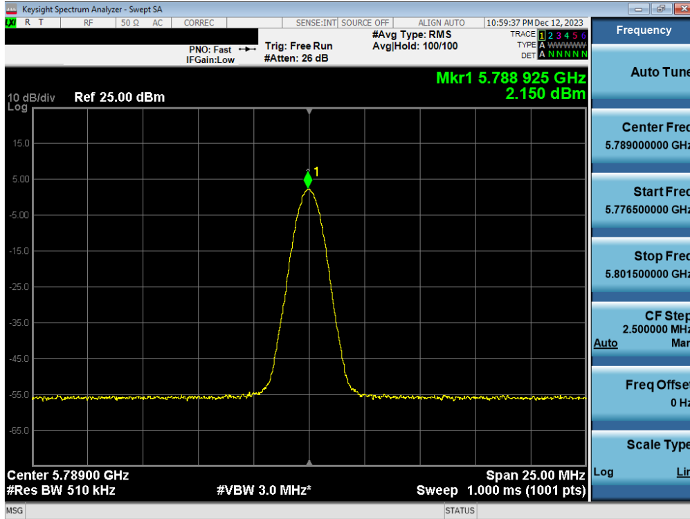
Plot 7-88. PSD TxBF Antenna 3b (BDR, iPA 5789MHz)
