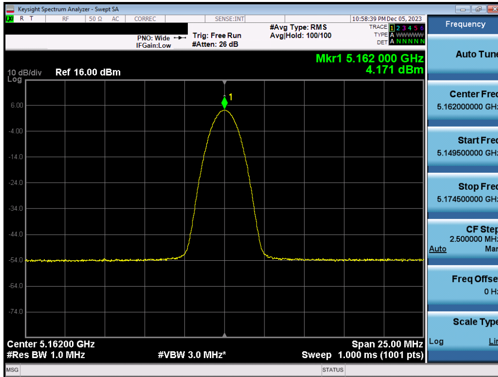
Plot 7-37. FCC/ISED PSD Antenna 3b (BDR, iPA – 5162MHz)
