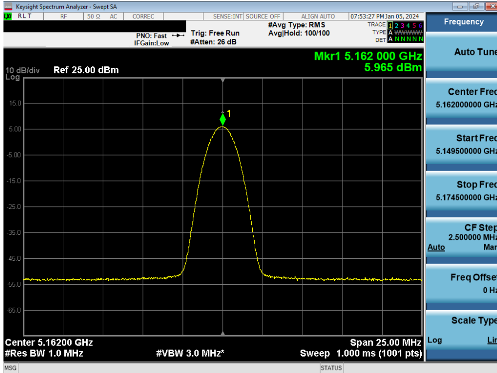
Plot 7-58. FCC PSD TxBF Antenna 5T (BDR, ePA – 5162MHz)
