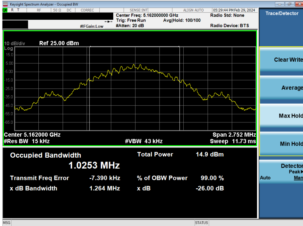
Plot 7-7. 26dB BW & 99% OBW Antenna 1b (BDR GFSK, ePA- 5162MHz)
