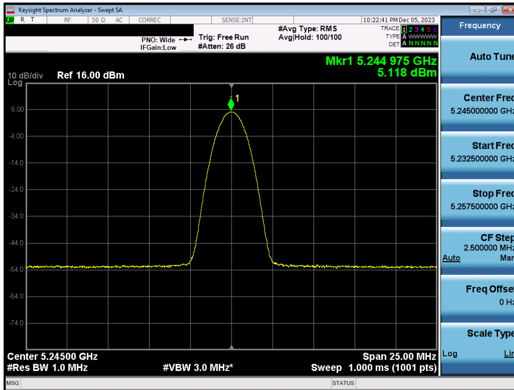
Plot 7-24. FCC/ISED PSD Antenna 5T (BDR, iPA– 5245MHz)
