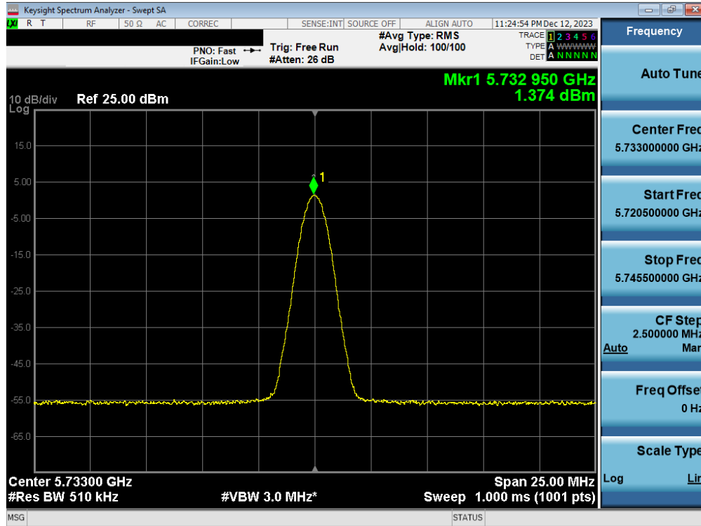
Plot 7-55. PSD Antenna 1b (BDR, iPA 5733MHz)
