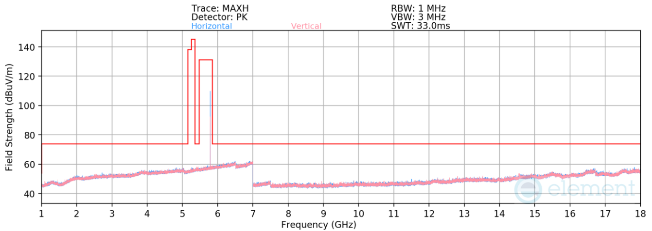
Plot 7-95. Radiated Spurious Emissions 1-18GHz Antenna 5T (BDR GFSK ePA– 5789MHz)
