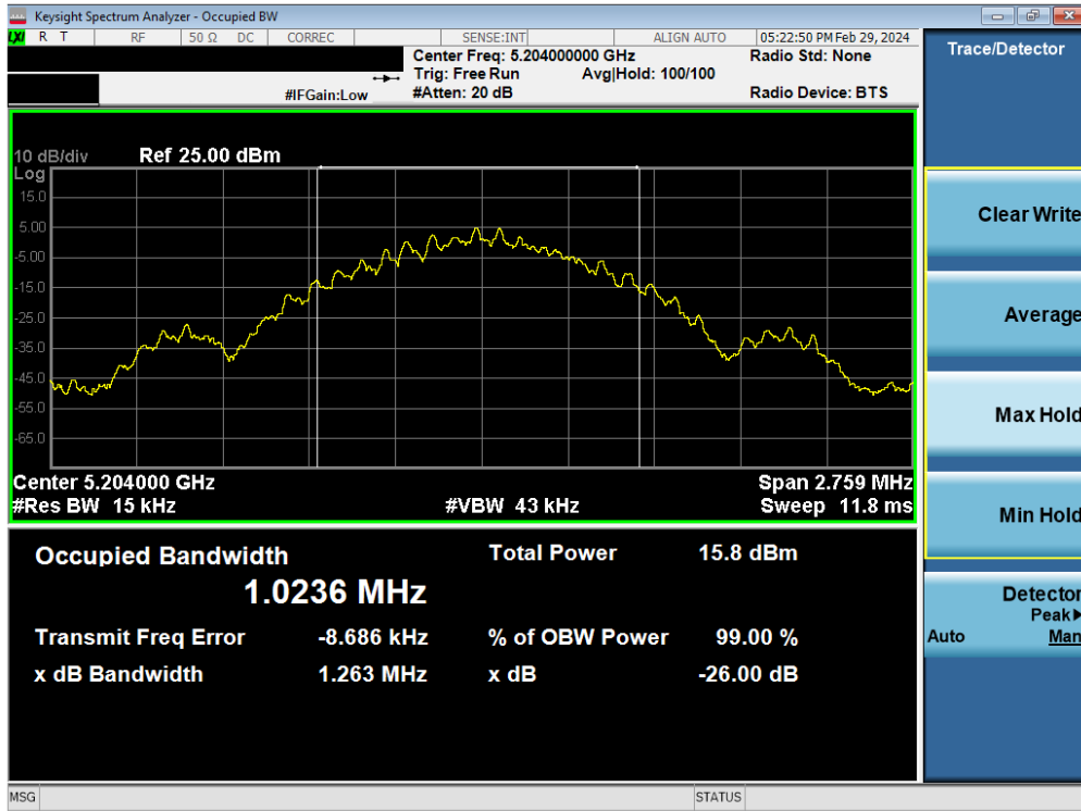
Plot 7-5. 26dB BW & 99% OBW Antenna 3b (BDR GFSK, ePA- 5204MHz)
