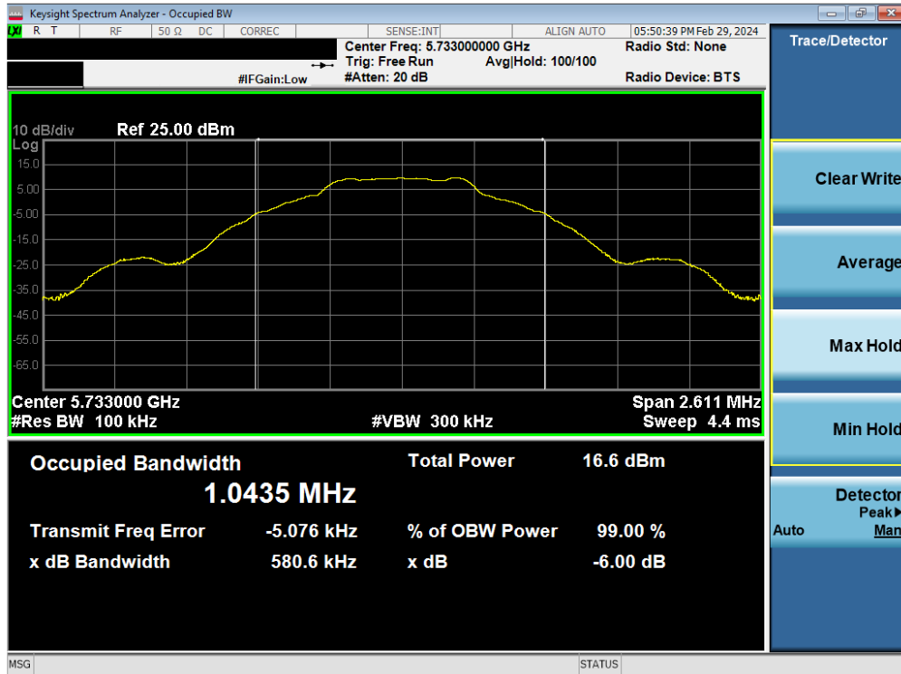
Plot 7-13. 6dB BW & 99% OBW Antenna 3b (BDR GFSK, 5733MHz)
