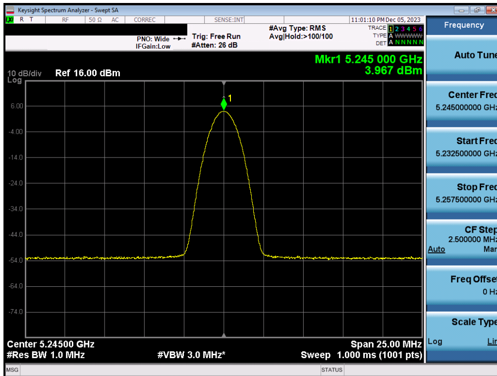
Plot 7-39. FCC/ISED PSD Antenna 3b (BDR, iPA– 5245MHz)
