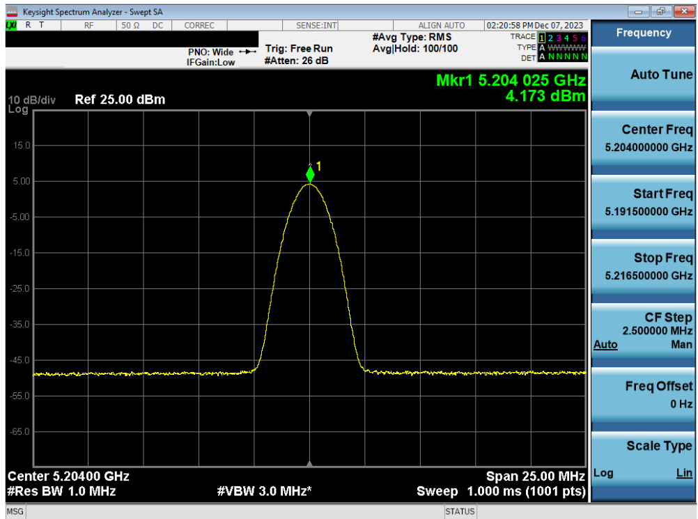
Plot 7-67. FCC/ISED PSD TxBF Antenna 3b (BDR, iPA – 5204MHz)
