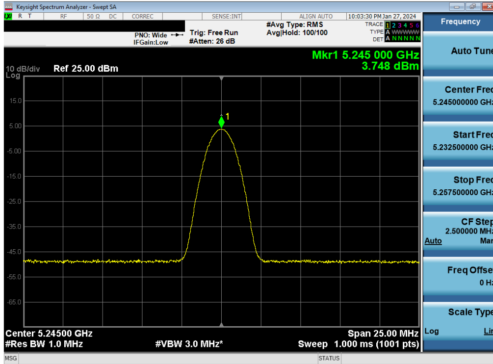
Plot 7-74. ISED PSD TxBF Antenna 5T (BDR, ePA- 5245MHz)
