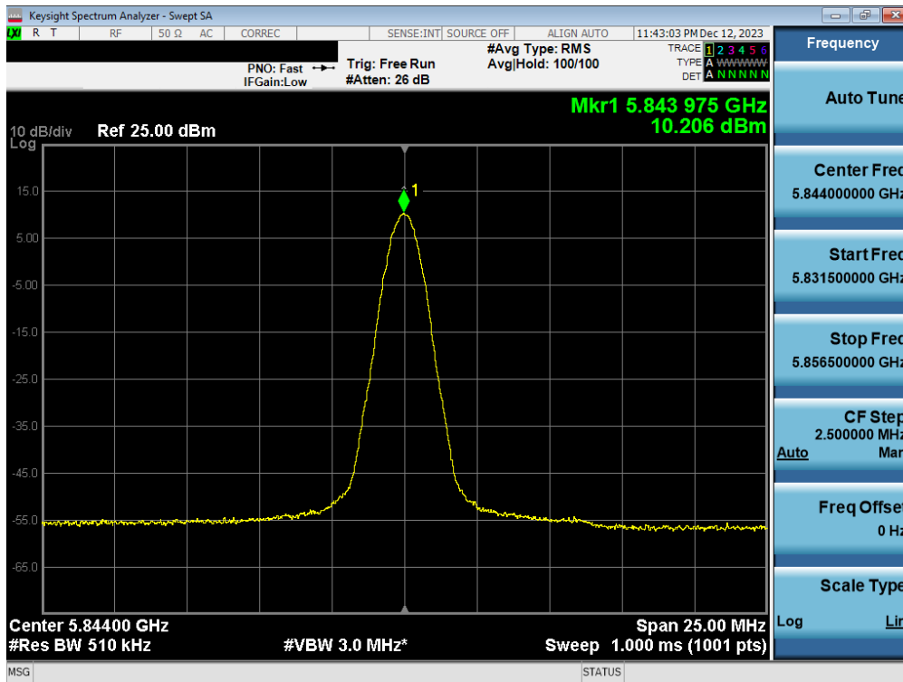
Plot 7-42. PSD Antenna 3b (BDR, ePA 5844MHz)
