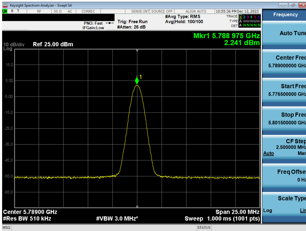
Plot 7-44. PSD Antenna 3b (BDR, iPA 5789MHz)
