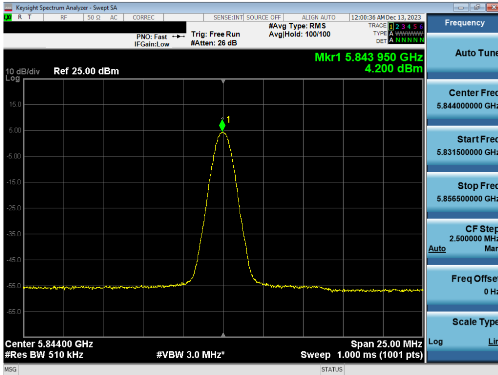
Plot 7-89. PSD TxBF Antenna 5T (BDR, iPA 5844MHz)
