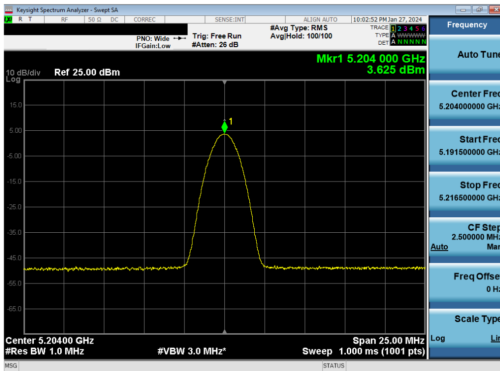
Plot 7-77. ISED PSD TxBF Antenna 5T (BDR, iPA – 5204MHz)
