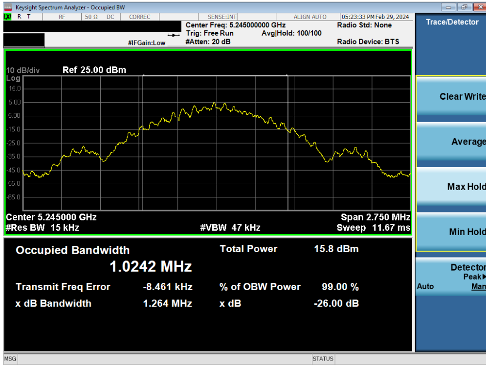
Plot 7-6. 26dB BW & 99% OBW Antenna 3b (BDR GFSK, ePA - 5245MHz)
