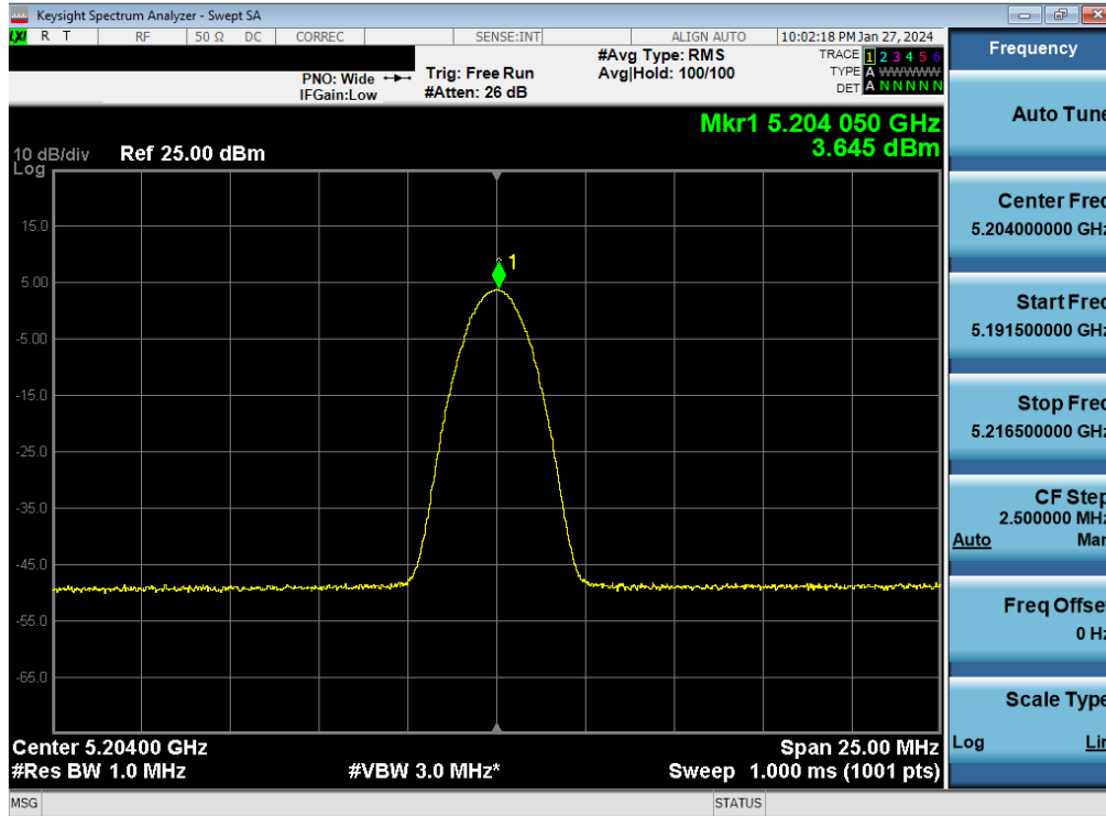
Plot 7-72. ISED PSD TxBF Antenna 5T (BDR, ePA – 5204MHz)
