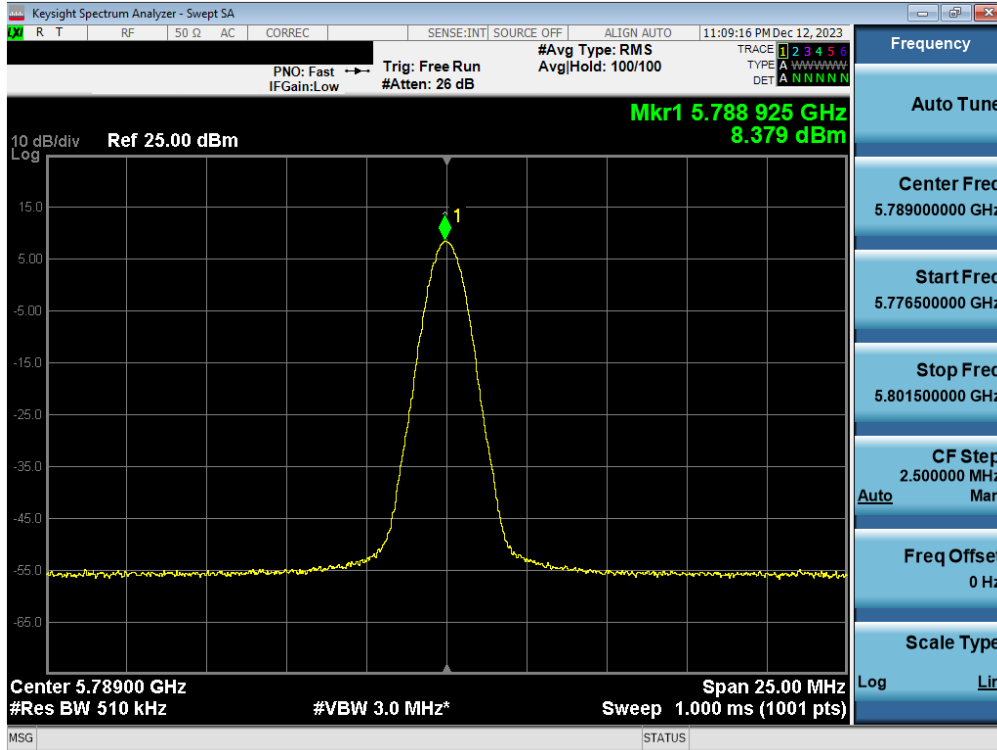
Plot 7-53. PSD Antenna 1b (BDR, ePA 5789MHz)
