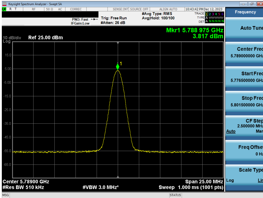
Plot 7-87. PSD TxBF Antenna 5T (BDR, iPA 5789MHz)
