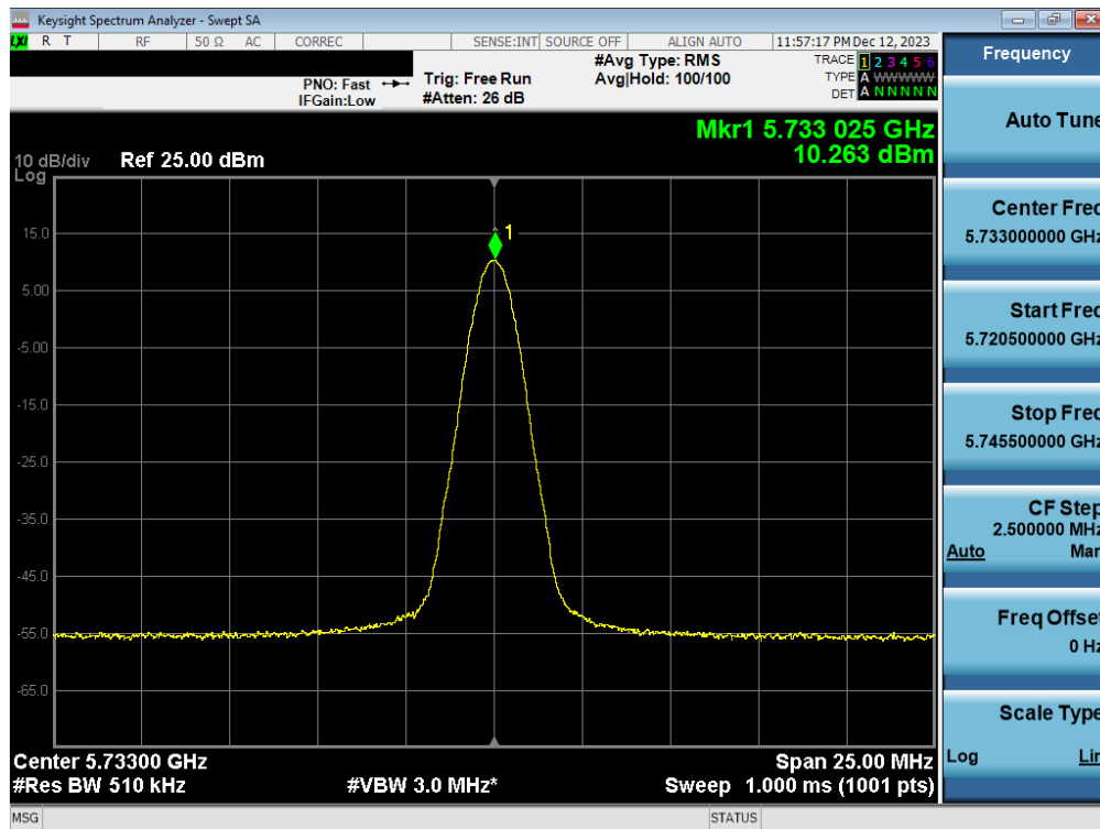
Plot 7-28. PSD Antenna 5T (BDR, ePA 5733MHz)
