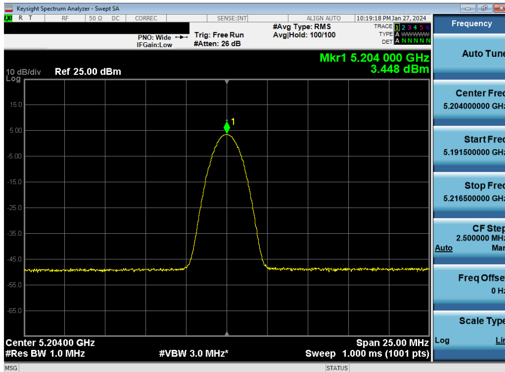
Plot 7-73. ISED PSD TxBF Antenna 3b (BDR, ePA – 5204MHz)
