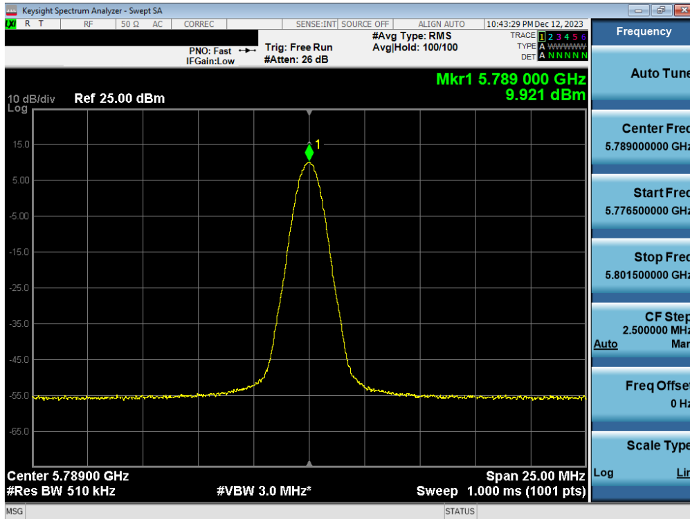
Plot 7-81. PSD TxBF Antenna 5T (BDR, ePA 5789MHz)
