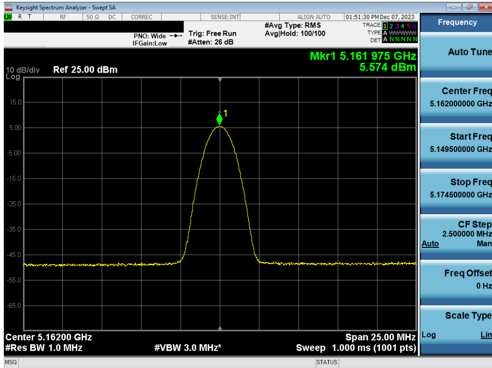
Plot 7-64. FCC PSD TxBF Antenna 5T (BDR, iPA – 5162MHz)
