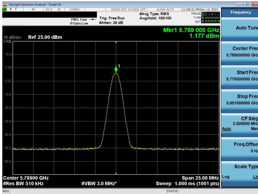
Plot 7-56. PSD Antenna 1b (BDR, iPA 5789MHz)
