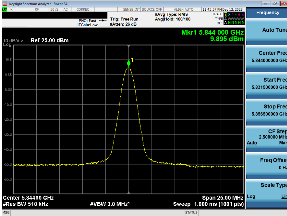
Plot 7-84. PSD TxBF Antenna 3b (BDR, ePA 5844MHz)
