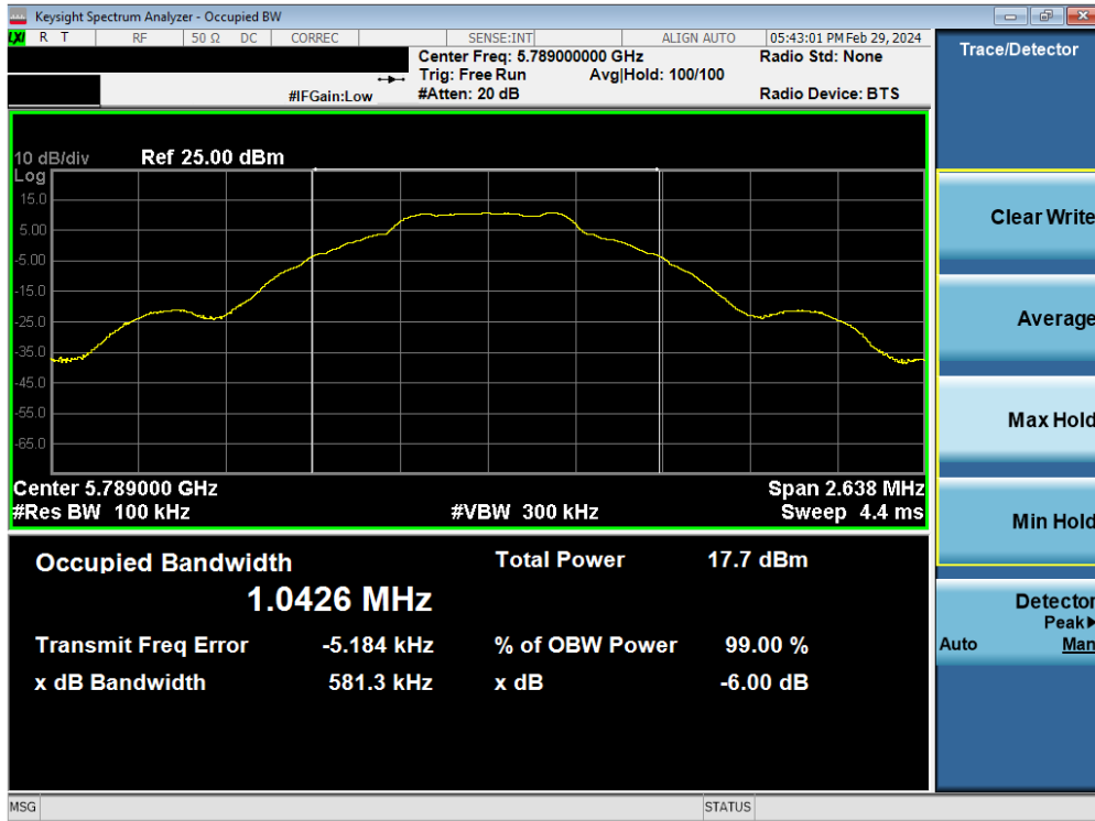
Plot 7-11. 6dB BW & 99% OBW Antenna 5T (BDR GFSK, 5789MHz)
