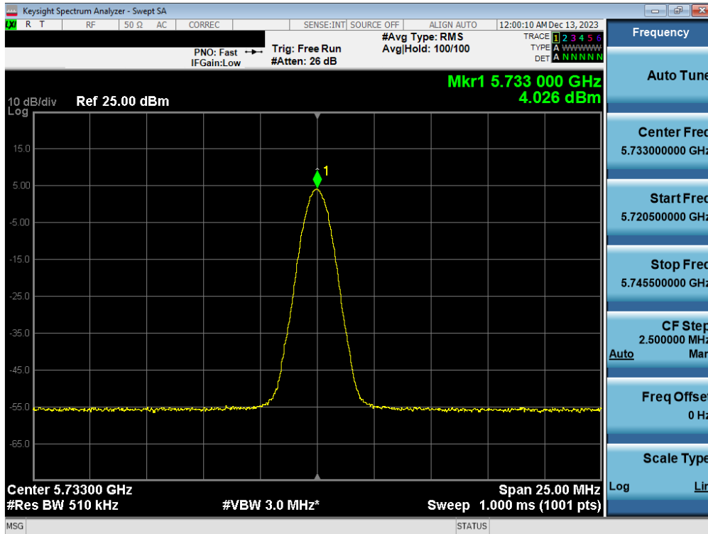
Plot 7-85. PSD TxBF Antenna 5T (BDR, iPA 5733MHz)
