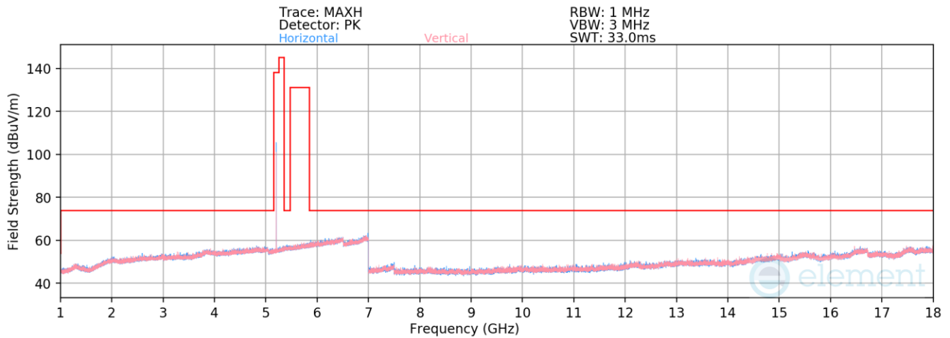
Plot 7-104. Radiated Spurious Emissions 1-18GHz Antenna 1b (BDR GFSK ePA – 5204MHz)
