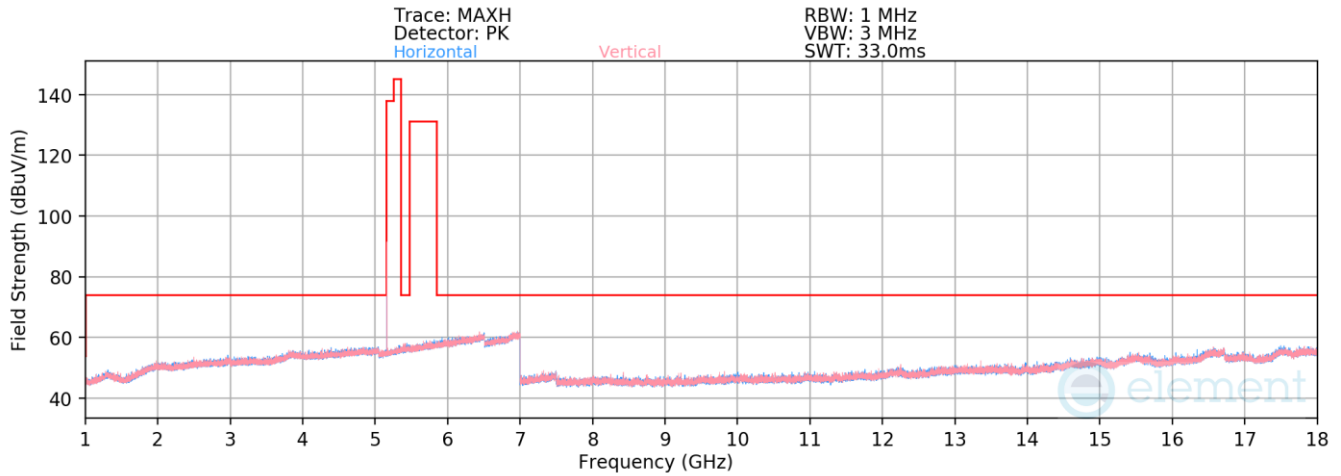
Plot 7-91. Radiated Spurious Emissions 1-18GHz Antenna 5T (BDR GFSK ePA – 5162MHz)
