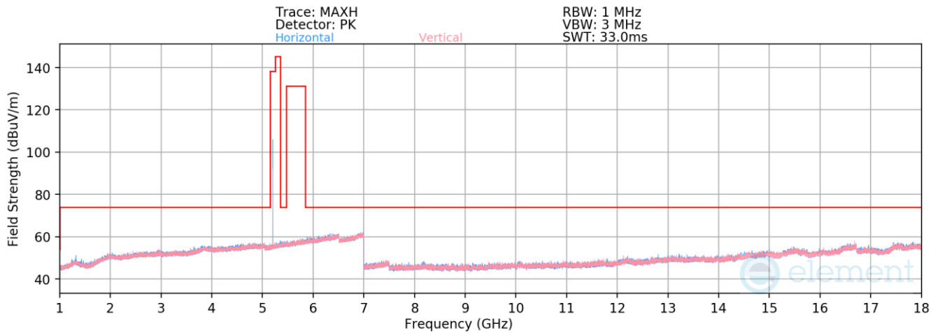
Plot 7-92. Radiated Spurious Emissions 1-18GHz Antenna 5T (BDR GFSK ePA – 5204MHz)
