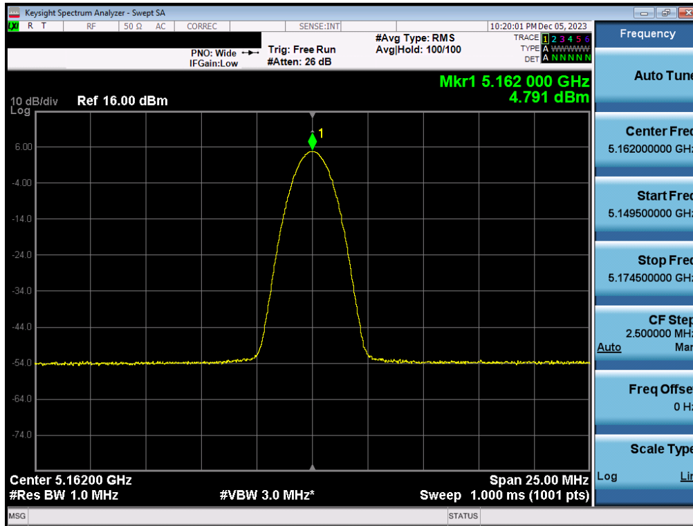
Plot 7-22. FCC/ISED PSD Antenna 5T (BDR, iPA - 5162MHz)
