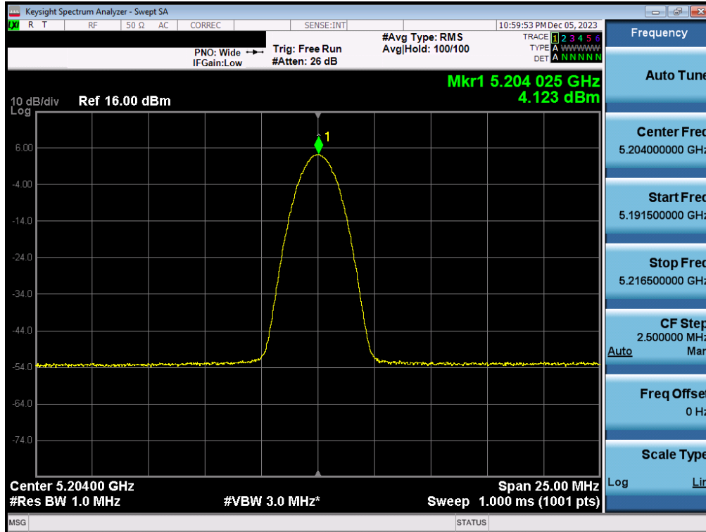
Plot 7-38. FCC/ISED PSD Antenna 3b (BDR, iPA – 5204MHz)
