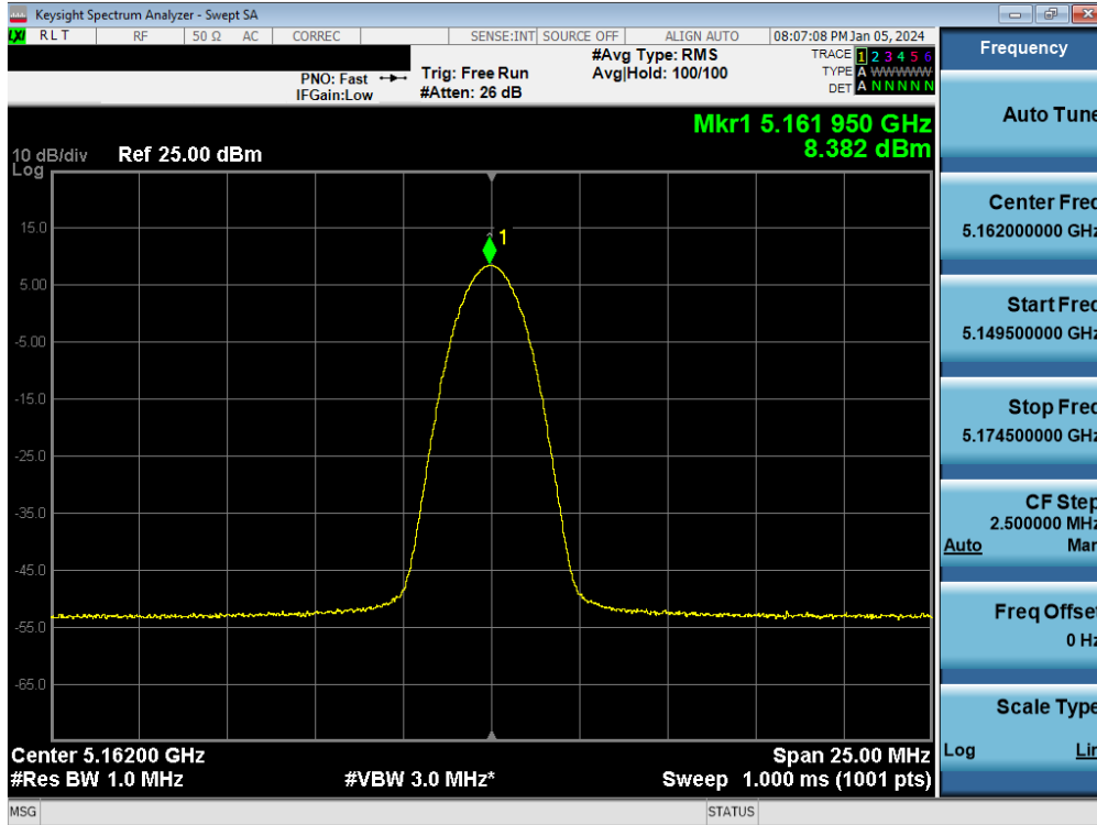
Plot 7-34. FCC/ISED PSD Antenna 3b (BDR, ePA – 5162MHz)
