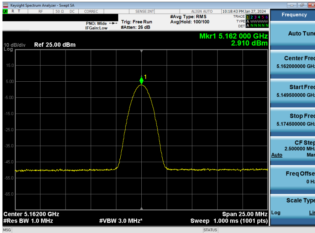
Plot 7-71. ISED PSD TxBF Antenna 3b (BDR, ePA – 5162MHz)
