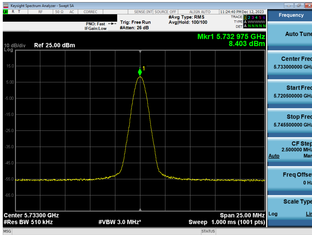
Plot 7-52. PSD Antenna 1b (BDR, ePA 5733MHz)
