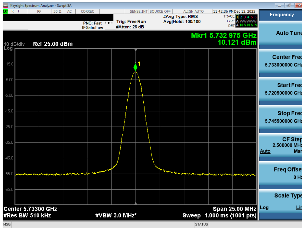
Plot 7-40. PSD Antenna 3b (BDR, ePA 5733MHz)
