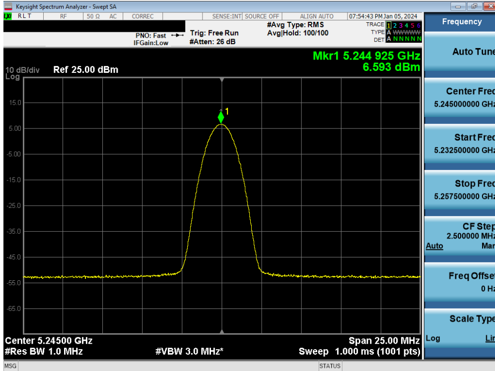
Plot 7-62. FCC PSD TxBF Antenna 5T (BDR, ePA- 5245MHz)
