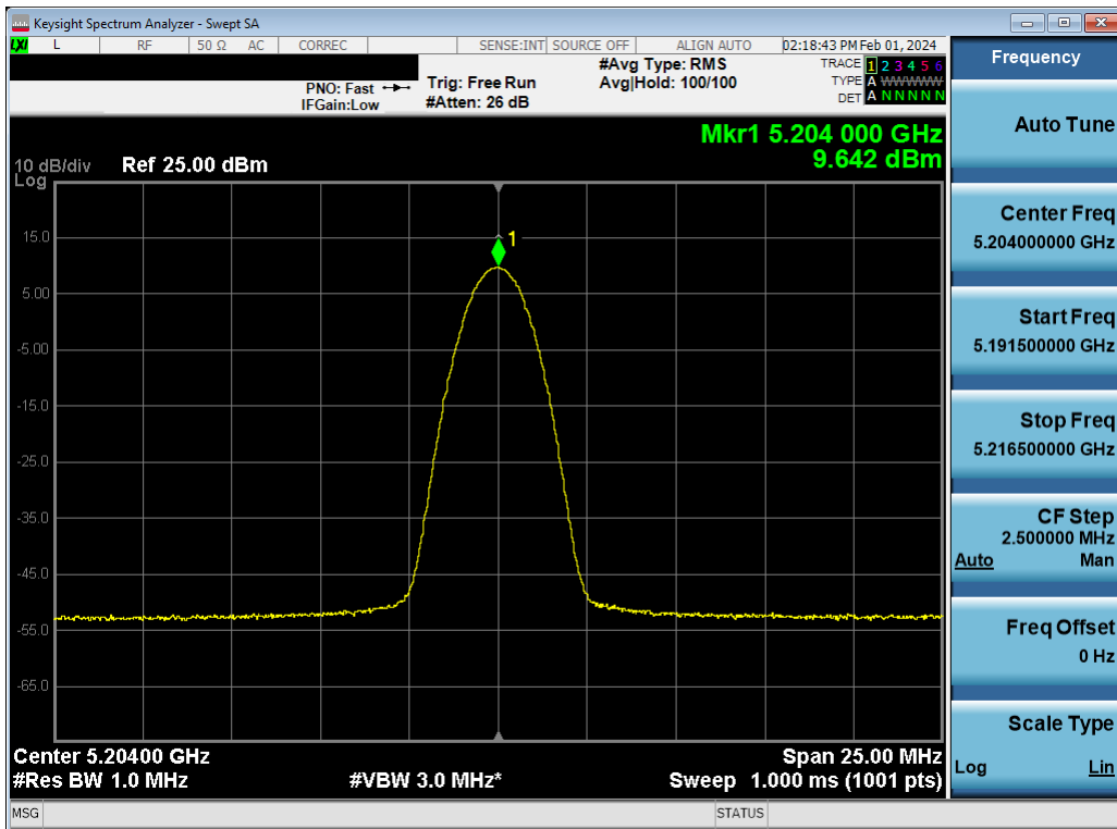
Plot 7-26. ISED PSD Antenna 5T (BDR, ePA – 5204MHz)
