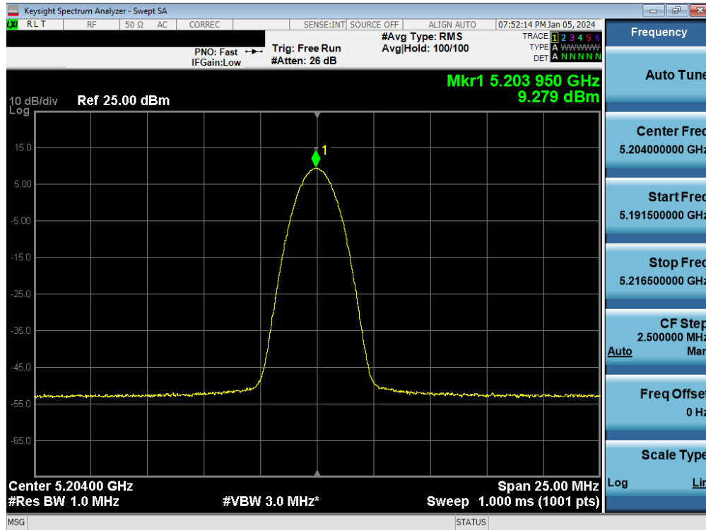
Plot 7-20. FCC PSD Antenna 5T (BDR, ePA – 5204MHz)
