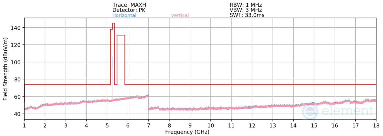
Plot 7-93. Radiated Spurious Emissions 1-18GHz Antenna 5T (BDR GFSK ePA – 5245MHz)
