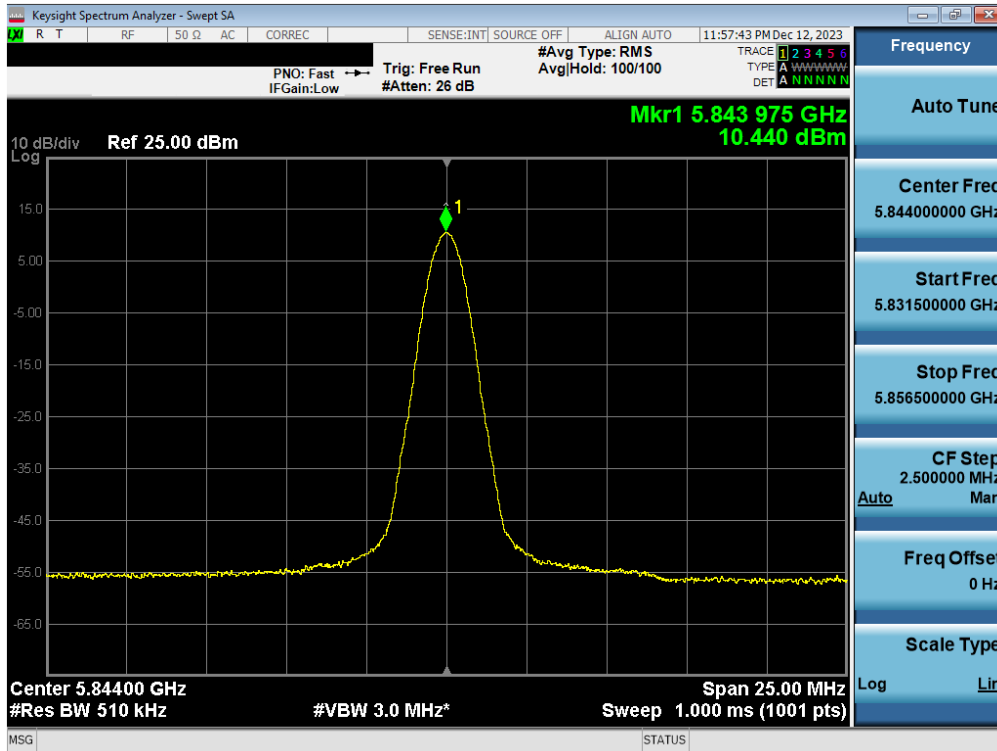
Plot 7-30. PSD Antenna 5T (BDR, ePA 5844MHz)
