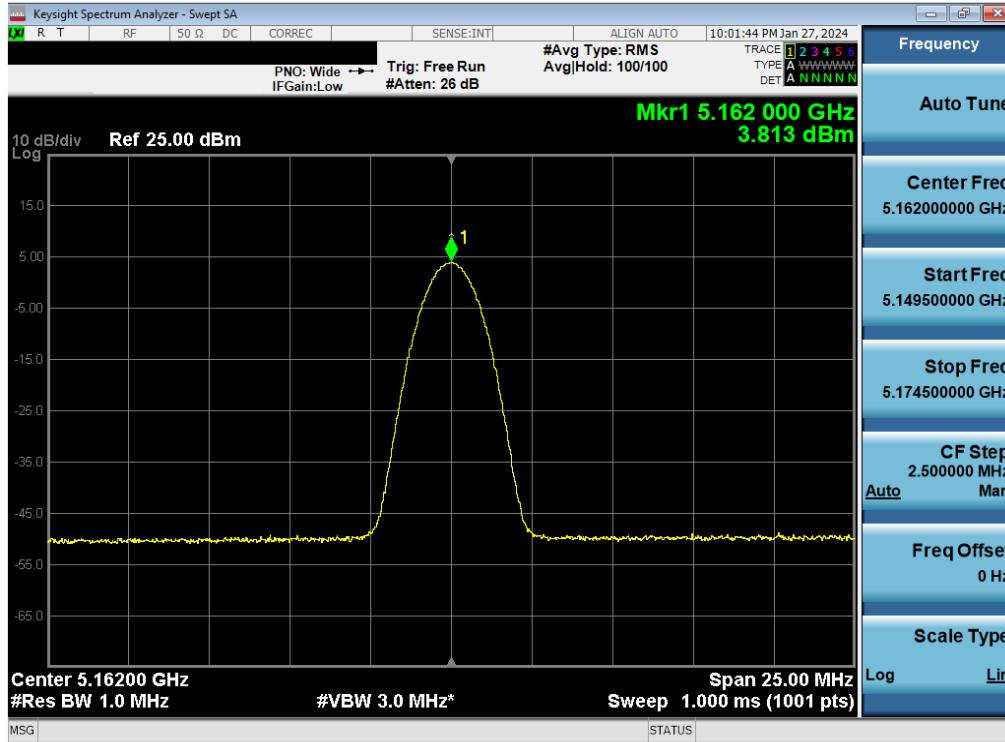
Plot 7-76. ISED PSD TxBF Antenna 5T (BDR, iPA – 5162MHz)
