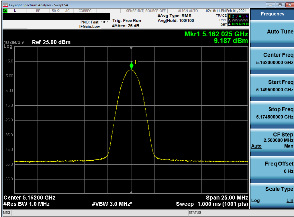
Plot 7-25. ISED PSD Antenna 5T (BDR, ePA – 5162MHz)
