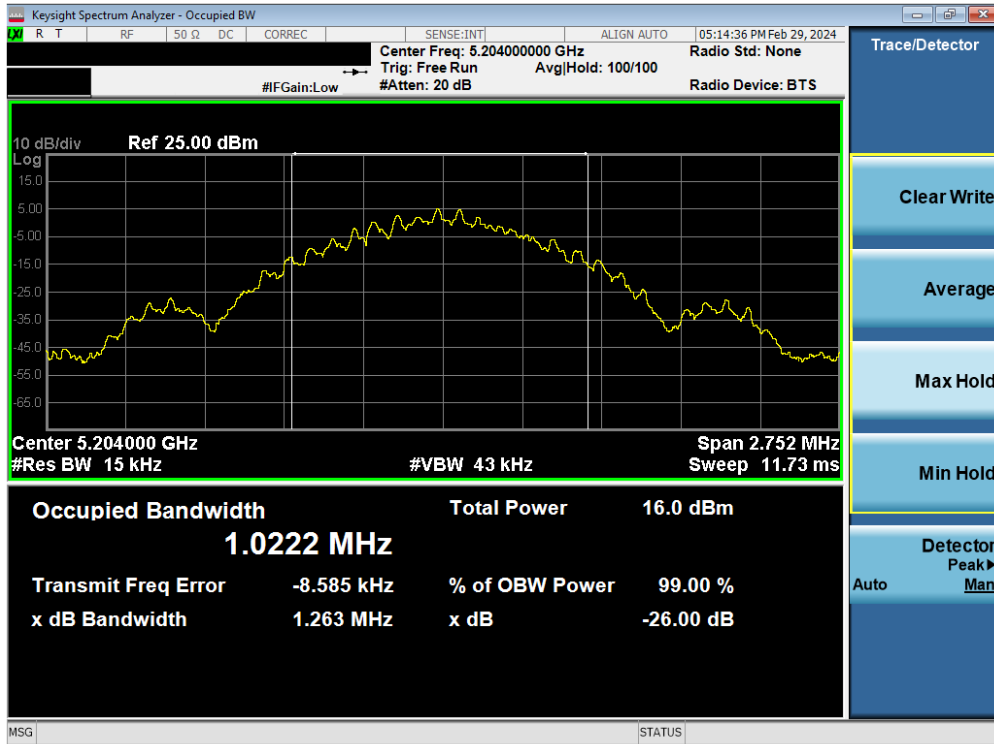
Plot 7-2. 26dB BW & 99% OBW Antenna 5T (BDR GFSK, ePA- 5204MHz)
