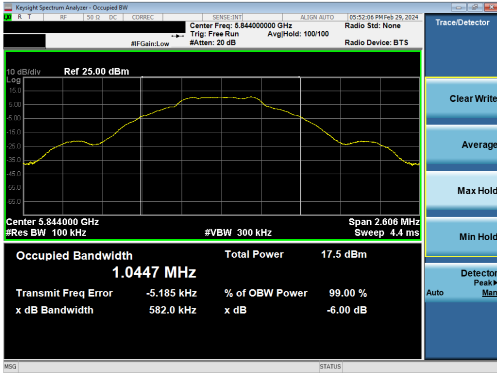
Plot 7-15. 6dB BW & 99% OBW Antenna 3b (BDR GFSK, 5844MHz)
