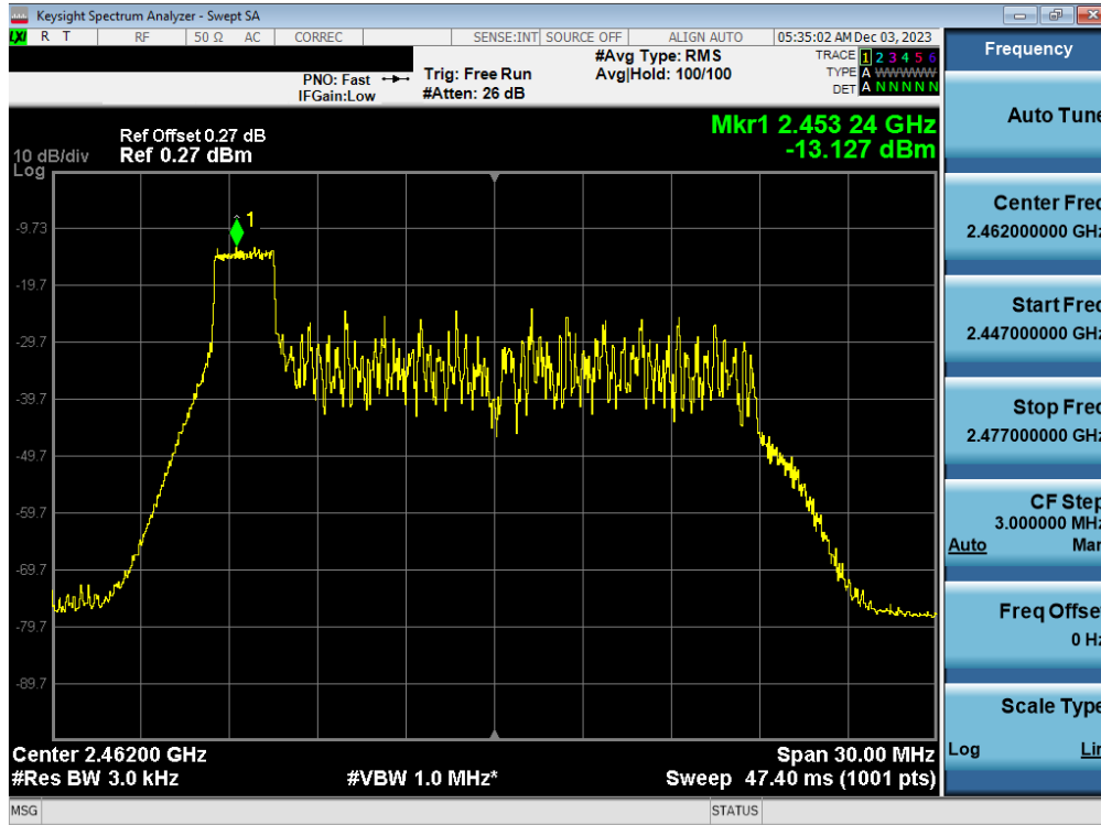
Plot 7-61. Power Spectral Density Plot Antenna 3a (802.11ax OFDMA – RU26 Index 0 – Ch. 11)
