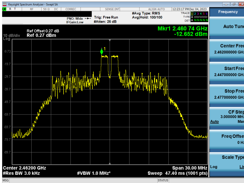
Plot 7-64. Power Spectral Density Plot Antenna 1a (802.11ax OFDMA – RU26 Index 4 – Ch. 11)
