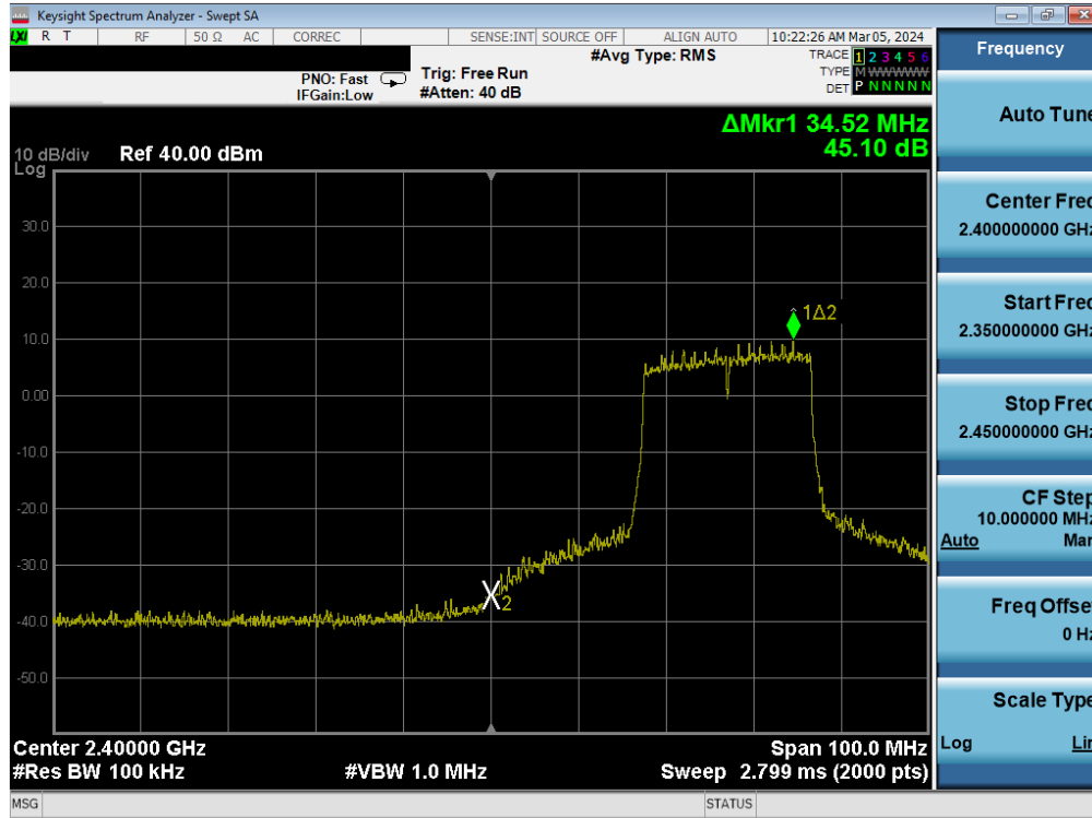
Plot 7-79. Band Edge Antenna 3a (802.11ax OFDMA – RU242 – Ch. 4)
