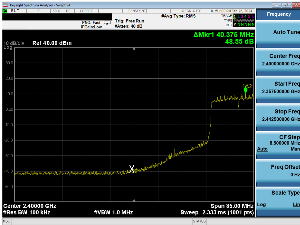
Plot 7-81. Band Edge Antenna 3a (802.11ax OFDMA – RU242 – Ch. 6(low))
