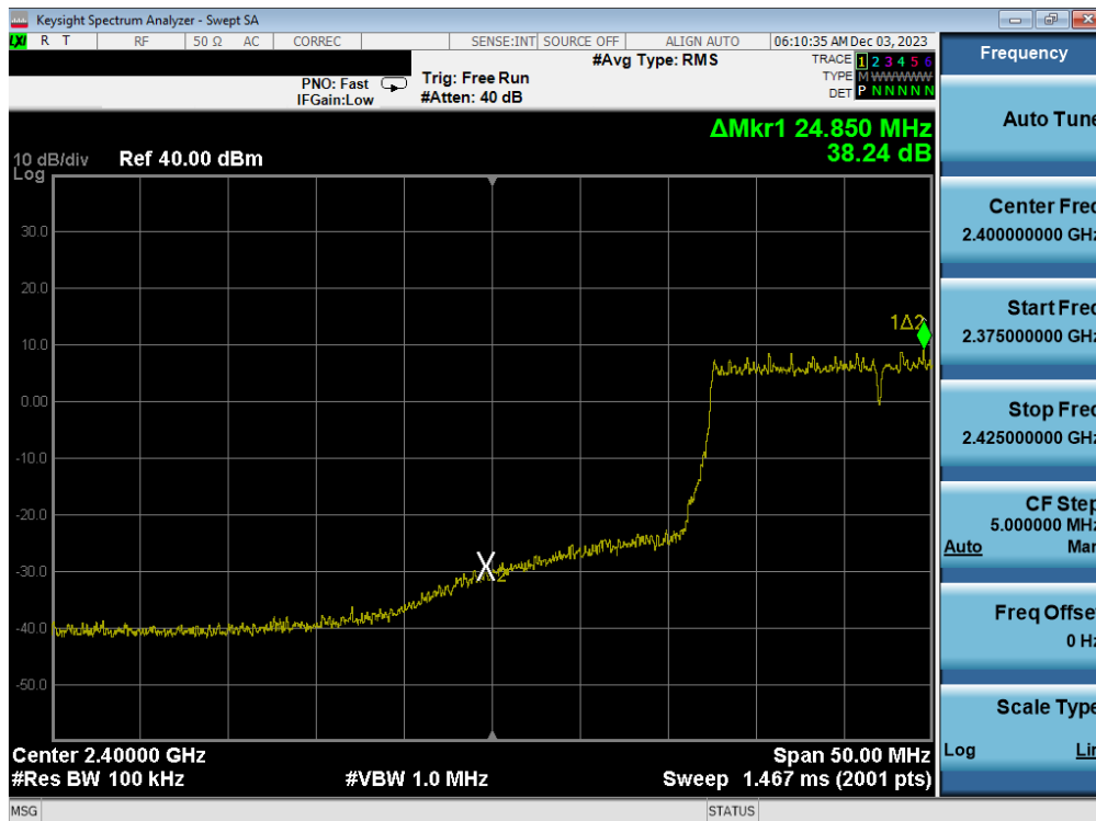
Plot 7-78. Band Edge Antenna 3a (802.11ax OFDMA – RU242 – Ch. 3)
