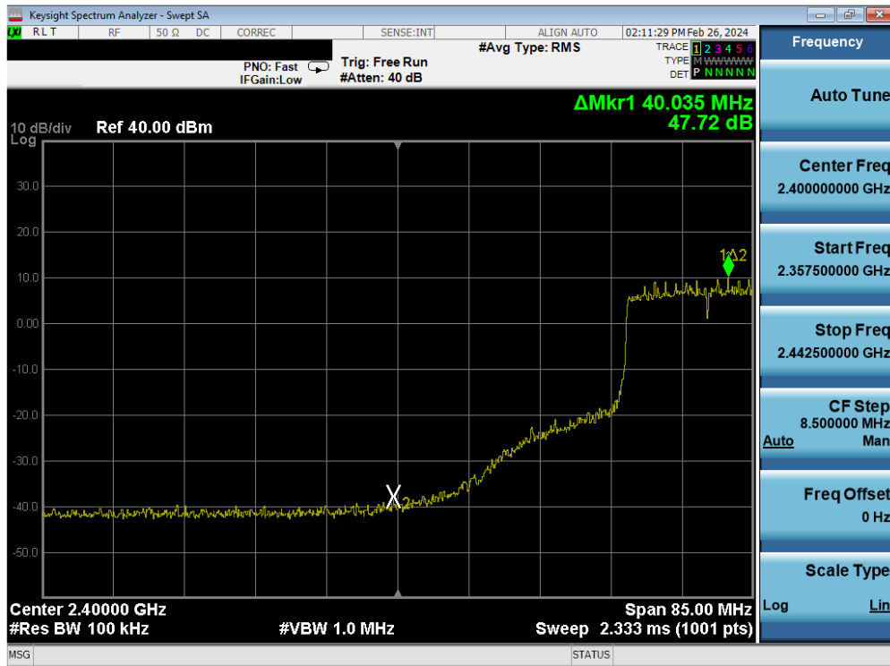
Plot 7-97. Band Edge Antenna 1a (802.11ax OFDMA – RU242 – Ch. 6(low))
