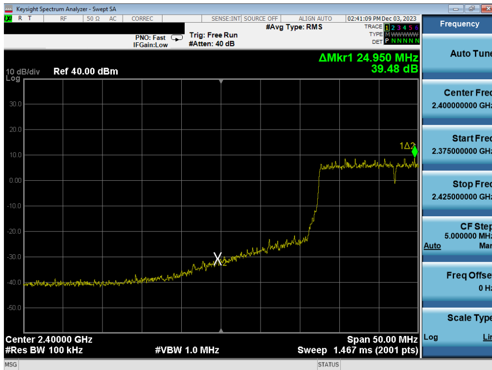
Plot 7-94. Band Edge Antenna 1a (802.11ax OFDMA – RU242 – Ch. 3)
