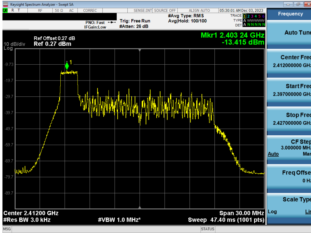
Plot 7-49. Power Spectral Density Plot Antenna 3a (802.11ax OFDMA – RU26 Index 0 – Ch. 1)
