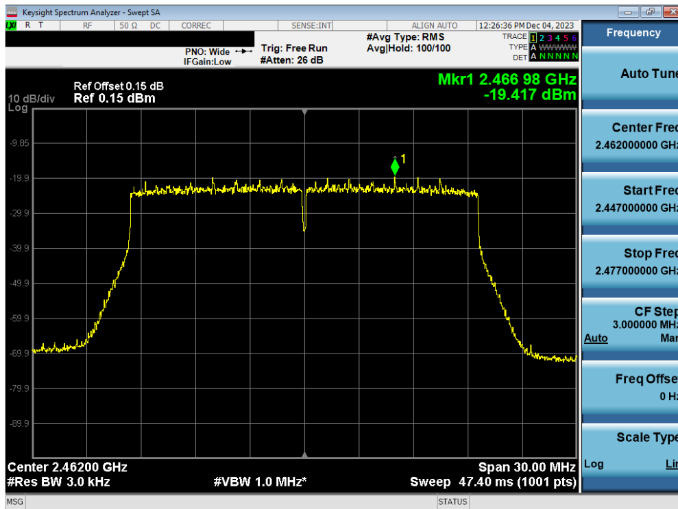
Plot 7-72. Power Spectral Density Plot Antenna 1a (802.11ax OFDMA – RU242 – Ch. 11)
