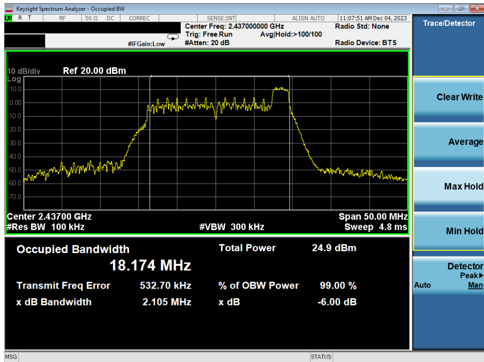
Plot 7-18. 6dB BW & 99% OBW Antenna 1a (802.11ax OFDMA – RU26 Index 8 – Ch. 6)
