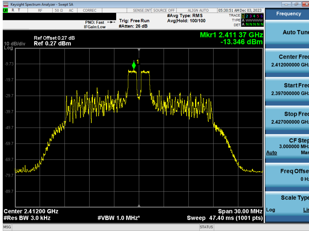
Plot 7-51. Power Spectral Density Plot Antenna 3a (802.11ax OFDMA – RU26 Index 4 – Ch. 1)
