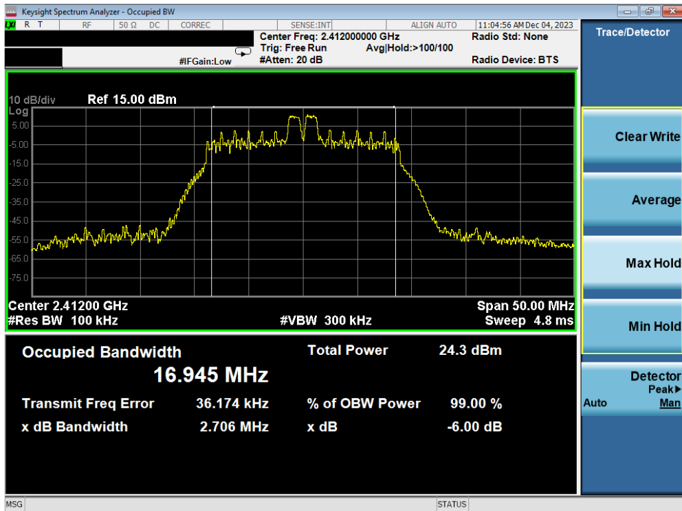
Plot 7-14. 6dB BW & 99% OBW Plot Antenna 1a (802.11ax OFDMA – RU26 Index 4 – Ch. 1)
