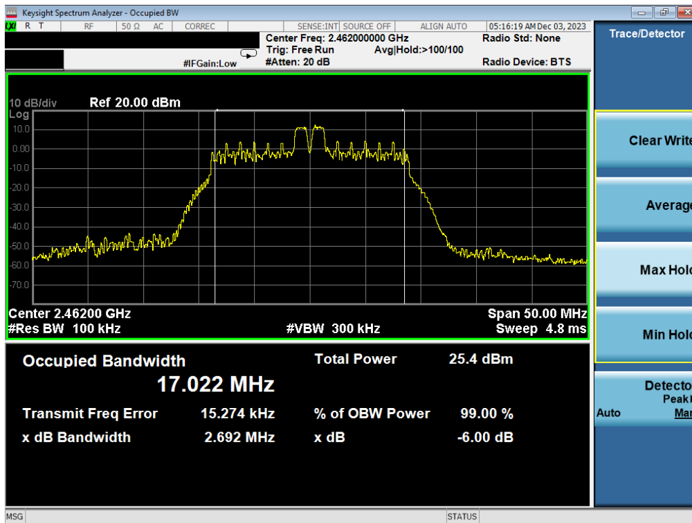
Plot 7-8. 6dB BW & 99% OBW Antenna 3a (802.11ax OFDMA – RU26 Index 4 – Ch. 11)
