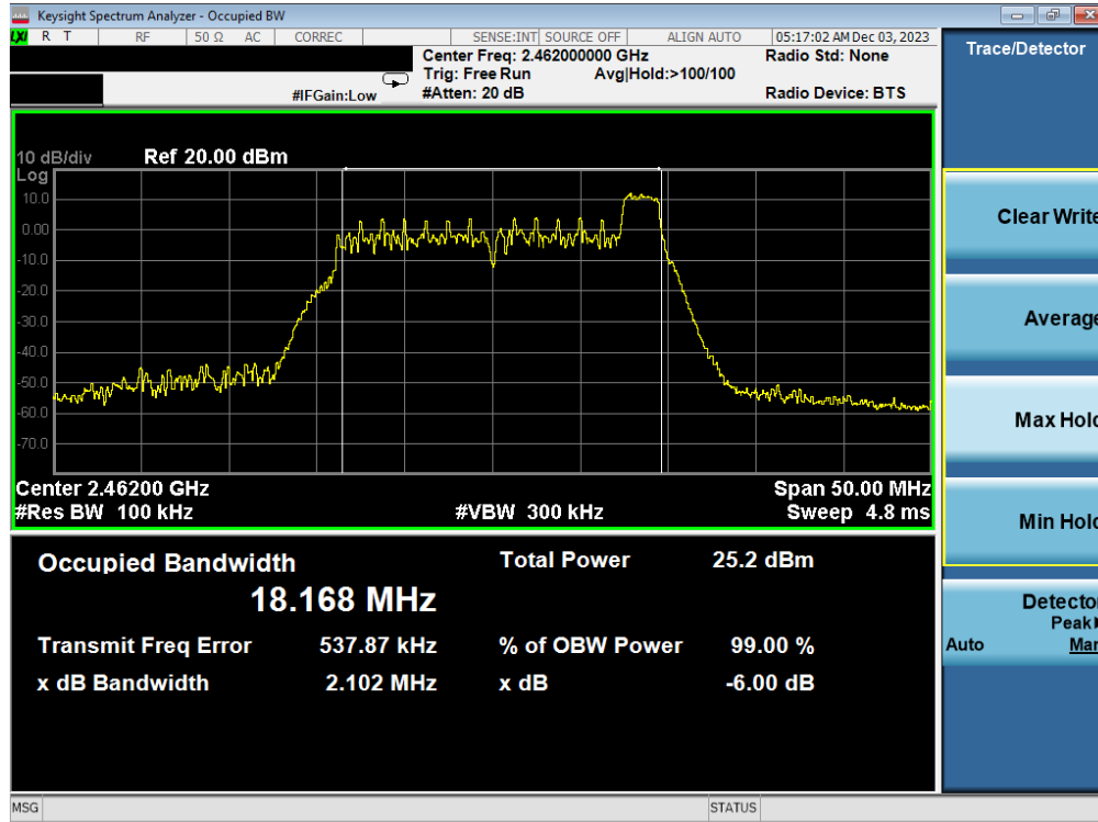
Plot 7-9. 6dB BW & 99% OBW Plot Antenna 3a (802.11ax OFDMA – RU26 Index 8 – Ch. 11)
