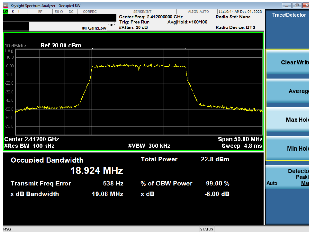
Plot 7-22. 6dB BW & 99% OBW Plot Antenna 1a (802.11ax OFDMA – RU242 – Ch. 1)
