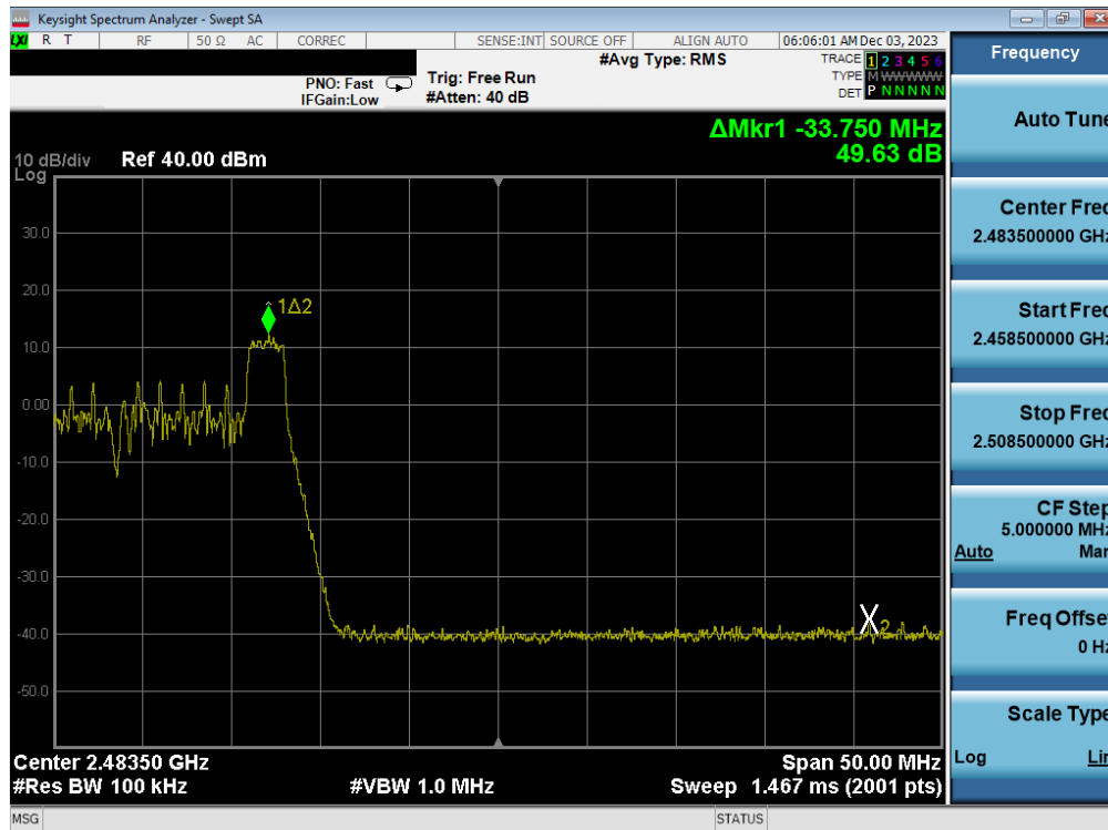
Plot 7-74. Band Edge Antenna 3a (802.11ax OFDMA – RU26 Index 8 – Ch. 11)
