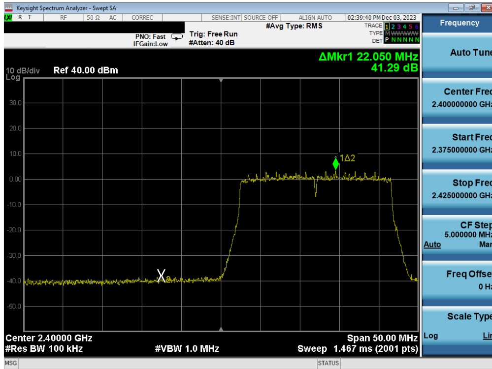
Plot 7-92. Band Edge Antenna 1a (802.11ax OFDMA – RU242 – Ch. 1)
