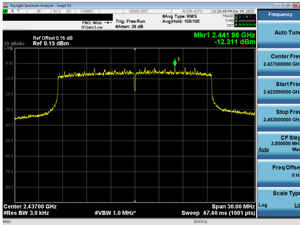
Plot 7-70. Power Spectral Density Plot Antenna 1a (802.11ax OFDMA – RU242 – Ch. 6)
