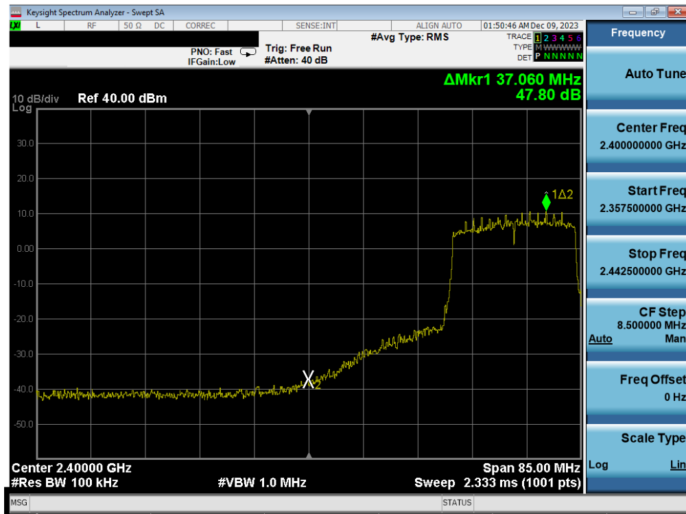
Plot 7-80. Band Edge Antenna 3a (802.11ax OFDMA – RU242 – Ch. 5)
