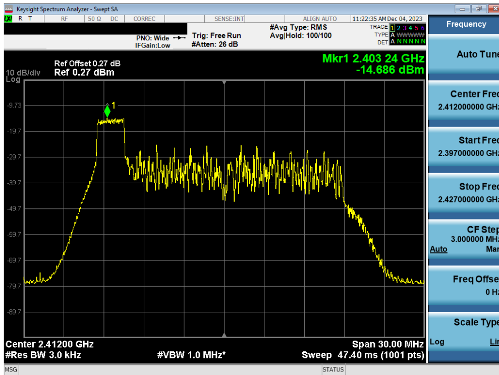
Plot 7-50. Power Spectral Density Plot Antenna 1a (802.11ax OFDMA – RU26 Index 0 – Ch. 1)
