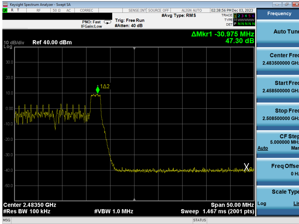
Plot 7-91. Band Edge Antenna 1a (802.11ax OFDMA – RU26 Index 8 – Ch. 12)
