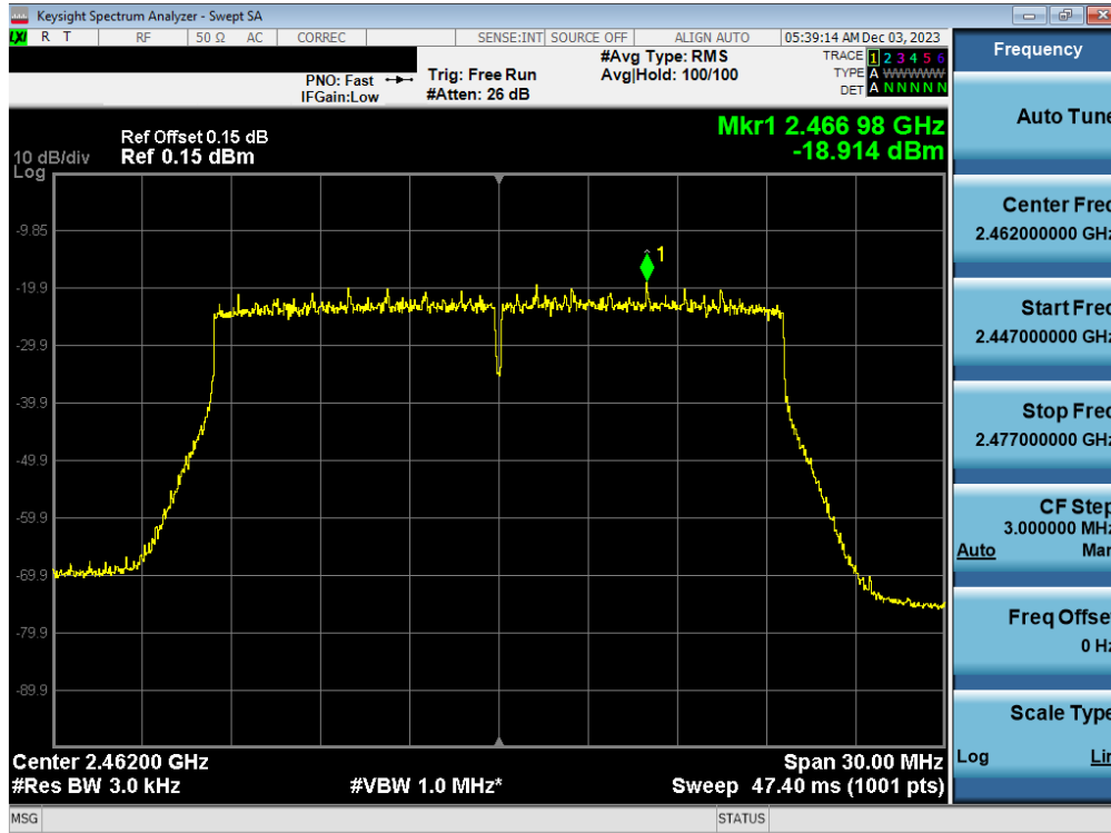
Plot 7-71. Power Spectral Density Plot Antenna 3a (802.11ax OFDMA – RU242 – Ch. 11)
