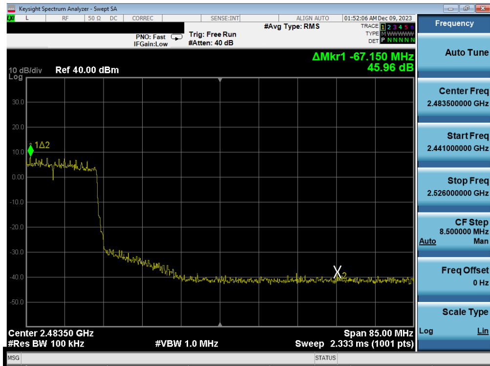
Plot 7-84. Band Edge Antenna 3a (802.11ax OFDMA – RU242 – Ch. 8)
