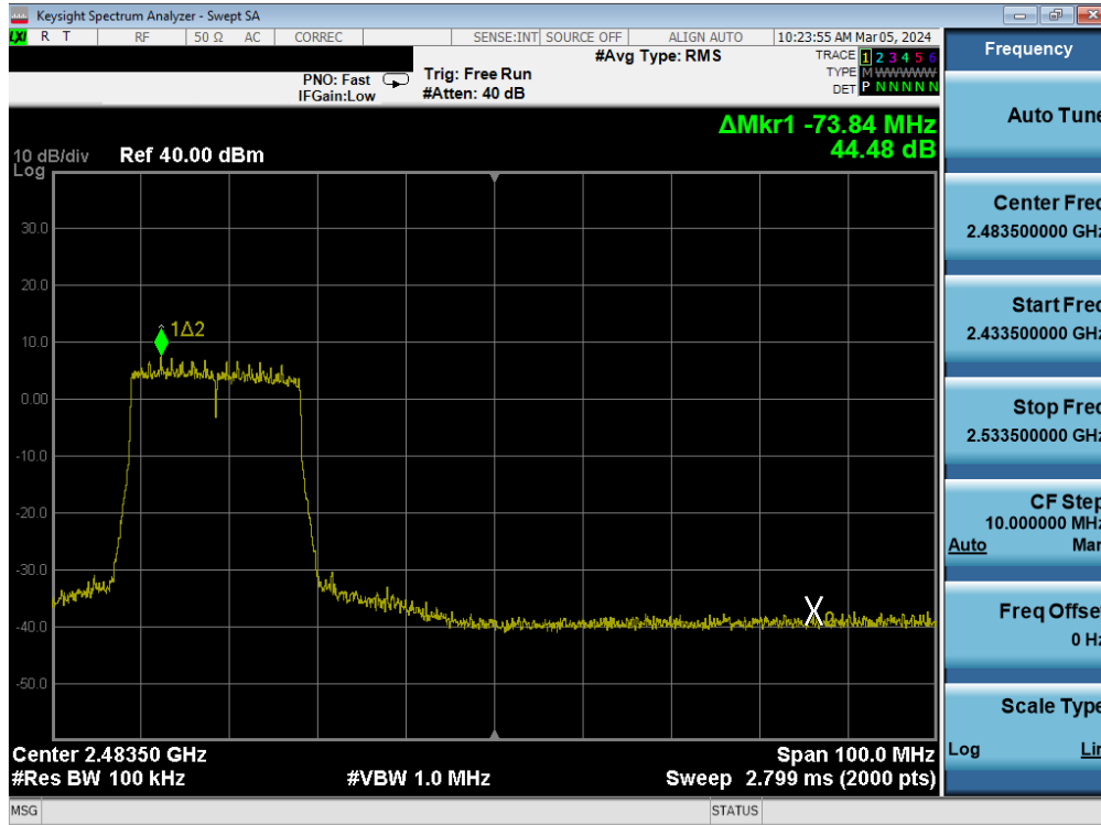
Plot 7-85. Band Edge Antenna 3a (802.11ax OFDMA - RU242 - Ch. 9)
