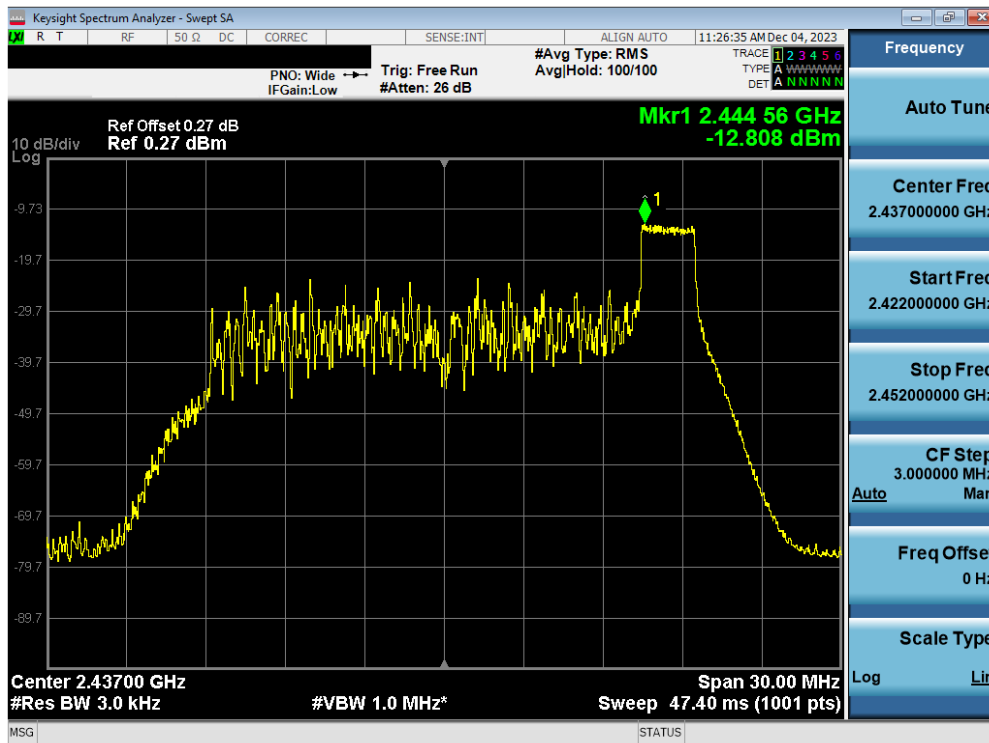
Plot 7-60. Power Spectral Density Plot Antenna 1a (802.11ax OFDMA – RU26 Index 8 – Ch. 6)
