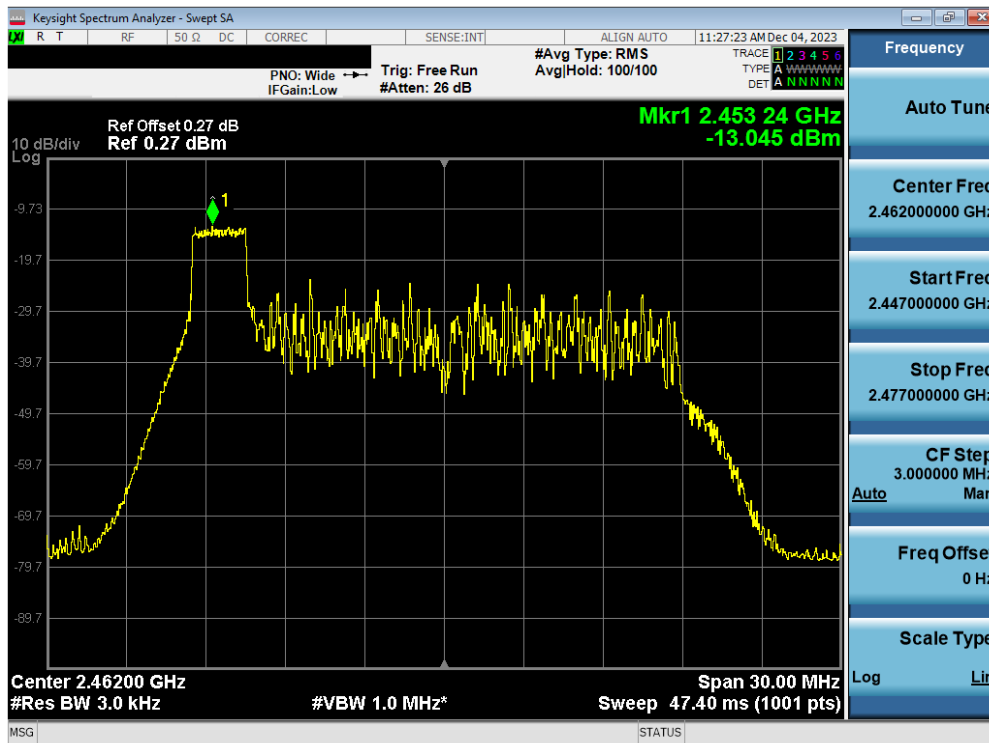
Plot 7-62. Power Spectral Density Plot Antenna 1a (802.11ax OFDMA – RU26 Index 0 – Ch. 11)
