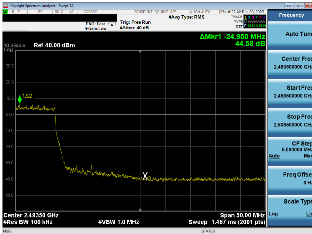
Plot 7-86. Band Edge Antenna 3a (802.11ax OFDMA - RU242 - Ch. 10)
