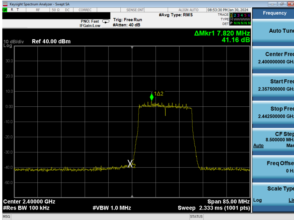
Plot 7-76. Band Edge Antenna 3a (802.11ax OFDMA – RU242 – Ch. 1)
