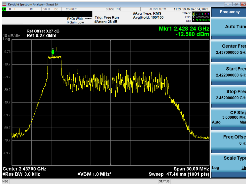
Plot 7-56. Power Spectral Density Plot Antenna 1a (802.11ax OFDMA – RU26 Index 0 – Ch. 6)
