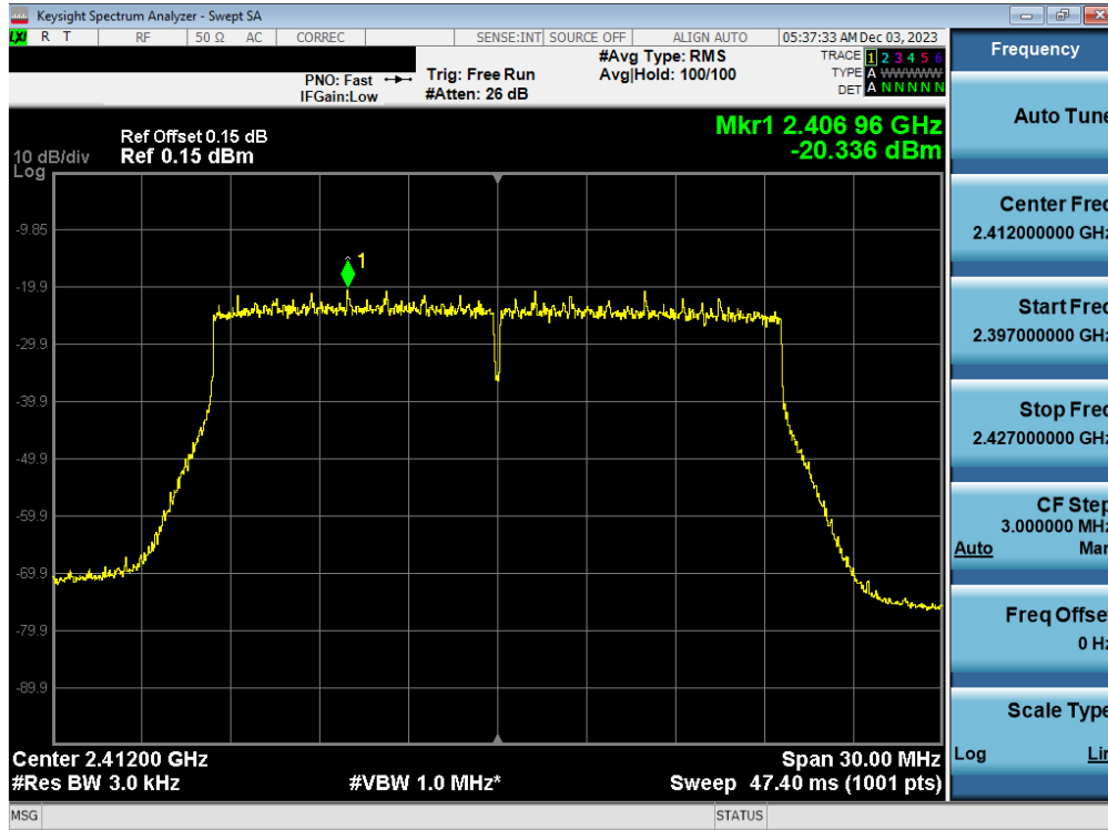
Plot 7-67. Power Spectral Density Plot Antenna 3a (802.11ax OFDMA – RU242 – Ch. 1)
