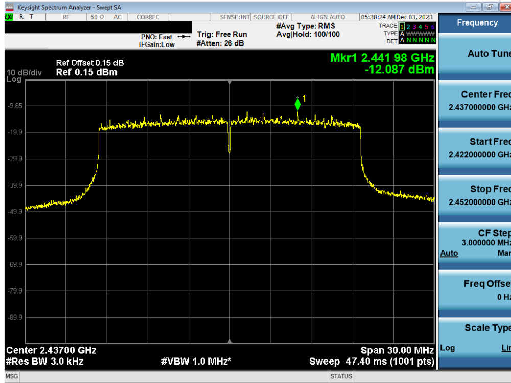
Plot 7-69. Power Spectral Density Plot Antenna 3a (802.11ax OFDMA – RU242 – Ch. 6)
