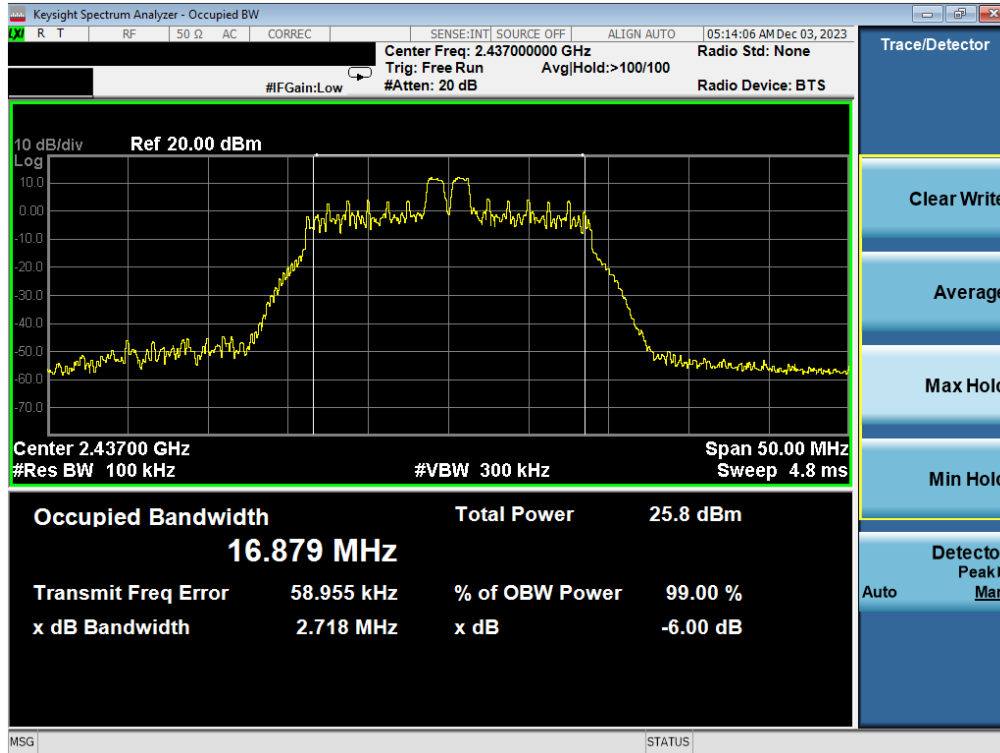
Plot 7-5. 6dB BW & 99% OBW Plot Antenna 3a (802.11ax OFDMA – RU26 Index 4 – Ch. 6)
