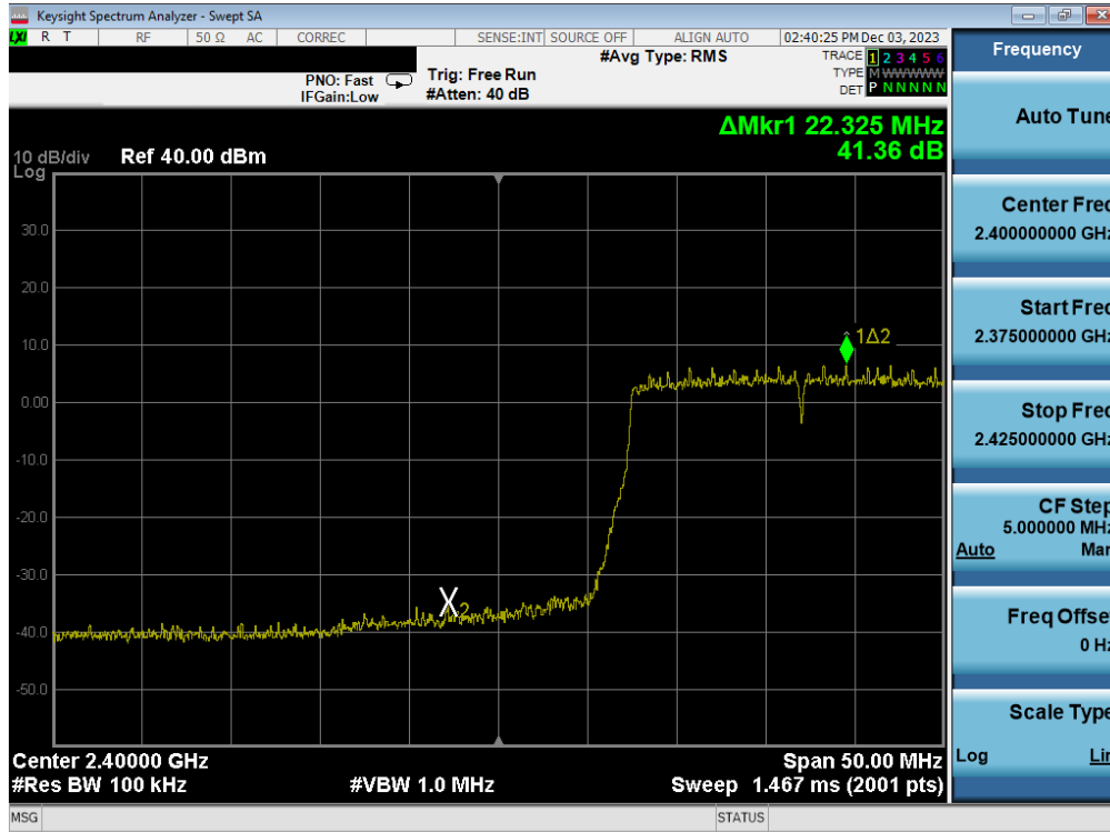
Plot 7-93. Band Edge Antenna 1a (802.11ax OFDMA – RU242 – Ch. 2)
