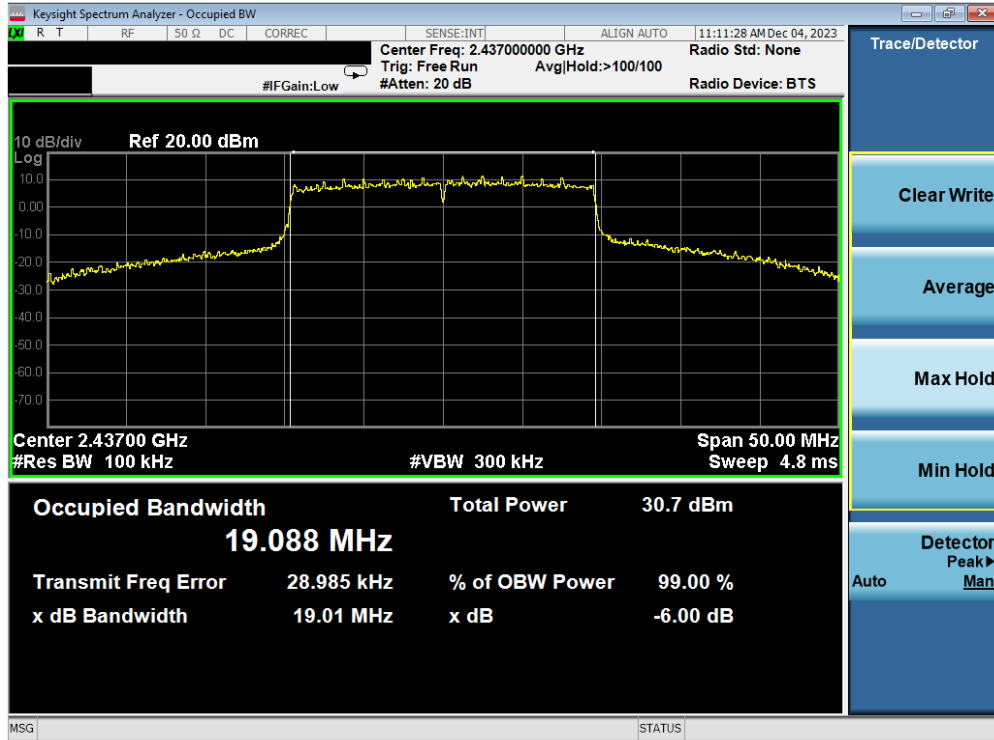
Plot 7-23. 6dB BW & 99% OBW Plot Antenna 1a (802.11ax OFDMA – RU242 – Ch. 6)
