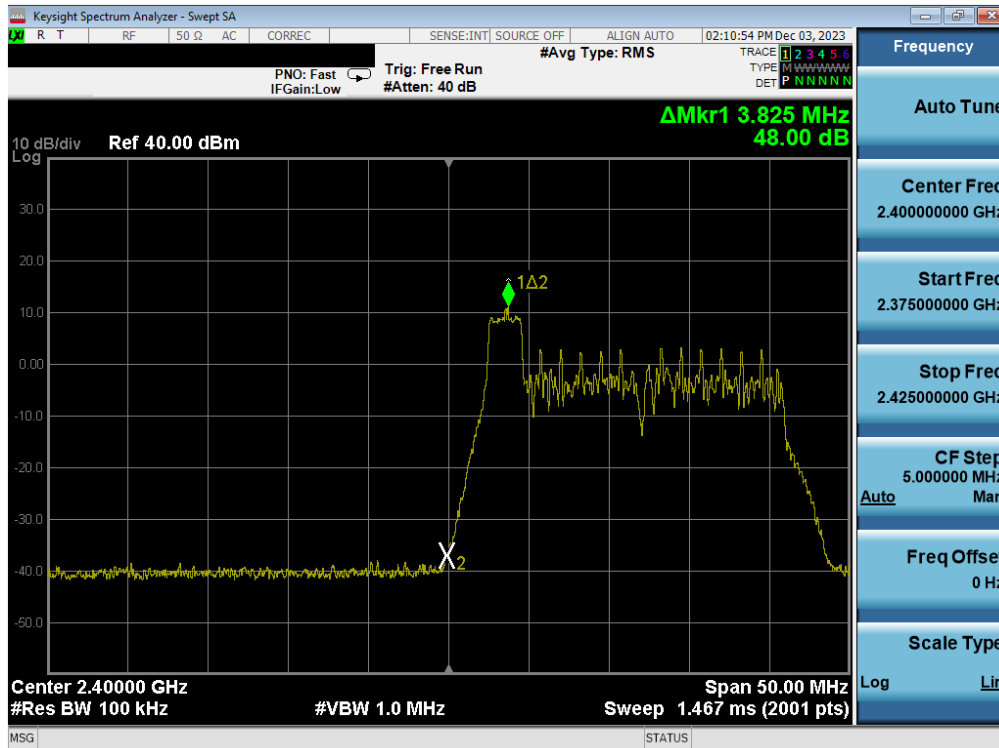
Plot 7-89. Band Edge Antenna 1a (802.11ax OFDMA – RU26 Index 0 – Ch. 1)
