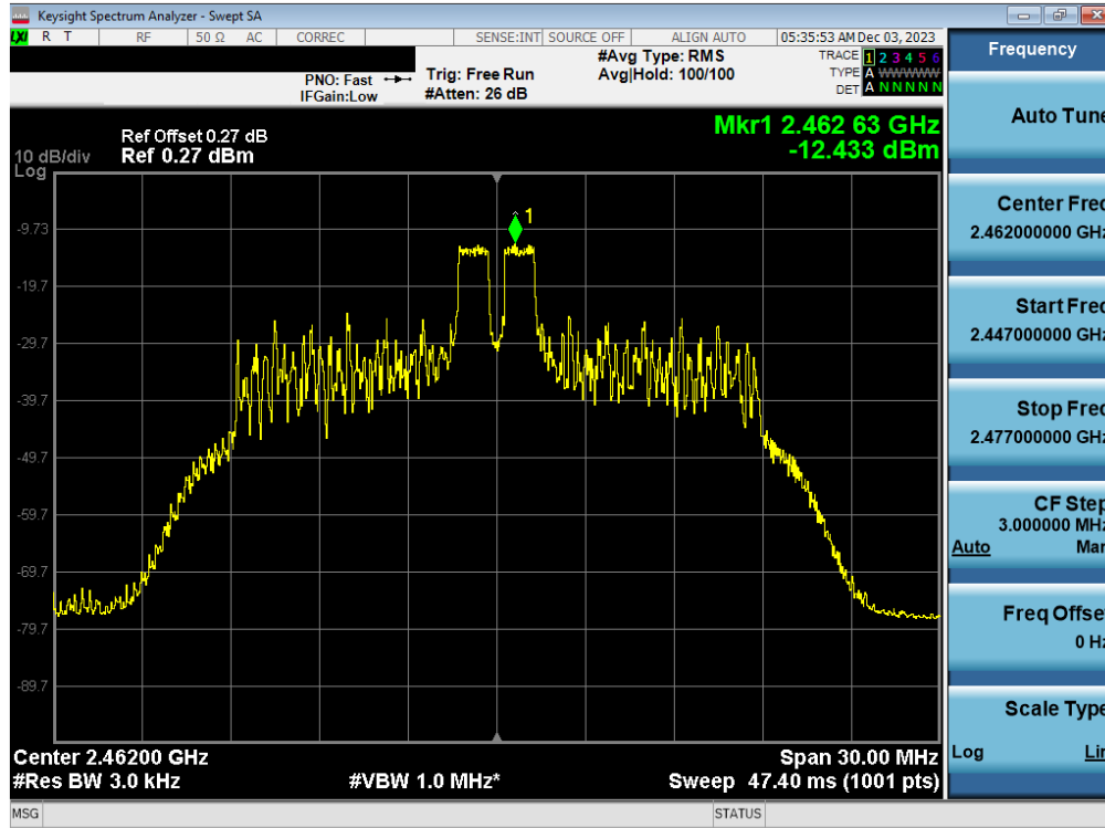
Plot 7-63. Power Spectral Density Plot Antenna 3a (802.11ax OFDMA – RU26 Index 4 – Ch. 11)
