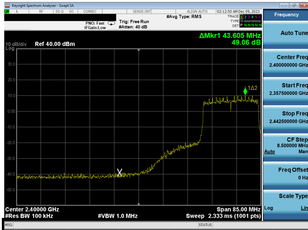
Plot 7-96. Band Edge Antenna 1a (802.11ax OFDMA – RU242 – Ch. 5)
