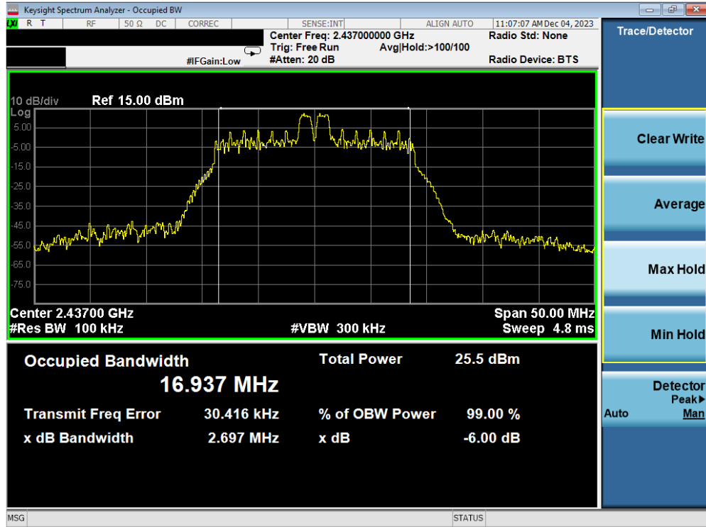
Plot 7-17. 6dB BW & 99% OBW Plot Antenna 1a (802.11ax OFDMA – RU26 Index 4 – Ch. 6)
