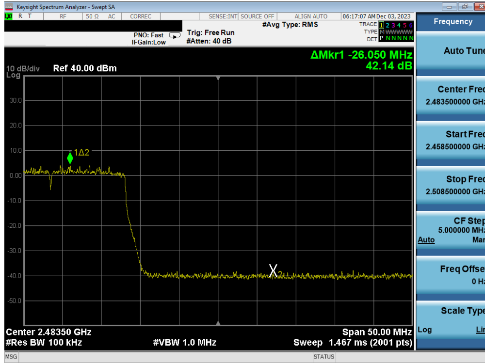
Plot 7-87. Band Edge Antenna 3a (802.11ax OFDMA – RU242 – Ch. 11)
