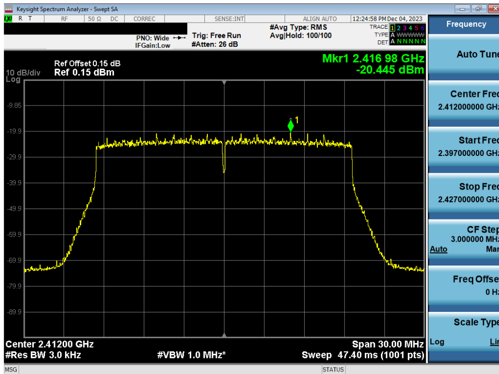
Plot 7-68. Power Spectral Density Plot Antenna 1a (802.11ax OFDMA – RU242 – Ch. 1)
