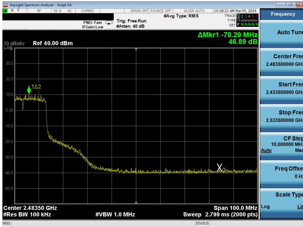
Plot 7-98. Band Edge Antenna 1a (802.11ax OFDMA – RU242 – Ch. 6(high))
