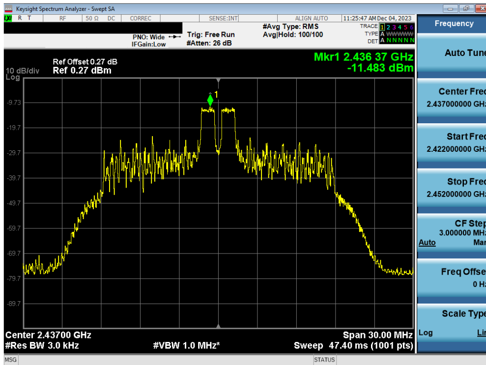
Plot 7-58. Power Spectral Density Plot Antenna 1a (802.11ax OFDMA – RU26 Index 4 – Ch. 6)
