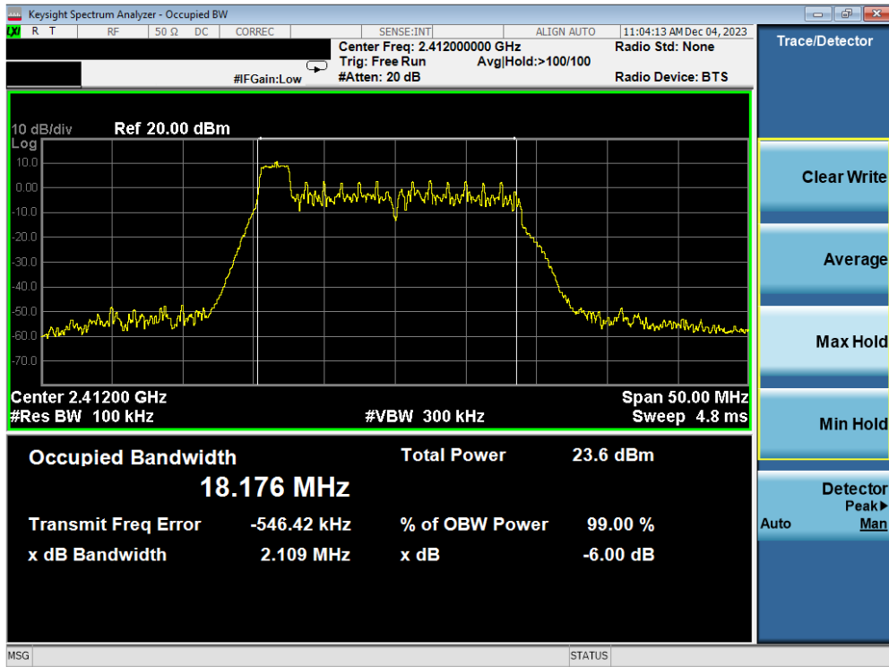
Plot 7-13. 6dB BW & 99% OBW Plot Antenna 1a (802.11ax OFDMA – RU26 Index 0 – Ch. 1)
