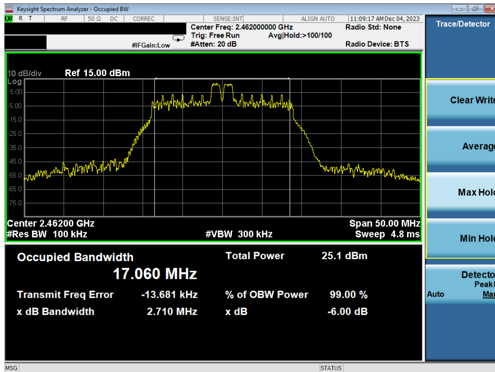
Plot 7-20. 6dB BW & 99% OBW Antenna 1a (802.11ax OFDMA – RU26 Index 4 – Ch. 11)
