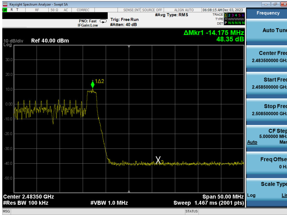
Plot 7-75. Band Edge Antenna 3a (802.11ax OFDMA – RU26 Index 8 – Ch. 12)
