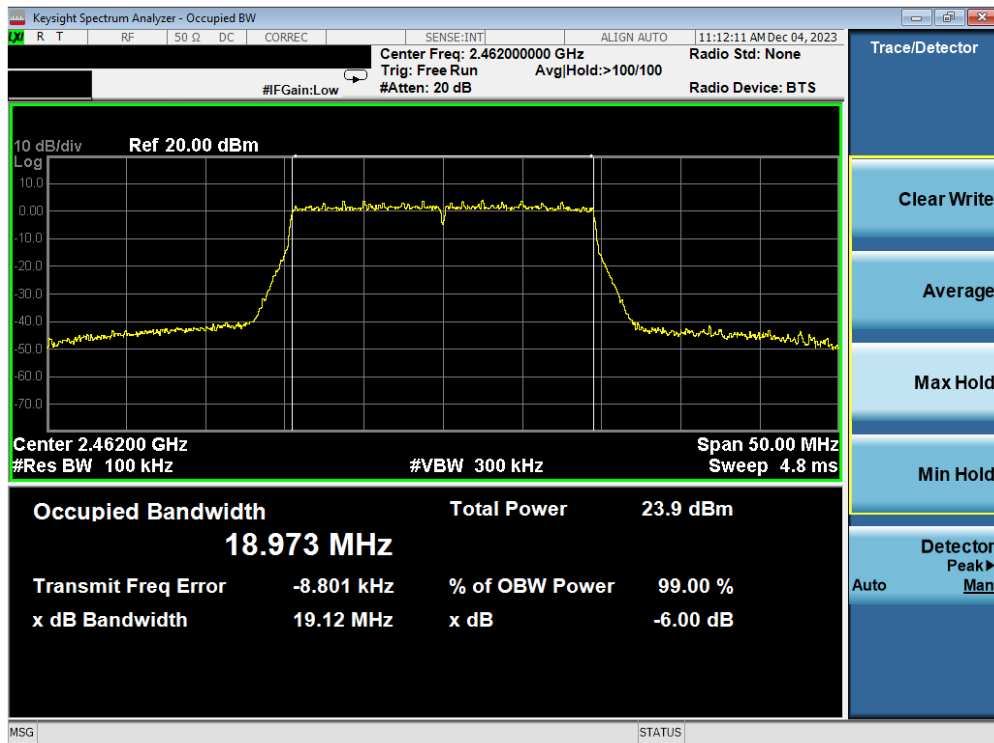
Plot 7-24. 6dB BW & 99% OBW Plot Antenna 1a (802.11ax OFDMA – RU242 – Ch. 11)
