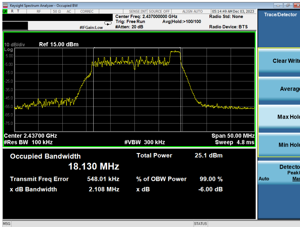
Plot 7-6. 6dB BW & 99% OBW Antenna 3a (802.11ax OFDMA – RU26 Index 8 – Ch. 6)
