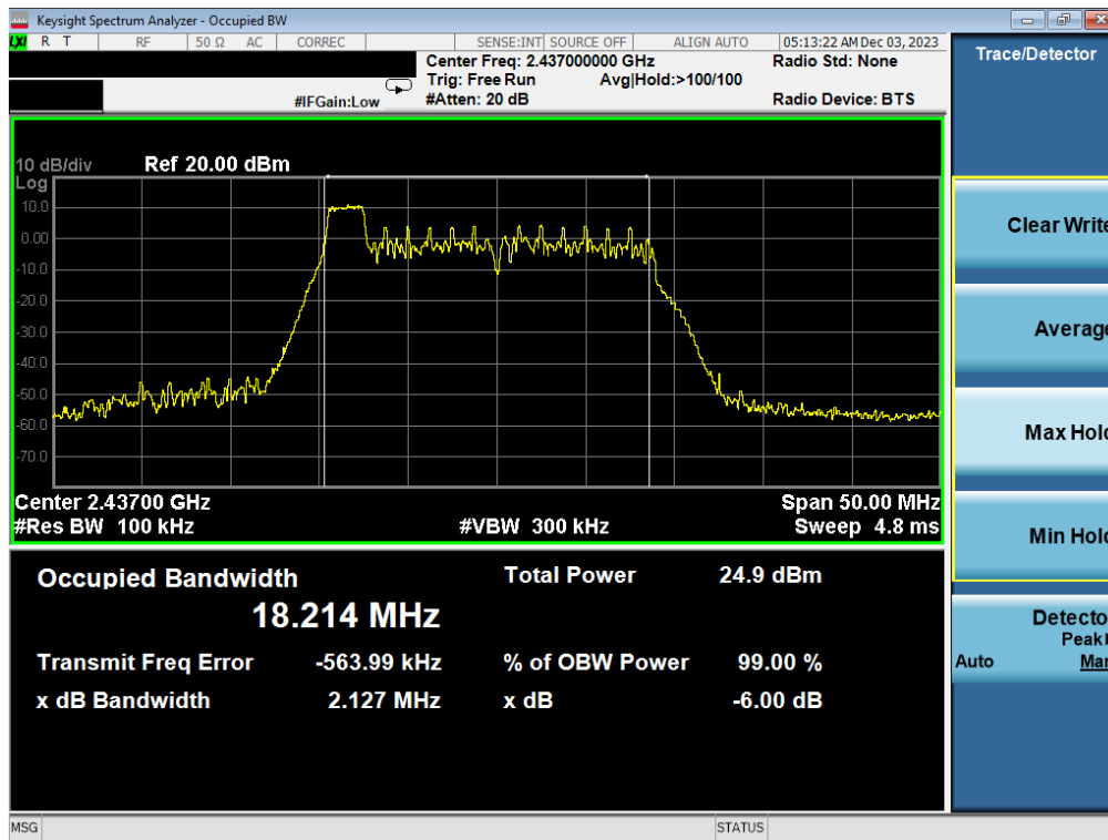
Plot 7-4. 6dB BW & 99% OBW Plot Antenna 3a (802.11ax OFDMA – RU26 Index 0 – Ch. 6)
