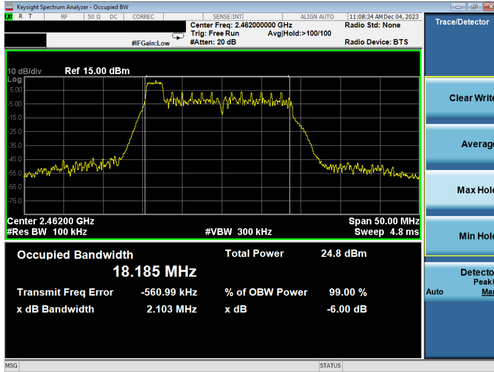
Plot 7-19. 6dB BW & 99% OBW Antenna 1a (802.11ax OFDMA – RU26 Index 0 – Ch. 11)
