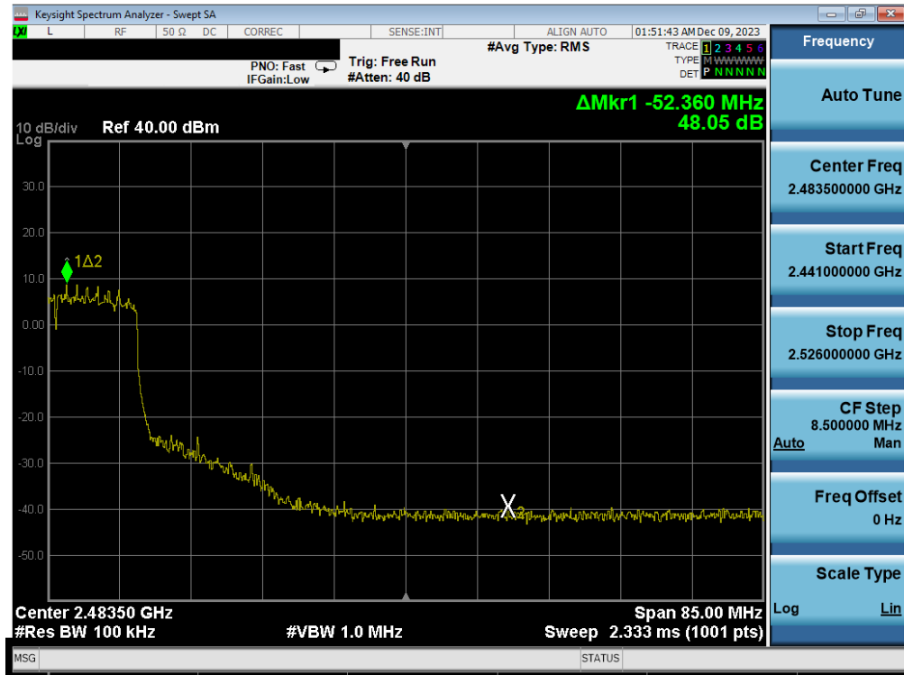
Plot 7-83. Band Edge Antenna 3a (802.11ax OFDMA – RU242 – Ch. 7)
