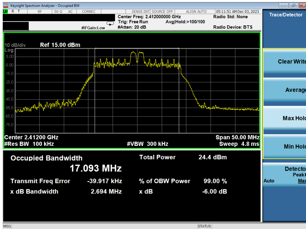
Plot 7-2. 6dB BW & 99% OBW Plot Antenna 3a (802.11ax OFDMA – RU26 Index 4 – Ch. 1)
