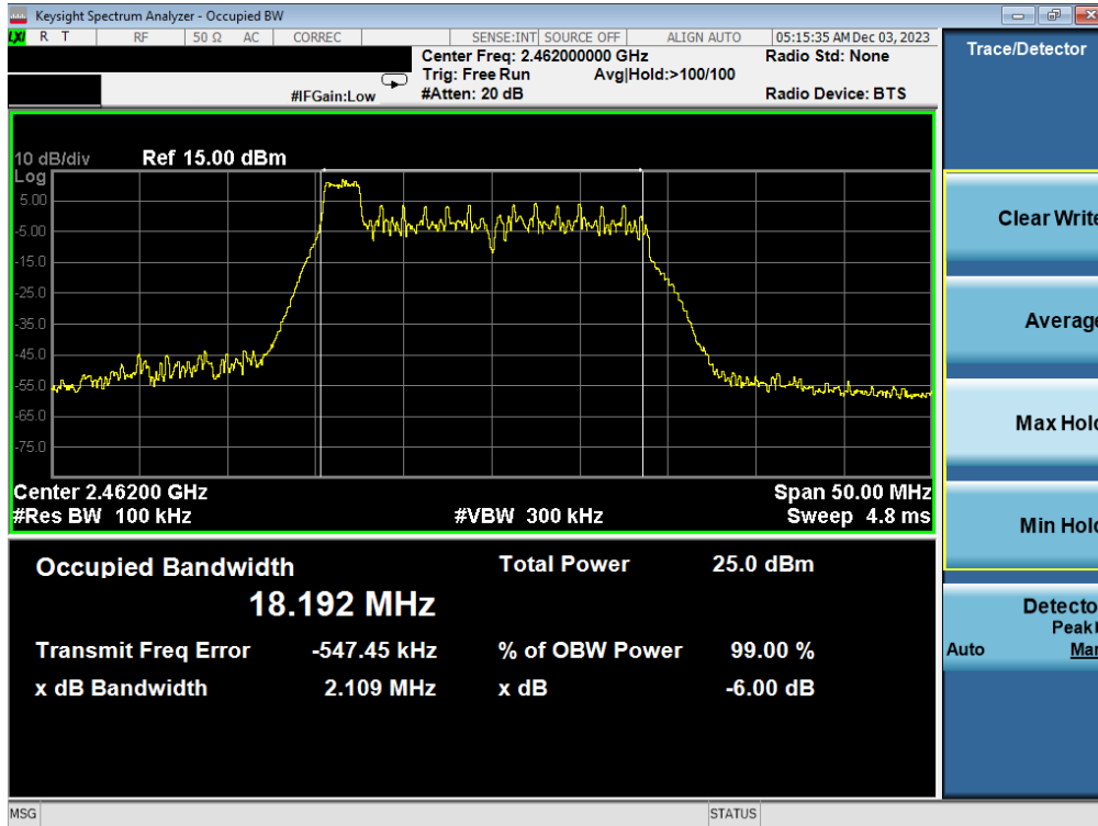
Plot 7-7. 6dB BW & 99% OBW Antenna 3a (802.11ax OFDMA – RU26 Index 0 – Ch. 11)
