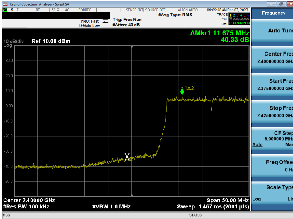
Plot 7-77. Band Edge Antenna 3a (802.11ax OFDMA – RU242 – Ch. 2)
