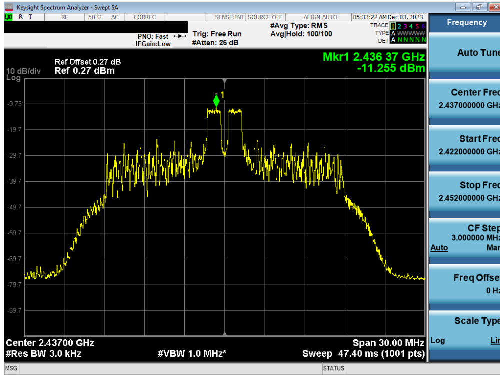
Plot 7-57. Power Spectral Density Plot Antenna 3a (802.11ax OFDMA – RU26 Index 4 – Ch. 6)
