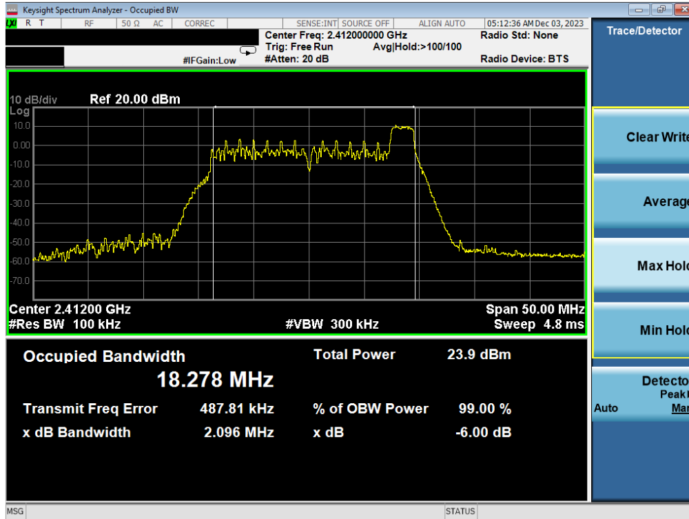
Plot 7-3. 6dB BW & 99% OBW Plot Antenna 3a (802.11ax OFDMA – RU26 Index 8 – Ch. 1)
