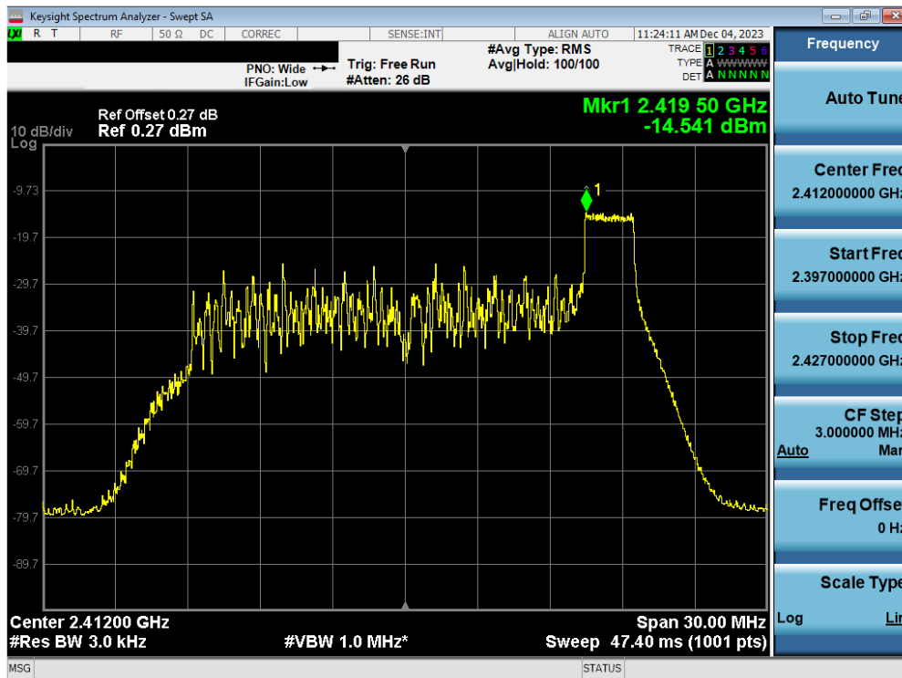
Plot 7-54. Power Spectral Density Plot Antenna 1a (802.11ax OFDMA – RU26 Index 8 – Ch. 1)
