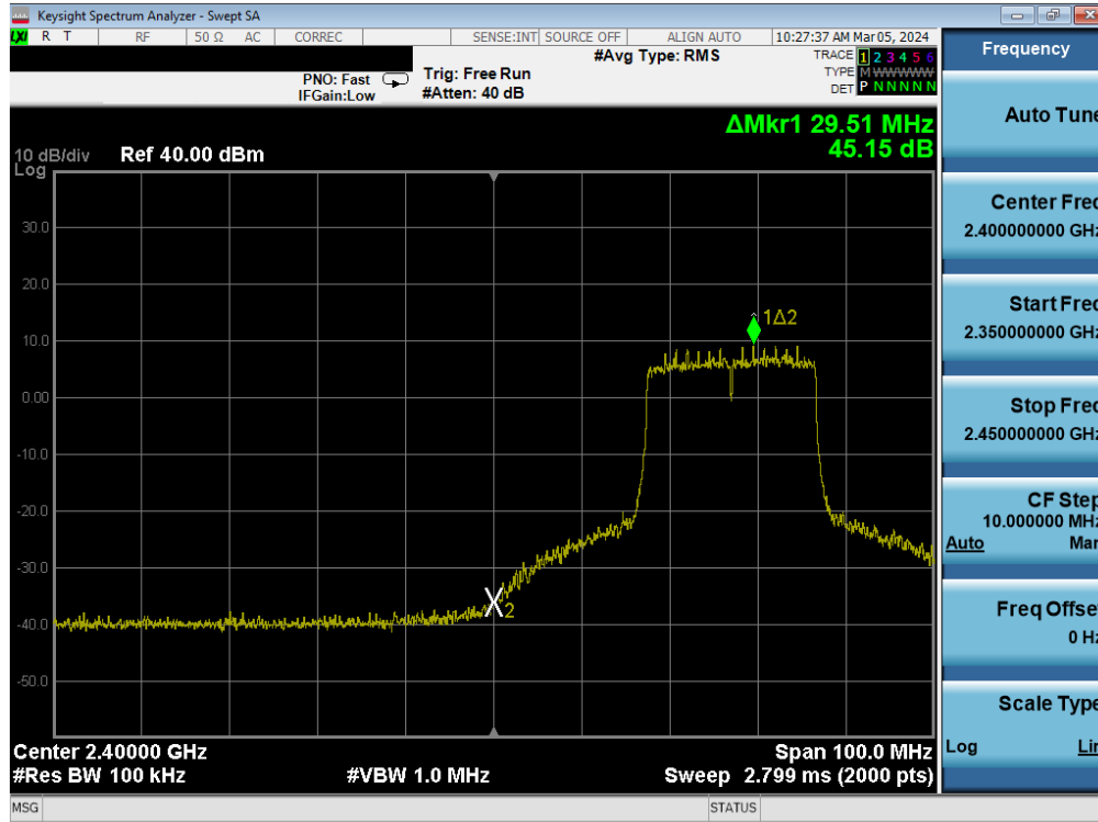
Plot 7-95. Band Edge Antenna 1a (802.11ax OFDMA – RU242 – Ch. 4)
