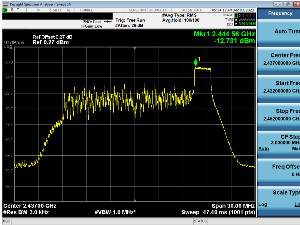
Plot 7-59. Power Spectral Density Plot Antenna 3a (802.11ax OFDMA – RU26 Index 8 – Ch. 6)
