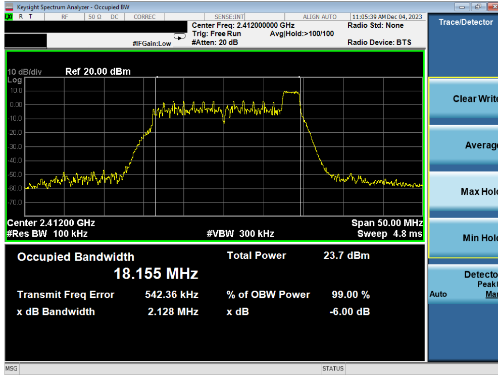
Plot 7-15. 6dB BW & 99% OBW Plot Antenna 1a (802.11ax OFDMA – RU26 Index 8 – Ch. 1)
