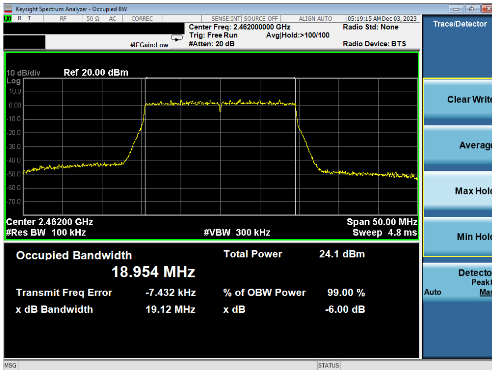
Plot 7-12. 6dB BW & 99% OBW Plot Antenna 3a (802.11ax OFDMA – RU242 – Ch. 11)
