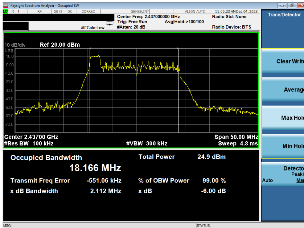
Plot 7-16. 6dB BW & 99% OBW Plot Antenna 1a (802.11ax OFDMA – RU26 Index 0 – Ch. 6)
