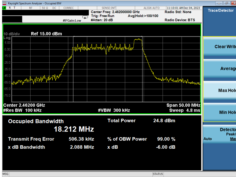
Plot 7-21. 6dB BW & 99% OBW Plot Antenna 1a (802.11ax OFDMA – RU26 Index 8 – Ch. 11)
