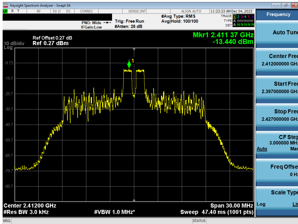
Plot 7-52. Power Spectral Density Plot Antenna 1a (802.11ax OFDMA – RU26 Index 4 – Ch. 1)
