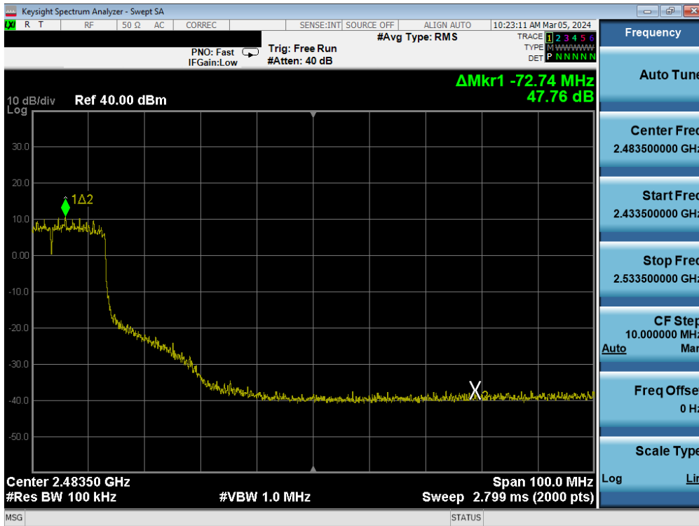
Plot 7-82. Band Edge Antenna 3a (802.11ax OFDMA – RU242 – Ch. 6(high))
