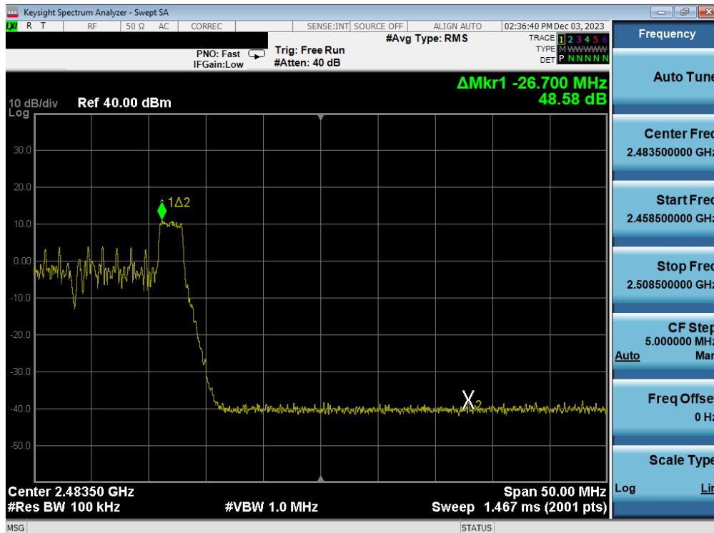
Plot 7-90. Band Edge Antenna 1a (802.11ax OFDMA – RU26 Index 8 – Ch. 11)
