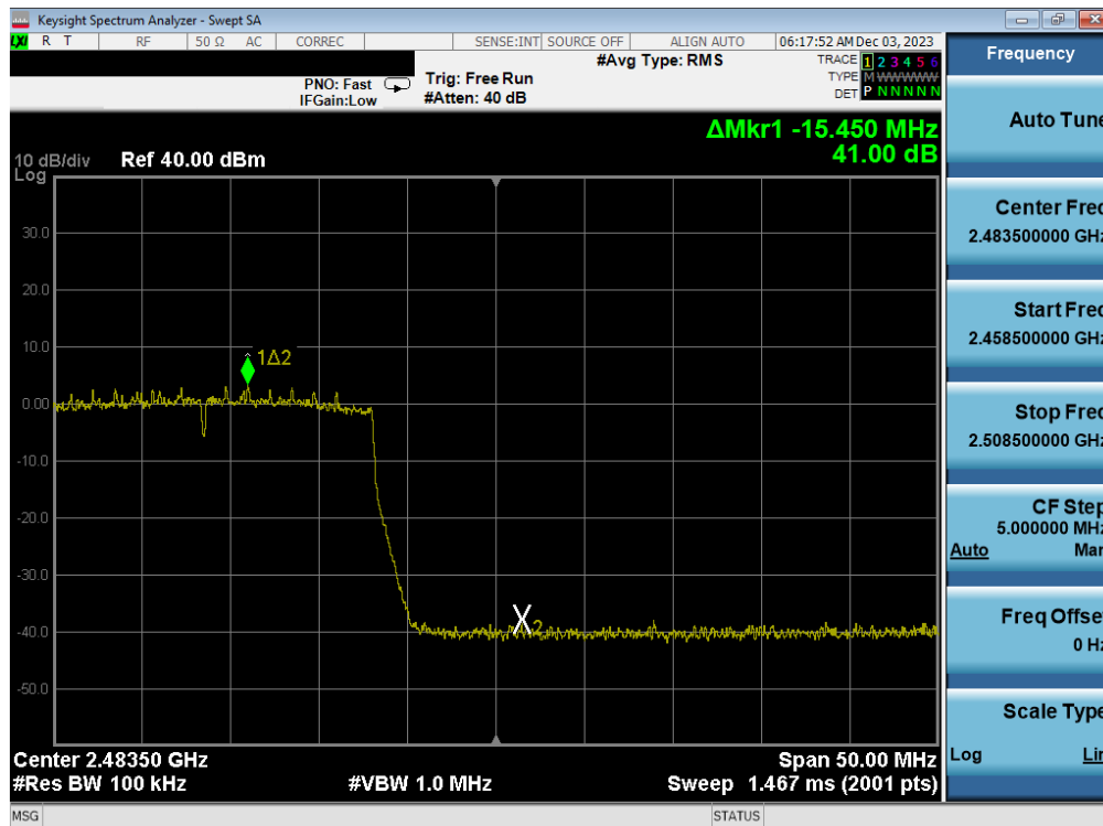
Plot 7-88. Band Edge Antenna 3a (802.11ax OFDMA – RU242 – Ch. 12)
