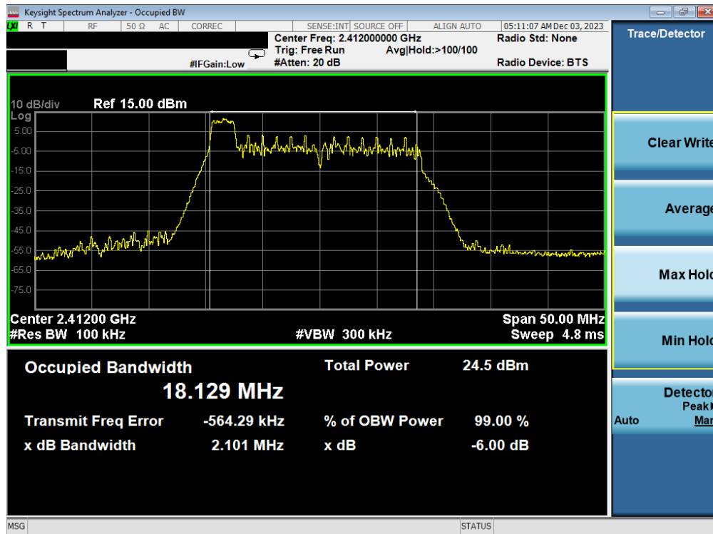
Plot 7-1. 6dB BW & 99% OBW Plot Antenna 3a (802.11ax OFDMA – RU26 Index 0 – Ch. 1)
