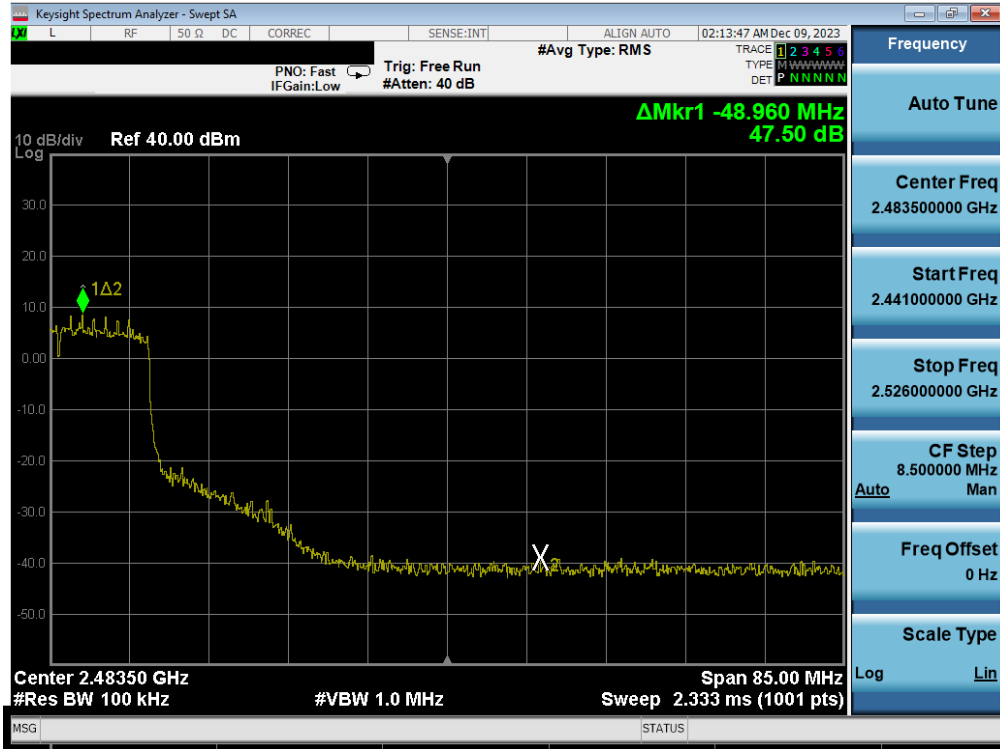
Plot 7-99. Band Edge Antenna 1a (802.11ax OFDMA – RU242 – Ch. 7)
