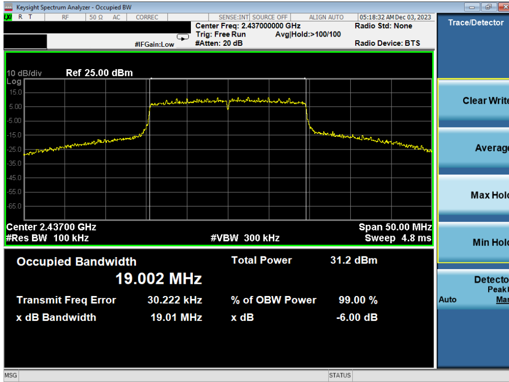
Plot 7-11. 6dB BW & 99% OBW Plot Antenna 3a (802.11ax OFDMA – RU242 – Ch. 6)
