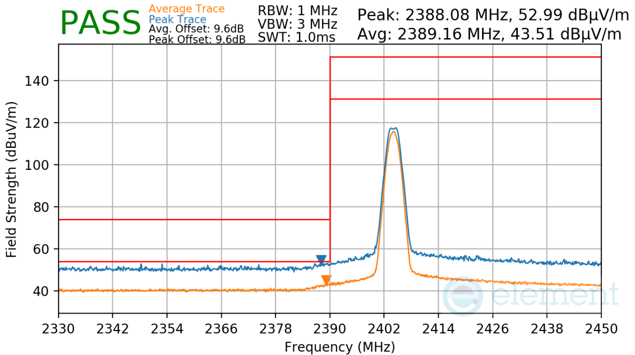
Plot 7-93. Radiated Restricted Lower Band Edge Measurement Antenna 3a (Average & Peak)
