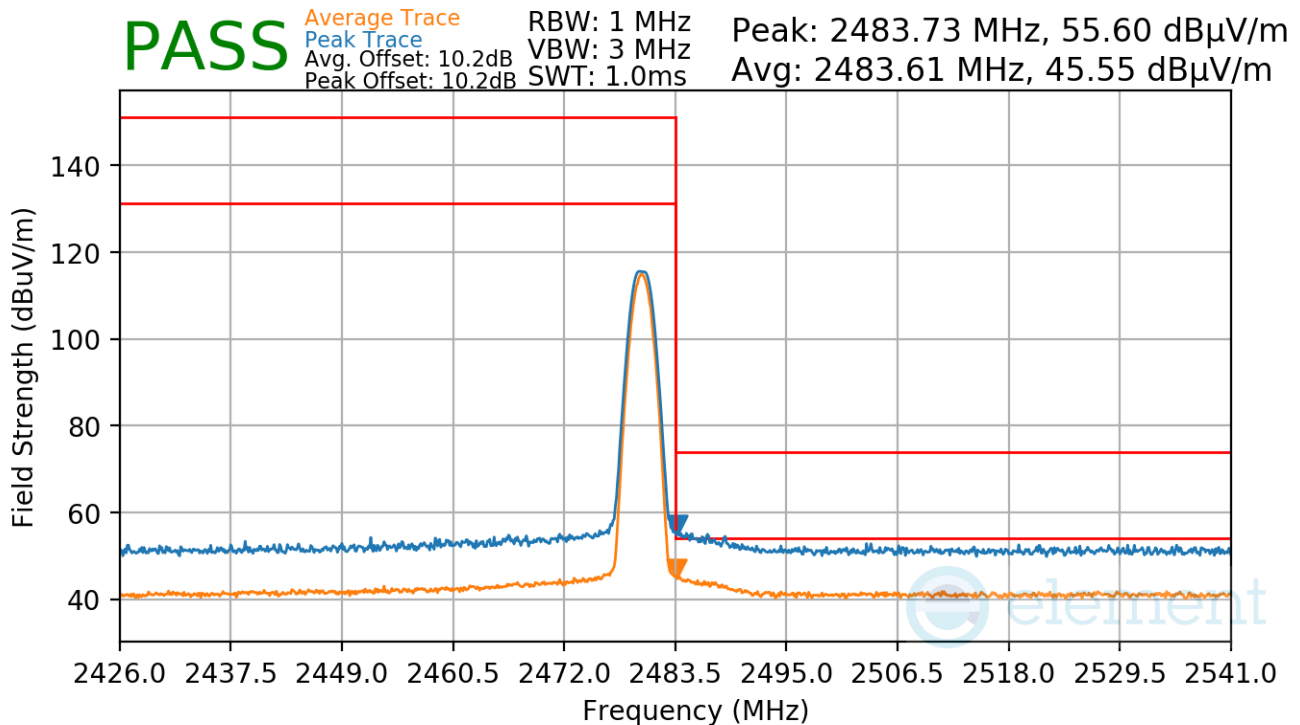
Plot 7-96. Radiated Restricted Upper Band Edge Measurement Antenna 1a (Average & Peak)
