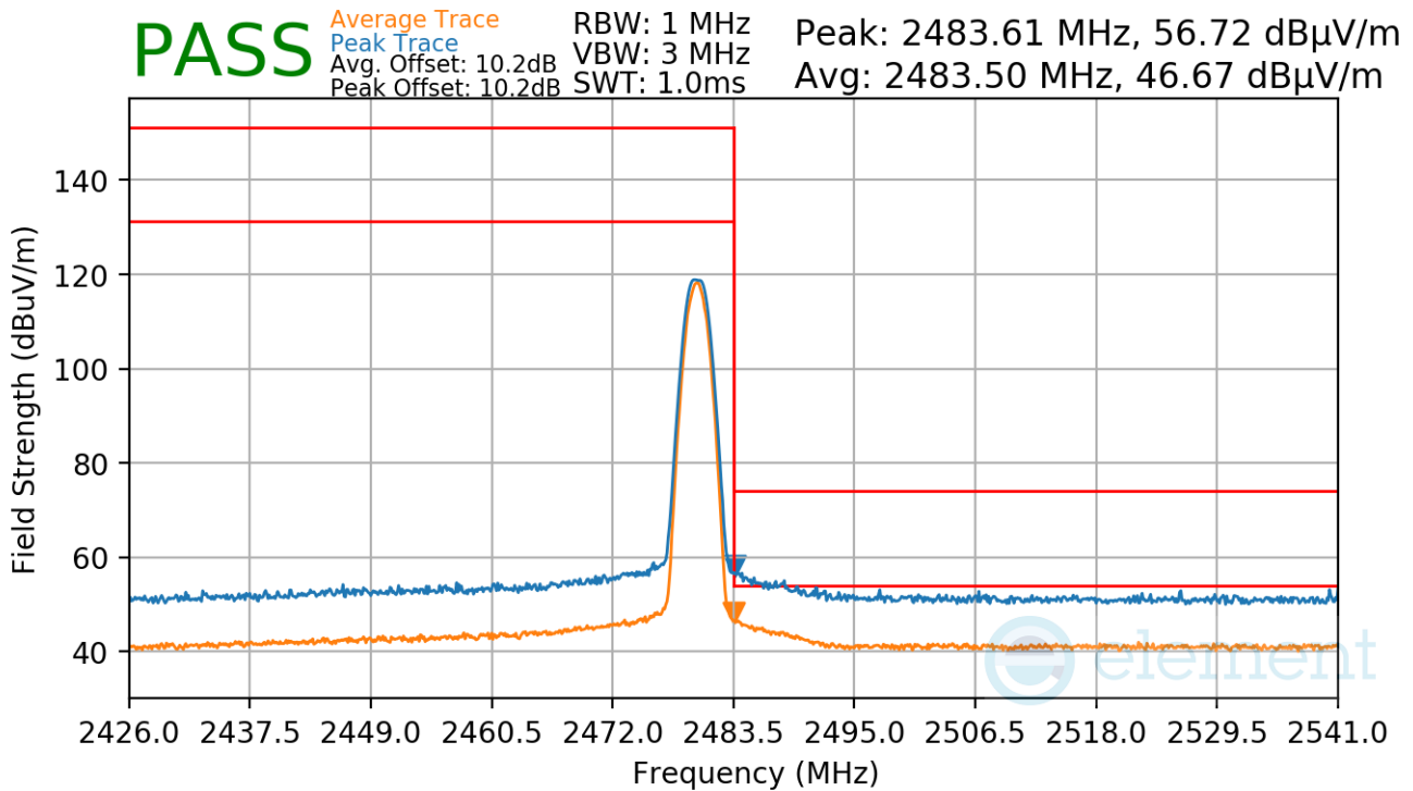
Plot 7-92. Radiated Restricted Upper Band Edge Measurement Antenna 3a (Average & Peak)
