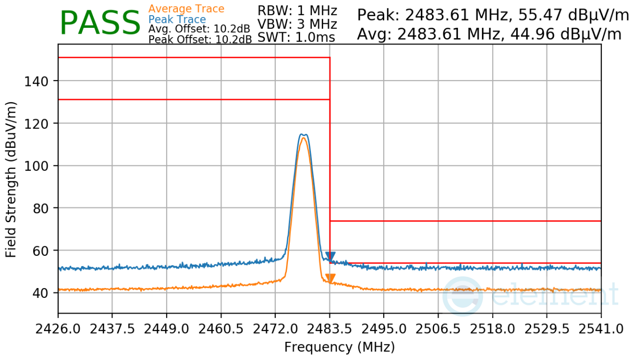
Plot 7-98. Radiated Restricted Upper Band Edge Measurement Antenna 1a (Average & Peak)
