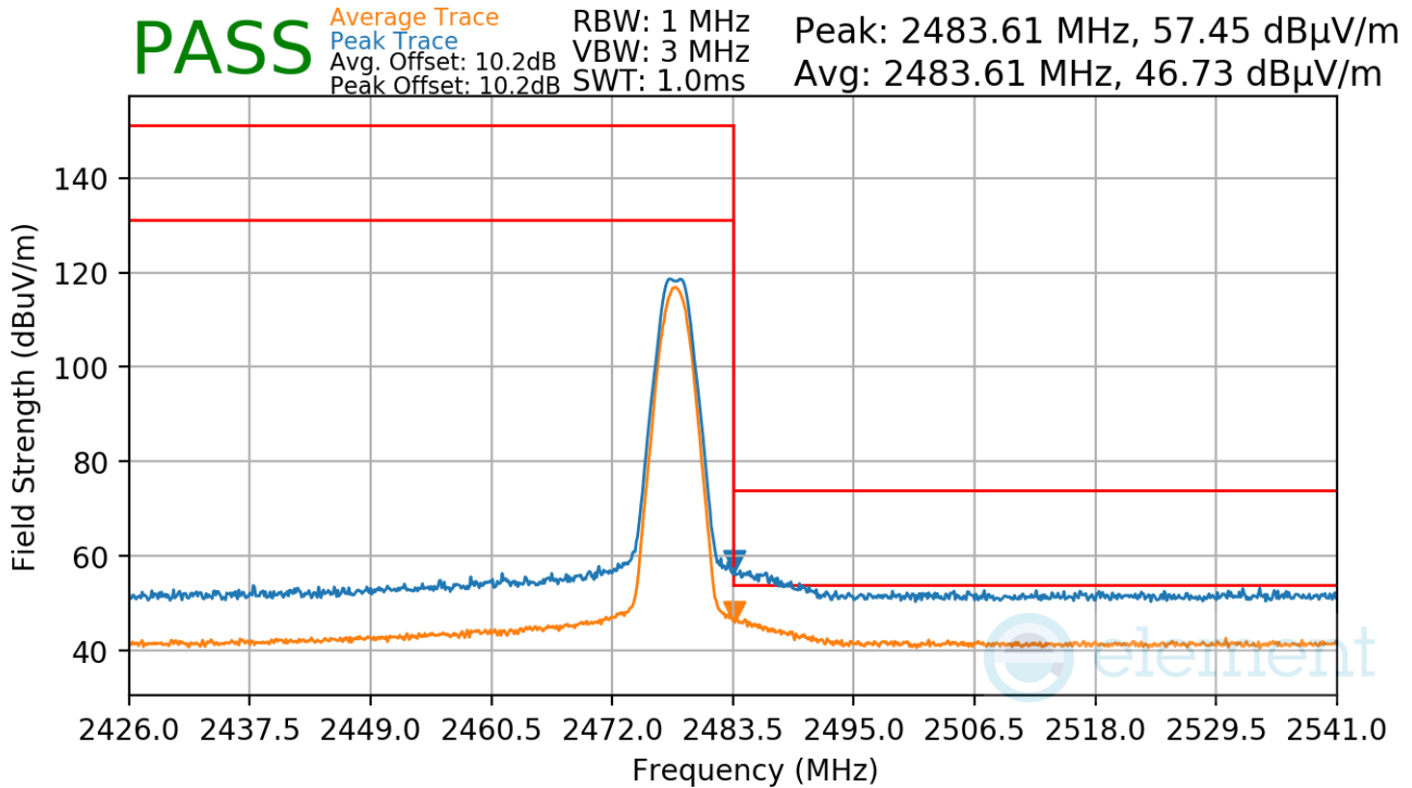
Plot 7-94. Radiated Restricted Upper Band Edge Measurement Antenna 3a (Average & Peak)
