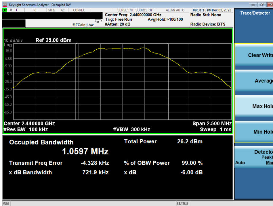
Plot 7-8. 6dB BW & 99% OBW Plot Antenna 1a (Bluetooth (LE), 1Mbps, ePA – Ch. 19)
