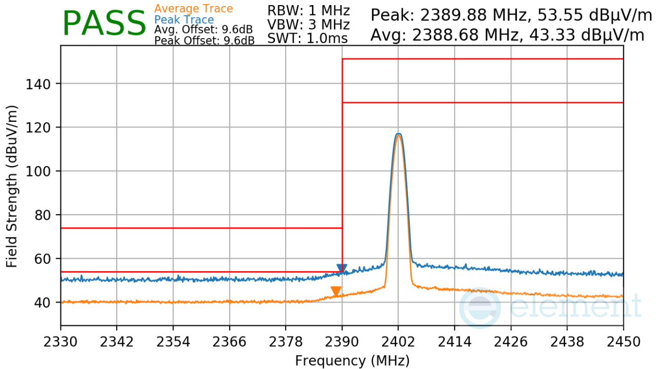
Plot 7-91. Radiated Restricted Lower Band Edge Measurement Antenna 3a (Average & Peak)
