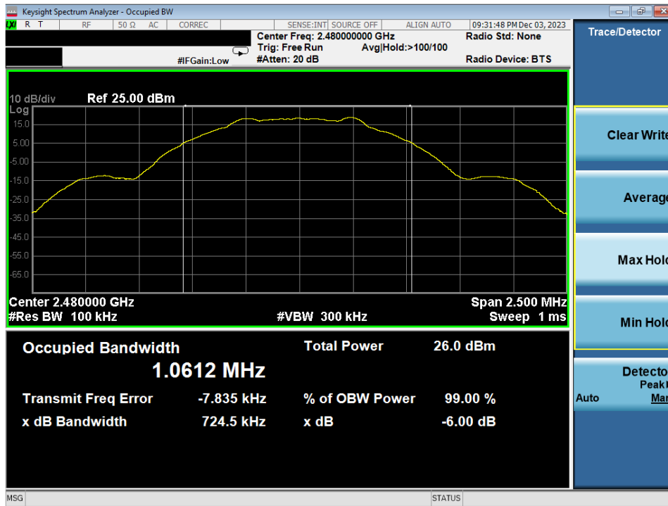
Plot 7-9. 6dB BW & 99% OBW Plot Antenna 1a (Bluetooth (LE), 1Mbps, ePA – Ch. 39)
