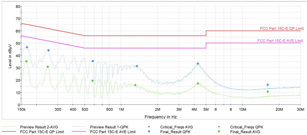
Plot 7-104. AC Line Conducted Plot with Bluetooth HDR Tx BF (L1, 4Mbps ePA - Ch.38 with AC/DC Adapter)
