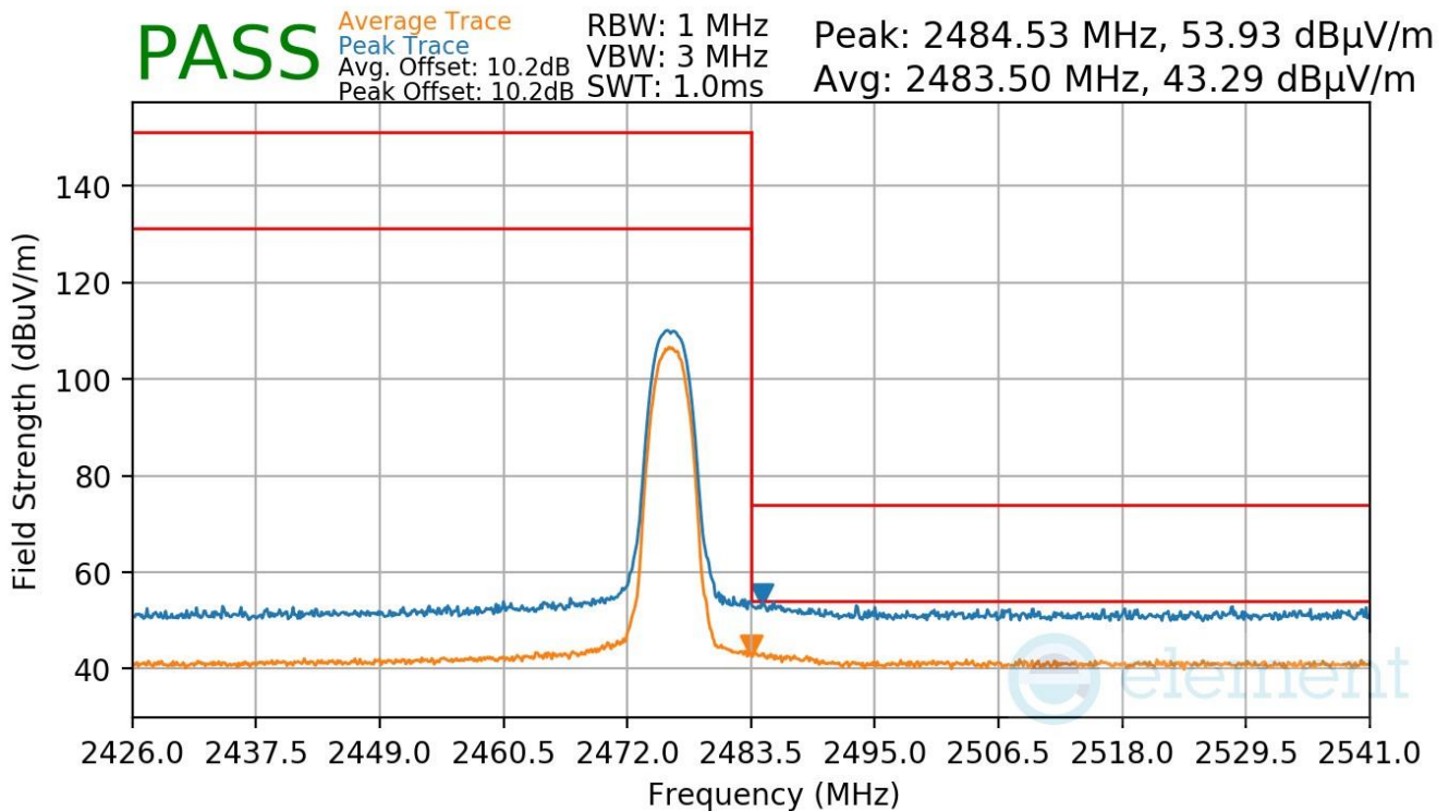
Plot 7-97. Radiated Restricted Upper Band Edge Measurement Antenna 1a
