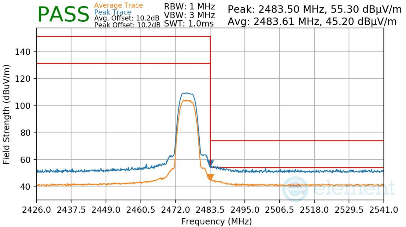
Plot 7-98. Radiated Restricted Upper Band Edge Measurement Antenna 1a
