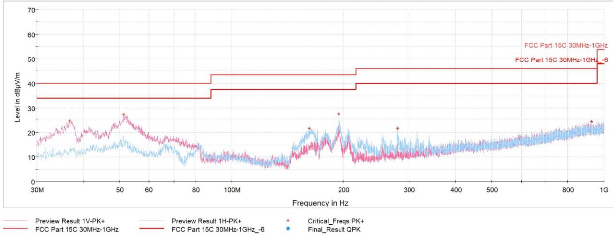
Plot 7-103. Radiated Spurious Emissions Below 1GHz TxBF (4Mbps, ePA – Ch.38 with AC/DC Adapter)
