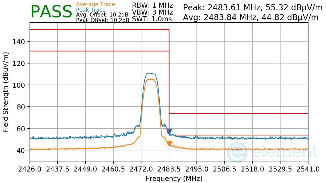
Plot 7-102. Radiated Restricted Upper Band Edge Measurement TxBF
