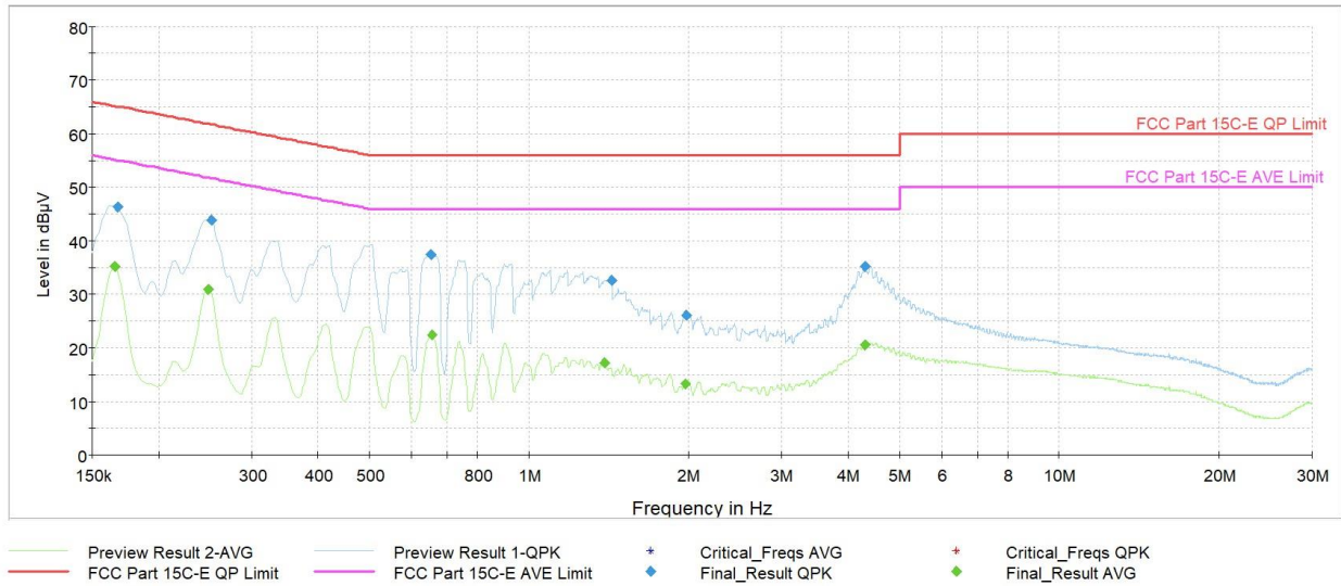
Plot 7-105. AC Line Conducted Plot with Bluetooth HDR (N, 4Mbps ePA - Ch.38 with AC/DC Adapter)
