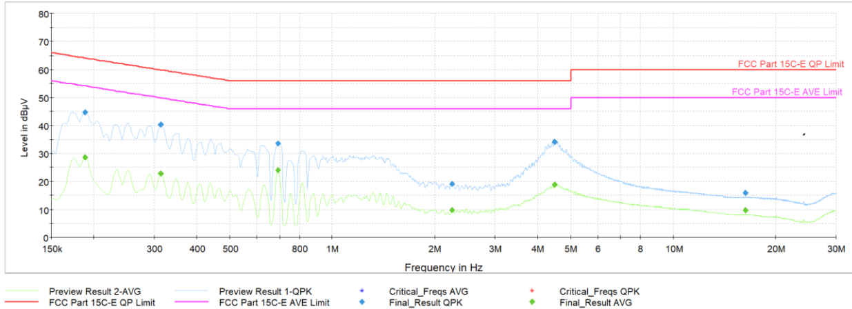
Plot 7-48. AC Line Conducted Emission with 802.15.4 (N, ePA Ch.11, Antenna 3a with AC/DC Adapter)
