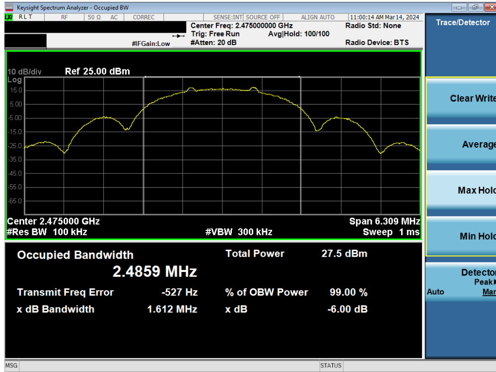
Plot 7-6. 6dB BW & 99% OBW Antenna 1a(802.15.4, Ch. 25)
