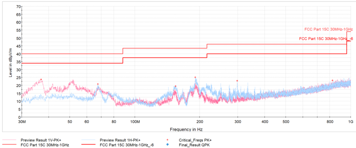
Plot 7-46. Radiated Spurious Emissions 30MHz-1GHz (ePA, Ch.11, Antenna 3a with AC/DC Adapter)
