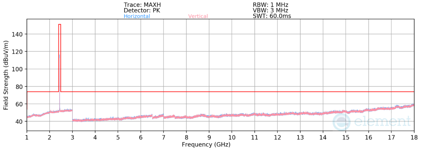
Plot 7-36. Radiated Spurious Emissions 1-18GHz Antenna 3a (802.15.4, ePA – Ch. 18)
