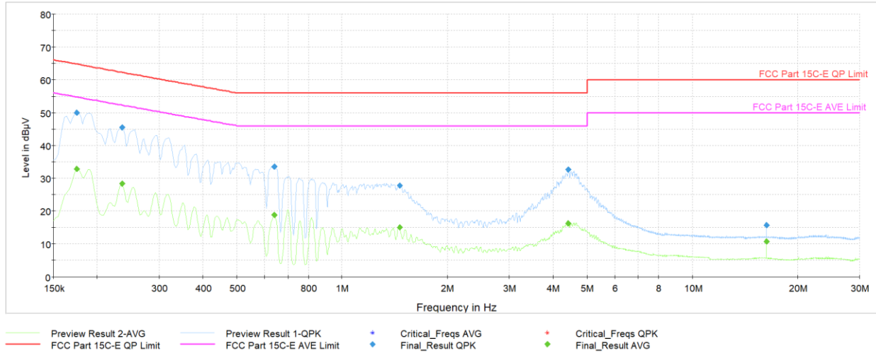
Plot 7-47. AC Line Conducted Emission with 802.15.4 (L1, ePA, Ch.11, Antenna 3a with AC/DC Adapter)
