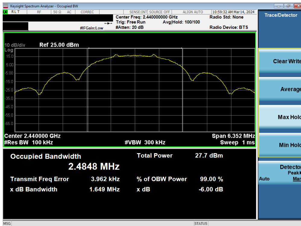
Plot 7-5. 6dB BW & 99% OBW Antenna 1a (802.15.4, Ch. 18)
