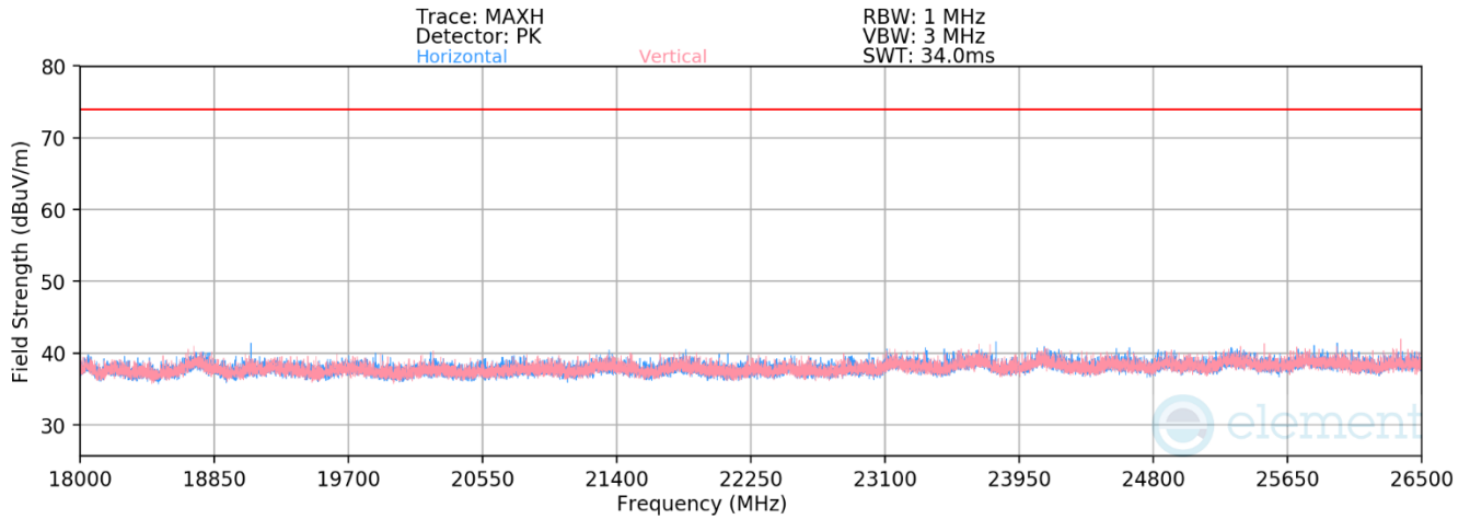
Plot 7-41. Radiated Spurious Emissions (802.15.4, ePA – Ch.11, Antenna 3a)
