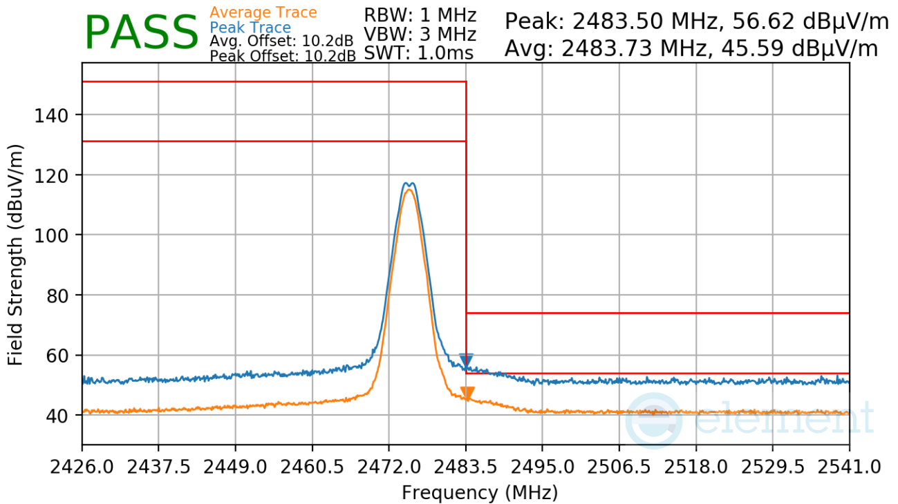
Plot 7-43. Radiated Restricted Upper Band Edge Measurement Antenna 3a
