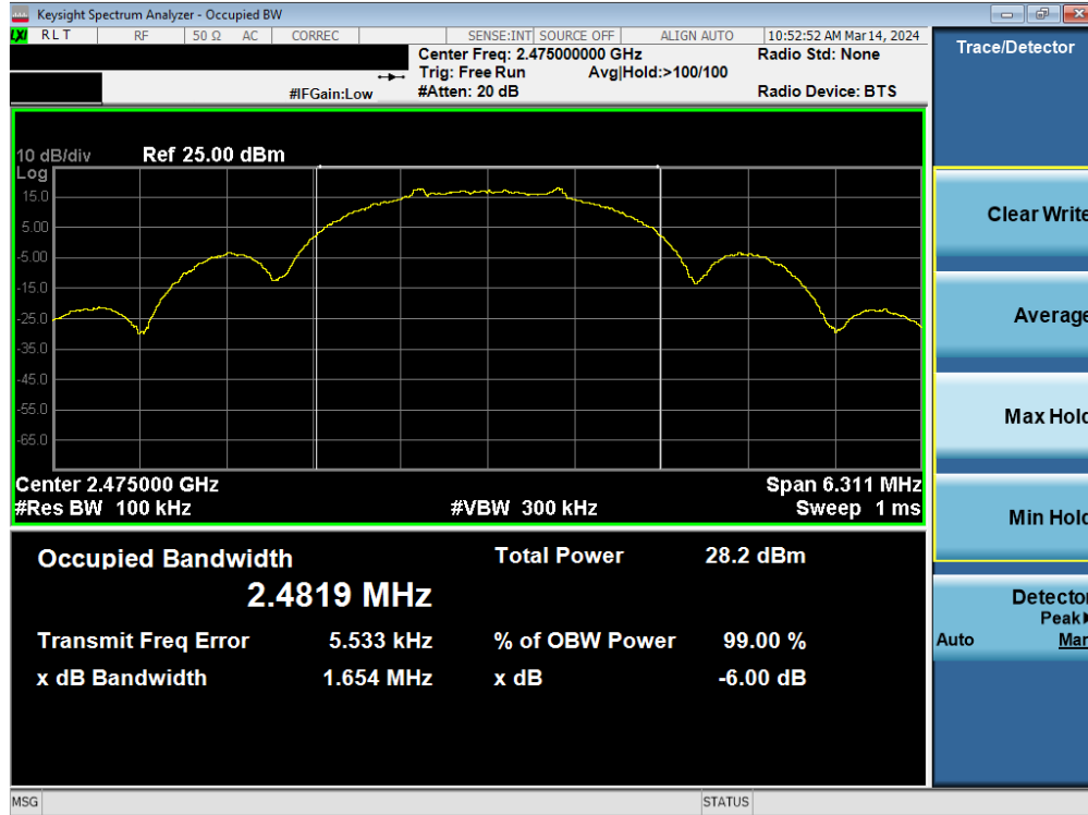
Plot 7-3. 6dB BW & 99% OBW Antenna 3a (802.15.4, Ch. 25)
