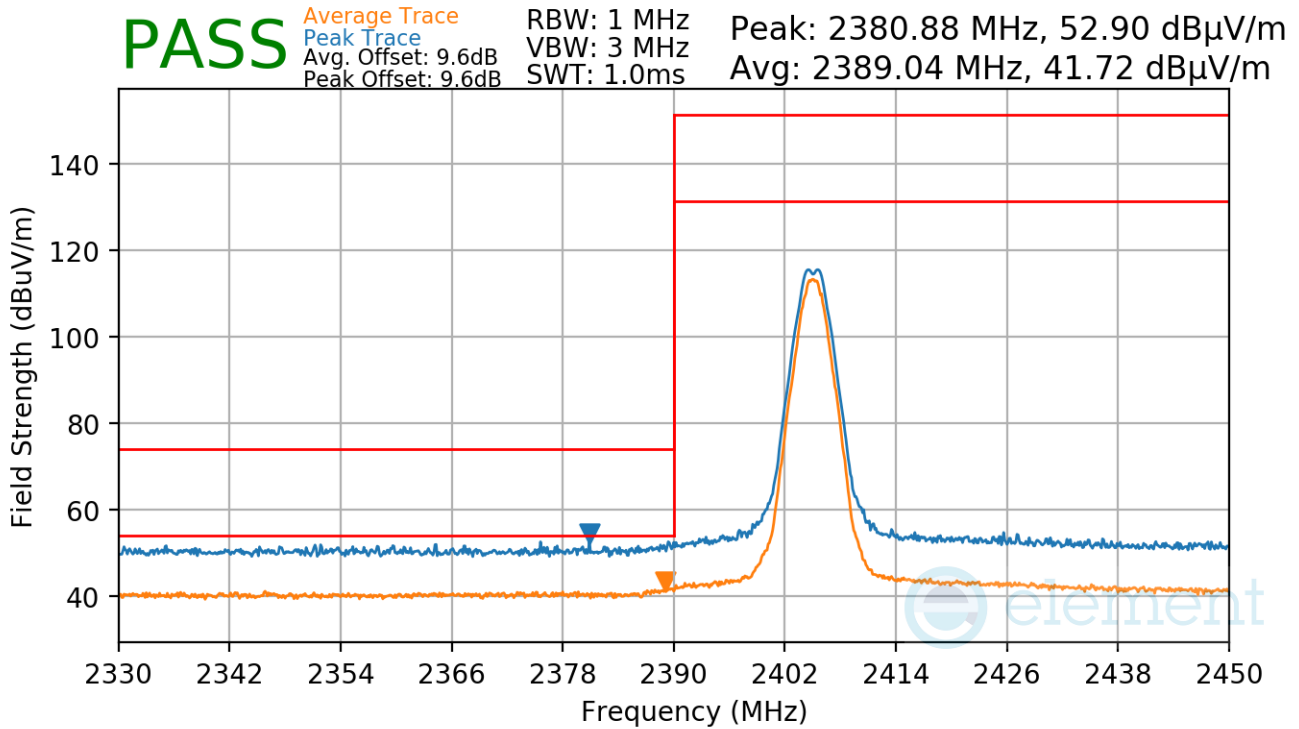
Plot 7-44. Radiated Restricted Lower Band Edge Measurement Antenna 1a
