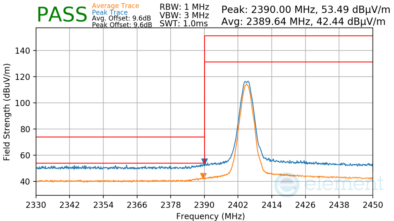
Plot 7-42. Radiated Restricted Lower Band Edge Measurement Antenna 3a
