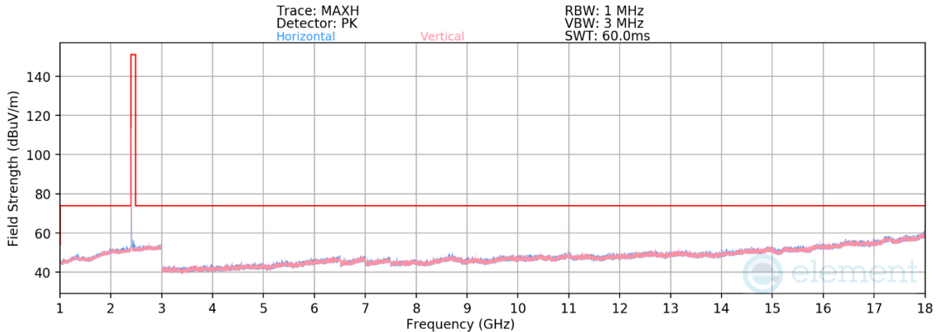
Plot 7-38. Radiated Spurious Emissions 1-18GHz Antenna 1a (802.15.4, ePA – Ch. 11)
