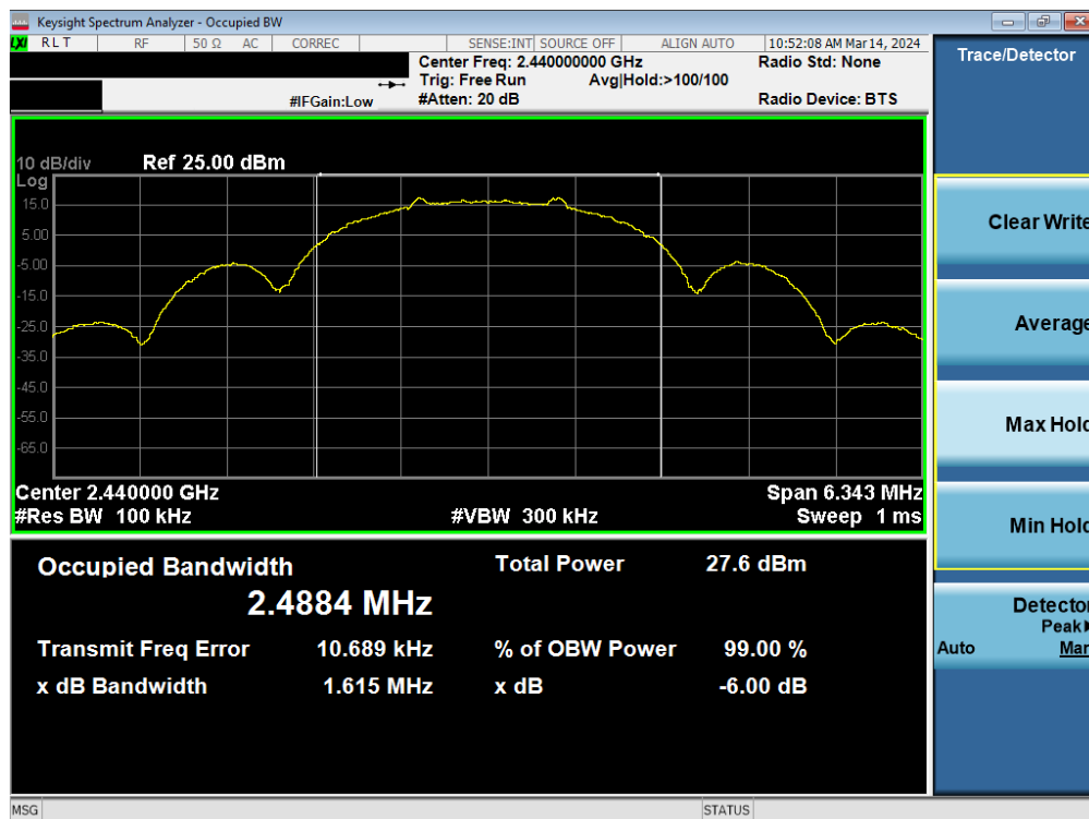
Plot 7-2. 6dB BW & 99% OBW Antenna 3a (802.15.4, Ch. 18)
