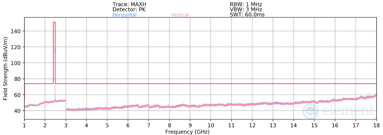
Plot 7-37. Radiated Spurious Emissions 1-18GHz Antenna 3a (802.15.4, ePA – Ch. 25)
