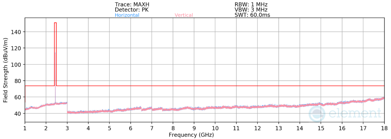
Plot 7-39. Radiated Spurious Emissions 1-18GHz Antenna 1a (802.15.4, ePA – Ch. 18)
