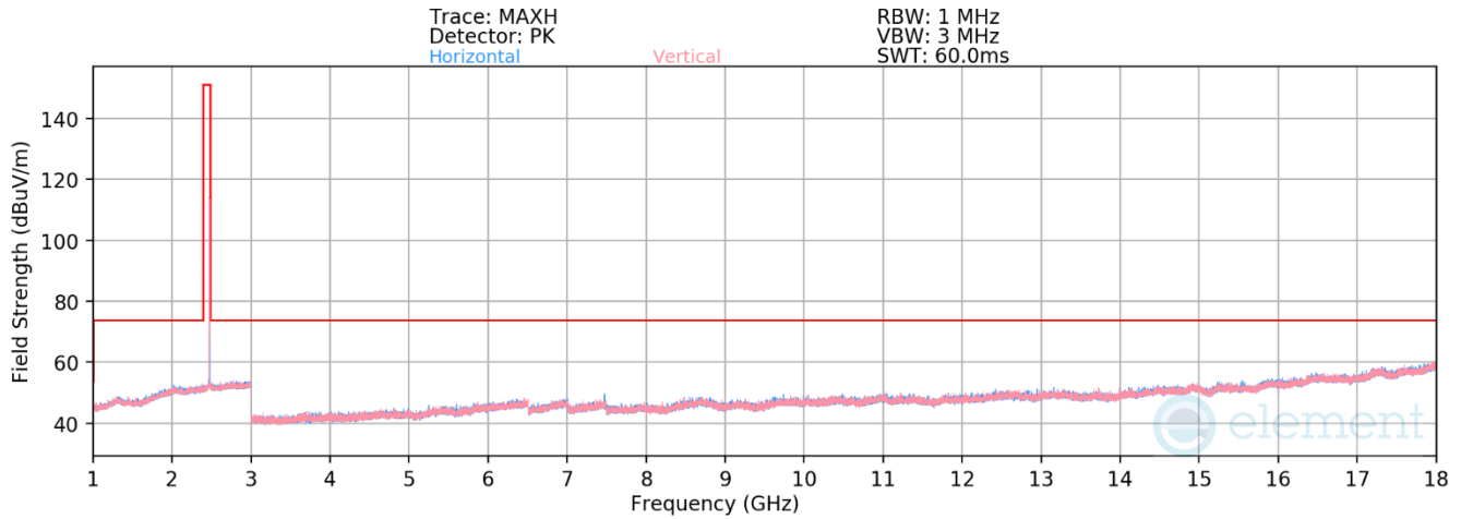
Plot 7-40. Radiated Spurious Emissions 1-18GHz Antenna 1a (802.15.4, ePA – Ch. 25)
