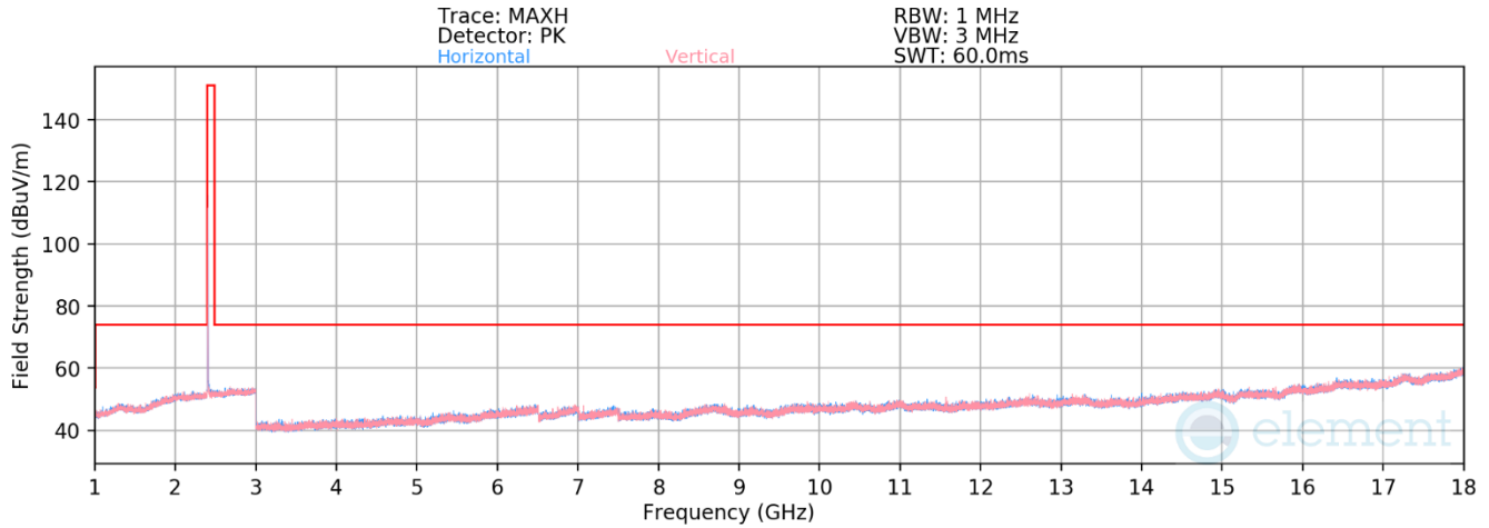
Plot 7-35. Radiated Spurious Emissions 1-18GHz Antenna 3a (802.15.4, ePA – Ch. 11)
