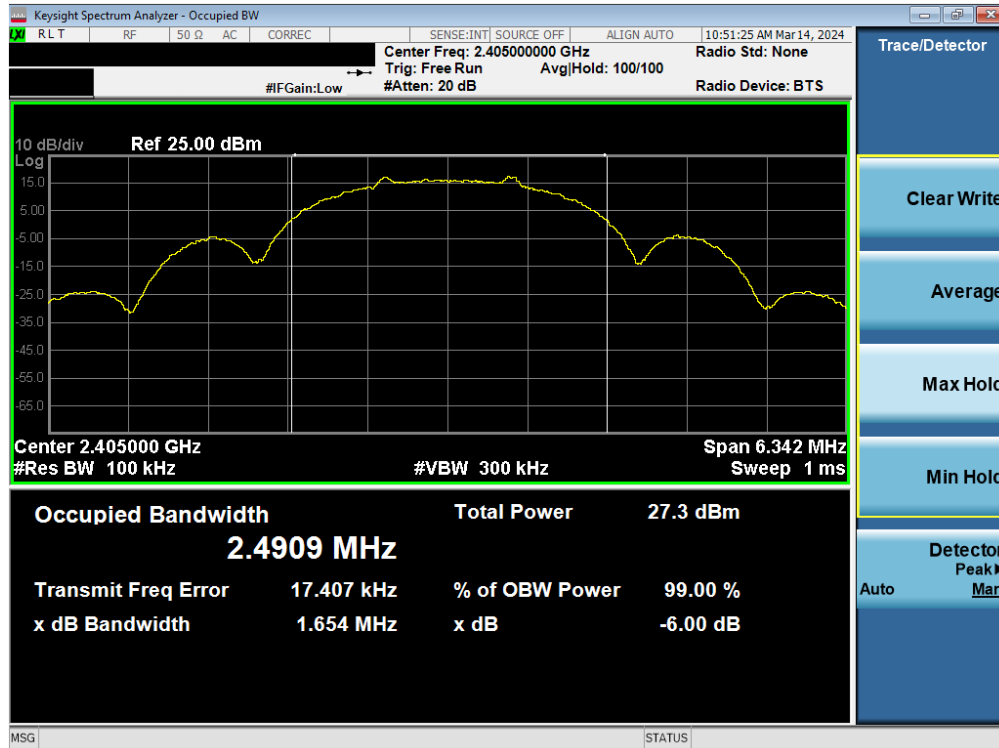
Plot 7-1. 6dB BW & 99% OBW Antenna 3a (802.15.4, Ch. 11)
