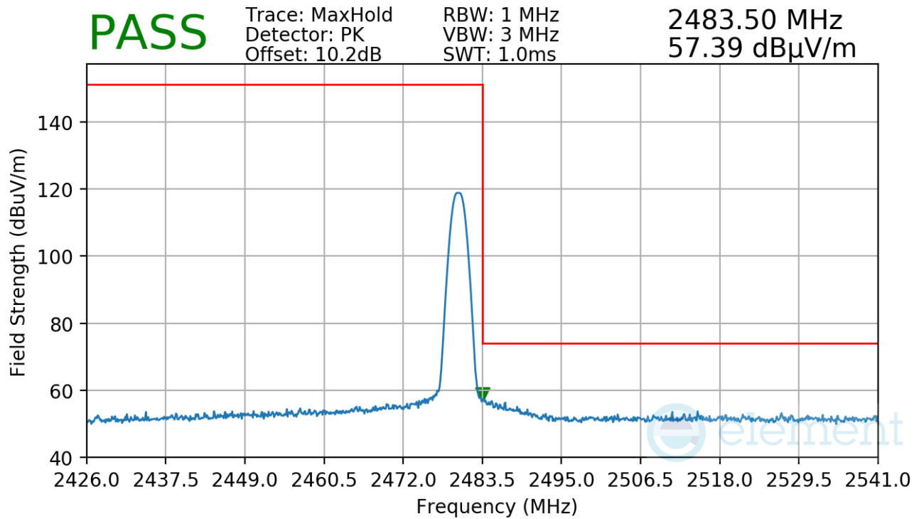
Plot 7-73. Radiated Restricted Upper Band Edge Measurement Antenna 3a
