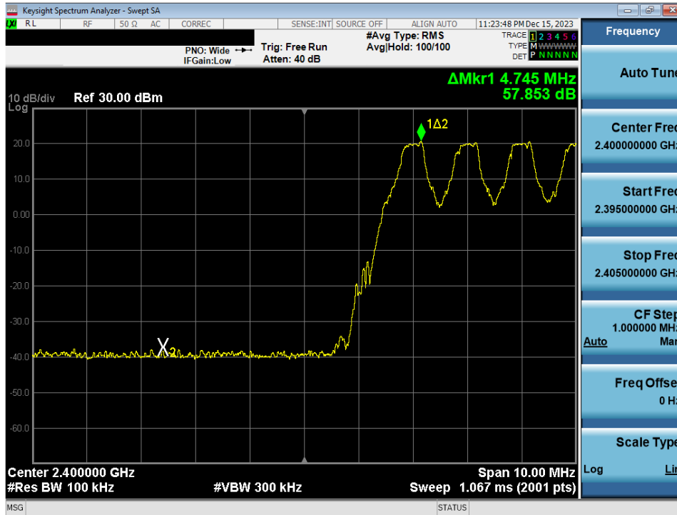
Plot 7-15. Band Edge Plot Antenna 3a (Bluetooth with Hopping Enabled, GFSK, ePA)
