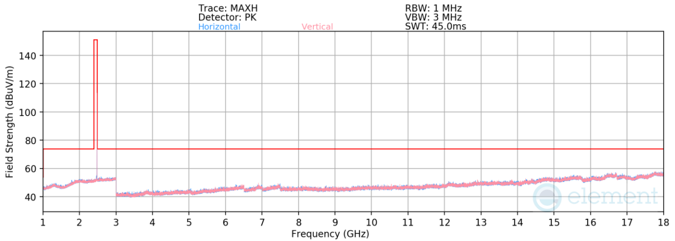
Plot 7-61. Radiated Spurious Emissions above 1GHz Antenna 3a (BT GFSK ePA – Ch. 78)
