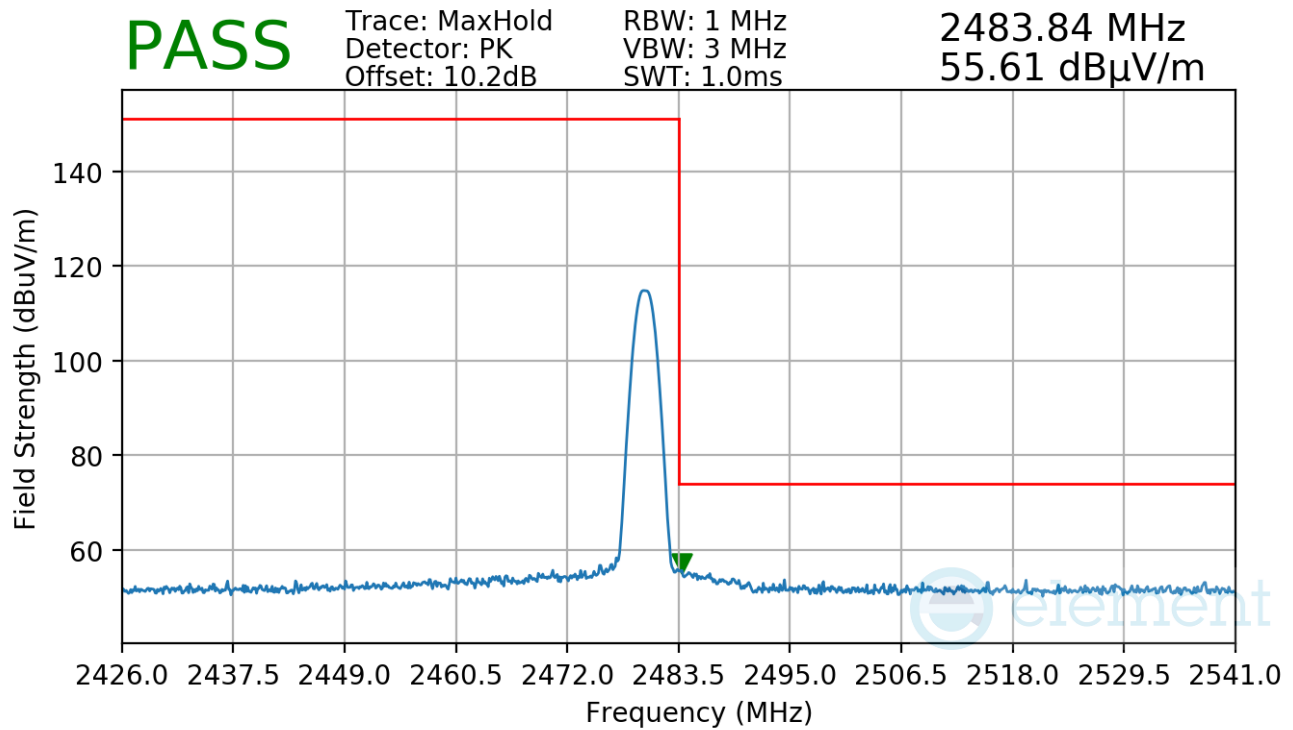
Plot 7-77. Radiated Restricted Upper Band Edge Measurement Antenna 1a
