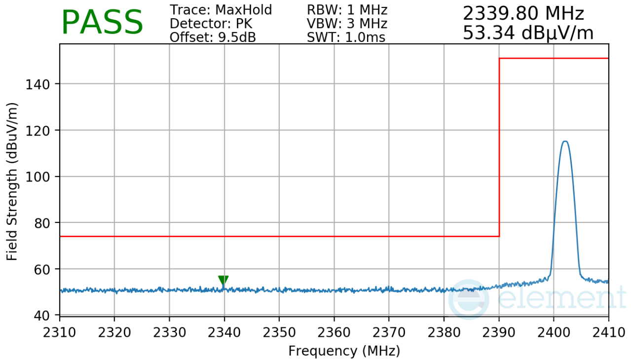
Plot 7-75. Radiated Restricted Lower Band Edge Measurement Antenna 1a
