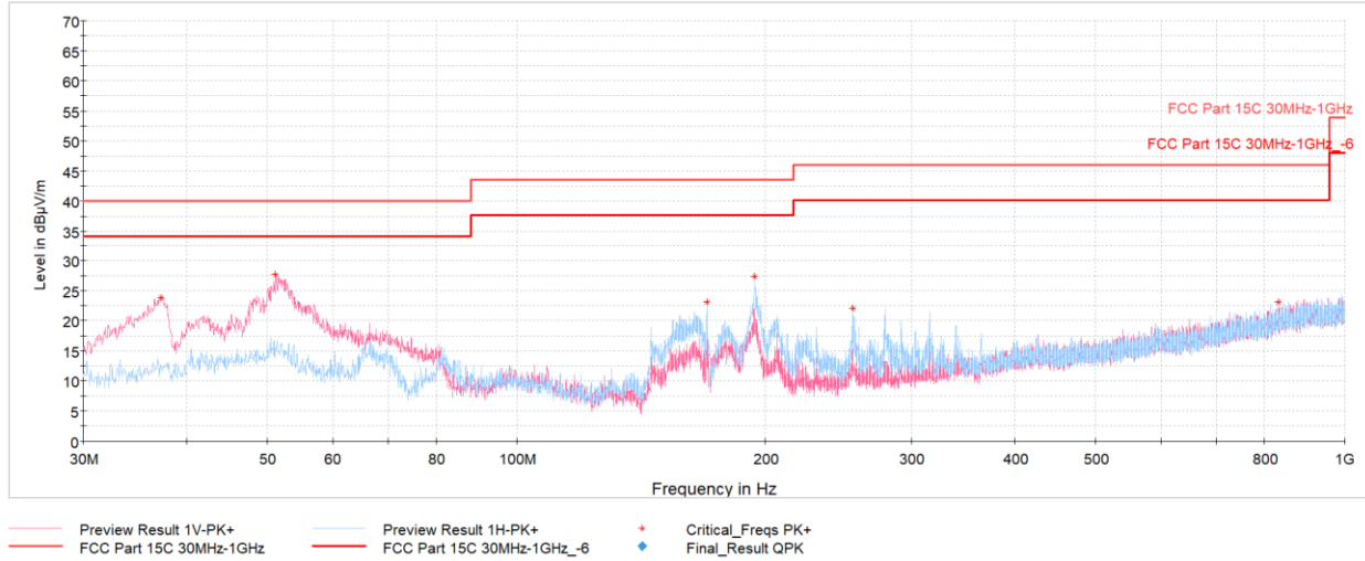
Plot 7-83. Radiated Spurious Emissions Below 1GHz TxBF (GFSK ePA – Ch.0, with AC/DC Adapter)
