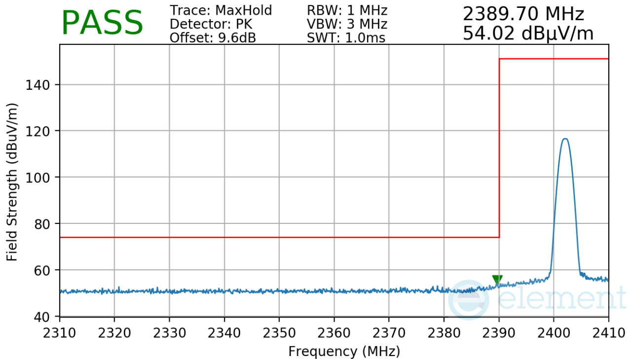
Plot 7-71. Radiated Restricted Lower Band Edge Measurement Antenna 3a
