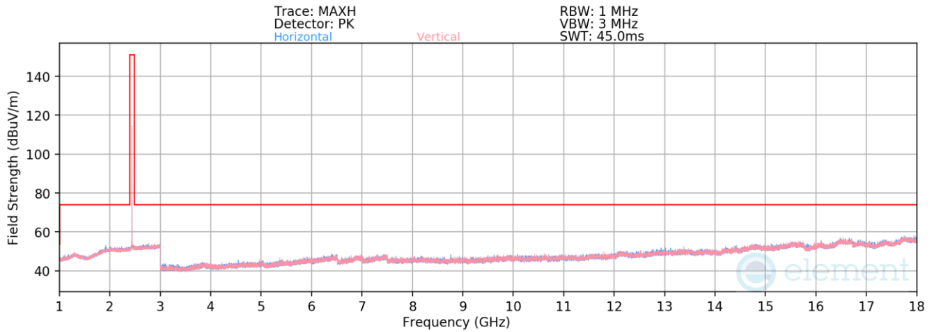
Plot 7-63. Radiated Spurious Emissions above 1GHz Antenna 1a (BT GFSK ePA – Ch. 39)
