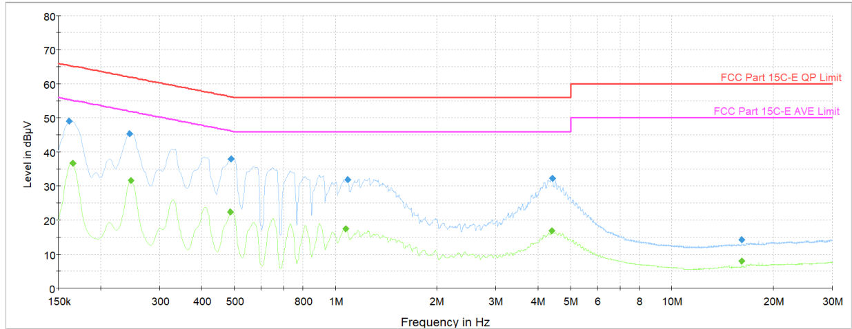
Plot 7-86. AC Line-Conducted Test Plot TxBF (N, GFSK ePA – Ch.39, with AC/DC Adapter)
