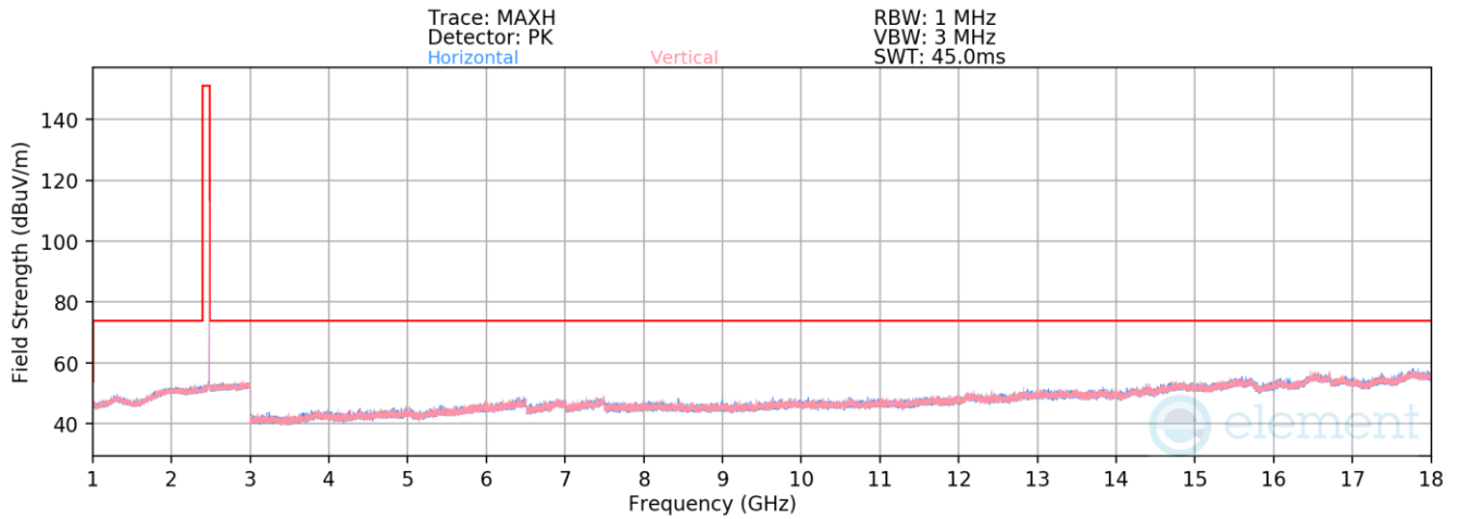
Plot 7-64. Radiated Spurious Emissions above 1GHz Antenna 1a (BT GFSK ePA – Ch. 78)
