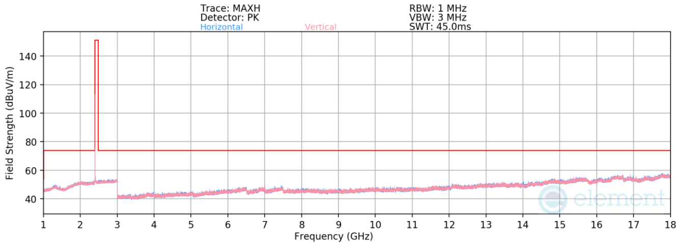
Plot 7-62. Radiated Spurious Emissions above 1GHz Antenna 1a (BT GFSK ePA – Ch. 0)
