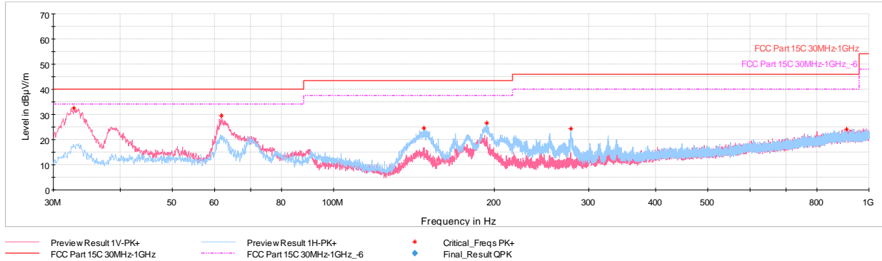
Plot 7-84. Radiated Spurious Emissions - Simultaneous Transmission (with AC/DC Adapter)
