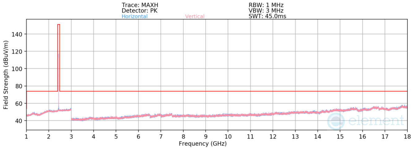
Plot 7-60. Radiated Spurious Emissions above 1GHz Antenna 3a (BT GFSK ePA – Ch. 39)
