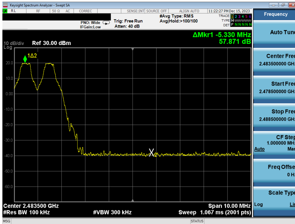
Plot 7-16. Band Edge Plot Antenna 3a (Bluetooth with Hopping Enabled, GFSK, ePA)
