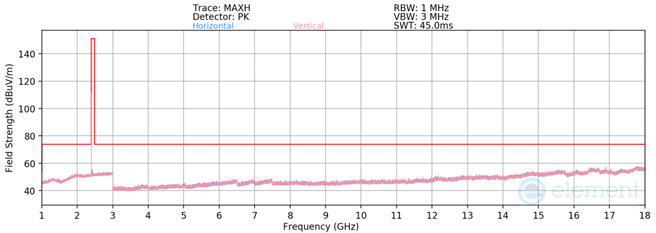
Plot 7-59. Radiated Spurious Emissions above 1GHz Antenna 3a (BT GFSK ePA – Ch. 0)
