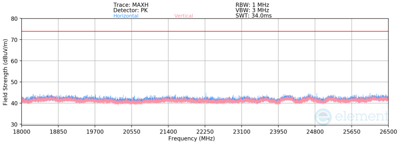
Plot 7-68. Radiated Spurious Emissions above 18GHz TxBF (BT GFSK ePA – Ch. 0)
