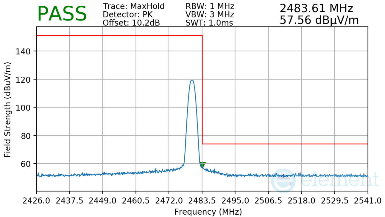
Plot 7-81. Radiated Restricted Upper Band Edge Measurement TxBF
