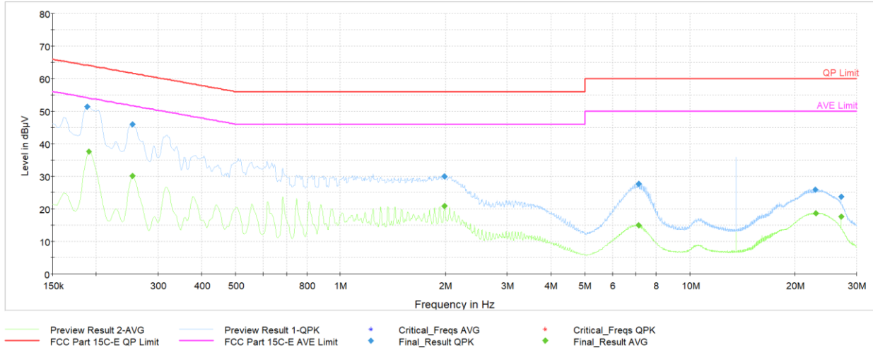
Plot 7-4. AC Line-Conducted Plot (L1, Charging Rate 2.6C, with Laptop)
