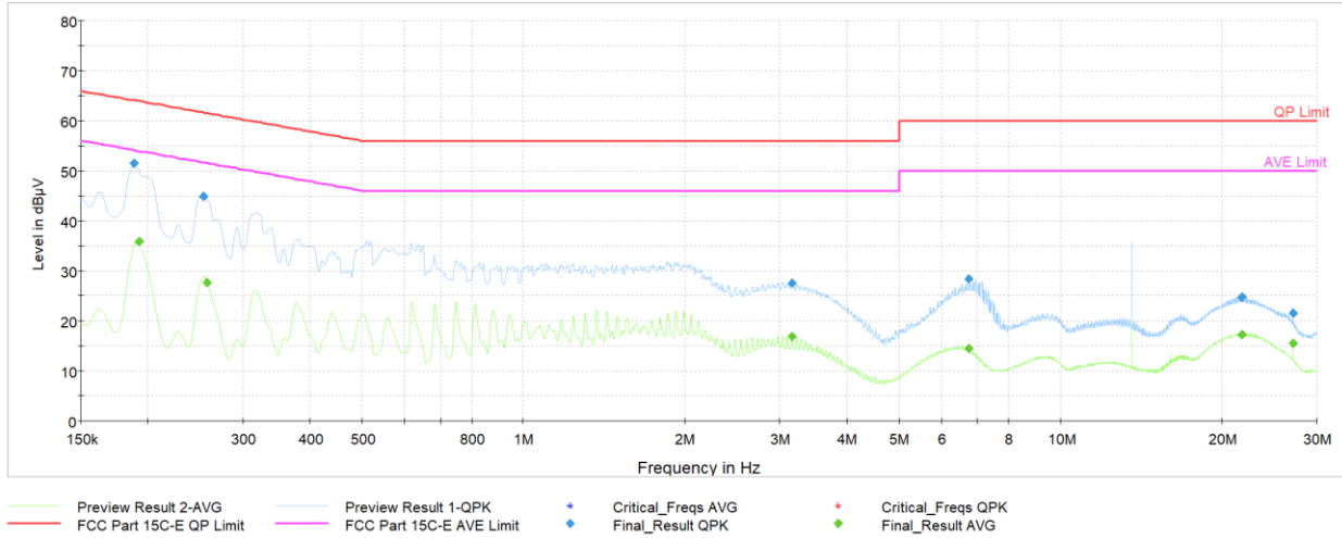
Plot 7-5. AC Line-Conducted Plot (N, Charging Rate 2.6C, with Laptop)
