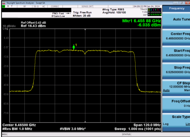
Plot 7-527. Power Spectral Density Plot SDM Primary Antenna WF7a LPI (80MHz 802.11ax (UNII Band 6) – Ch. 103, MCS11)
