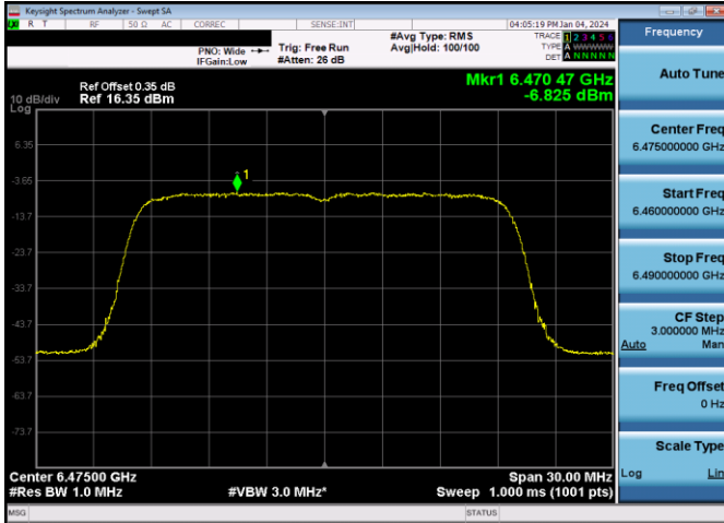
Plot 7-523. Power Spectral Density Plot SDM Primary Antenna WF7a LPI (20MHz 802.11ax (UNII Band 6) – Ch. 105, MCS11)
