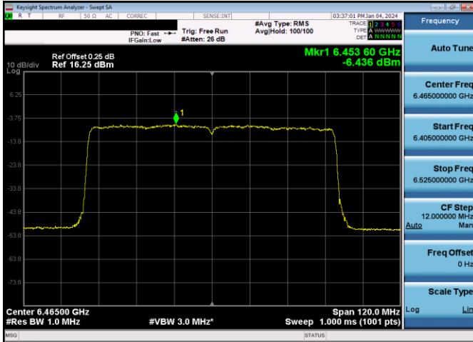
Plot 7-495. Power Spectral Density Plot SDM Primary Antenna WF7a LPI (80MHz 802.11ax (UNII Band 6) – Ch. 103, MCS4)
