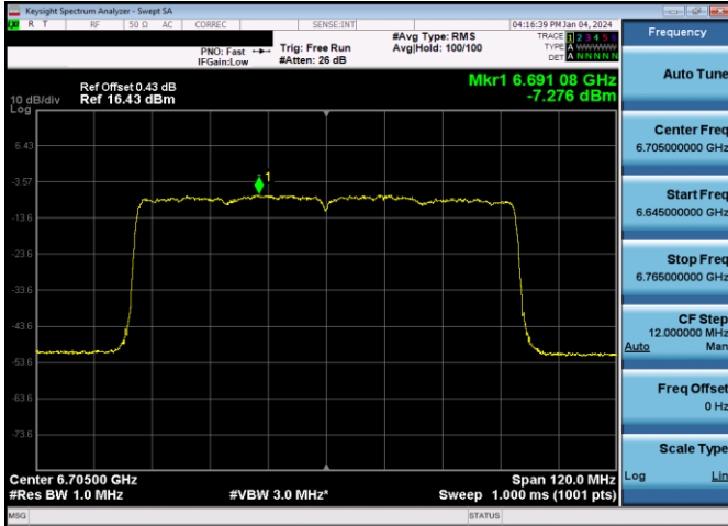
Plot 7-535. Power Spectral Density Plot SDM Primary Antenna WF7a LPI (80MHz 802.11ax (UNII Band 7) – Ch. 151, MCS11)
