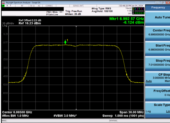
Plot 7-507. Power Spectral Density Plot SDM Primary Antenna WF7a LPI (20MHz 802.11ax (UNII Band 8) – Ch. 209, MCS4)
