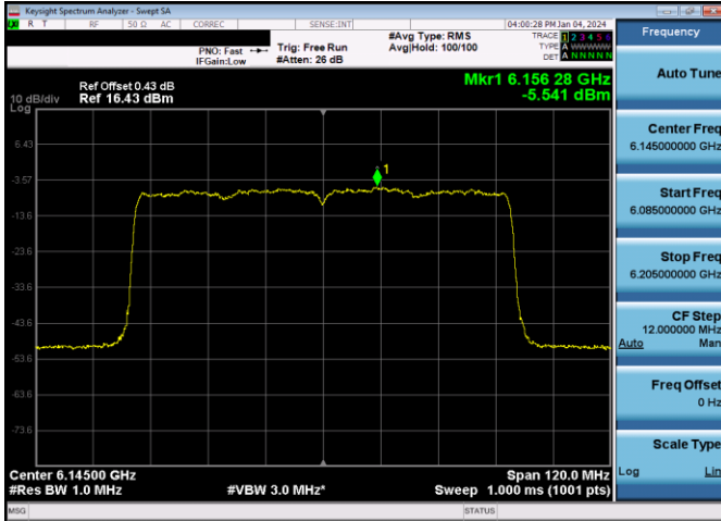
Plot 7-519. Power Spectral Density Plot SDM Primary Antenna WF7a LPI (80MHz 802.11ax (UNII Band 5) – Ch. 39, MCS11)
