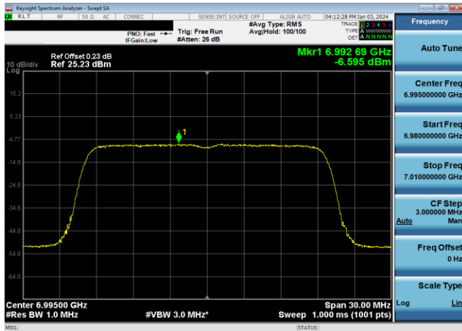
Plot 7-508. Power Spectral Density Plot SDM Primary Antenna WF2a LPI (20MHz 802.11ax (UNII Band 8) – Ch. 209, MCS4)
