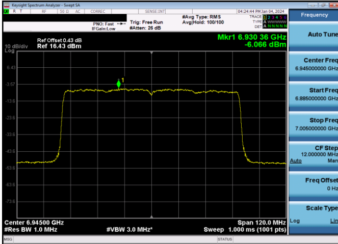
Plot 7-543. Power Spectral Density Plot SDM Primary Antenna WF7a LPI (80MHz 802.11ax (UNII Band 8) – Ch. 199, MCS11)
