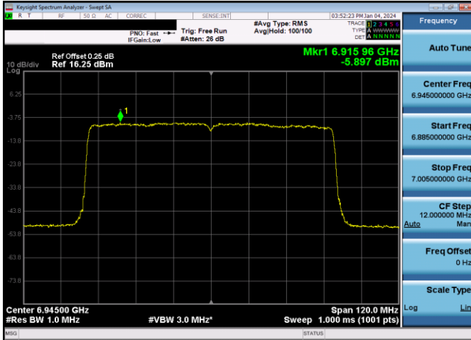
Plot 7-511. Power Spectral Density Plot SDM Primary Antenna WF7a LPI (80MHz 802.11ax (UNII Band 8) – Ch. 199, MCS4)
