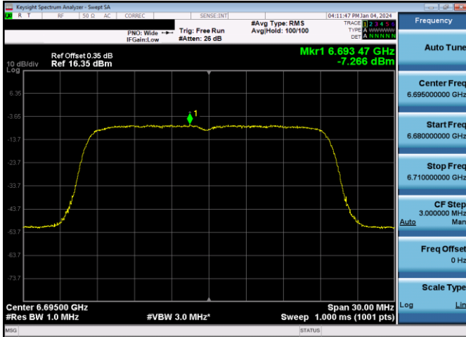
Plot 7-531. Power Spectral Density Plot SDM Primary Antenna WF7a LPI (20MHz 802.11ax (UNII Band 7) – Ch. 149, MCS11)
