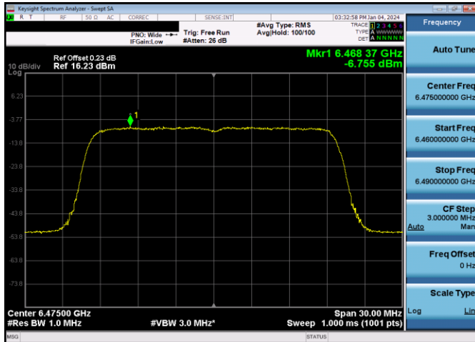
Plot 7-491. Power Spectral Density Plot SDM Primary Antenna WF7a LPI (20MHz 802.11ax (UNII Band 6) – Ch. 105, MCS4)
