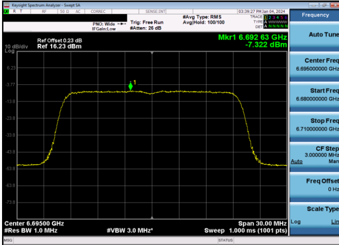
Plot 7-499. Power Spectral Density Plot SDM Primary Antenna WF7a LPI (20MHz 802.11ax (UNII Band 7) – Ch. 149, MCS4)
