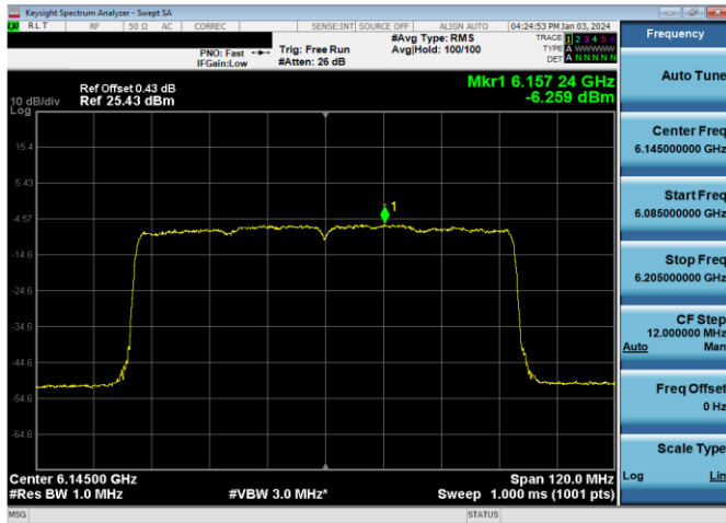
Plot 7-520. Power Spectral Density Plot SDM Primary Antenna WF2a LPI (80MHz 802.11ax (UNII Band 5) – Ch. 39, MCS11)
