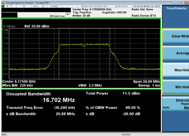
Plot 7-1. 26dB & 99% Bandwidth Plot Antenna WF7a (20MHz 802.11a (UNII Band 5) – Ch. 45, 12Mbps)
