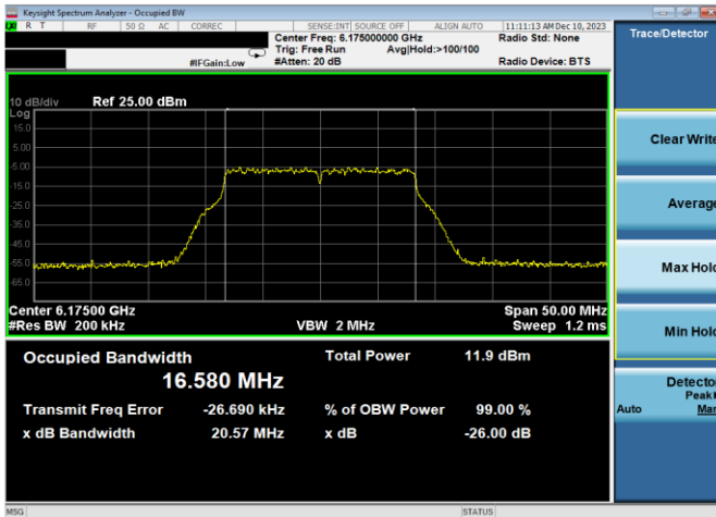
Plot 7-41. 26dB & 99% Bandwidth Plot Antenna WF7a (20MHz 802.11a (UNII Band 5) – Ch. 45, 54Mbps)
