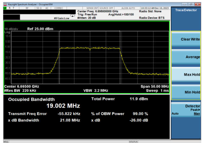
Plot 7-12. 26dB & 99% Bandwidth Plot Antenna WF7a (20MHz 802.11ax (UNII Band 7) – Ch. 149, MCS2)
