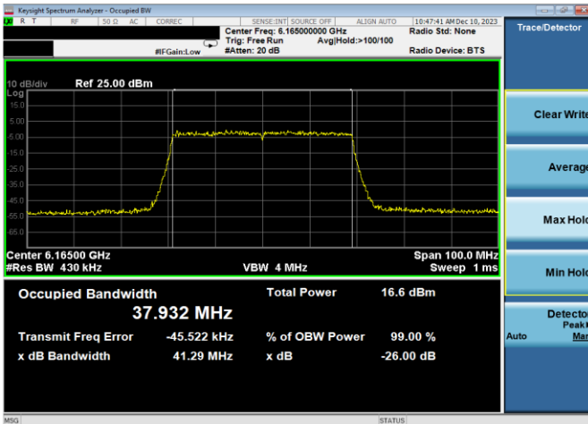
Plot 7-23. 26dB & 99% Bandwidth Plot Antenna WF7a (40MHz 802.11ax (UNII Band 5) – Ch. 43, MCS4)
