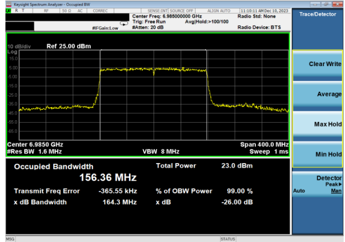
Plot 7-40. 26dB & 99% Bandwidth Plot Antenna WF7a (160MHz 802.11ax (UNII Band 8) – Ch. 207, MCS4)
