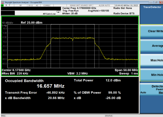
Plot 7-21. 26dB & 99% Bandwidth Plot Antenna WF7a (20MHz 802.11a (UNII Band 5) – Ch. 45, 24Mbps)
