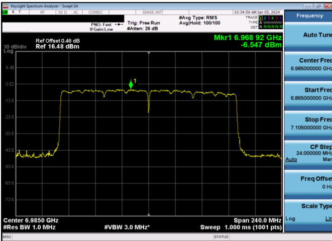
Plot 7-864. LPI Power Spectral Density Plot SDM Antenna WF7b (160MHz 802.11ax RU996x2 (UNII Band 8) – Ch. 207)
