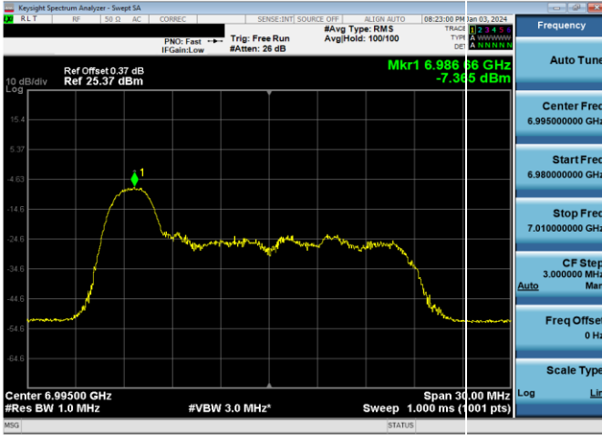
Plot 7-833. LPI Power Spectral Density Plot SDM Antenna WF2a (20MHz 802.11ax RU26 (UNII Band 8) – Ch. 209)
