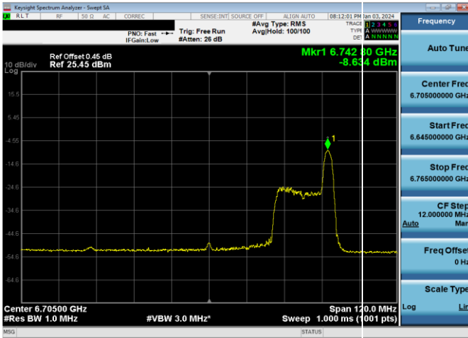
Plot 7-821. LPI Power Spectral Density Plot SDM Antenna WF2a (80MHz 802.11ax RU26 (UNII Band 7) – Ch. 151)
