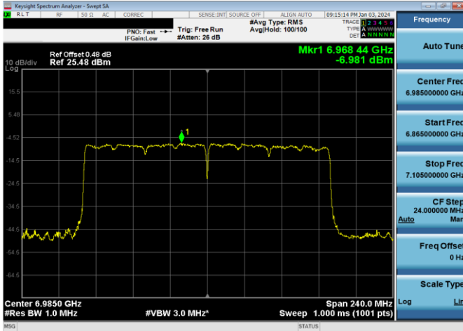
Plot 7-863. LPI Power Spectral Density Plot SDM Antenna WF2a (160MHz 802.11ax RU996x2 (UNII Band 8) – Ch. 207)
