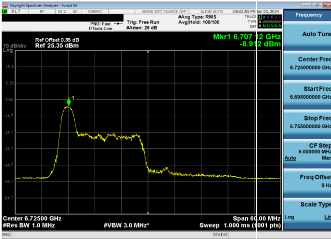
Plot 7-809. LPI Power Spectral Density Plot SDM Antenna WF2a (40MHz 802.11ax RU26 (UNII Band 7) – Ch. 155)
