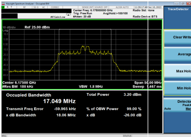
Plot 7-2. 26dB & 99% Bandwidth Plot Antenna WF7a (20MHz 802.11ax RU26 (UNII Band 5) – Ch. 45)
