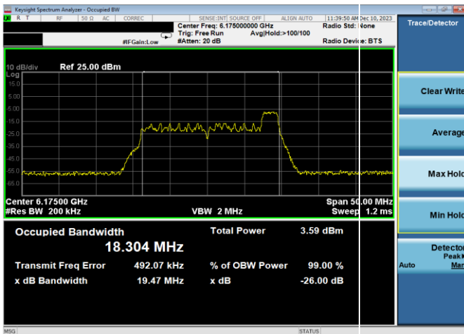
Plot 7-3. 26dB & 99% Bandwidth Plot Antenna WF7a (20MHz 802.11ax RU26 (UNII Band 5) – Ch. 45)
