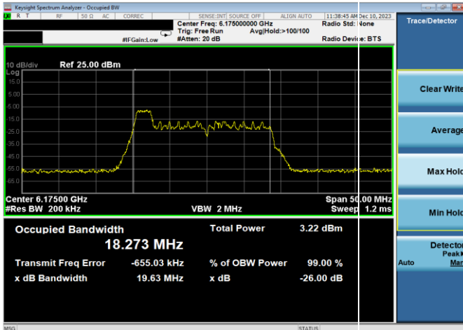
Plot 7-1. 26dB & 99% Bandwidth Plot Antenna WF7a (20MHz 802.11ax RU26 (UNII Band 5) – Ch. 45)
