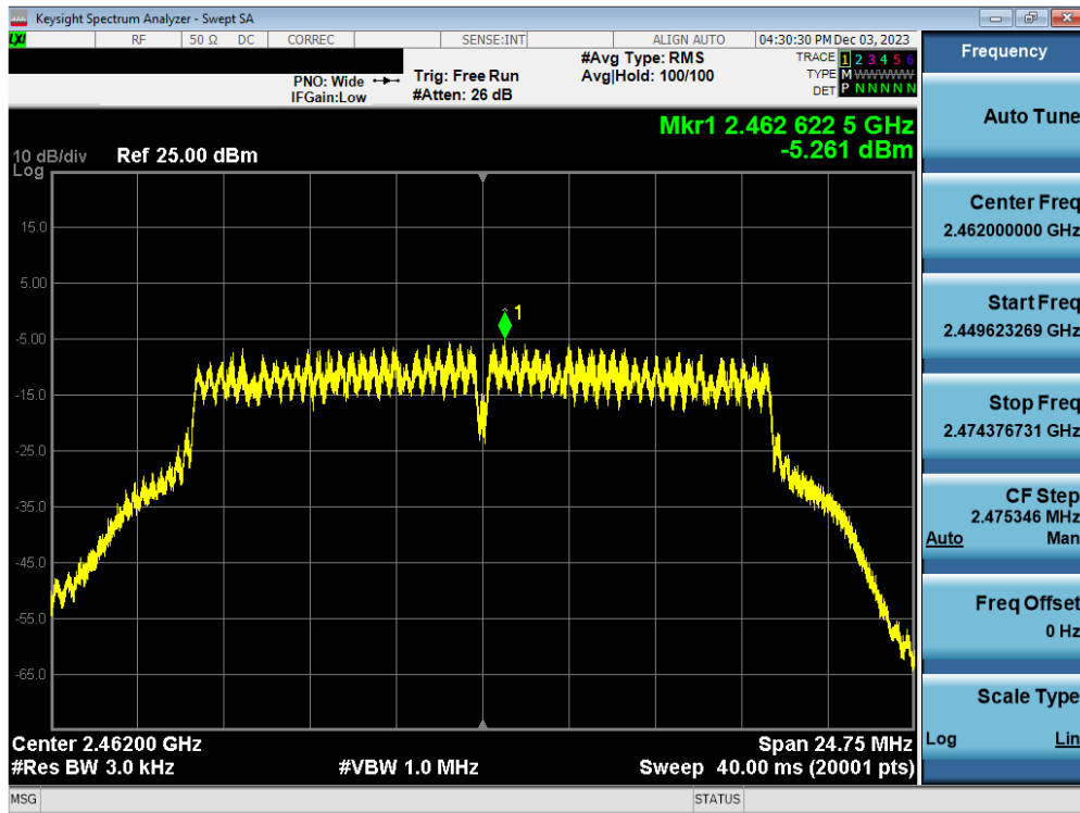
Plot 7-102. Power Spectral Density Plot Antenna WF2b (802.11g – Ch. 11) – 24Mbps
