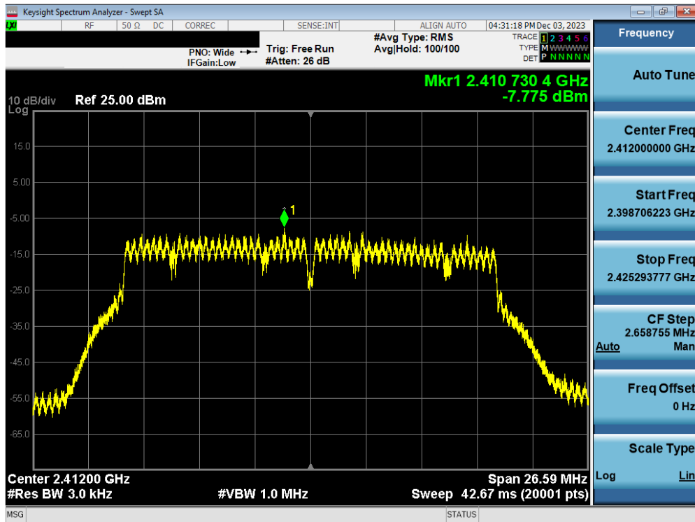
Plot 7-103. Power Spectral Density Plot Antenna WF2b (802.11n (2.4GHz) – Ch. 1) – MCS4
