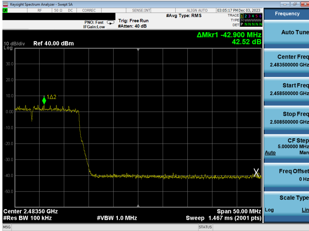
Plot 7-87. Band Edge Antenna WF7b (802.11ax OFDMA – RU242 – Ch. 11)
