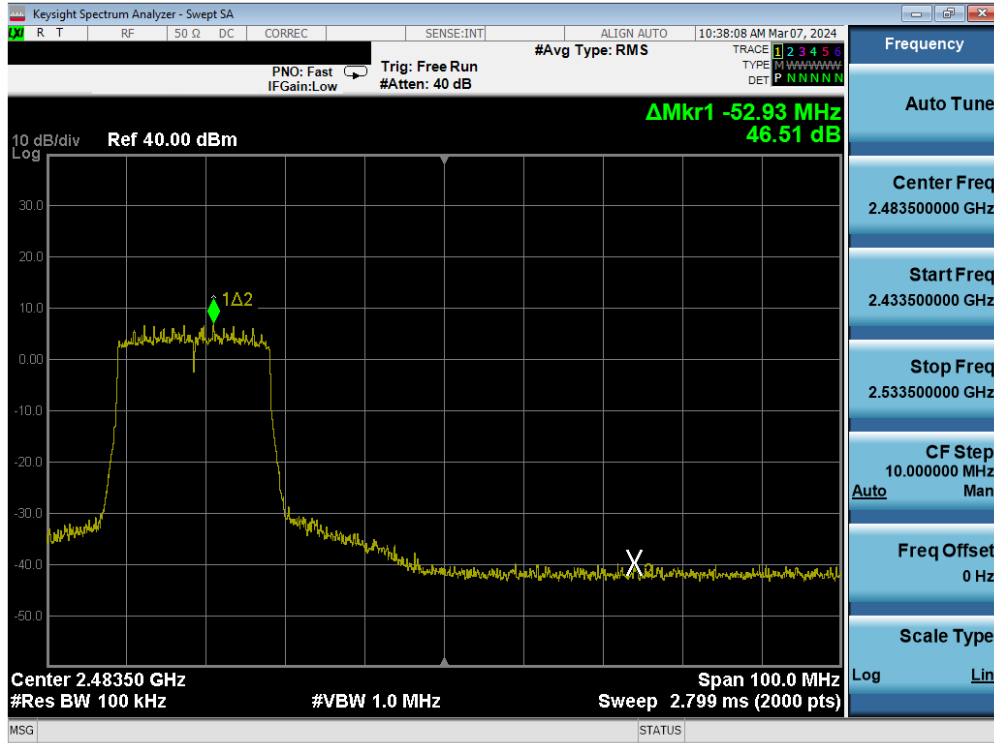
Plot 7-85. Band Edge Antenna WF7b (802.11ax OFDMA – RU242 – Ch. 9)
