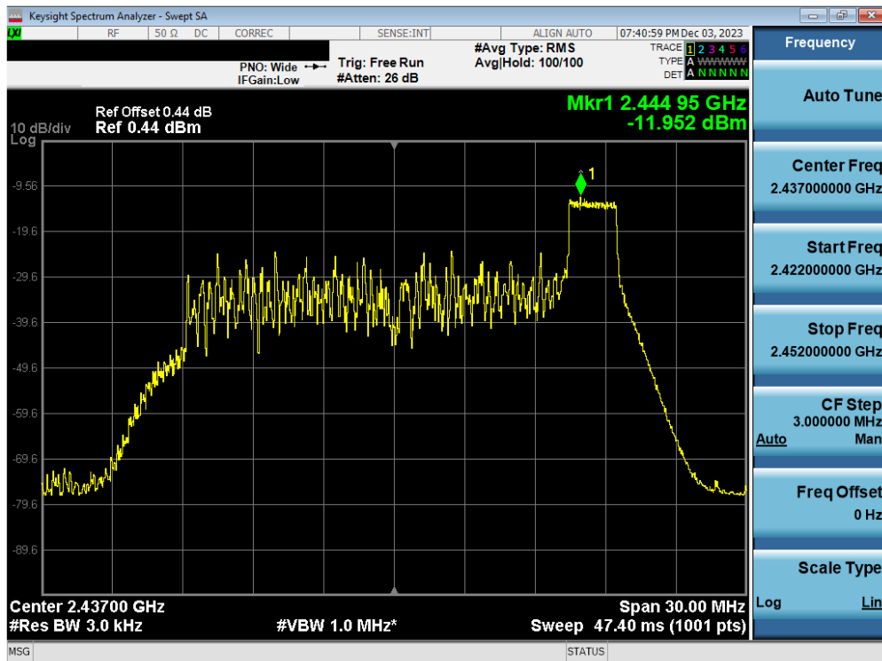
Plot 7-60. Power Spectral Density Plot Antenna WF2b (802.11ax OFDMA – RU26 Index 8 – Ch. 6)
