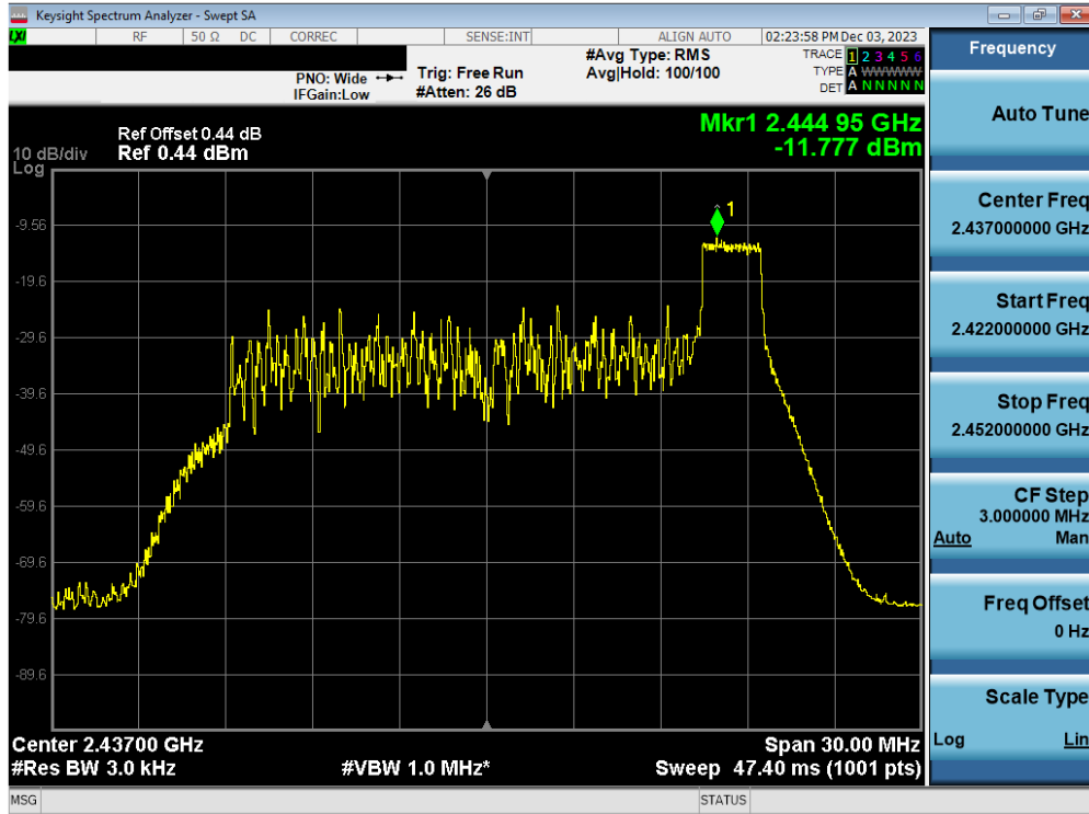
Plot 7-59. Power Spectral Density Plot Antenna WF7b (802.11ax OFDMA – RU26 Index 8 – Ch. 6)
