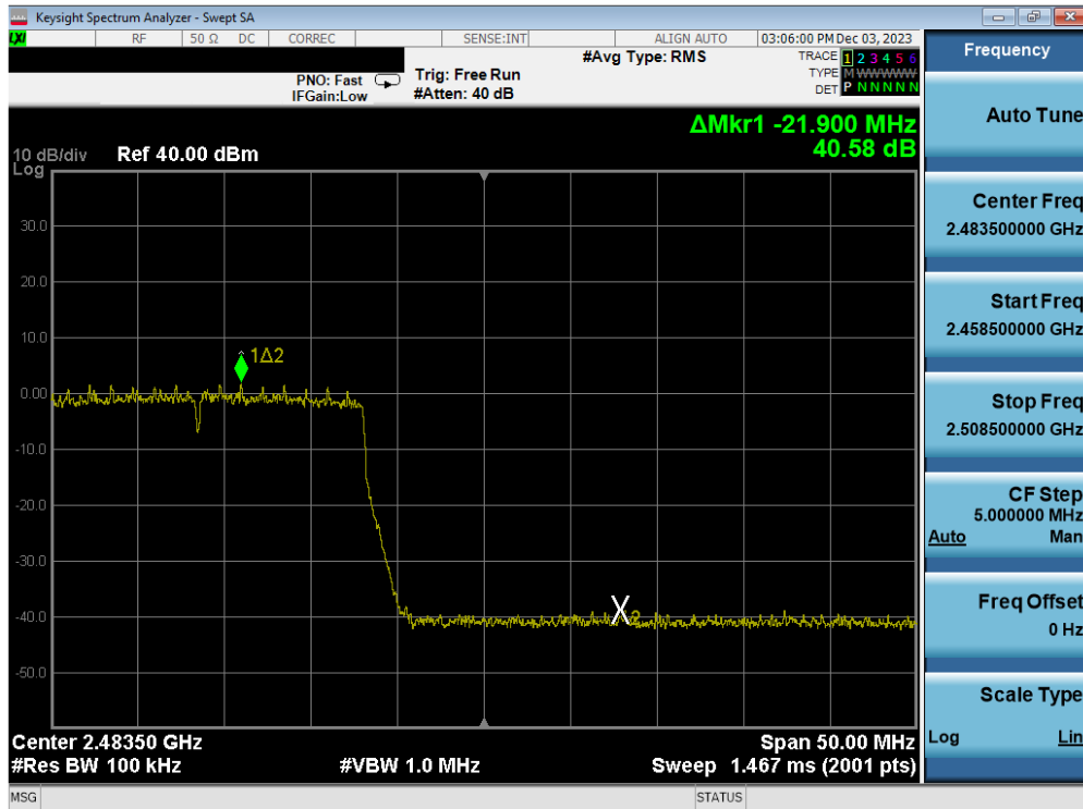
Plot 7-88. Band Edge Antenna WF7b (802.11ax OFDMA – RU242 – Ch. 12)
