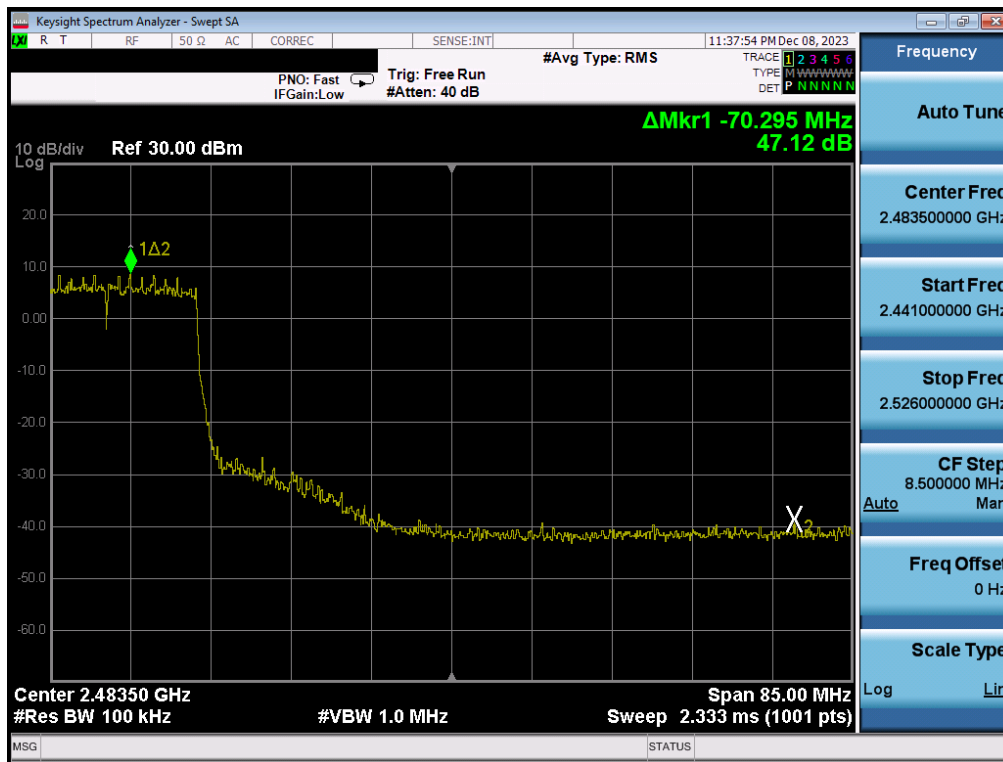
Plot 7-100. Band Edge Antenna WF2b (802.11ax OFDMA – RU242 – Ch. 8)
