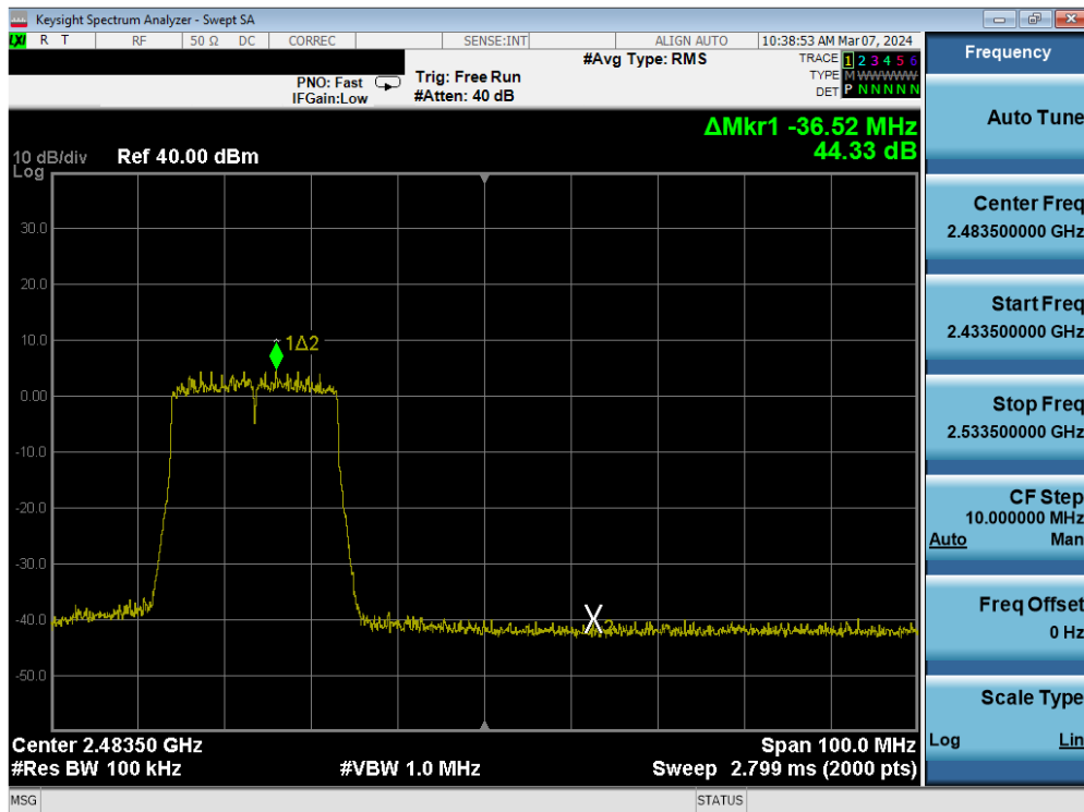
Plot 7-86. Band Edge Antenna WF7b (802.11ax OFDMA – RU242 – Ch. 10)
