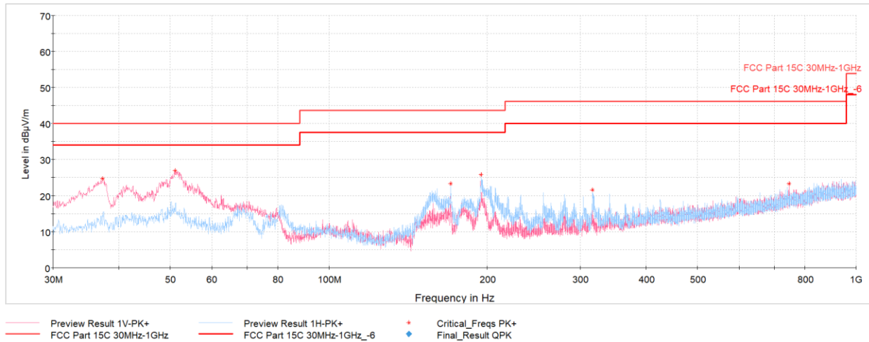
Plot 7-103. Radiated Spurious Emissions Below 1GHz TxBF (1Mbps, ePA – Ch.19, Pol. H & V, with AC/DC Adapter)
