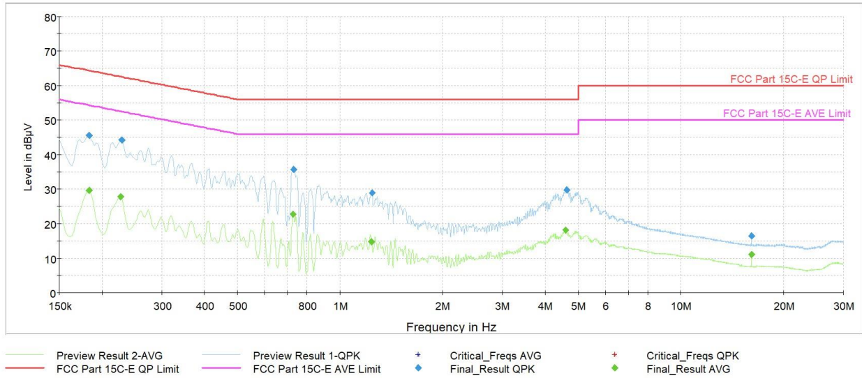
Plot 7-104. AC Line Conducted Plot with Bluetooth LE Tx BF (L1, 1Mbps ePA – Ch.19 with AC/DC Adapter)
