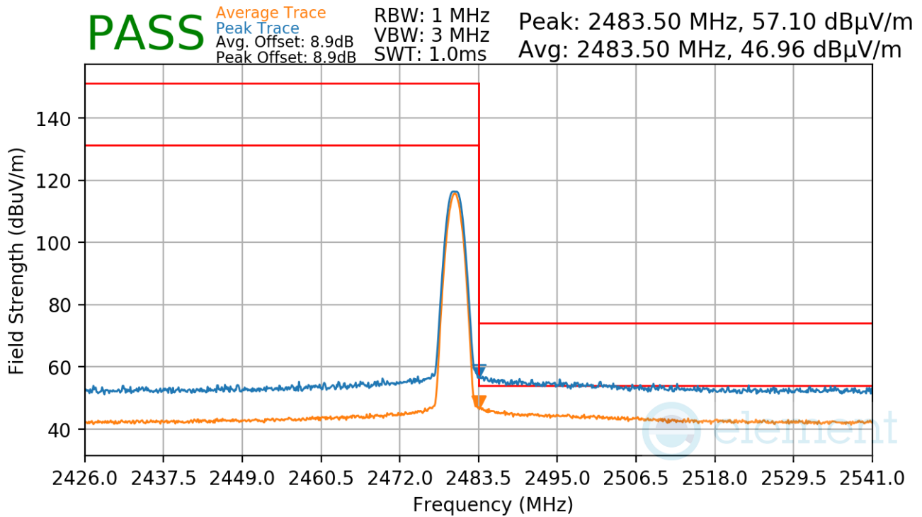
Plot 7-96. Radiated Restricted Upper Band Edge Measurement Antenna WF2b (Average & Peak)
