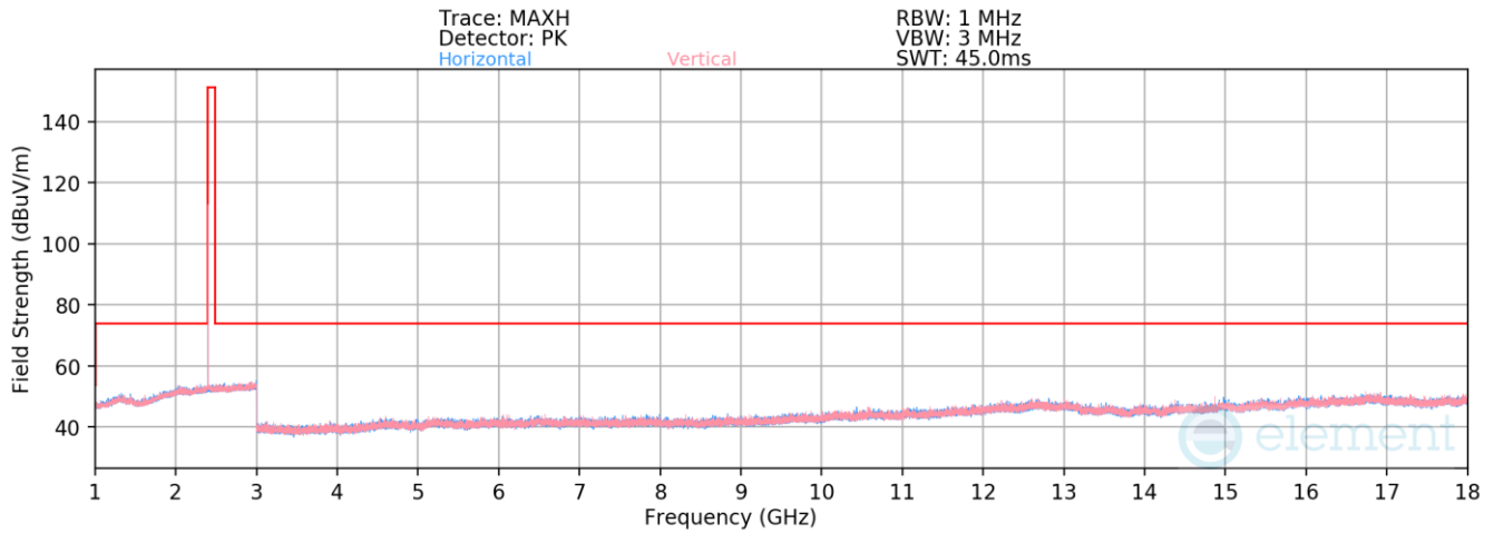
Plot 7-84. Radiated Spurious Emissions 1-18GHz Antenna WF2b (1Mbps, ePA – Ch. 0)
