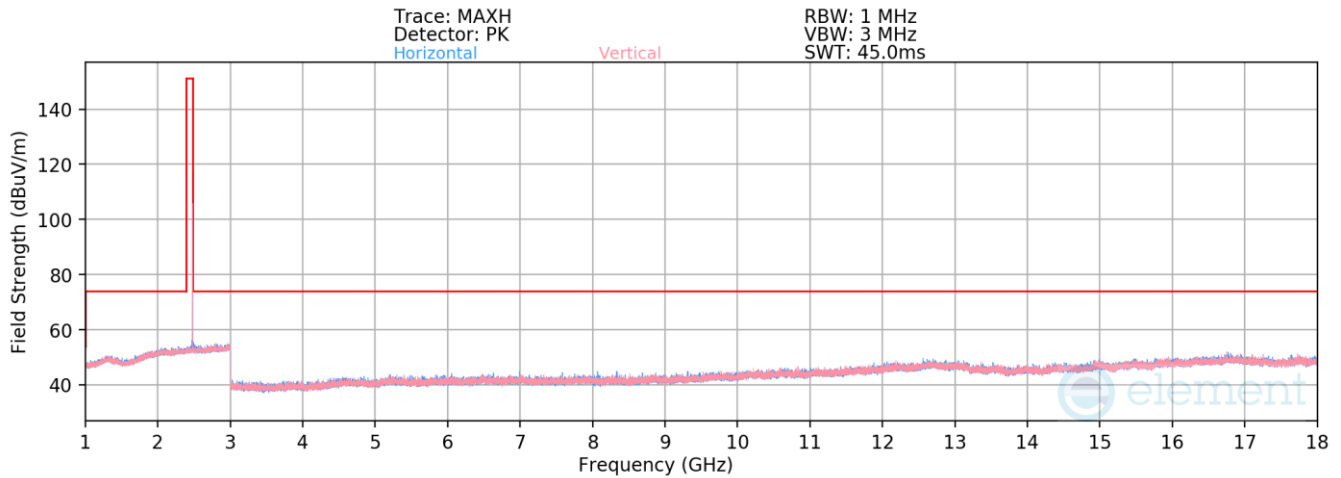
Plot 7-83. Radiated Spurious Emissions 1-18GHz Antenna WF7b (1Mbps ePA – Ch. 39)
