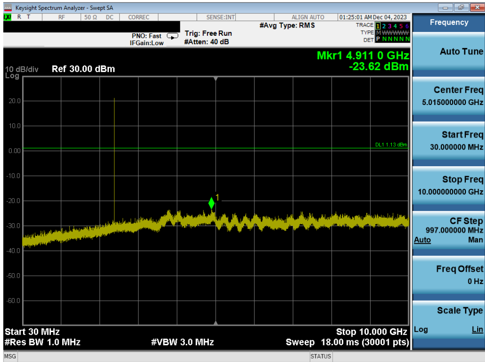
Plot 7-75. Conducted Spurious Plot Antenna WF2b (Bluetooth (LE), 1Mbps, ePA – Ch. 0)
