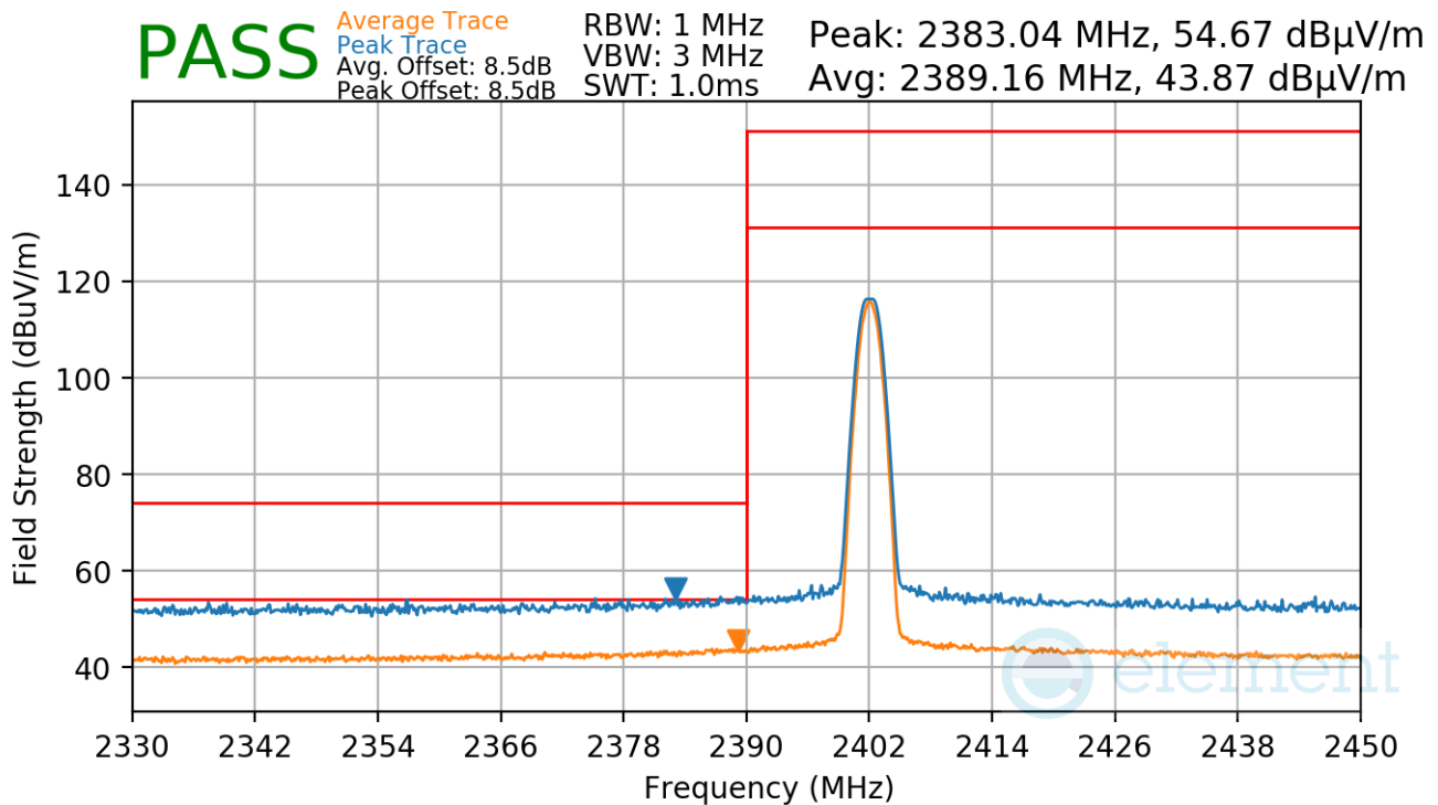
Plot 7-95. Radiated Restricted Lower Band Edge Measurement Antenna WF2b (Average & Peak)
