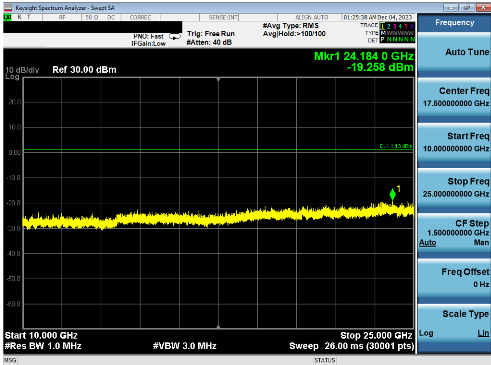
Plot 7-76. Conducted Spurious Plot Antenna WF2b (Bluetooth (LE), 1Mbps, ePA – Ch. 0)
