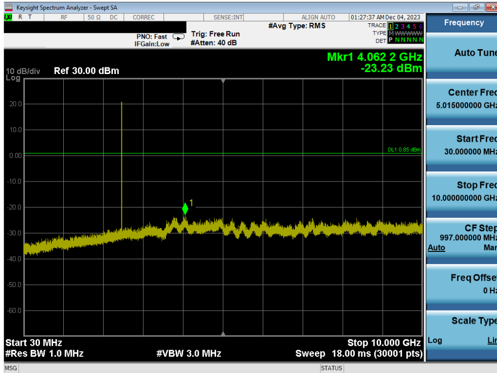
Plot 7-79. Conducted Spurious Plot Antenna WF2b (Bluetooth (LE), 1Mbps, ePA – Ch. 39)
