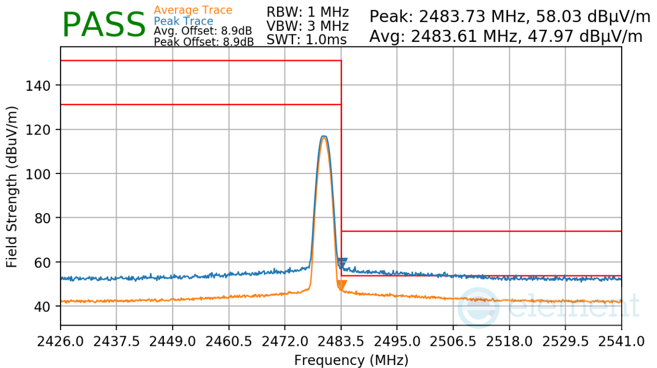
Plot 7-92. Radiated Restricted Upper Band Edge Measurement Antenna WF7b (Average & Peak)
