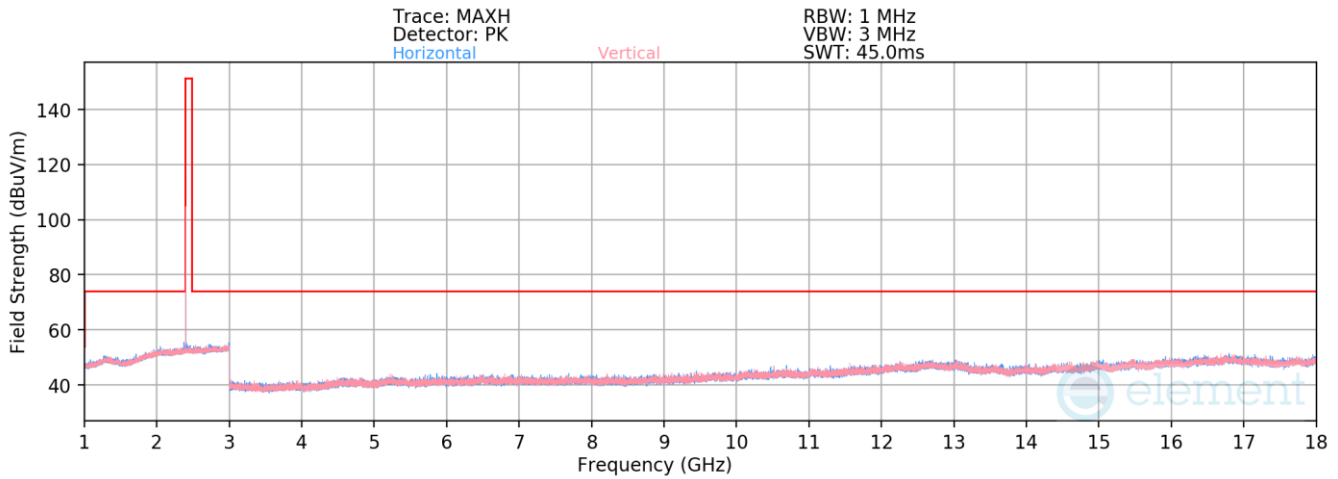
Plot 7-81. Radiated Spurious Emissions 1-18GHz Antenna WF7b (1Mbps, ePA – Ch. 0)
