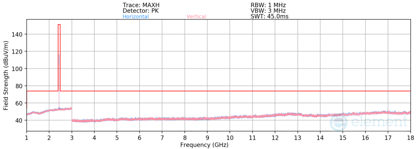
Plot 7-82. Radiated Spurious Emissions 1-18GHz Antenna WF7b (1Mbps, ePA – Ch. 19)
