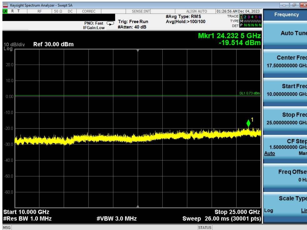
Plot 7-78. Conducted Spurious Plot Antenna WF2b (Bluetooth (LE), 1Mbps, ePA – Ch. 19)
