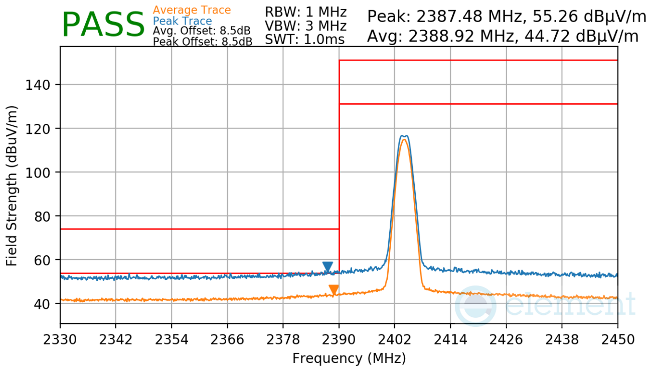
Plot 7-93. Radiated Restricted Lower Band Edge Measurement Antenna WF7b (Average & Peak)
