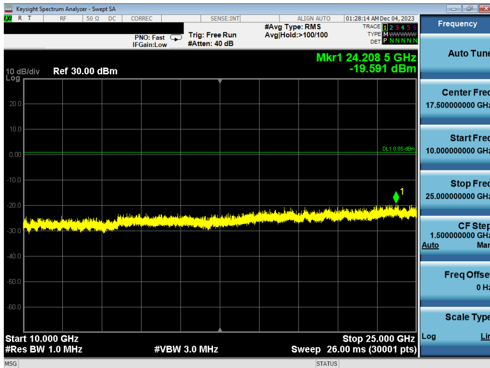
Plot 7-80. Conducted Spurious Plot Antenna WF2b (Bluetooth (LE), 1Mbps, ePA – Ch. 39)
