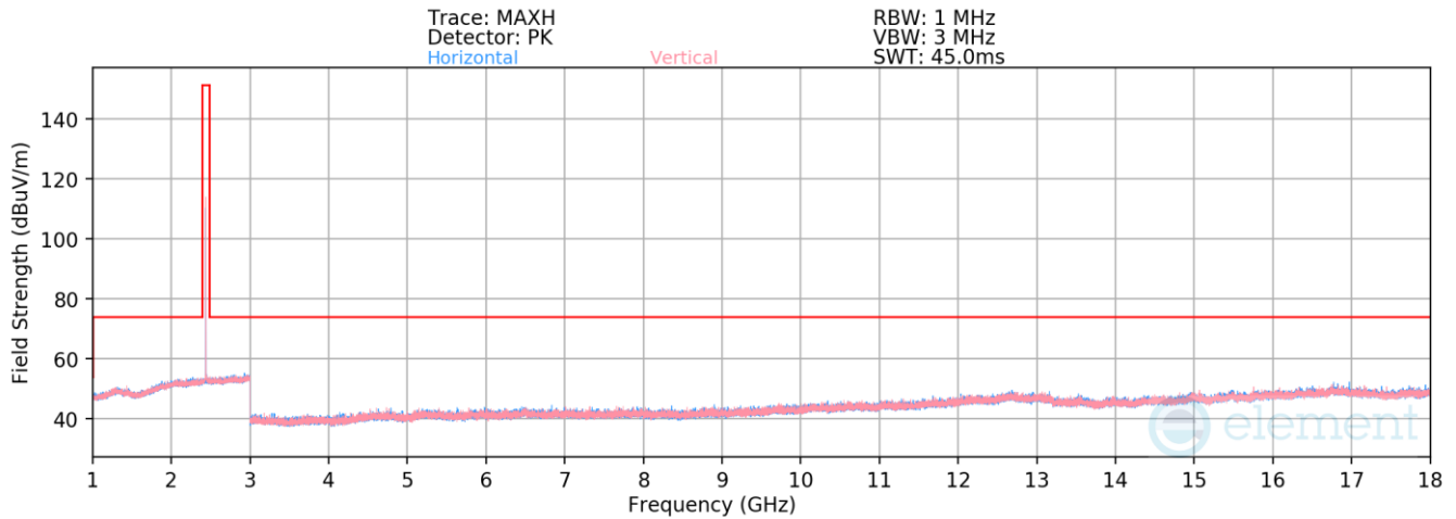
Plot 7-85. Radiated Spurious Emissions 1-18GHz Antenna WF2b (1Mbps, ePA – Ch. 19)
