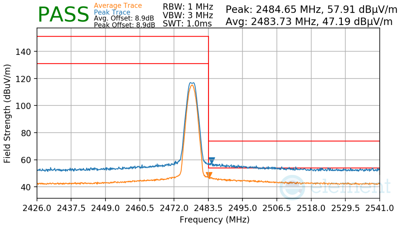
Plot 7-94. Radiated Restricted Upper Band Edge Measurement Antenna WF7b (Average & Peak)
