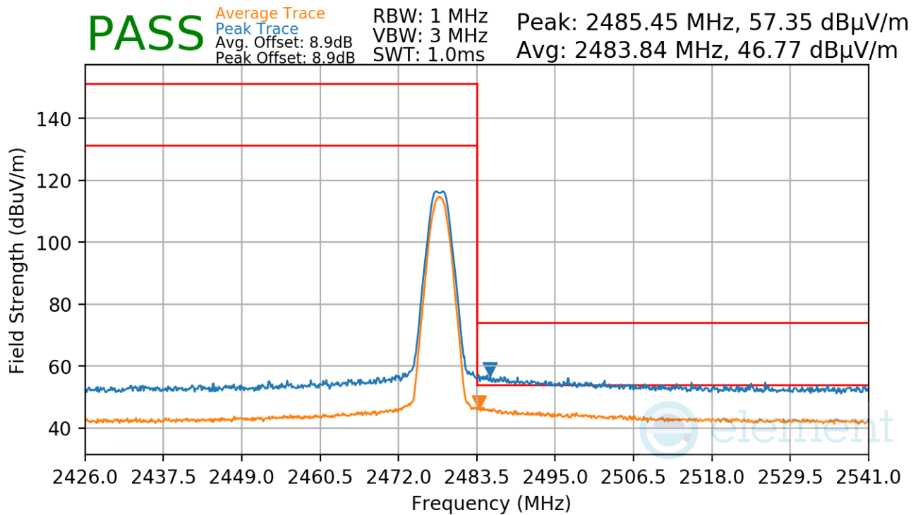
Plot 7-98. Radiated Restricted Upper Band Edge Measurement Antenna WF2b (Average & Peak)
