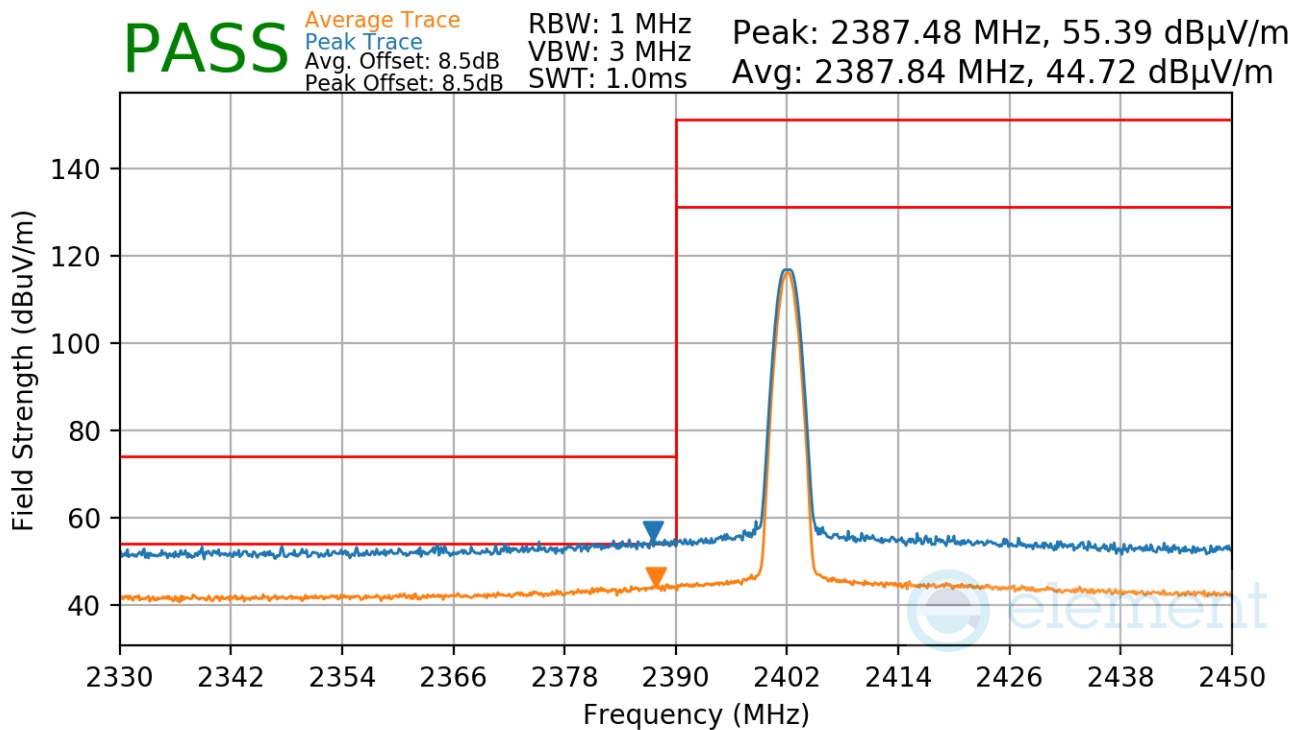
Plot 7-91. Radiated Restricted Lower Band Edge Measurement Antenna WF7b (Average & Peak)
