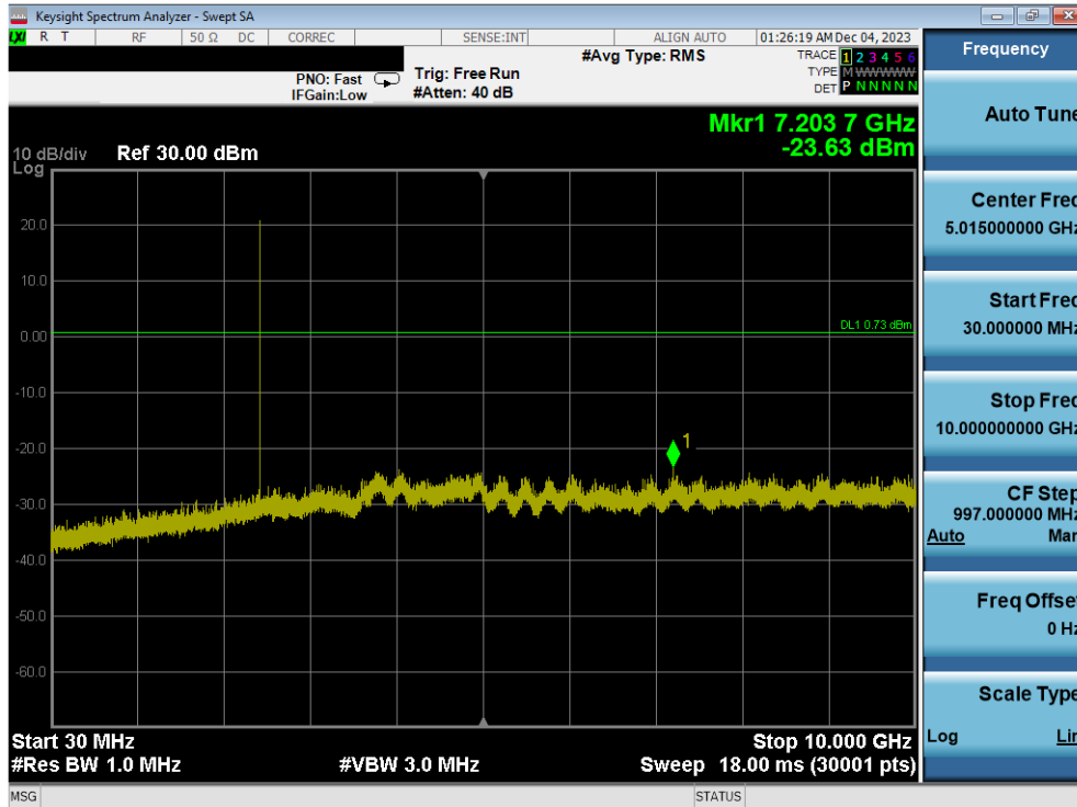
Plot 7-77. Conducted Spurious Plot Antenna WF2b (Bluetooth (LE), 1Mbps, ePA – Ch. 19)
