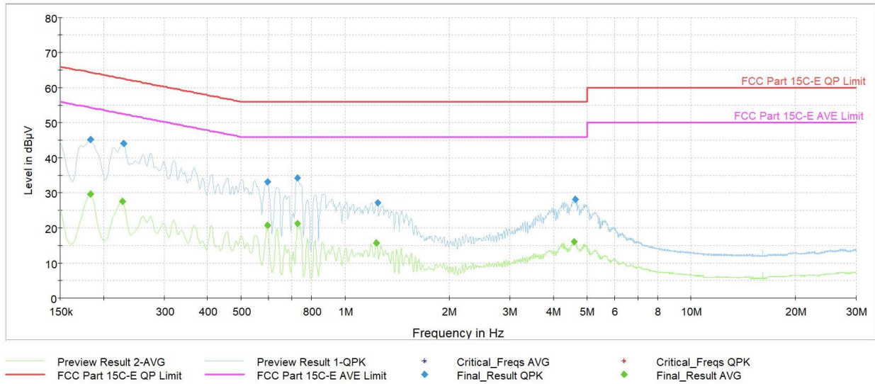
Plot 7-105. AC Line Conducted Plot with Bluetooth LE Tx BF (N, 1Mbps ePA – Ch.19, with AC/DC Adapter)
