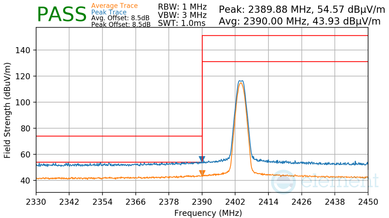
Plot 7-97. Radiated Restricted Lower Band Edge Measurement Antenna WF2b (Average & Peak)
