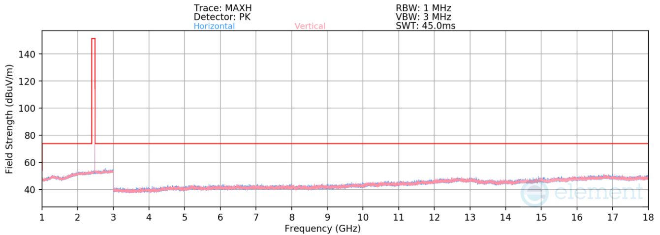
Plot 7-86. Radiated Spurious Emissions 1-18GHz Antenna WF2b (1Mbps ePA – Ch. 39)
