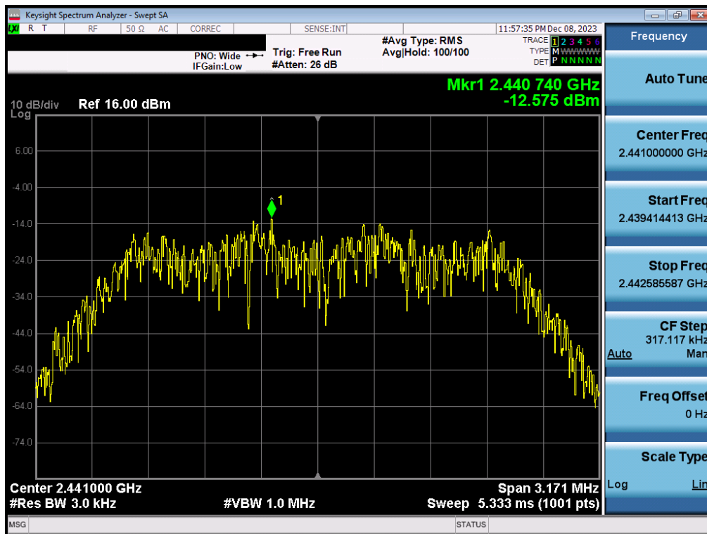
Plot 7-46. Power Spectral Density Plot TxBF Antenna WF2b (Bluetooth (HDR4), 4Mbps, iPA – Ch. 38)
