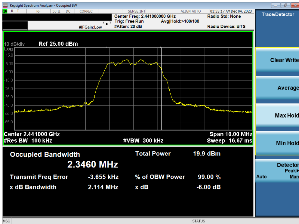
Plot 7-8. 6dB BW & 99% OBW Plot Antenna WF2b (Bluetooth (HDR4), 4Mbps, ePA – Ch. 38)
