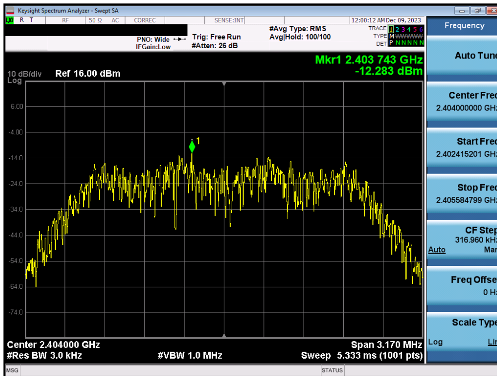
Plot 7-28. Power Spectral Density Plot Antenna WF2b (Bluetooth (HDR4), 4Mbps, iPA – Ch. 1)
