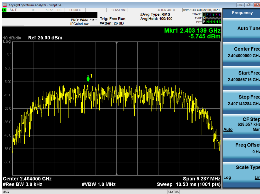
Plot 7-50. Power Spectral Density Plot TxBF Antenna WF2b (Bluetooth (HDR8), 8Mbps, ePA – Ch. 1)
