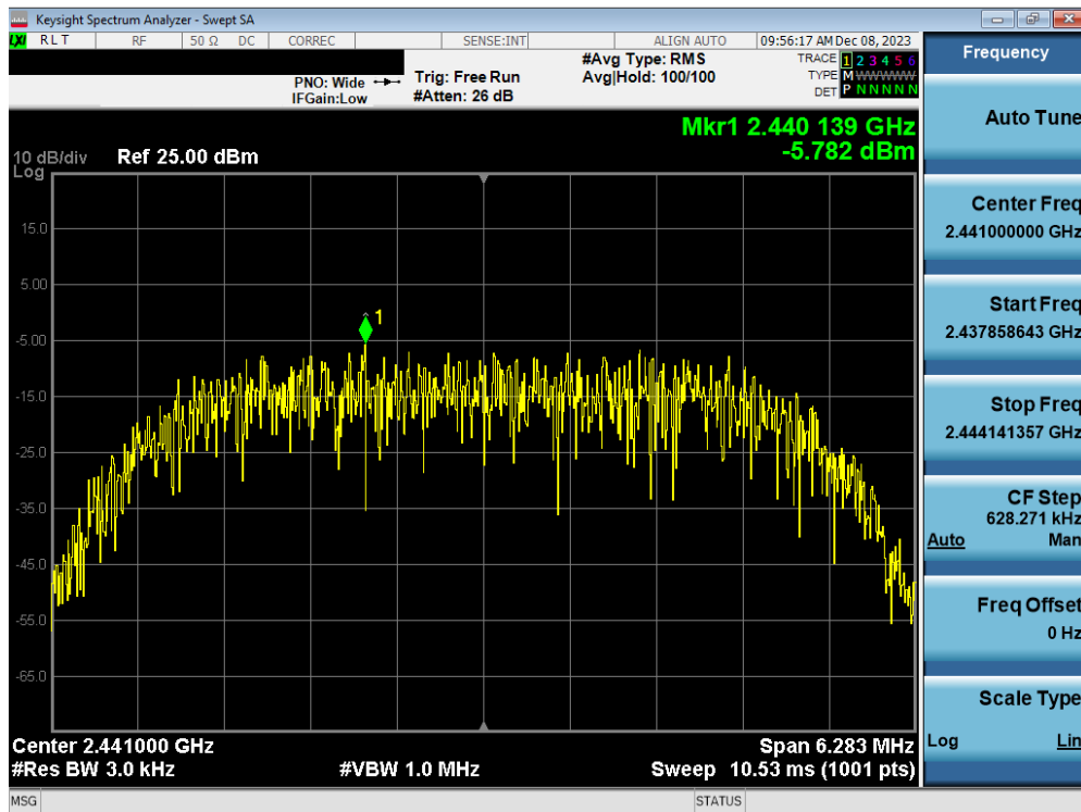
Plot 7-52. Power Spectral Density Plot TxBF Antenna WF2b (Bluetooth (HDR8), 8Mbps, ePA – Ch. 38)
