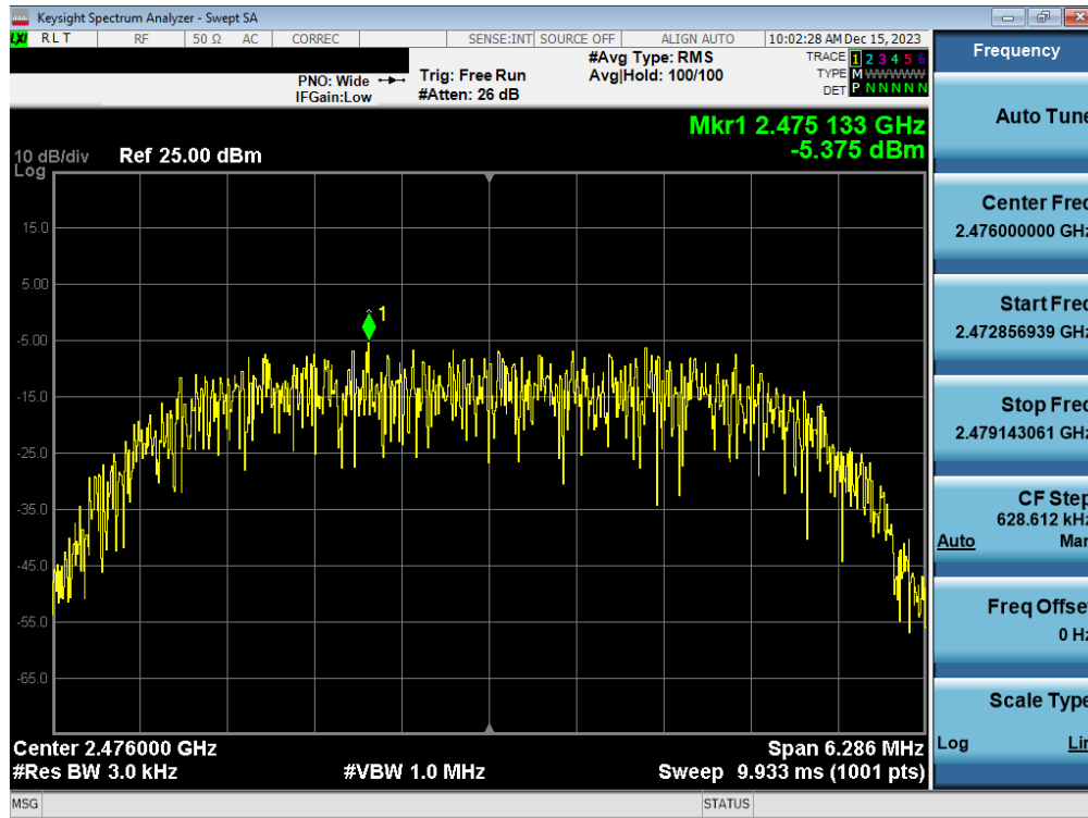
Plot 7-33. Power Spectral Density Plot Antenna WF2b (Bluetooth (HDR8), 8Mbps, ePA – Ch. 73)
