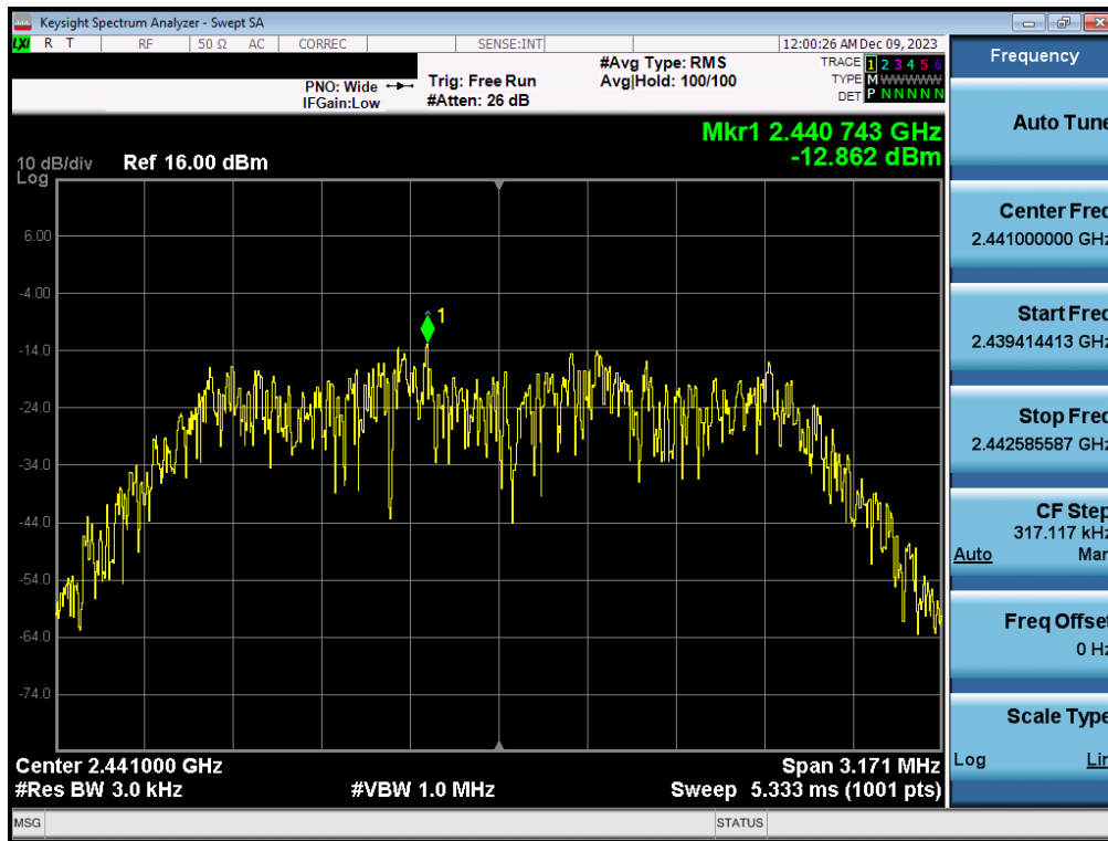
Plot 7-29. Power Spectral Density Plot Antenna WF2b (Bluetooth (HDR4), 4Mbps, iPA – Ch. 38)
