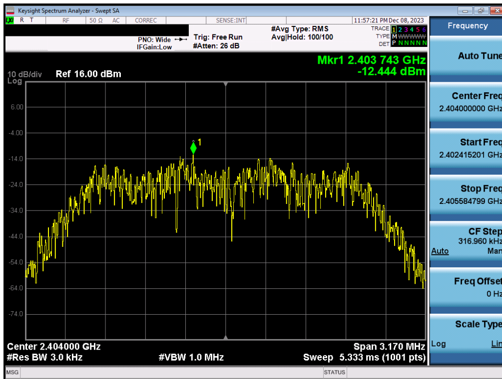
Plot 7-44. Power Spectral Density Plot TxBF Antenna WF2b (Bluetooth (HDR4), 4Mbps, iPA – Ch. 1)
