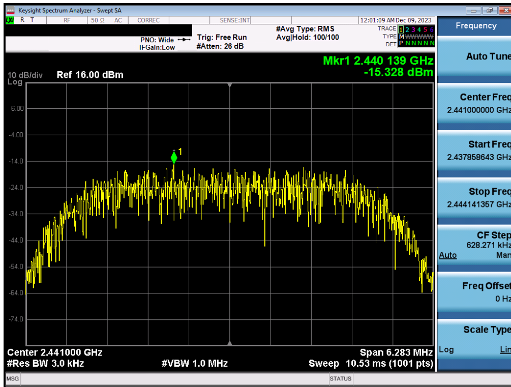
Plot 7-35. Power Spectral Density Plot Antenna WF2b (Bluetooth (HDR8), 8Mbps, iPA – Ch. 38)
