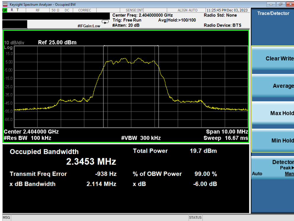
Plot 7-1. 6dB BW & 99% OBW Plot Antenna WF7b (Bluetooth (HDR4), 4Mbps, ePA – Ch. 1)
