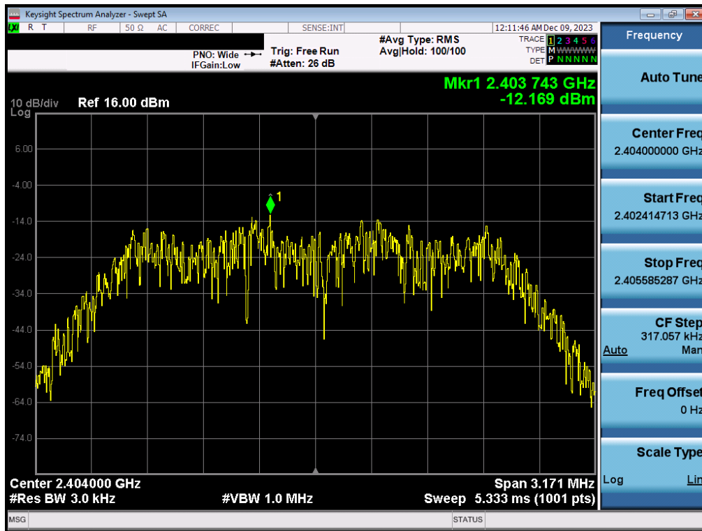
Plot 7-43. Power Spectral Density Plot TxBF Antenna WF7b (Bluetooth (HDR4), 4Mbps, iPA – Ch. 1)
