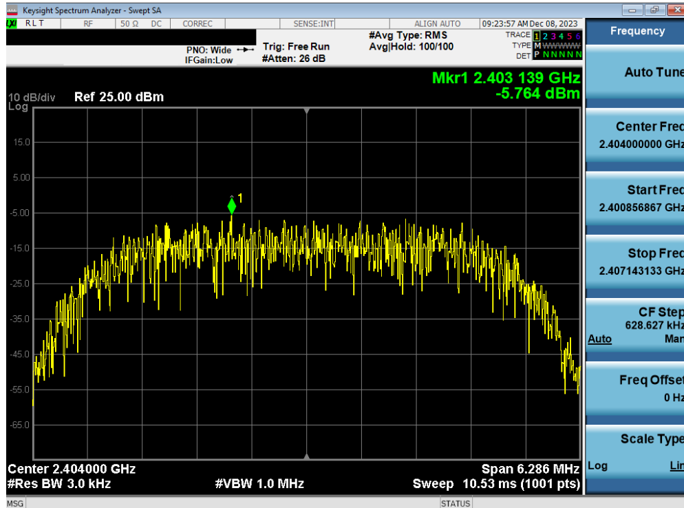
Plot 7-49. Power Spectral Density Plot TxBF Antenna WF7b (Bluetooth (HDR8), 8Mbps, ePA – Ch. 1)
