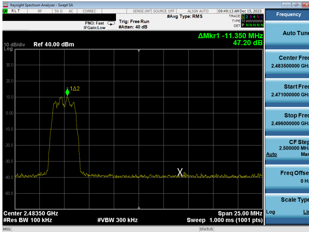
Plot 7-62. Band Edge Plot Antenna WF7b (Bluetooth (HDR4), ePA – Ch. 73)
