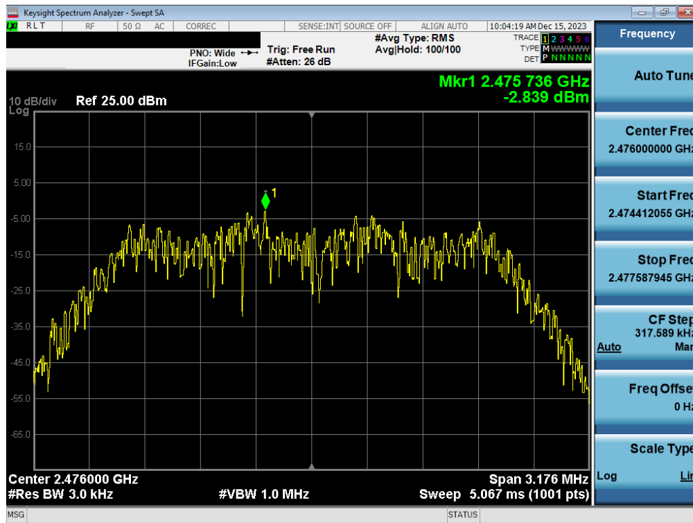
Plot 7-42. Power Spectral Density Plot TxBF Antenna WF2b (Bluetooth (HDR4), 4Mbps, ePA – Ch. 73)
