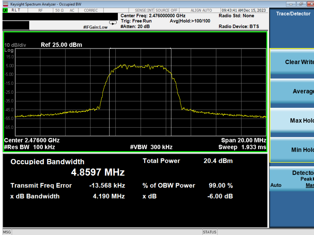
Plot 7-6. 6dB BW & 99% OBW Plot Antenna WF7b (Bluetooth (HDR8), 8Mbps, ePA – Ch. 73)
