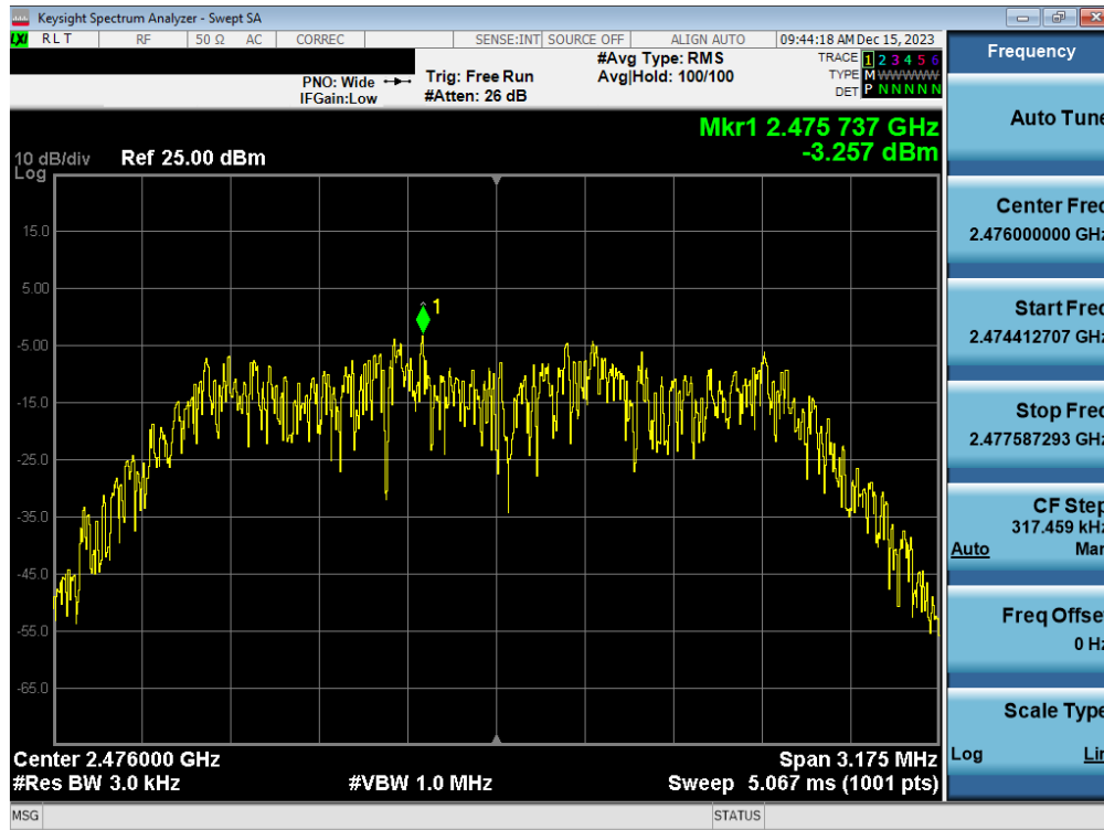
Plot 7-15. Power Spectral Density Plot Antenna WF7b (Bluetooth (HDR4), 4Mbps, ePA – Ch. 73)
