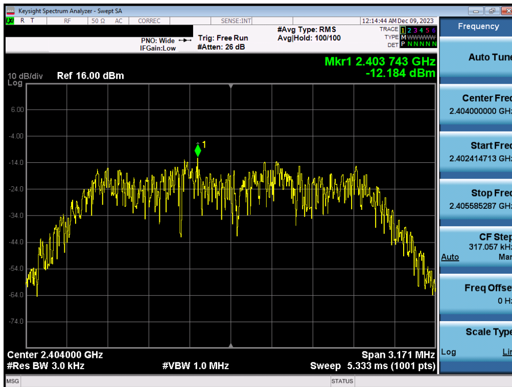
Plot 7-16. Power Spectral Density Plot Antenna WF7b (Bluetooth (HDR4), 4Mbps, iPA – Ch. 1)
