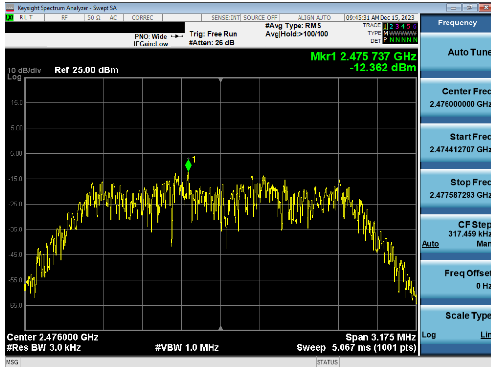
Plot 7-18. Power Spectral Density Plot Antenna WF7b (Bluetooth (HDR4), 4Mbps, iPA – Ch. 73)
