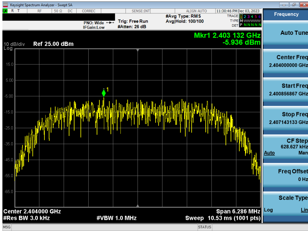
Plot 7-19. Power Spectral Density Plot Antenna WF7b (Bluetooth (HDR8), 8Mbps, ePA – Ch. 1)
