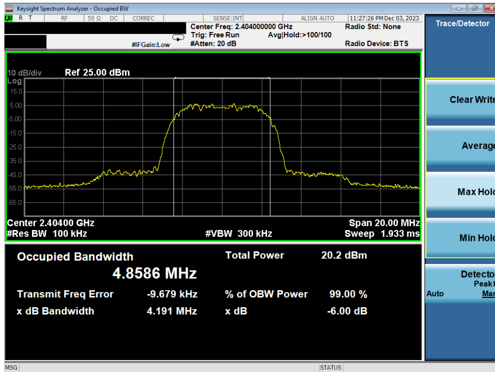
Plot 7-4. 6dB BW & 99% OBW Plot Antenna WF7b (Bluetooth (HDR8), 8Mbps, ePA – Ch. 1)
