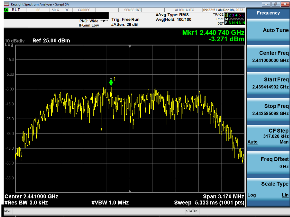
Plot 7-39. Power Spectral Density Plot TxBF Antenna WF7b (Bluetooth (HDR4), 4Mbps, ePA – Ch. 38)
