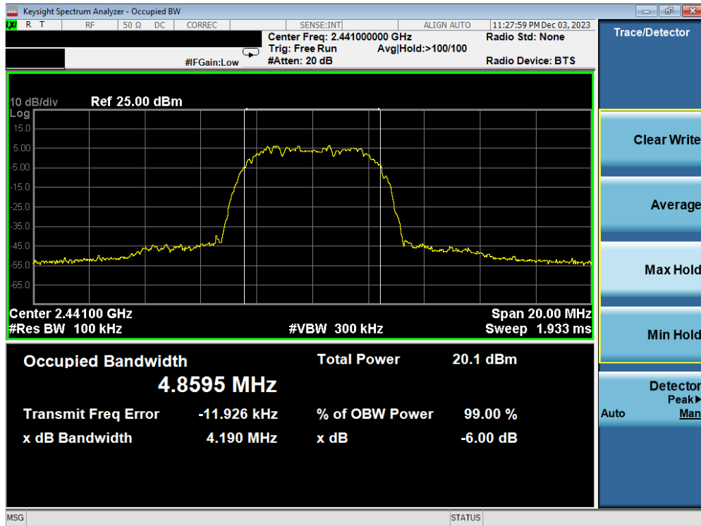
Plot 7-5. 6dB BW & 99% OBW Plot Antenna WF7b (Bluetooth (HDR8), 8Mbps, ePA – Ch. 38)
