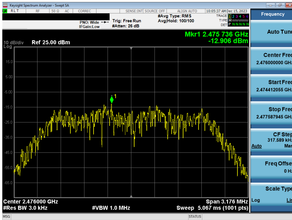
Plot 7-48. Power Spectral Density Plot TxBF Antenna WF2b (Bluetooth (HDR4), 4Mbps, iPA – Ch. 73)
