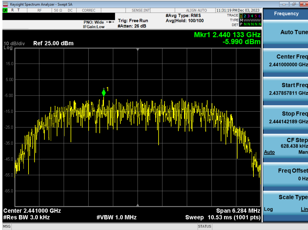
Plot 7-20. Power Spectral Density Plot Antenna WF7b (Bluetooth (HDR8), 8Mbps, ePA – Ch. 38)
