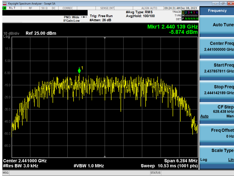
Plot 7-51. Power Spectral Density Plot TxBF Antenna WF7b (Bluetooth (HDR8), 8Mbps, ePA – Ch. 38)
