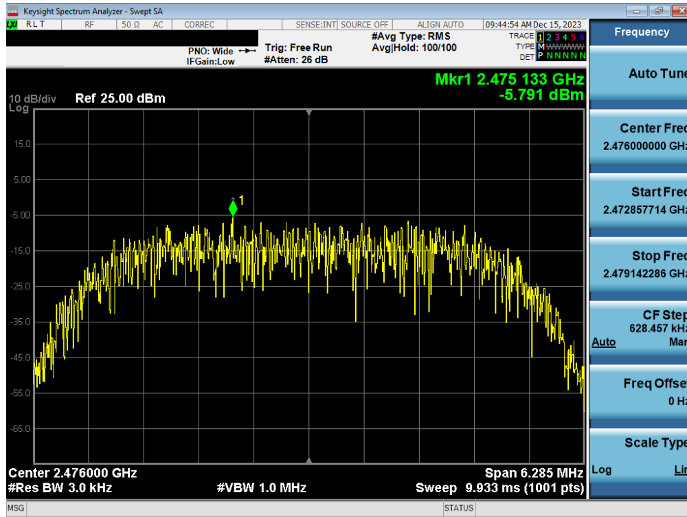
Plot 7-21. Power Spectral Density Plot Antenna WF7b (Bluetooth (HDR8), 8Mbps, ePA – Ch. 73)
