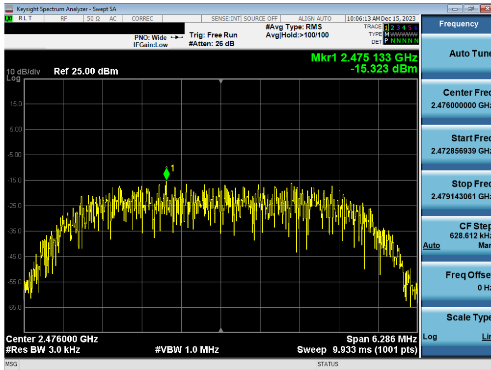
Plot 7-60. Power Spectral Density Plot Tx BF Antenna WF2b (Bluetooth (HDR8), 8Mbps, iPA – Ch. 73)
