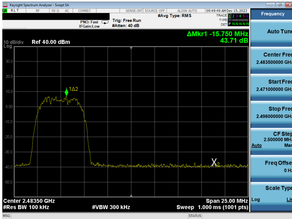
Plot 7-64. Band Edge Plot Antenna WF7b (Bluetooth (HDR8), ePA – Ch. 73)
