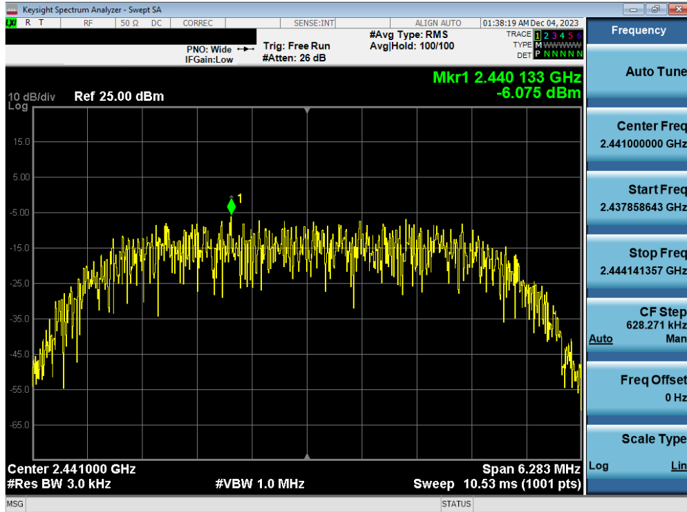
Plot 7-32. Power Spectral Density Plot Antenna WF2b (Bluetooth (HDR8), 8Mbps, ePA – Ch. 38)
