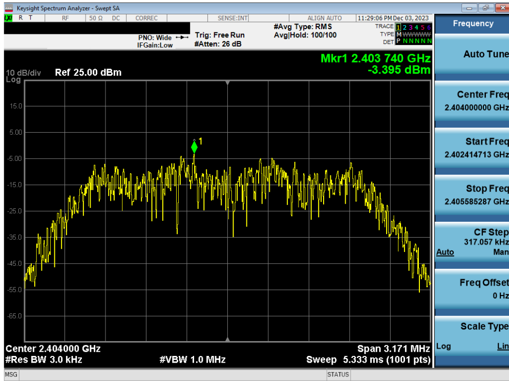
Plot 7-13. Power Spectral Density Plot Antenna WF7b (Bluetooth (HDR4), 4Mbps, ePA – Ch. 1)
