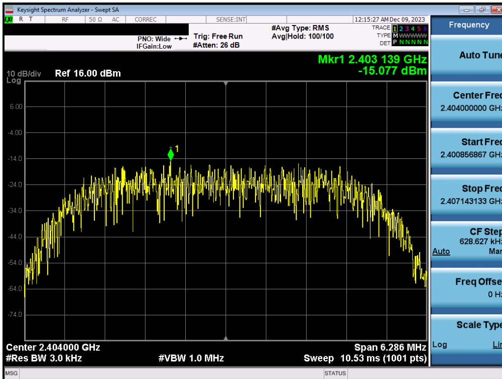
Plot 7-22. Power Spectral Density Plot Antenna WF7b (Bluetooth (HDR8), 8Mbps, iPA – Ch. 1)
