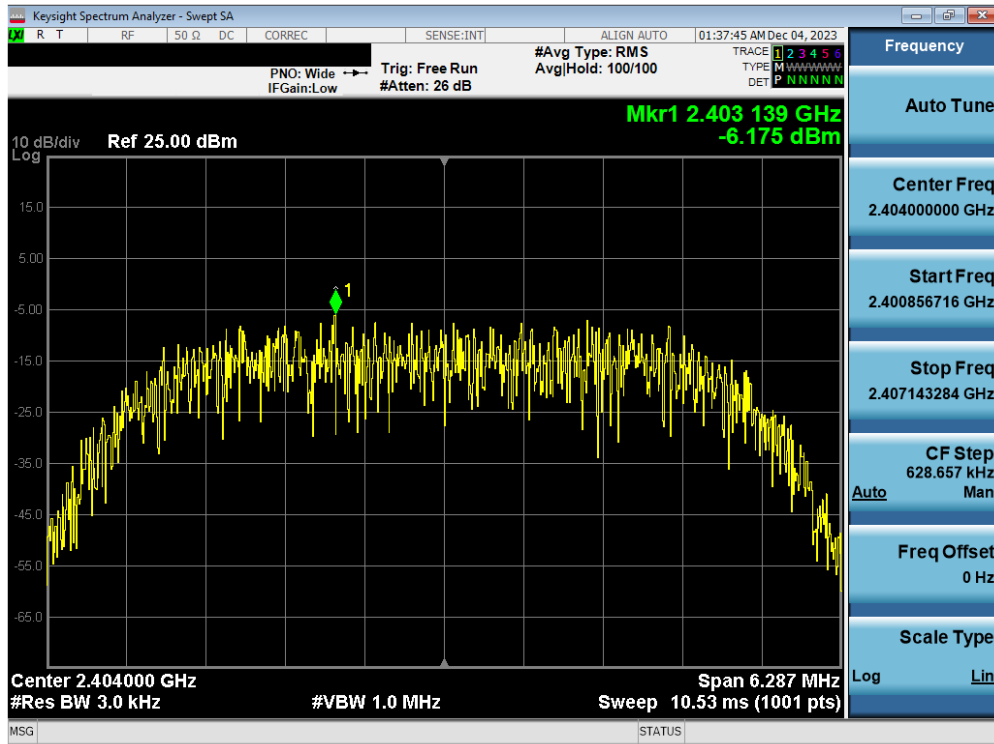
Plot 7-31. Power Spectral Density Plot Antenna WF2b (Bluetooth (HDR8), 8Mbps, ePA – Ch. 1)
