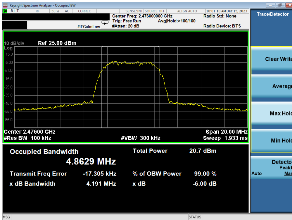
Plot 7-12. 6dB BW & 99% OBW Plot Antenna WF2b (Bluetooth (HDR8), 8Mbps, ePA – Ch. 73)
