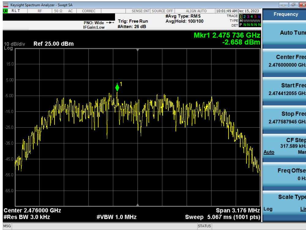
Plot 7-27. Power Spectral Density Plot Antenna WF2b (Bluetooth (HDR4), 4Mbps, ePA – Ch. 73)
