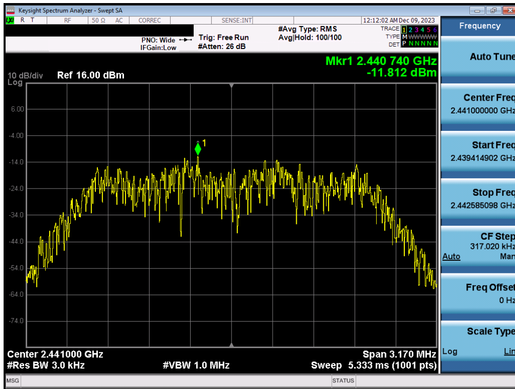
Plot 7-45. Power Spectral Density Plot TxBF Antenna WF7b (Bluetooth (HDR4), 4Mbps, iPA – Ch. 38)
