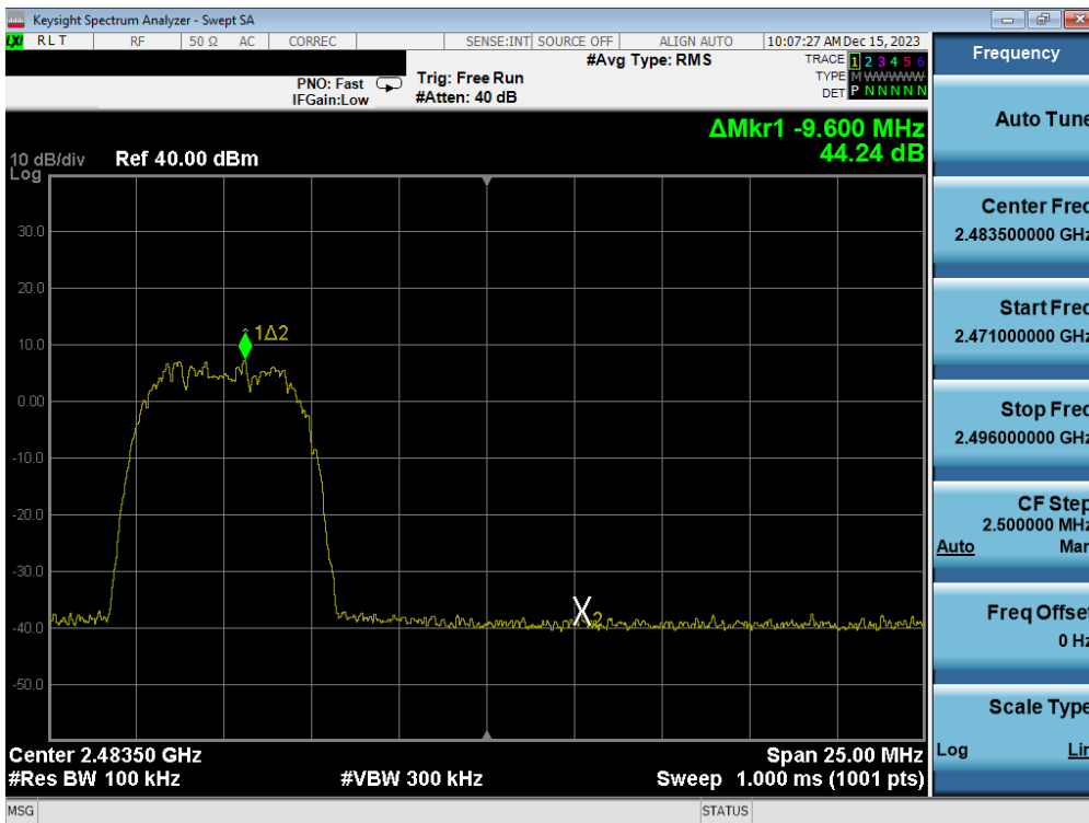
Plot 7-68. Band Edge Plot Antenna WF2b (Bluetooth (HDR8), ePA – Ch. 73)
