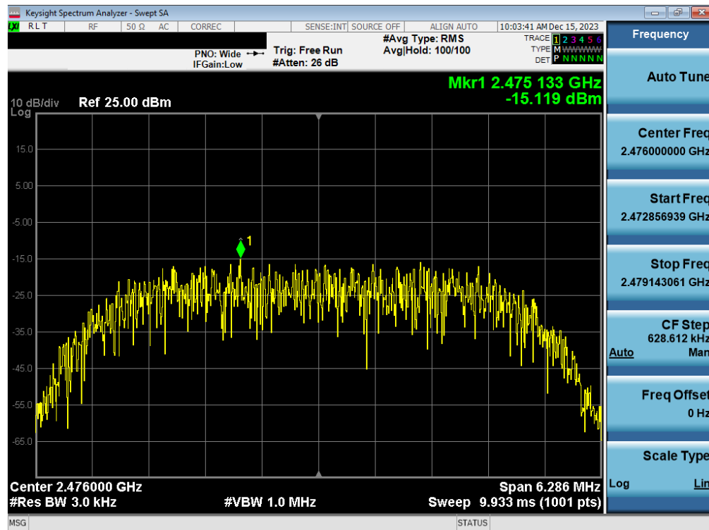
Plot 7-36. Power Spectral Density Plot Antenna WF2b (Bluetooth (HDR8), 8Mbps, iPA – Ch. 73)
