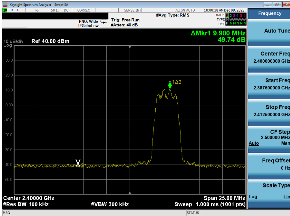
Plot 7-65. Band Edge Plot Antenna WF2b (Bluetooth (HDR4), ePA – Ch. 1)
