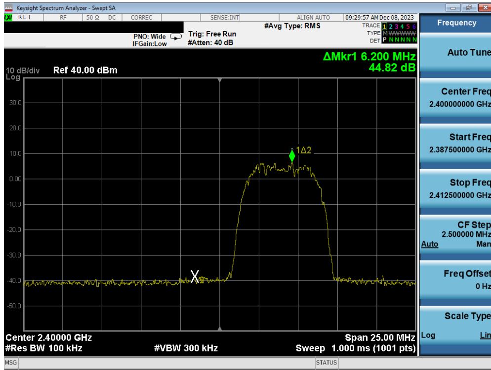
Plot 7-63. Band Edge Plot Antenna WF7b (Bluetooth (HDR8), ePA – Ch. 1)
