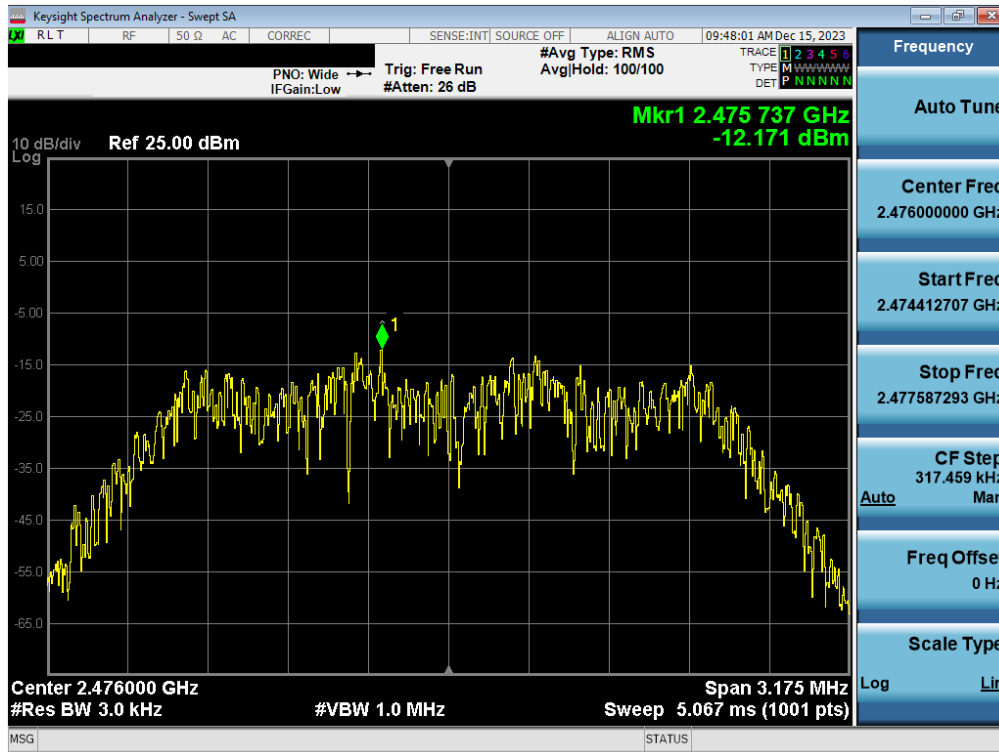
Plot 7-47. Power Spectral Density Plot TxBF Antenna WF7b (Bluetooth (HDR4), 4Mbps, iPA – Ch. 73)
