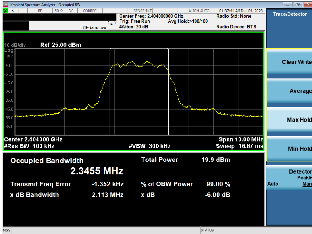
Plot 7-7. 6dB BW & 99% OBW Plot Antenna WF2b (Bluetooth (HDR4), 4Mbps, ePA – Ch. 1)
