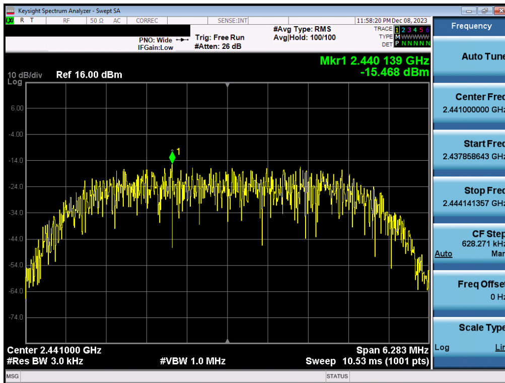
Plot 7-58. Power Spectral Density Plot TxBF Antenna WF2b (Bluetooth (HDR8), 8Mbps, iPA – Ch. 38)
