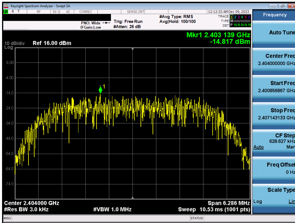
Plot 7-55. Power Spectral Density Plot TxBF Antenna WF7b (Bluetooth (HDR8), 8Mbps, iPA – Ch. 1)
