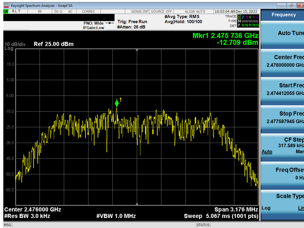
Plot 7-30. Power Spectral Density Plot Antenna WF2b (Bluetooth (HDR4), 4Mbps, iPA – Ch. 73)
