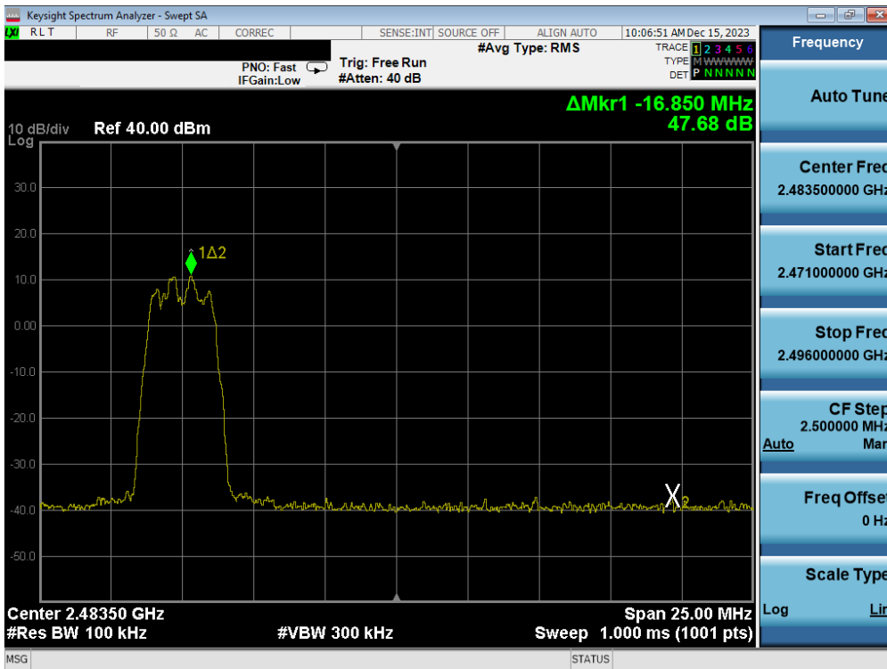
Plot 7-66. Band Edge Plot Antenna WF2b (Bluetooth (HDR4), ePA – Ch. 73)
