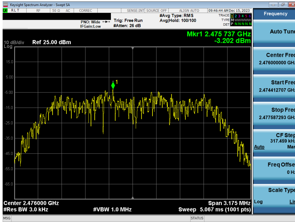
Plot 7-41. Power Spectral Density Plot TxBF Antenna WF7b (Bluetooth (HDR4), 4Mbps, ePA – Ch. 73)
