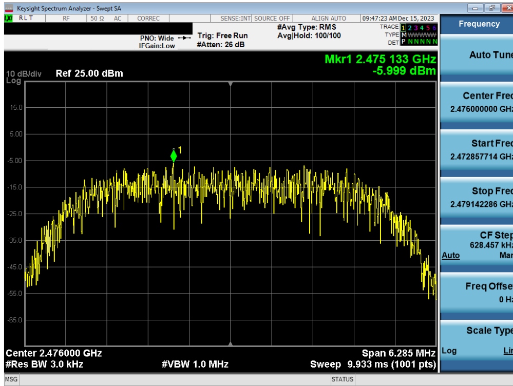
Plot 7-53. Power Spectral Density Plot Tx BF Antenna WF7b (Bluetooth (HDR8), 8Mbps, ePA – Ch. 73)
