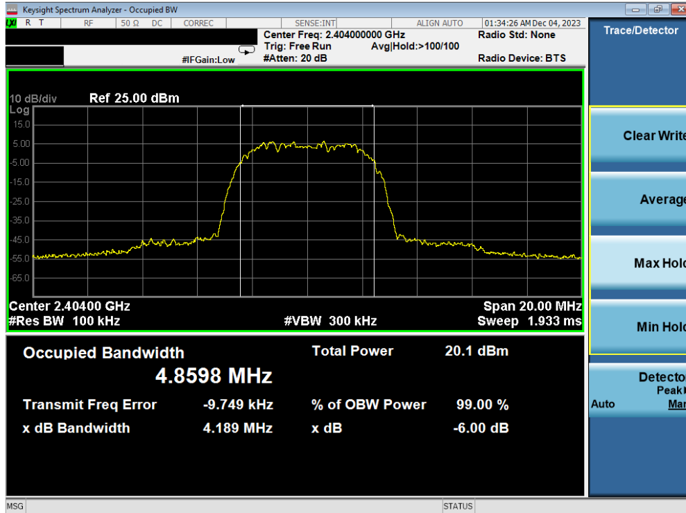
Plot 7-10. 6dB BW & 99% OBW Plot Antenna WF2b (Bluetooth (HDR8), 8Mbps, ePA – Ch. 1)
