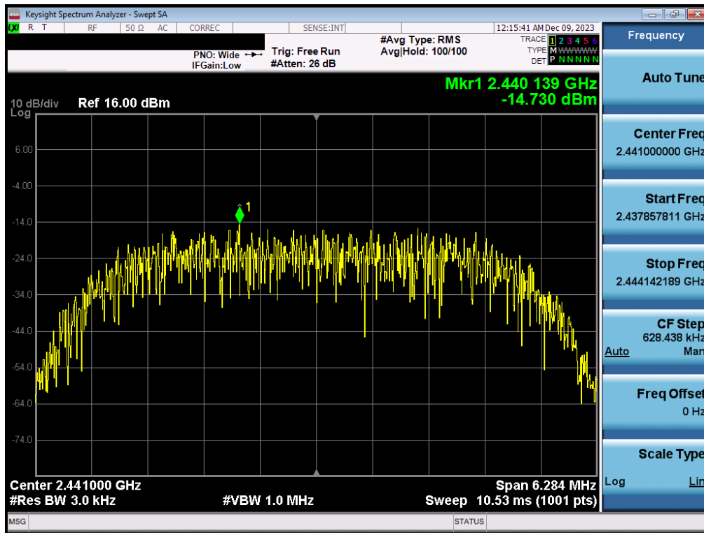
Plot 7-23. Power Spectral Density Plot Antenna WF7b (Bluetooth (HDR8), 8Mbps, iPA – Ch. 38)
