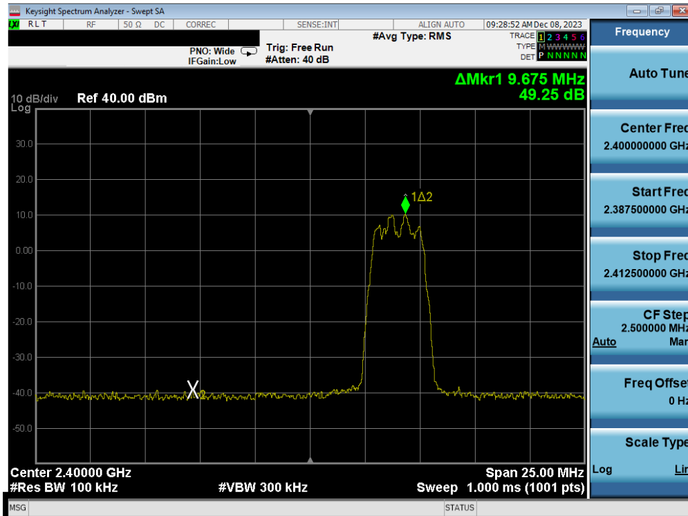
Plot 7-61. Band Edge Plot Antenna WF7b (Bluetooth (HDR4), ePA – Ch. 1)
