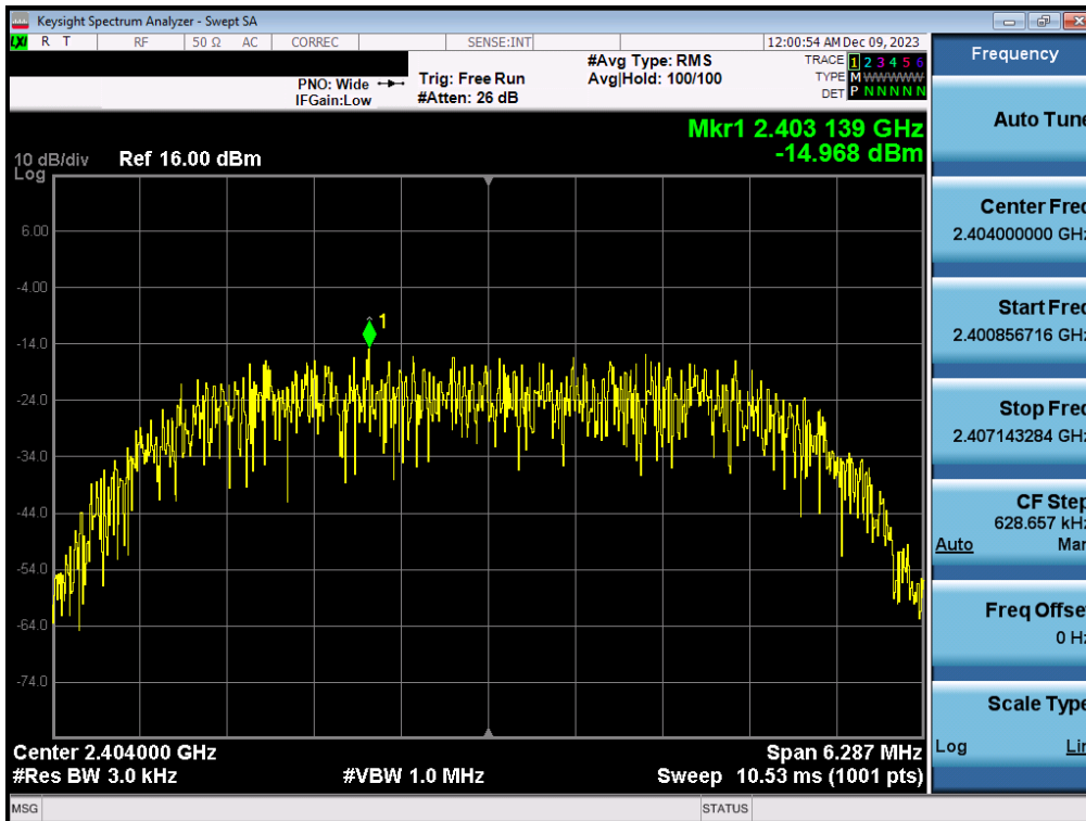
Plot 7-34. Power Spectral Density Plot Antenna WF2b (Bluetooth (HDR8), 8Mbps, iPA – Ch. 1)
