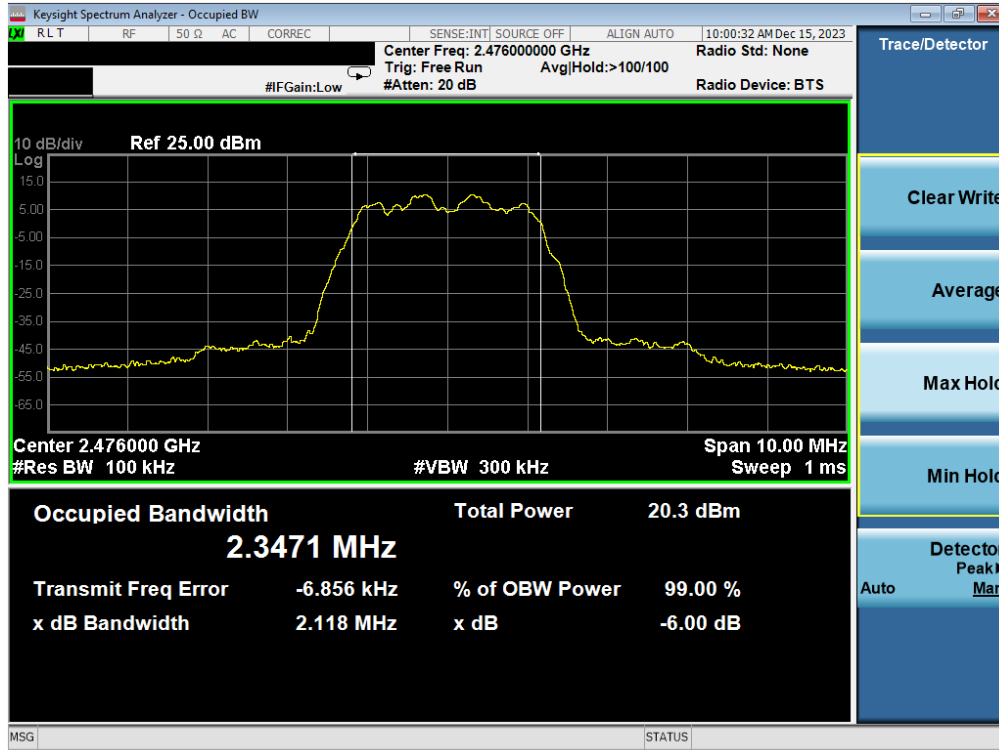
Plot 7-9. 6dB BW & 99% OBW Plot Antenna WF2b (Bluetooth (HDR4), 4Mbps, ePA – Ch. 73)
