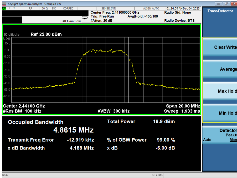
Plot 7-11. 6dB BW & 99% OBW Plot Antenna WF2b (Bluetooth (HDR8), 8Mbps, ePA – Ch. 38)
