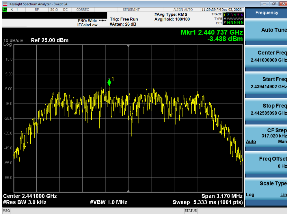
Plot 7-14. Power Spectral Density Plot Antenna WF7b (Bluetooth (HDR4), 4Mbps, ePA – Ch. 38)
