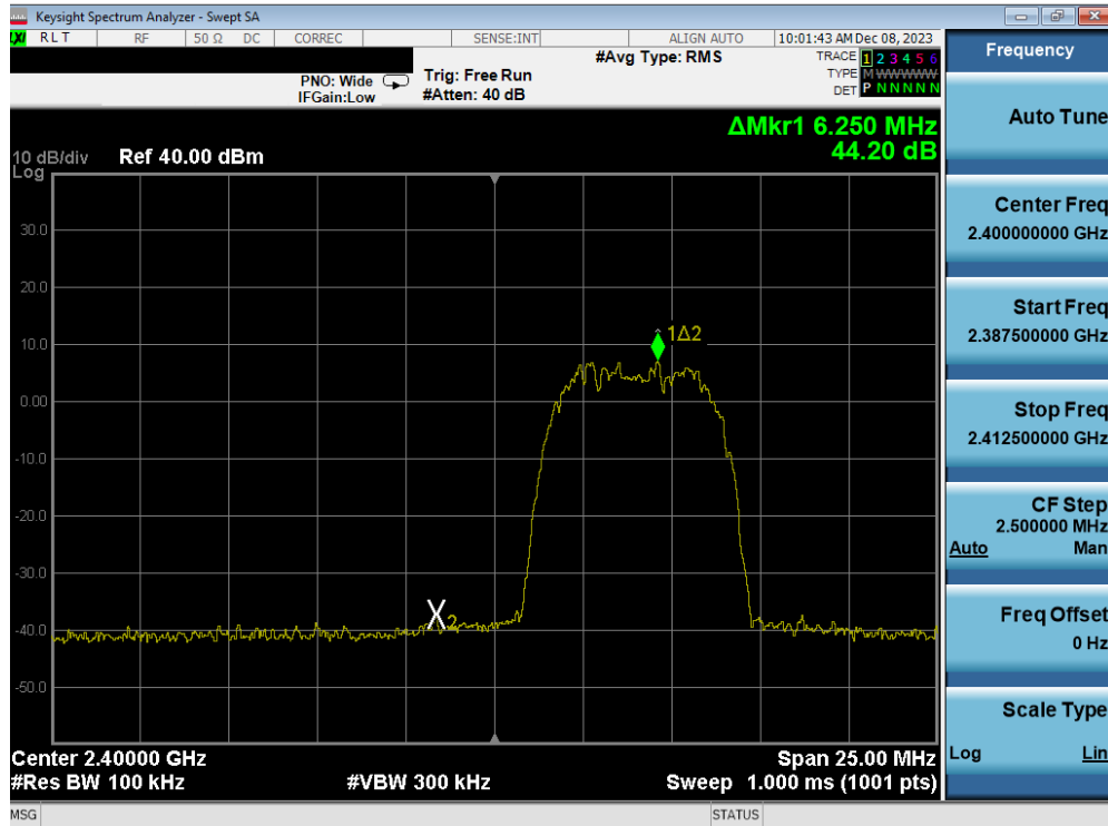
Plot 7-67. Band Edge Plot Antenna WF2b (Bluetooth (HDR8), ePA – Ch. 1)
