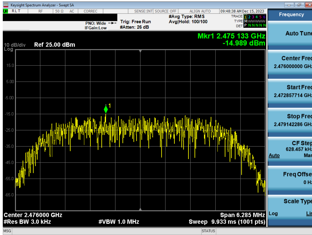
Plot 7-59. Power Spectral Density Plot Tx BF Antenna WF7b (Bluetooth (HDR8), 8Mbps, iPA – Ch. 73)
