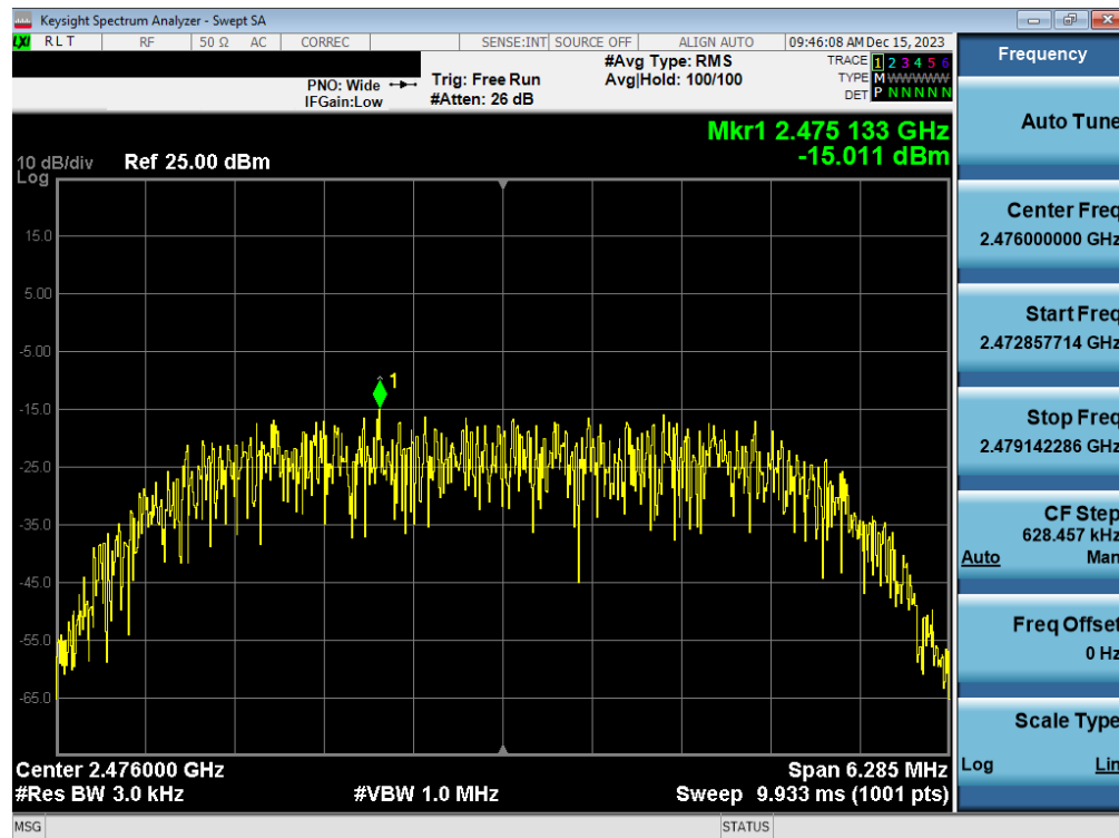
Plot 7-24. Power Spectral Density Plot Antenna WF7b (Bluetooth (HDR8), 8Mbps, iPA – Ch. 73)
