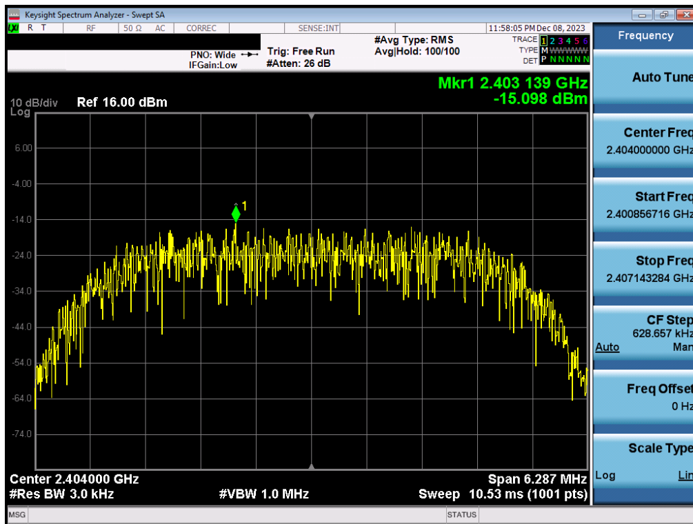
Plot 7-56. Power Spectral Density Plot TxBF Antenna WF2b (Bluetooth (HDR8), 8Mbps, iPA – Ch. 1)
