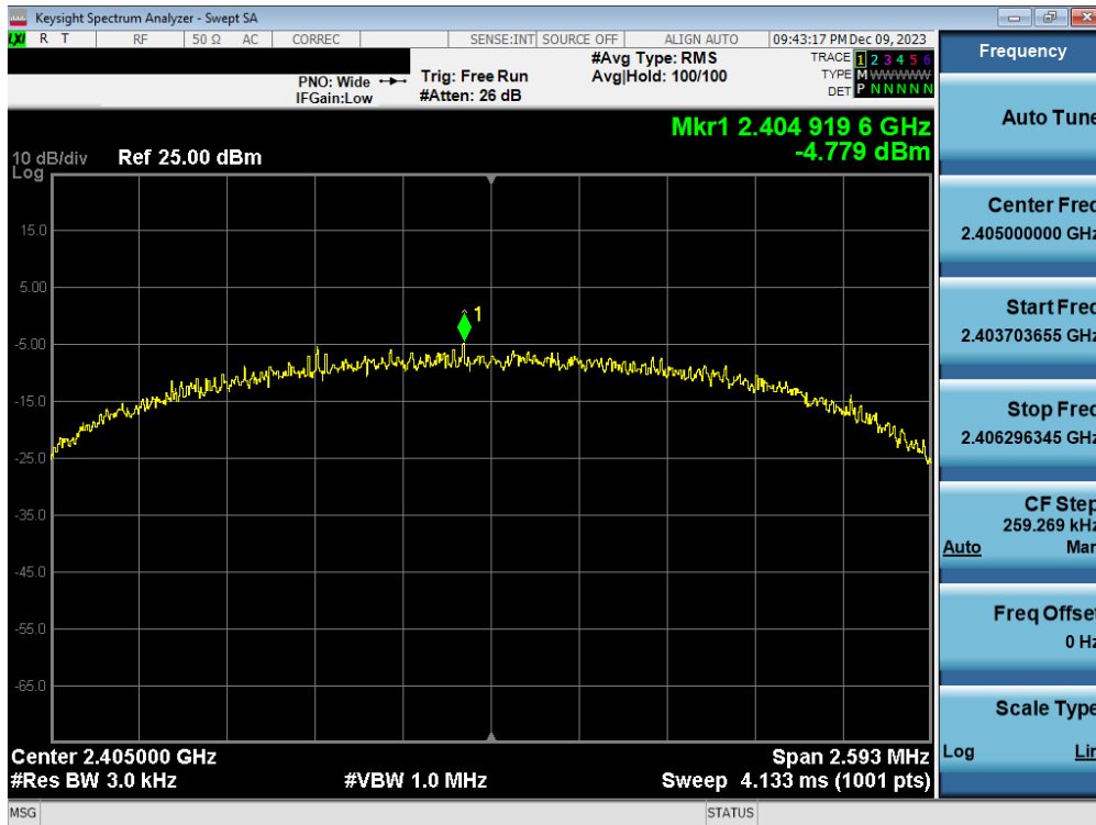
Plot 7-16. Power Spectral Density Antenna WF2b (802.15.4, iPA – Ch. 11)
