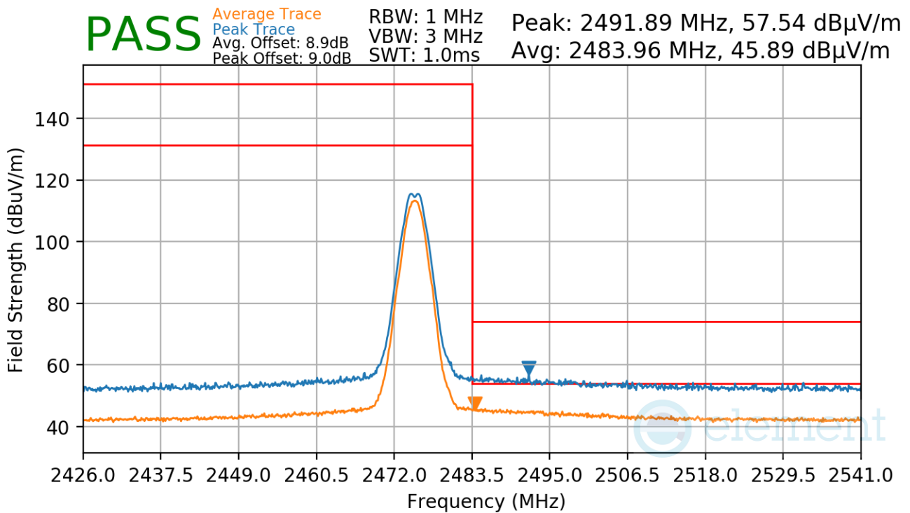
Plot 7-43. Radiated Restricted Upper Band Edge Measurement Antenna WF7b
