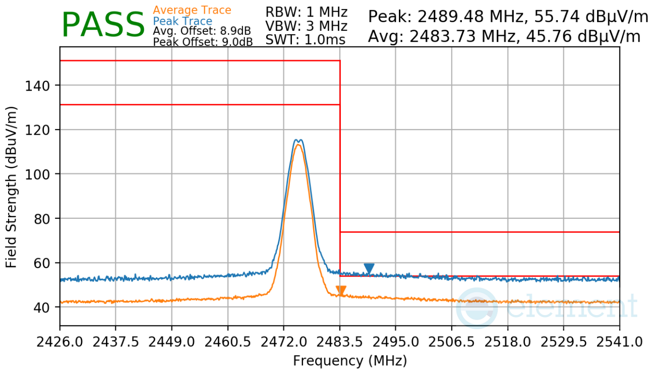
Plot 7-45. Radiated Restricted Upper Band Edge Measurement Antenna WF2b
