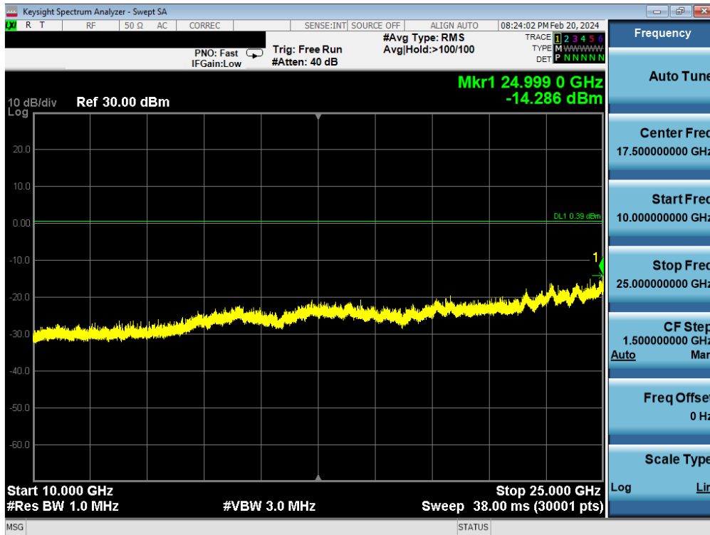
Plot 7-28. Conducted Spurious Antenna WF7b (802.15.4, ePA – Ch. 25)
