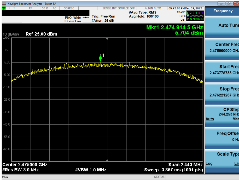
Plot 7-15. Power Spectral Density Antenna WF2b (802.15.4, ePA – Ch. 25)
