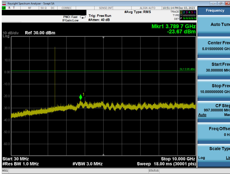
Plot 7-45. Conducted Spurious Plot Antenna WF7b (Bluetooth, GFSK, ePA – Ch. 0)
