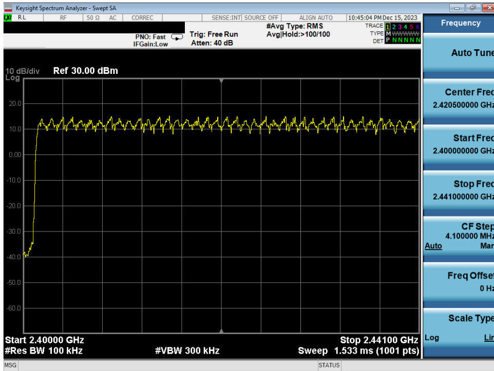
Plot 7-43. Low End Spectrum Channel Hopping Plot Antenna WF2b (Bluetooth, 8DPSK, ePA)
