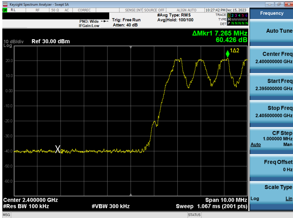
Plot 7-23. Band Edge Plot Antenna WF2b (Bluetooth with Hopping Enabled, GFSK, ePA)
