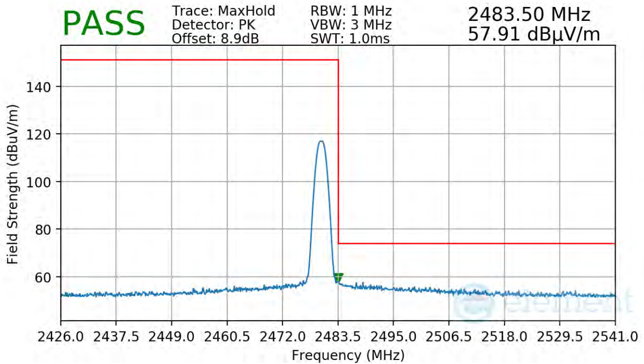
Plot 7-73. Radiated Restricted Upper Band Edge Measurement Antenna WF7b
