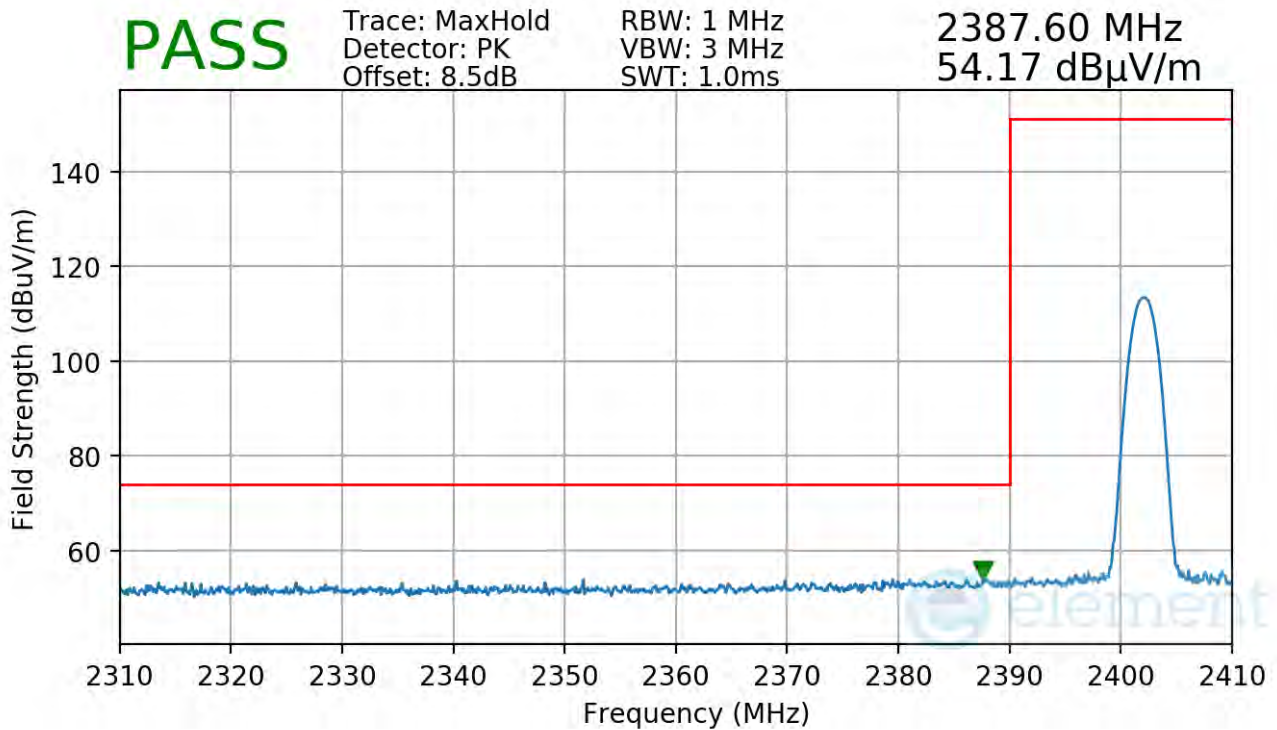
Plot 7-72. Radiated Restricted Lower Band Edge Measurement Antenna WF7b
