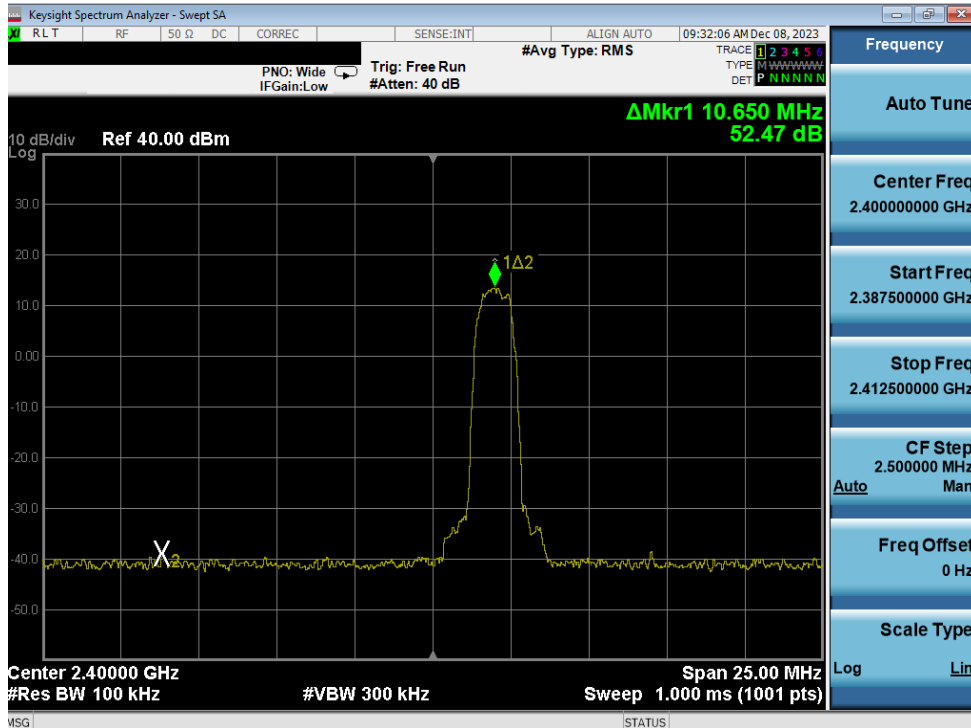
Plot 7-17. Band Edge Plot Antenna WF7b (Bluetooth with Hopping Disabled, 8DPSK, ePA – Ch. 0)
