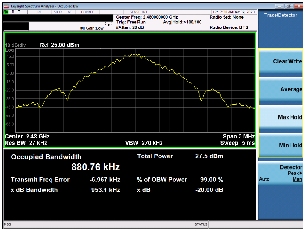
Plot 7-3. 20dB BW and 99% OBW Plot Antenna WF7b (Bluetooth, GFSK, ePA – Ch. 78)
