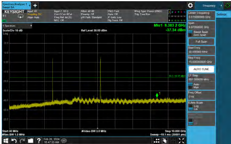
Plot 7-57. Conducted Simultaneous Tx Spurious Plot Antenna WF7b (Bluetooth + UNII)
