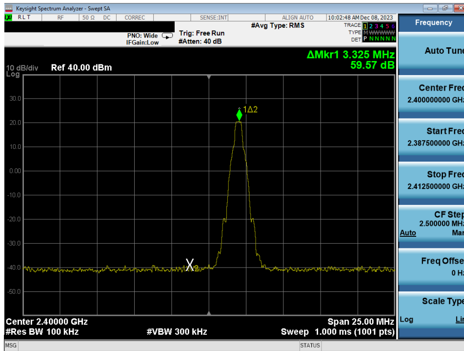
Plot 7-21. Band Edge Plot Antenna WF2b (Bluetooth with Hopping Disabled, GFSK, ePA – Ch. 0)
