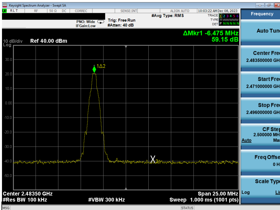
Plot 7-22. Band Edge Plot Antenna WF2b (Bluetooth with Hopping Disabled, GFSK, ePA – Ch. 78)
