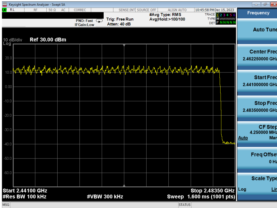
Plot 7-44. High End Spectrum Channel Hopping Plot Antenna WF2b (Bluetooth, 8DPSK, ePA)
