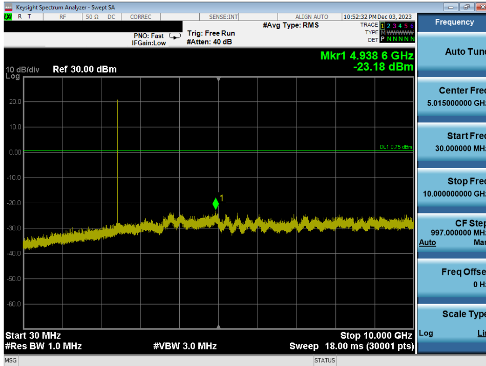
Plot 7-47. Conducted Spurious Plot Antenna WF7b (Bluetooth, GFSK, ePA – Ch. 39)
