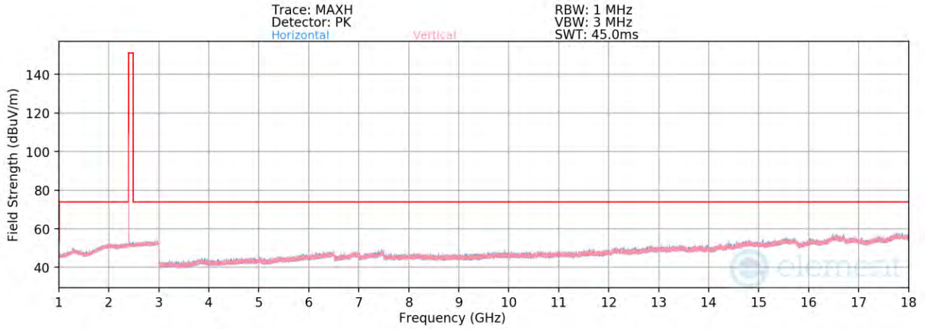
Plot 7-62. Radiated Spurious Emissions above 1GHz Antenna WF2b (BT GFSK ePA – Ch. 0)
