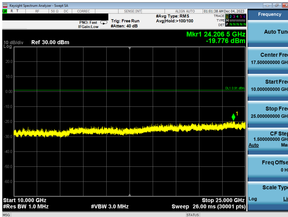
Plot 7-56. Conducted Spurious Plot Antenna WF2b (Bluetooth, GFSK, ePA – Ch. 78)
