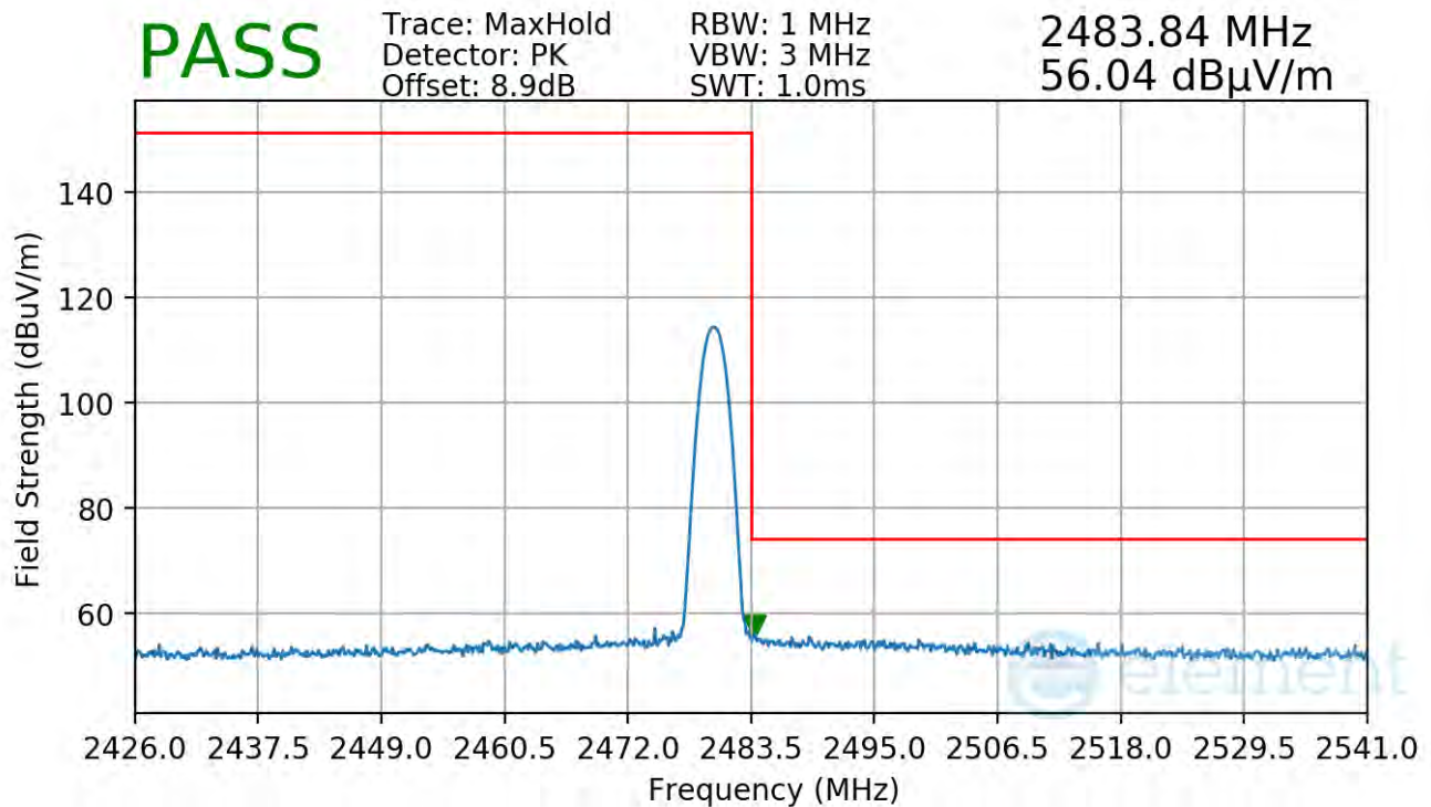
Plot 7-74. Radiated Restricted Upper Band Edge Measurement Antenna WF7b
