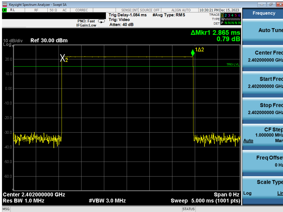
Plot 7-35. Time of Occupancy Plot Antenna WF2b (Bluetooth, GFSK, ePA)
