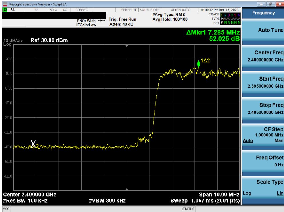
Plot 7-19. Band Edge Plot Antenna WF7b (Bluetooth with Hopping Enabled, 8DPSK, ePA)
