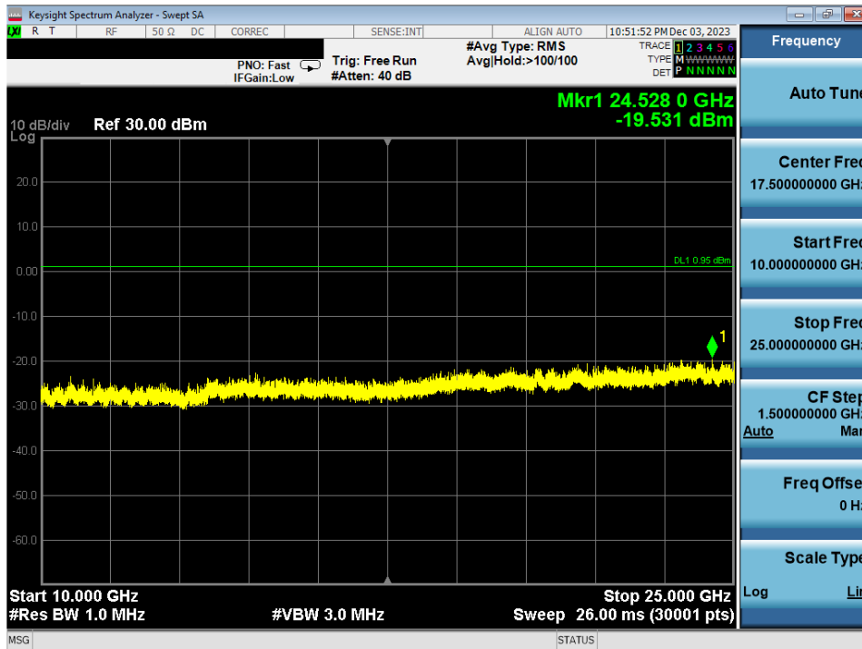
Plot 7-46. Conducted Spurious Plot Antenna WF7b (Bluetooth, GFSK, ePA – Ch. 0)
