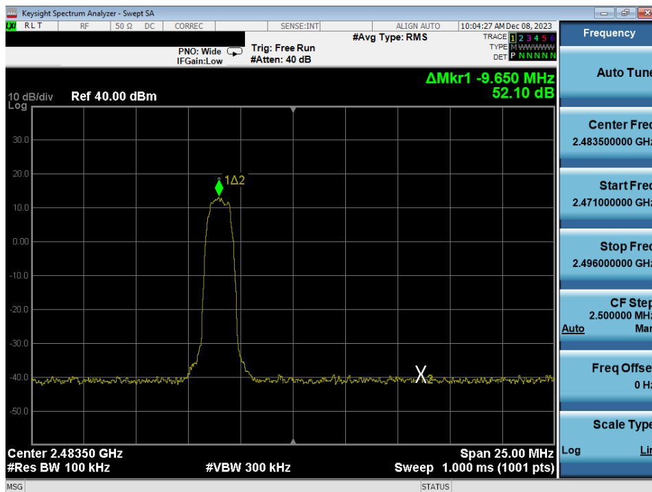
Plot 7-26. Band Edge Plot Antenna WF2b (Bluetooth with Hopping Disabled, 8DPSK, ePA – Ch. 78)
