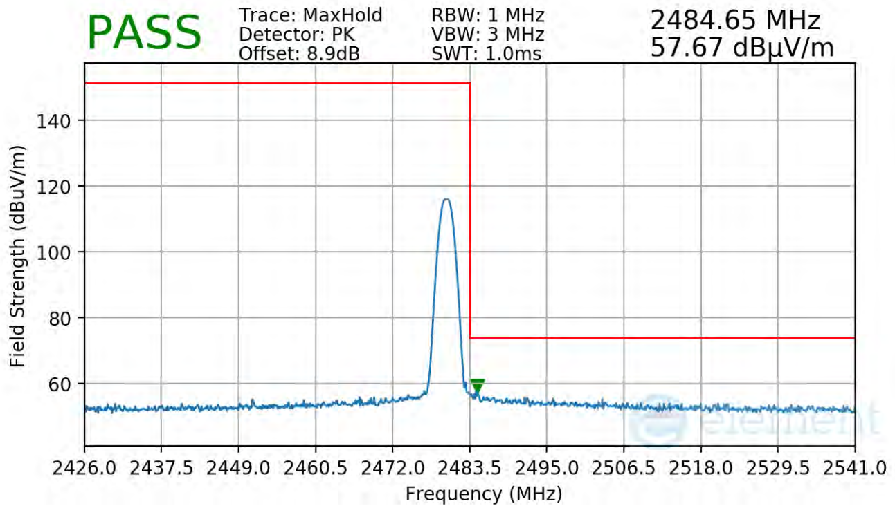
Plot 7-77. Radiated Restricted Upper Band Edge Measurement Antenna WF2b
