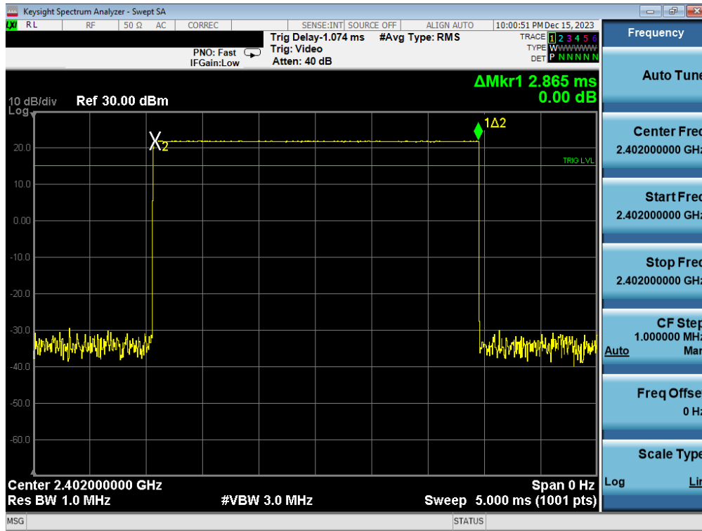
Plot 7-33. Time of Occupancy Plot Antenna WF7b (Bluetooth, GFSK, ePA)
