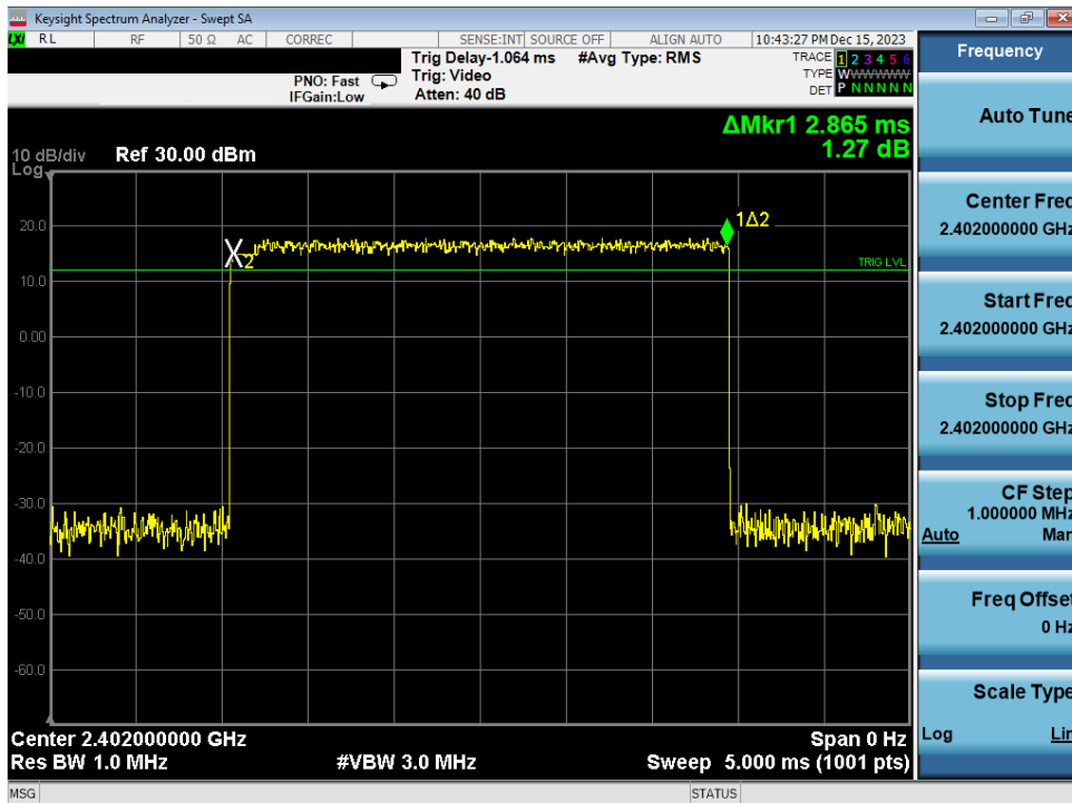
Plot 7-36. Time of Occupancy Plot Antenna WF2b (Bluetooth, 8DPSK, ePA)
