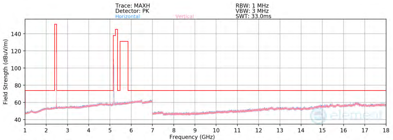
Plot 7-69. Radiated Spurious Emissions 1 - 18GHz – Simultaneous Transmission
