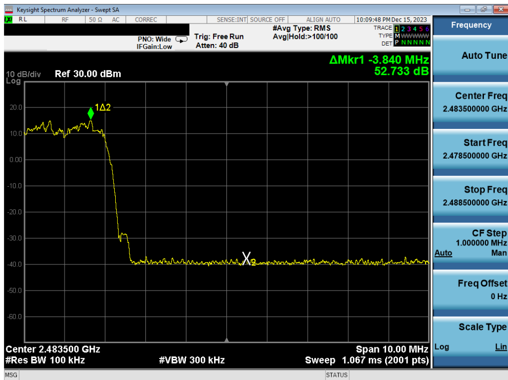
Plot 7-20. Band Edge Plot Antenna WF7b (Bluetooth with Hopping Enabled, 8DPSK, ePA)
