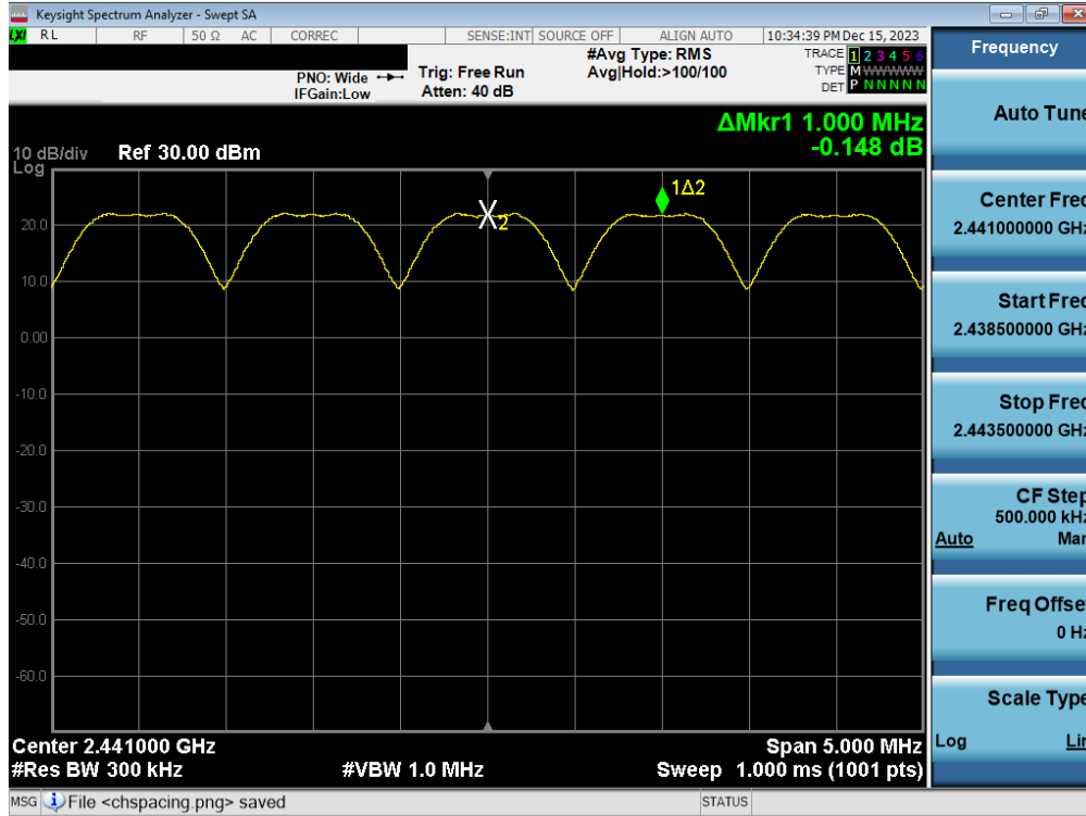
Plot 7-31. Channel Spacing Plot Antenna WF2b (Bluetooth, GFSK, ePA)
