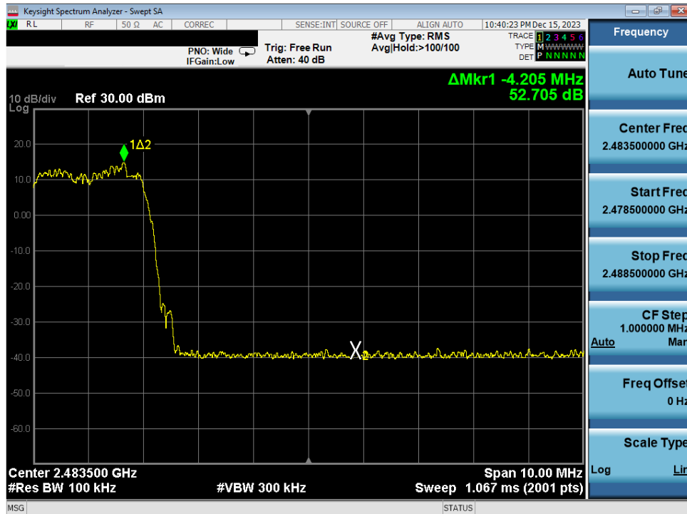
Plot 7-28. Band Edge Plot Antenna WF2b (Bluetooth with Hopping Enabled, 8DPSK, ePA)
