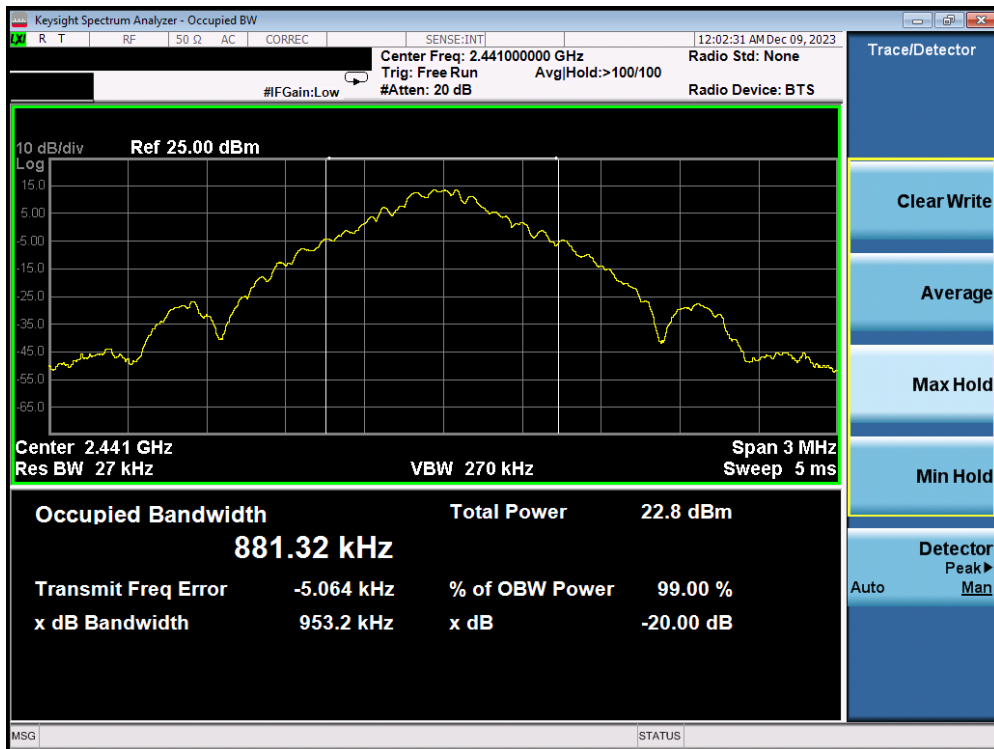
Plot 7-8. 20dB BW and 99% OBW Plot Antenna WF2b (Bluetooth, GFSK, ePA – Ch. 39)
