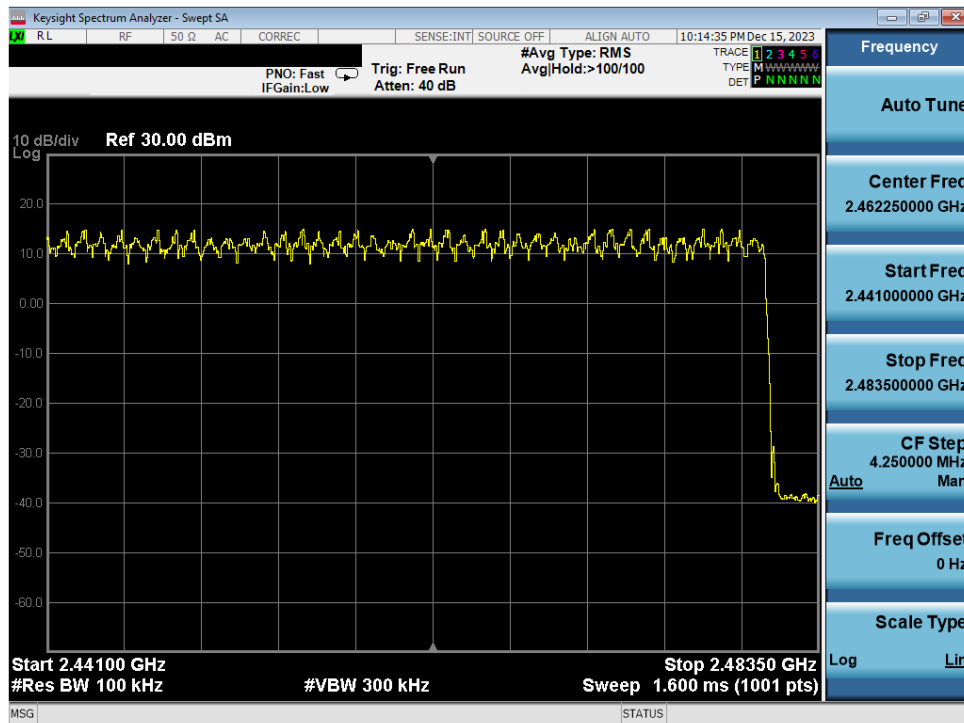
Plot 7-40. High End Spectrum Channel Hopping Plot Antenna WF7b (Bluetooth, 8DPSK, ePA)
