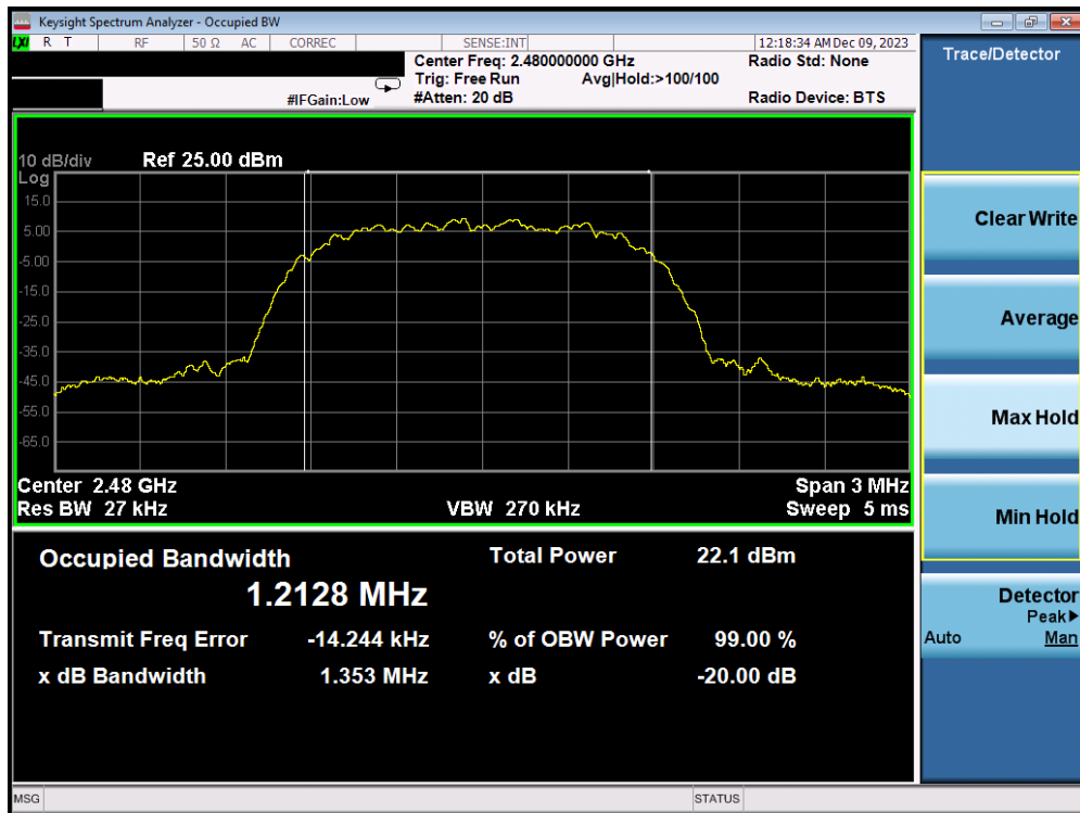
Plot 7-6. 20dB BW and 99% OBW Plot Antenna WF7b (Bluetooth, 8DPSK, ePA – Ch. 78)
