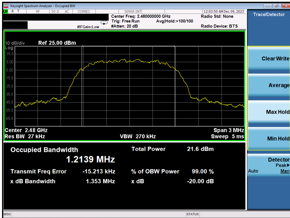
Plot 7-12. 20dB BW and 99% OBW Plot Antenna WF2b (Bluetooth, 8DPSK, ePA – Ch. 78)
