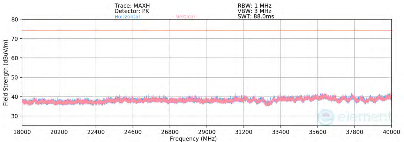
Plot 7-70. Radiated Spurious Emissions Above 18GHz – Simultaneous Transmission
