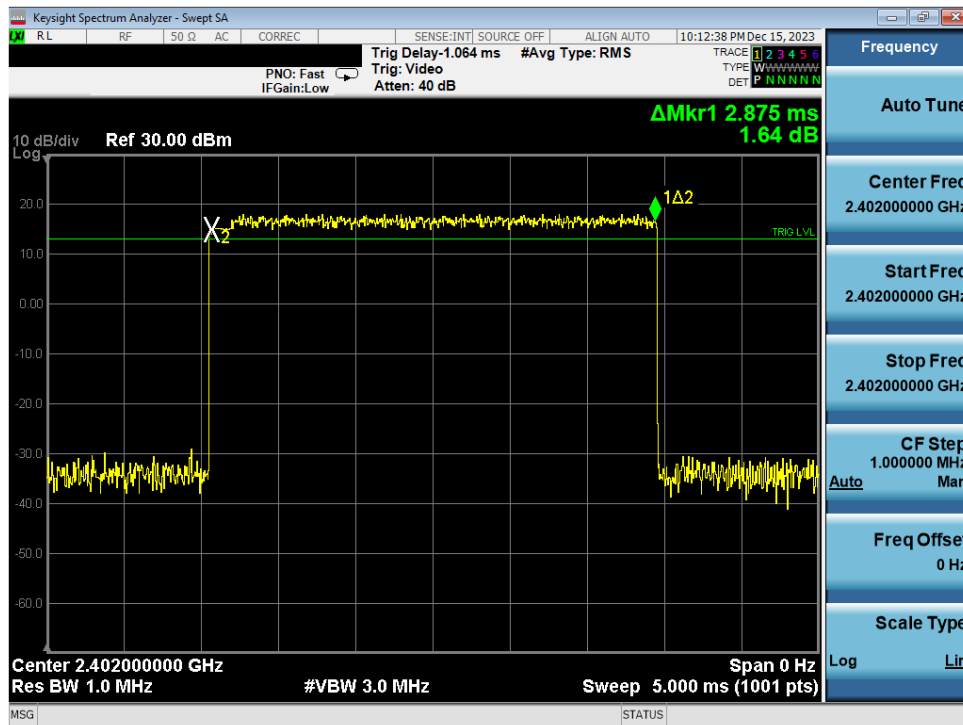
Plot 7-34. Time of Occupancy Plot Antenna WF7b (Bluetooth, 8DPSK, ePA)
