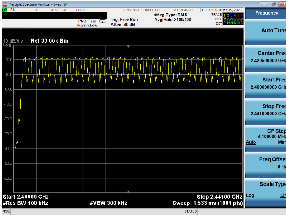
Plot 7-41. Low End Spectrum Channel Hopping Plot Antenna WF2b (Bluetooth, GFSK, ePA)
