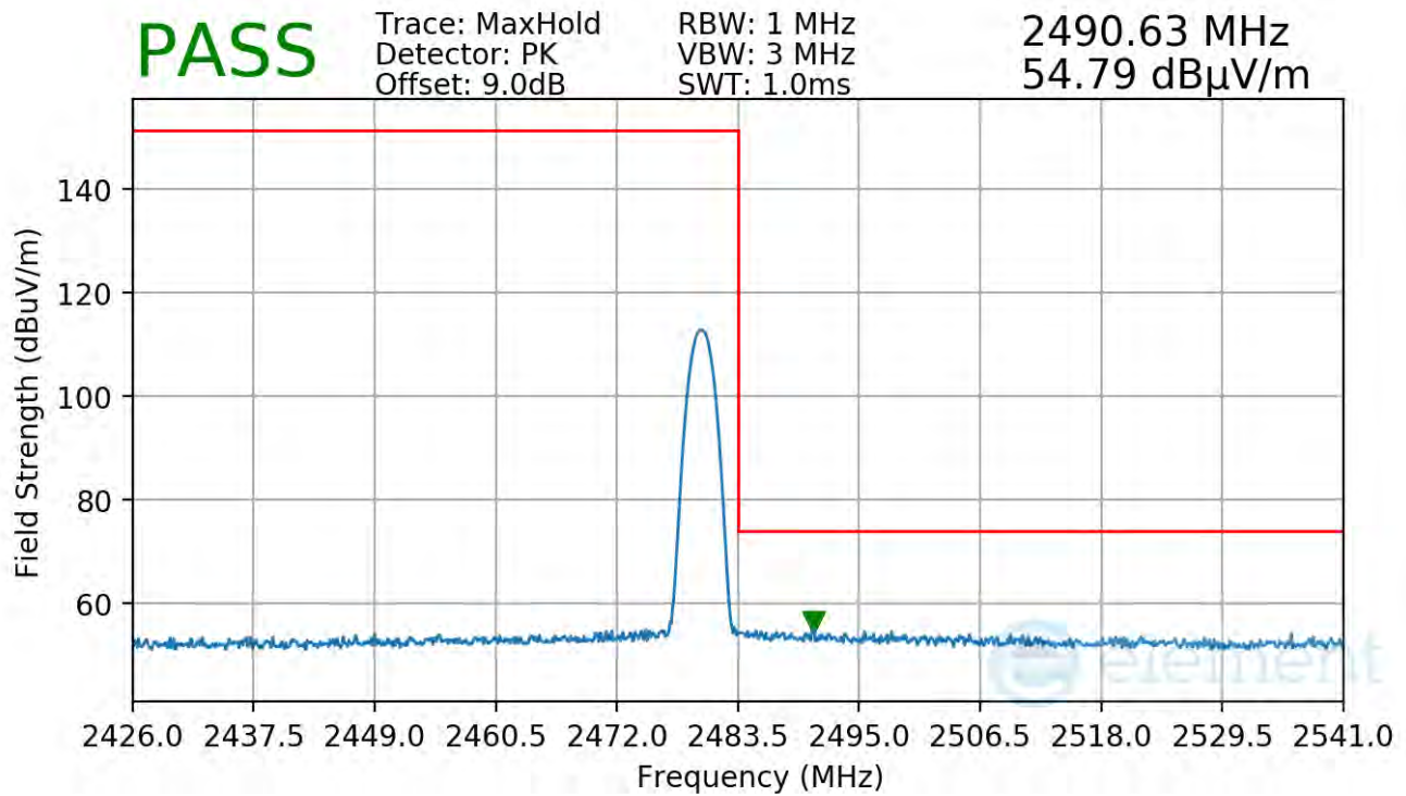
Plot 7-78. Radiated Restricted Upper Band Edge Measurement Antenna WF2b
