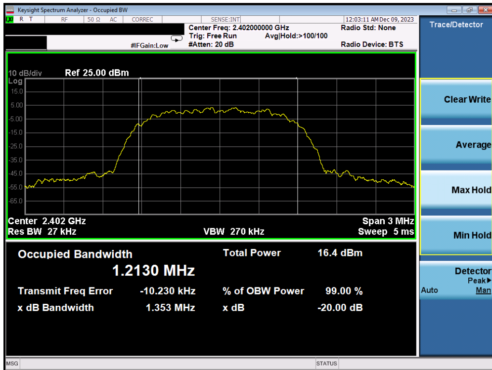
Plot 7-10. 20dB BW and 99% OBW Plot Antenna WF2b (Bluetooth, 8DPSK, ePA – Ch. 0)
