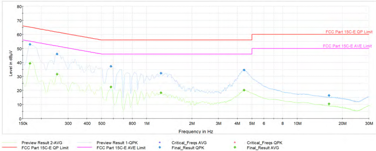
Plot 7-86. AC Line-Conducted Test Plot TxBF (N, GFSK ePA – Ch.0, with AC/DC Adapter)
