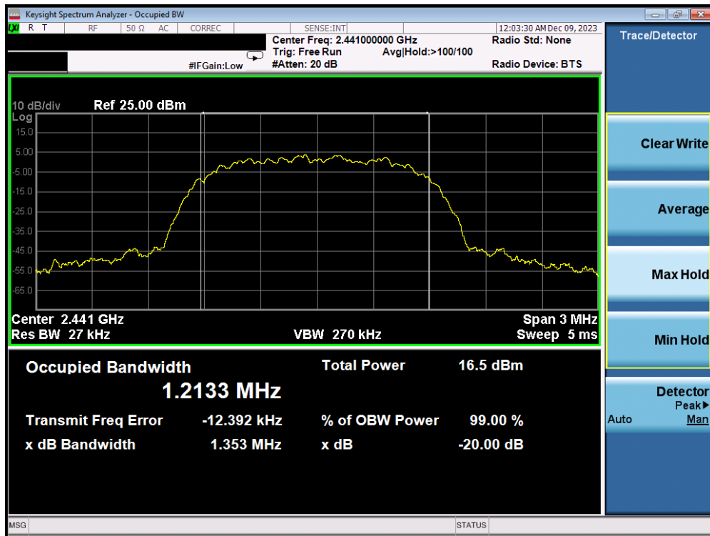
Plot 7-11. 20dB BW and 99% OBW Plot Antenna WF2b (Bluetooth, 8DPSK, ePA – Ch. 39)
