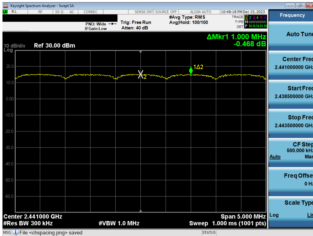
Plot 7-32. Channel Spacing Plot Antenna WF2b (Bluetooth, 8DPSK, ePA)
