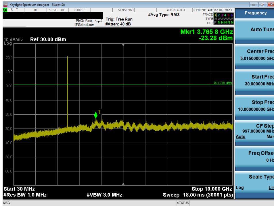
Plot 7-55. Conducted Spurious Plot Antenna WF2b (Bluetooth, GFSK, ePA – Ch. 78)
