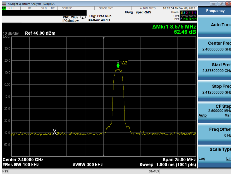
Plot 7-25. Band Edge Plot Antenna WF2b (Bluetooth with Hopping Disabled, 8DPSK, ePA – Ch. 0)
