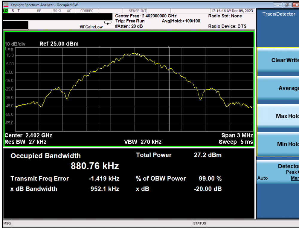
Plot 7-1. 20dB BW and 99% OBW Plot Antenna WF7b (Bluetooth, GFSK, ePA – Ch. 0)
