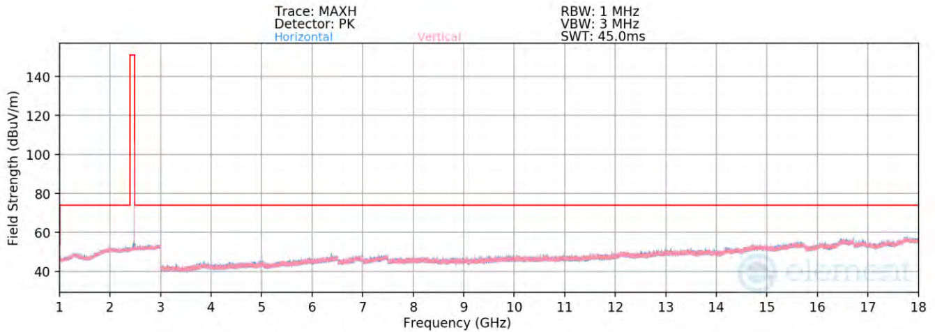
Plot 7-61. Radiated Spurious Emissions above 1GHz Antenna WF7b (BT GFSK ePA – Ch. 78)
