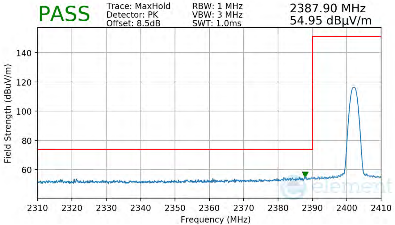
Plot 7-71. Radiated Restricted Lower Band Edge Measurement Antenna WF7b
