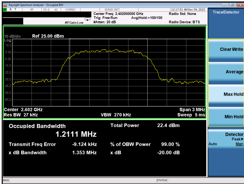
Plot 7-4. 20dB BW and 99% OBW Plot Antenna WF7b (Bluetooth, 8DPSK, ePA – Ch. 0)
