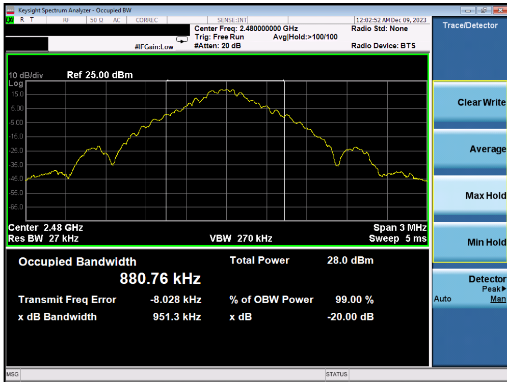
Plot 7-9. 20dB BW and 99% OBW Plot Antenna WF2b (Bluetooth, GFSK, ePA – Ch. 78)
