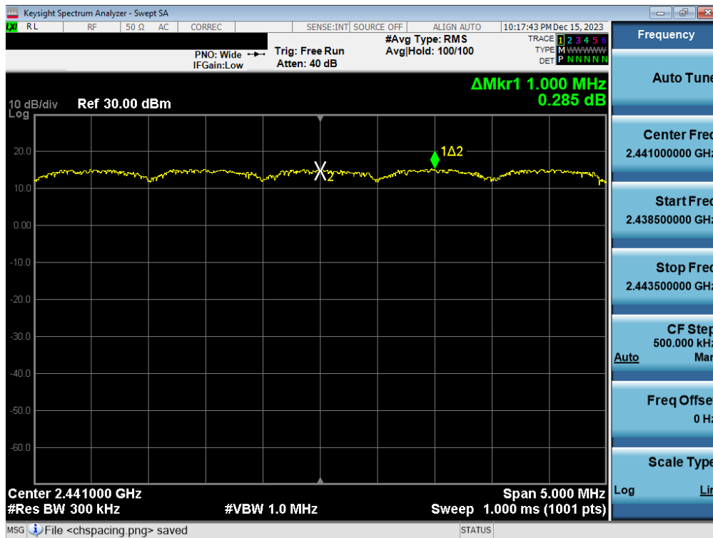
Plot 7-30. Channel Spacing Plot Antenna WF7b (Bluetooth, 8DPSK, ePA)
