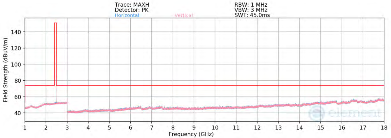
Plot 7-64. Radiated Spurious Emissions above 1GHz Antenna WF2b (BT GFSK ePA – Ch. 78)
