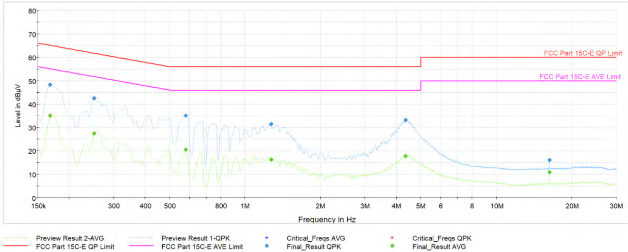
Plot 7-85. AC Line-Conducted Test Plot TxBF (L1, GFSK ePA – Ch.0, with AC/DC Adapter)
