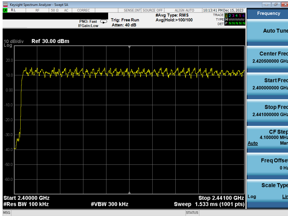
Plot 7-39. Low End Spectrum Channel Hopping Plot Antenna WF7b (Bluetooth, 8DPSK, ePA)
