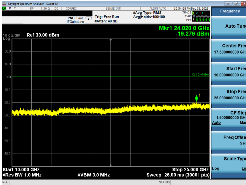
Plot 7-50. Conducted Spurious Plot Antenna WF7b (Bluetooth, GFSK, ePA – Ch. 78)
