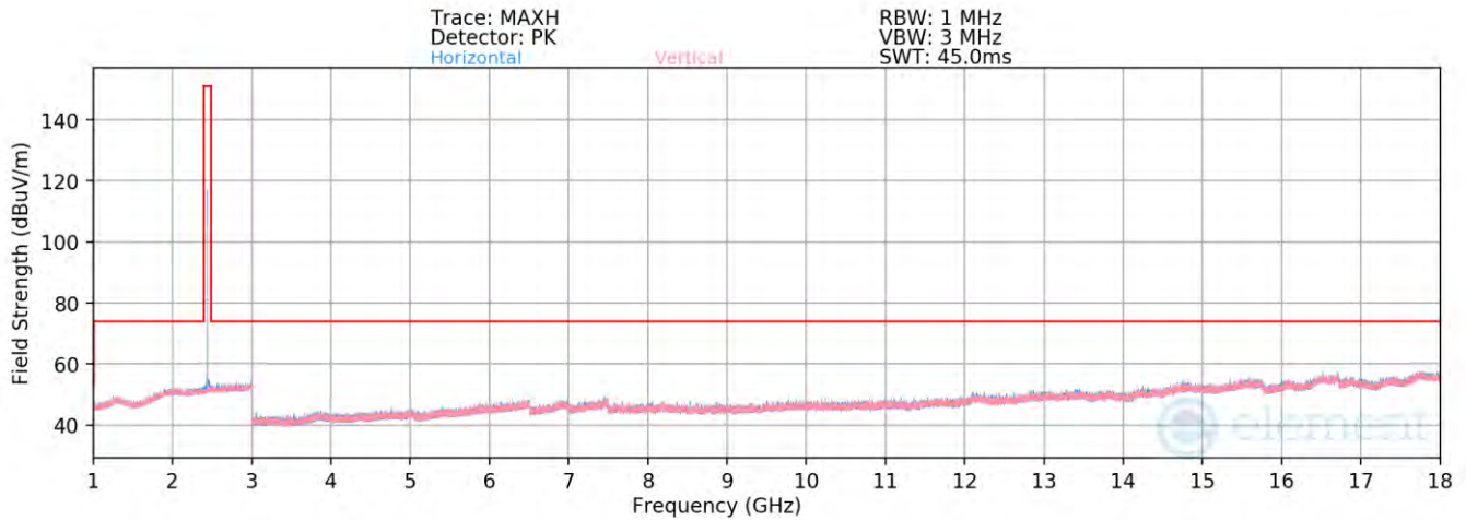
Plot 7-60. Radiated Spurious Emissions above 1GHz Antenna WF7b (BT GFSK ePA – Ch. 39)
