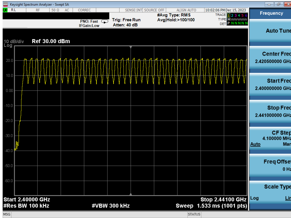
Plot 7-37. Low End Spectrum Channel Hopping Plot Antenna WF7b (Bluetooth, GFSK, ePA)
