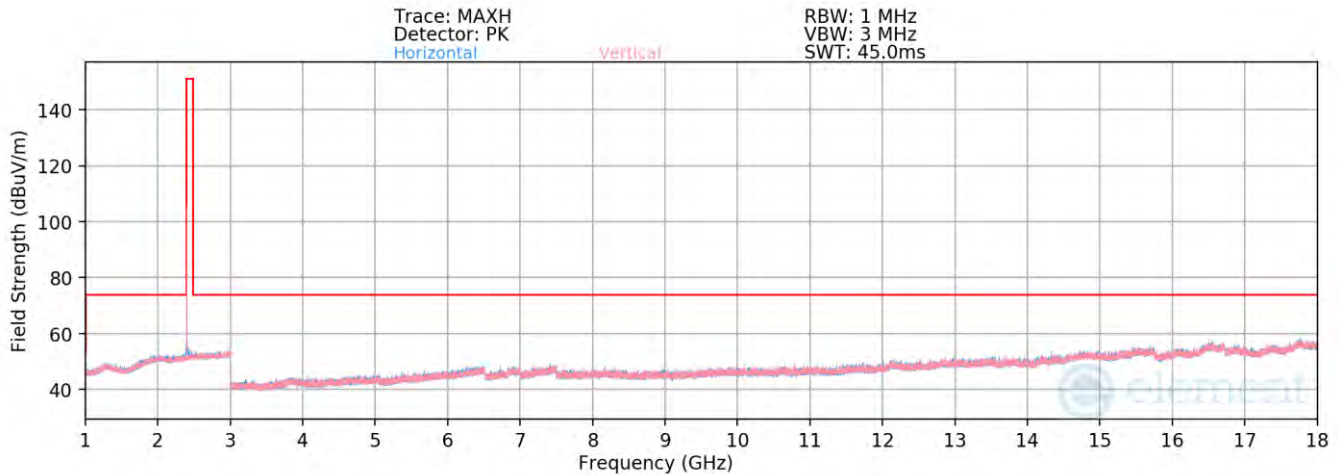
Plot 7-59. Radiated Spurious Emissions above 1GHz Antenna WF7b (BT GFSK ePA – Ch. 0)
