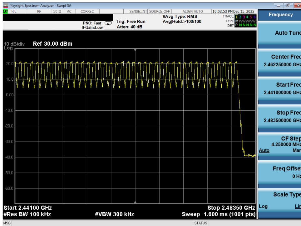
Plot 7-38. High End Spectrum Channel Hopping Plot Antenna WF7b (Bluetooth, GFSK, ePA)
