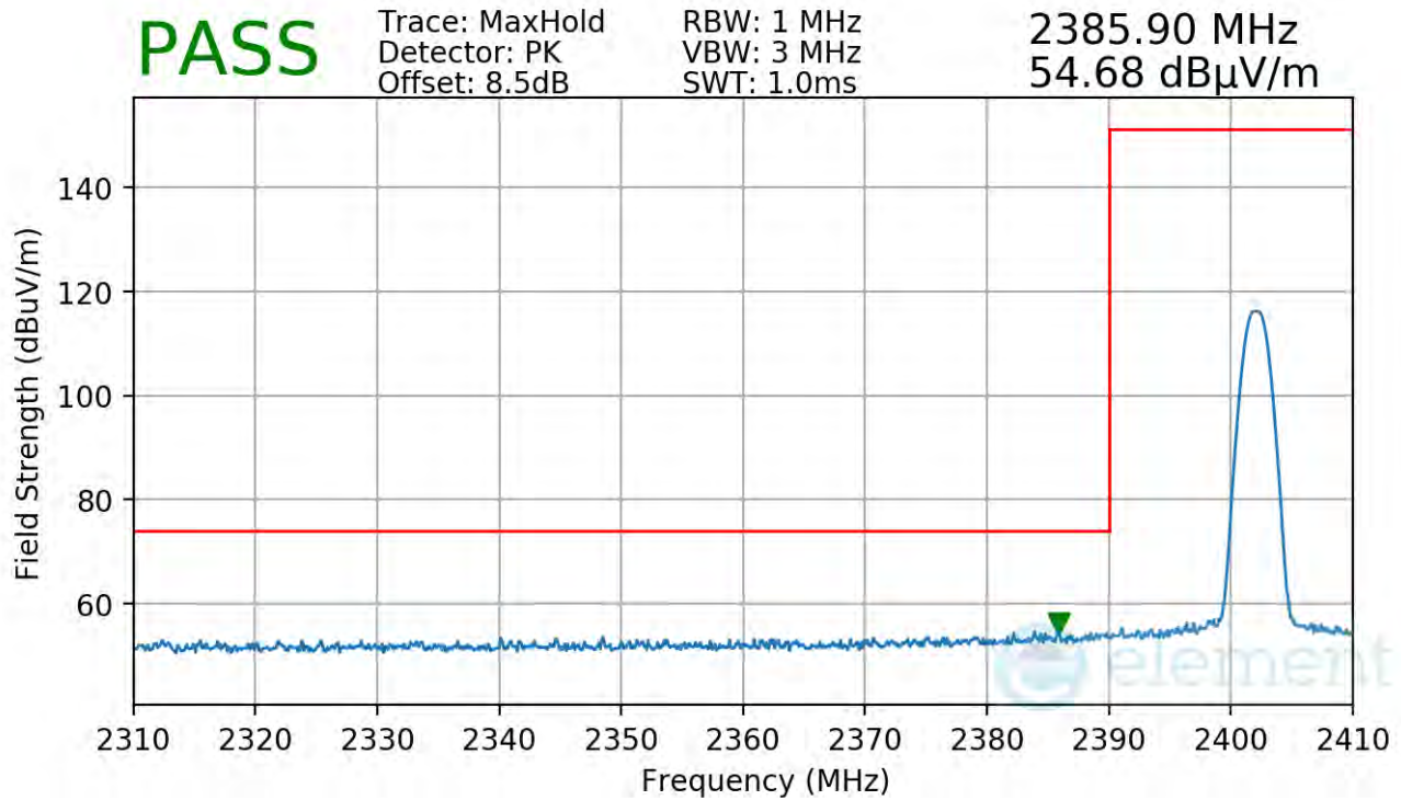
Plot 7-75. Radiated Restricted Lower Band Edge Measurement Antenna WF2b
