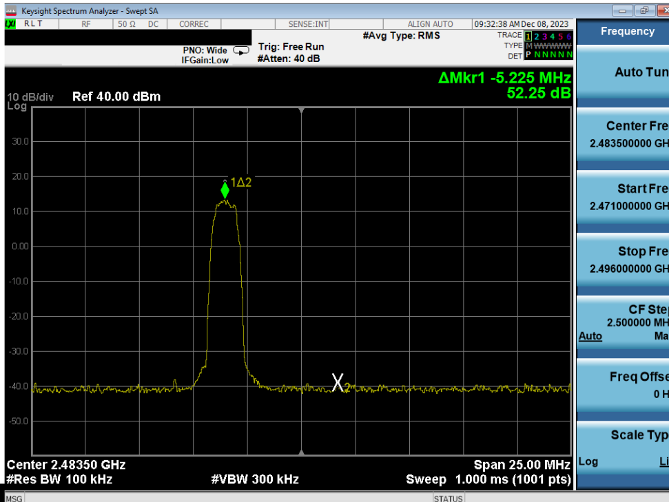
Plot 7-18. Band Edge Plot Antenna WF7b (Bluetooth with Hopping Disabled, 8DPSK, ePA – Ch. 78)
