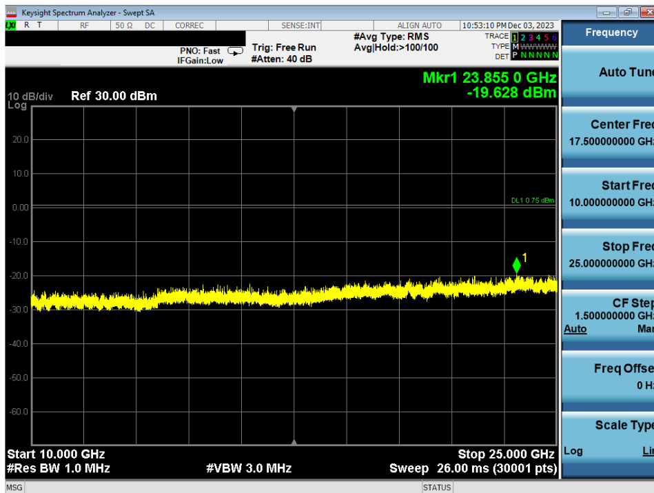
Plot 7-48. Conducted Spurious Plot Antenna WF7b (Bluetooth, GFSK, ePA Ch. 39)
