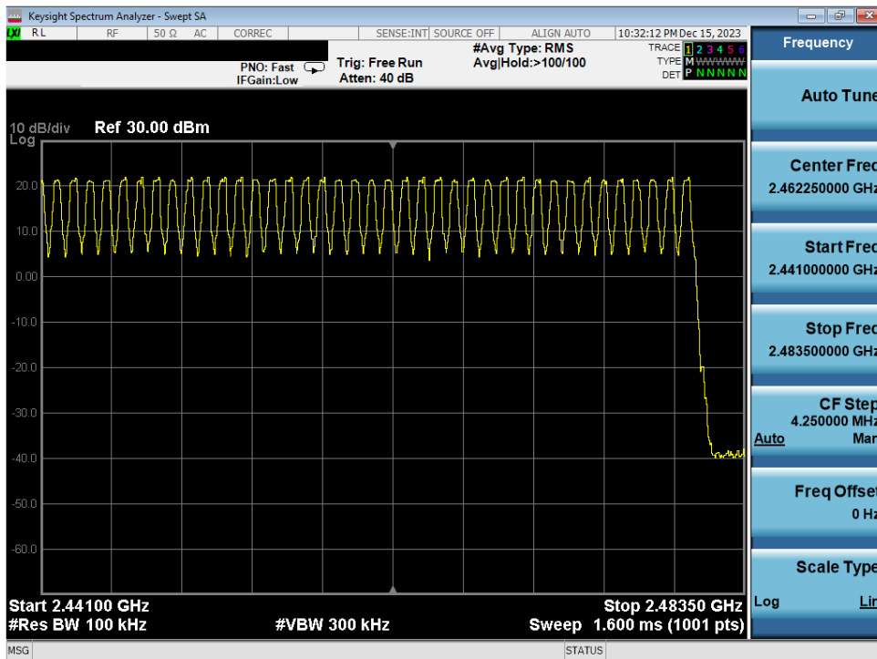
Plot 7-42. High End Spectrum Channel Hopping Plot Antenna WF2b (Bluetooth, GFSK, ePA)
