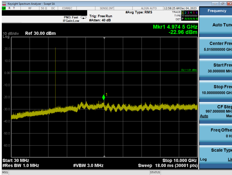
Plot 7-51. Conducted Spurious Plot Antenna WF2b (Bluetooth, GFSK, ePA – Ch. 0)
