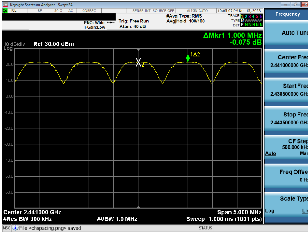
Plot 7-29. Channel Spacing Plot Antenna WF7b (Bluetooth, GFSK, ePA)
