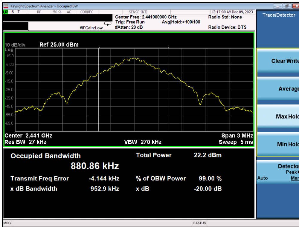
Plot 7-2. 20dB BW and 99% OBW Plot Antenna WF7b (Bluetooth, GFSK, ePA – Ch. 39)
