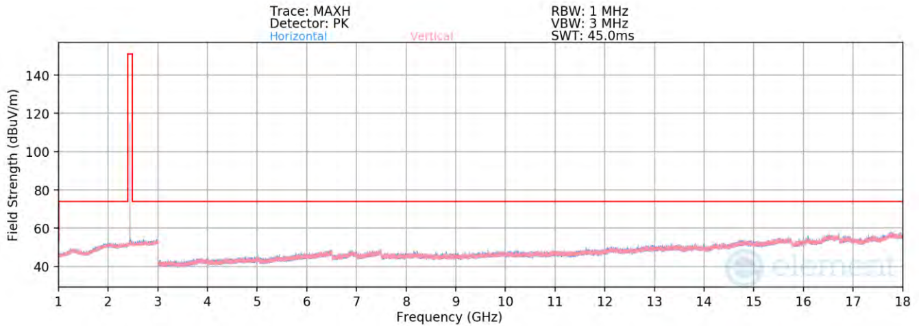
Plot 7-63. Radiated Spurious Emissions above 1GHz Antenna WF2b (BT GFSK ePA – Ch. 39)
