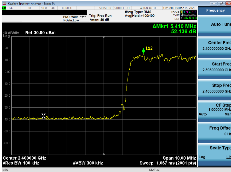
Plot 7-27. Band Edge Plot Antenna WF2b (Bluetooth with Hopping Enabled, 8DPSK, ePA)
