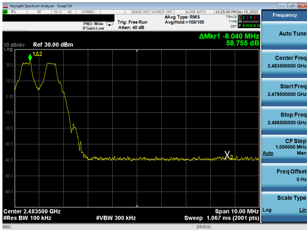
Plot 7-24. Band Edge Plot Antenna WF2b (Bluetooth with Hopping Enabled, GFSK, ePA)
