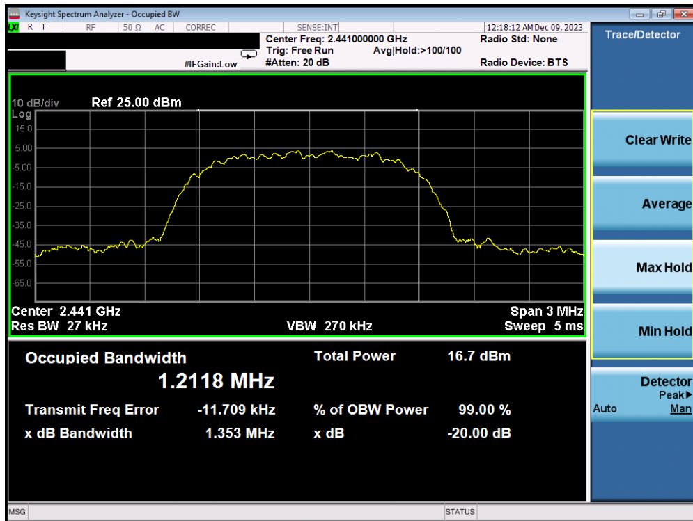
Plot 7-5. 20dB BW and 99% OBW Plot Antenna WF7b (Bluetooth, 8DPSK, ePA – Ch. 39)
