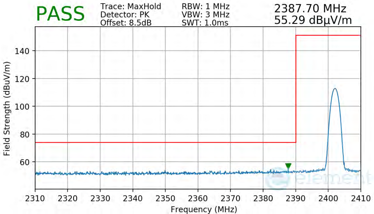
Plot 7-76. Radiated Restricted Lower Band Edge Measurement Antenna WF2b
