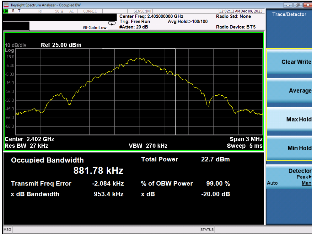
Plot 7-7. 20dB BW and 99% OBW Plot Antenna WF2b (Bluetooth, GFSK, ePA – Ch. 0)
