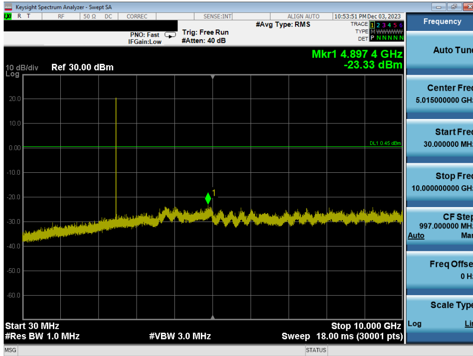
Plot 7-49. Conducted Spurious Plot Antenna WF7b (Bluetooth, GFSK, ePA – Ch. 78)
