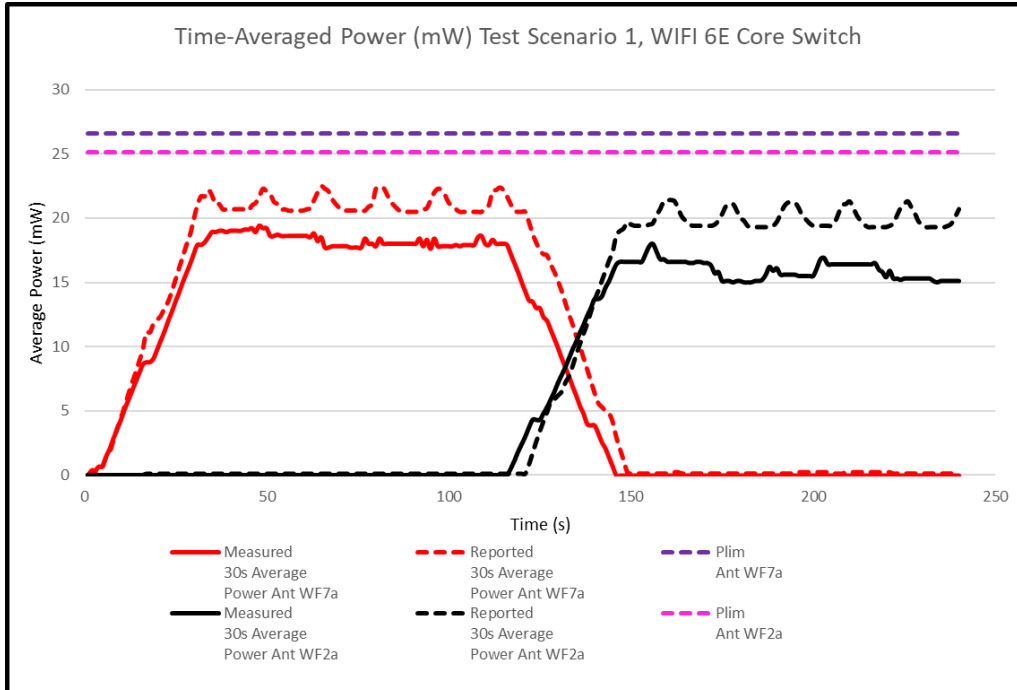
Figure H-6 30s Average Power vs. Time, 6 GHz
