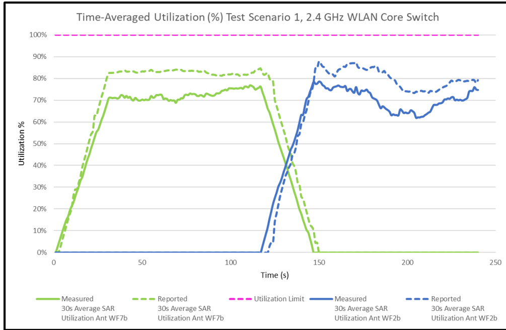
Figure H-1 30s Average SAR Utilization vs. Time, 2.4 GHz
