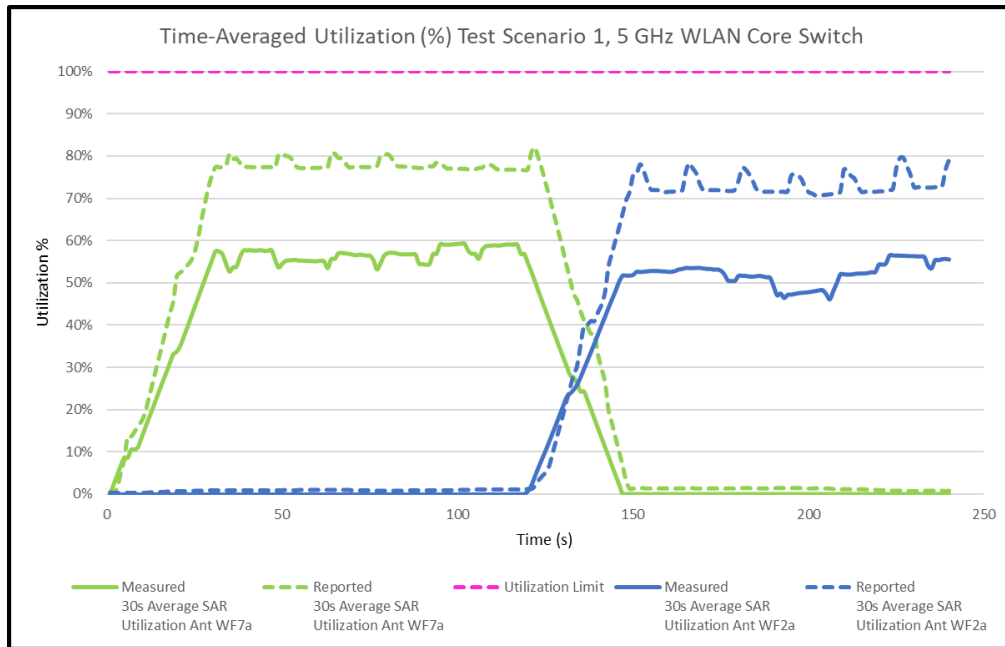
Figure H-3 30s Average SAR Utilization vs. Time, 5 GHz
