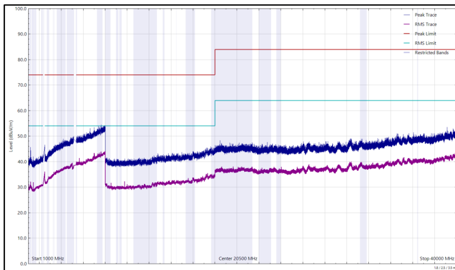
Figure 33 - 2437 MHz (CH6), HT20, Core 1 and 5204 MHz, HDR8, ePA, Core 0, 1 GHz to 40 GHz, Vertical
