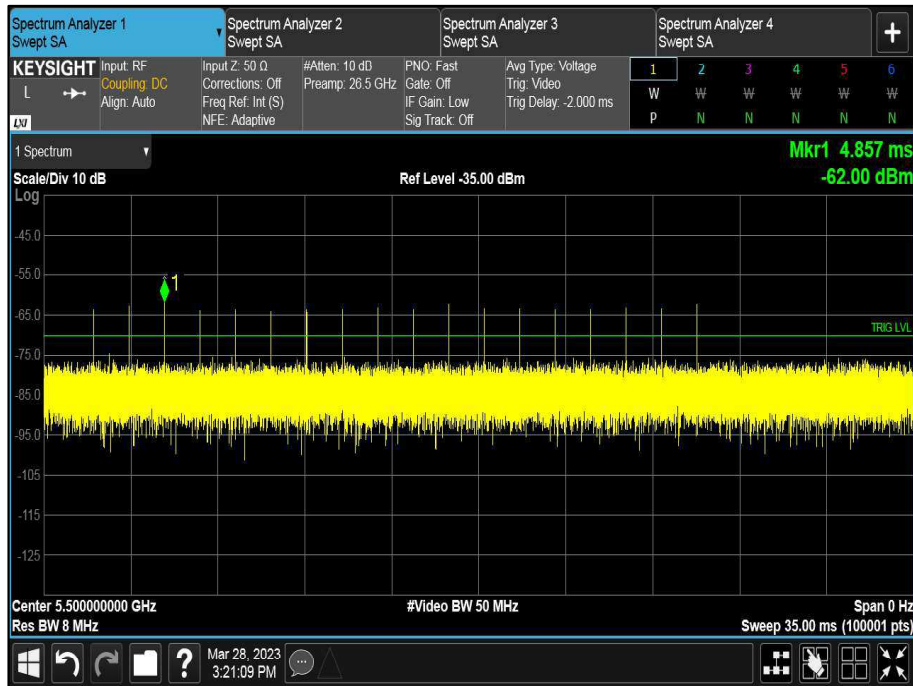
Figure 594 - Verification of Radar Type 0
