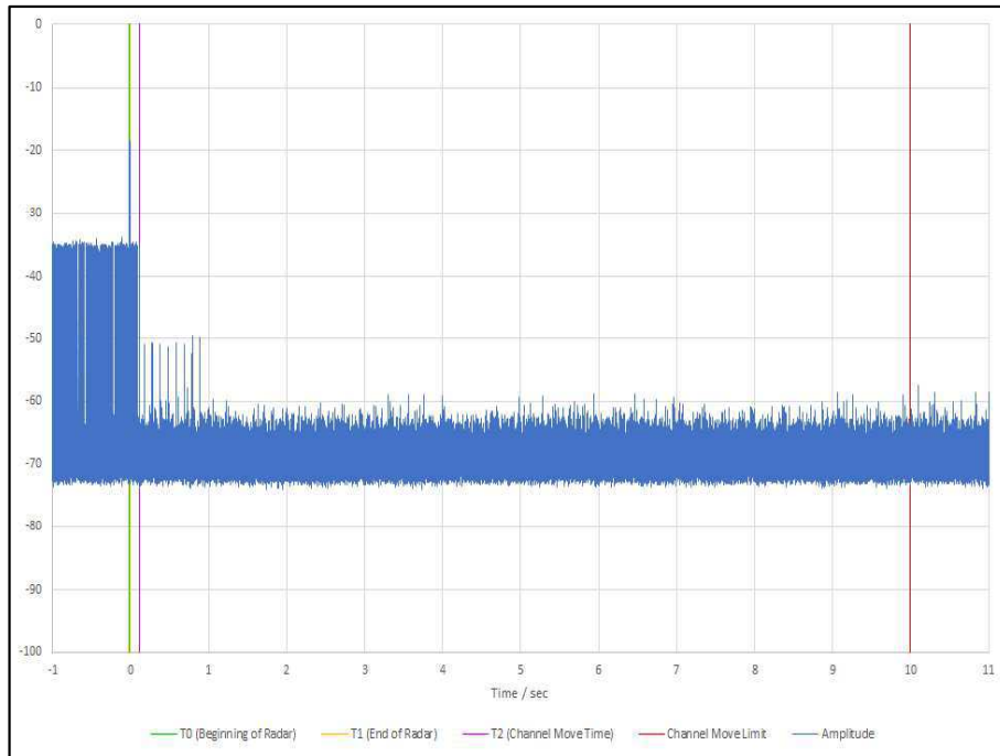
Figure 597 - First 12 s of Channel Shutdown Period
