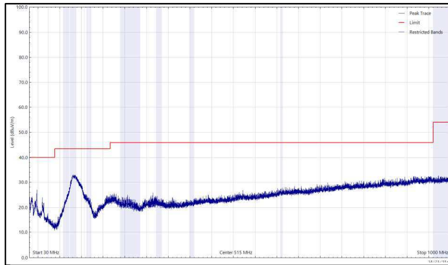
Figure 591 - U-NII-3 - 5825 MHz (CH165), VHT20, CDD, Core 0 + Core 1, 30 MHz to 1 GHz, Vertical (Peak)
