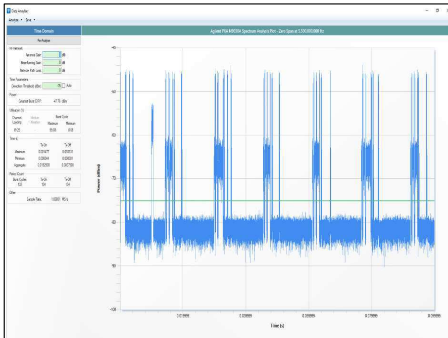
Figure 595 - Channel Loading
