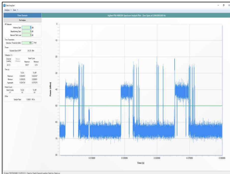
Figure 601 - Channel Loading
