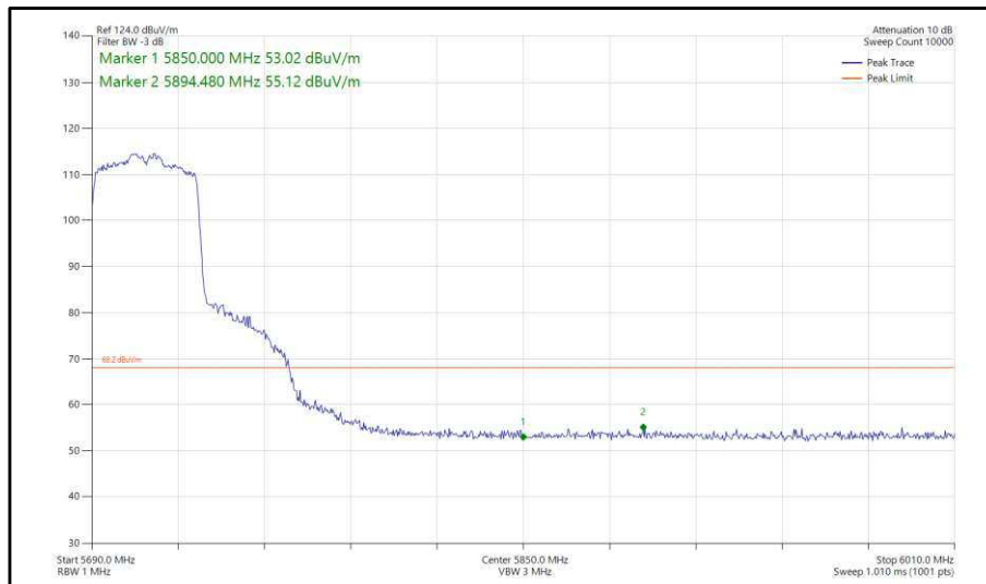
Figure 372 - 802.11ax, HE40, SU, SISO, Core 0 - 5710 MHz, Band Edge Frequency 5850 MHz
