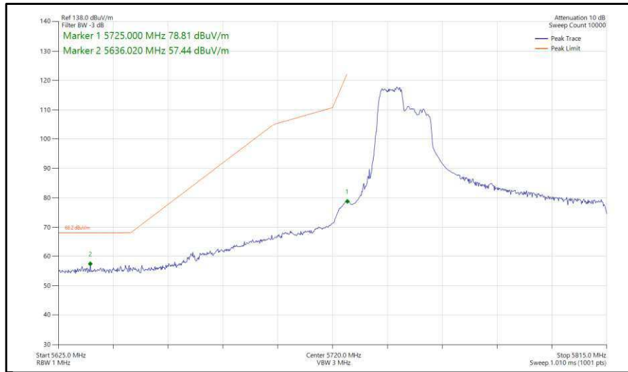
Figure 439 - 802.11ax, HE80, RU 106-53, SISO, Core 0 - 5775 MHz, Band Edge Frequency 5725 MHz
