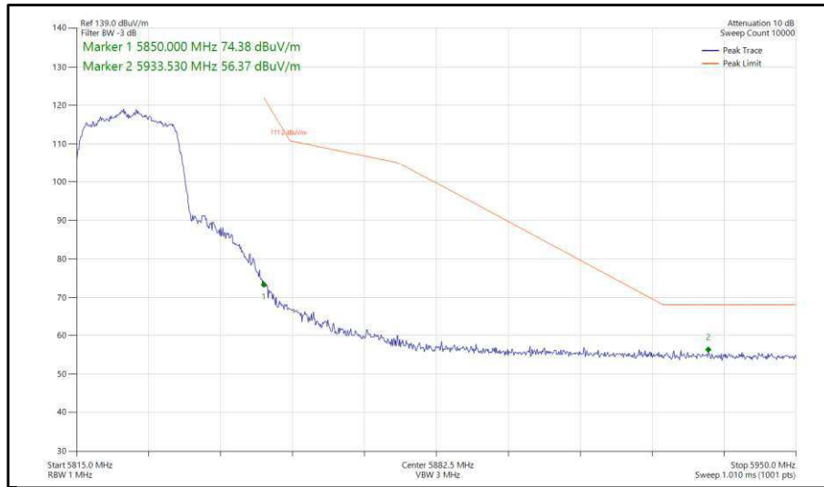
Figure 346 - 802.11n, HT20, SDM, Core 0-1 - 5825 MHz, Band Edge Frequency 5850 MHz
