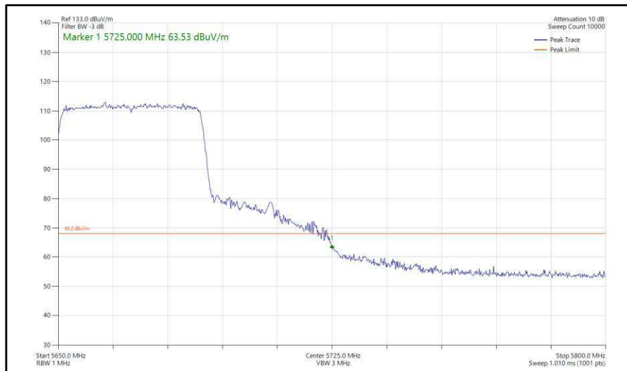
Figure 383 - 802.11ax, HE40, SU, SISO, Core 1 - 5670 MHz, Band Edge Frequency 5725 MHz
