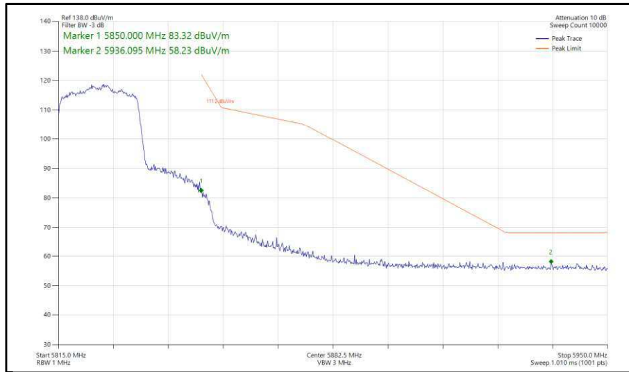
Figure 360 - 802.11ax, HE20, SU, TxBF, Core 0-1 - 5825 MHz, Band Edge Frequency 5850 MHz
