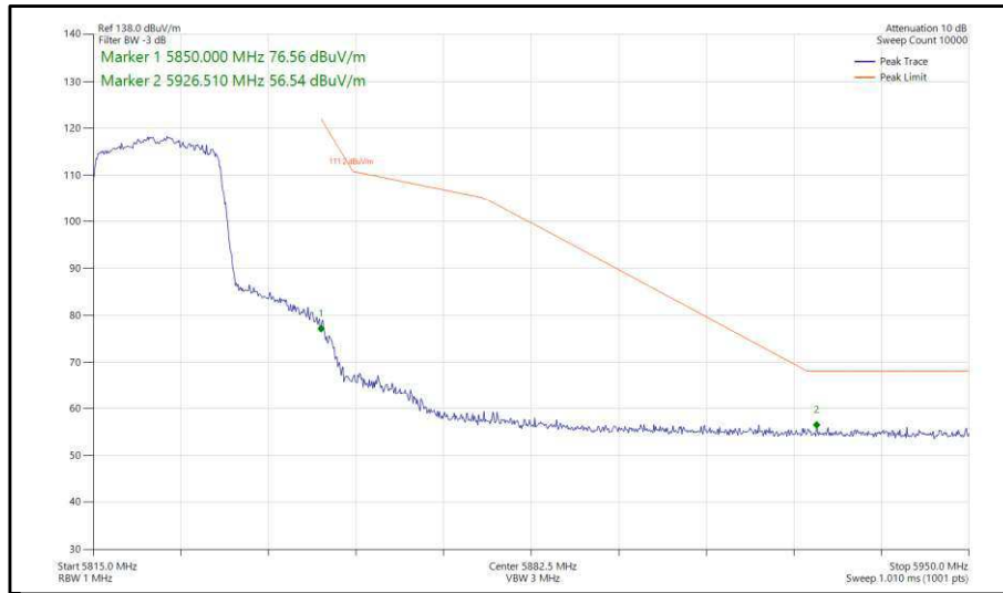
Figure 317 - 802.11ax, HE20, SU, SISO, Core 1 - 5825 MHz, Band Edge Frequency 5850 MHz
