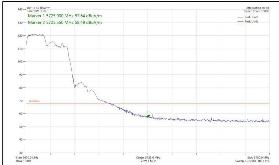
Figure 342 - 802.11ax, HE20, RU 106-53, SDM, Core 0-1 - 5680 MHz, Band Edge Frequency 5725 MHz
