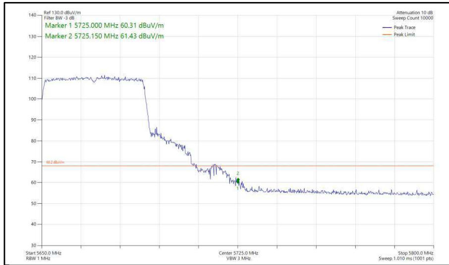
Figure 429 - 802.11ax, HE40, SU, TxBF, Core 0-1 - 5670 MHz, Band Edge Frequency 5725 MHz
