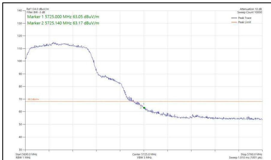
Figure 325 - 802.11n, HT20, CDD, Core 0-1 - 5700 MHz, Band Edge Frequency 5725 MHz
