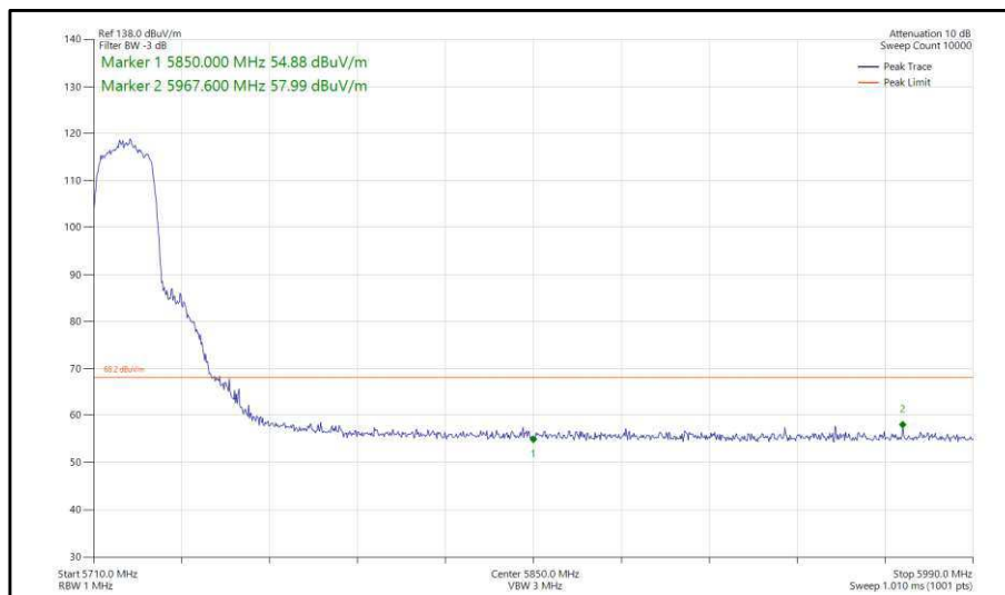
Figure 357 - 802.11ac, VHT20, TxBF, Core 0-1 - 5720 MHz, Band Edge Frequency 5850 MHz
