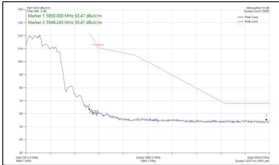
Figure 334 - 802.11ax, HE20, RU 106-53, CDD, Core 0-1 - 5825 MHz, Band Edge Frequency 5850 MHz
