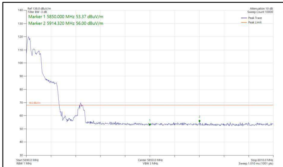
Figure 404 - 802.11ax, HE40, RU 52-37, CDD, Core 0-1 - 5710 MHz, Band Edge Frequency 5850 MHz
