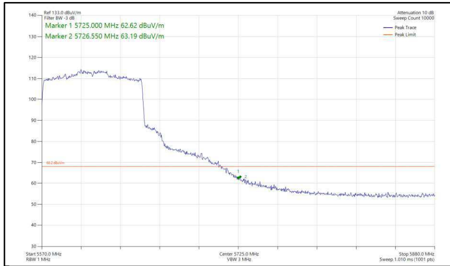
Figure 456 - 802.11ax, HE80, SU, SISO, Core 1 - 5610 MHz, Band Edge Frequency 5725 MHz
