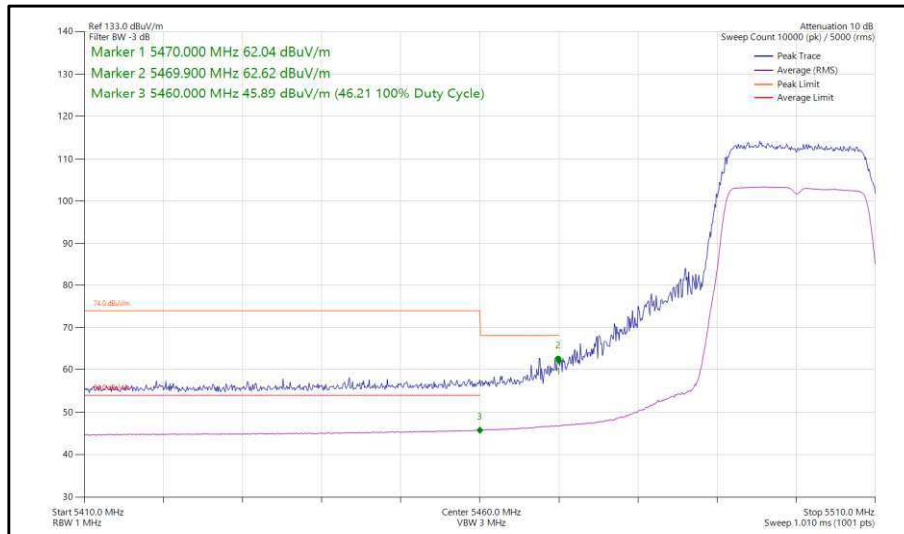
Figure 351 - 802.11ac, VHT20, TxBF, Core 0-1 - 5500 MHz, Band Edge Frequency 5470 MHz
