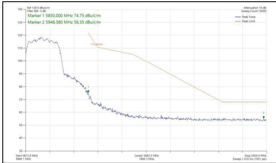
Figure 330 - 802.11n, HT20, CDD, Core 0-1 - 5825 MHz, Band Edge Frequency 5850 MHz
