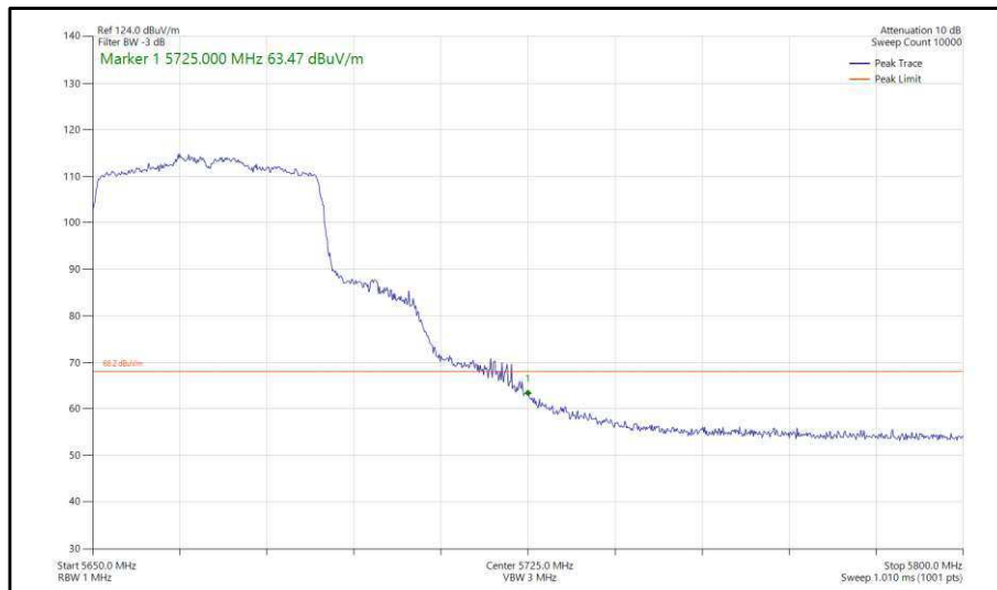
Figure 416 - 802.11ax, HE40, SU, SDM, Core 0-1 - 5670 MHz, Band Edge Frequency 5725 MHz
