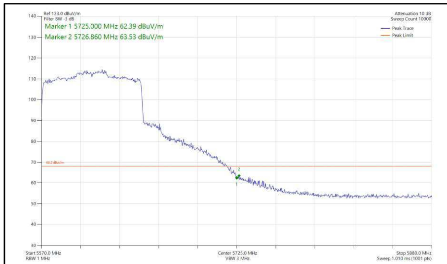
Figure 441 - 802.11ax, HE80, SU, SISO, Core 0 - 5610 MHz, Band Edge Frequency 5725 MHz
