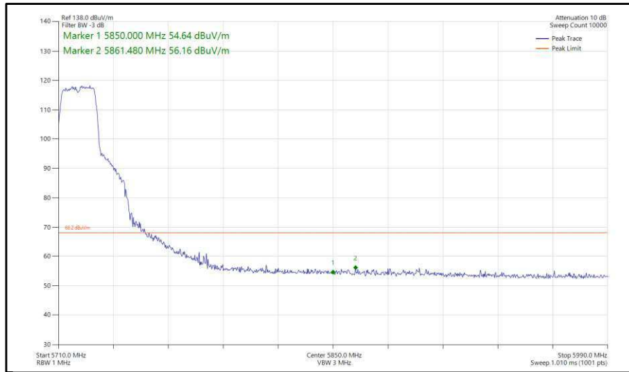
Figure 313 - 802.11n, HT20, SISO, Core 1 - 5720 MHz, Band Edge Frequency 5850 MHz
