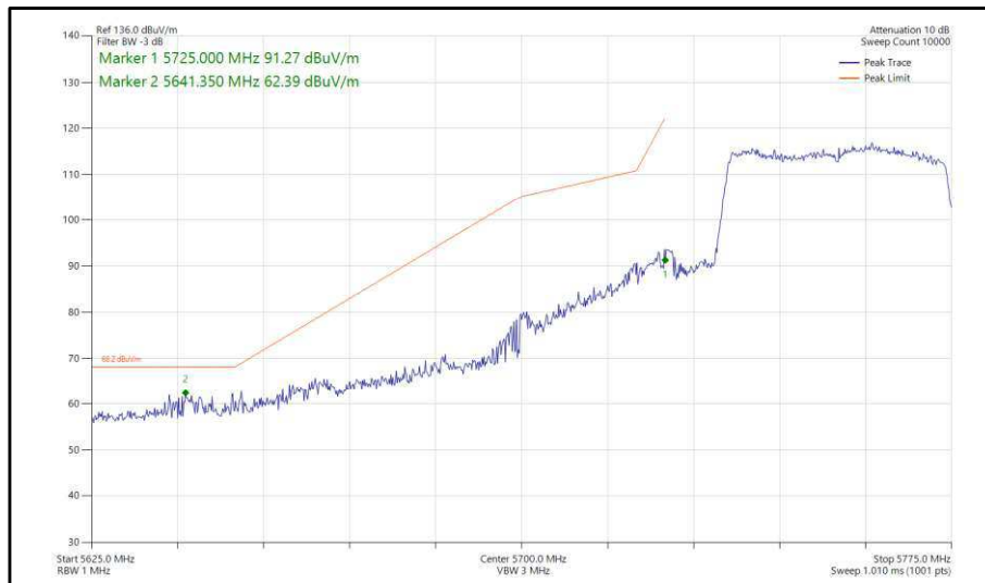
Figure 427 - 802.11ax, HE40, SU, TxBF, Core 0-1 - 5755 MHz, Band Edge Frequency 5725 MHz
