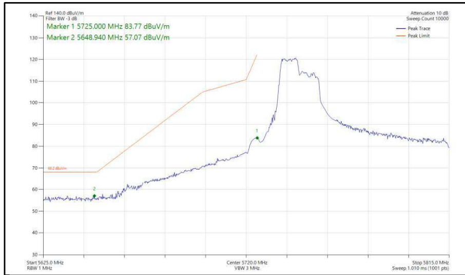
Figure 454 - 802.11ax, HE80, RU 106-53, SISO, Core 1 - 5775 MHz, Band Edge Frequency 5725 MHz
