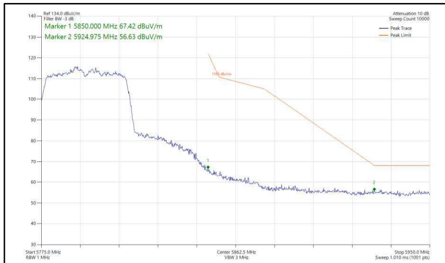
Figure 402 - 802.11n, HT40, CDD, Core 0-1 - 5795 MHz, Band Edge Frequency 5850 MHz
