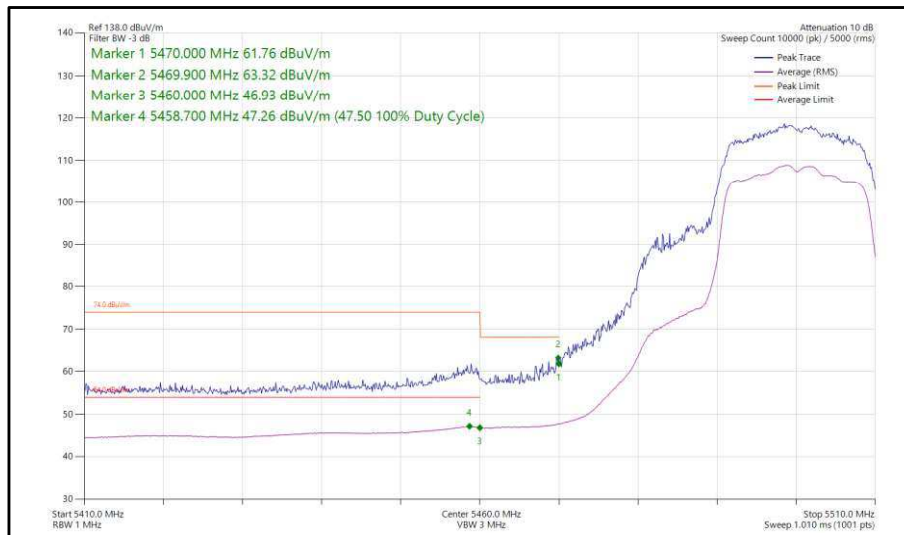
Figure 319 - 802.11n, HT20, CDD, Core 0-1 - 5500 MHz, Band Edge Frequency 5470 MHz
