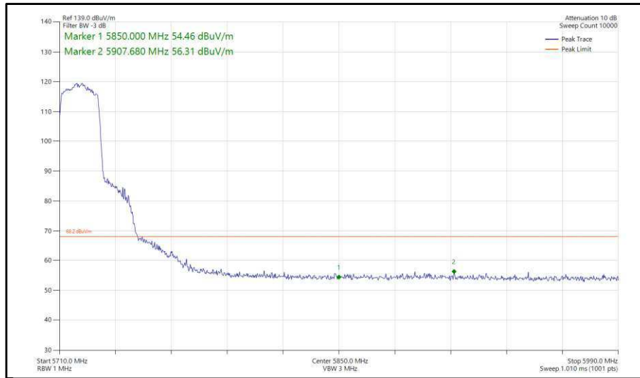
Figure 315 - 802.11ax, HE20, SU, SISO, Core 1 - 5720 MHz, Band Edge Frequency 5850 MHz
