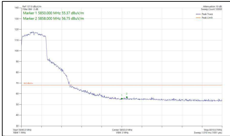
Figure 387 - 802.11ax, HE40, SU, SISO, Core 1 - 5710 MHz, Band Edge Frequency 5850 MHz
