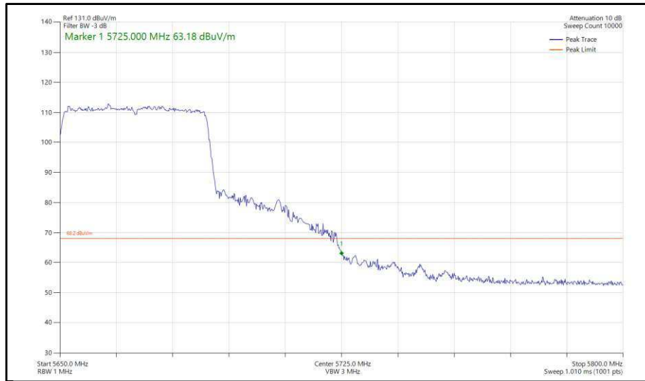
Figure 368 - 802.11ax, HE40, SU, SISO, Core 0 - 5670 MHz, Band Edge Frequency 5725 MHz
