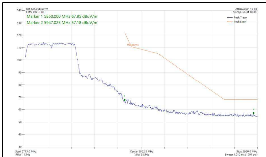
Figure 419 - 802.11n, HT40, SDM, Core 0-1 - 5795 MHz, Band Edge Frequency 5850 MHz
