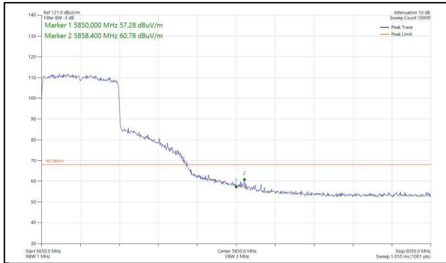
Figure 445 - 802.11ax, HE80, SU, SISO, Core 0 - 5690 MHz, Band Edge Frequency 5850 MHz
