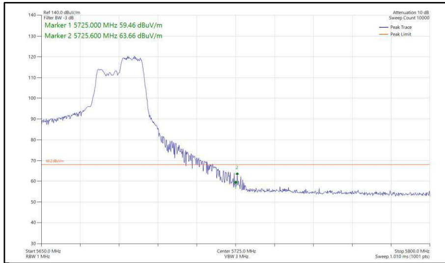
Figure 400 - 802.11ax, HE40, RU 106-56, CDD, Core 0-1 - 5670 MHz, Band Edge Frequency 5725 MHz
