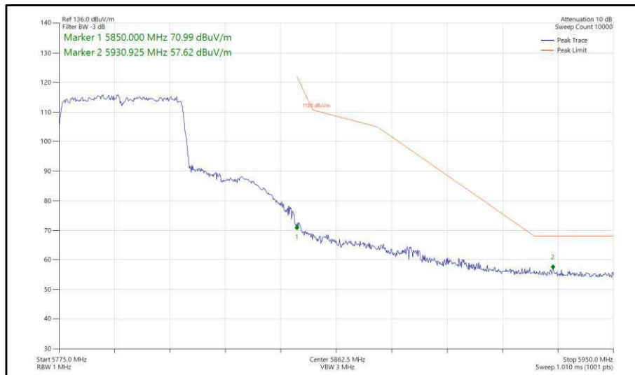
Figure 422 - 802.11ax, HE40, SU, SDM, Core 0-1 - 5795 MHz, Band Edge Frequency 5850 MHz
