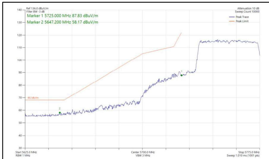
Figure 396 - 802.11ax, HE40, SU, CDD, Core 0-1 - 5755 MHz, Band Edge Frequency 5725 MHz
