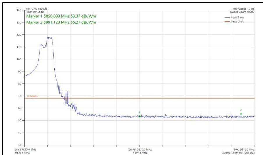
Figure 373 - 802.11ax, HE40, RU 106-56, SISO, Core 0 - 5710 MHz, Band Edge Frequency 5850 MHz
