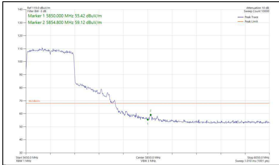
Figure 443 - 802.11ac, VHT80, SISO, Core 0 - 5690 MHz, Band Edge Frequency 5850 MHz
