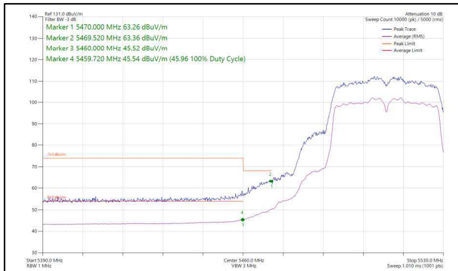
Figure 391 - 802.11n, HT40, CDD, Core 0-1 - 5510 MHz, Band Edge Frequency 5470 MHz
