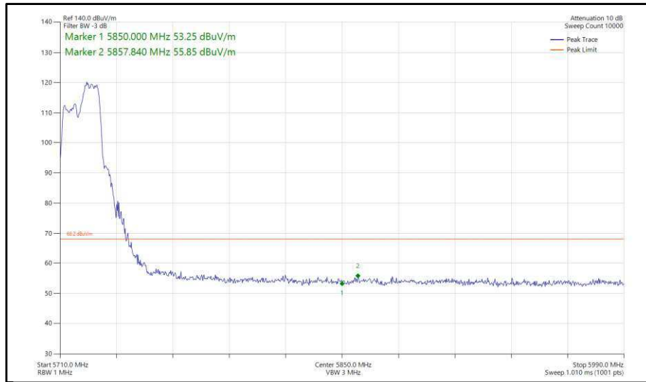
Figure 332 - 802.11ax, HE20, RU 106-54, CDD, Core 0-1 - 5720 MHz, Band Edge Frequency 5850 MHz
