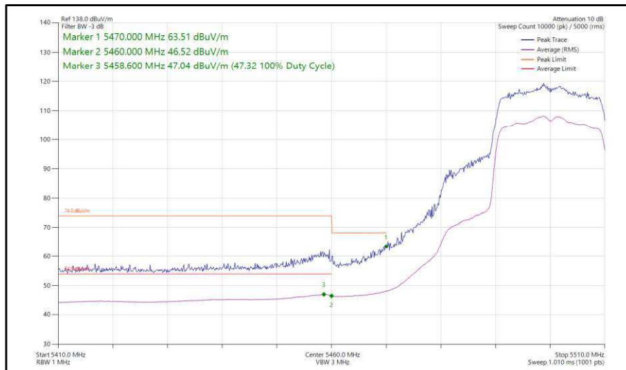
Figure 320 - 802.11ax, HE20, SU, CDD, Core 0-1 - 5500 MHz, Band Edge Frequency 5470 MHz
