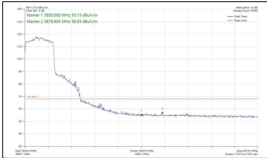
Figure 420 - 802.11ax, HE40, SU, SDM, Core 0-1 - 5710 MHz, Band Edge Frequency 5850 MHz
