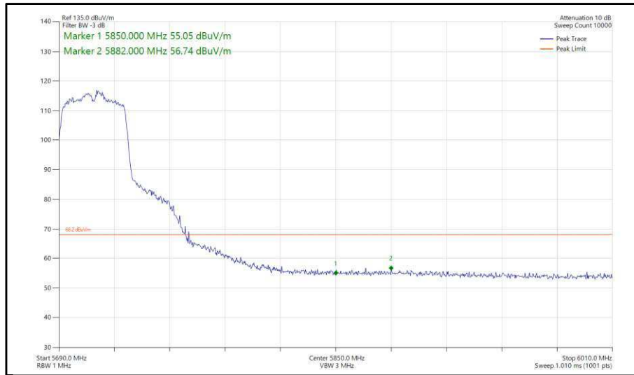
Figure 385 - 802.11n, HT40, SISO, Core 1 - 5710 MHz, Band Edge Frequency 5850 MHz
