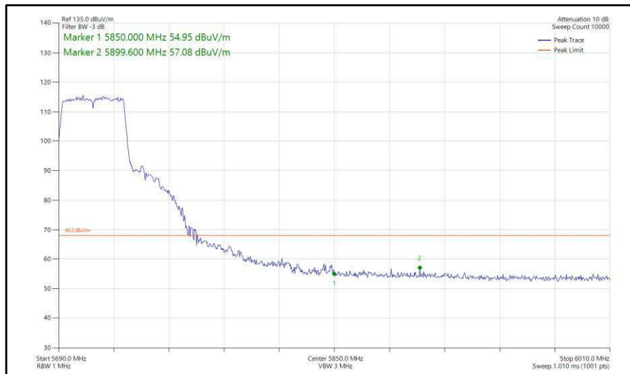
Figure 418 - 802.11n, HT40, SDM, Core 0-1 - 5710 MHz, Band Edge Frequency 5850 MHz
