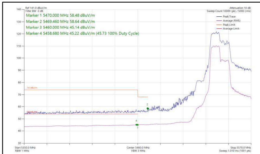
Figure 394 - 802.11ax, HE40, RU 106-53, CDD, Core 0-1 - 5550 MHz, Band Edge Frequency 5470 MHz
