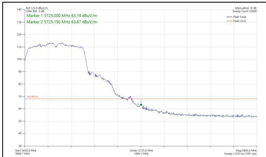
Figure 414 - 802.11n, HT40, SDM, Core 0-1 - 5670 MHz, Band Edge Frequency 5725 MHz
