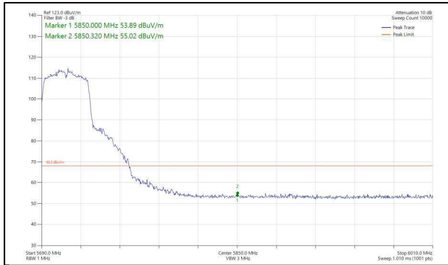
Figure 370 - 802.11n, HT40, SISO, Core 0 - 5710 MHz, Band Edge Frequency 5850 MHz
