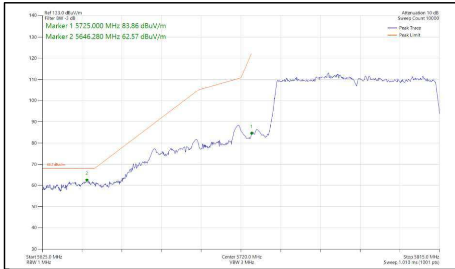
Figure 452 - 802.11ac, VHT80, SISO, Core 1 - 5775 MHz, Band Edge Frequency 5725 MHz
