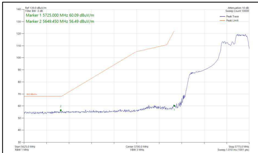
Figure 381 - 802.11ax, HE40, RU 106-56, SISO, Core 1 - 5755 MHz, Band Edge Frequency 5725 MHz
