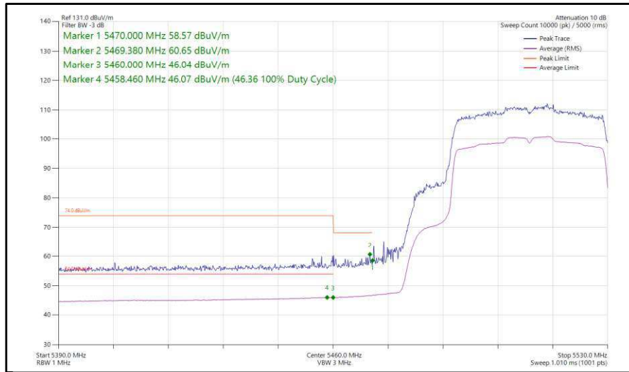
Figure 425 - 802.11ax, HE40, SU, TxBF, Core 0-1 - 5510 MHz, Band Edge Frequency 5470 MHz
