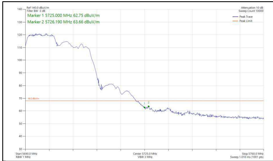
Figure 328 - 802.11ax, HE20, RU 106-53, CDD, Core 0-1 - 5700 MHz, Band Edge Frequency 5725 MHz
