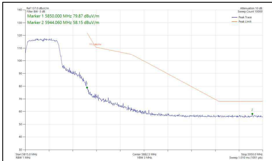
Figure 358 - 802.11ac, VHT20, TxBF, Core 0-1 - 5825 MHz, Band Edge Frequency 5850 MHz
