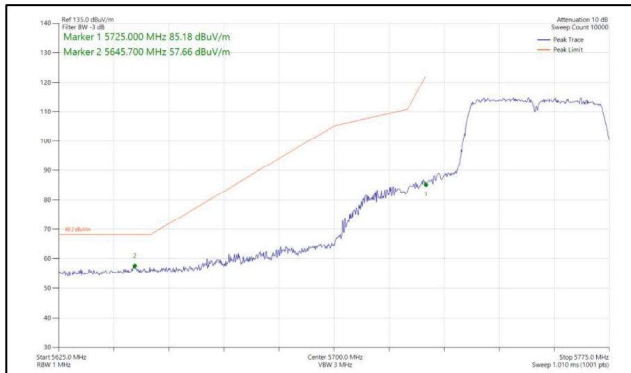
Figure 379 - 802.11n, HT40, SISO, Core 1 - 5755 MHz, Band Edge Frequency 5725 MHz
