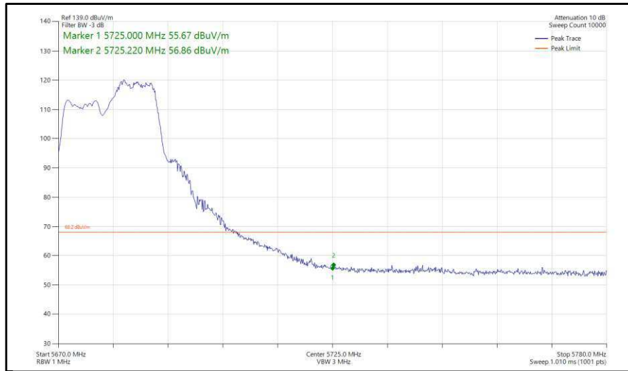
Figure 326 - 802.11ax, HE20, RU 106-54, CDD, Core 0-1 - 5680 MHz, Band Edge Frequency 5725 MHz
