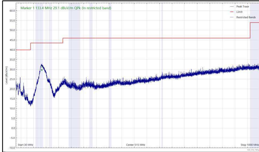
Figure 133 - 2437 MHz (CH6), HE20, RU26-0, CDD, Core 0 + Core 1, 30 MHz to 1 GHz, Horizontal (Peak)
