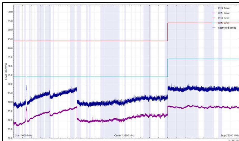
Figure 112 - 2437 MHz (CH6), 802.11g, Core 0, 1 GHz to 26 GHz, Vertical
