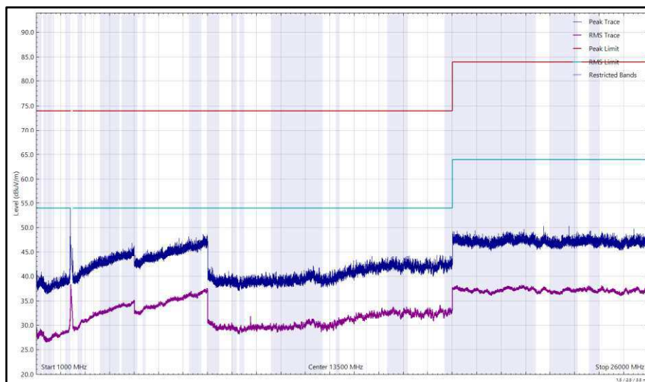
Figure 104 - 2437 MHz (CH6), 802.11b, Core 1, 1 GHz to 26 GHz, Vertical
