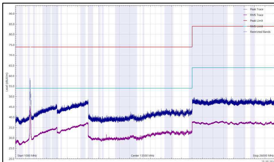
Figure 128 - 2437 MHz (CH6), HT20, CDD, Core 0 + Core 1, 1 GHz to 26 GHz, Vertical
