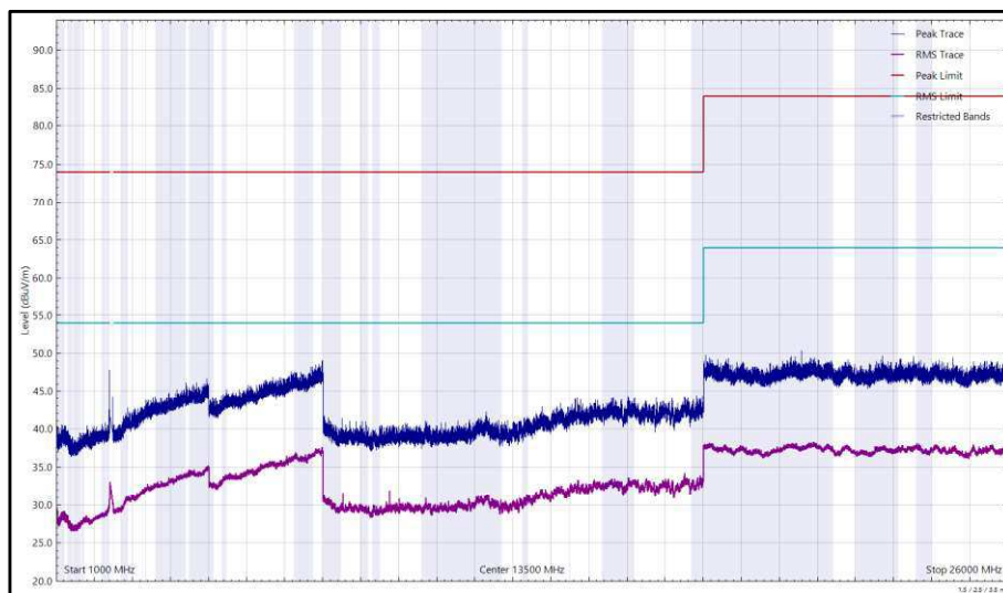
Figure 96 - 2437 MHz (CH6), 802.11b, Core 0, 1 GHz to 26 GHz, Vertical
