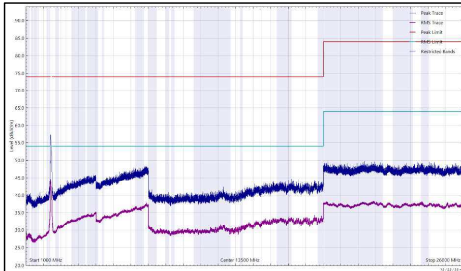
Figure 118 - 2437 MHz (CH6), 802.11g, Core 1, 1 GHz to 26 GHz, Horizontal
