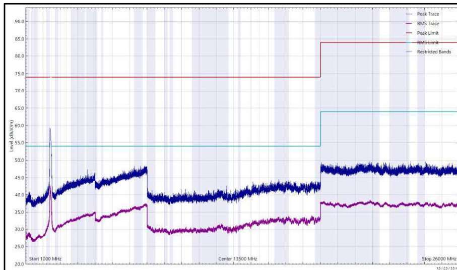
Figure 134 - 2437 MHz (CH6), HE20, RU26-0, CDD, Core 0 + Core 1, 1 GHz to 26 GHz, Horizontal
