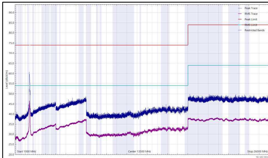
Figure 126 - 2437 MHz (CH6), HT20, CDD, Core 0 + Core 1, 1 GHz to 26 GHz, Horizontal
