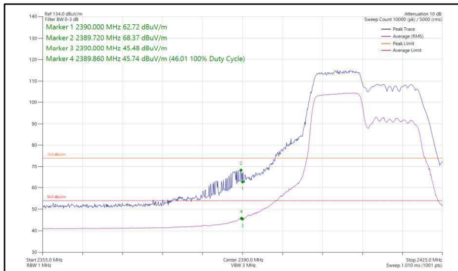
Figure 25 - 802.11ax, HE20, RU 106-53, SISO, Core 1 - 2412 MHz, Band Edge Frequency 2390 MHz
