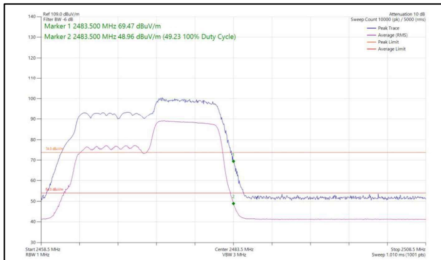
Figure 40 - 802.11ax, HE20, RU 106-54, SISO, Core 1 - 2472 MHz, Band Edge Frequency 2483.5 MHz
