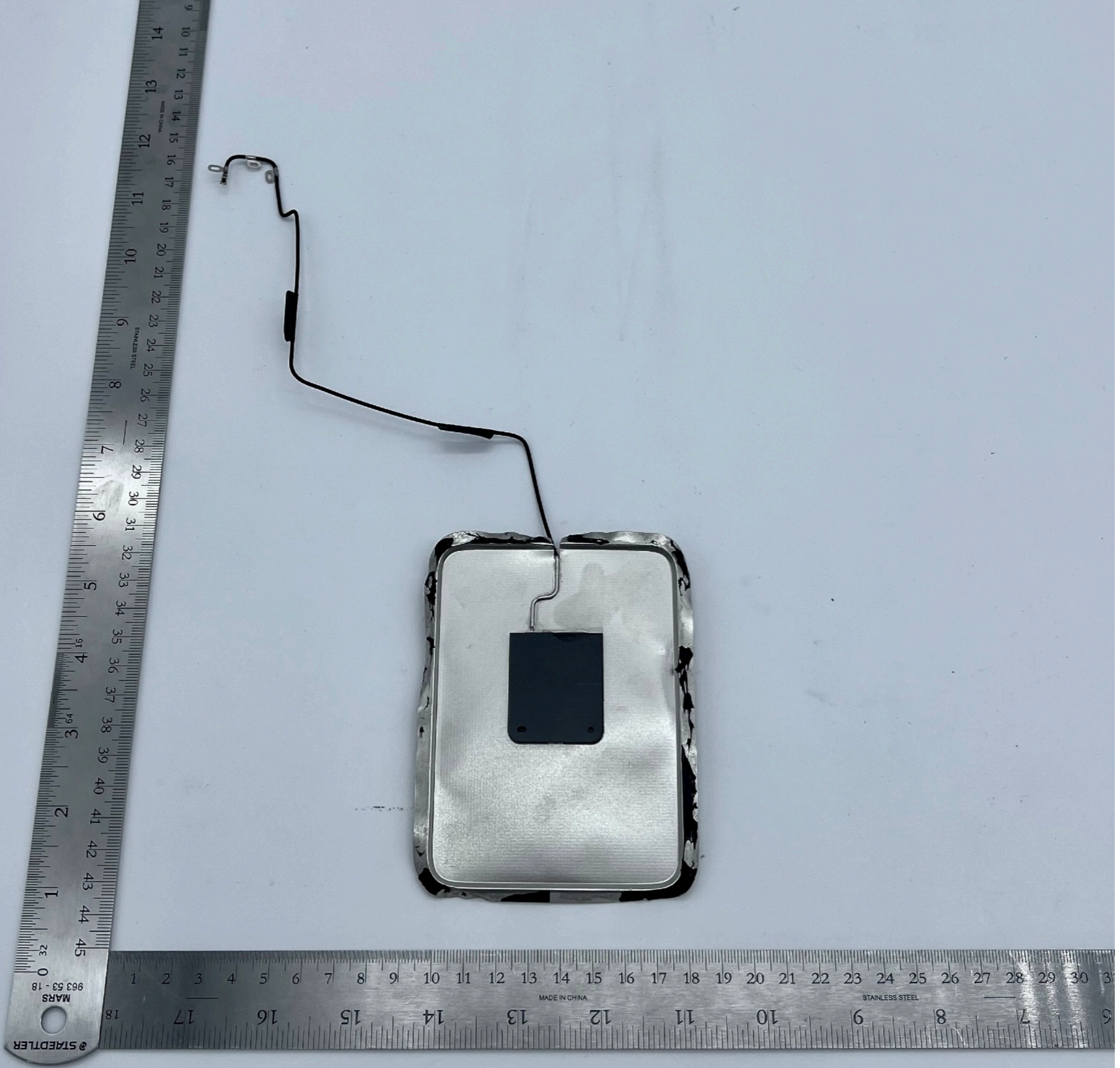
A2873 Antenna WF2 - Back
