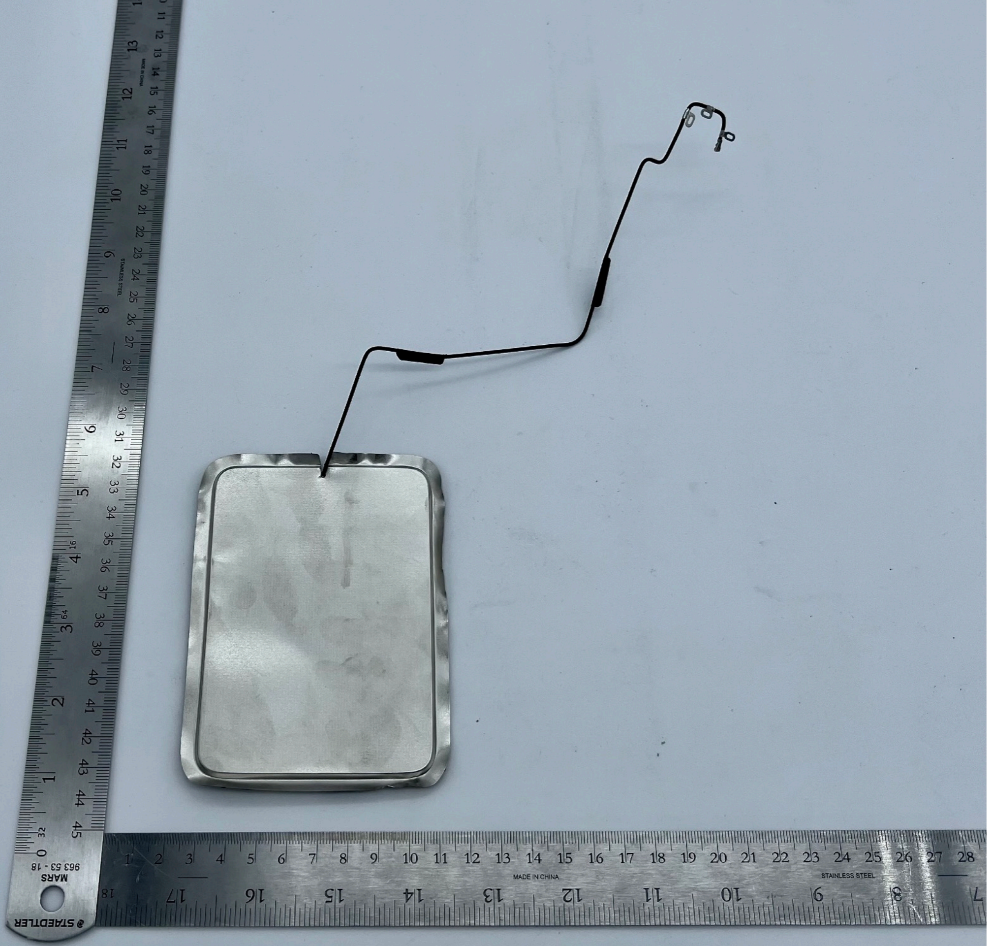
A2873 Antenna WF2 - Front
