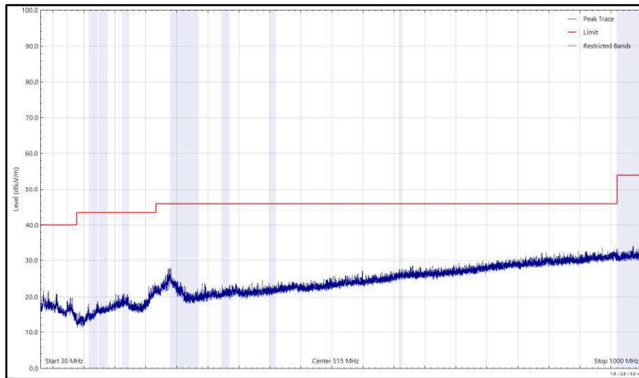
Figure 524 - U-NII-3 - 5825 MHz (CH165), VHT20, CDD, Core 0 + Core 1, 30 MHz to 1 GHz, Horizontal (Peak)
