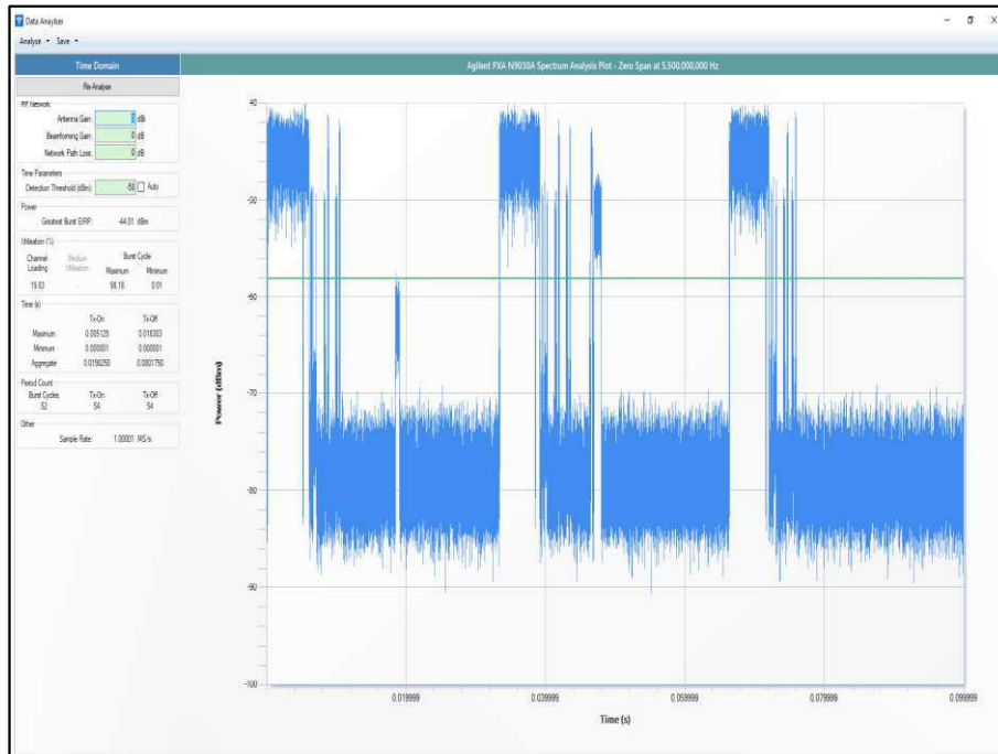
Figure 536 - Channel Loading
