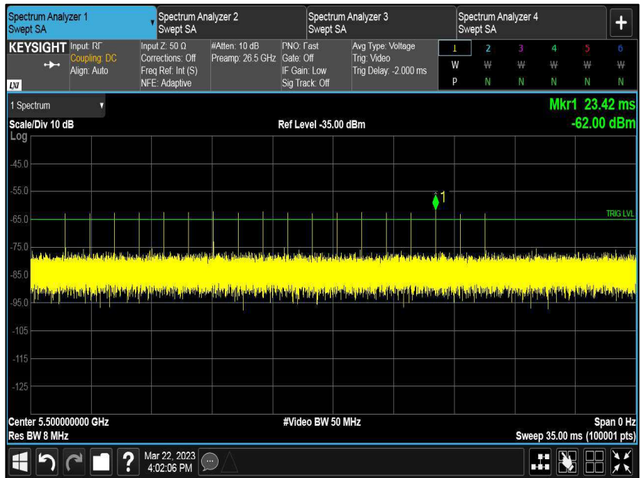
Figure 529 - Verification of Radar Type 0
