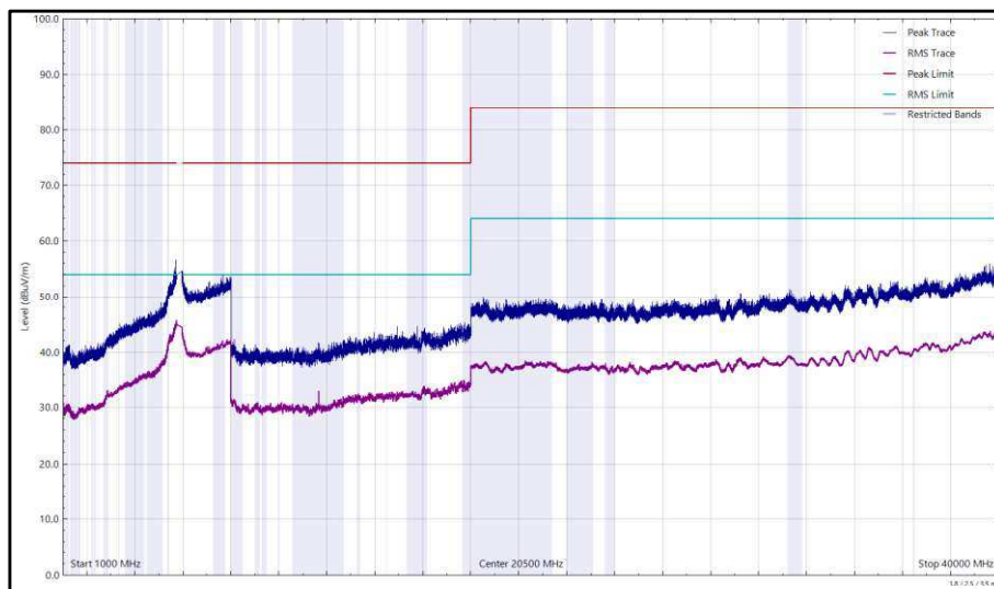
Figure 525 - U-NII-3 - 5825 MHz (CH165), VHT20, CDD, Core 0 + Core 1, 1 GHz to 40 GHz, Horizontal
