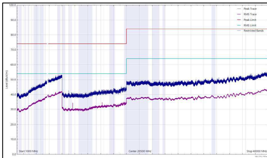
Figure 523 - U-NII-3 - 5745 MHz (CH149), VHT20, CDD, Core 0 + Core 1, 1 GHz to 40 GHz, Vertical
