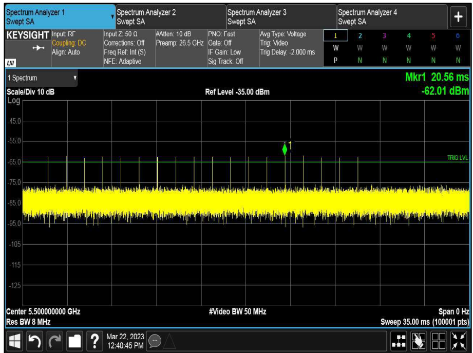
Figure 535 - Verification of Radar Type 0
