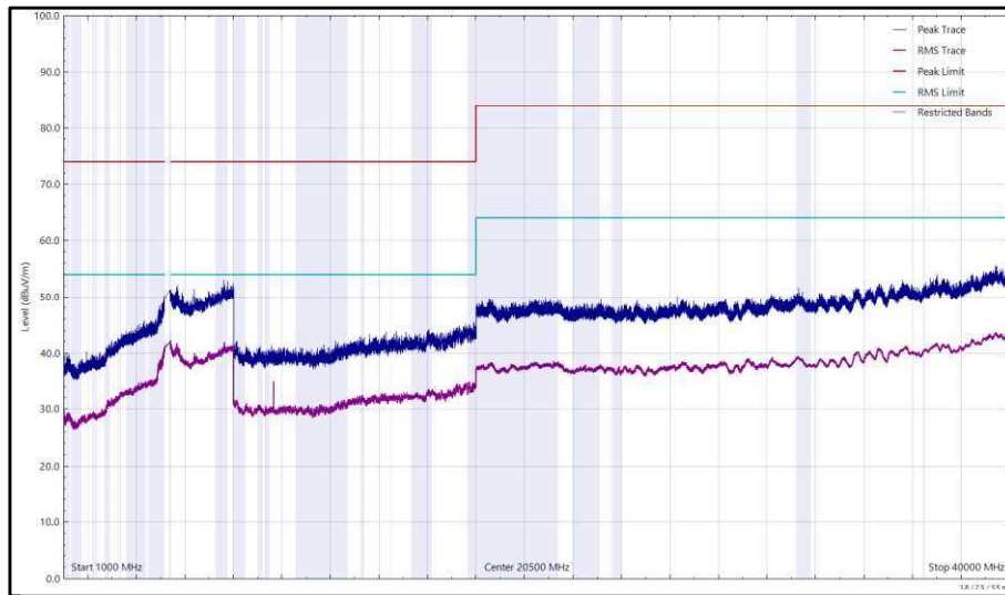
Figure 517 - U-NII-2A - 5320 MHz (CH64), VHT20, CDD, Core 0 + Core 1, 1 GHz to 40 GHz, Vertical
