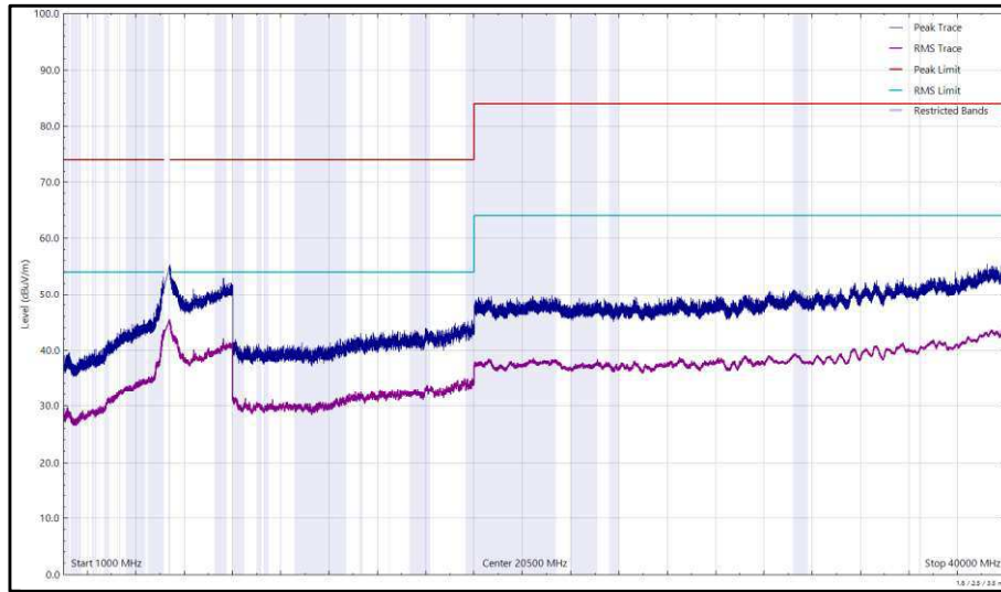
Figure 516 - U-NII-2A - 5320 MHz (CH64), VHT20, CDD, Core 0 + Core 1, 1 GHz to 40 GHz, Horizontal
