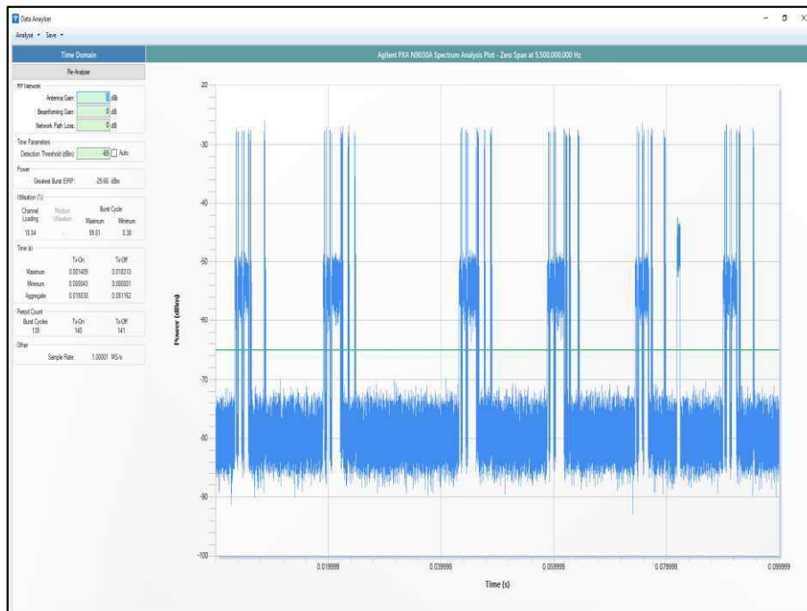
Figure 530 - Channel Loading
