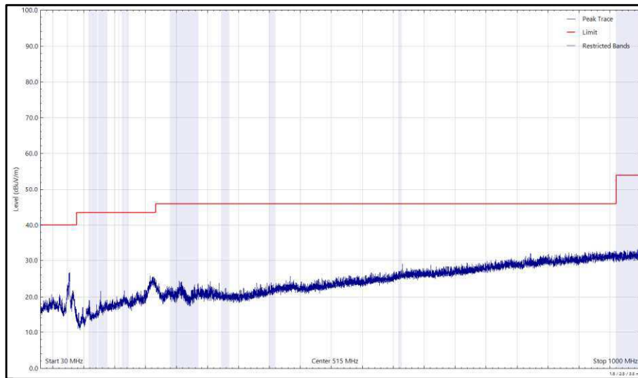
Figure 117 - 2437 MHz (CH6), 802.11g, Core 1, 30 MHz to 1 GHz, Horizontal (Peak)
