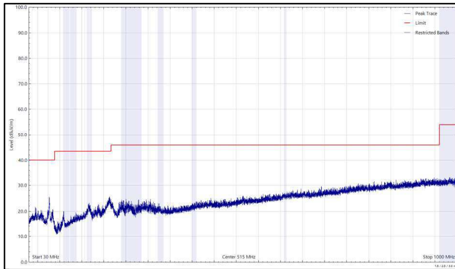
Figure 109 - 2437 MHz (CH6), 802.11g, Core 0, 30 MHz to 1 GHz, Horizontal (Peak)
