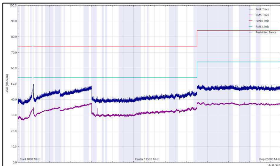
Figure 110 - 2437 MHz (CH6), 802.11g, Core 0, 1 GHz to 26 GHz, Horizontal
