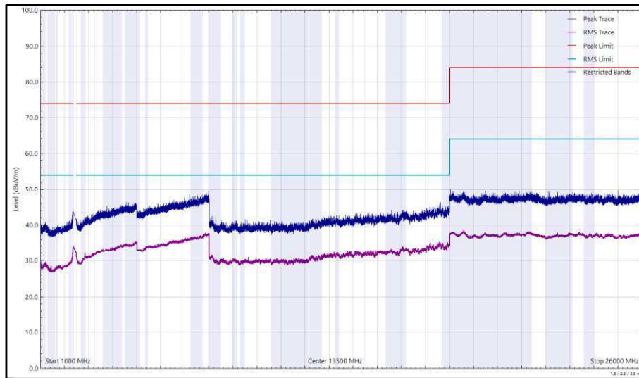
Figure 115 - 2412 MHz (CH1), 802.11g, Core 1, 1 GHz to 26 GHz, Horizontal
