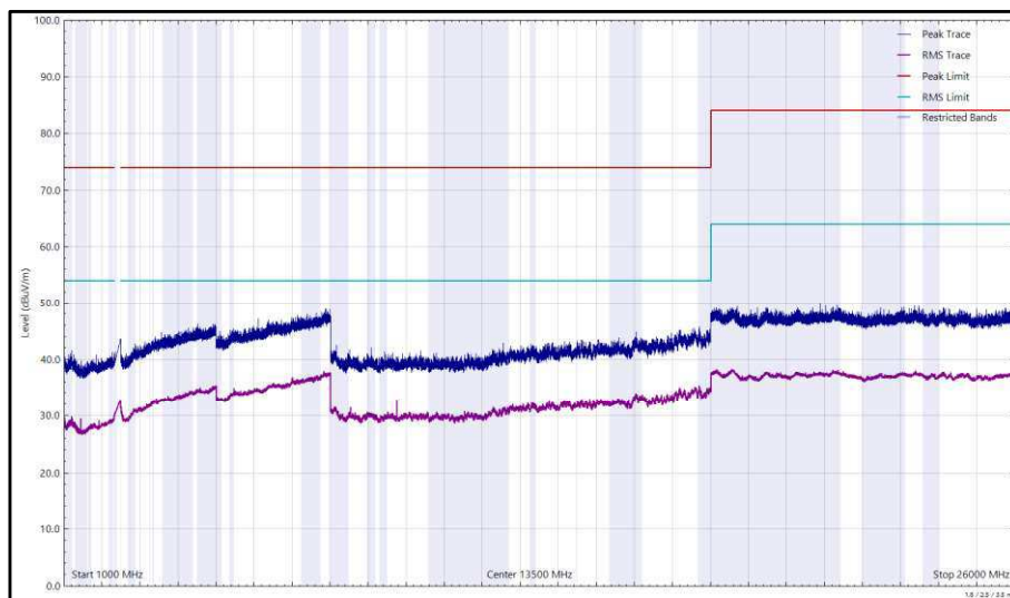
Figure 120 - 2437 MHz (CH6), 802.11g, Core 1, 1 GHz to 26 GHz, Vertical
