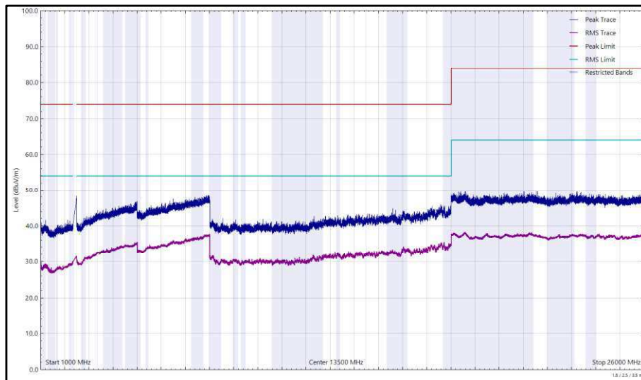
Figure 102 - 2437 MHz (CH6), 802.11b, Core 1, 1 GHz to 26 GHz, Horizontal
