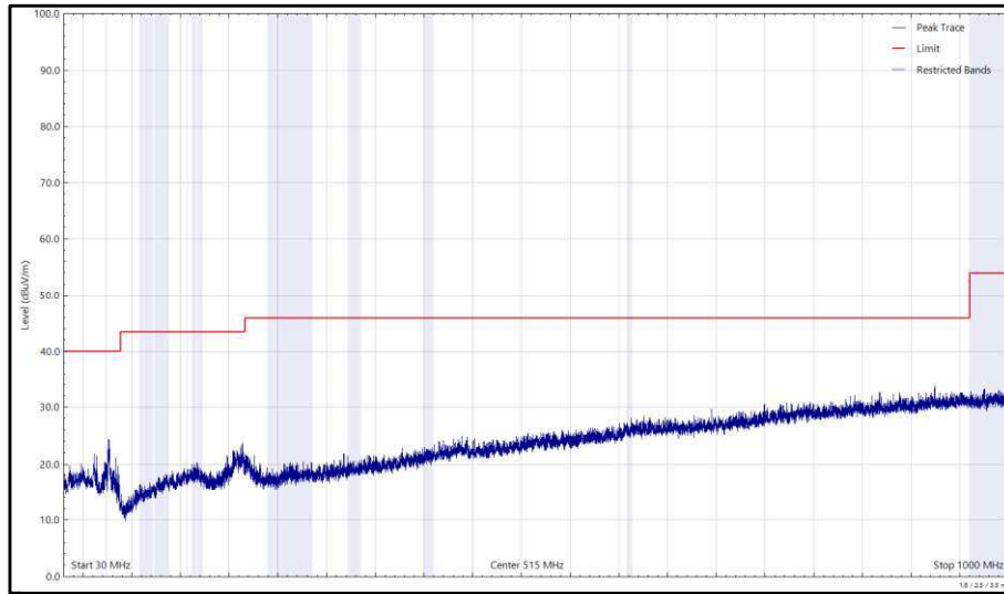
Figure 125 - 2437 MHz (CH6), HT20, CDD, Core 0 + Core 1, 30 MHz to 1 GHz, Horizontal (Peak)
