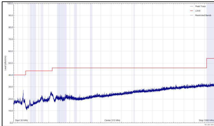
Figure 101 - 2437 MHz (CH6), 802.11b, Core 1, 30 MHz to 1 GHz, Horizontal (Peak)
