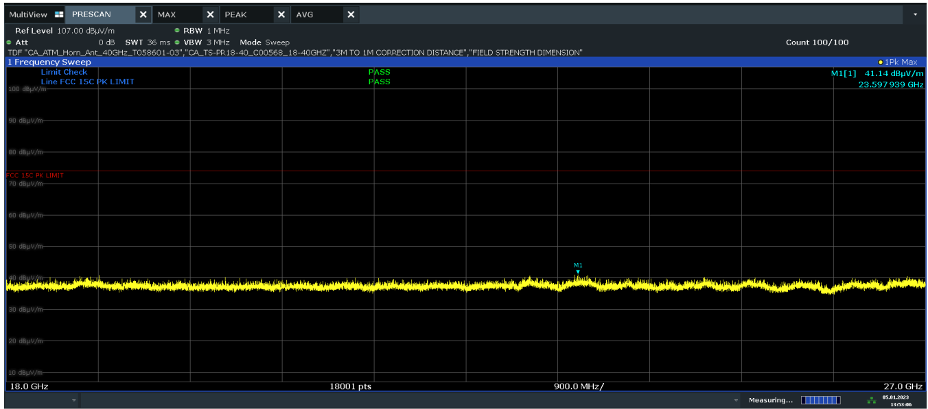
Plot 7-26. Radiated Spurious Emissions Above 18GHz H Polarity (1Mbps – Ch. 19)
