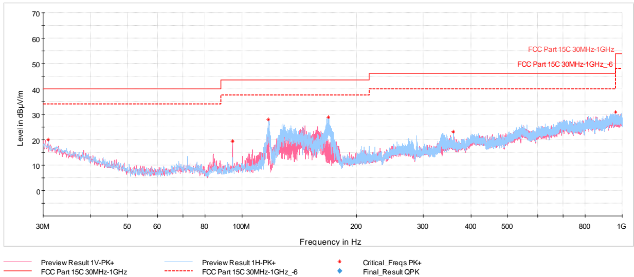
Plot 7-32. Radiated Spurious Emissions Below 1GHz (1Mbps – Ch.19, Pol. H & V, with Laptop)
