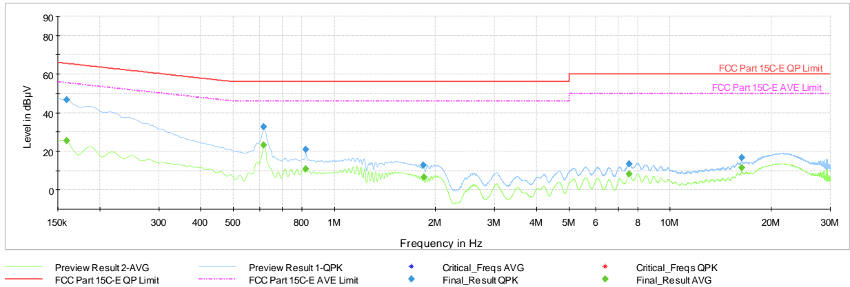
Plot 7-34. AC Line Conducted Plot with Bluetooth LE (N, 1Mbps – Ch.0, with Laptop)
