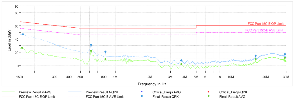
Plot 7-33. AC Line Conducted Plot with Bluetooth LE (L1, 1Mbps – Ch.0 with Laptop)
