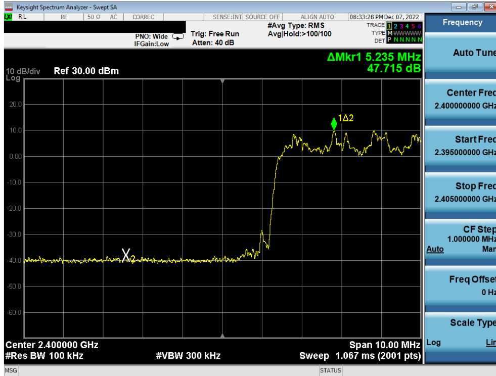
Plot 7-13. Band Edge Plot (Bluetooth with Hopping Enabled, 8DPSK, 2.4GHz)
