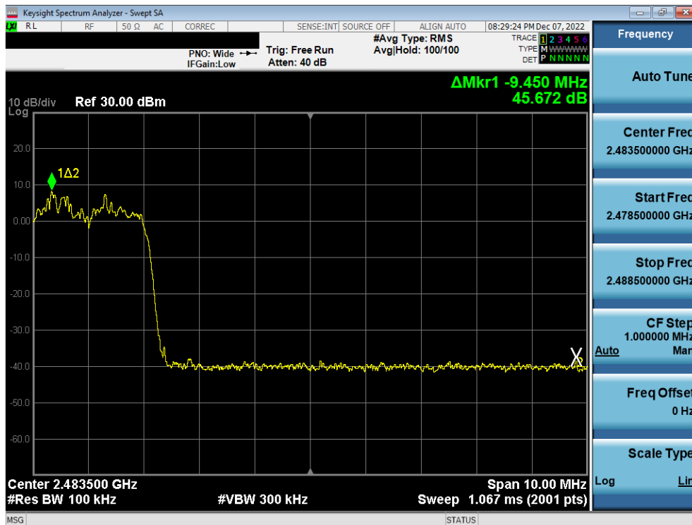
Plot 7-14. Band Edge Plot (Bluetooth with Hopping Enabled, 8DPSK, 2.4GHz)
