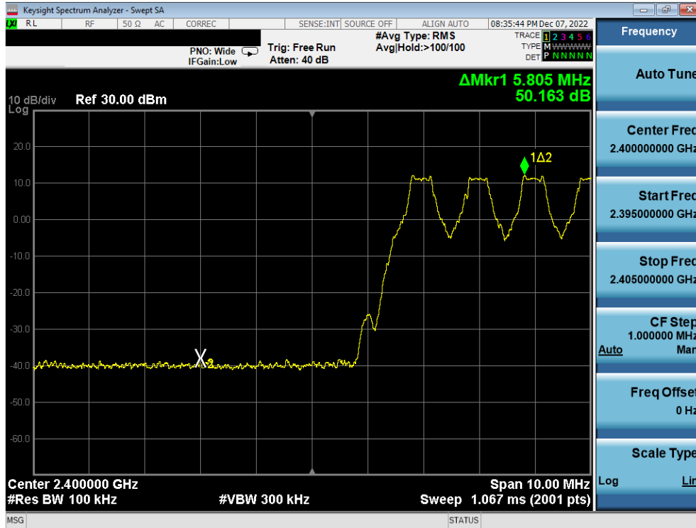
Plot 7-9. Band Edge Plot (Bluetooth with Hopping Enabled, GFSK, 2.4GHz)
